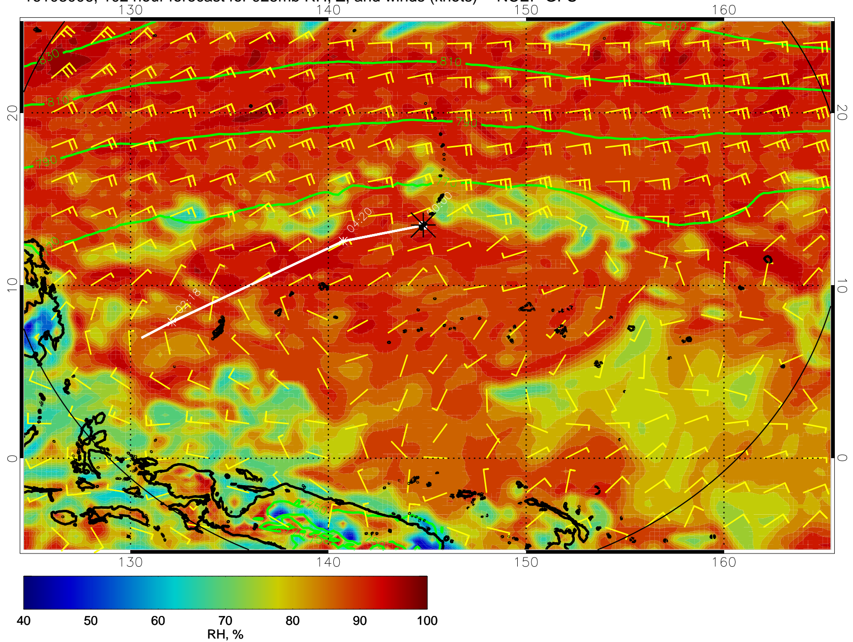
16103006, 102 hour forecast for 925mb RH, Z, and winds (knots) -- NCEP GFS
