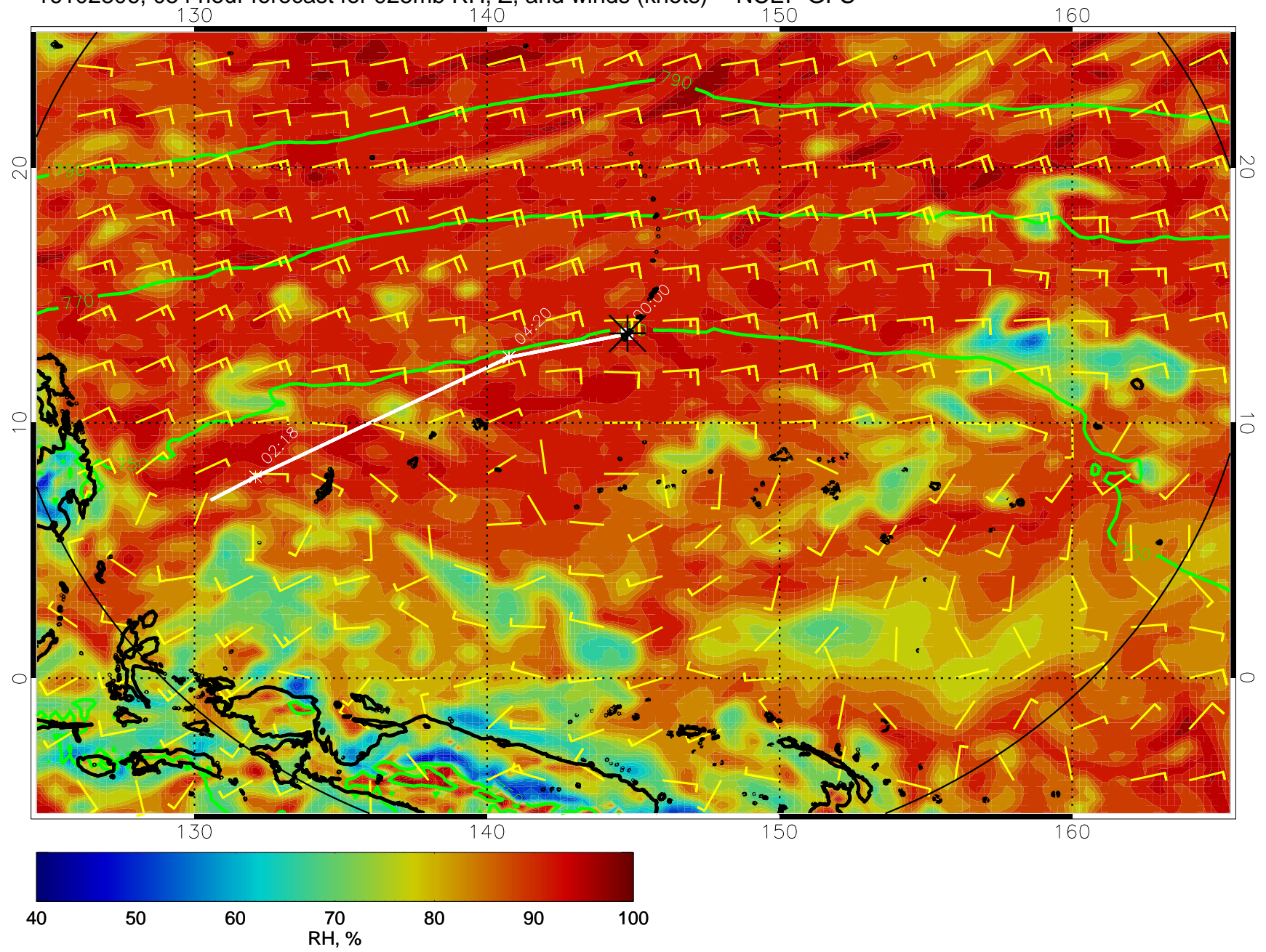
16102806, 054 hour forecast for 925mb RH, Z, and winds (knots) -- NCEP GFS
