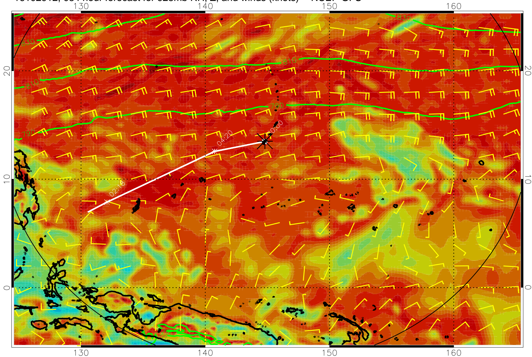
16102912, 084 hour forecast for 925mb RH, Z, and winds (knots) -- NCEP GFS
