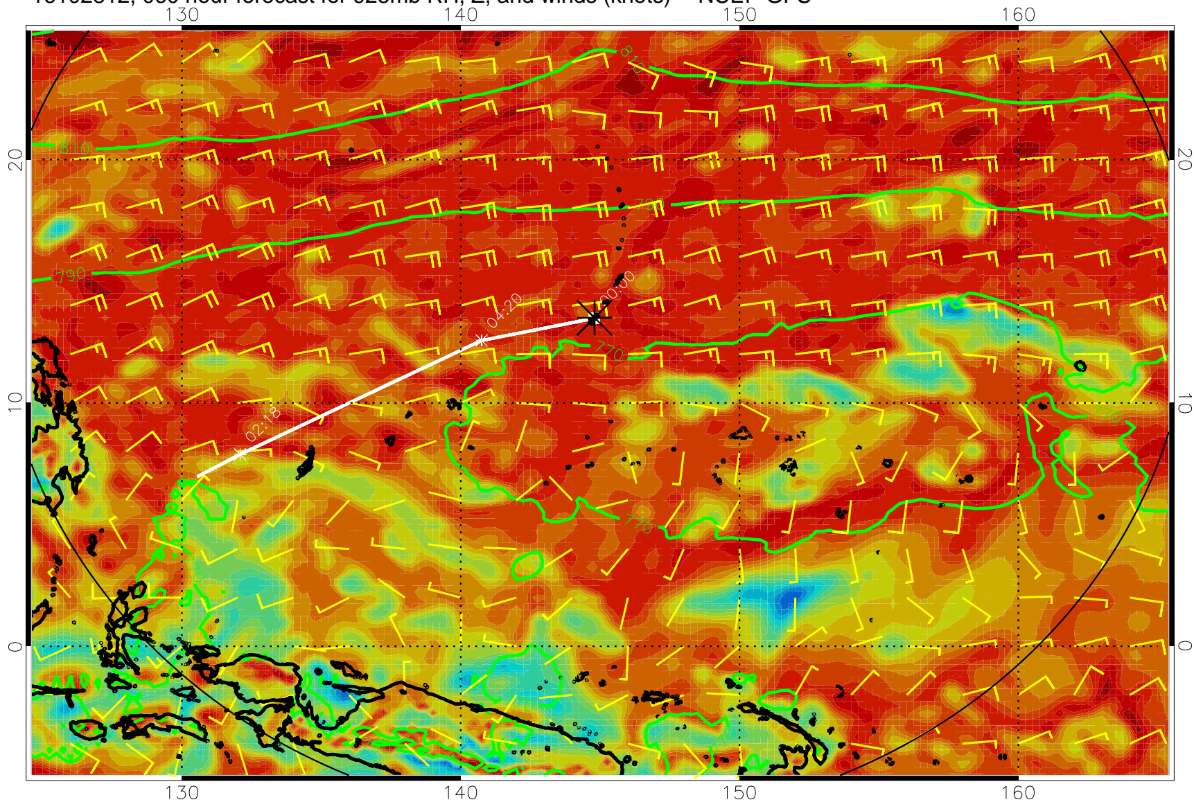
16102812, 060 hour forecast for 925mb RH, Z, and winds (knots) -- NCEP GFS
