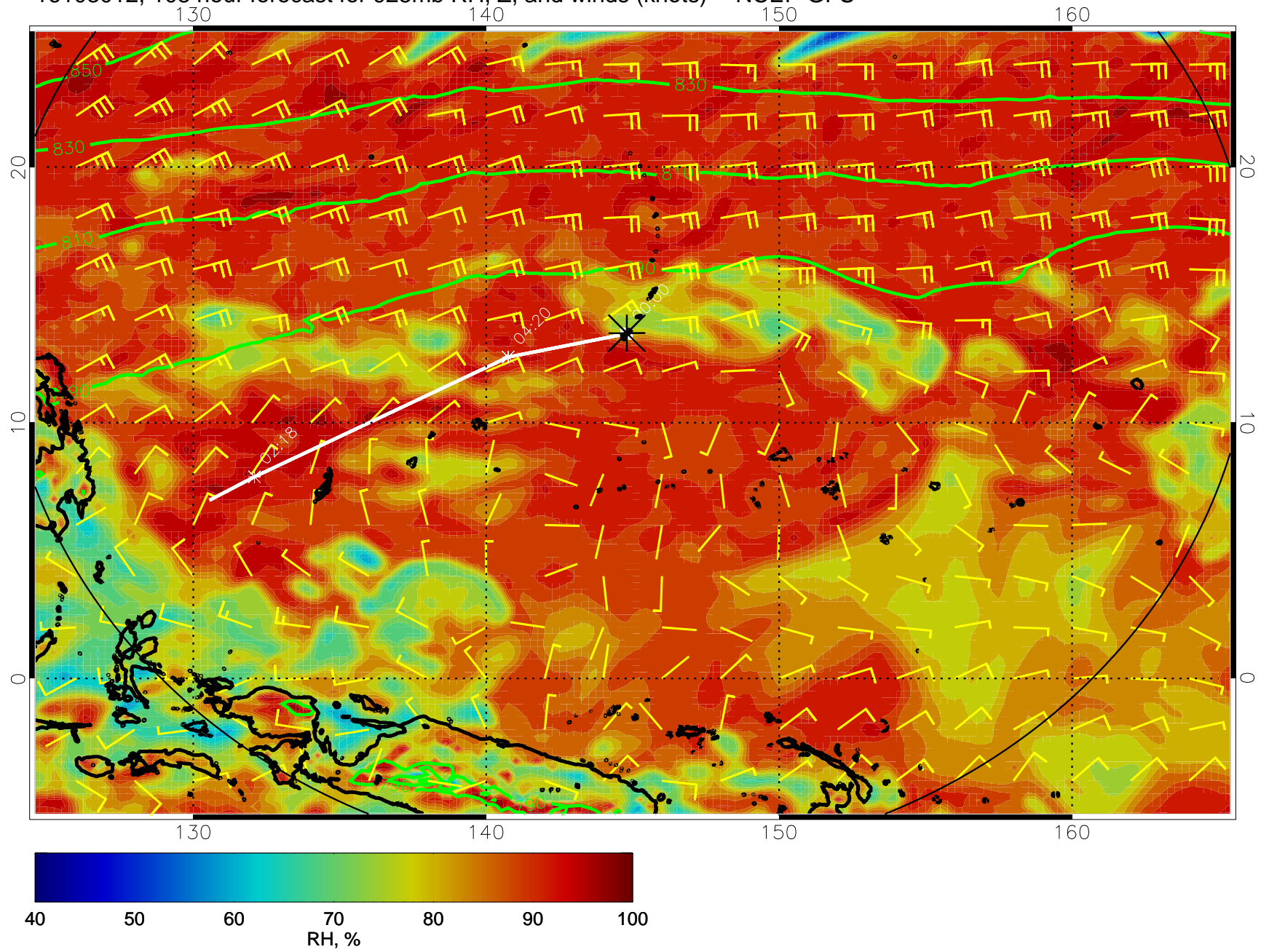
16103012, 108 hour forecast for 925mb RH, Z, and winds (knots) -- NCEP GFS
