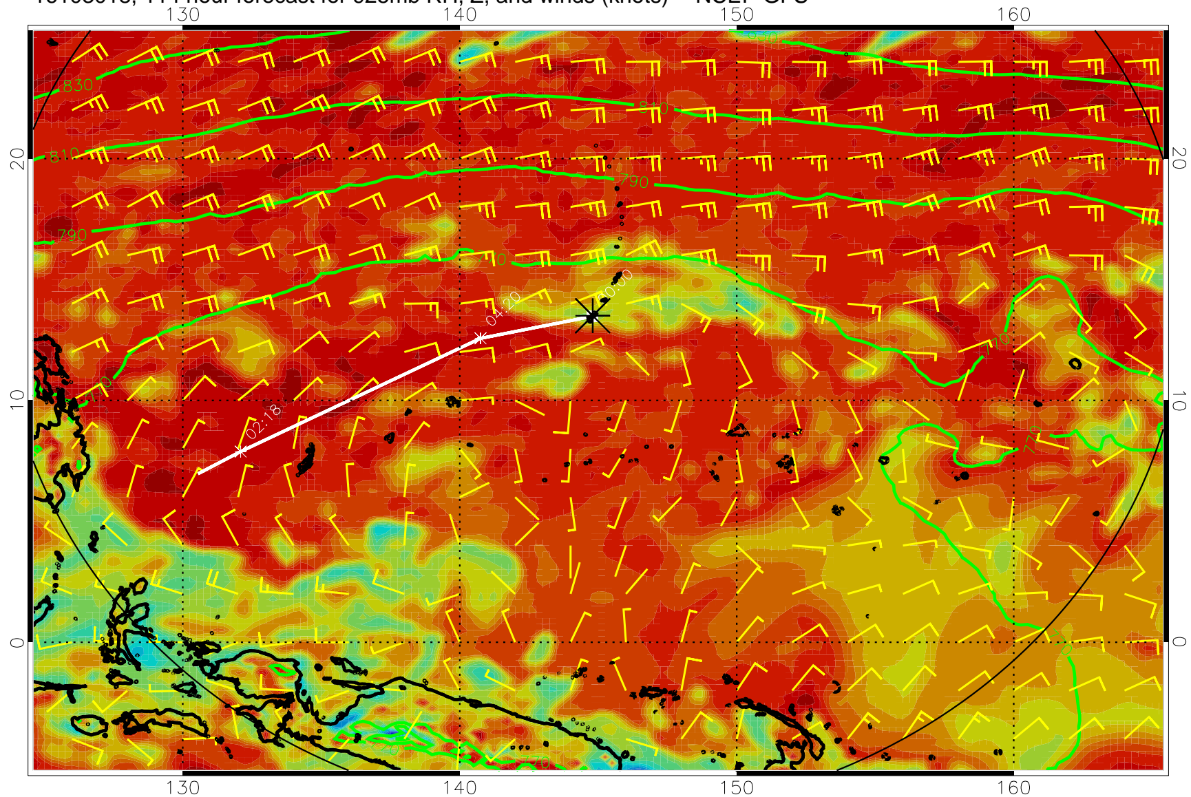
16103018, 114 hour forecast for 925mb RH, Z, and winds (knots) -- NCEP GFS
