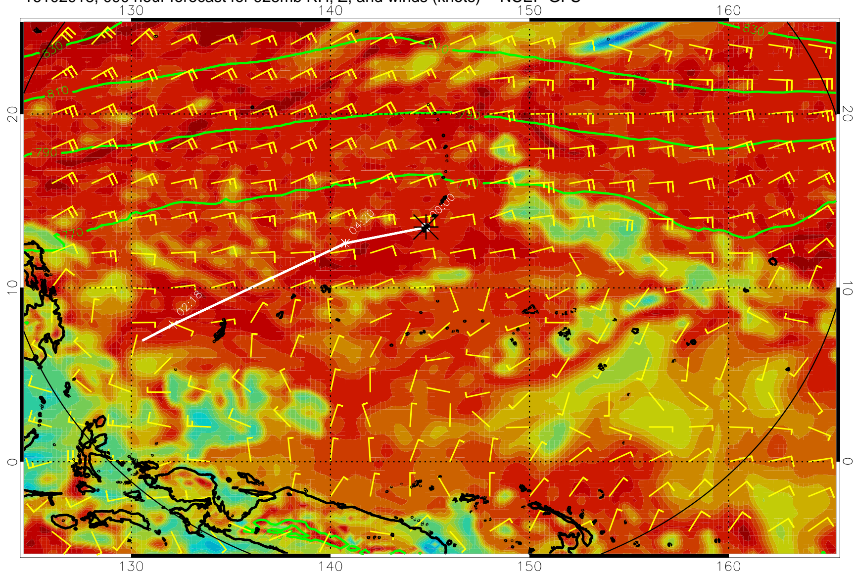
16102918, 090 hour forecast for 925mb RH, Z, and winds (knots) -- NCEP GFS
