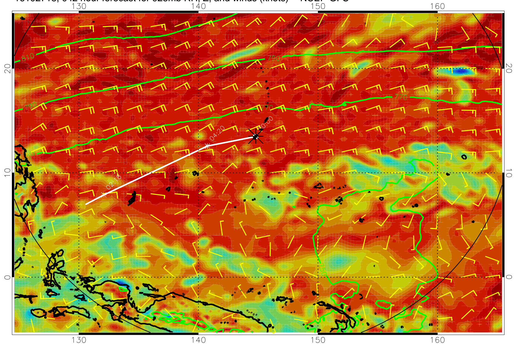
16102718, 042 hour forecast for 925mb RH, Z, and winds (knots) -- NCEP GFS
