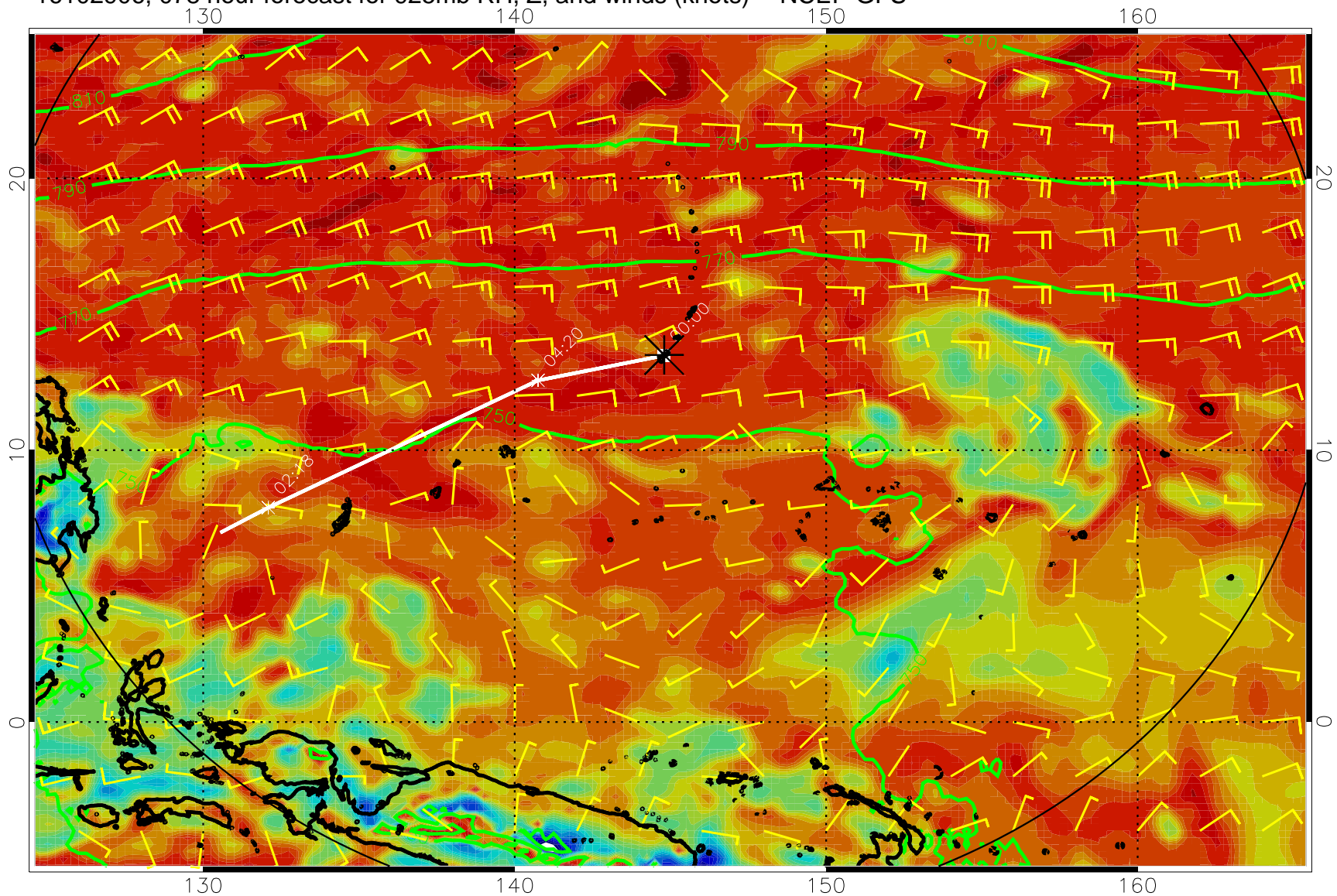
16102906, 078 hour forecast for 925mb RH, Z, and winds (knots) -- NCEP GFS
