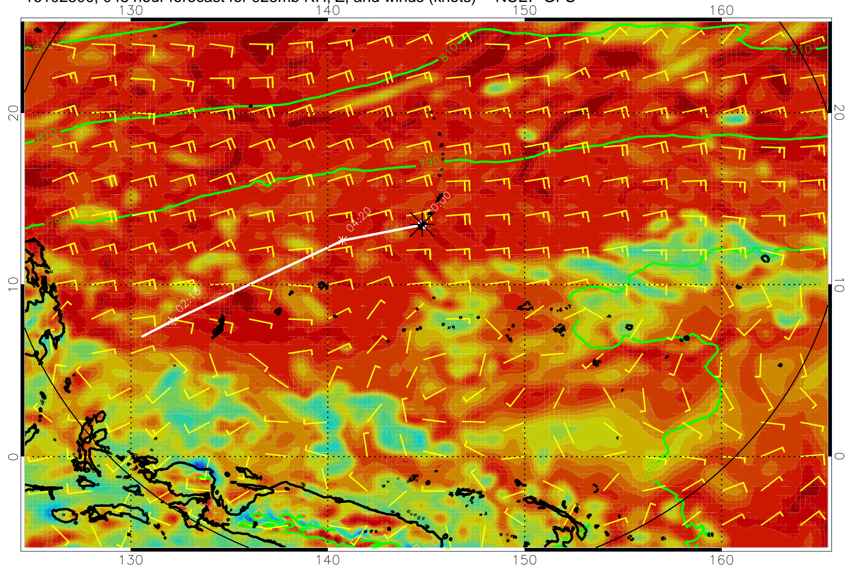
16102800, 048 hour forecast for 925mb RH, Z, and winds (knots) -- NCEP GFS
