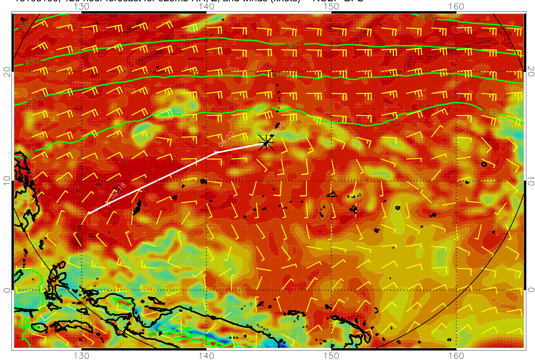
16103100, 120 hour forecast for 925mb RH, Z, and winds (knots) -- NCEP GFS
