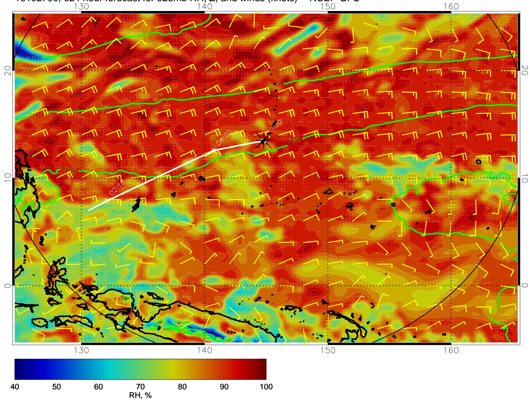
16102700, 024 hour forecast for 925mb RH, Z, and winds (knots) -- NCEP GFS
