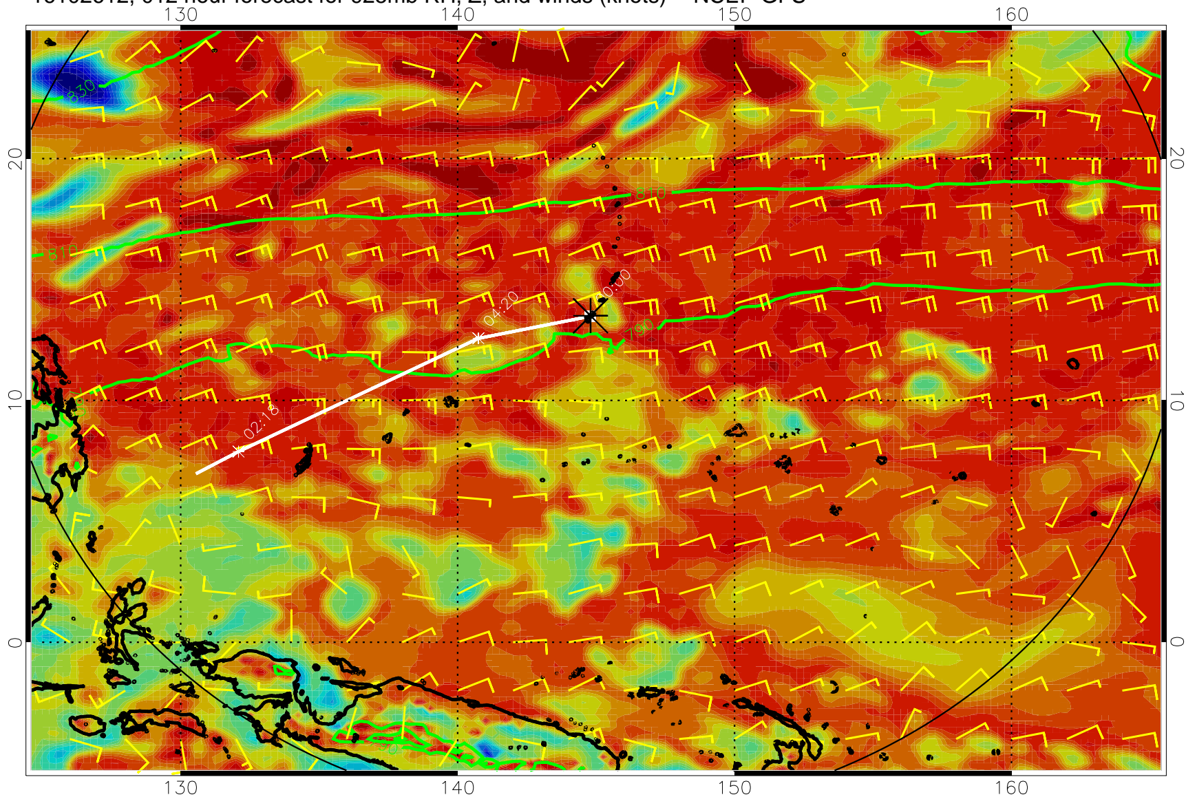
16102612, 012 hour forecast for 925mb RH, Z, and winds (knots) -- NCEP GFS
