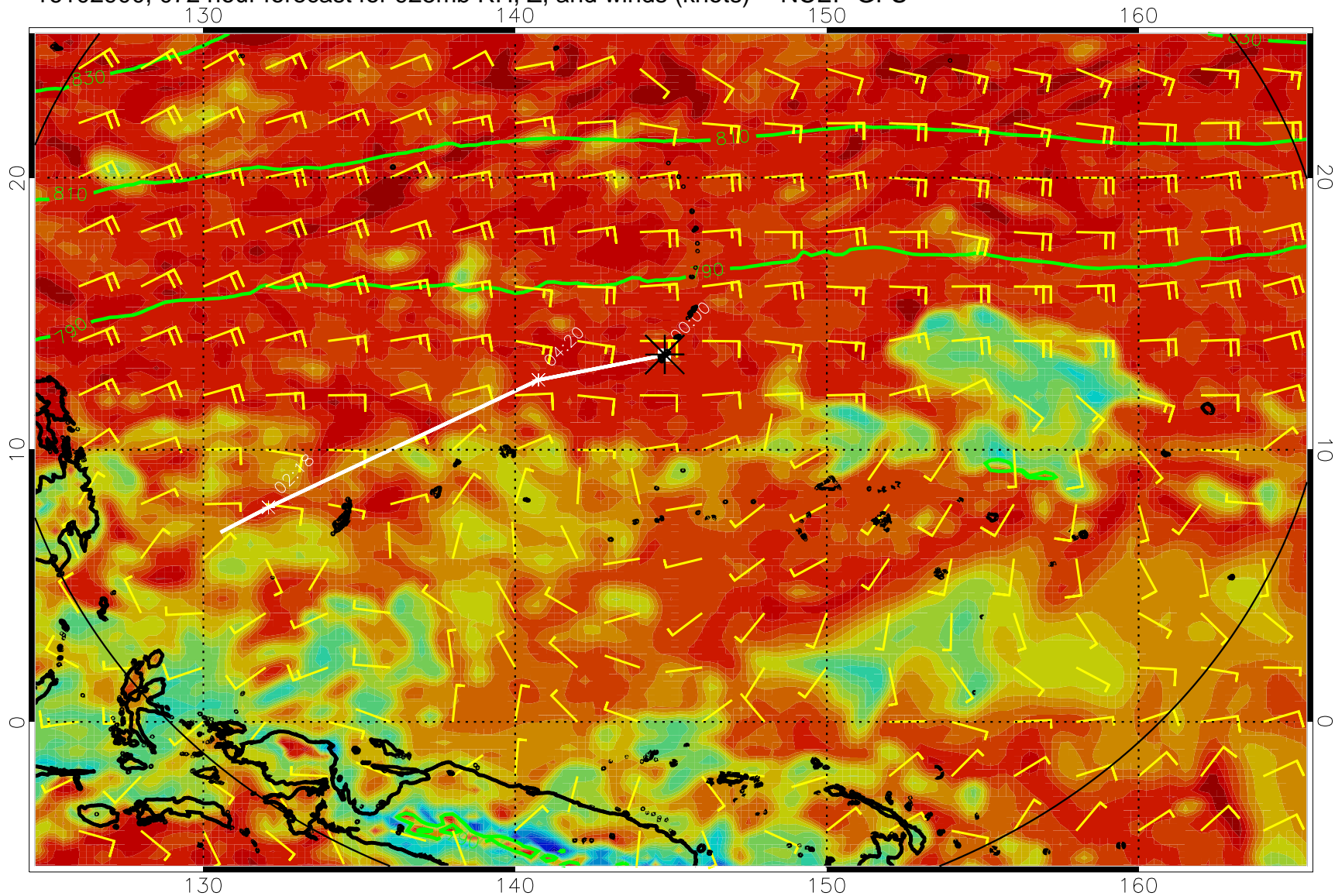
16102900, 072 hour forecast for 925mb RH, Z, and winds (knots) -- NCEP GFS
