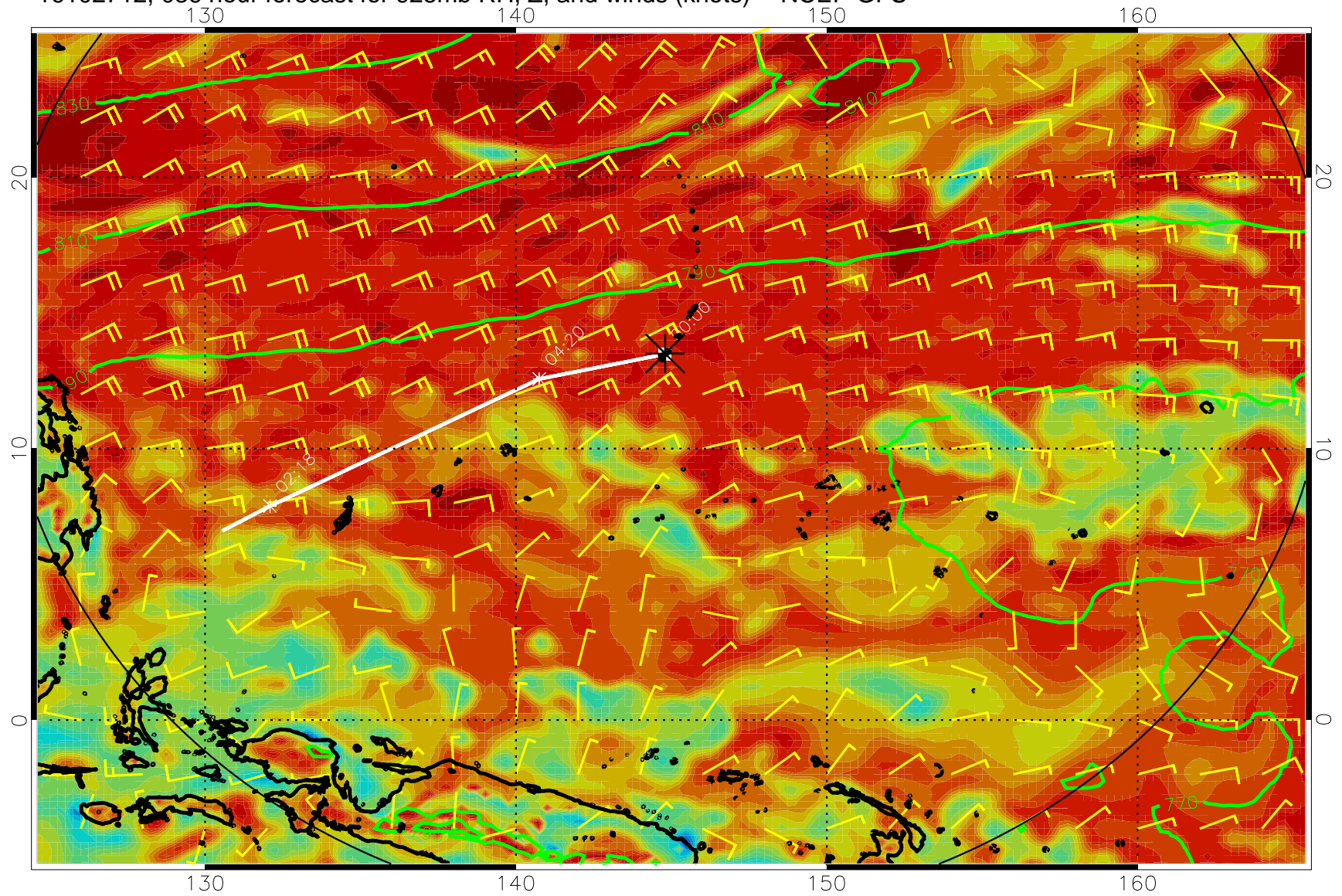
16102712, 036 hour forecast for 925mb RH, Z, and winds (knots) -- NCEP GFS
