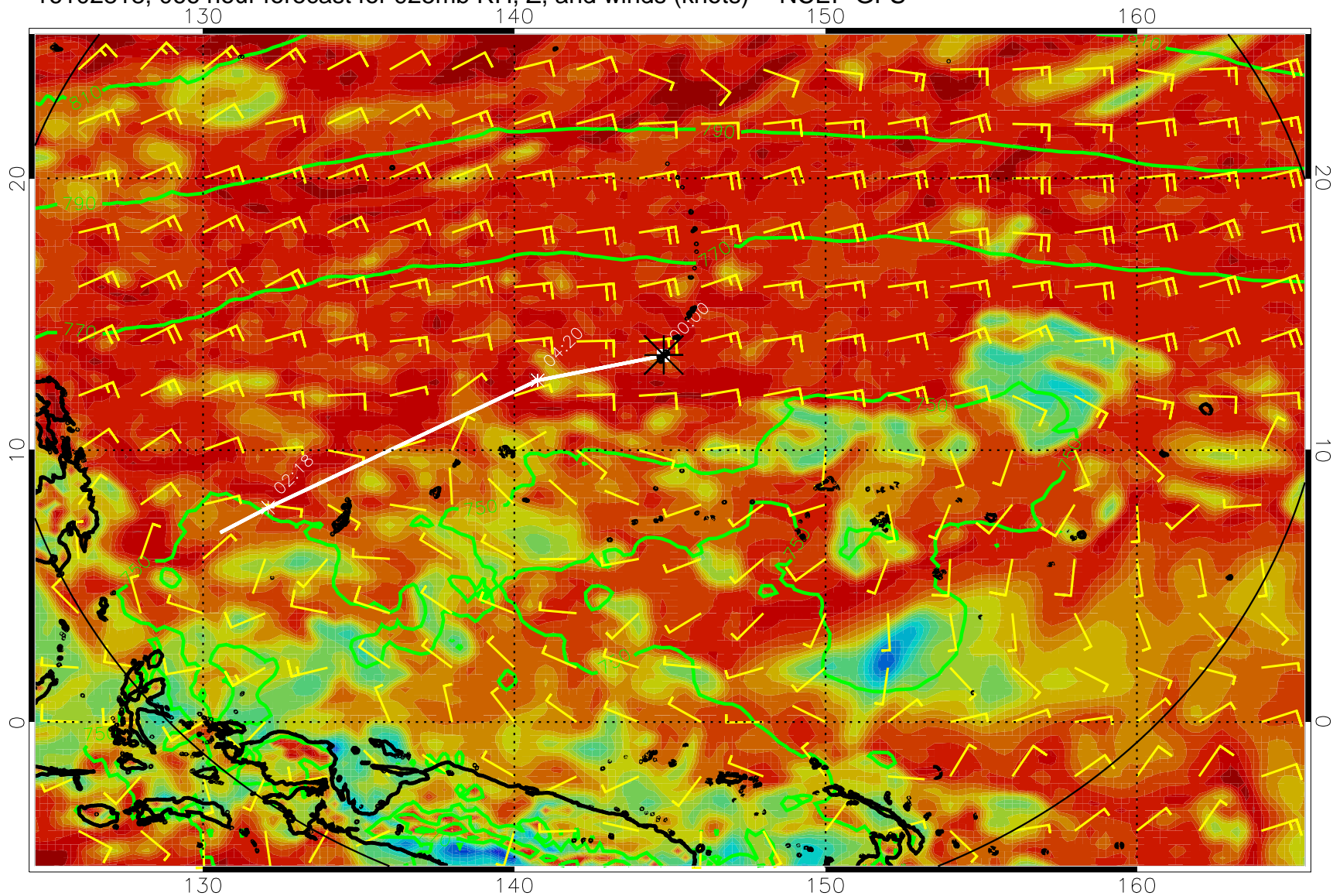
16102818, 066 hour forecast for 925mb RH, Z, and winds (knots) -- NCEP GFS
