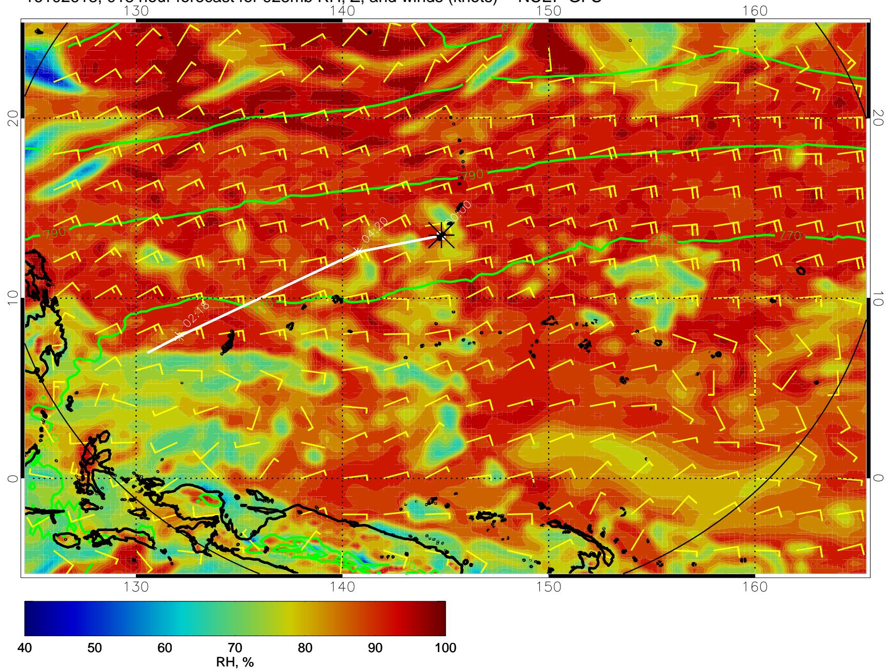
16102618, 018 hour forecast for 925mb RH, Z, and winds (knots) -- NCEP GFS
