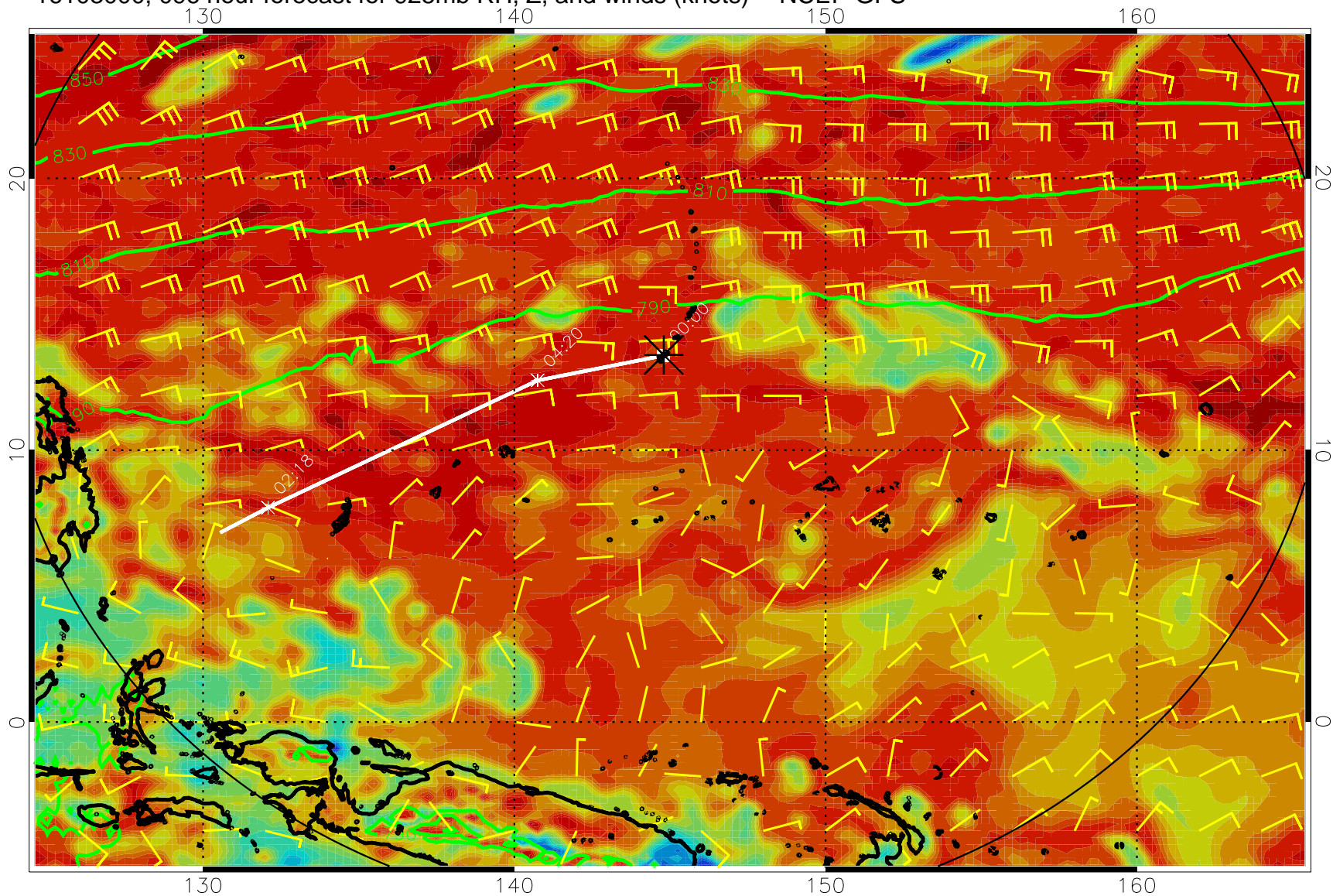
16103000, 096 hour forecast for 925mb RH, Z, and winds (knots) -- NCEP GFS
