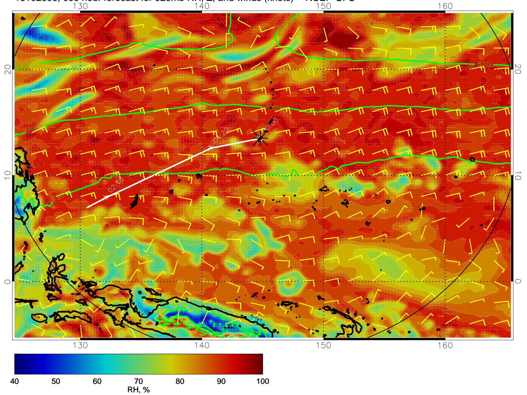
16102606, 006 hour forecast for 925mb RH, Z, and winds (knots) -- NCEP GFS
