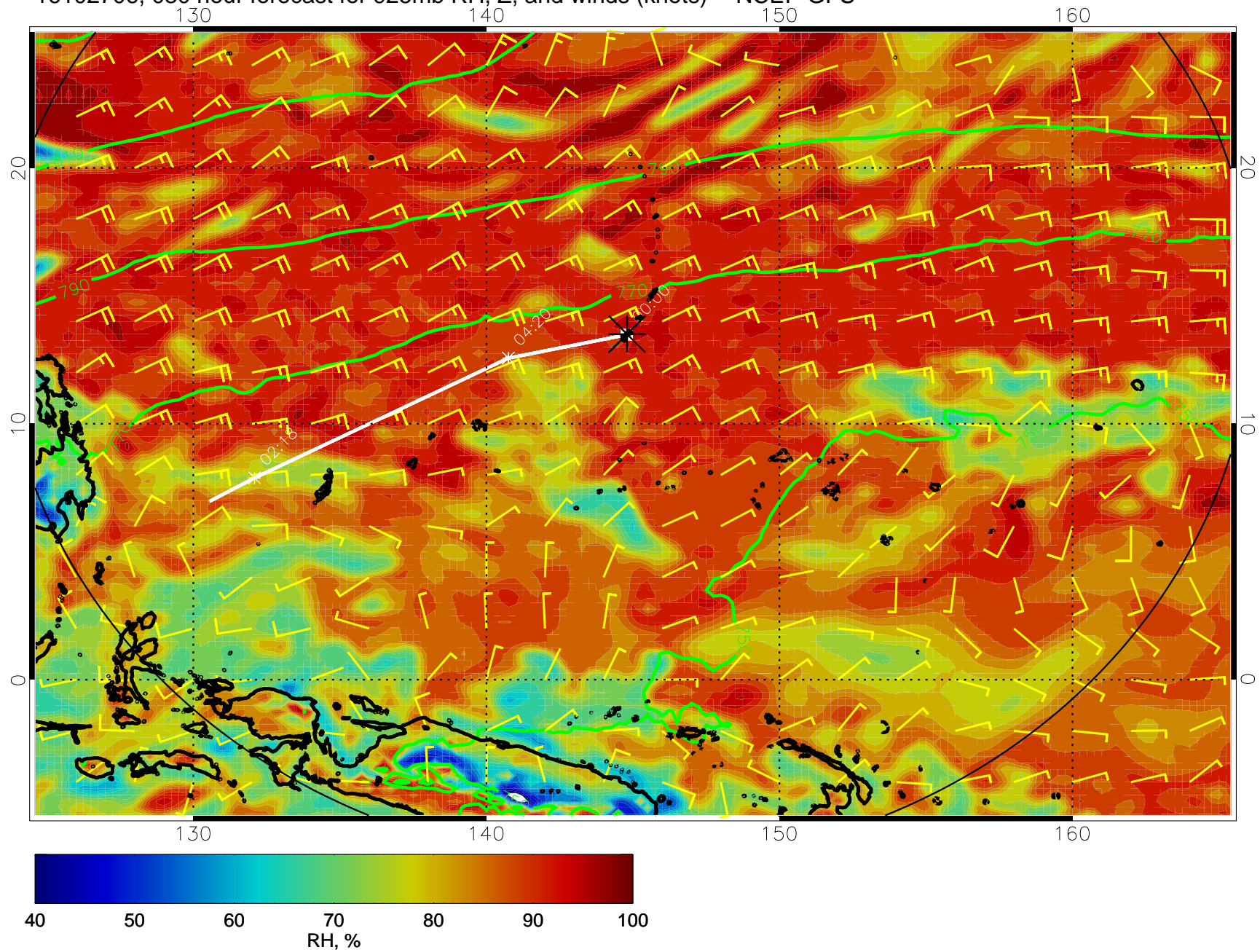
16102706, 030 hour forecast for 925mb RH, Z, and winds (knots) -- NCEP GFS
