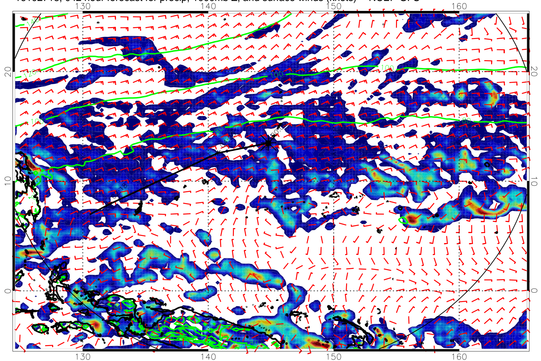
16102718, 042 hour forecast for precip, 1000mb Z, and surface winds (knots) -- NCEP GFS
