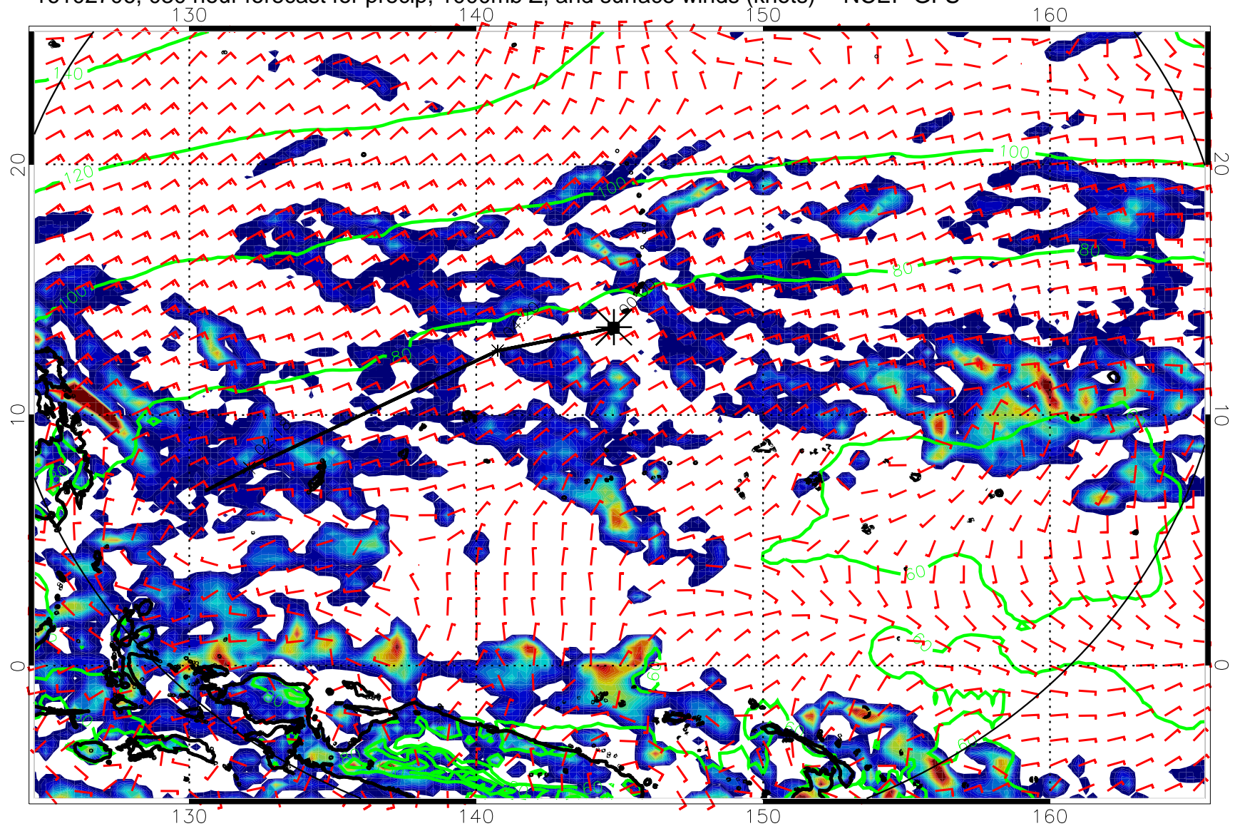
16102706, 030 hour forecast for precip, 1000mb Z, and surface winds (knots) -- NCEP GFS
