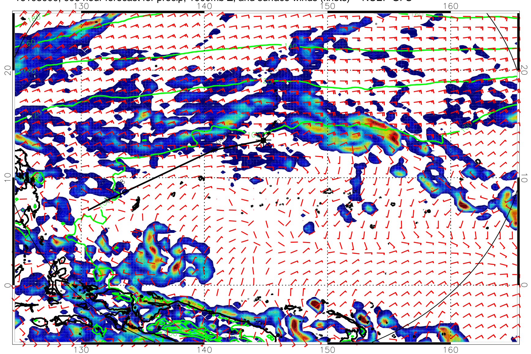
16103000, 096 hour forecast for precip, 1000mb Z, and surface winds (knots) -- NCEP GFS
