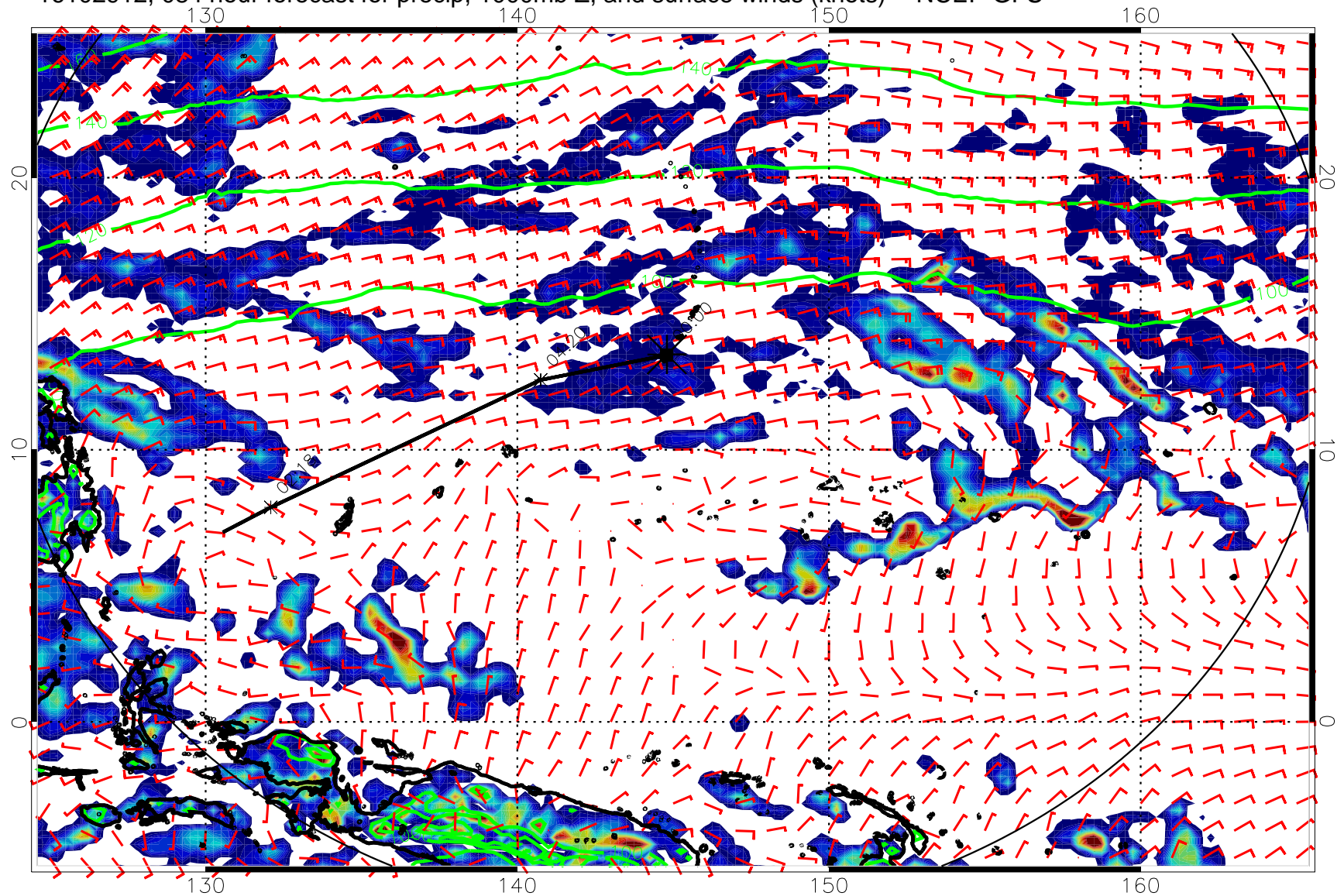
16102912, 084 hour forecast for precip, 1000mb Z, and surface winds (knots) -- NCEP GFS
