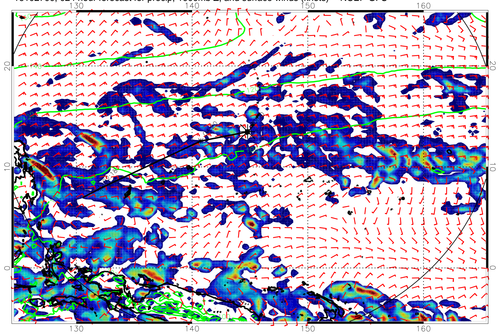
16102700, 024 hour forecast for precip, 1000mb Z, and surface winds (knots) -- NCEP GFS
