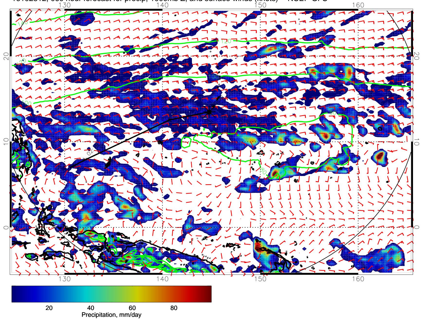
16102812, 060 hour forecast for precip, 1000mb Z, and surface winds (knots) -- NCEP GFS
