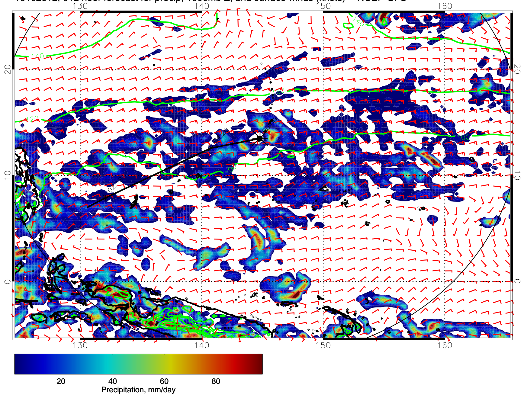
16102612, 012 hour forecast for precip, 1000mb Z, and surface winds (knots) -- NCEP GFS
