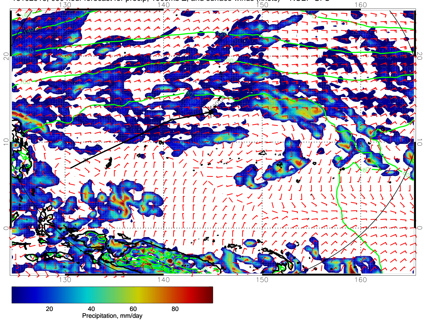
16102918, 090 hour forecast for precip, 1000mb Z, and surface winds (knots) -- NCEP GFS
