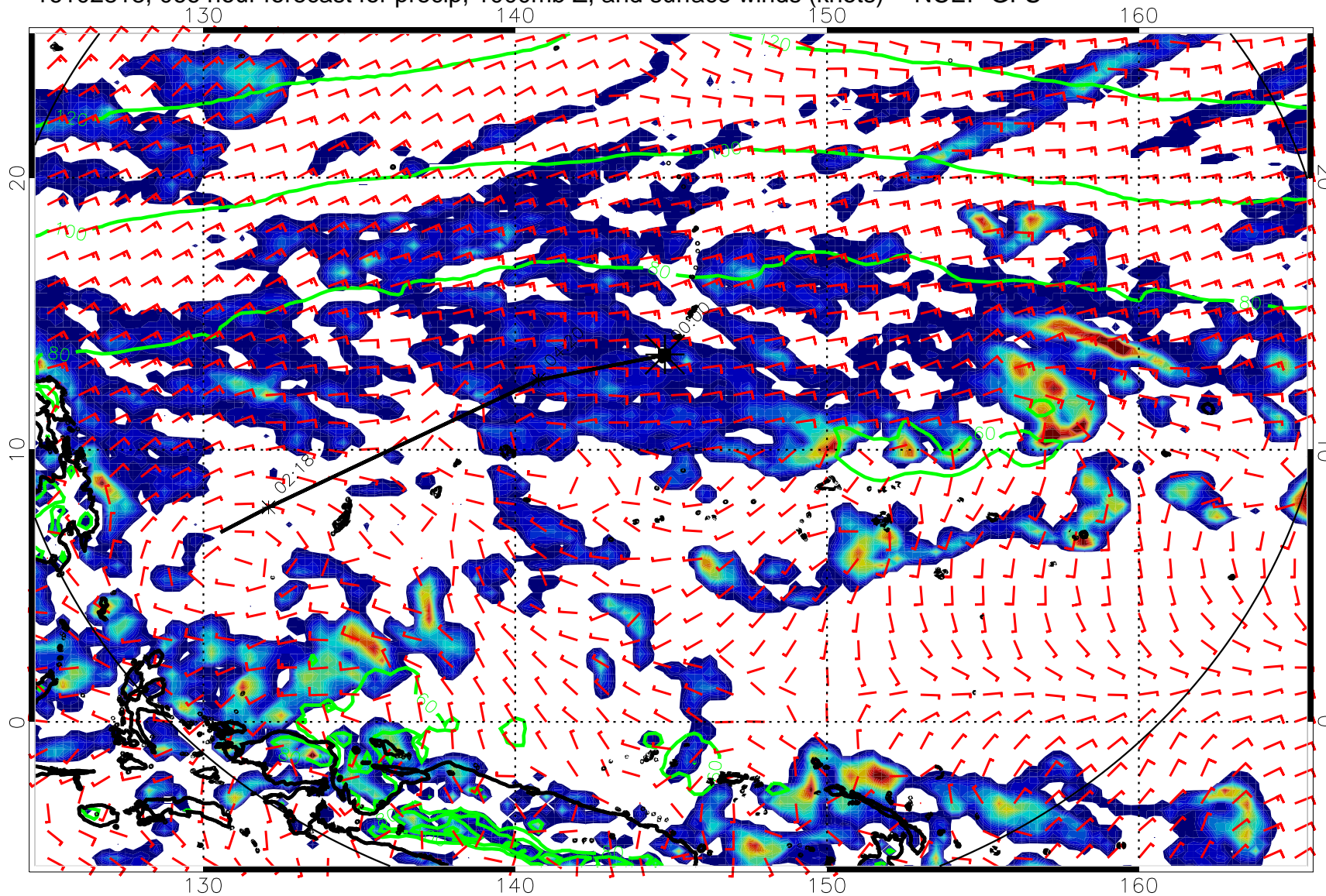
16102818, 066 hour forecast for precip, 1000mb Z, and surface winds (knots) -- NCEP GFS
