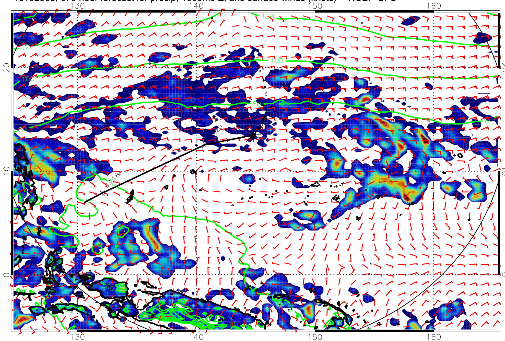
16102906, 078 hour forecast for precip, 1000mb Z, and surface winds (knots) -- NCEP GFS
