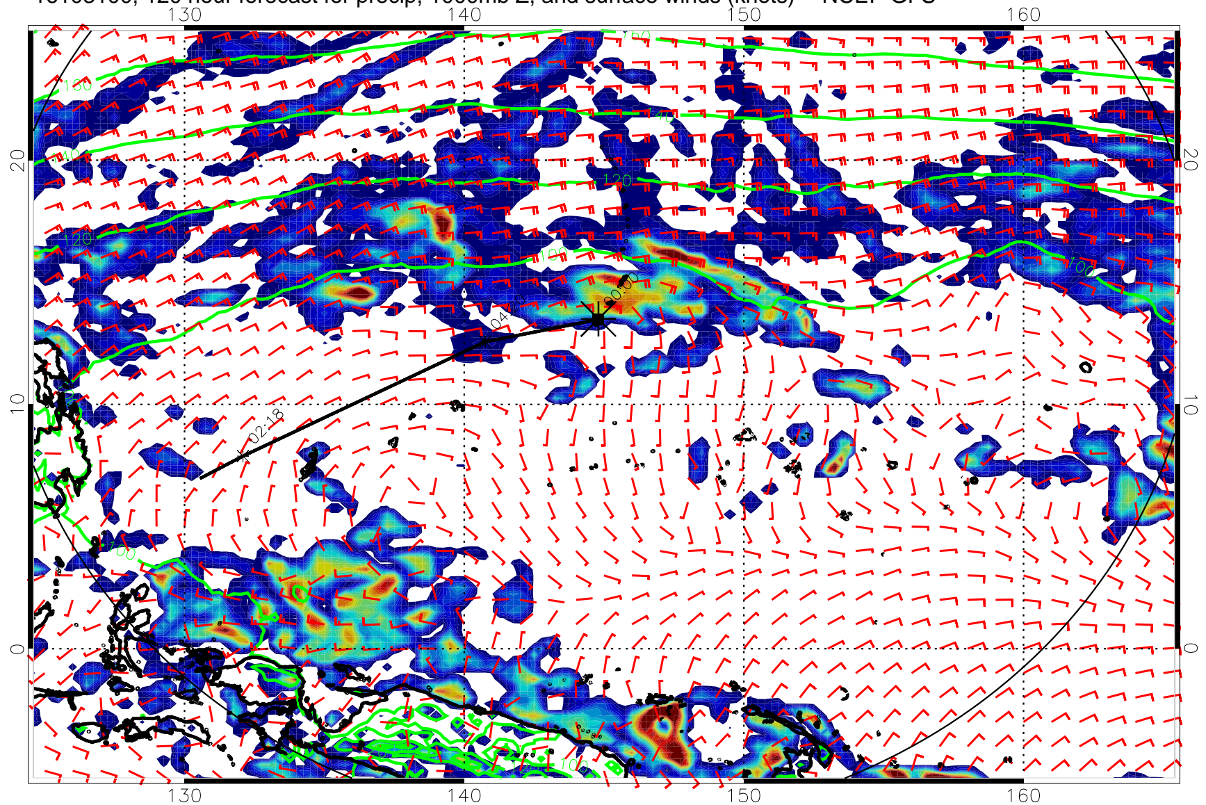
16103100, 120 hour forecast for precip, 1000mb Z, and surface winds (knots) -- NCEP GFS
