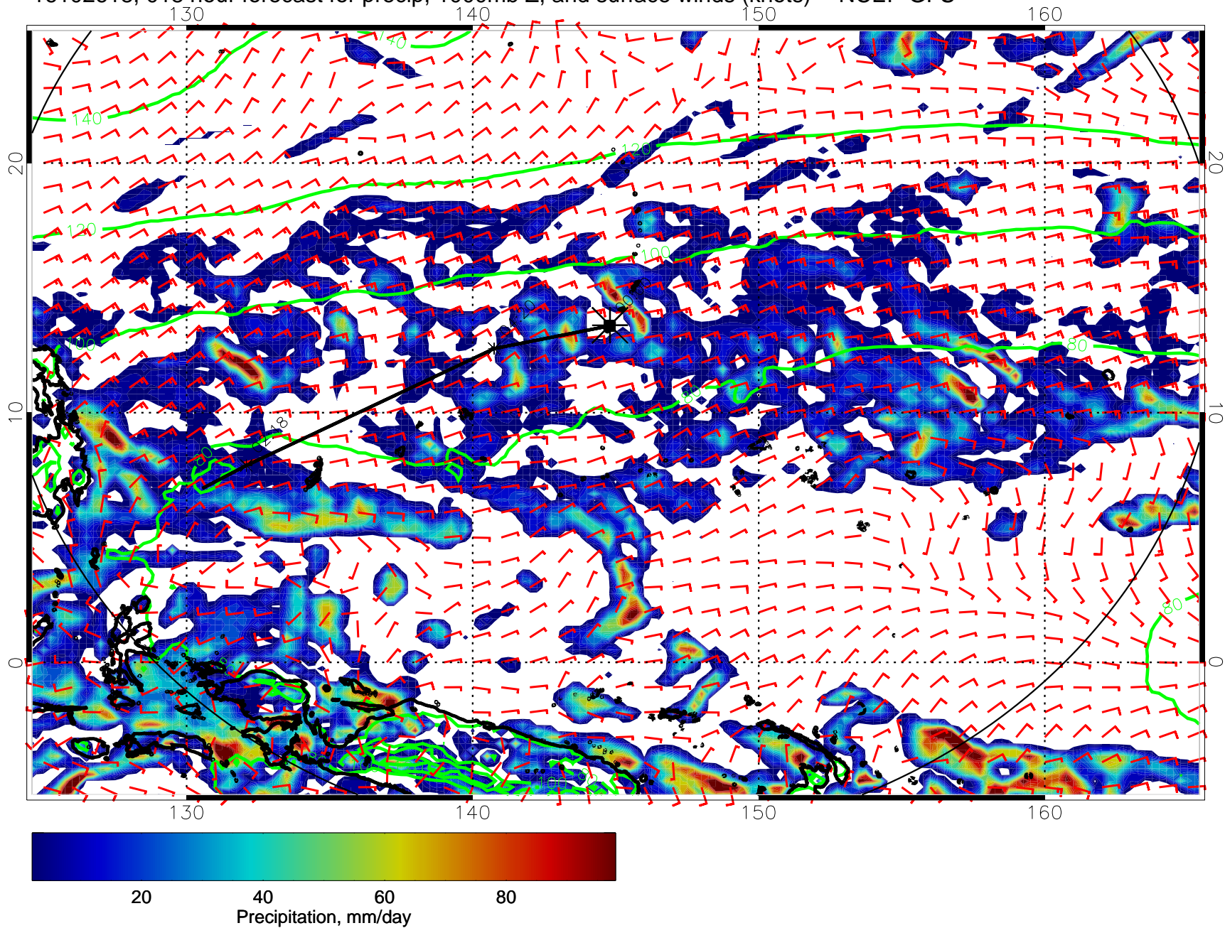
16102618, 018 hour forecast for precip, 1000mb Z, and surface winds (knots) -- NCEP GFS
