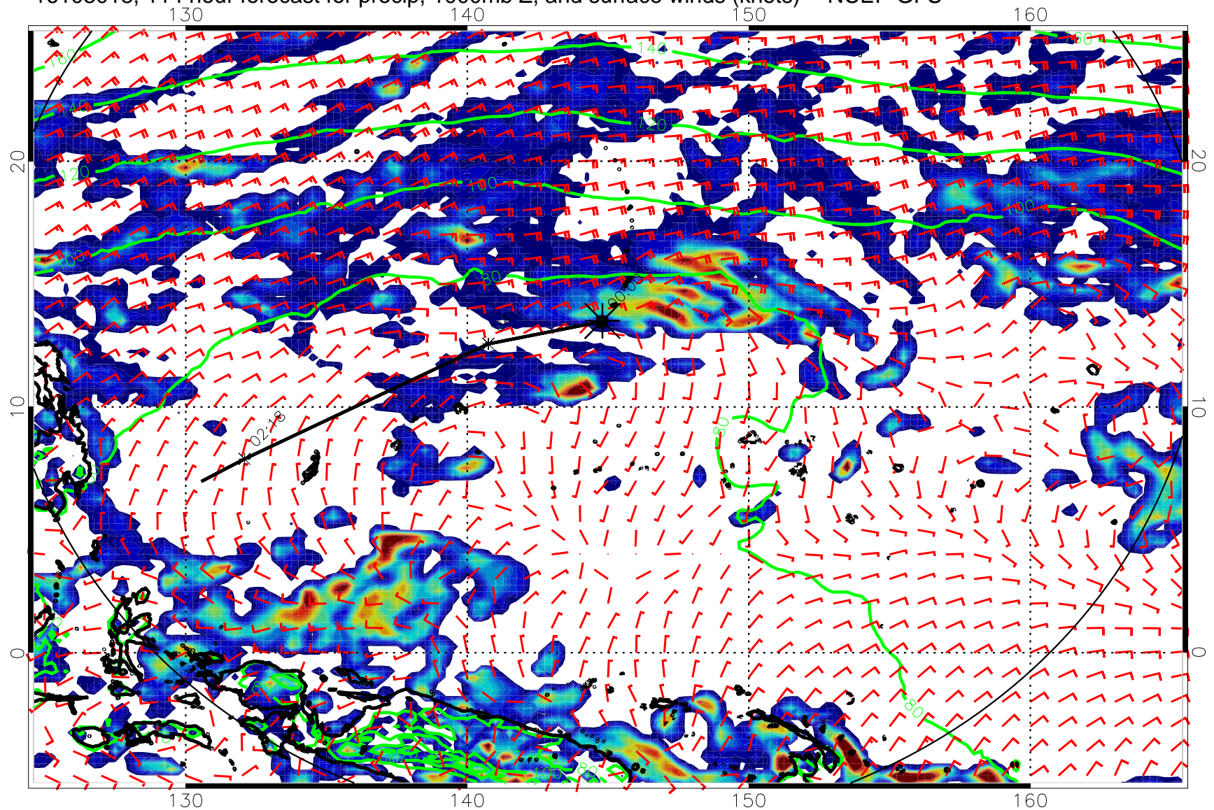
16103018, 114 hour forecast for precip, 1000mb Z, and surface winds (knots) -- NCEP GFS
