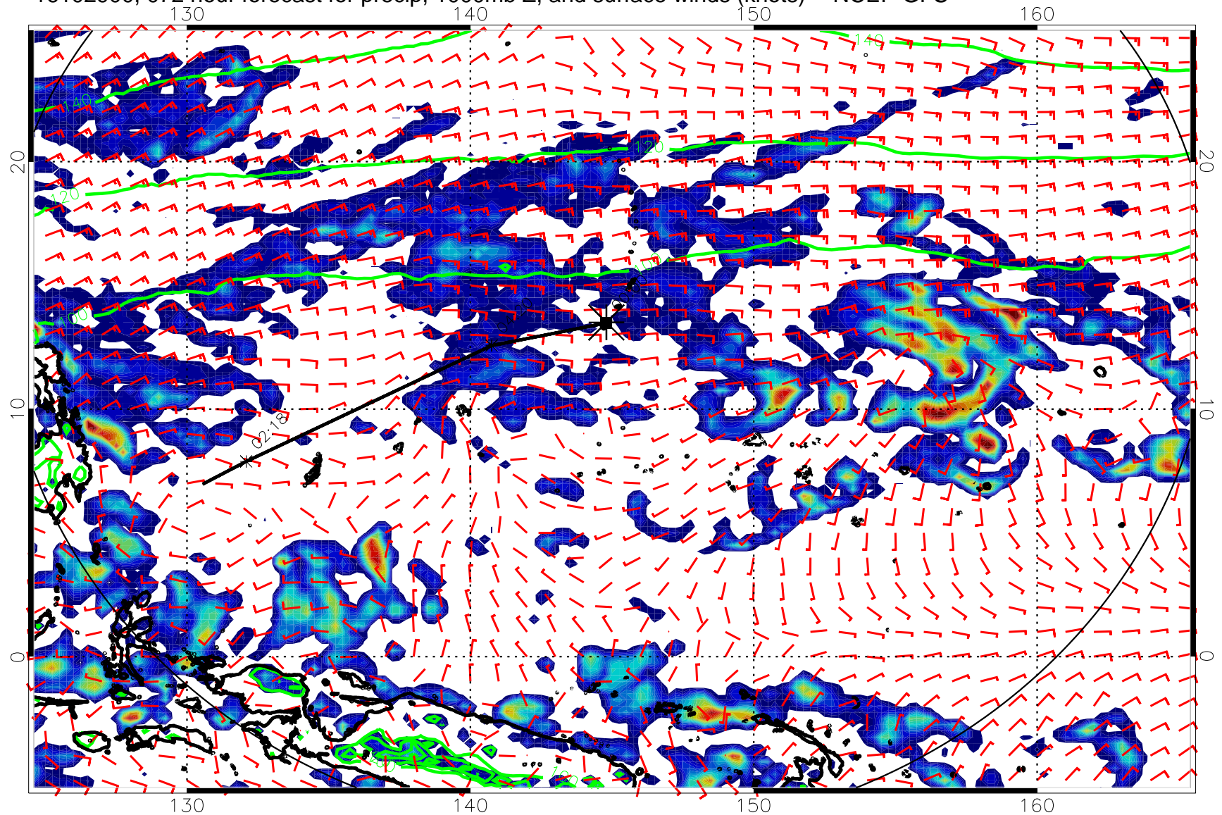
16102900, 072 hour forecast for precip, 1000mb Z, and surface winds (knots) -- NCEP GFS
