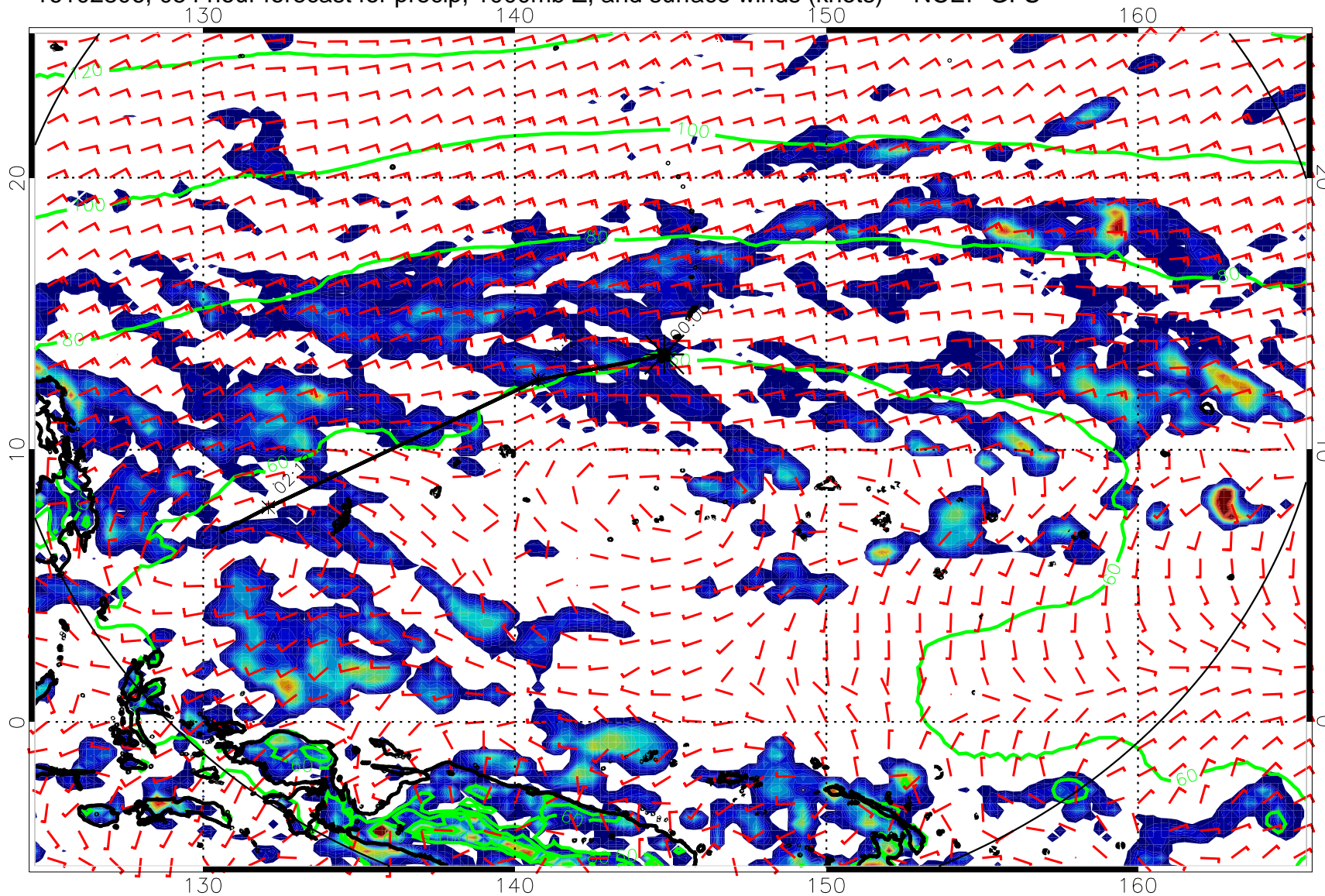
16102806, 054 hour forecast for precip, 1000mb Z, and surface winds (knots) -- NCEP GFS
