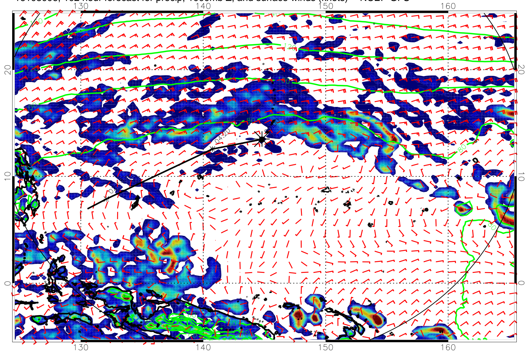
16103006, 102 hour forecast for precip, 1000mb Z, and surface winds (knots) -- NCEP GFS
