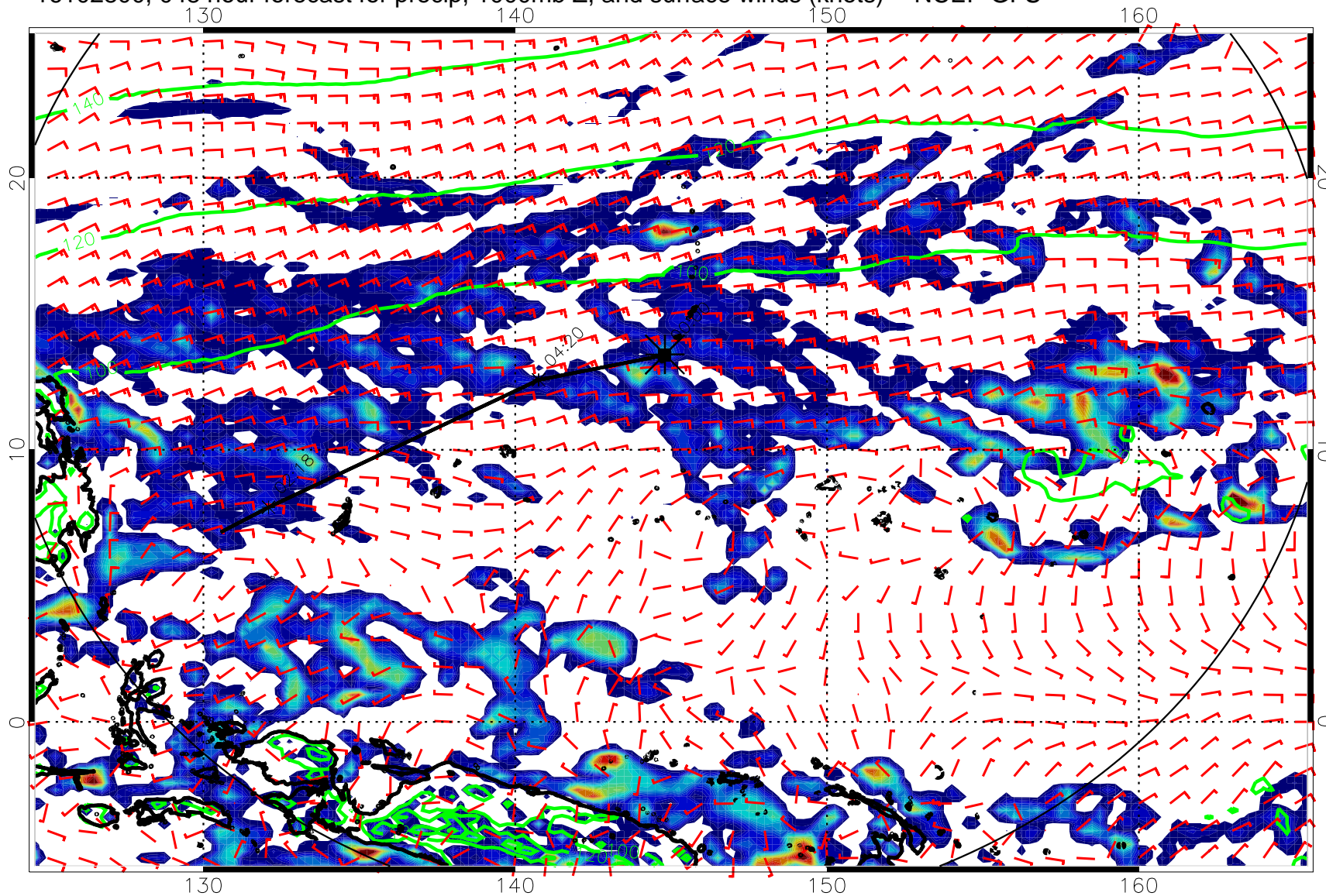
16102800, 048 hour forecast for precip, 1000mb Z, and surface winds (knots) -- NCEP GFS
