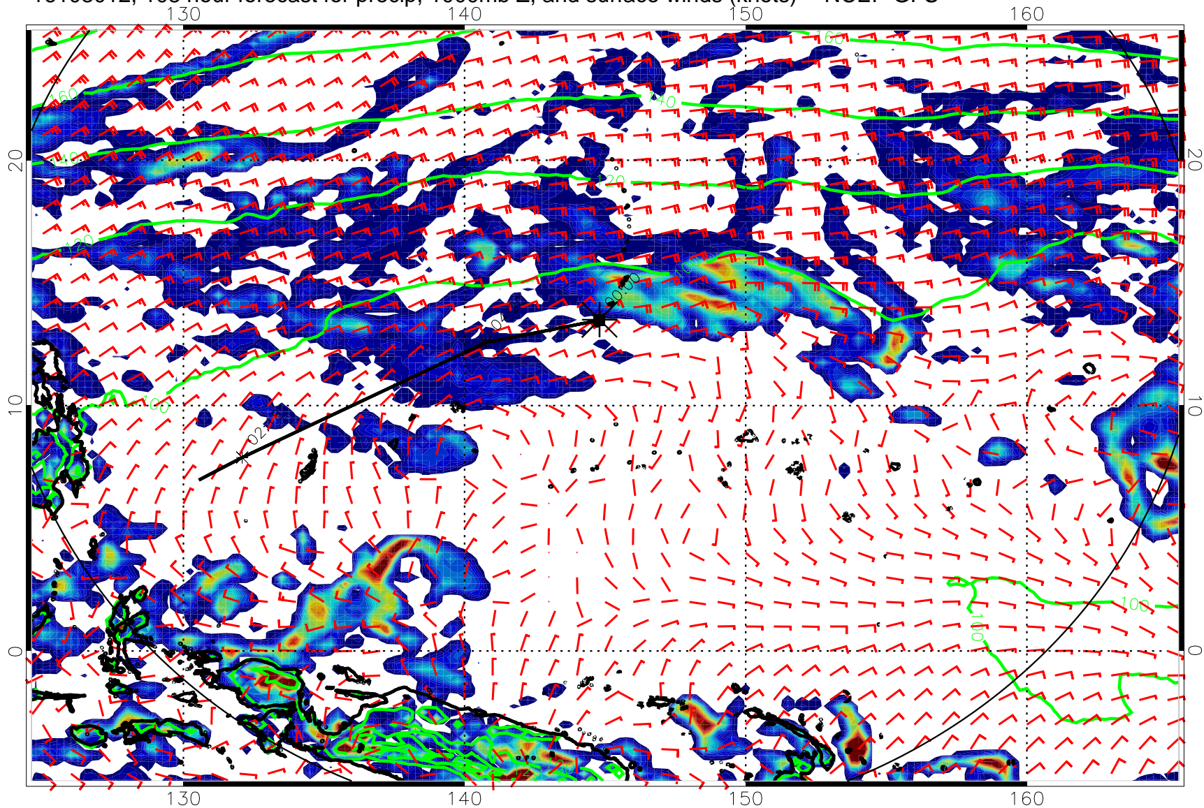
16103012, 108 hour forecast for precip, 1000mb Z, and surface winds (knots) -- NCEP GFS
