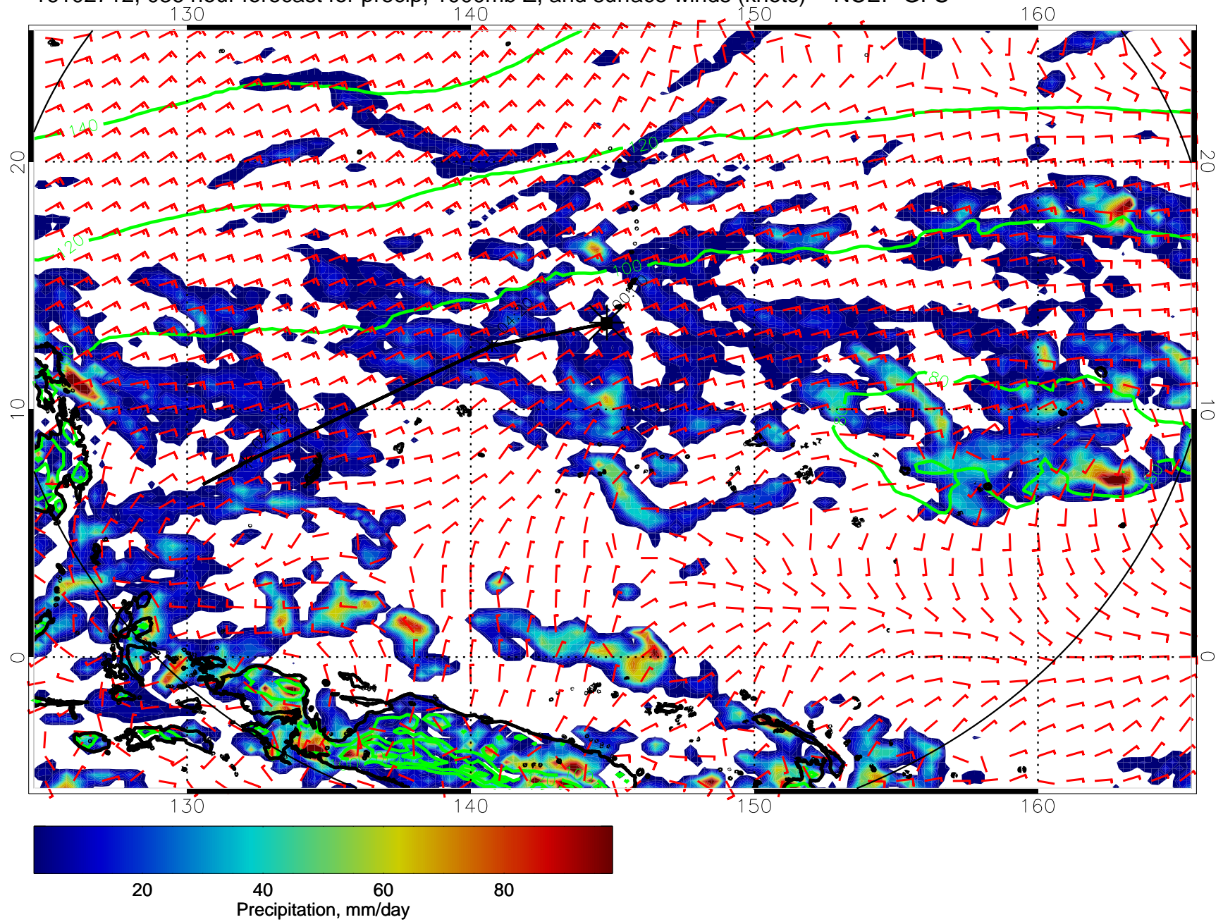
16102712, 036 hour forecast for precip, 1000mb Z, and surface winds (knots) -- NCEP GFS
