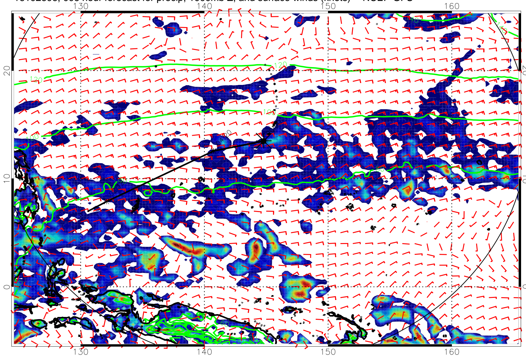
16102606, 006 hour forecast for precip, 1000mb Z, and surface winds (knots) -- NCEP GFS
