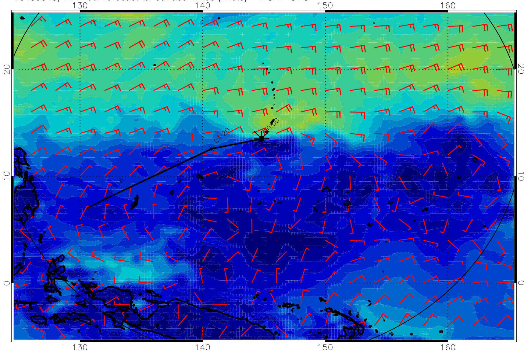
16103018, 114 hour forecast for surface winds (knots) -- NCEP GFS
