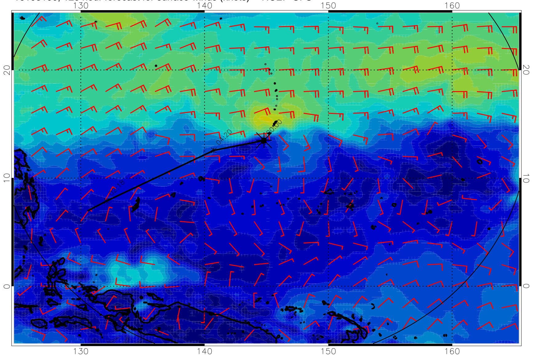
16103100, 120 hour forecast for surface winds (knots) -- NCEP GFS
