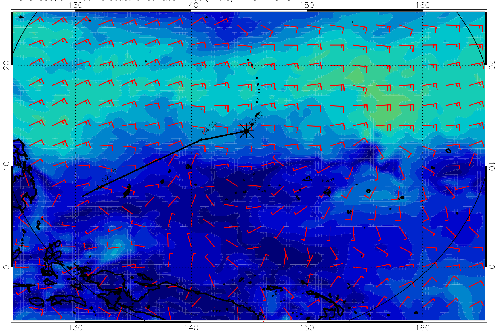
16102900, 072 hour forecast for surface winds (knots) -- NCEP GFS
