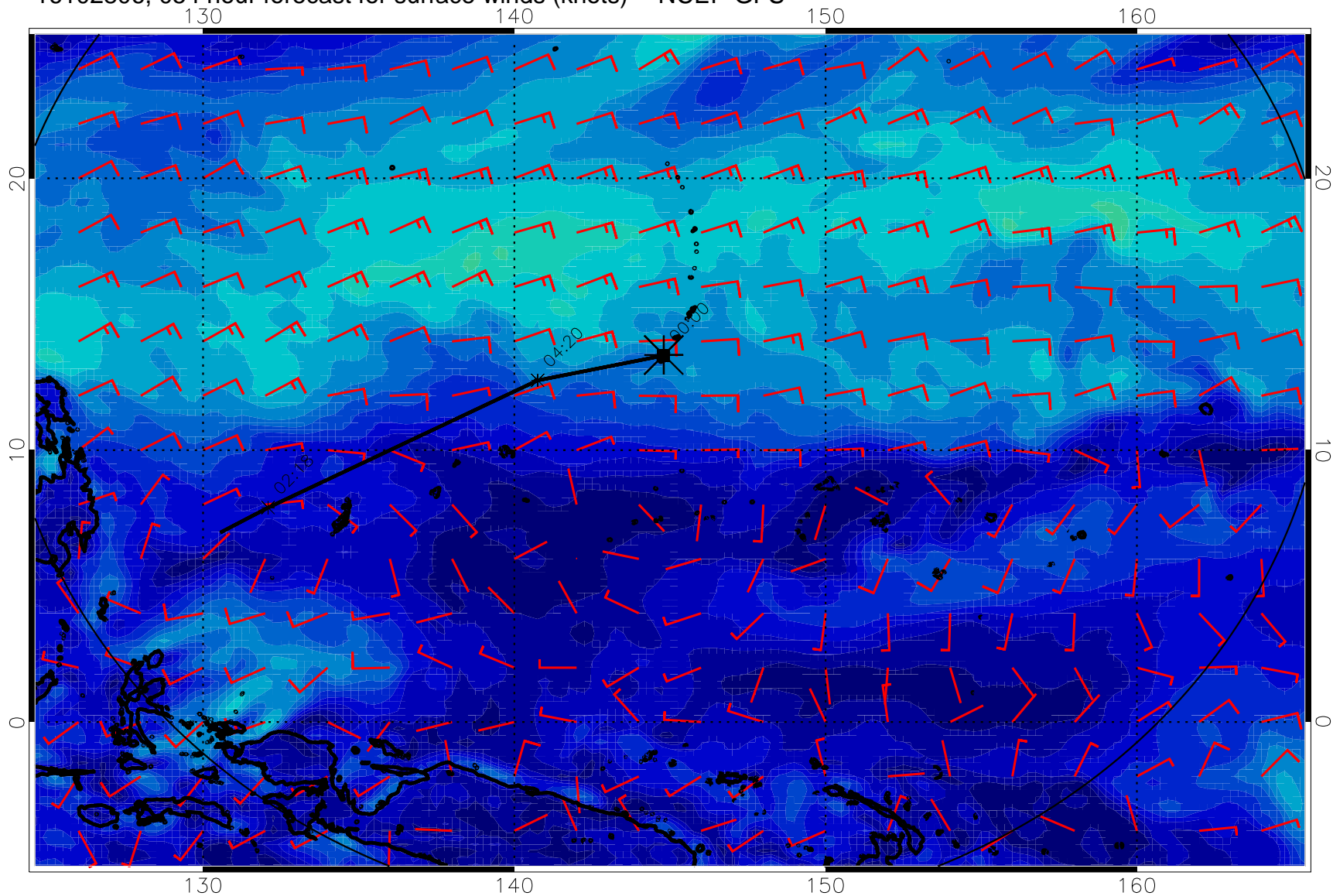
16102806, 054 hour forecast for surface winds (knots) -- NCEP GFS
