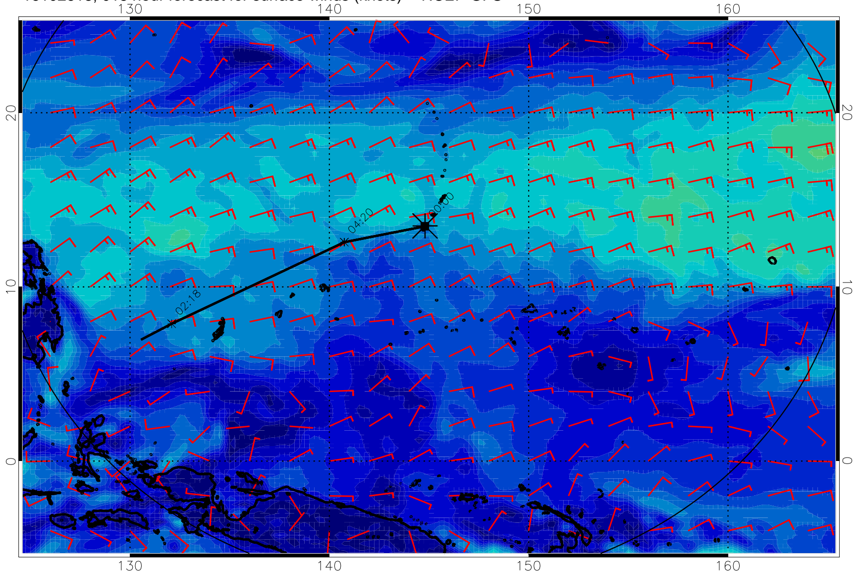
16102618, 018 hour forecast for surface winds (knots) -- NCEP GFS
