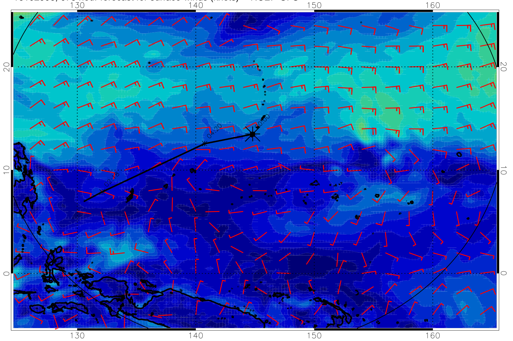
16102906, 078 hour forecast for surface winds (knots) -- NCEP GFS
