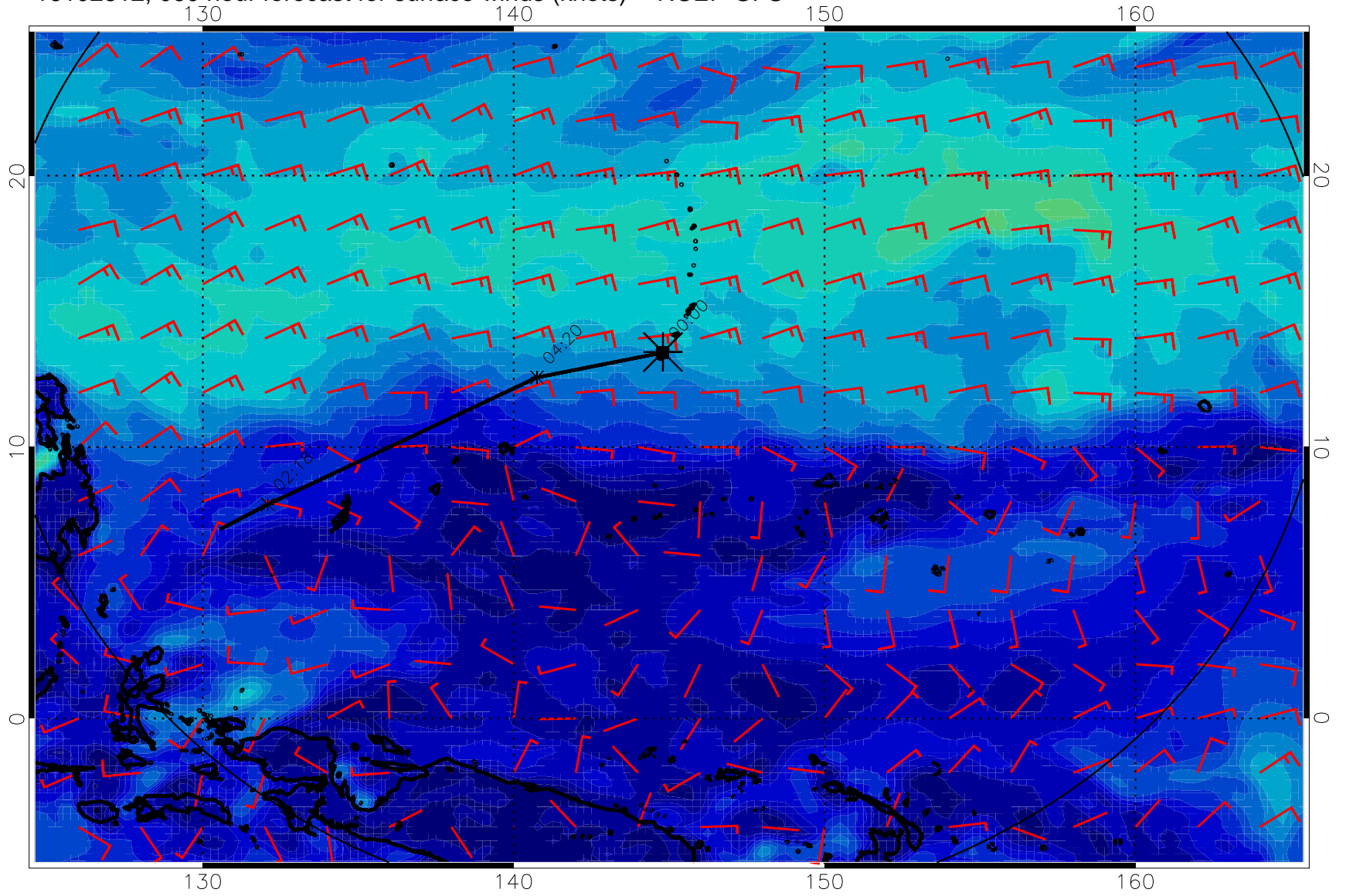
16102812, 060 hour forecast for surface winds (knots) -- NCEP GFS
