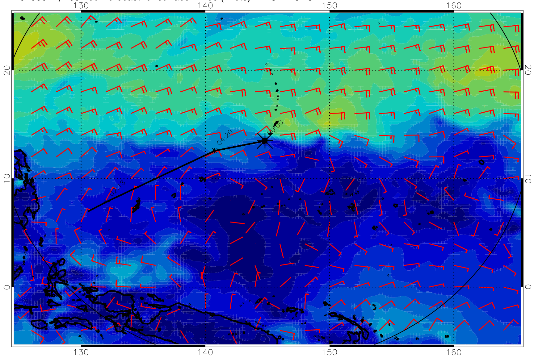
16103012, 108 hour forecast for surface winds (knots) -- NCEP GFS
