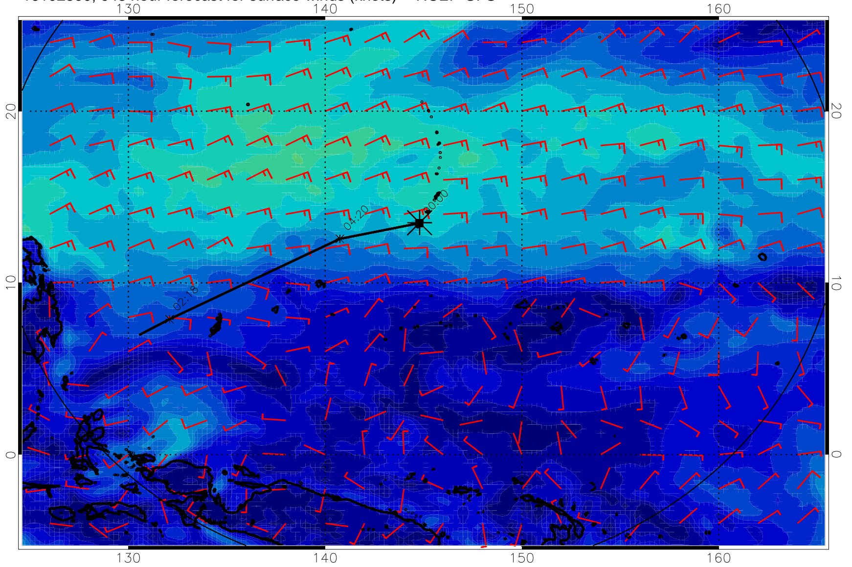
16102800, 048 hour forecast for surface winds (knots) -- NCEP GFS
