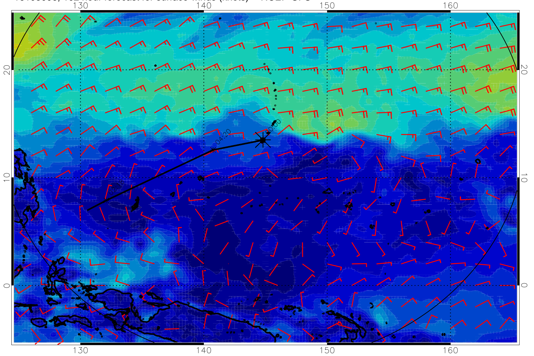
16103006, 102 hour forecast for surface winds (knots) -- NCEP GFS
