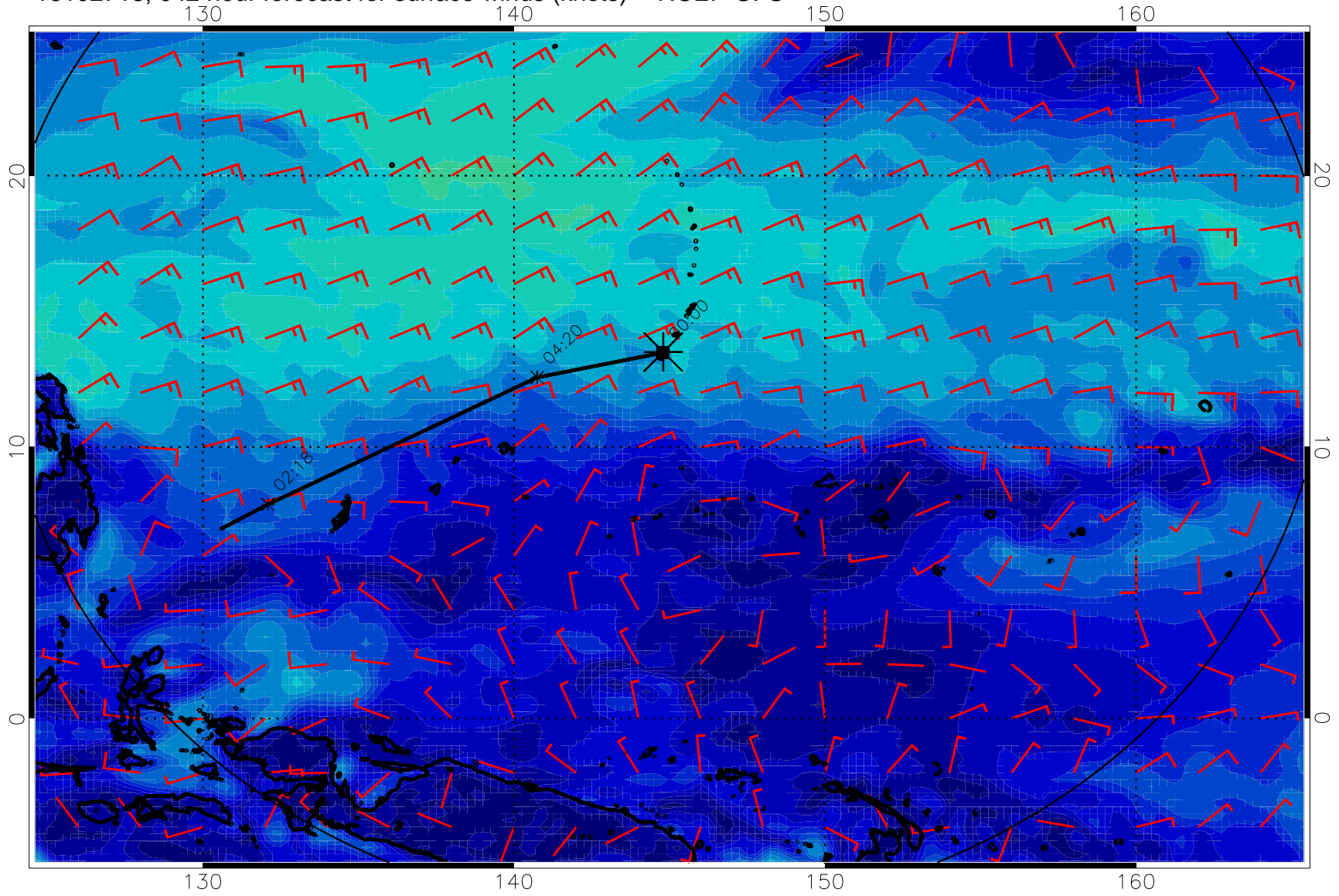
16102718, 042 hour forecast for surface winds (knots) -- NCEP GFS
