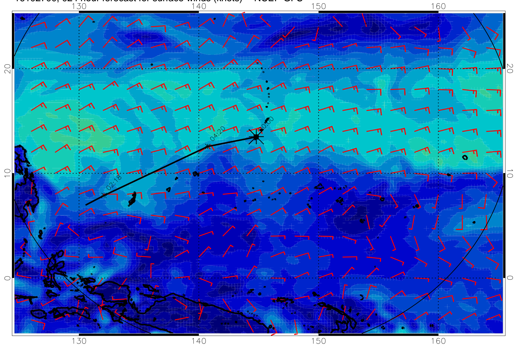
16102700, 024 hour forecast for surface winds (knots) -- NCEP GFS
