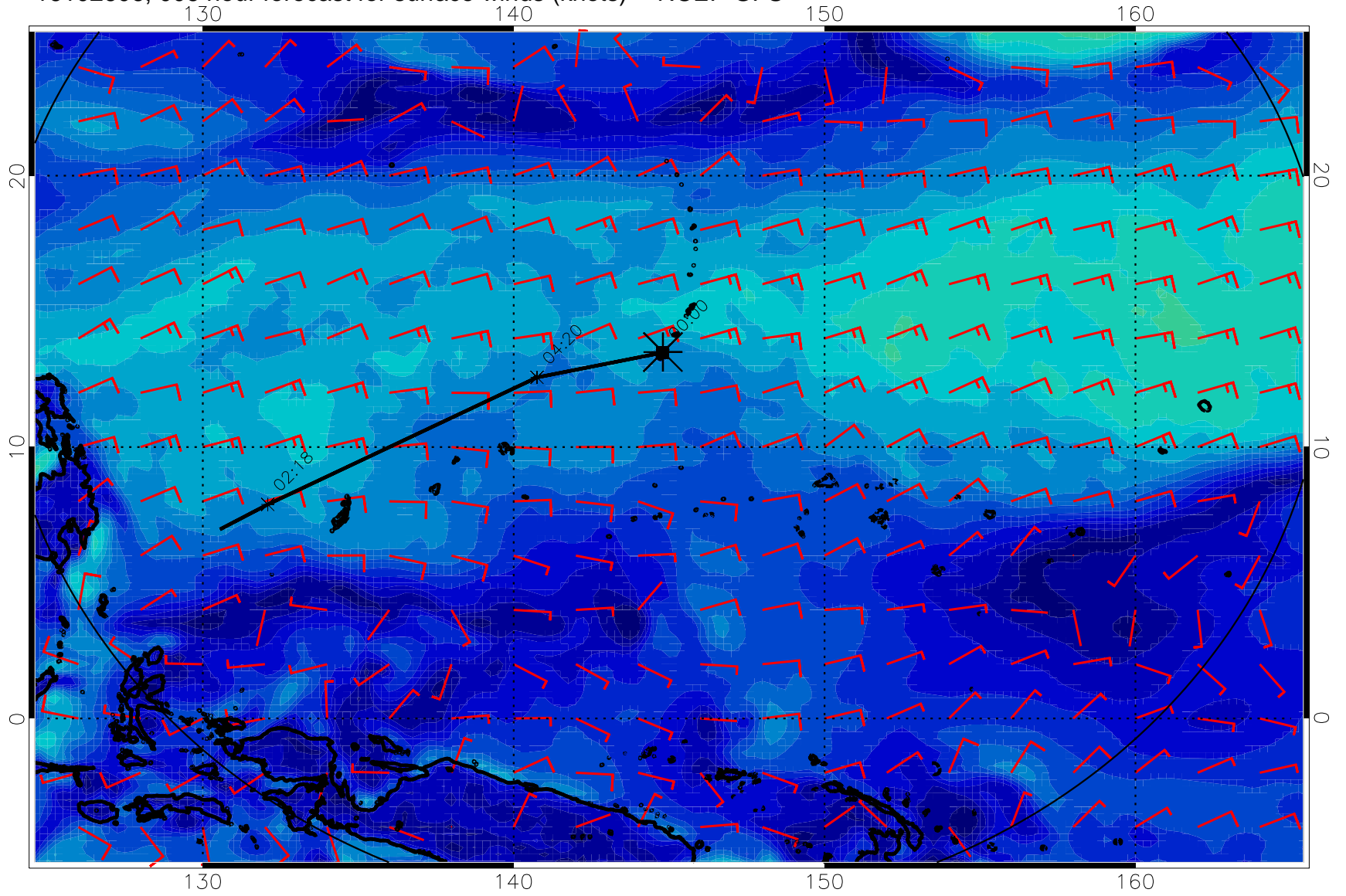
16102606, 006 hour forecast for surface winds (knots) -- NCEP GFS
