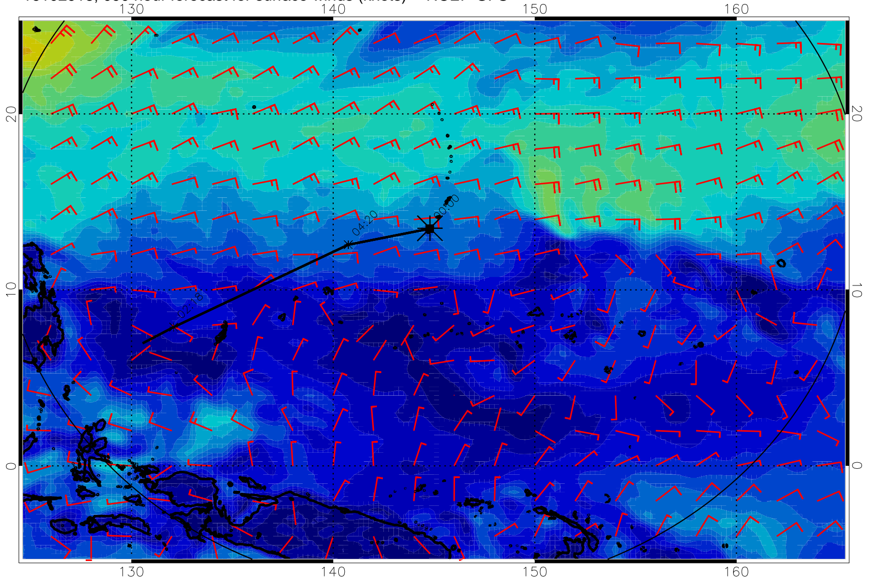
16102918, 090 hour forecast for surface winds (knots) -- NCEP GFS
