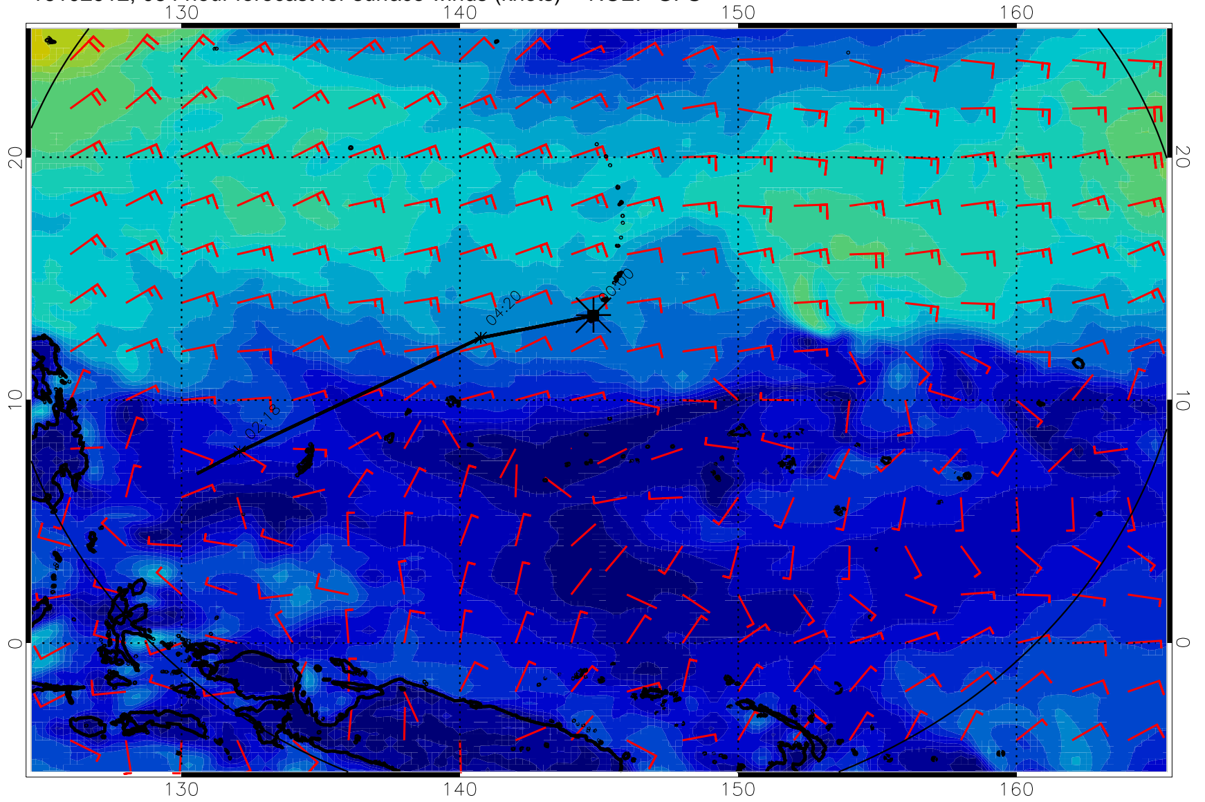
16102912, 084 hour forecast for surface winds (knots) -- NCEP GFS
