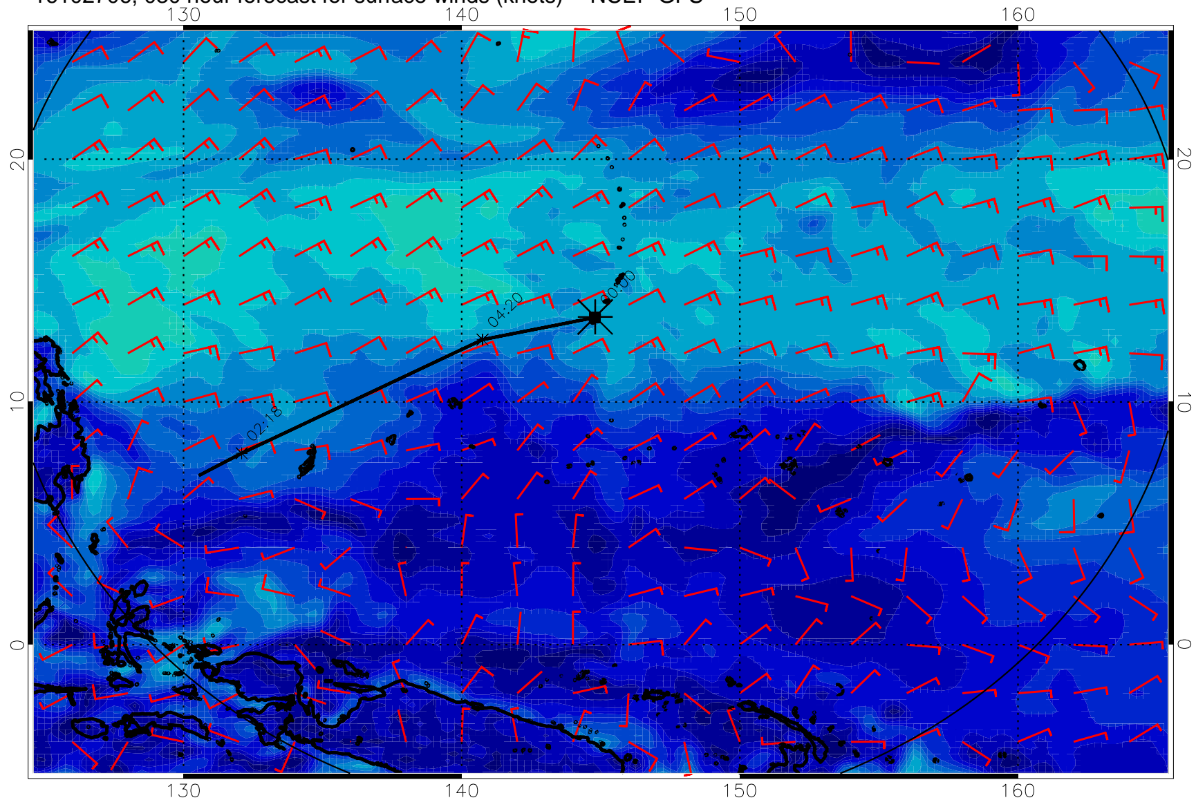
16102706, 030 hour forecast for surface winds (knots) -- NCEP GFS
