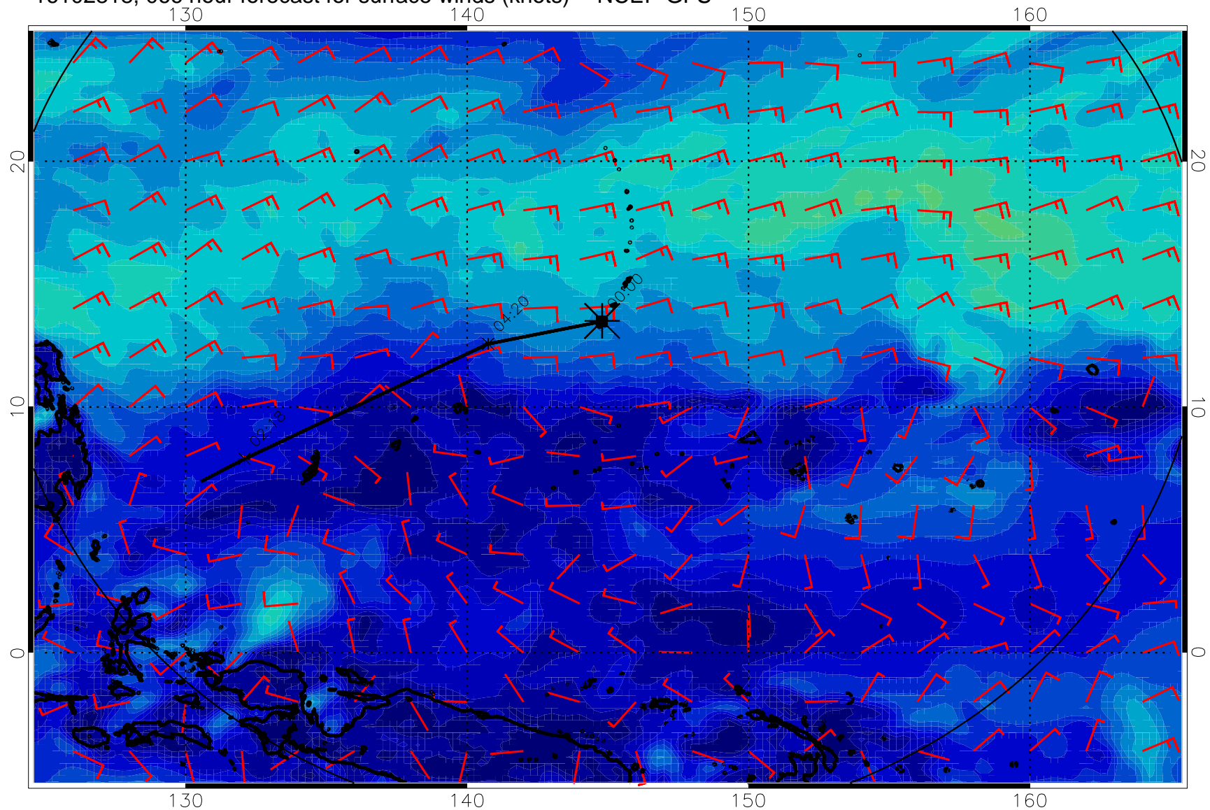
16102818, 066 hour forecast for surface winds (knots) -- NCEP GFS
