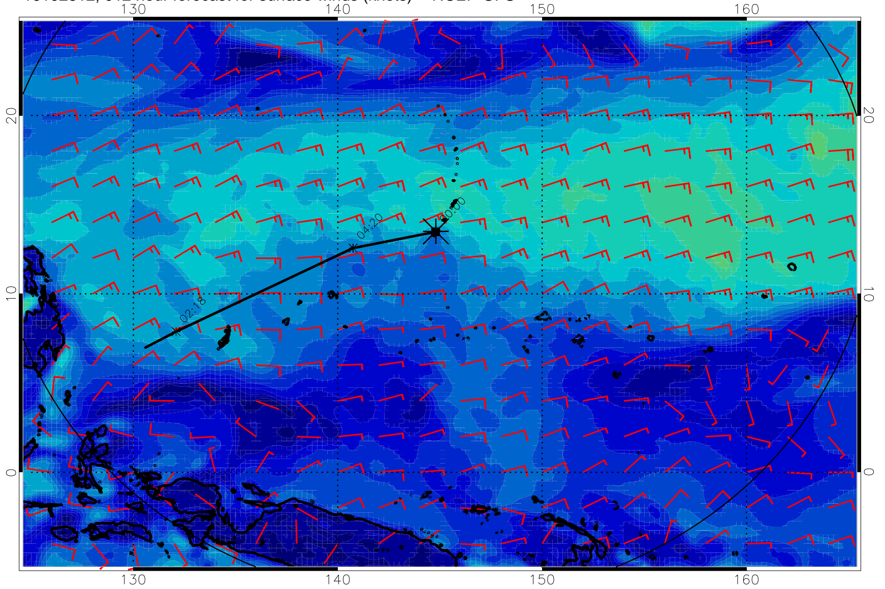
16102612, 012 hour forecast for surface winds (knots) -- NCEP GFS
