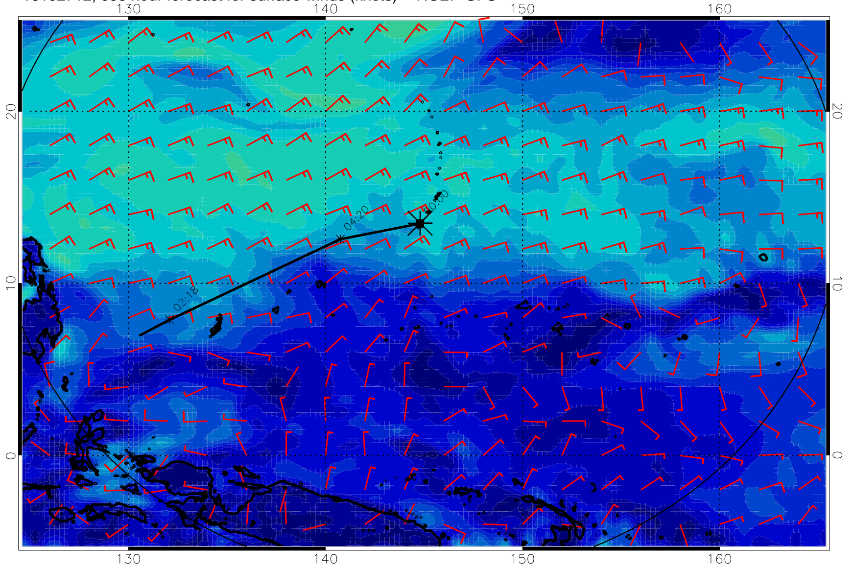
16102712, 036 hour forecast for surface winds (knots) -- NCEP GFS
