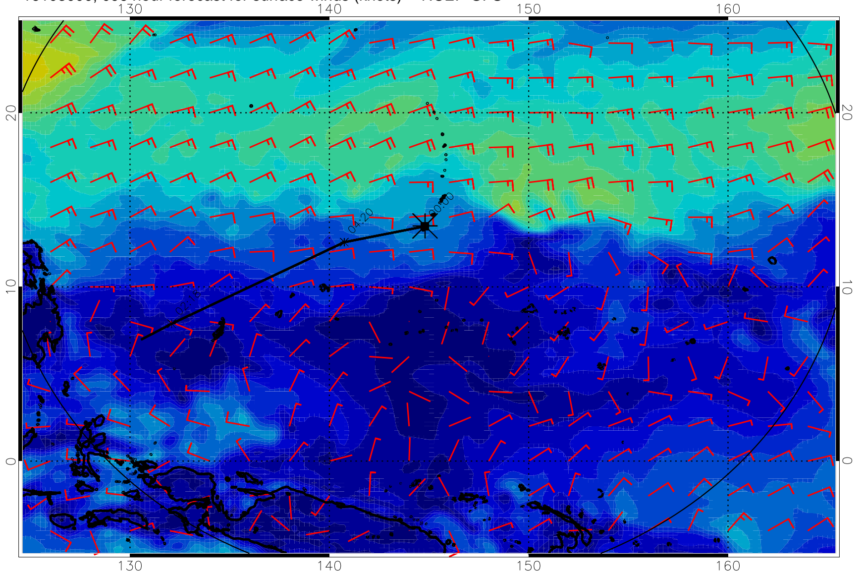
16103000, 096 hour forecast for surface winds (knots) -- NCEP GFS
