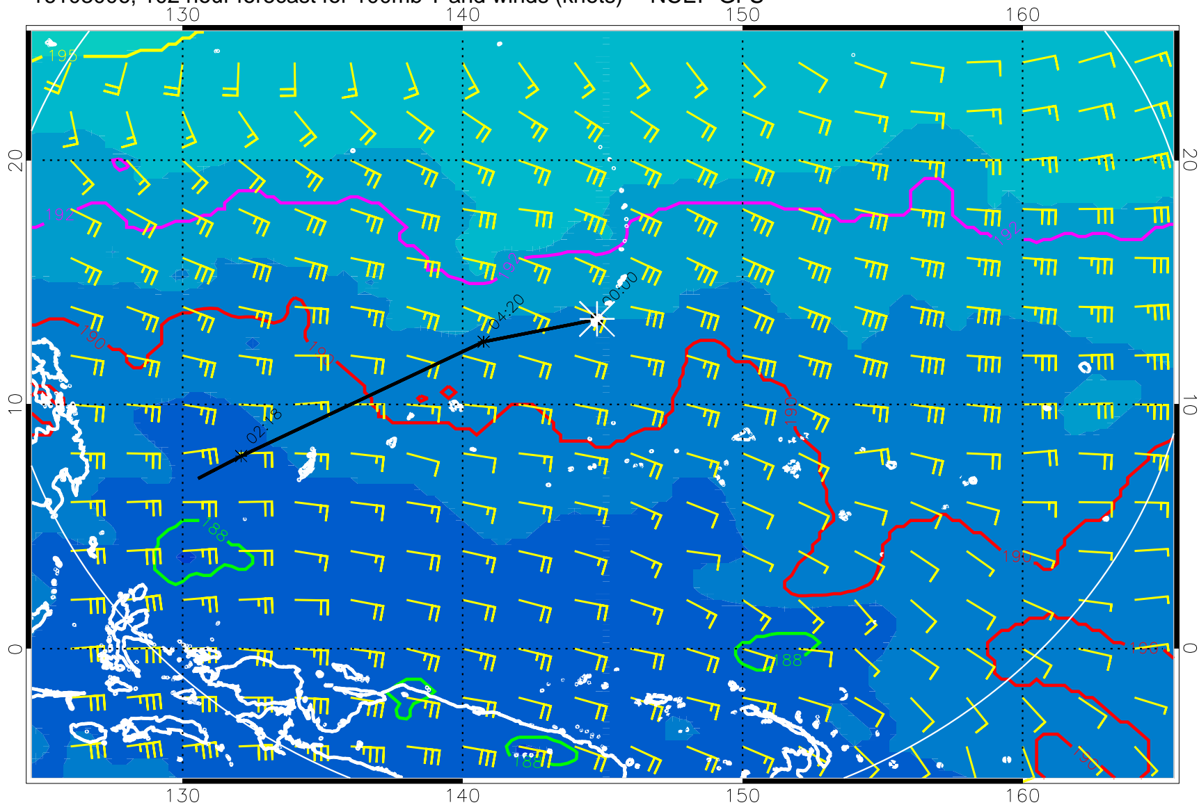
16103006, 102 hour forecast for 100mb T and winds (knots) -- NCEP GFS
