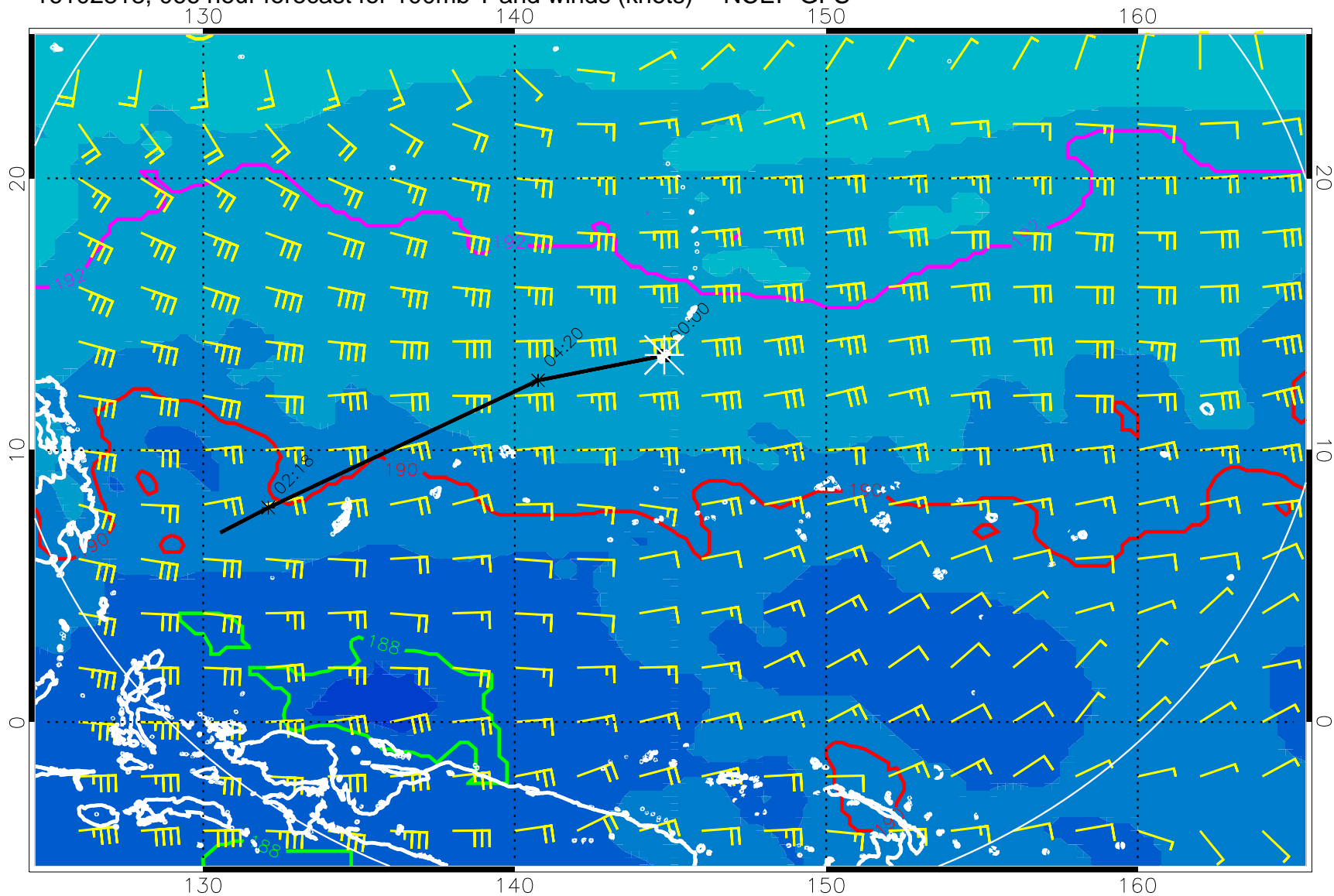
16102818, 066 hour forecast for 100mb T and winds (knots) -- NCEP GFS
