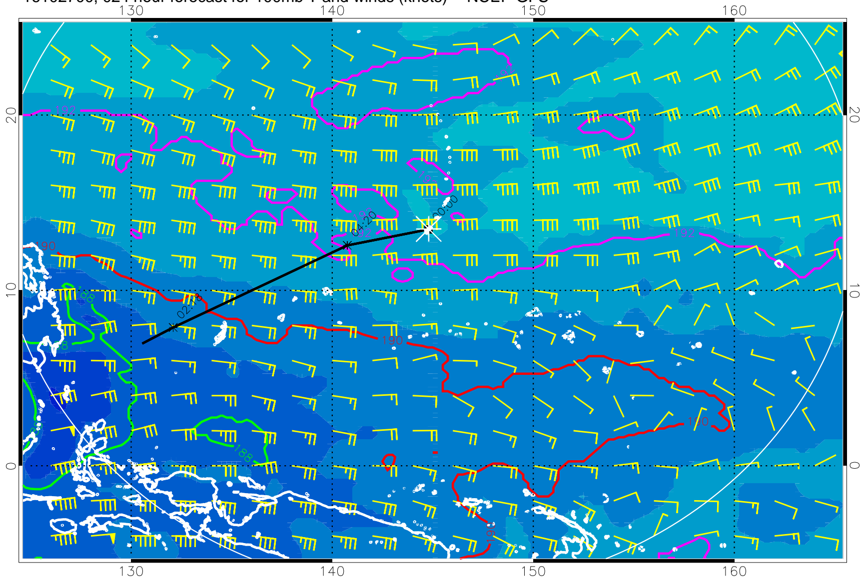
16102700, 024 hour forecast for 100mb T and winds (knots) -- NCEP GFS
