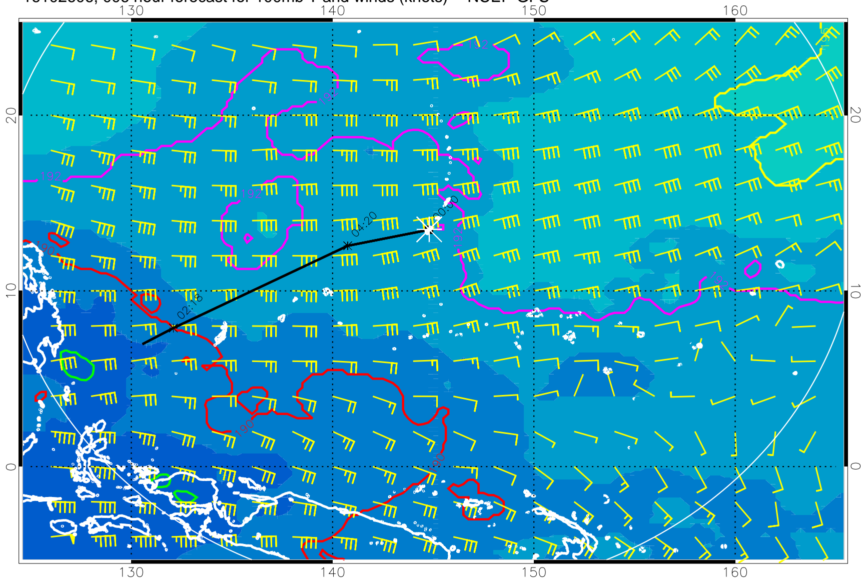
16102606, 006 hour forecast for 100mb T and winds (knots) -- NCEP GFS
