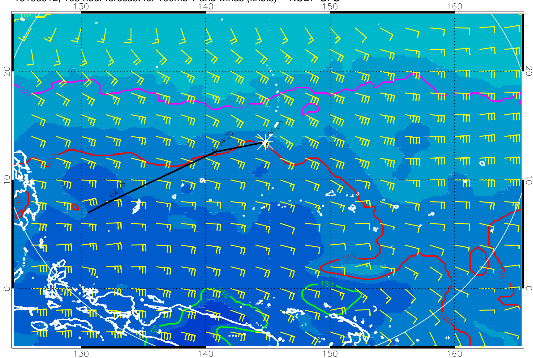
16103012, 108 hour forecast for 100mb T and winds (knots) -- NCEP GFS
