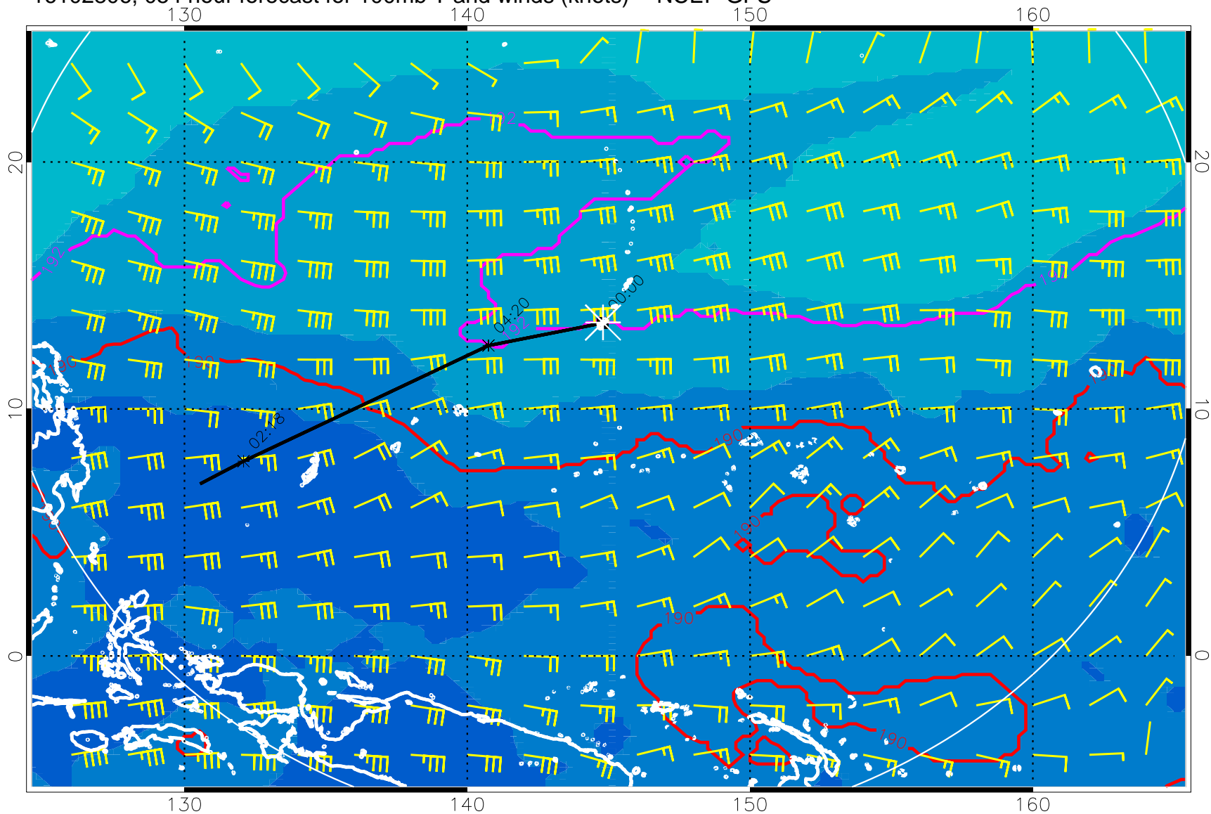
16102806, 054 hour forecast for 100mb T and winds (knots) -- NCEP GFS
