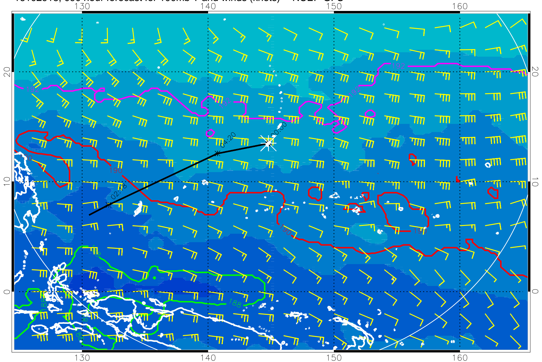
16102918, 090 hour forecast for 100mb T and winds (knots) -- NCEP GFS
