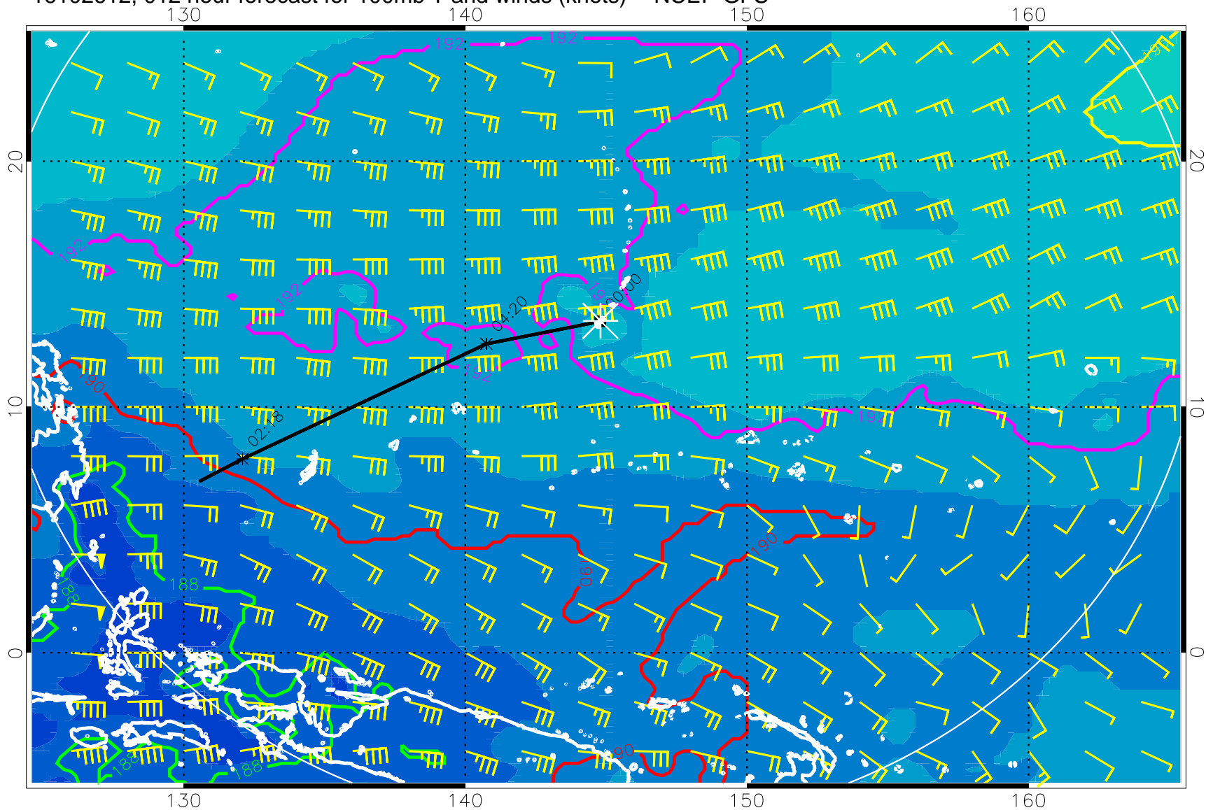
16102612, 012 hour forecast for 100mb T and winds (knots) -- NCEP GFS
