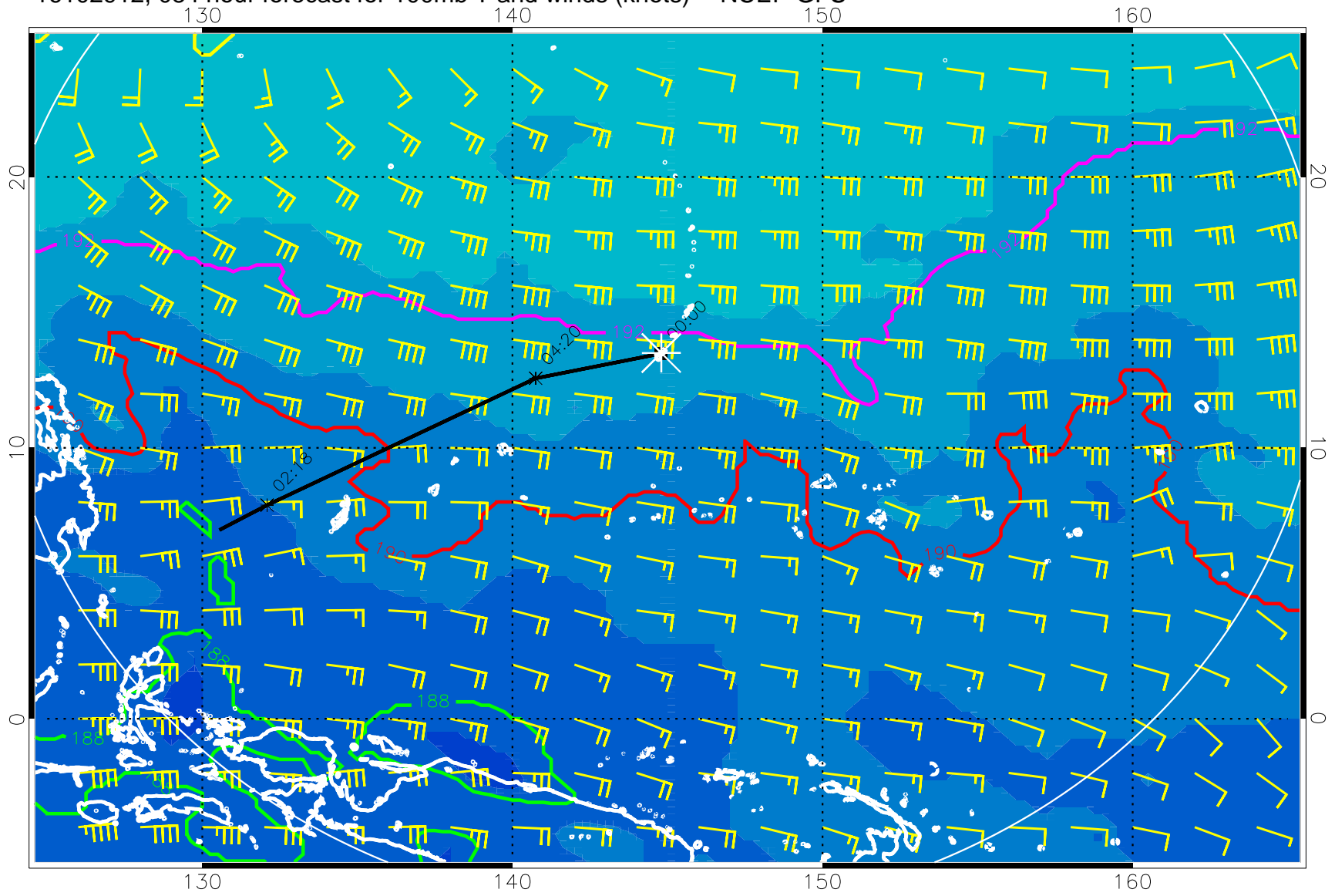
16102912, 084 hour forecast for 100mb T and winds (knots) -- NCEP GFS
