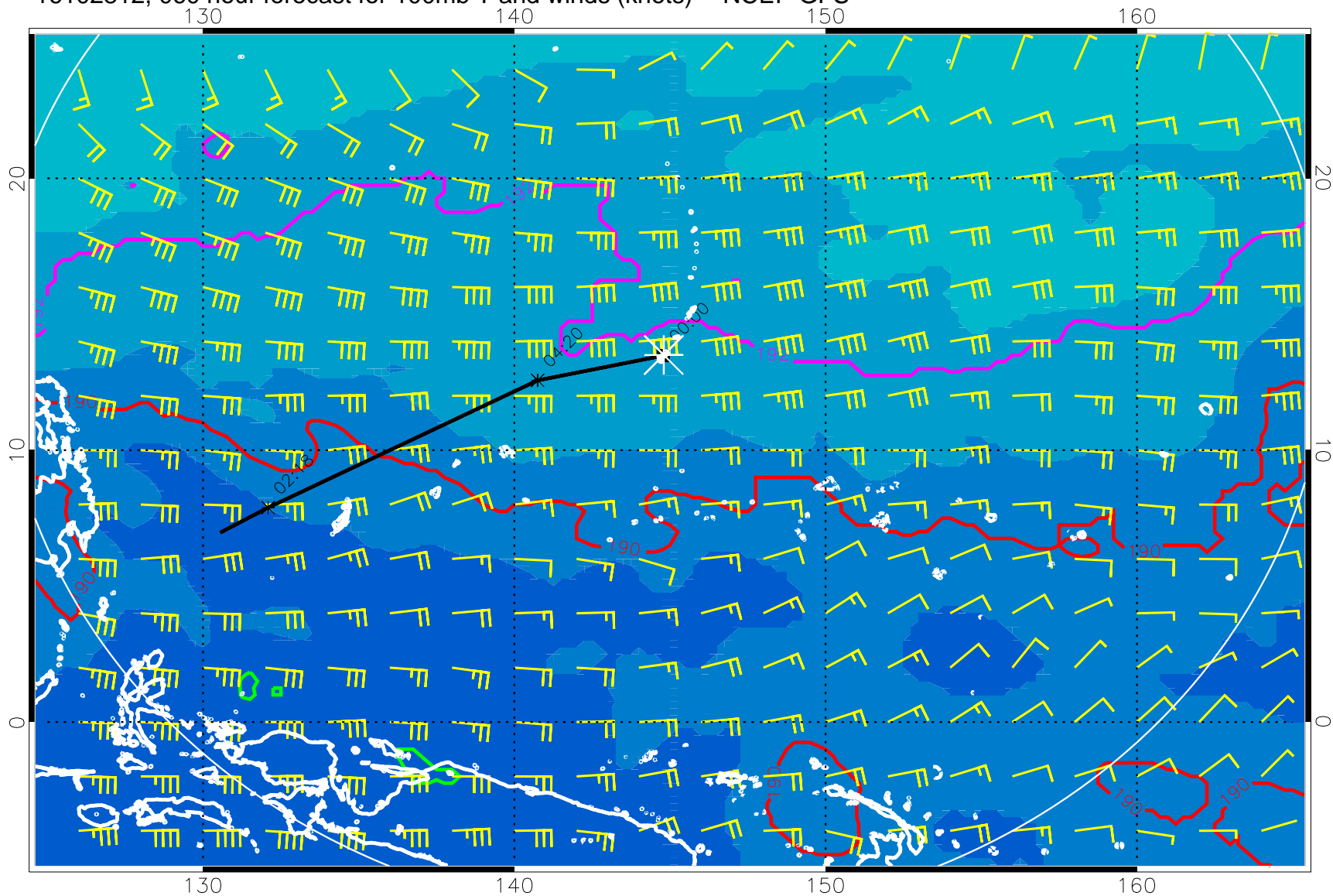
16102812, 060 hour forecast for 100mb T and winds (knots) -- NCEP GFS
