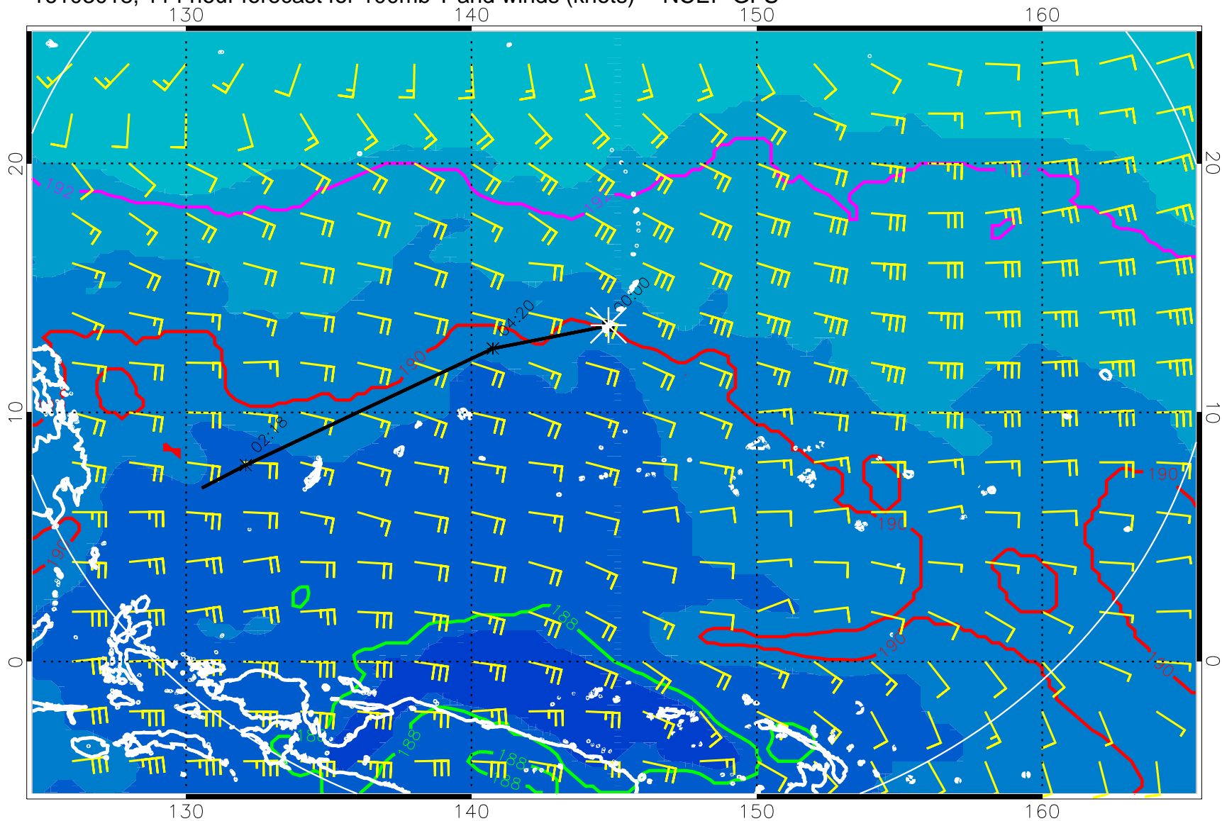
16103018, 114 hour forecast for 100mb T and winds (knots) -- NCEP GFS
