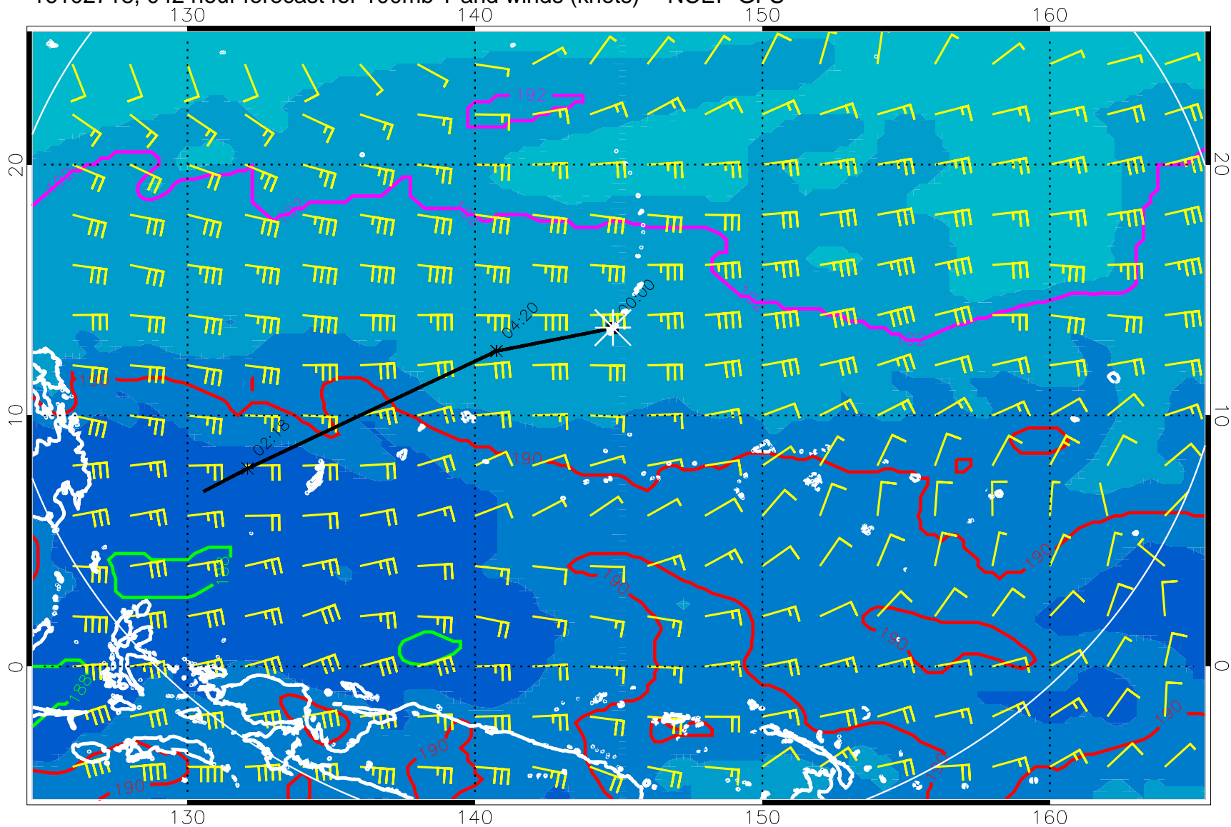
16102718, 042 hour forecast for 100mb T and winds (knots) -- NCEP GFS
