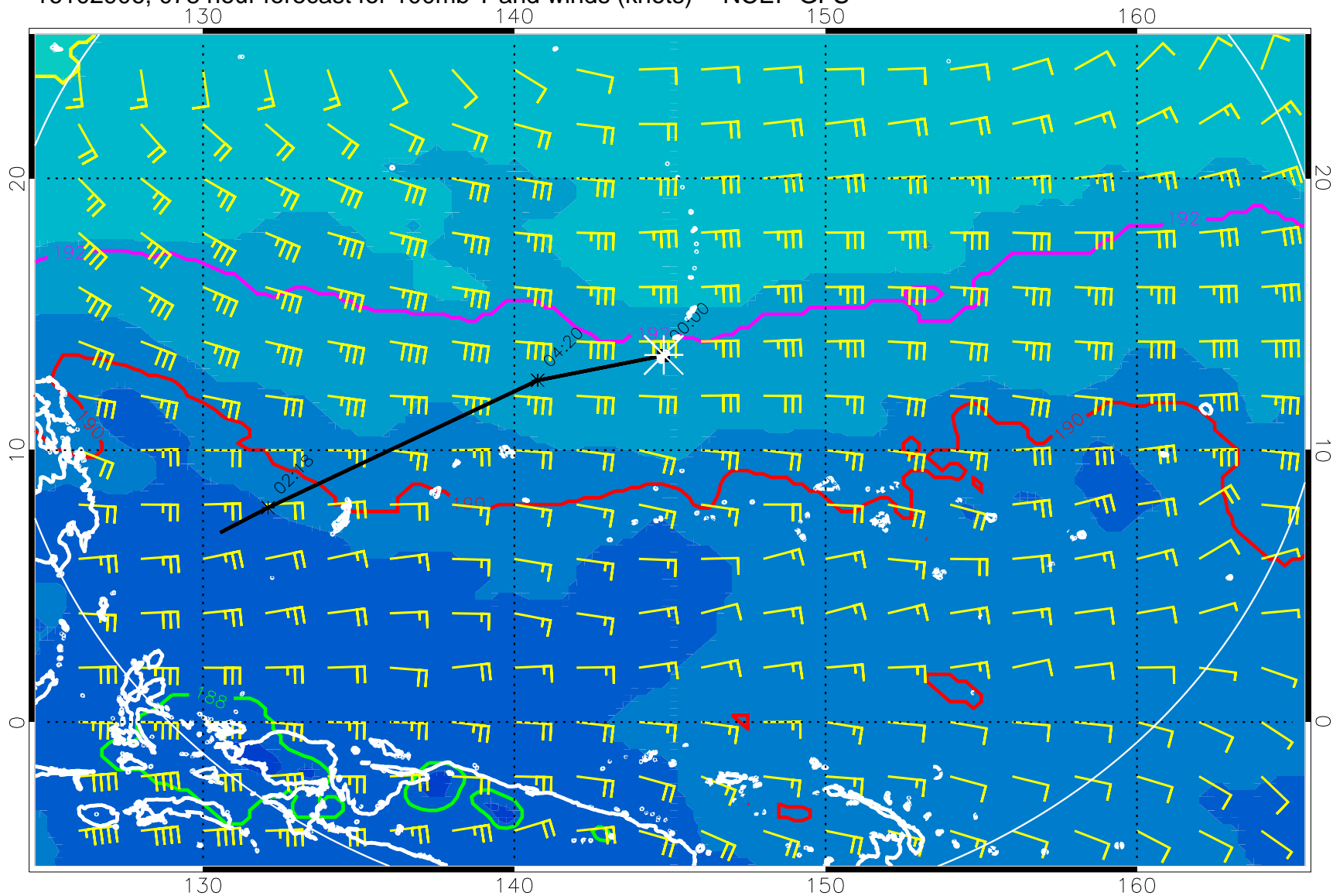
16102906, 078 hour forecast for 100mb T and winds (knots) -- NCEP GFS
