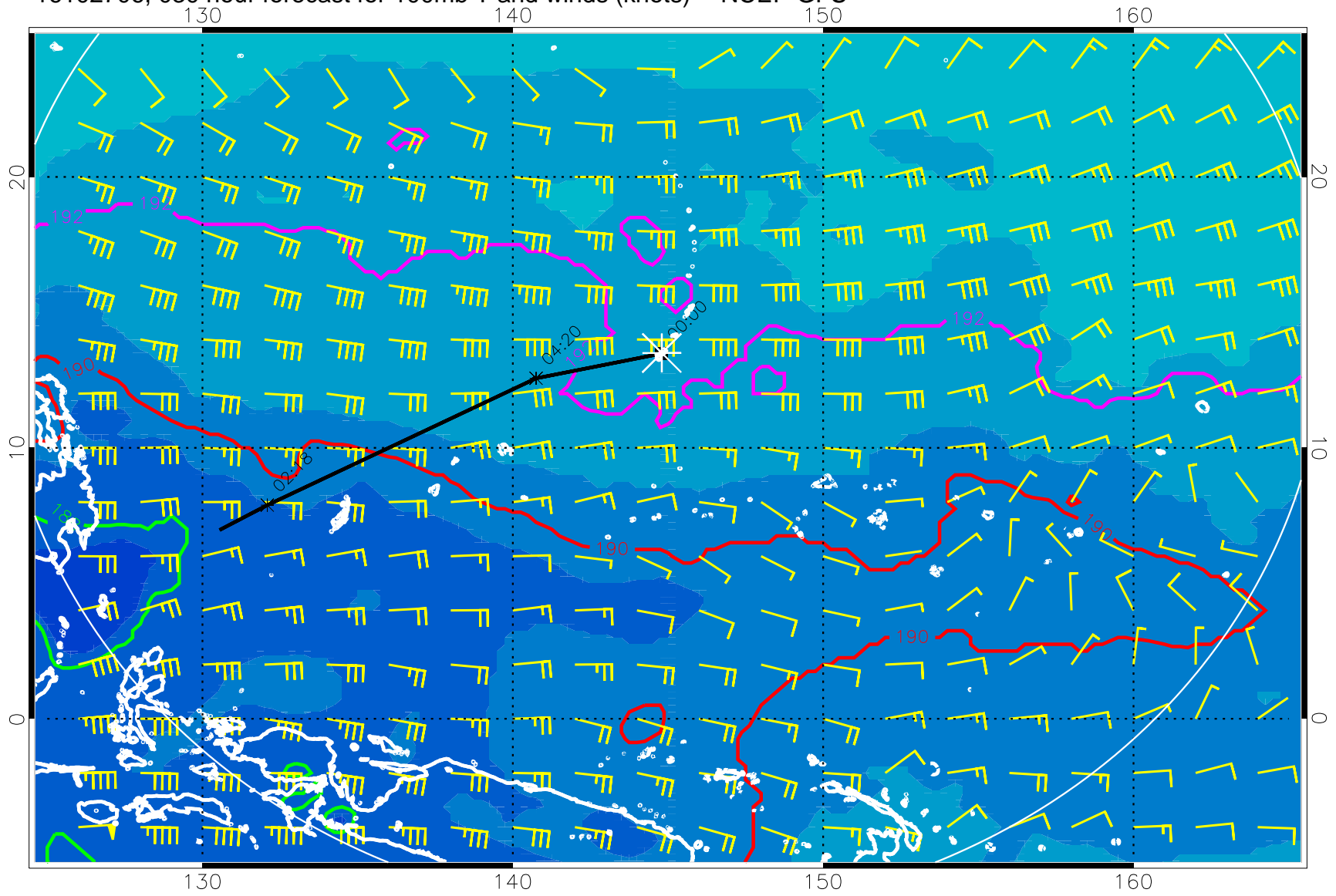
16102706, 030 hour forecast for 100mb T and winds (knots) -- NCEP GFS
