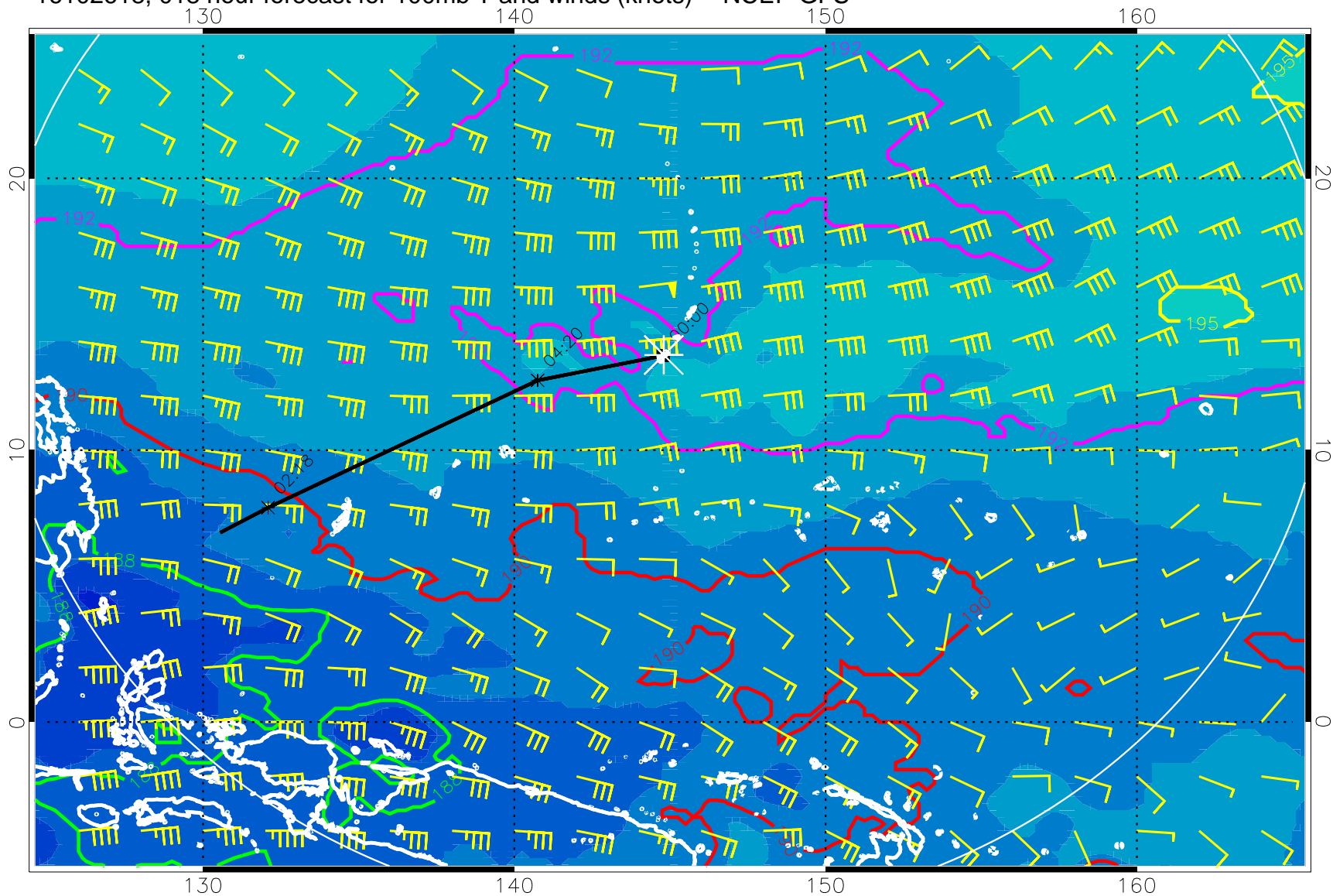
16102618, 018 hour forecast for 100mb T and winds (knots) -- NCEP GFS
