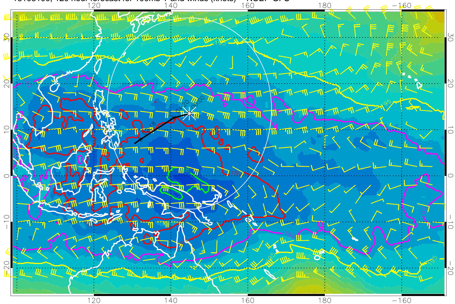
16103100, 120 hour forecast for 100mb T and winds (knots) -- NCEP GFS
