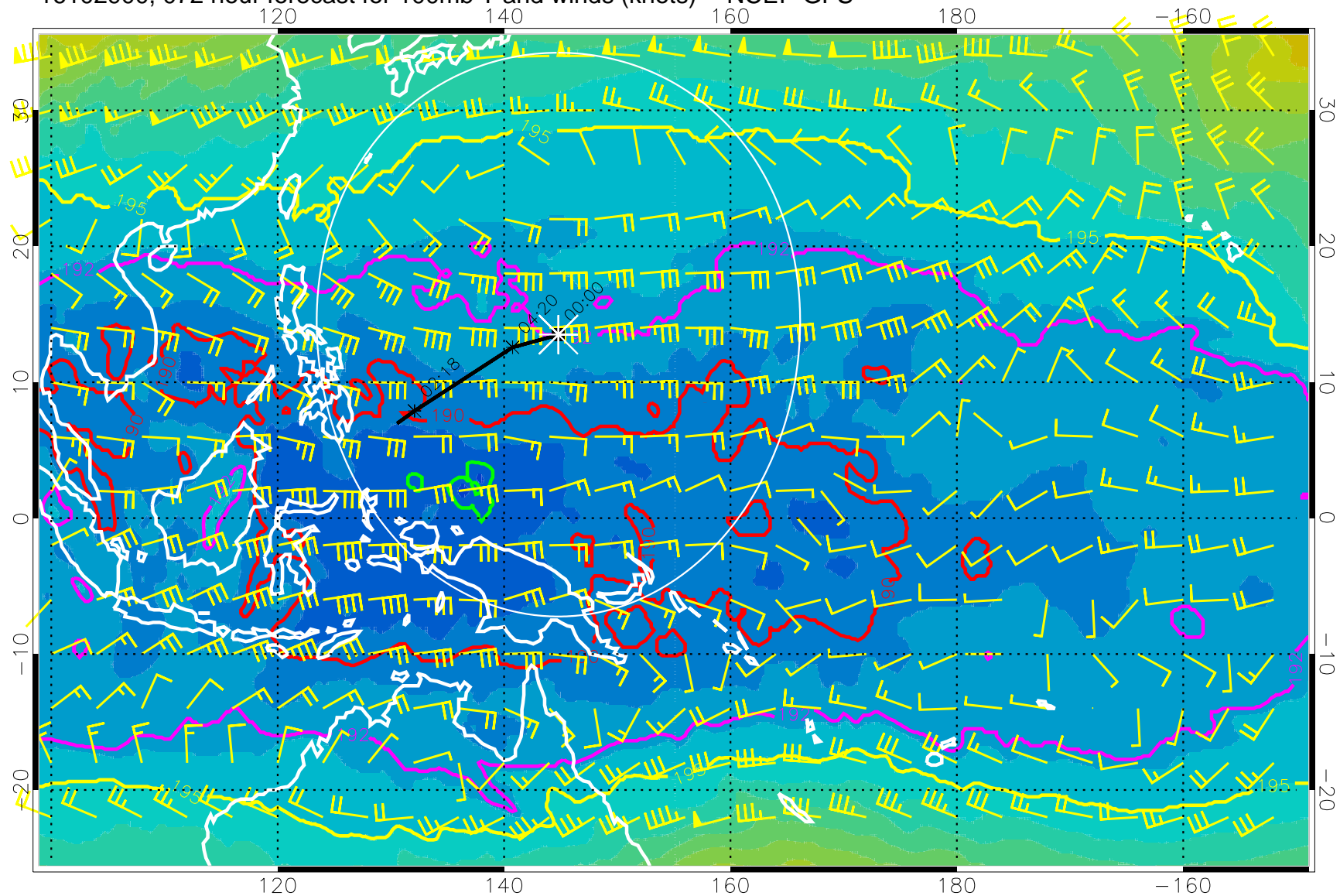
16102900, 072 hour forecast for 100mb T and winds (knots) -- NCEP GFS
