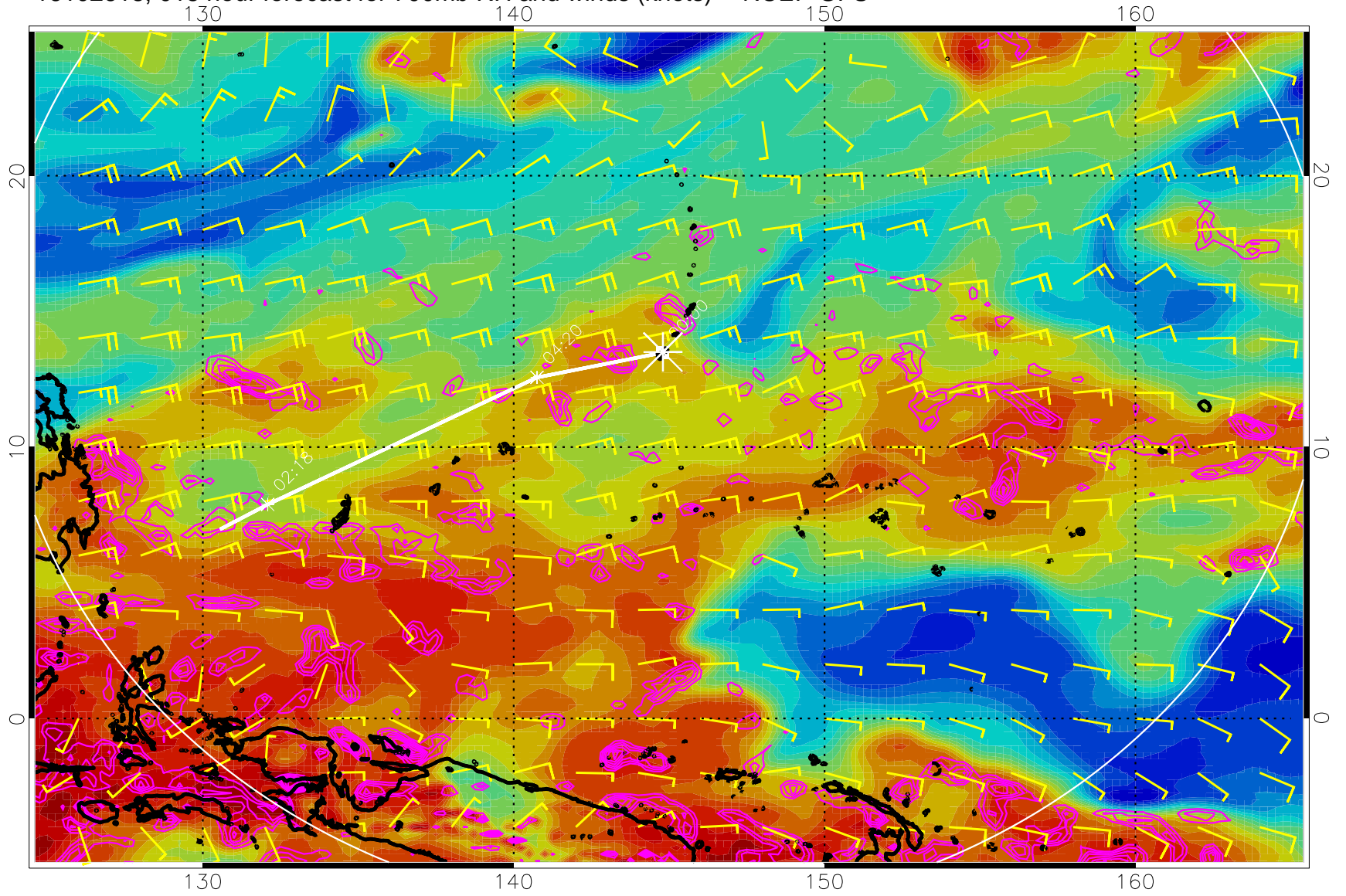
16102618, 018 hour forecast for 700mb RH and winds (knots) -- NCEP GFS
