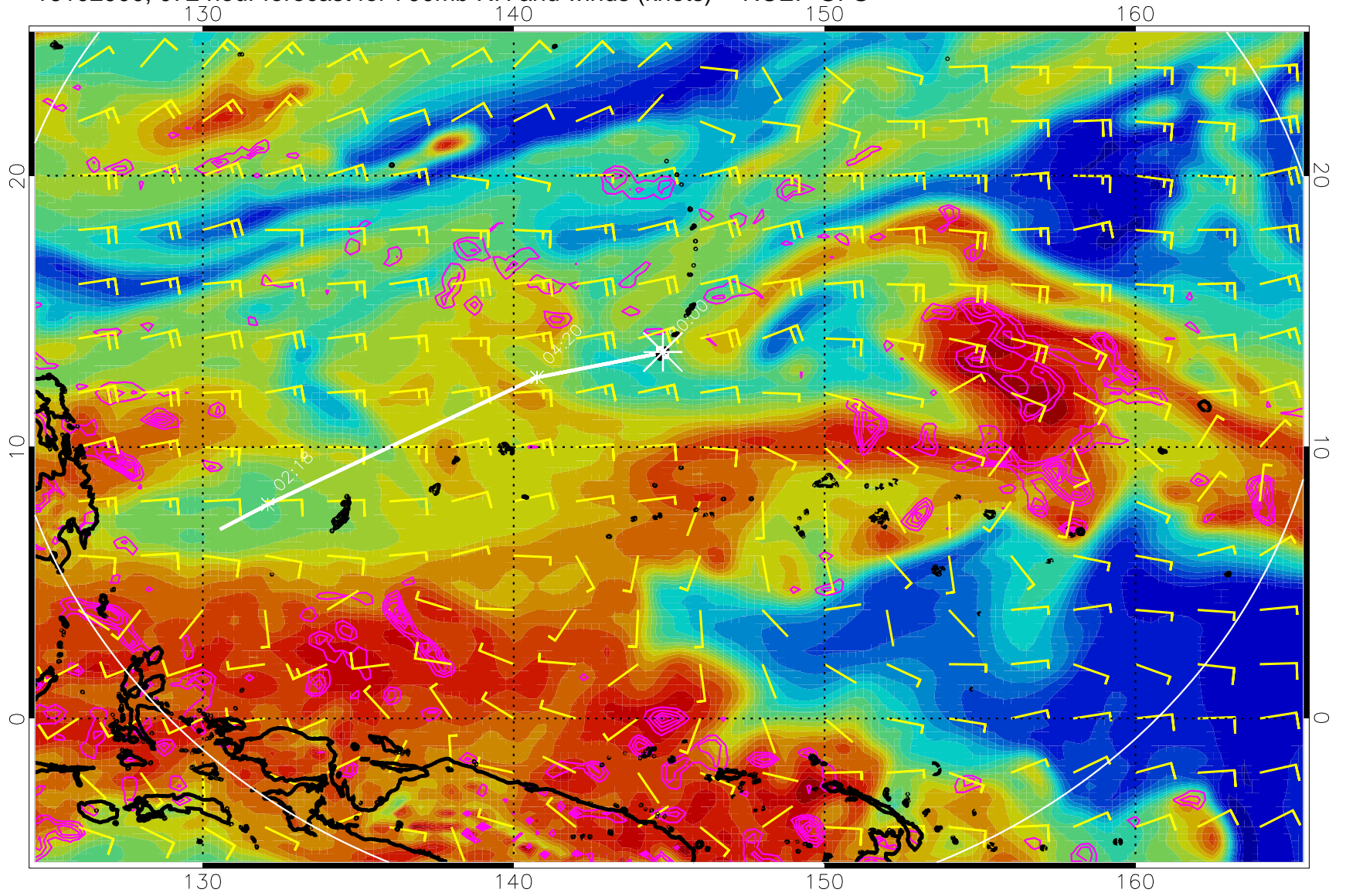
16102900, 072 hour forecast for 700mb RH and winds (knots) -- NCEP GFS
