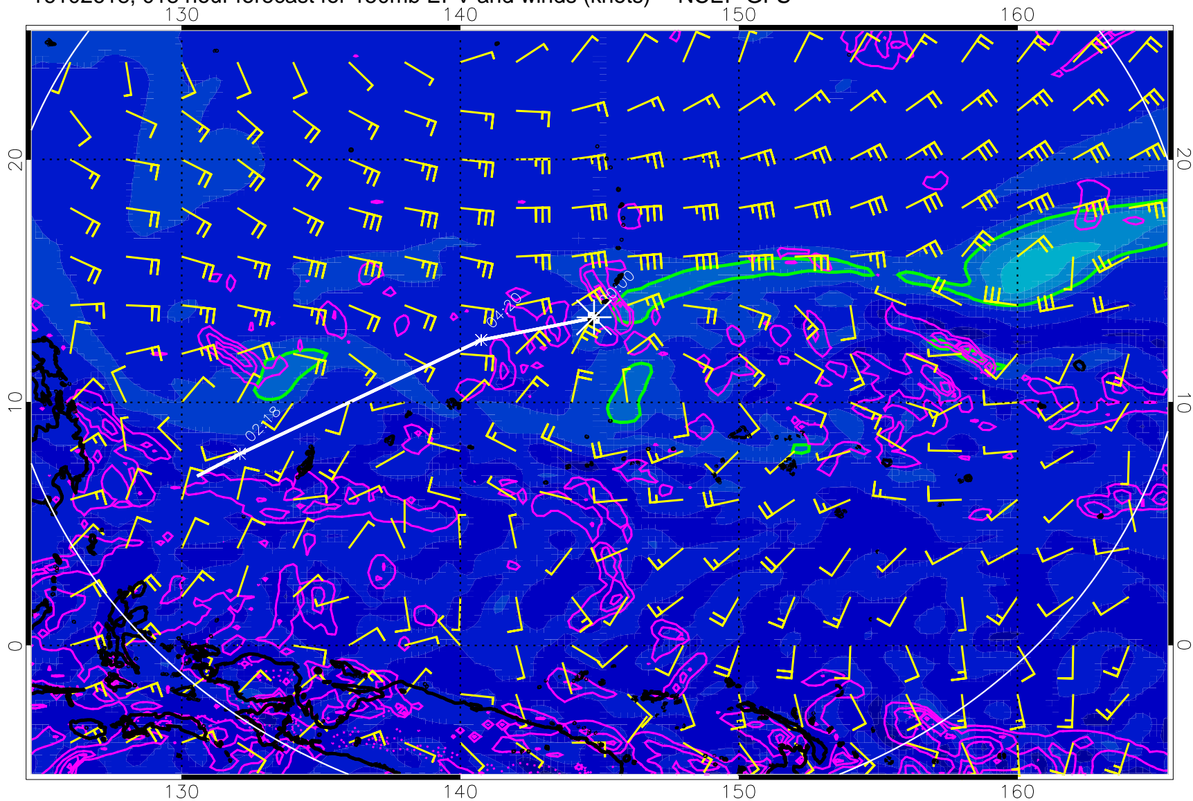
16102618, 018 hour forecast for 150mb EPV and winds (knots) -- NCEP GFS
