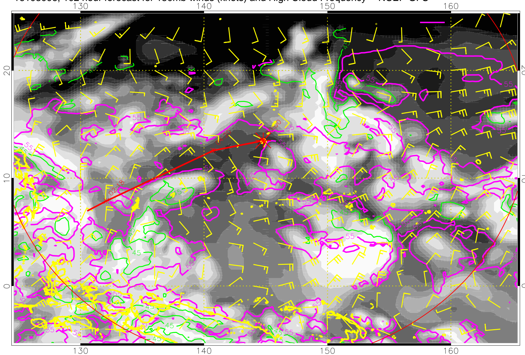
16103006, 102 hour forecast for 150mb winds (knots) and High Cloud Frequency -- NCEP GFS
