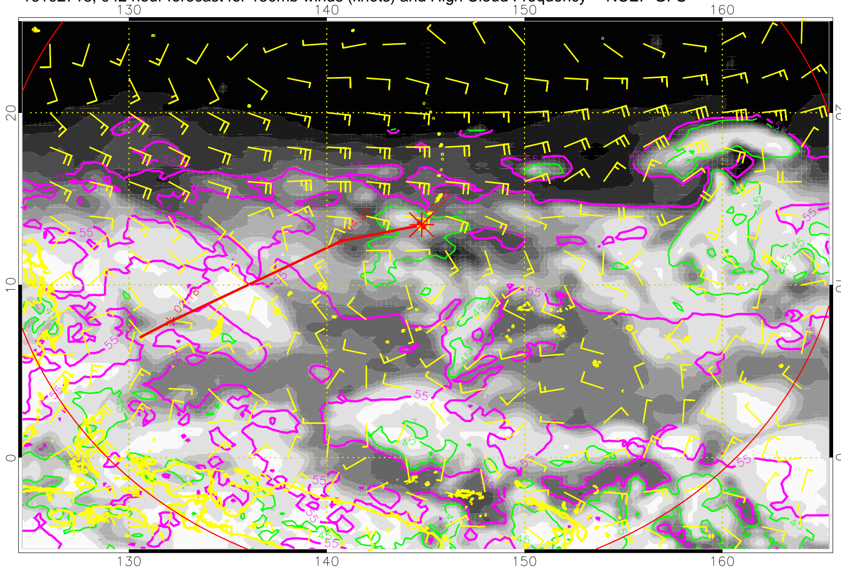
16102718, 042 hour forecast for 150mb winds (knots) and High Cloud Frequency -- NCEP GFS
