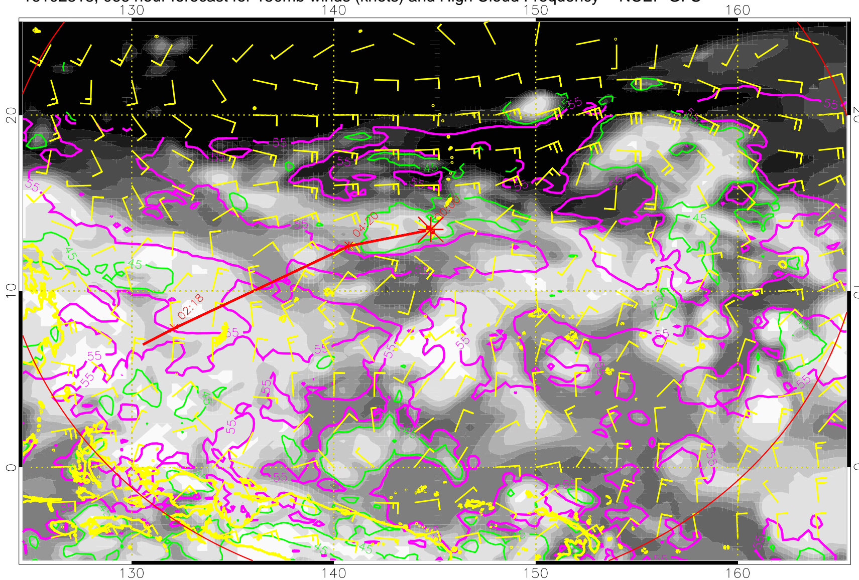
16102818, 066 hour forecast for 150mb winds (knots) and High Cloud Frequency -- NCEP GFS
