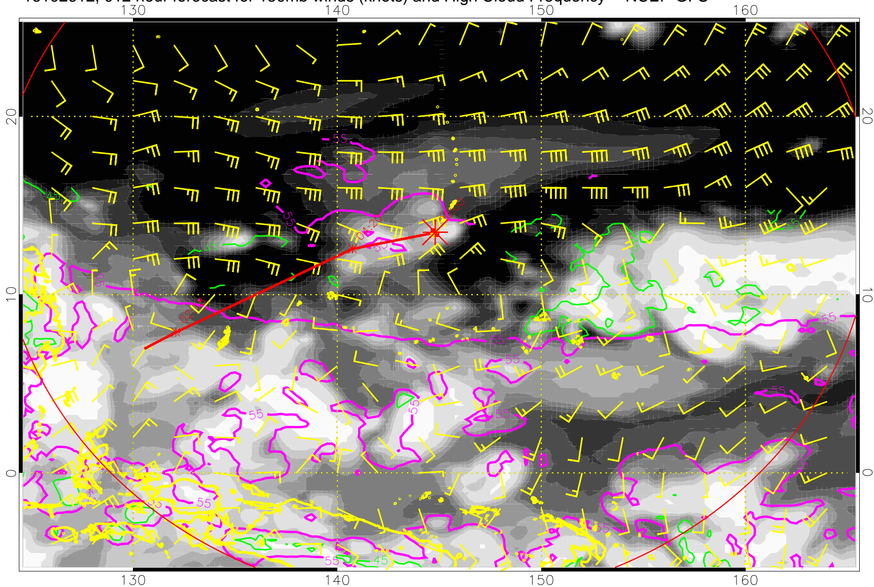
16102612, 012 hour forecast for 150mb winds (knots) and High Cloud Frequency -- NCEP GFS
