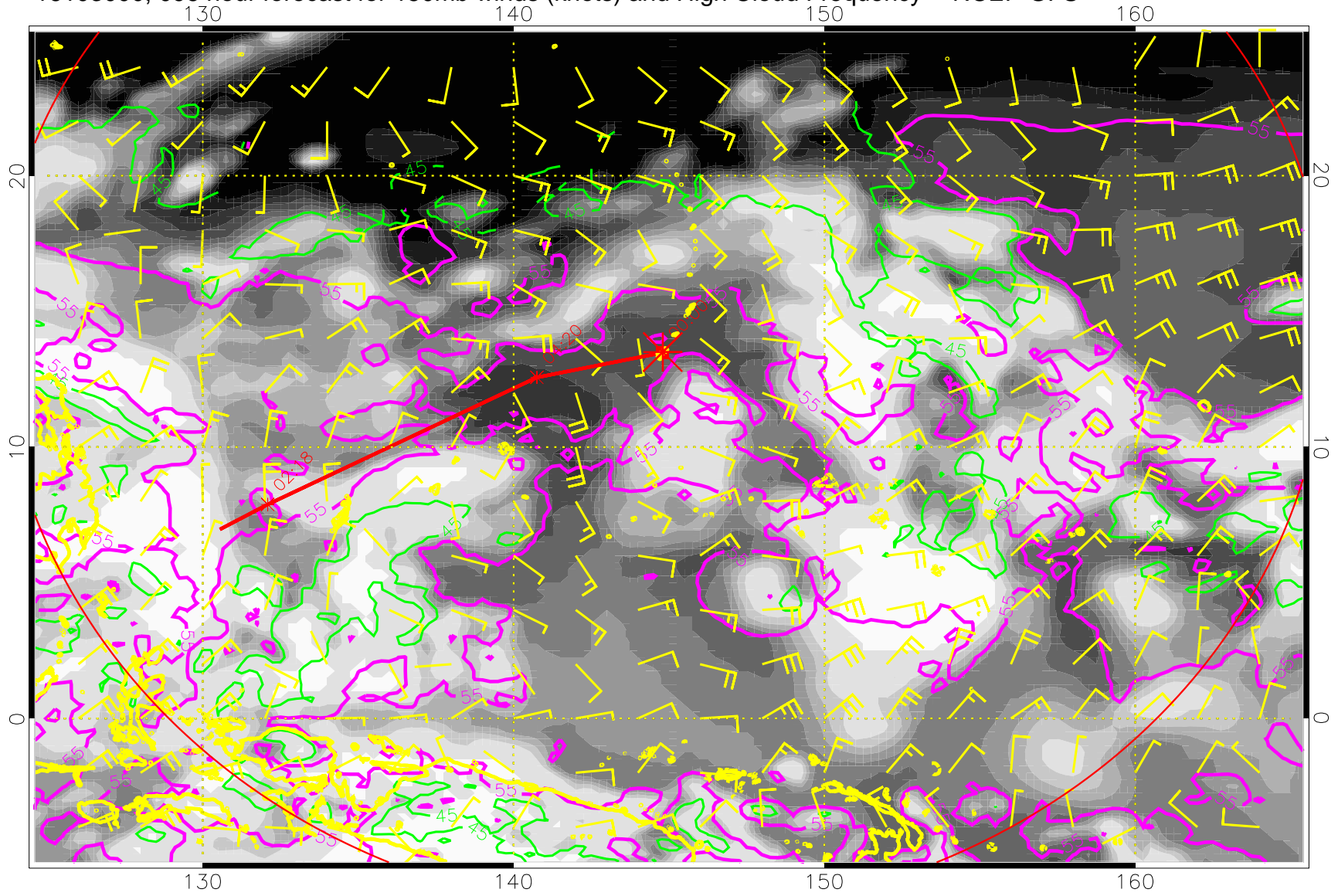
16103000, 096 hour forecast for 150mb winds (knots) and High Cloud Frequency -- NCEP GFS
