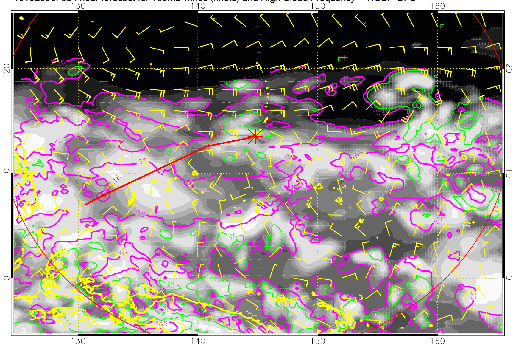
16102806, 054 hour forecast for 150mb winds (knots) and High Cloud Frequency -- NCEP GFS
