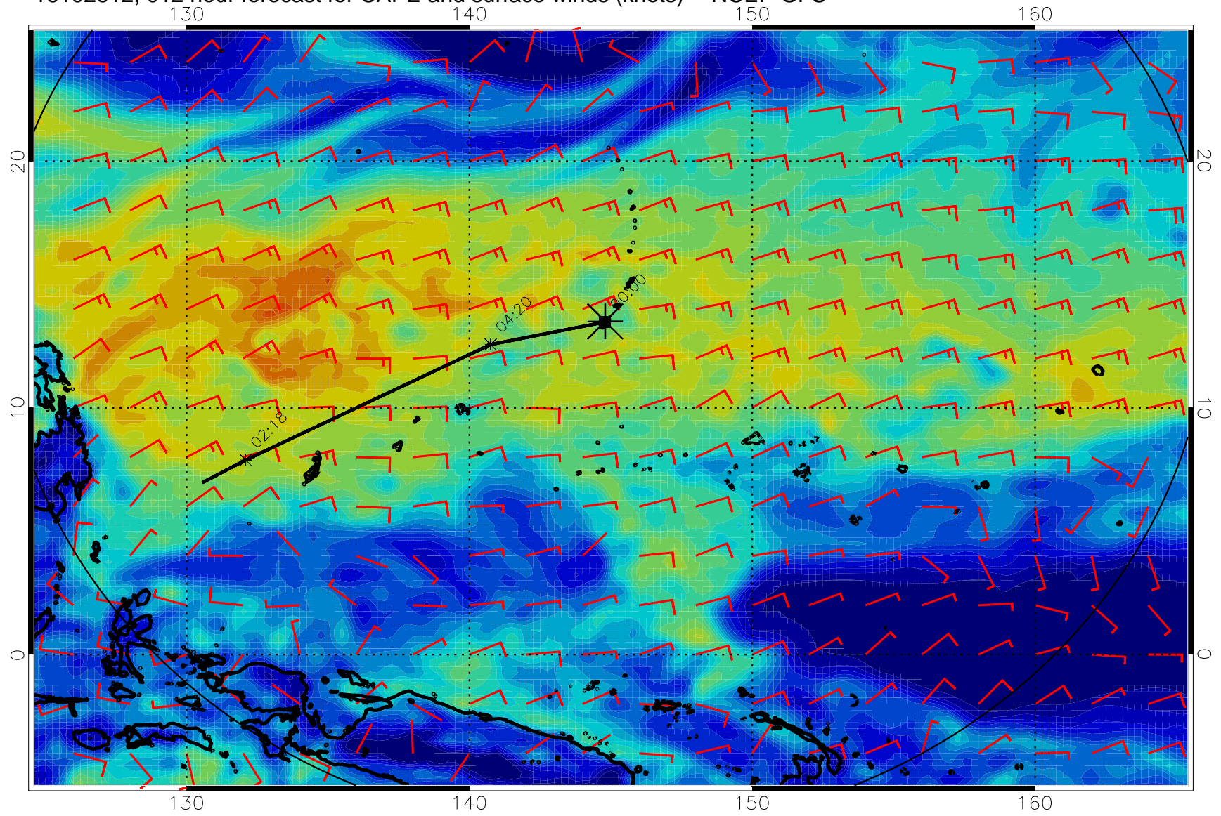
16102612, 012 hour forecast for CAPE and surface winds (knots) -- NCEP GFS
