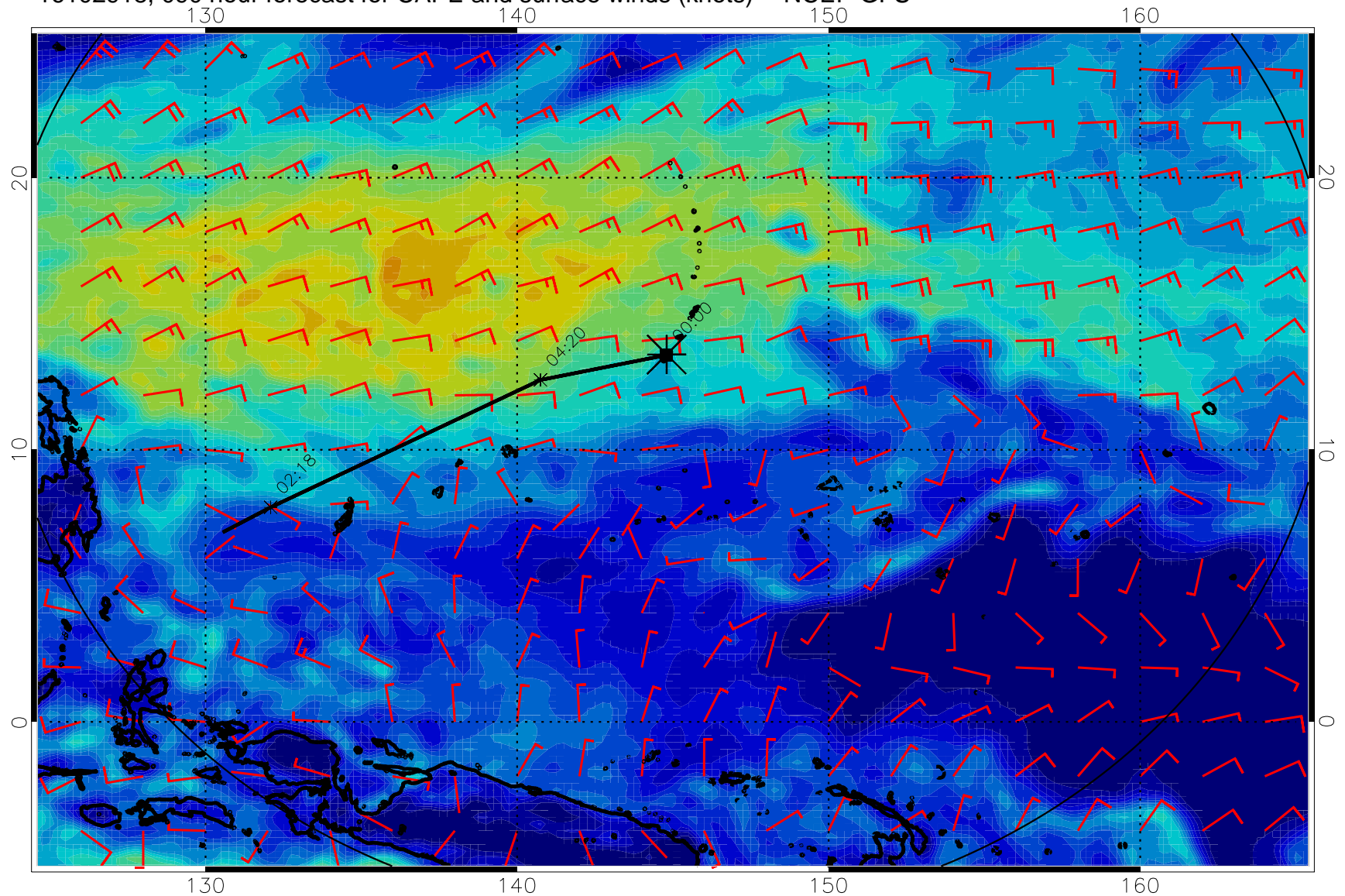
16102918, 090 hour forecast for CAPE and surface winds (knots) -- NCEP GFS
