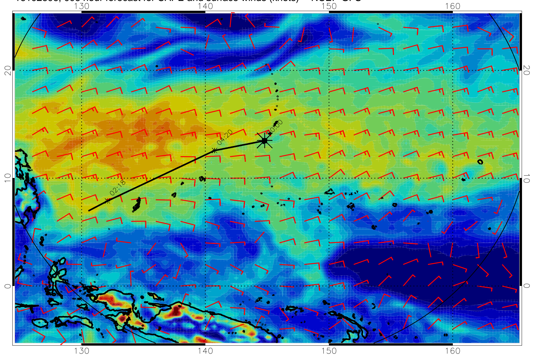
16102606, 006 hour forecast for CAPE and surface winds (knots) -- NCEP GFS
