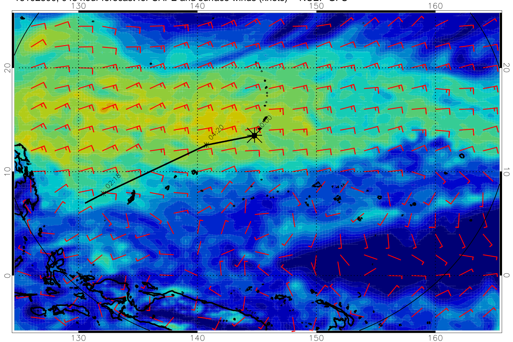
16102800, 048 hour forecast for CAPE and surface winds (knots) -- NCEP GFS
