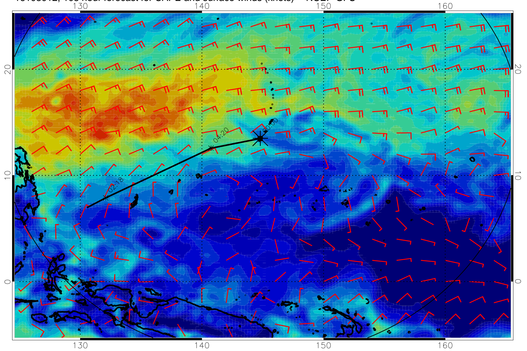
16103012, 108 hour forecast for CAPE and surface winds (knots) -- NCEP GFS
