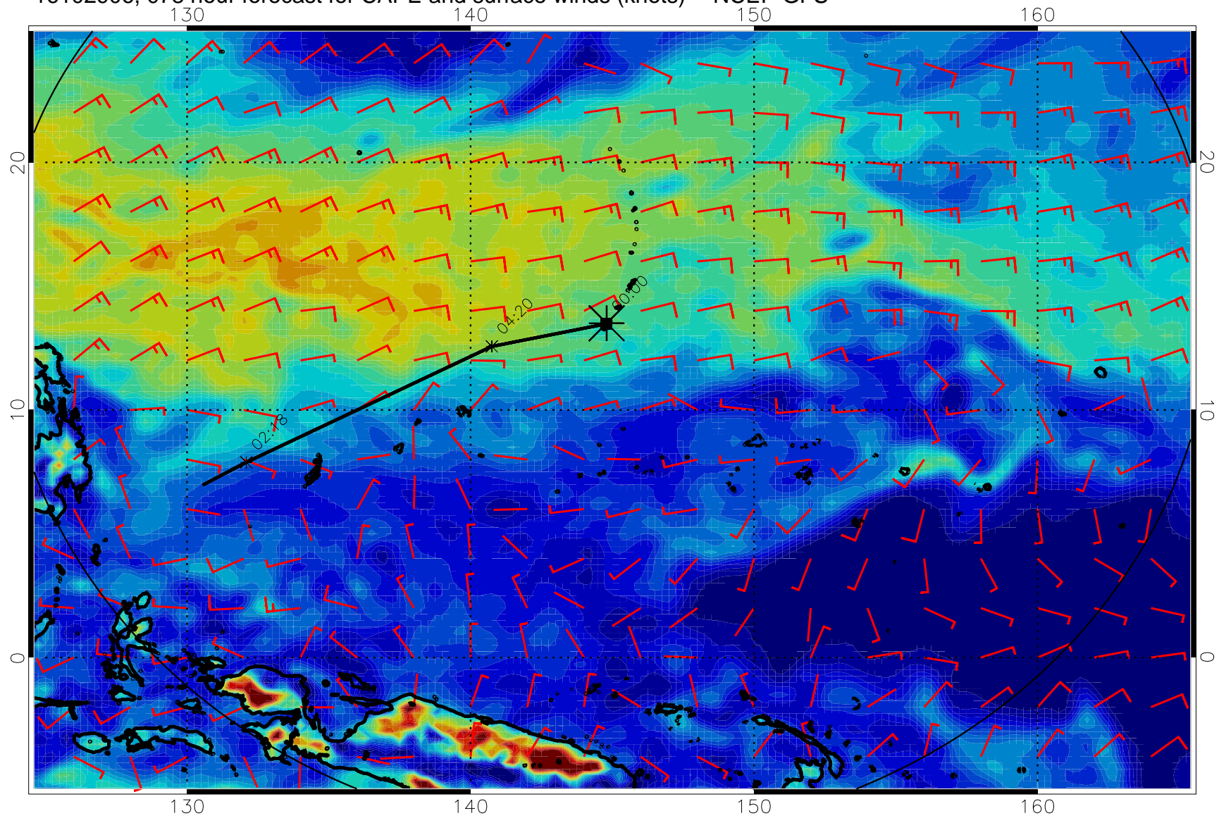
16102906, 078 hour forecast for CAPE and surface winds (knots) -- NCEP GFS
