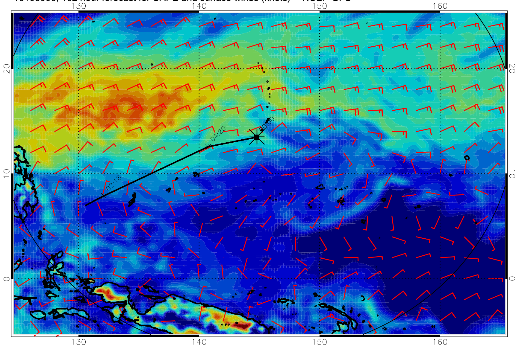
16103006, 102 hour forecast for CAPE and surface winds (knots) -- NCEP GFS
