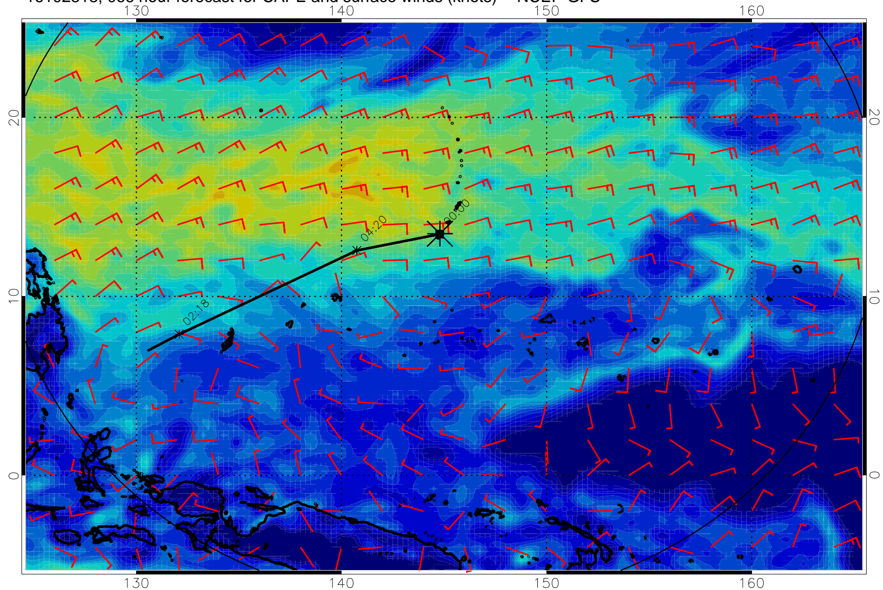
16102818, 066 hour forecast for CAPE and surface winds (knots) -- NCEP GFS
