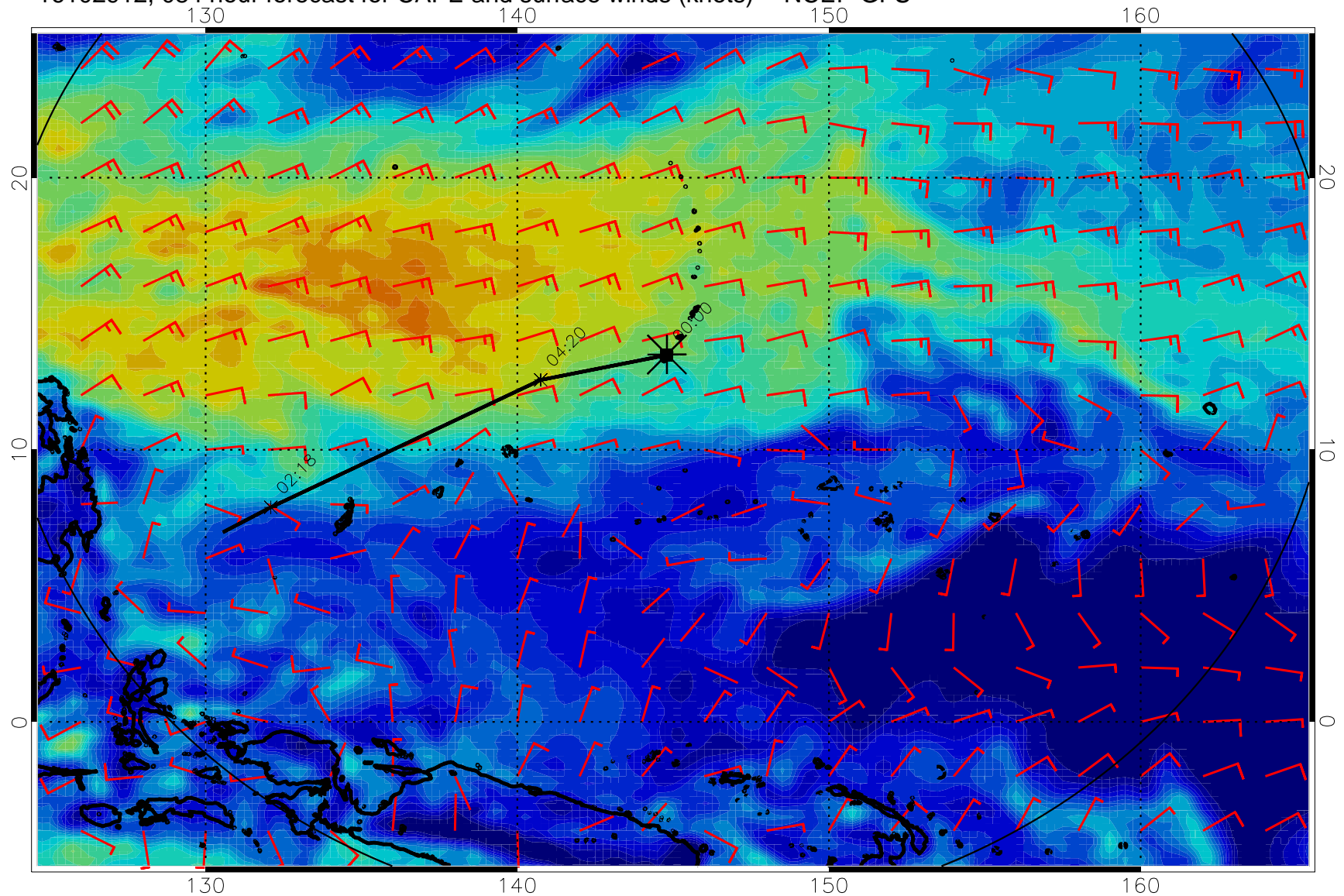
16102912, 084 hour forecast for CAPE and surface winds (knots) -- NCEP GFS
