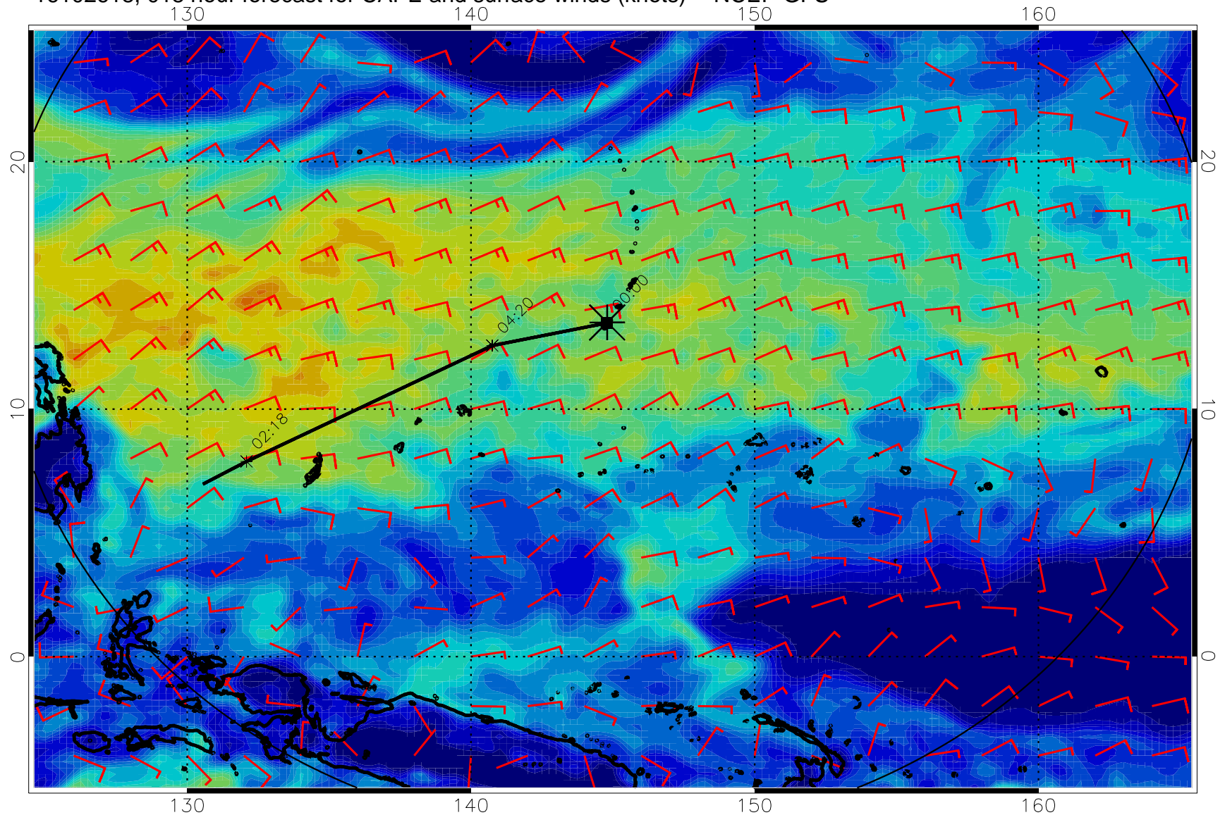
16102618, 018 hour forecast for CAPE and surface winds (knots) -- NCEP GFS
