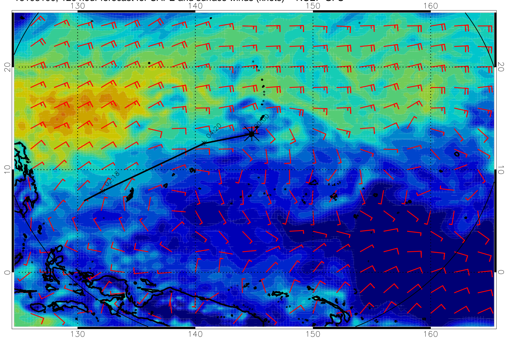
16103100, 120 hour forecast for CAPE and surface winds (knots) -- NCEP GFS
