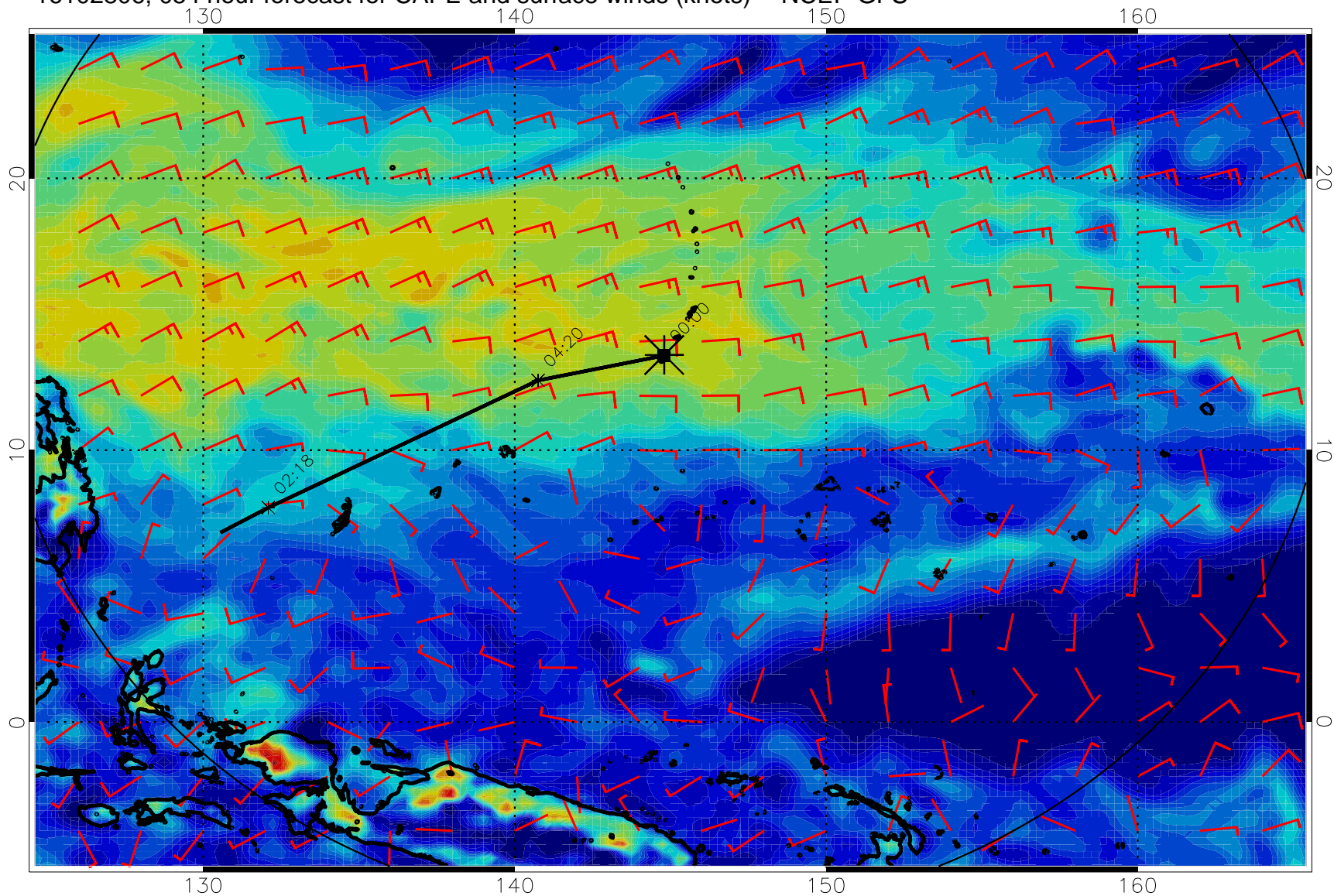
16102806, 054 hour forecast for CAPE and surface winds (knots) -- NCEP GFS
