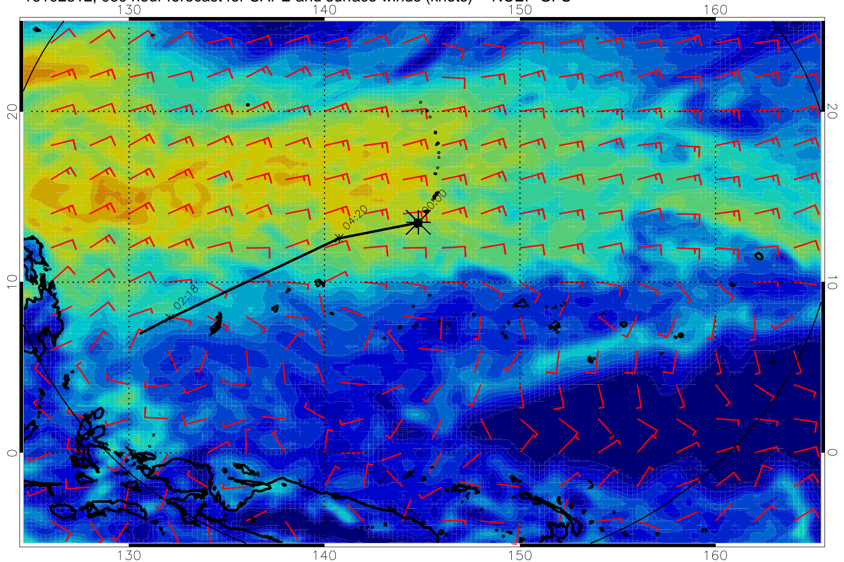
16102812, 060 hour forecast for CAPE and surface winds (knots) -- NCEP GFS
