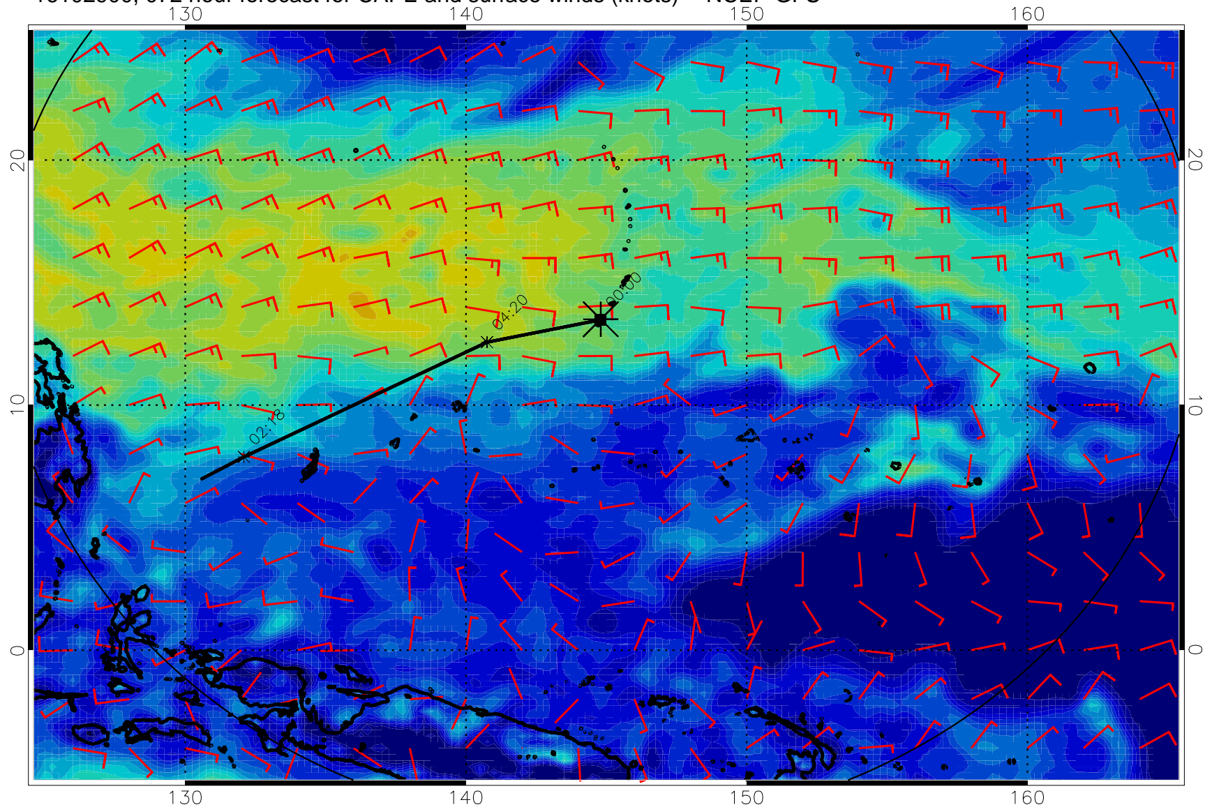
16102900, 072 hour forecast for CAPE and surface winds (knots) -- NCEP GFS
