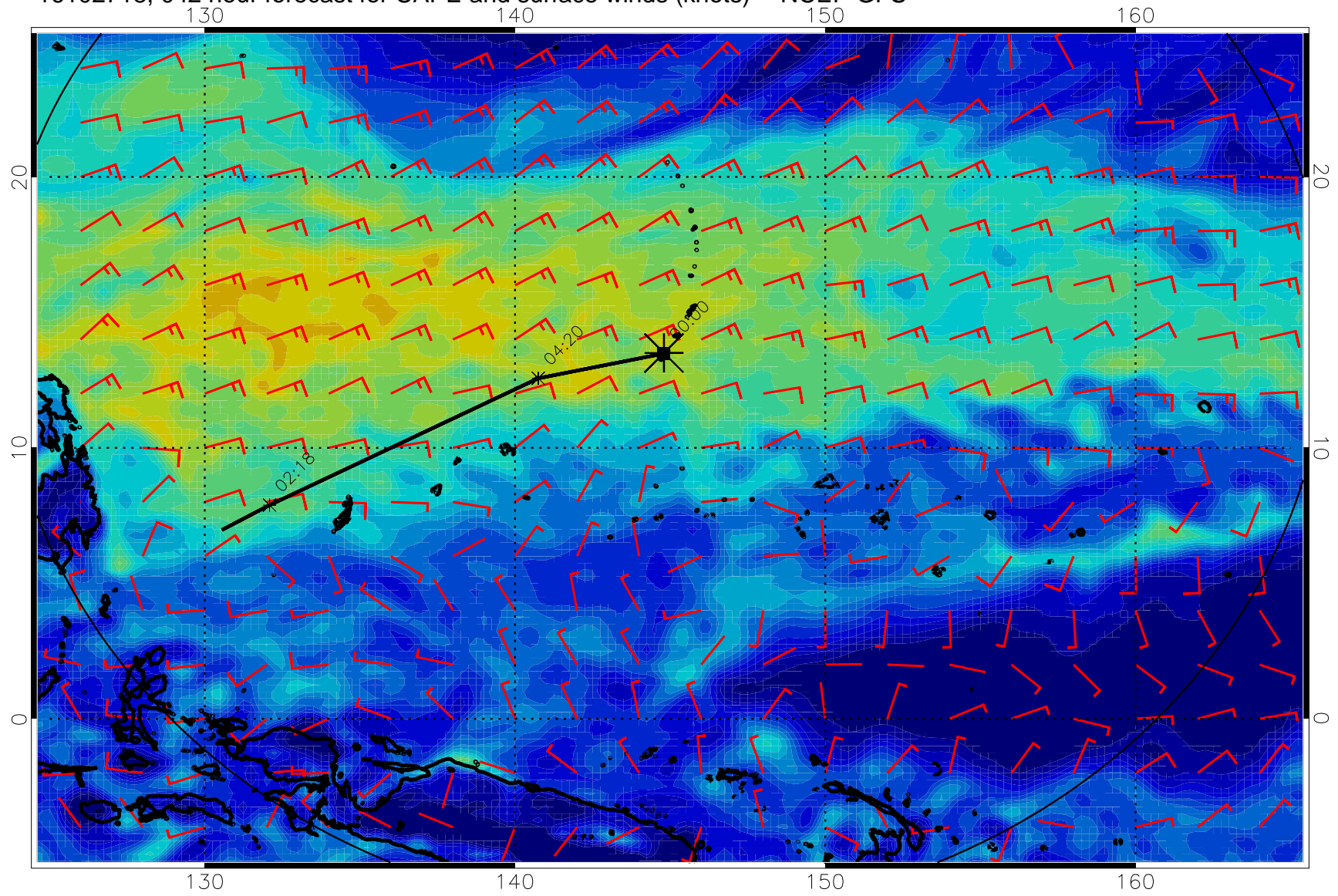
16102718, 042 hour forecast for CAPE and surface winds (knots) -- NCEP GFS
