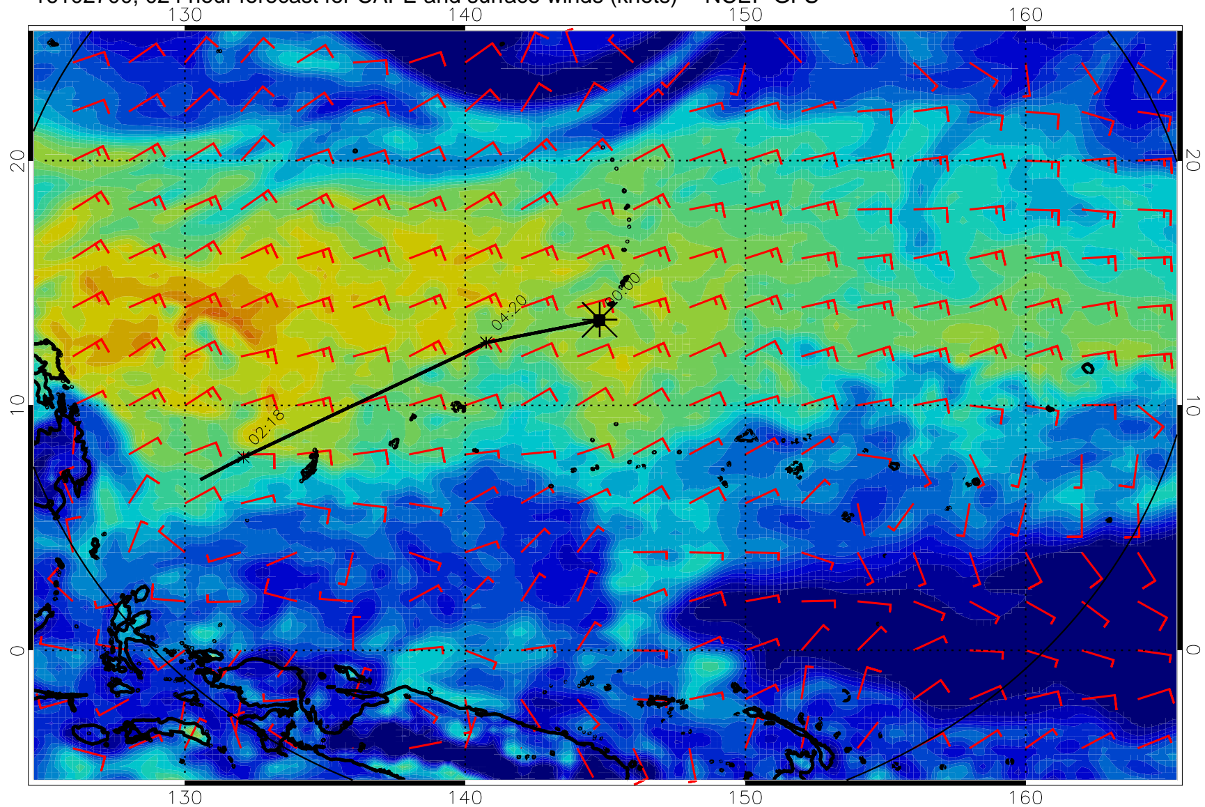
16102700, 024 hour forecast for CAPE and surface winds (knots) -- NCEP GFS
