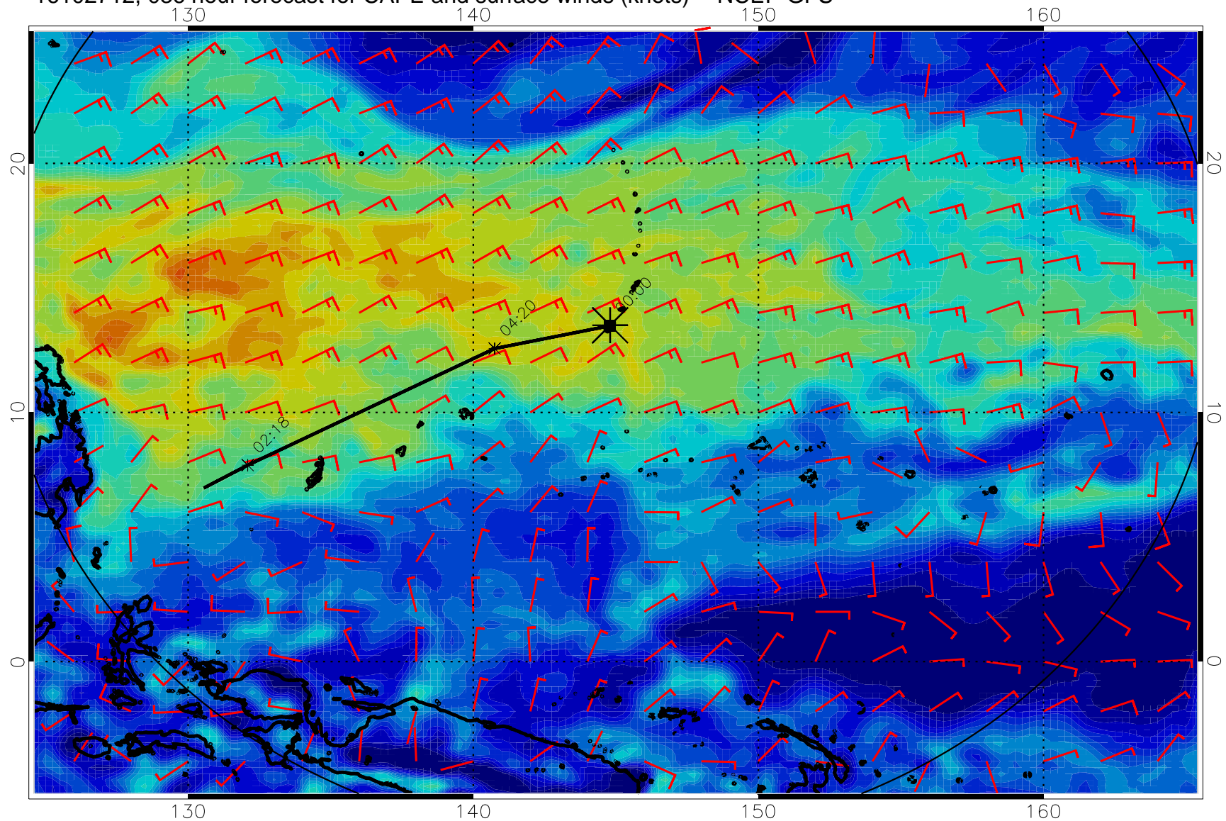
16102712, 036 hour forecast for CAPE and surface winds (knots) -- NCEP GFS
