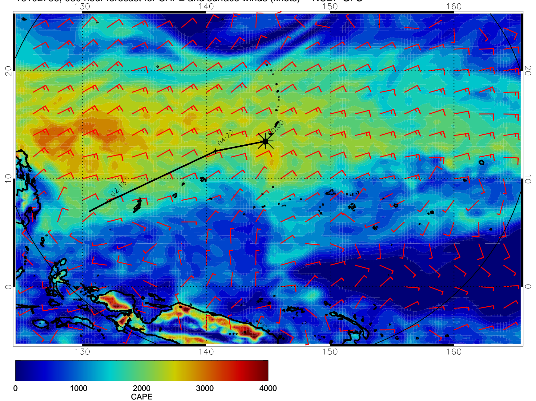
16102706, 030 hour forecast for CAPE and surface winds (knots) -- NCEP GFS
