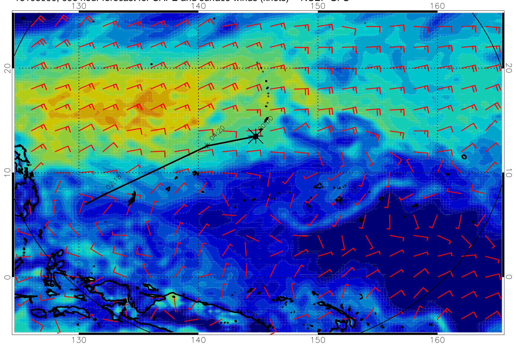
16103000, 096 hour forecast for CAPE and surface winds (knots) -- NCEP GFS
