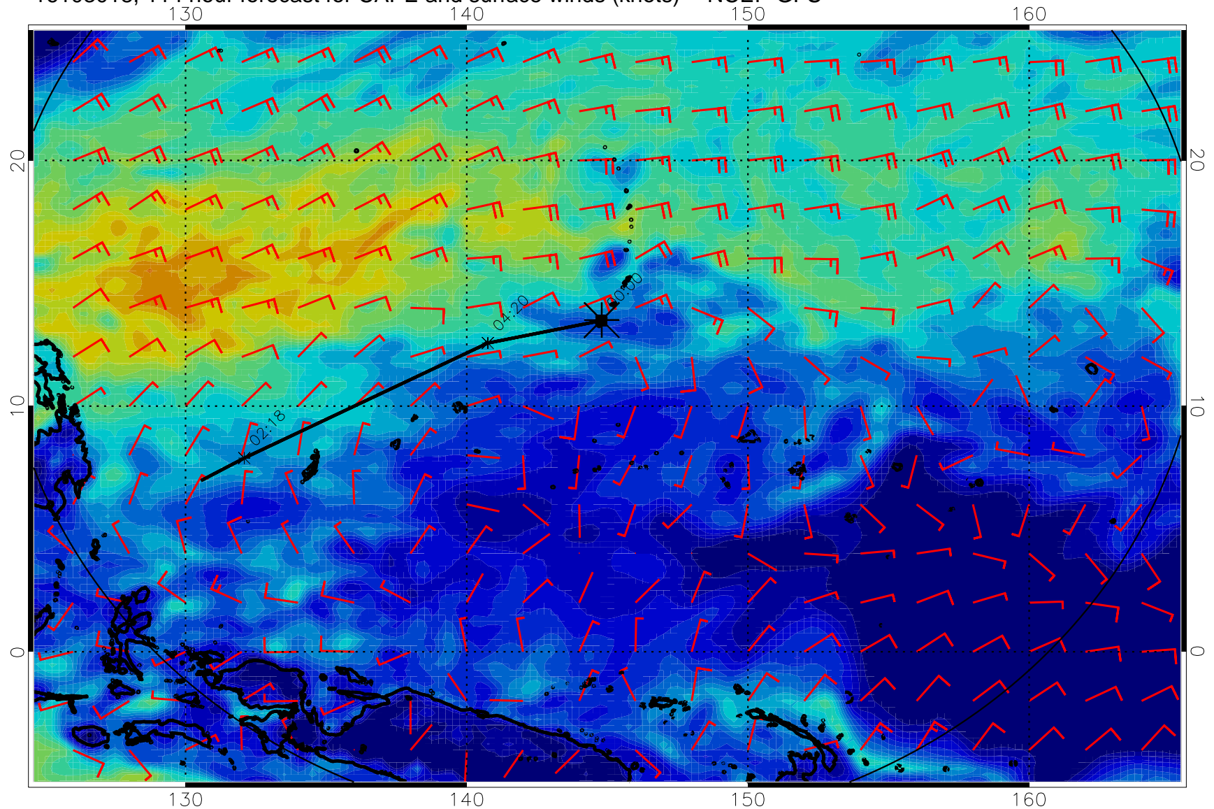
16103018, 114 hour forecast for CAPE and surface winds (knots) -- NCEP GFS
