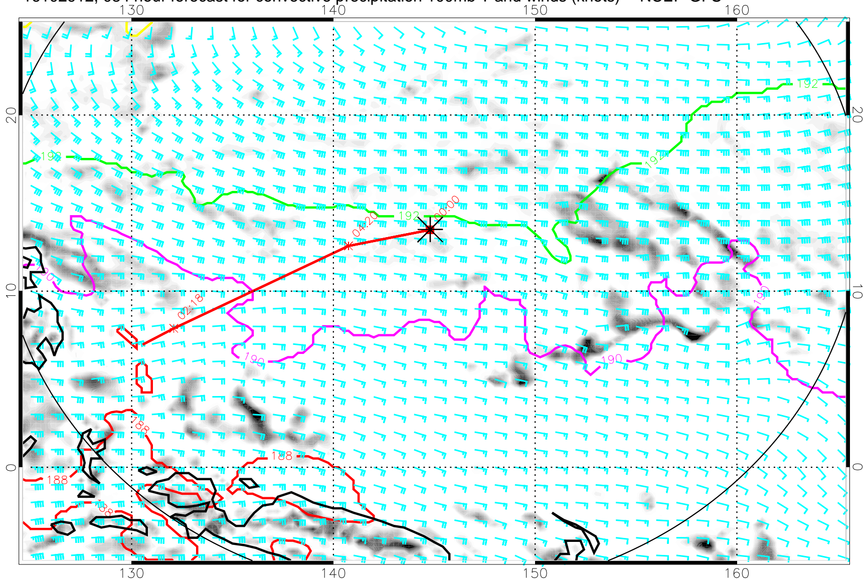
16102912, 084 hour forecast for convective precipitation 100mb T and winds (knots) -- NCEP GFS
