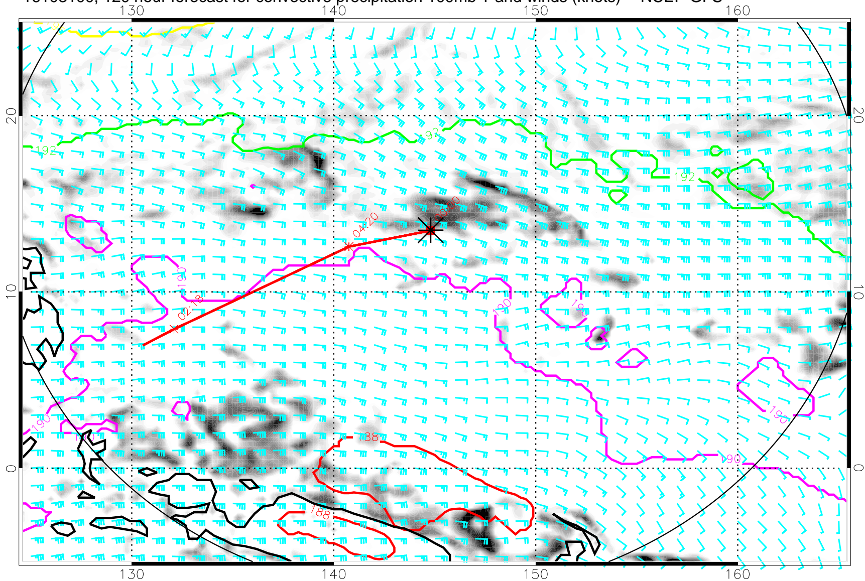
16103100, 120 hour forecast for convective precipitation 100mb T and winds (knots) -- NCEP GFS
