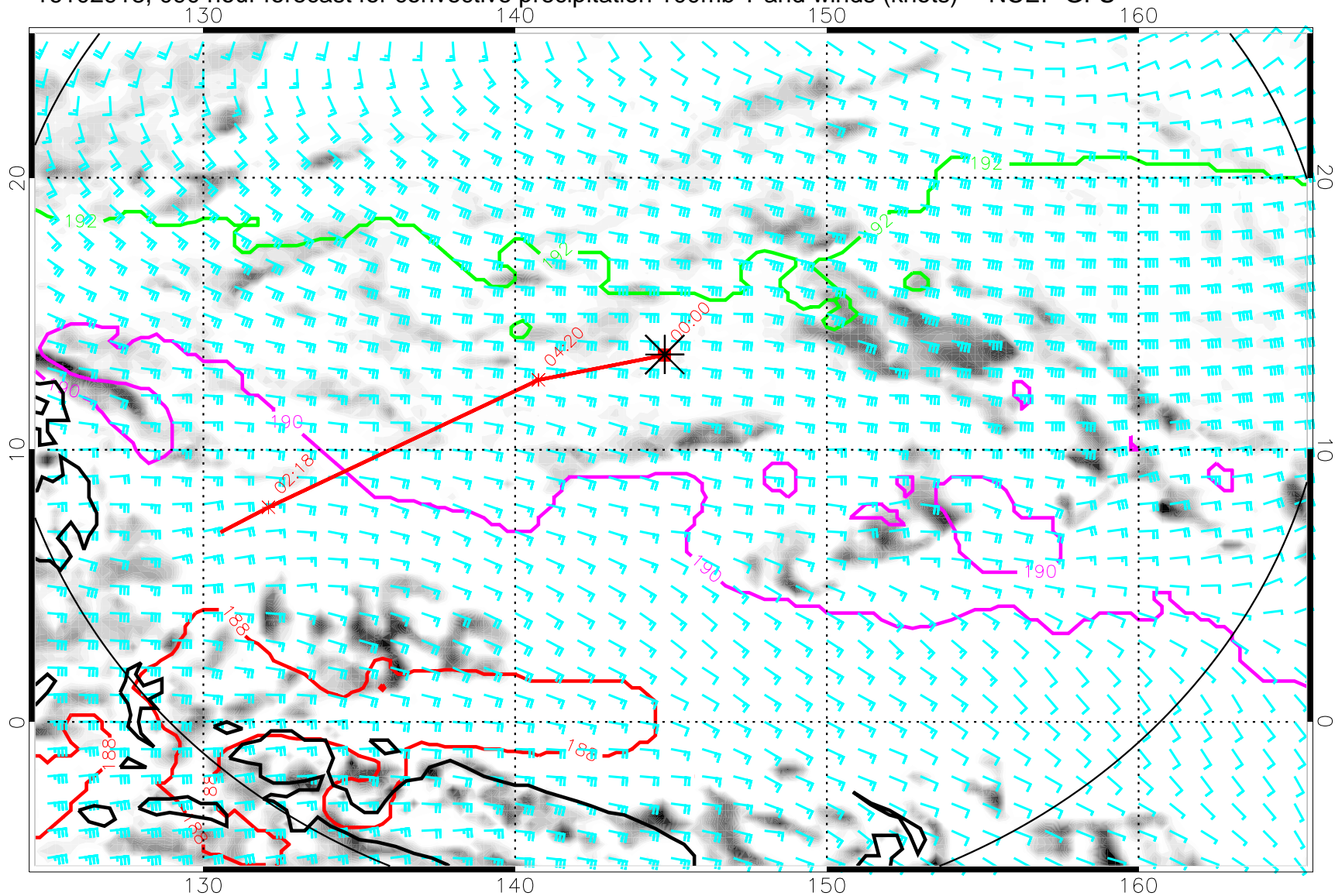
16102918, 090 hour forecast for convective precipitation 100mb T and winds (knots) -- NCEP GFS
