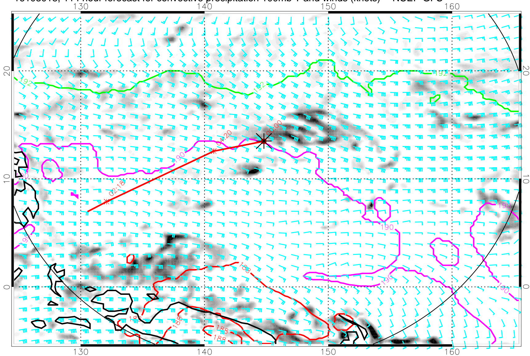
16103018, 114 hour forecast for convective precipitation 100mb T and winds (knots) -- NCEP GFS
