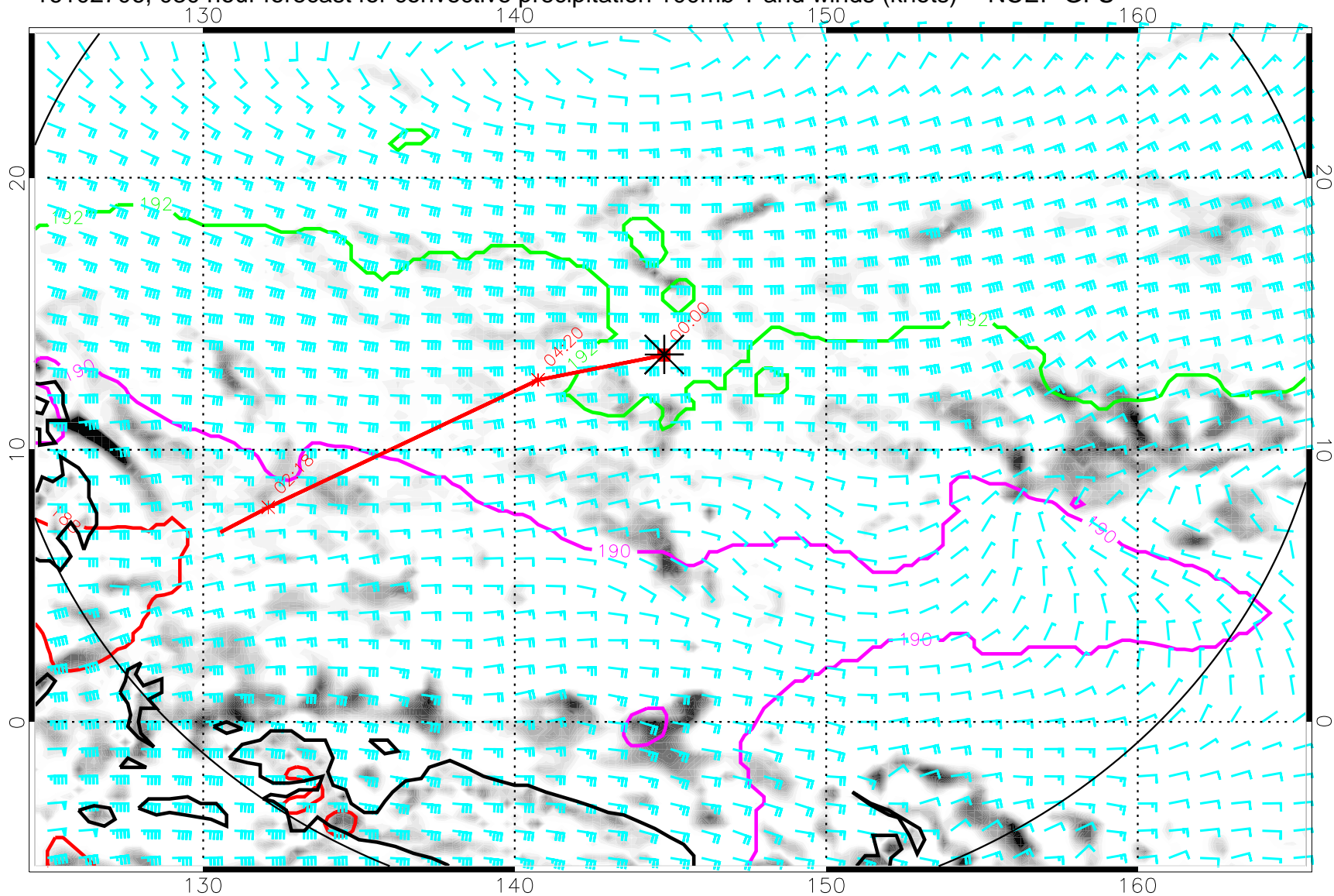
16102706, 030 hour forecast for convective precipitation 100mb T and winds (knots) -- NCEP GFS
