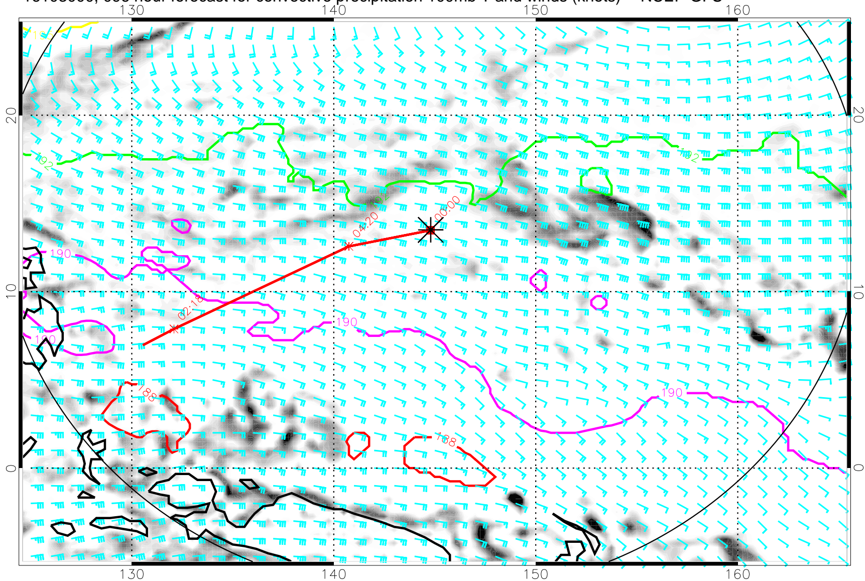
16103000, 096 hour forecast for convective precipitation 100mb T and winds (knots) -- NCEP GFS
