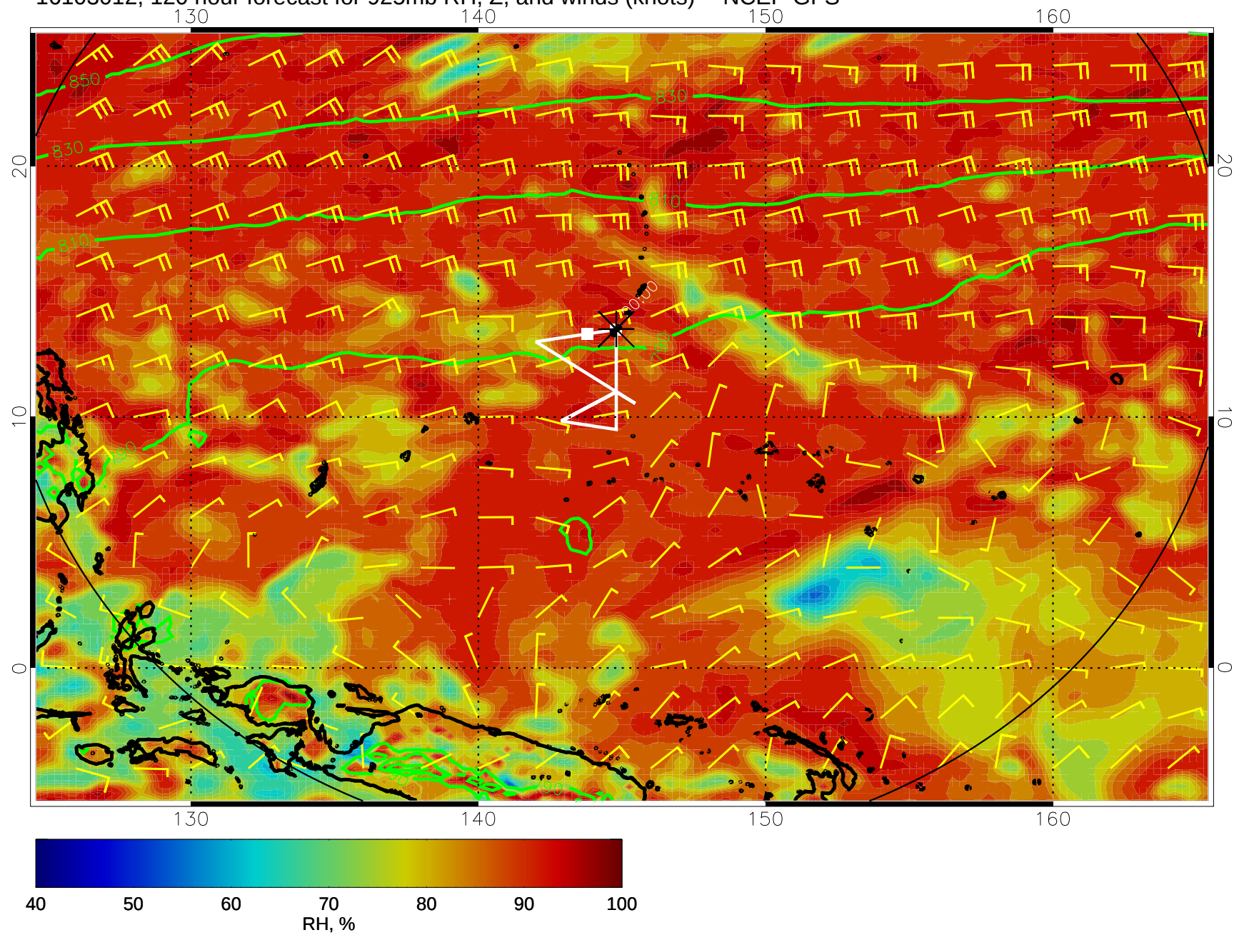
16103012, 120 hour forecast for 925mb RH, Z, and winds (knots) -- NCEP GFS
