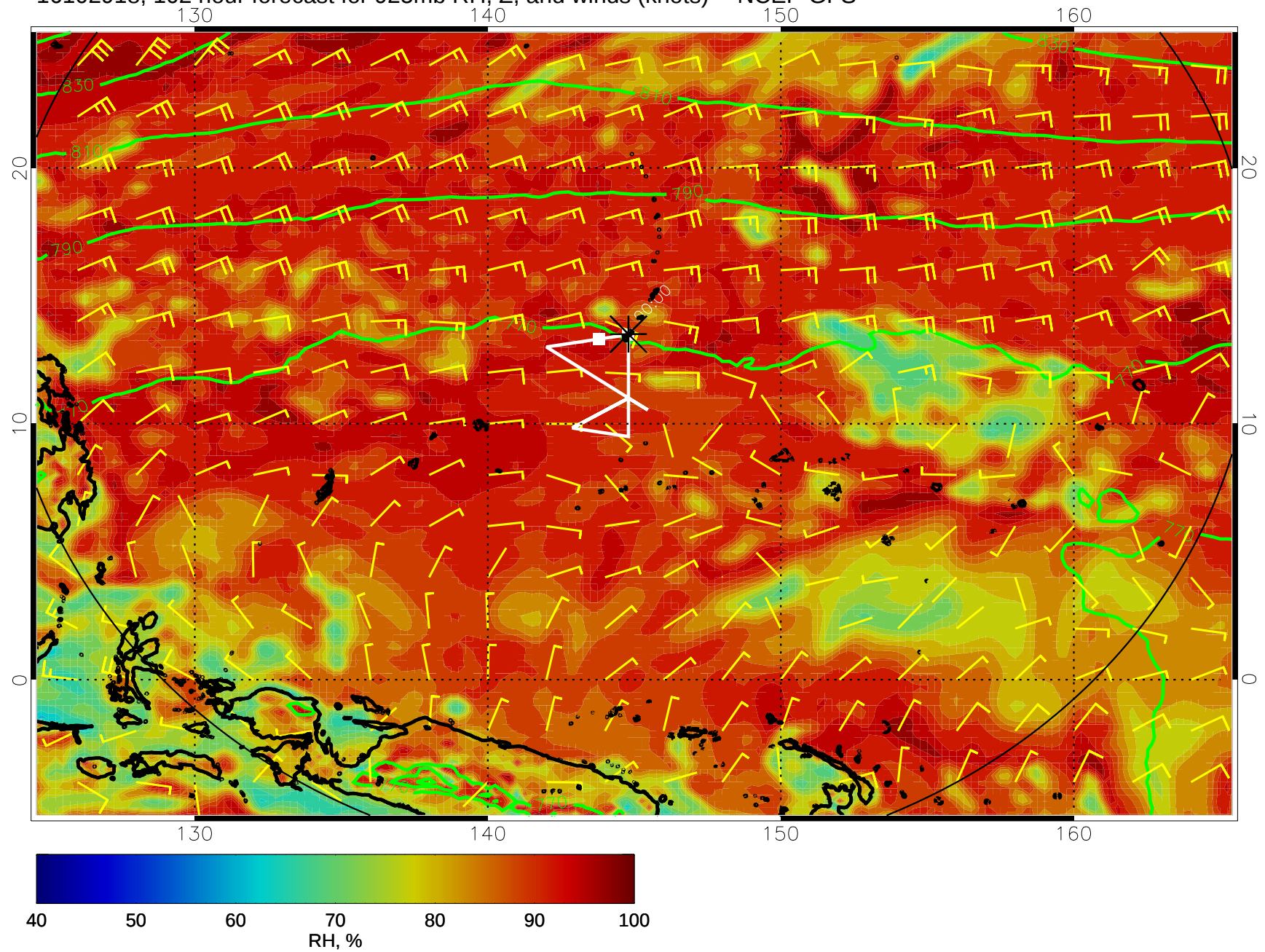
16102918, 102 hour forecast for 925mb RH, Z, and winds (knots) -- NCEP GFS
