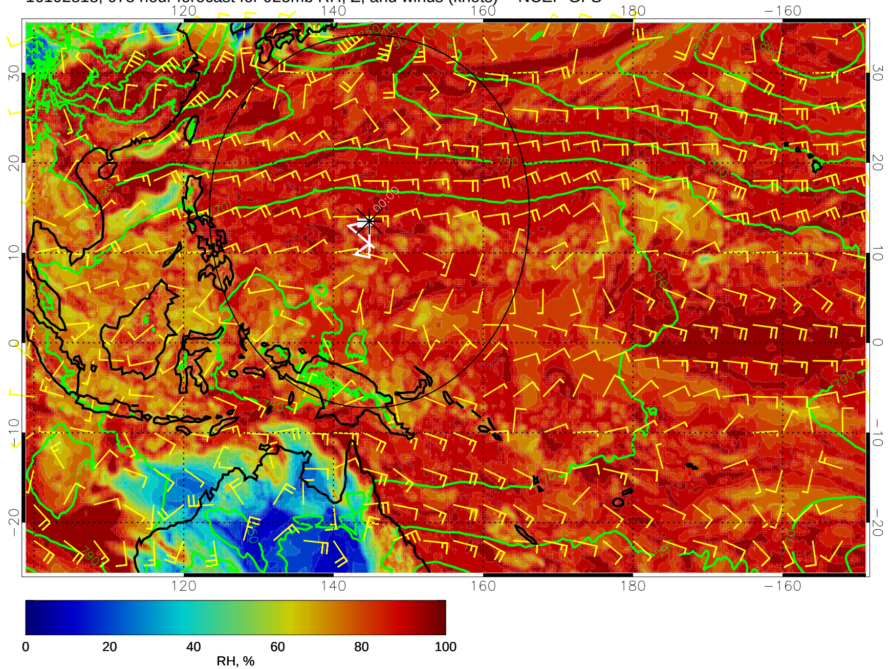
16102818, 078 hour forecast for 925mb RH, Z, and winds (knots) -- NCEP GFS
