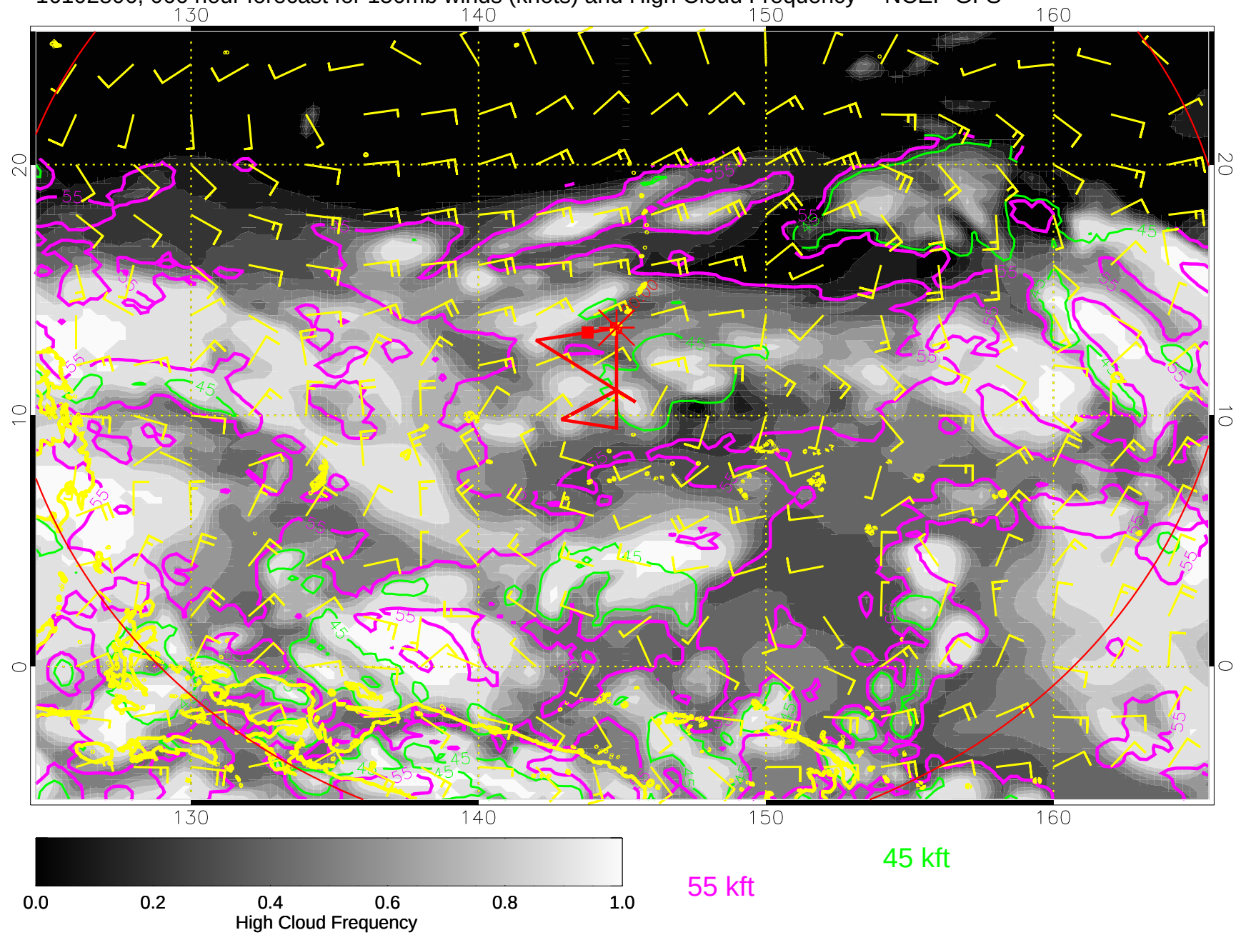
16102806, 066 hour forecast for 150mb winds (knots) and High Cloud Frequency -- NCEP GFS
