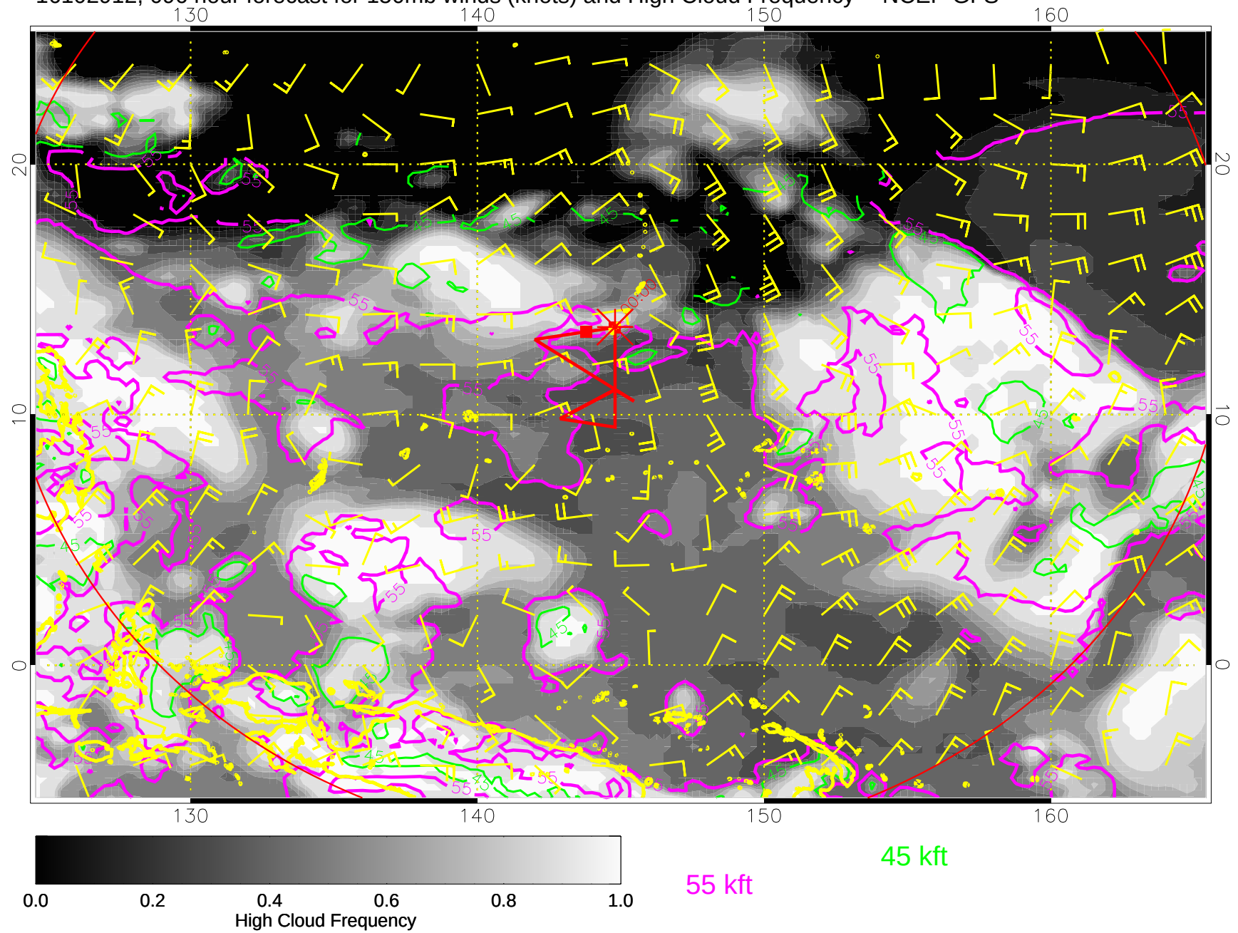
16102912, 096 hour forecast for 150mb winds (knots) and High Cloud Frequency -- NCEP GFS
