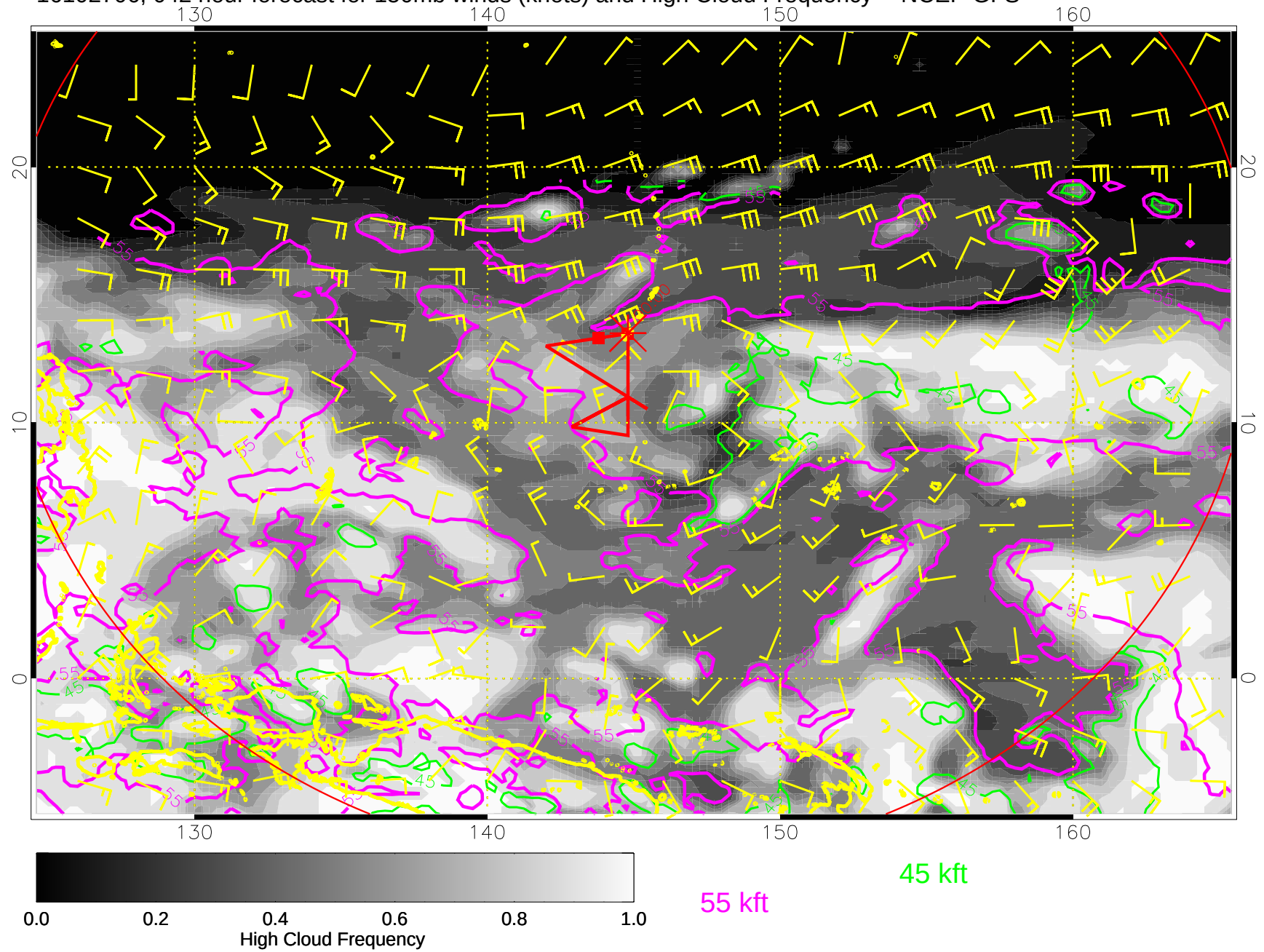
16102706, 042 hour forecast for 150mb winds (knots) and High Cloud Frequency -- NCEP GFS
