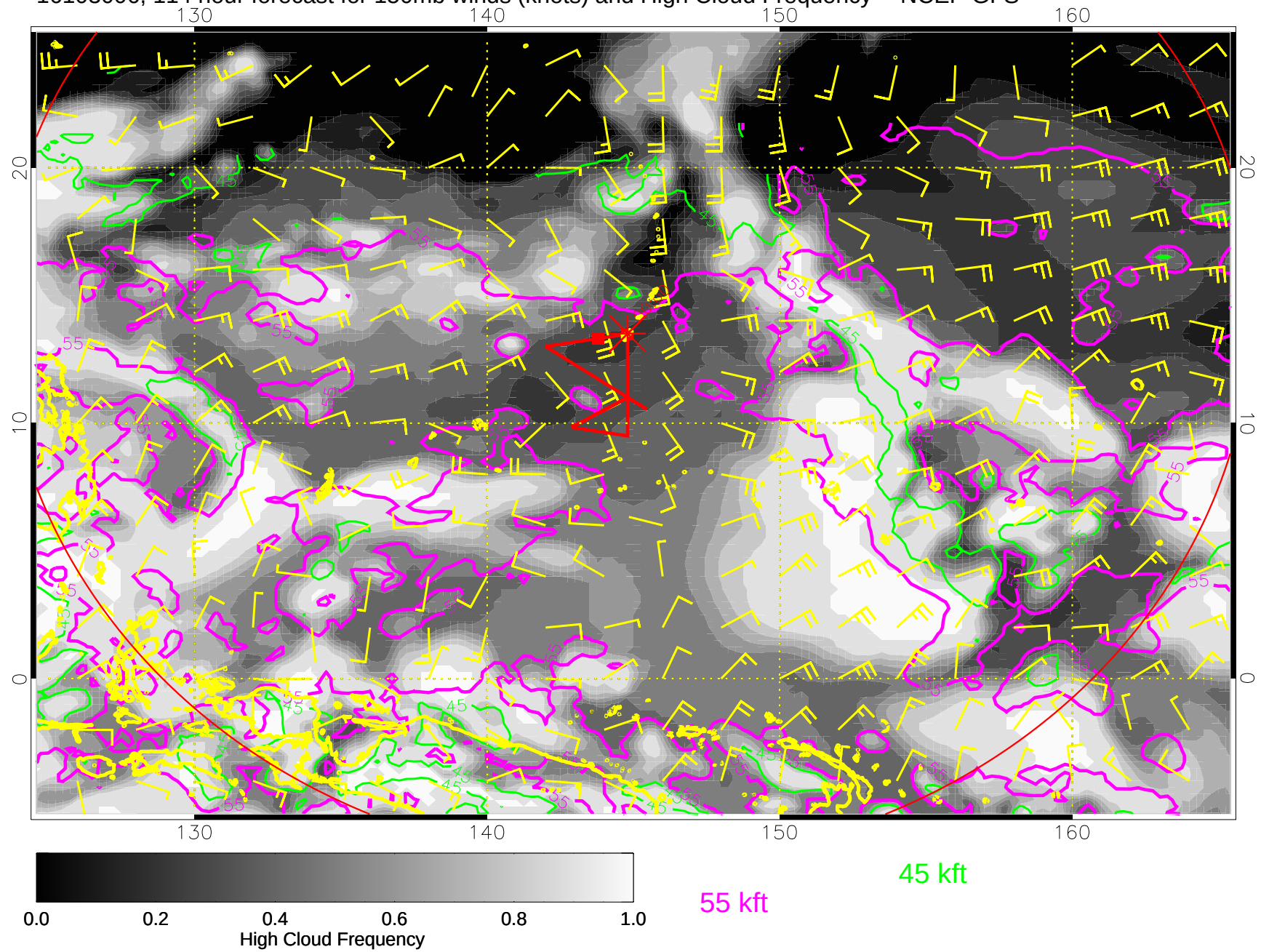
16103006, 114 hour forecast for 150mb winds (knots) and High Cloud Frequency -- NCEP GFS
