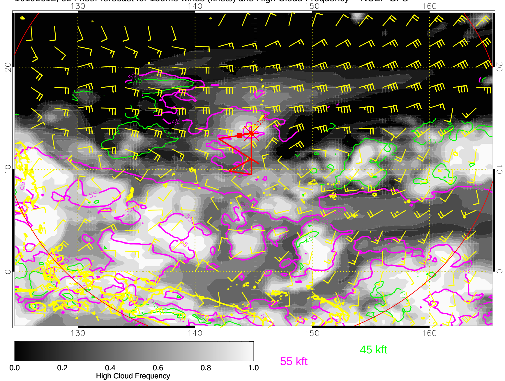
16102612, 024 hour forecast for 150mb winds (knots) and High Cloud Frequency -- NCEP GFS
