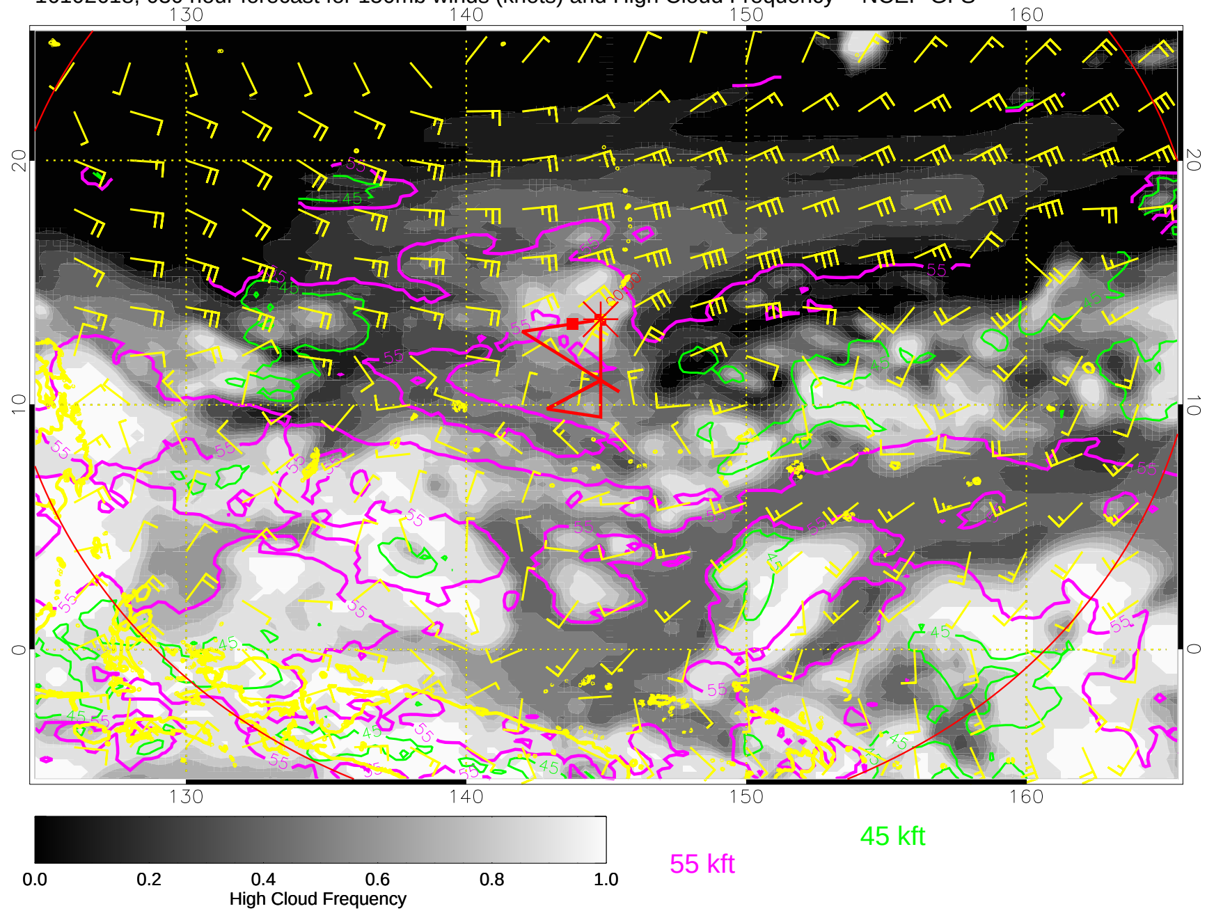
16102618, 030 hour forecast for 150mb winds (knots) and High Cloud Frequency -- NCEP GFS
