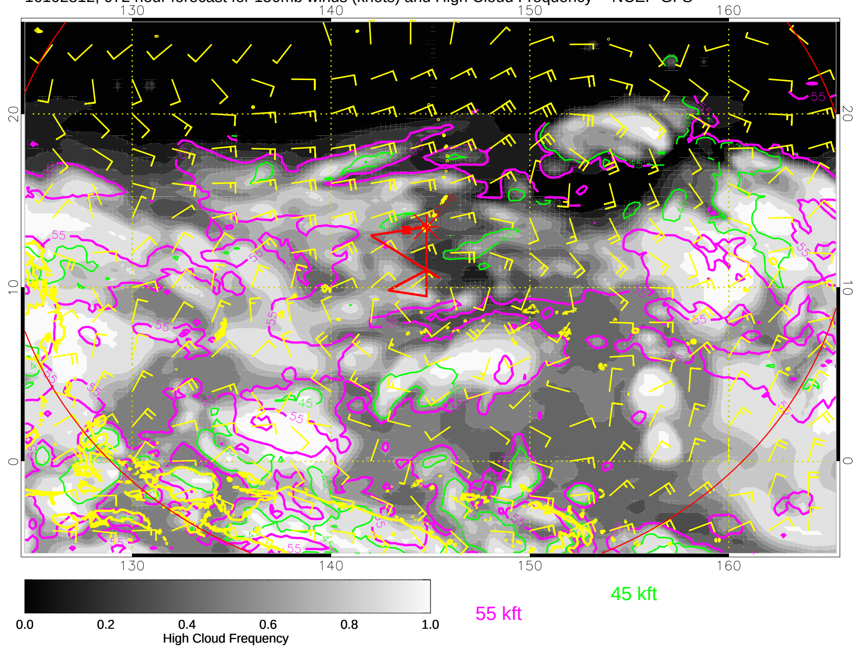
16102812, 072 hour forecast for 150mb winds (knots) and High Cloud Frequency -- NCEP GFS
