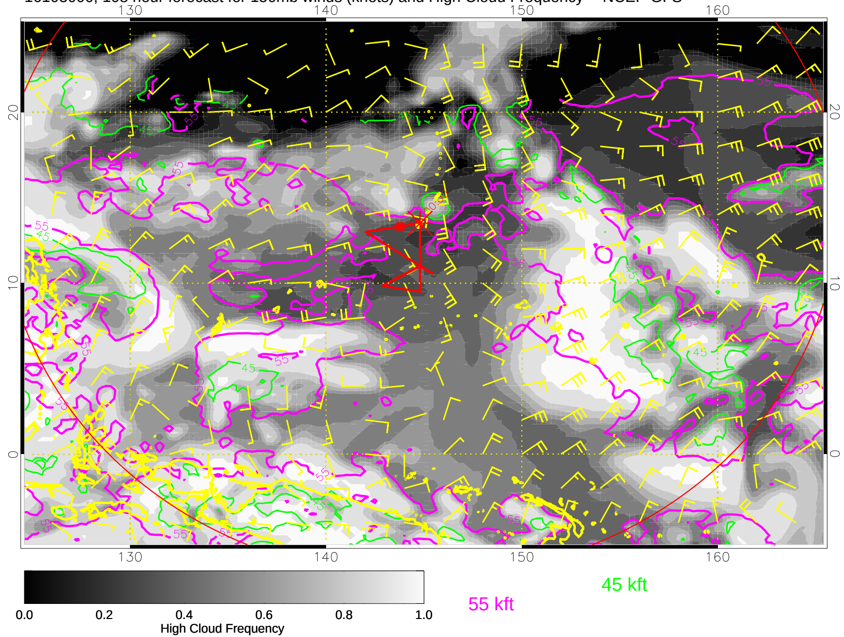
16103000, 108 hour forecast for 150mb winds (knots) and High Cloud Frequency -- NCEP GFS
