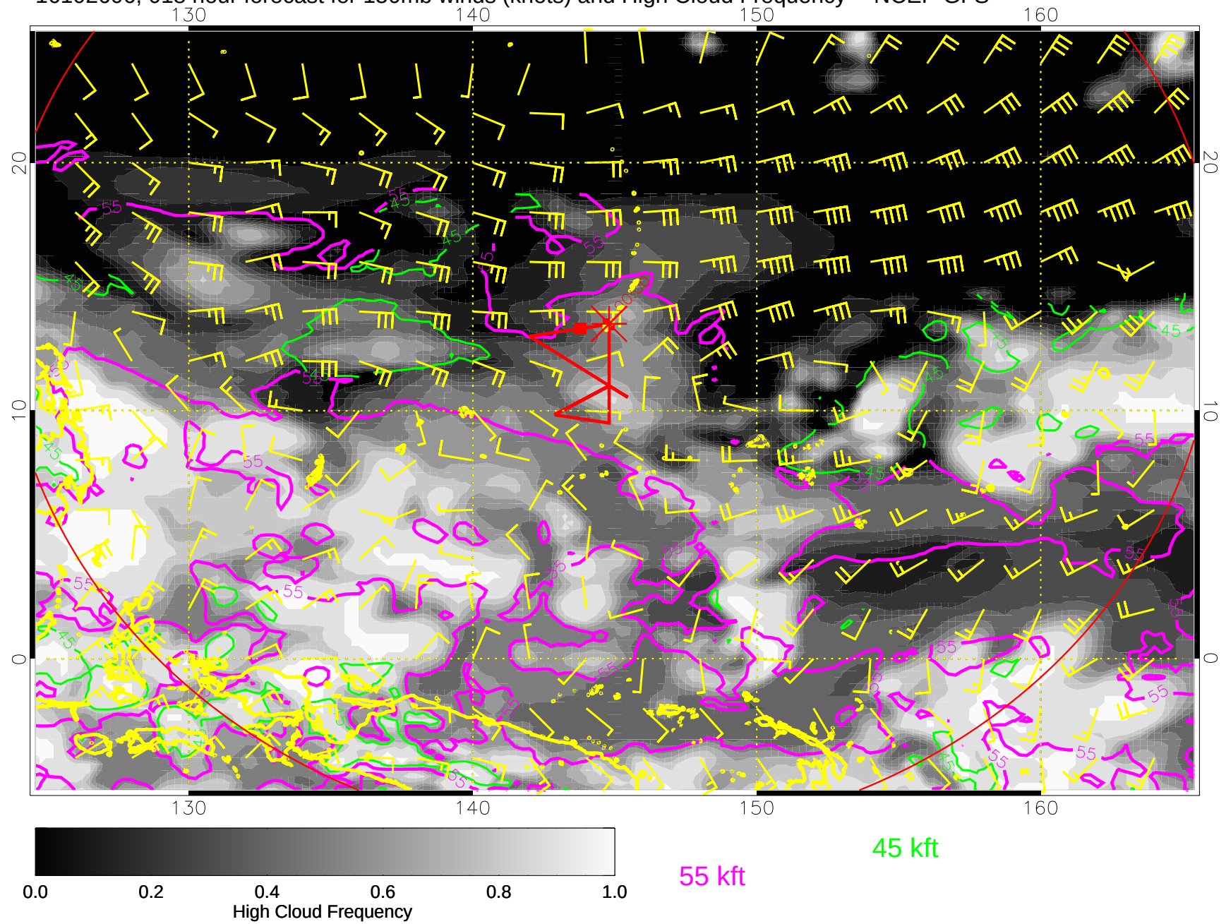
16102606, 018 hour forecast for 150mb winds (knots) and High Cloud Frequency -- NCEP GFS
