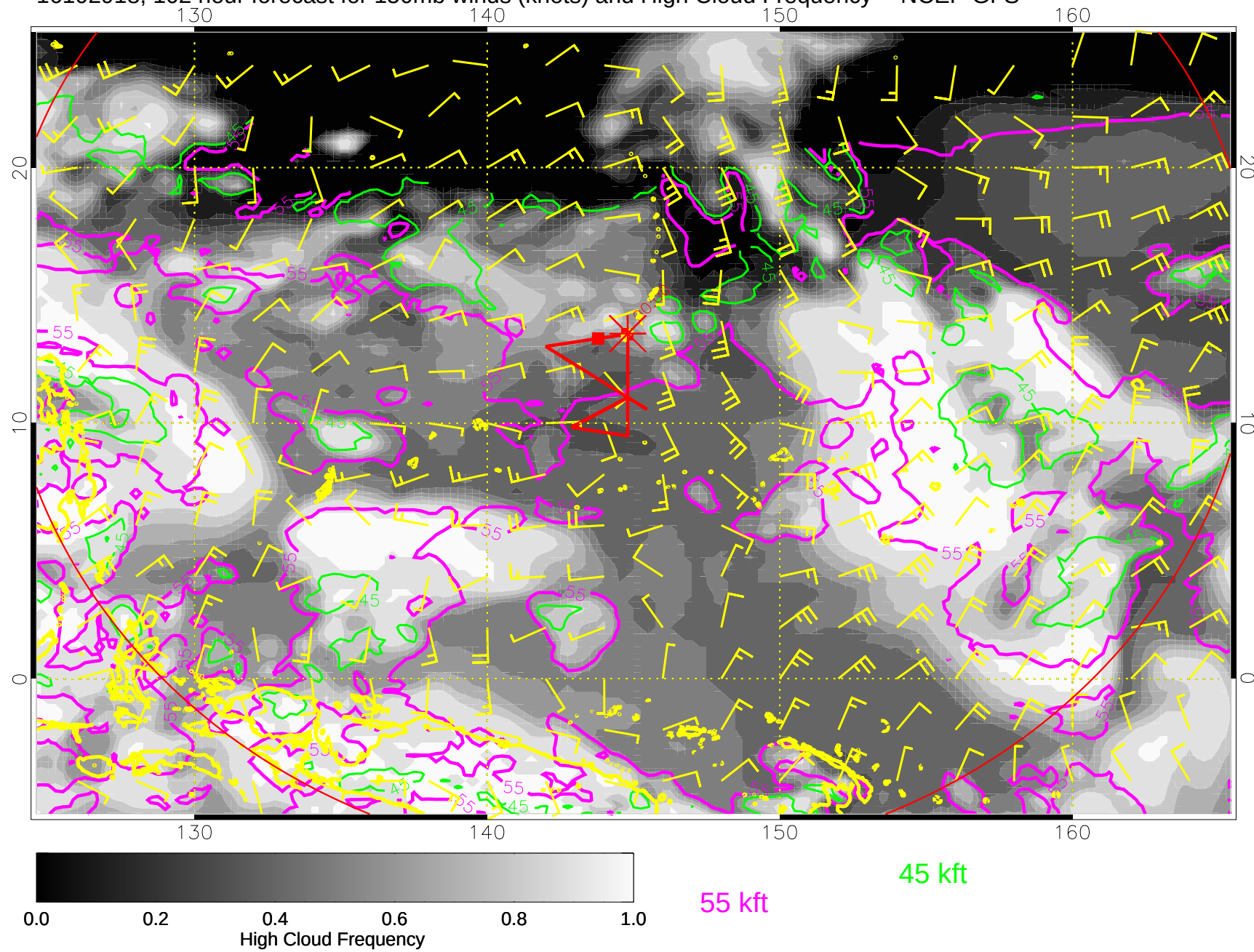
16102918, 102 hour forecast for 150mb winds (knots) and High Cloud Frequency -- NCEP GFS
