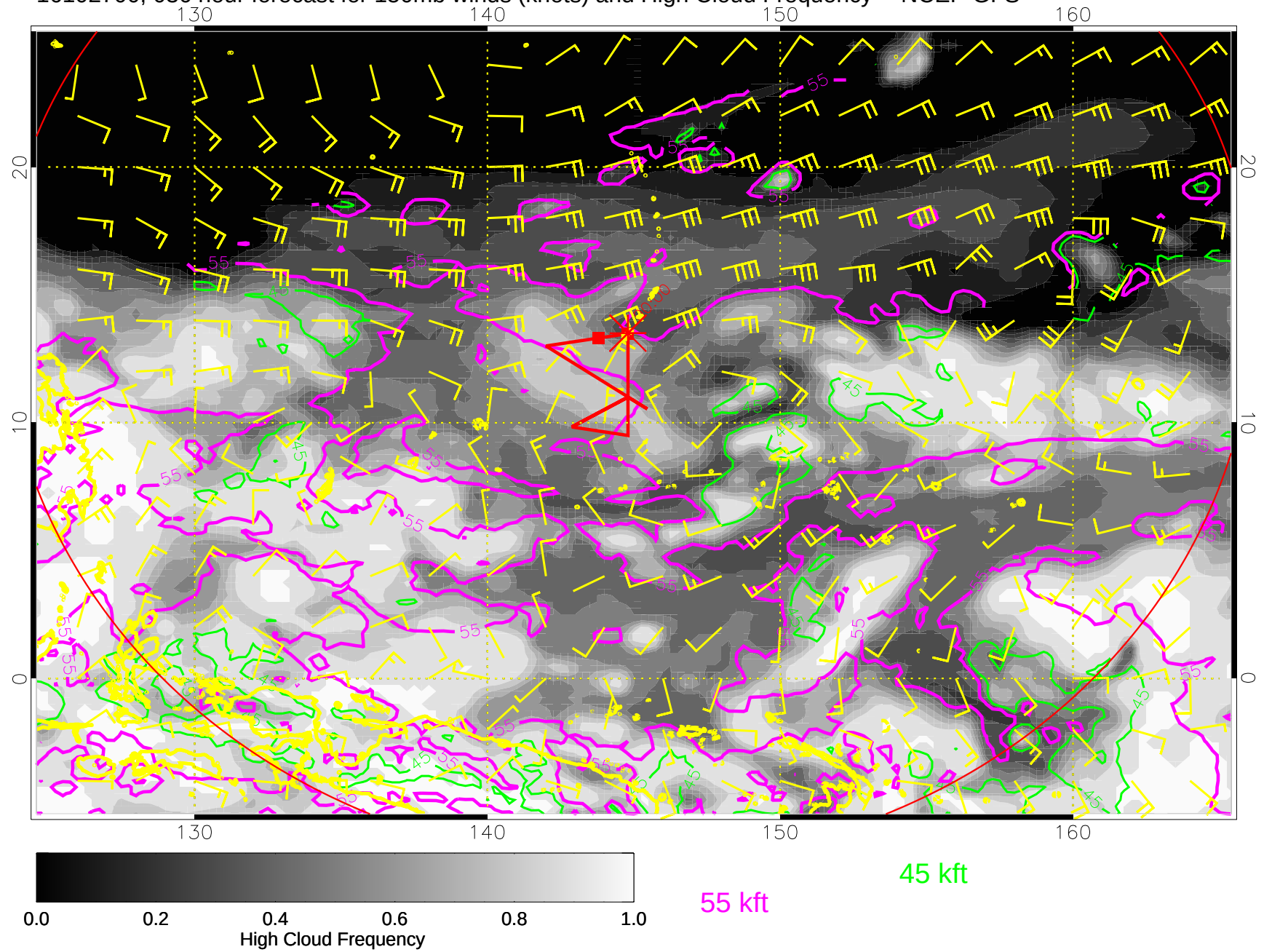
16102700, 036 hour forecast for 150mb winds (knots) and High Cloud Frequency -- NCEP GFS
