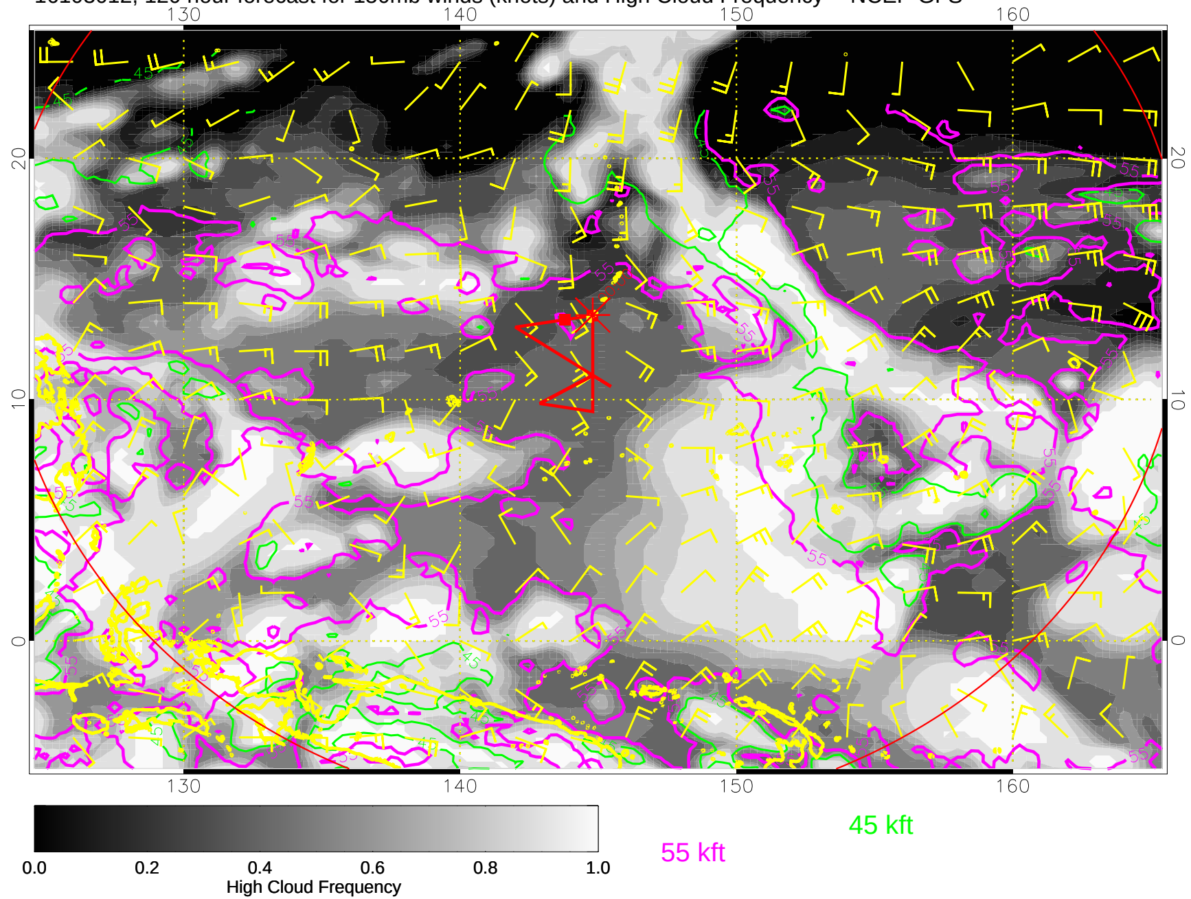
16103012, 120 hour forecast for 150mb winds (knots) and High Cloud Frequency -- NCEP GFS
