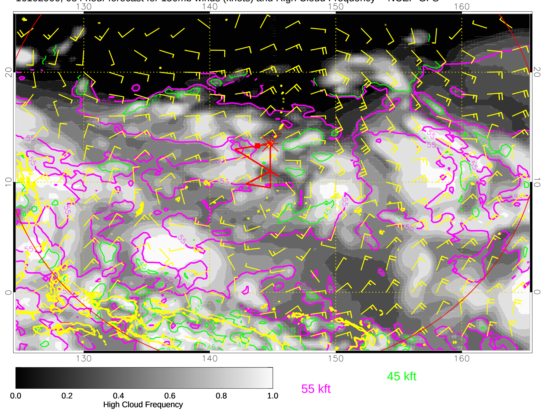
16102900, 084 hour forecast for 150mb winds (knots) and High Cloud Frequency -- NCEP GFS
