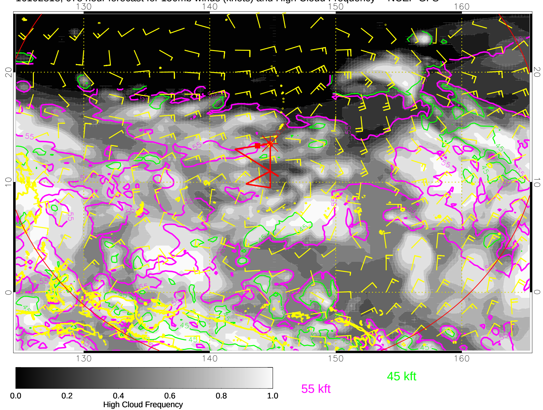
16102818, 078 hour forecast for 150mb winds (knots) and High Cloud Frequency -- NCEP GFS
