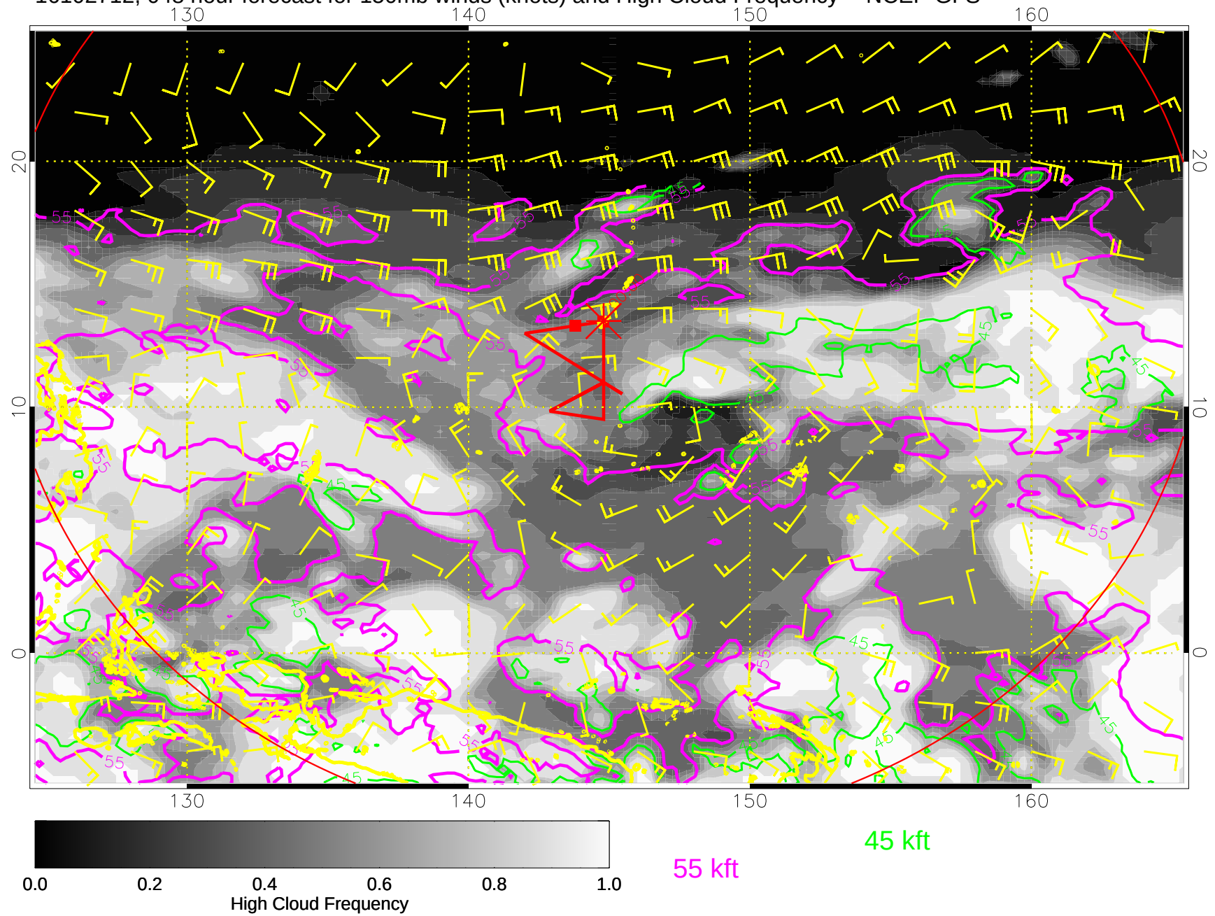
16102712, 048 hour forecast for 150mb winds (knots) and High Cloud Frequency -- NCEP GFS
