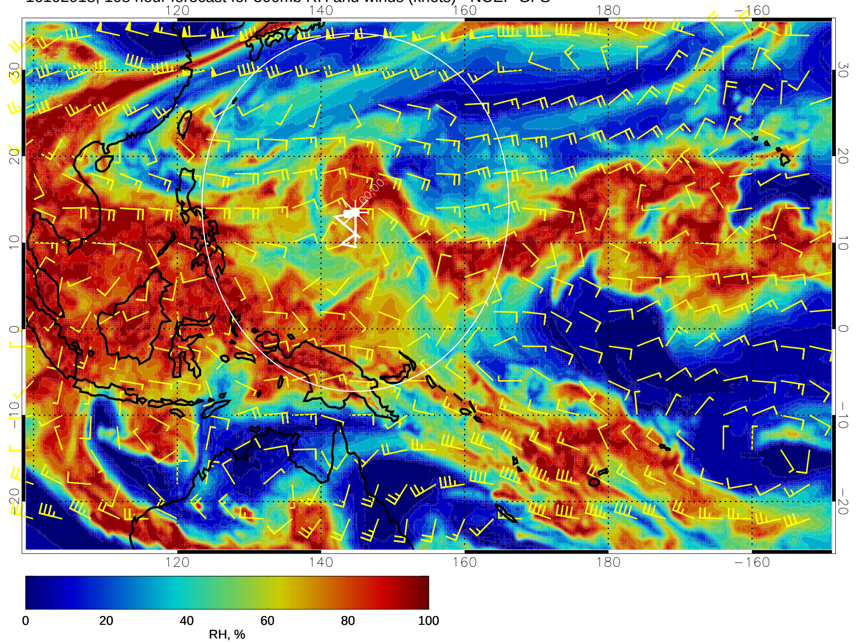
16102918, 108 hour forecast for 500mb RH and winds (knots) - NCEP GFS
