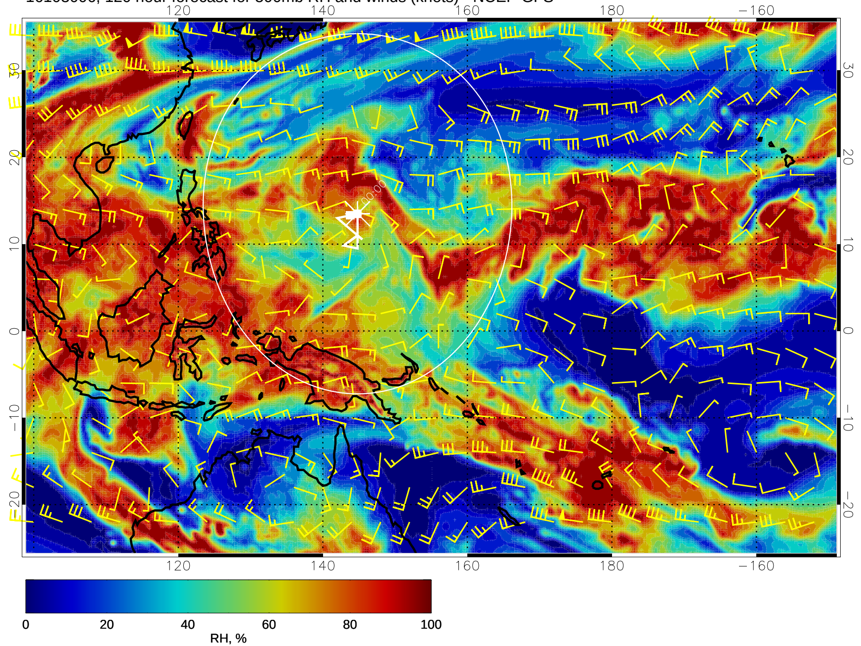
16103006, 120 hour forecast for 500mb RH and winds (knots) - NCEP GFS
