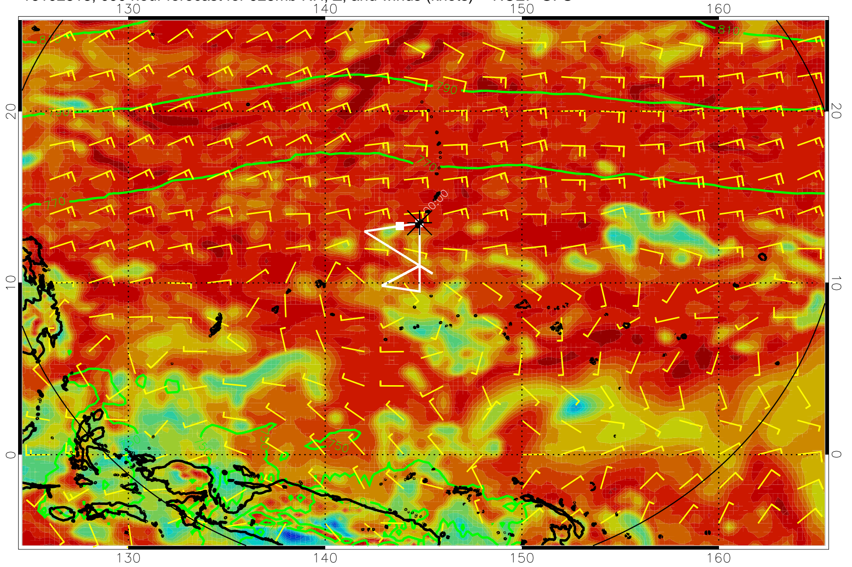
16102818, 090 hour forecast for 925mb RH, Z, and winds (knots) -- NCEP GFS
