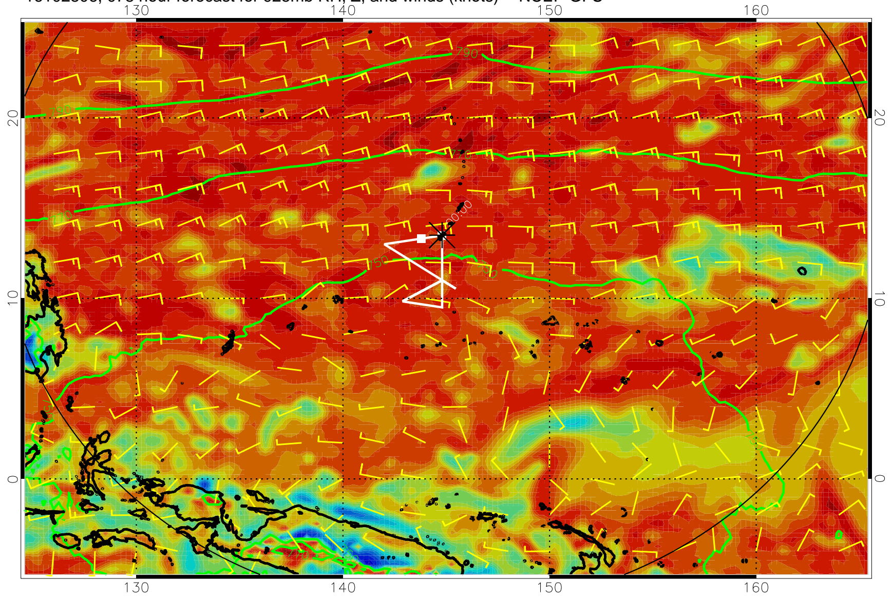
16102806, 078 hour forecast for 925mb RH, Z, and winds (knots) -- NCEP GFS
