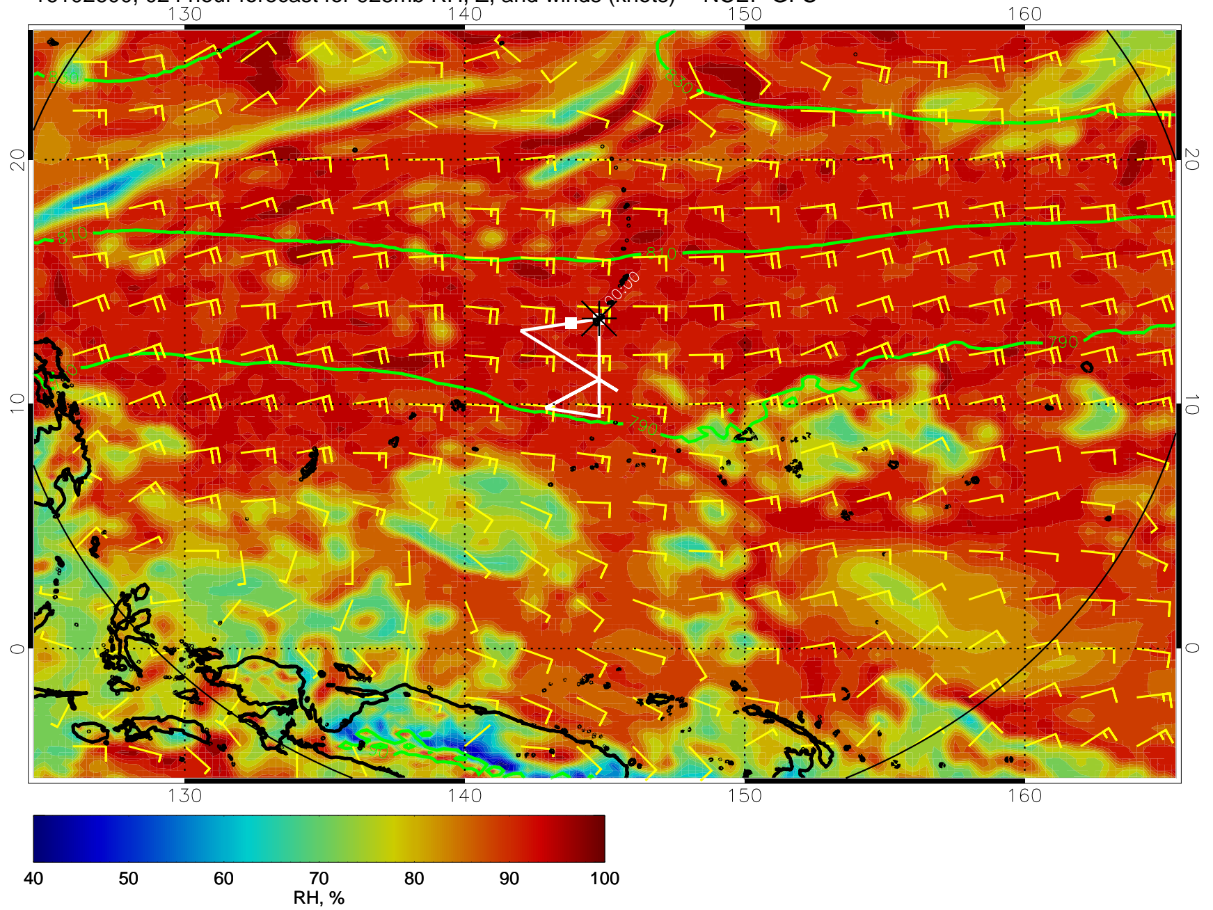
16102600, 024 hour forecast for 925mb RH, Z, and winds (knots) -- NCEP GFS
