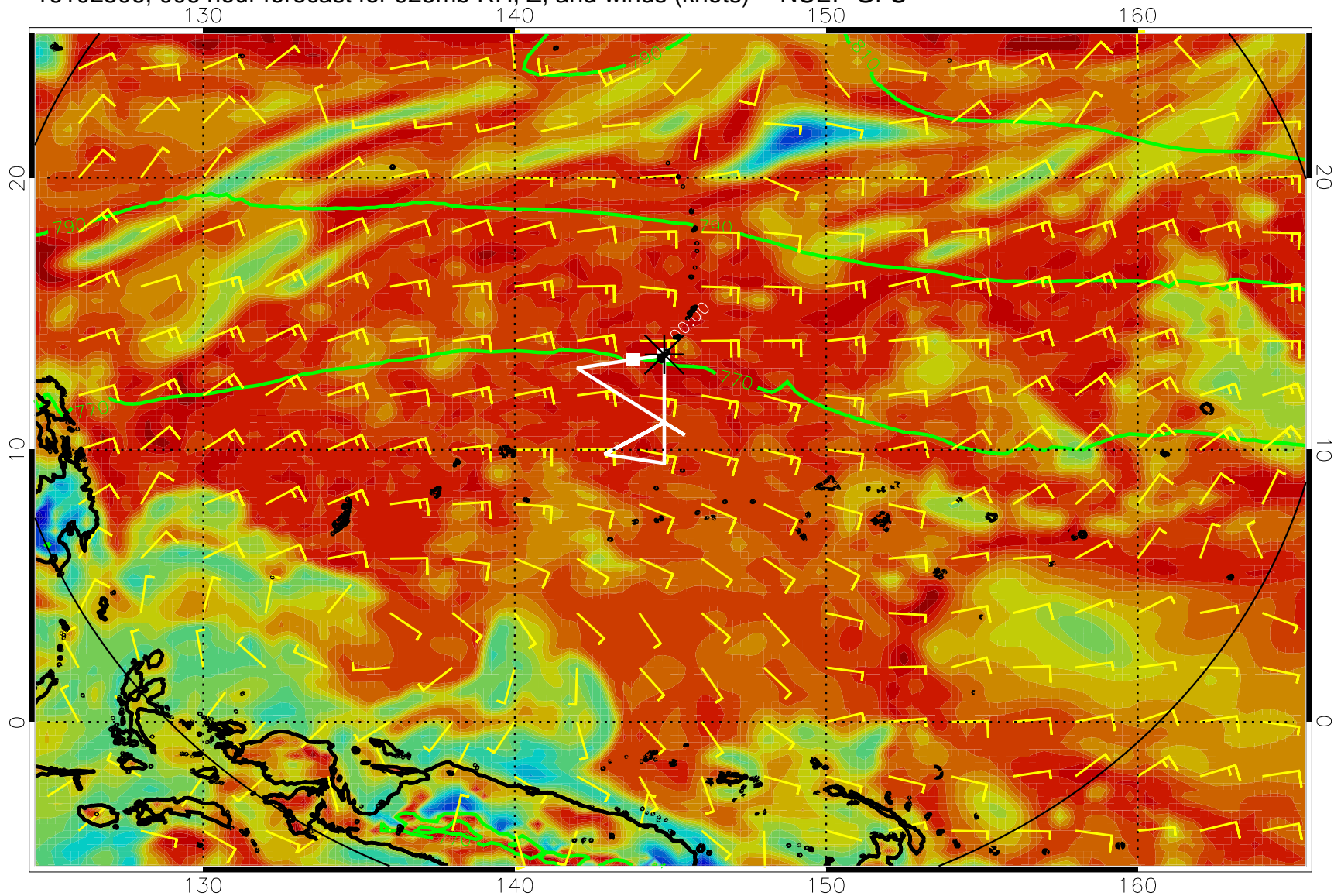
16102506, 006 hour forecast for 925mb RH, Z, and winds (knots) -- NCEP GFS
