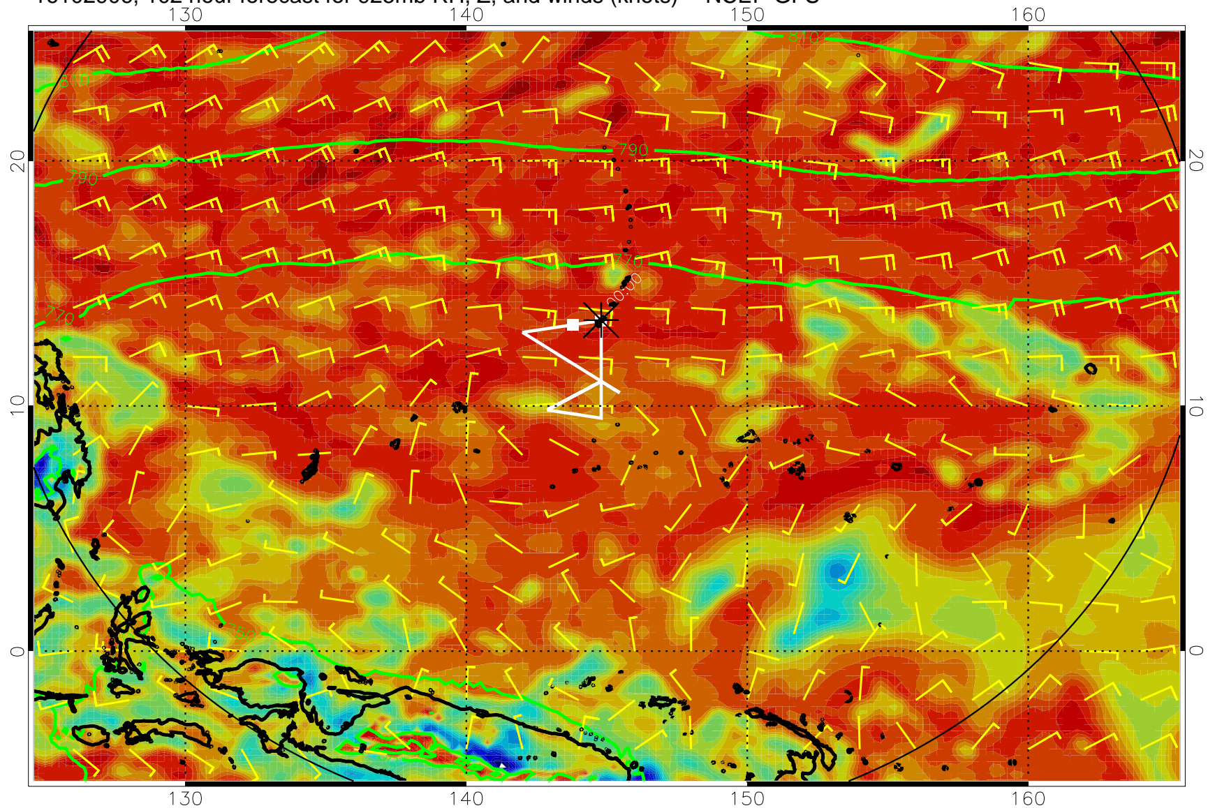
16102906, 102 hour forecast for 925mb RH, Z, and winds (knots) -- NCEP GFS
