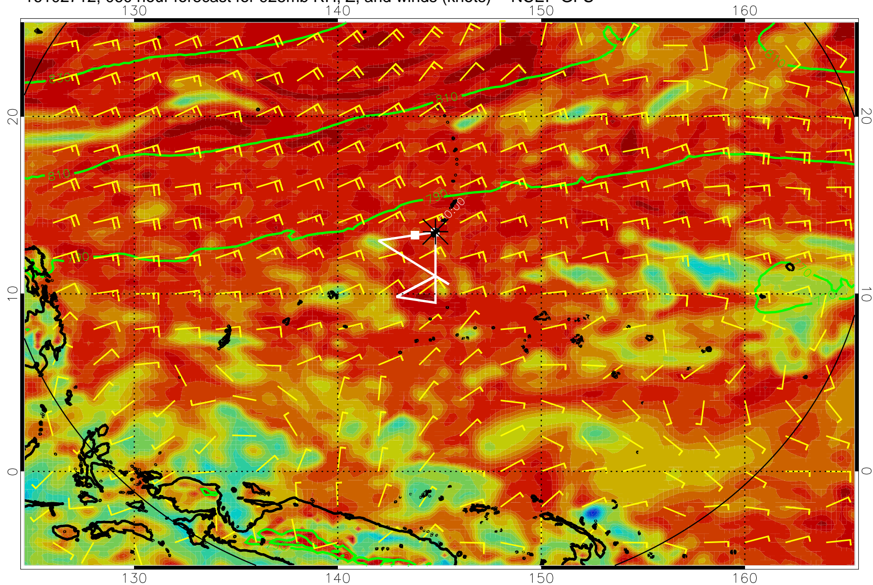
16102712, 060 hour forecast for 925mb RH, Z, and winds (knots) -- NCEP GFS
