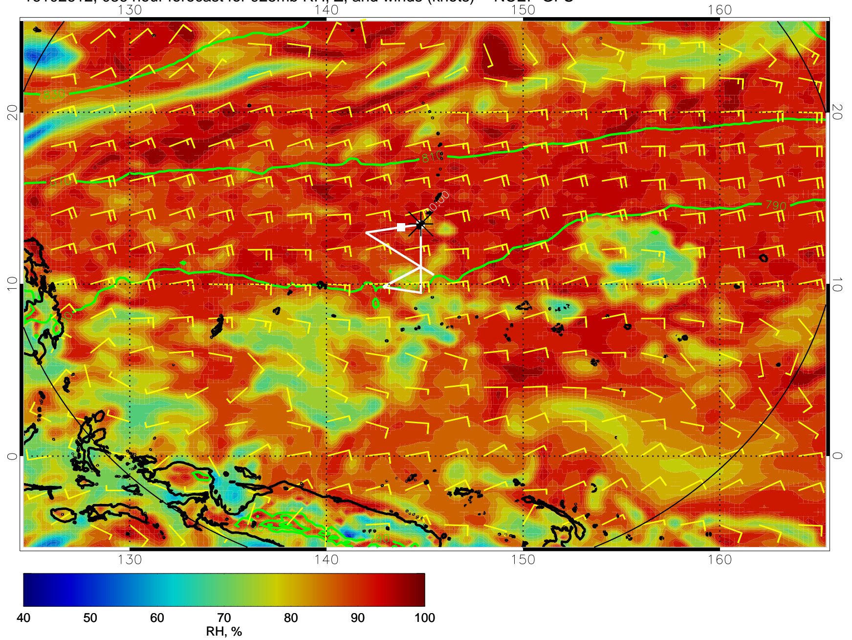
16102612, 036 hour forecast for 925mb RH, Z, and winds (knots) -- NCEP GFS
