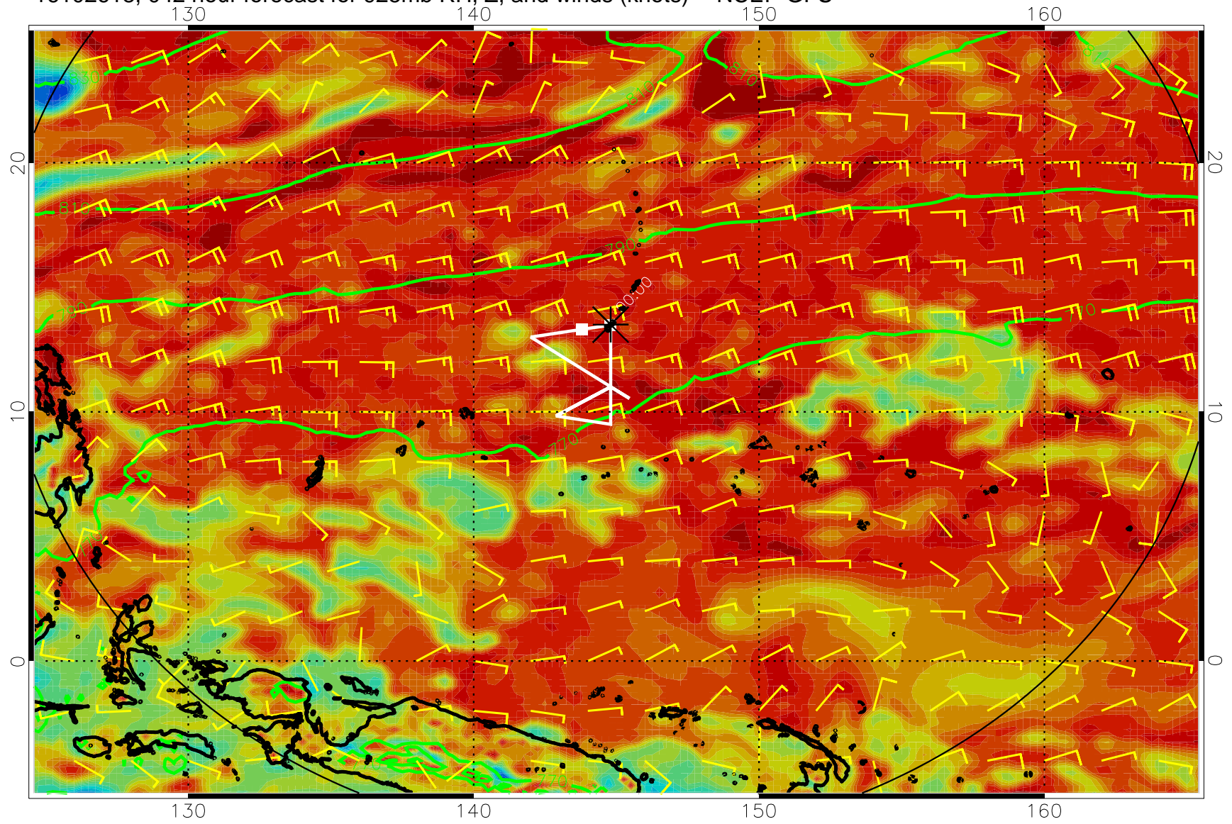
16102618, 042 hour forecast for 925mb RH, Z, and winds (knots) -- NCEP GFS
