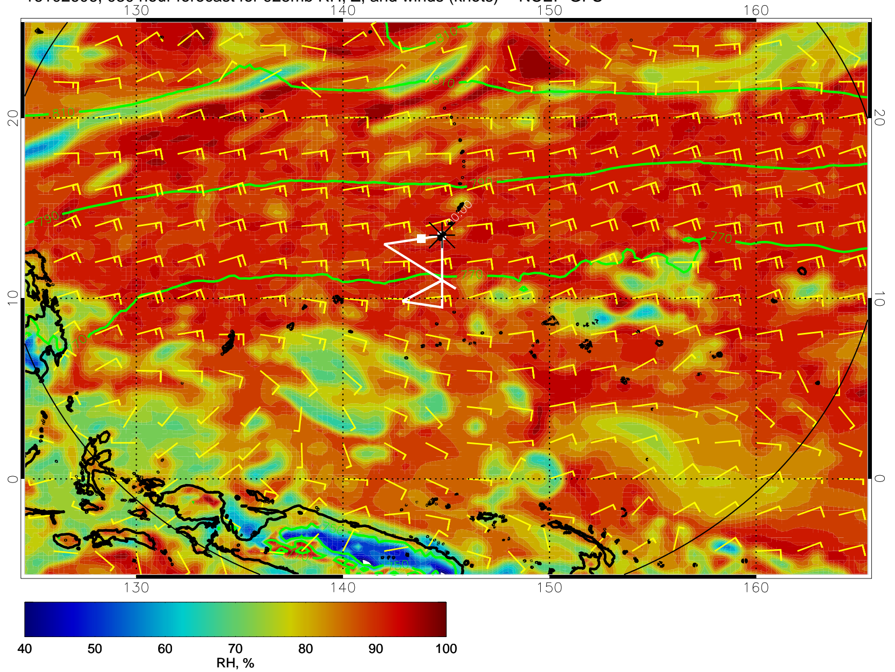
16102606, 0300 hour forecast for 925mb RH, Z, and winds (knots) -- NCEP GFS
