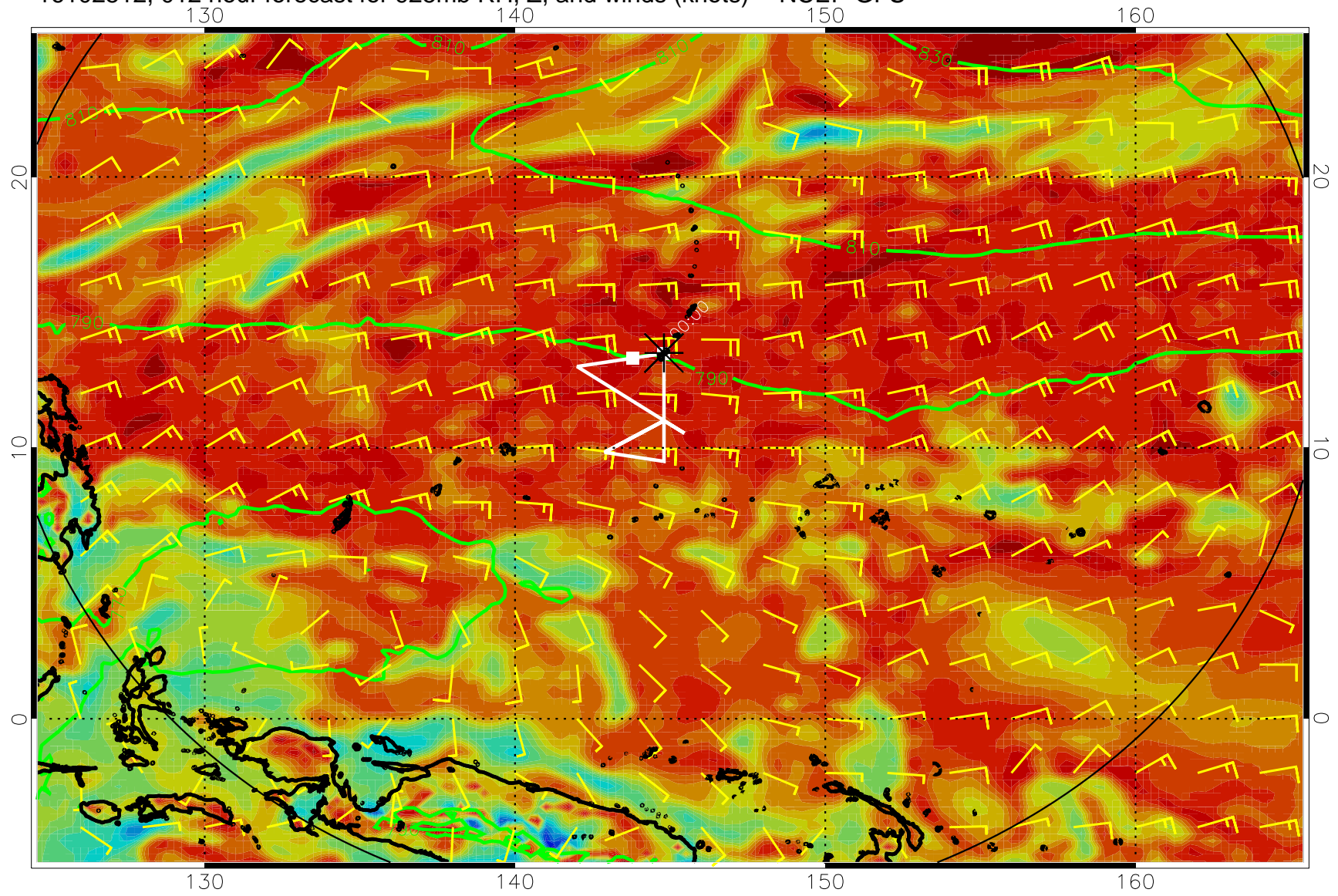
16102512, 012 hour forecast for 925mb RH, Z, and winds (knots) -- NCEP GFS
