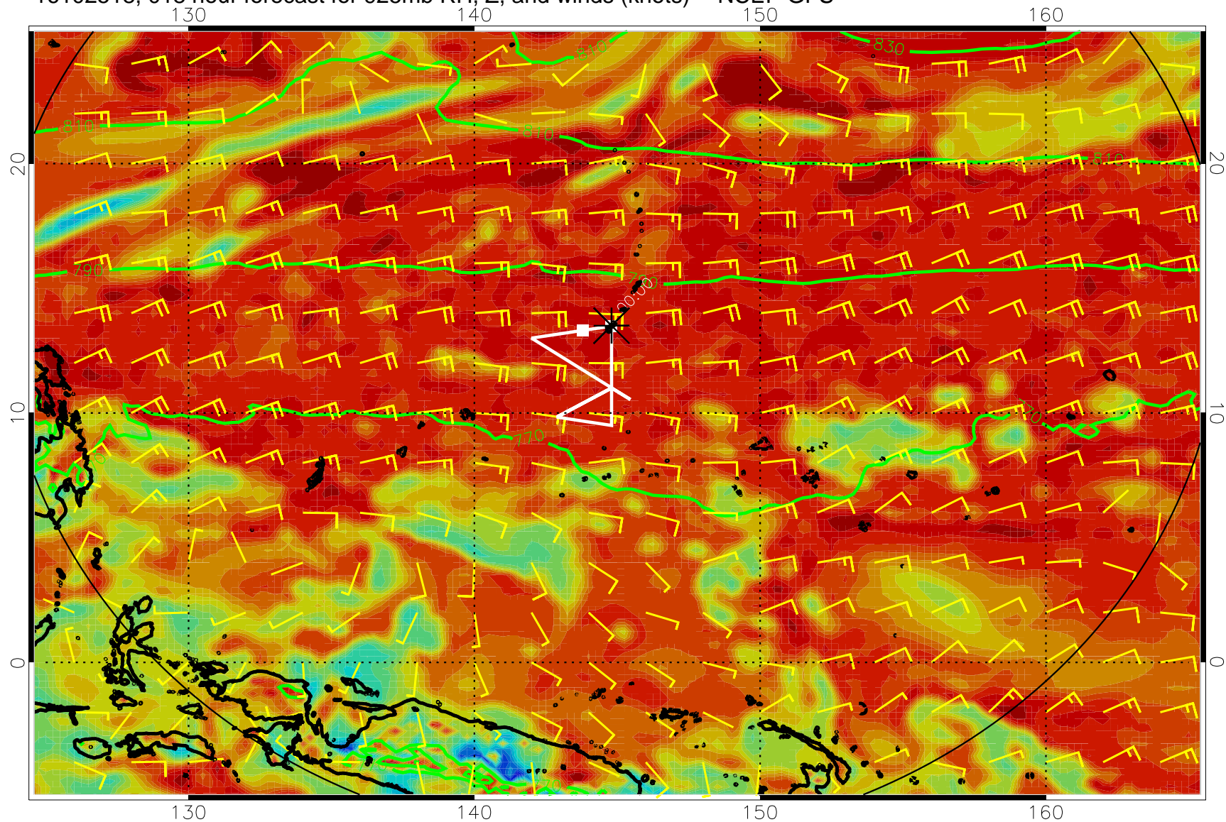
16102518, 018 hour forecast for 925mb RH, Z, and winds (knots) -- NCEP GFS
