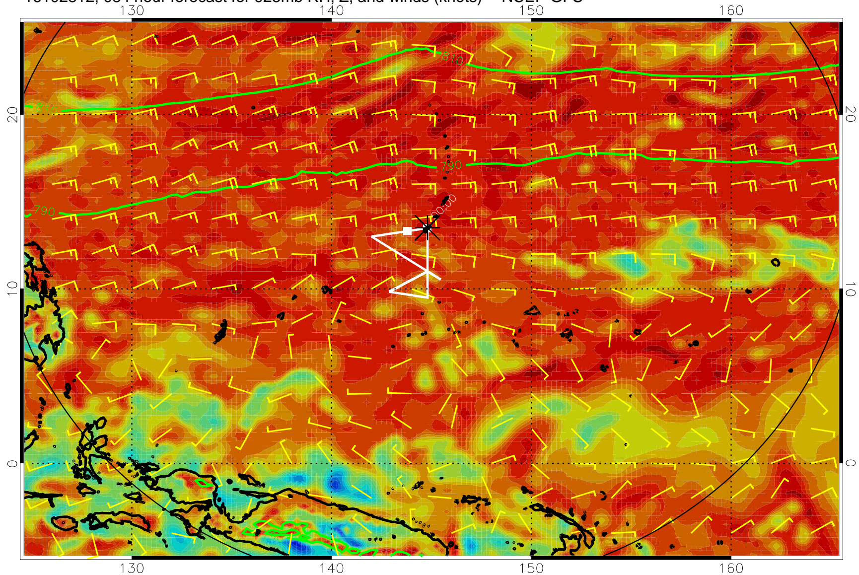
16102812, 084 hour forecast for 925mb RH, Z, and winds (knots) -- NCEP GFS
