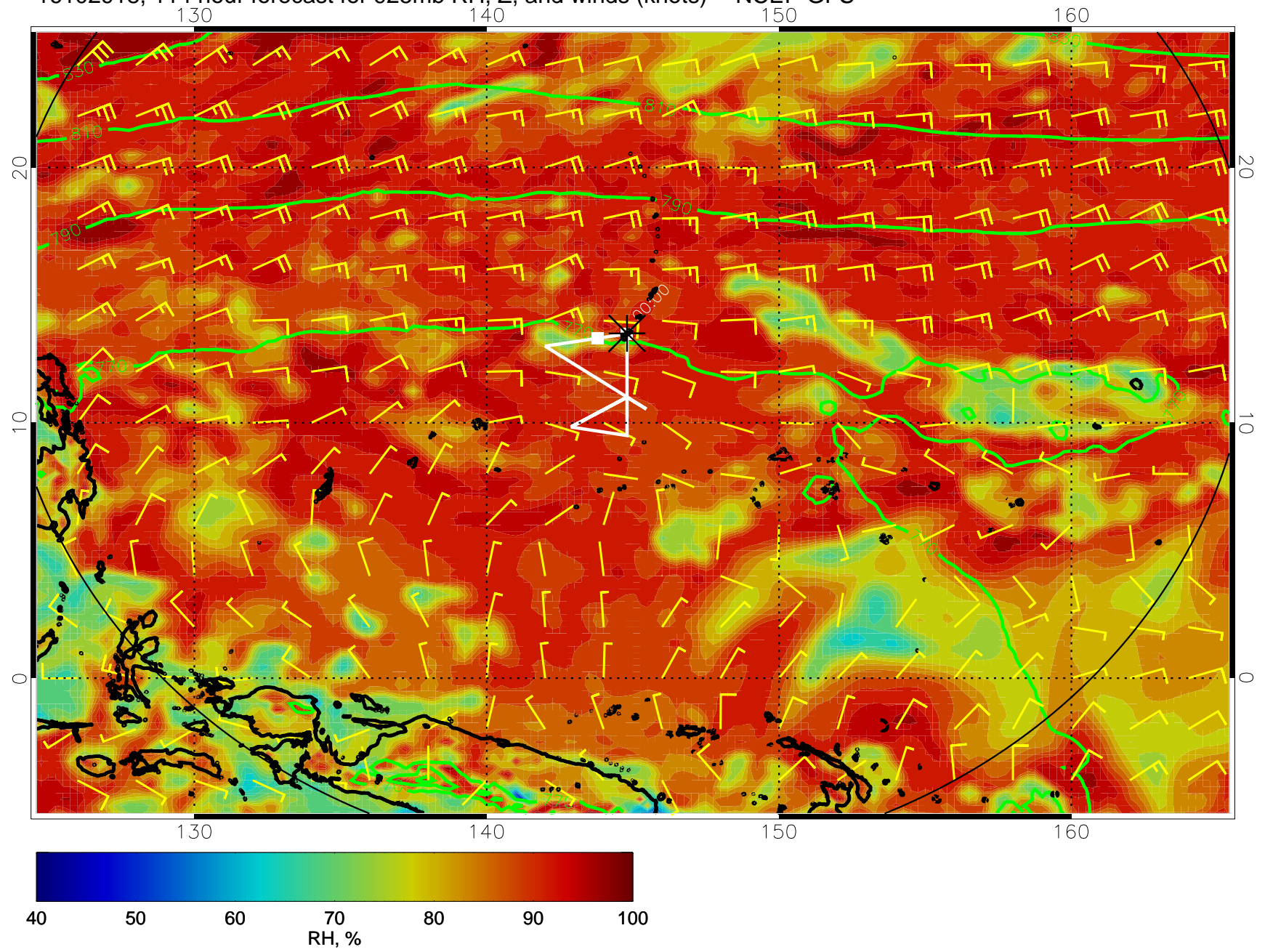
16102918, 114 hour forecast for 925mb RH, Z, and winds (knots) -- NCEP GFS
