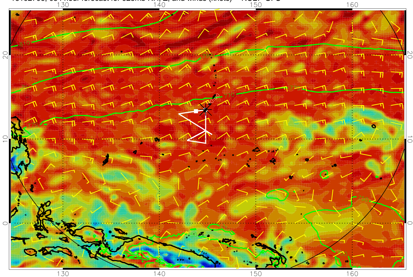
16102706, 054 hour forecast for 925mb RH, Z, and winds (knots) -- NCEP GFS
