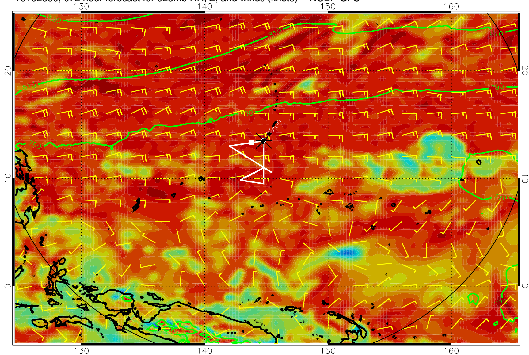
16102800, 072 hour forecast for 925mb RH, Z, and winds (knots) -- NCEP GFS
