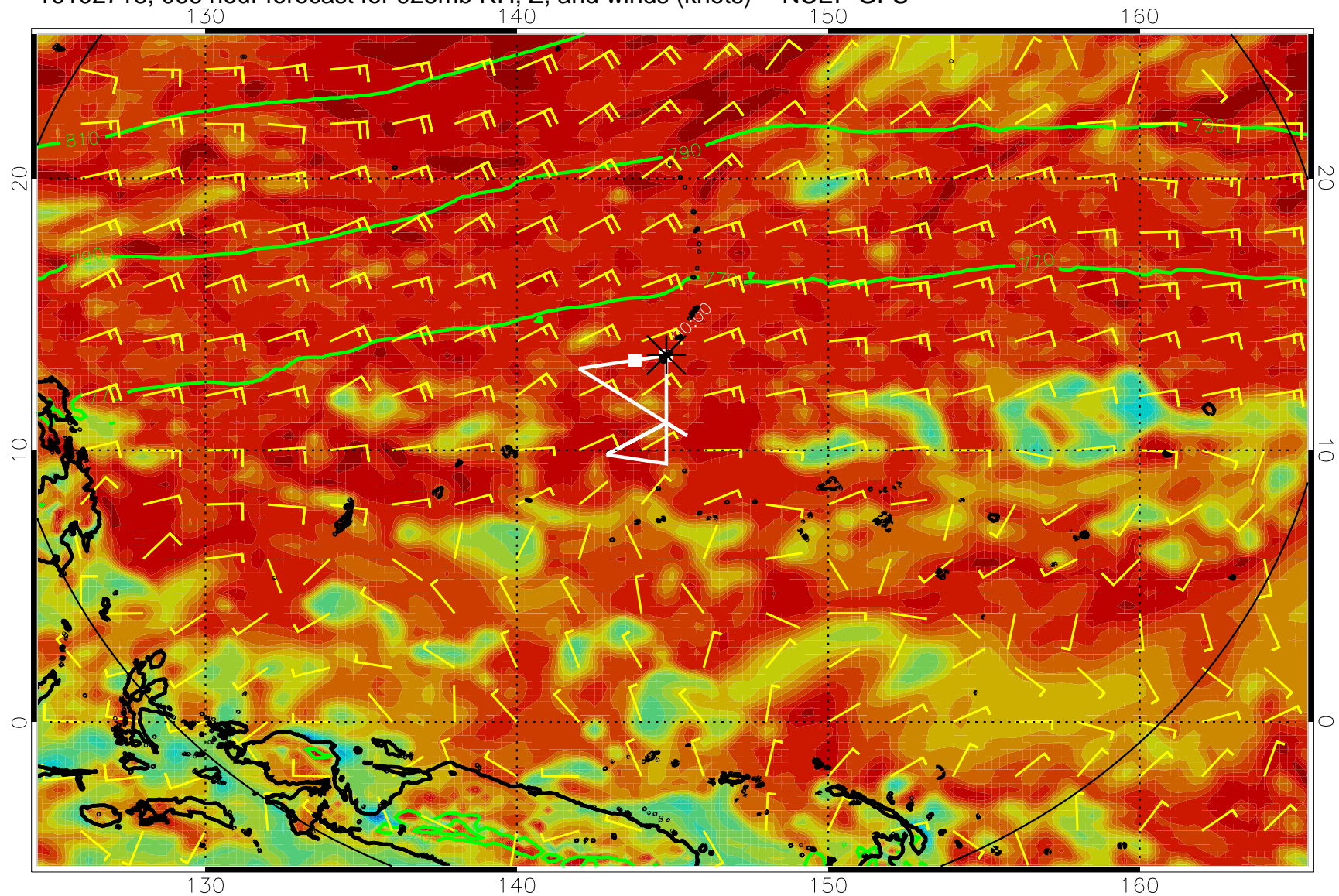
16102718, 066 hour forecast for 925mb RH, Z, and winds (knots) -- NCEP GFS
