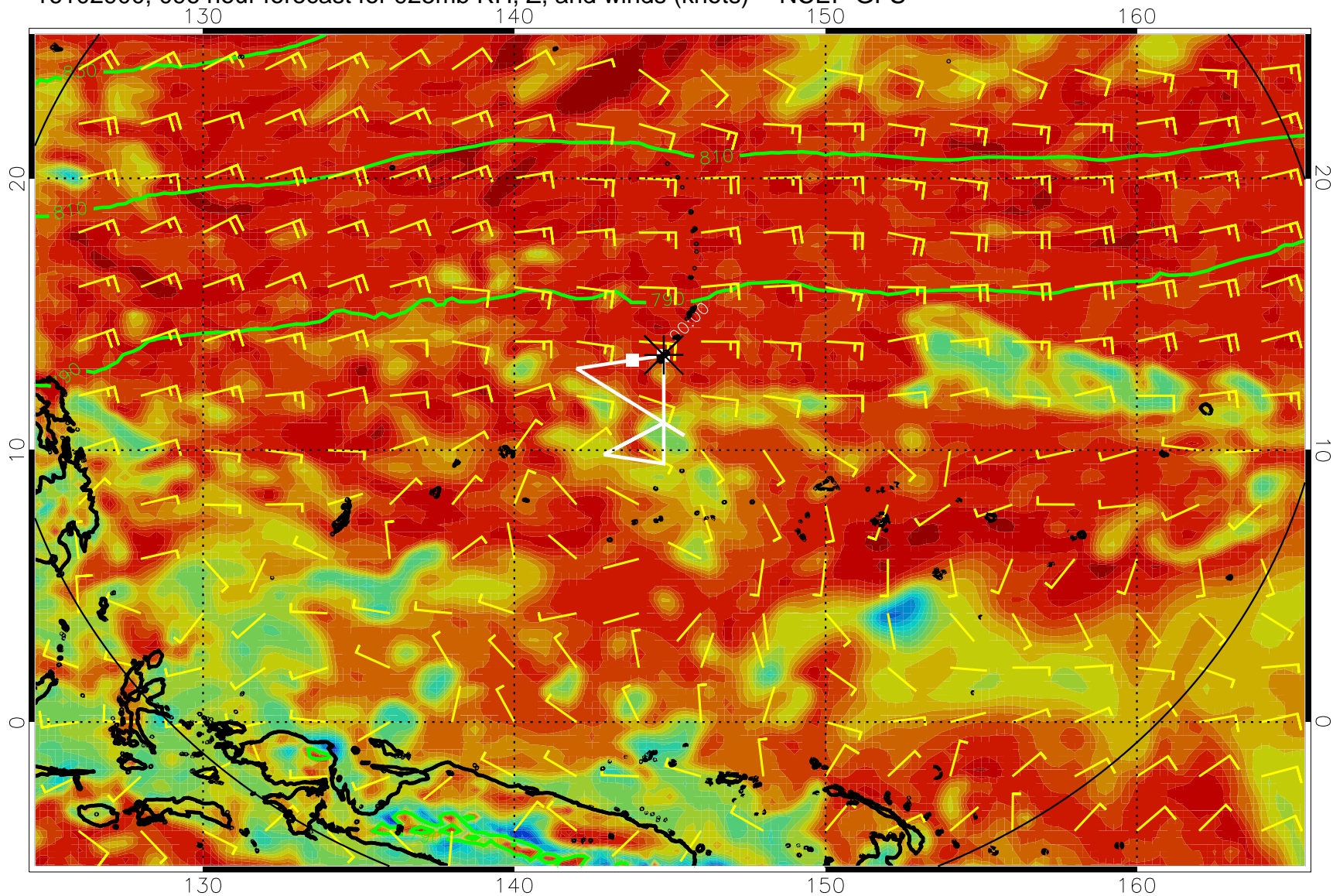
16102900, 096 hour forecast for 925mb RH, Z, and winds (knots) -- NCEP GFS
