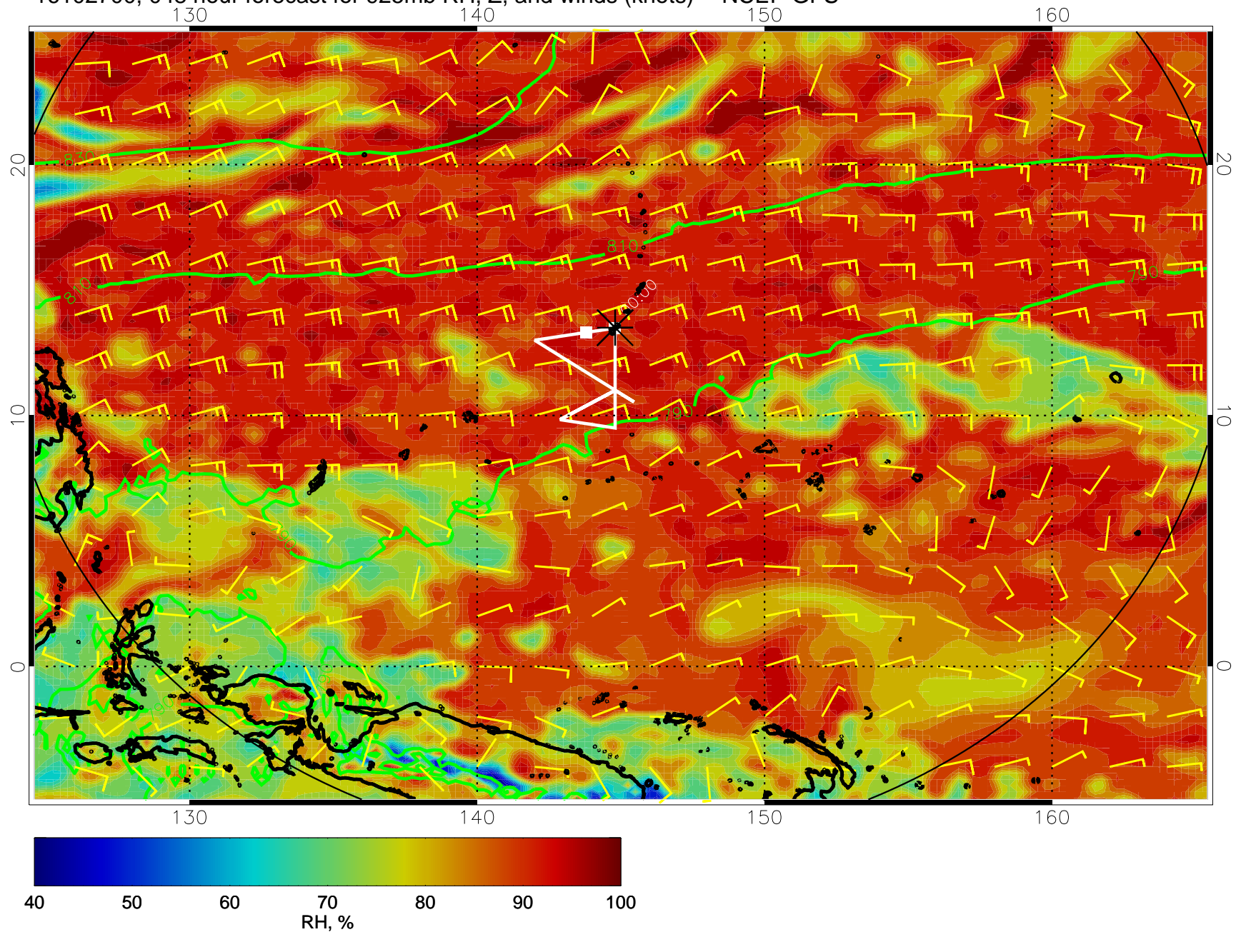
16102700, 048 hour forecast for 925mb RH, Z, and winds (knots) -- NCEP GFS
