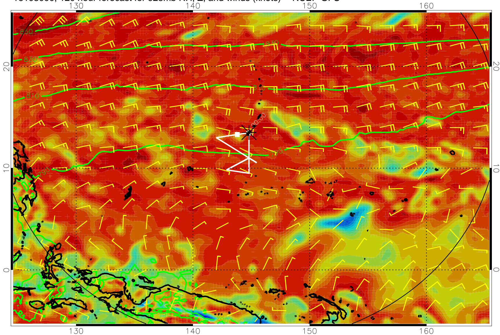
16103000, 120 hour forecast for 925mb RH, Z, and winds (knots) -- NCEP GFS
