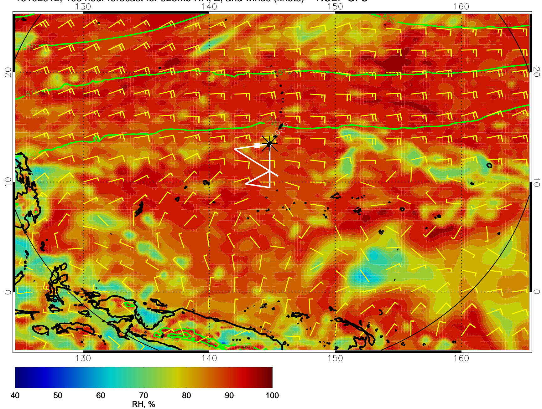
16102912, 108 hour forecast for 925mb RH, Z, and winds (knots) -- NCEP GFS
