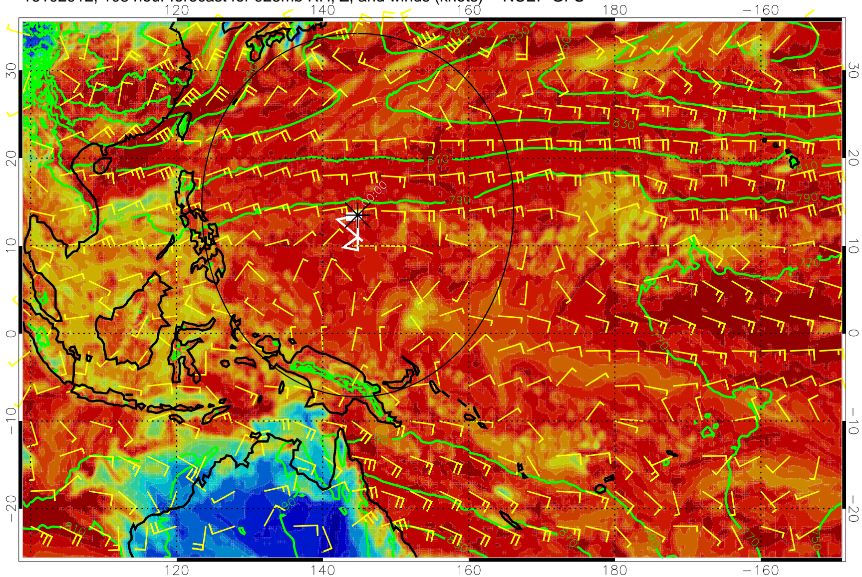
16102912, 108 hour forecast for 925mb RH, Z, and winds (knots) -- NCEP GFS
