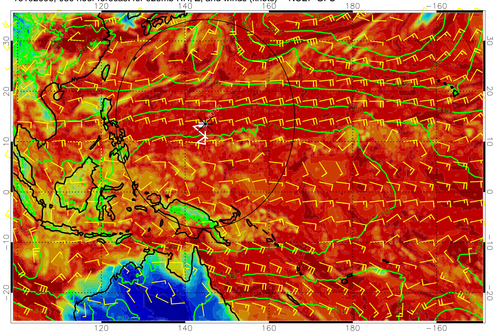
16102606, 030 hour forecast for 925mb RH, Z, and winds (knots) -- NCEP GFS
