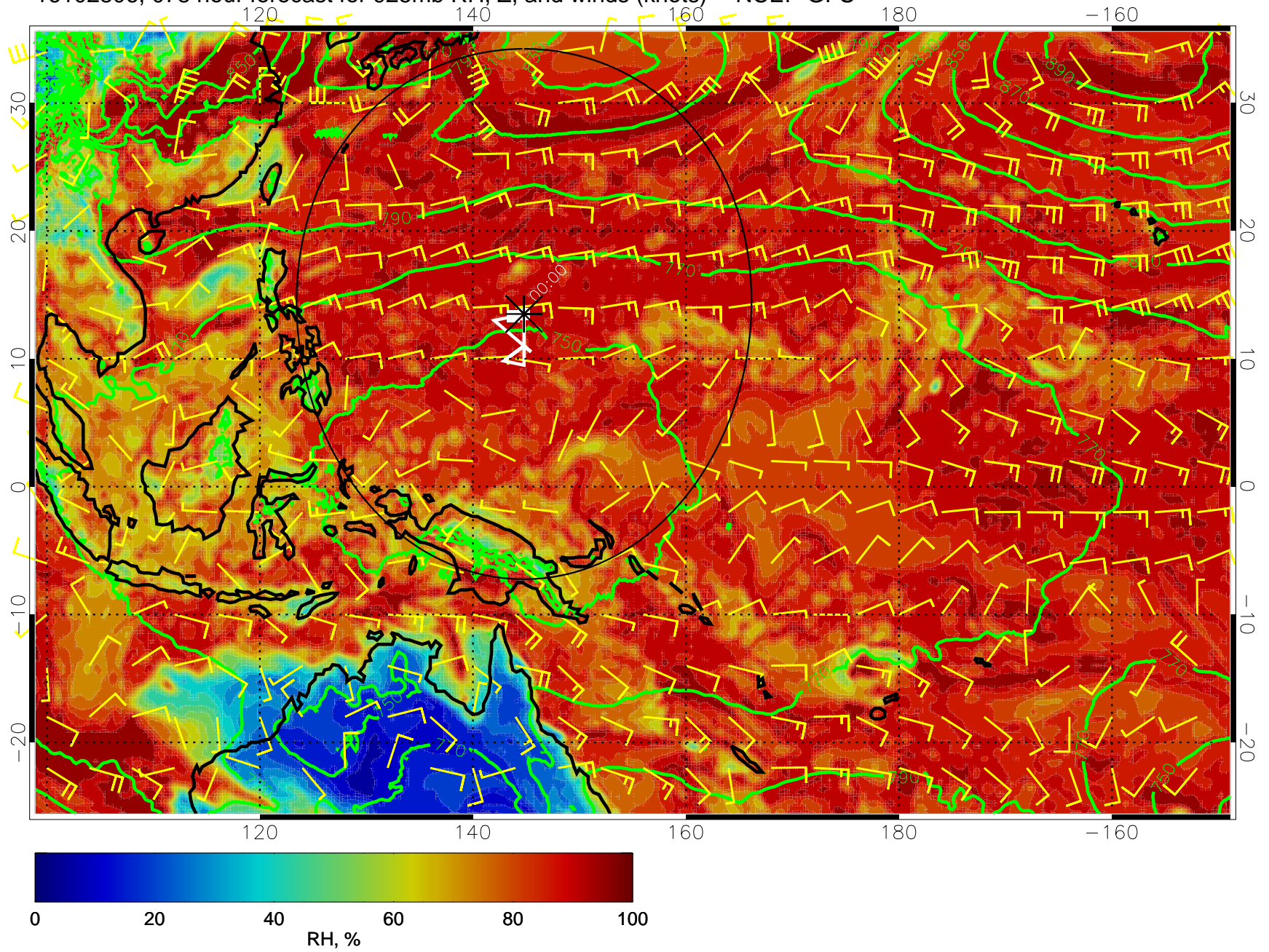
16102806, 078 hour forecast for 925mb RH, Z, and winds (knots) -- NCEP GFS
