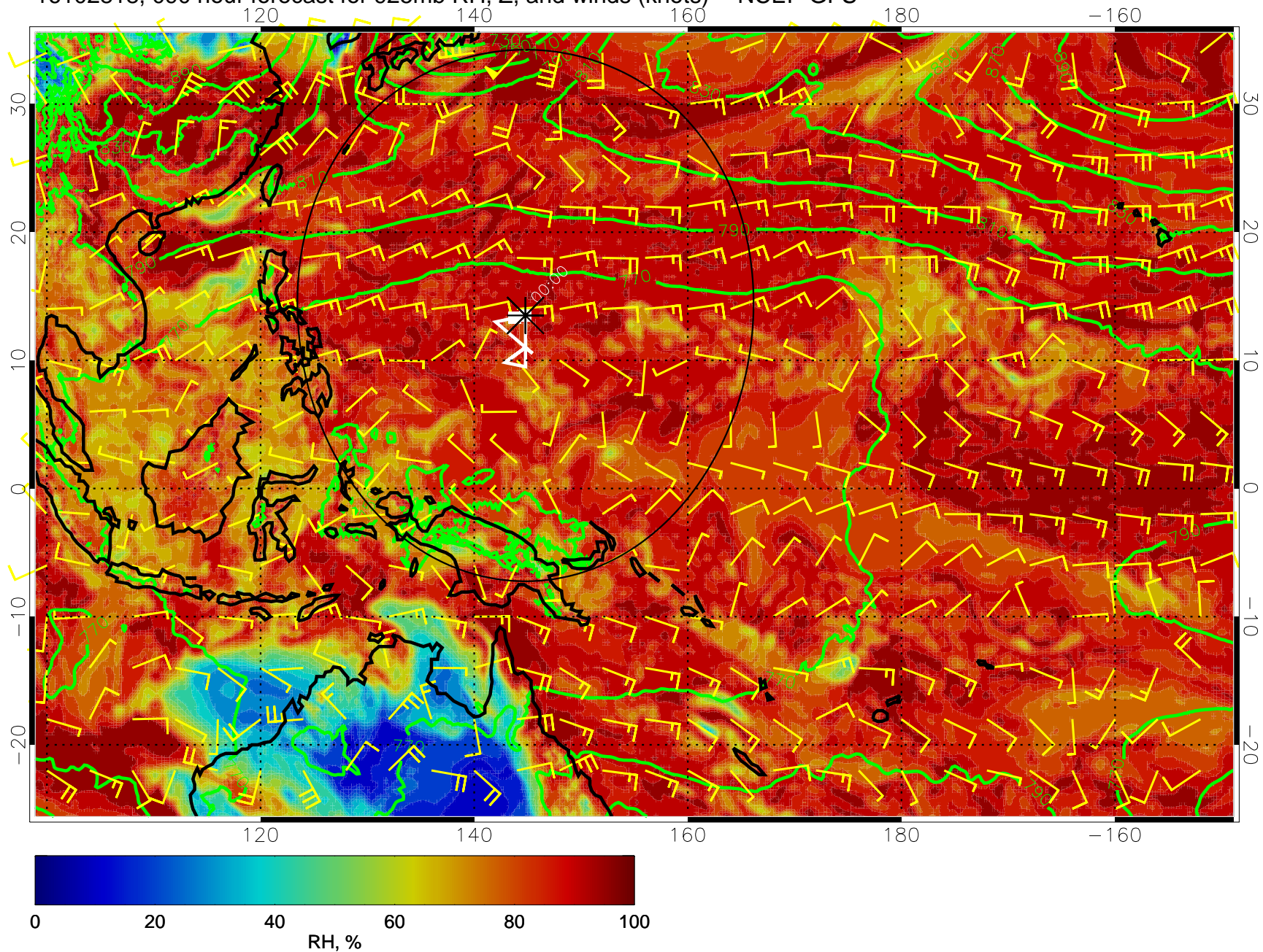
16102818, 090 hour forecast for 925mb RH, Z, and winds (knots) -- NCEP GFS
