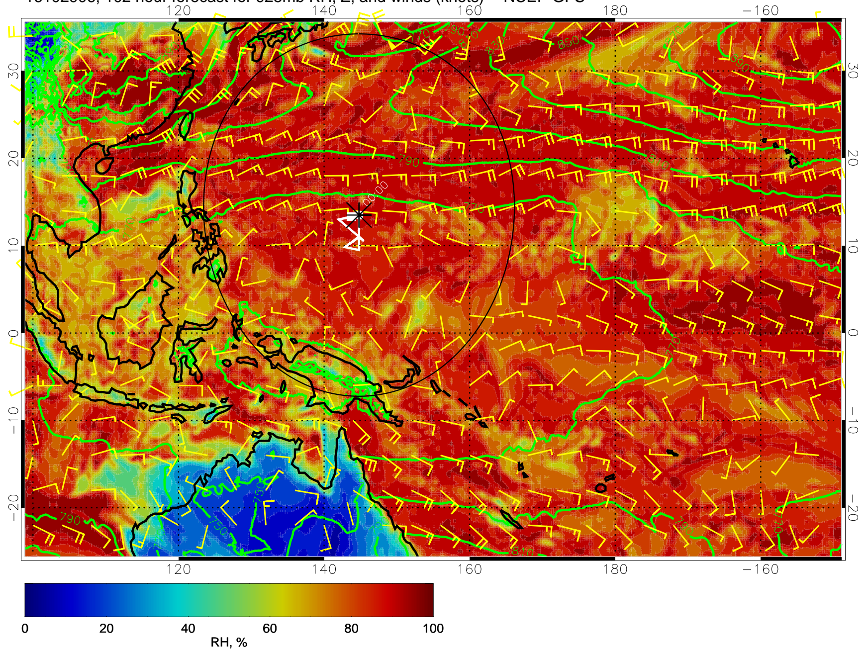
16102906, 102 hour forecast for 925mb RH, Z, and winds (knots) -- NCEP GFS
