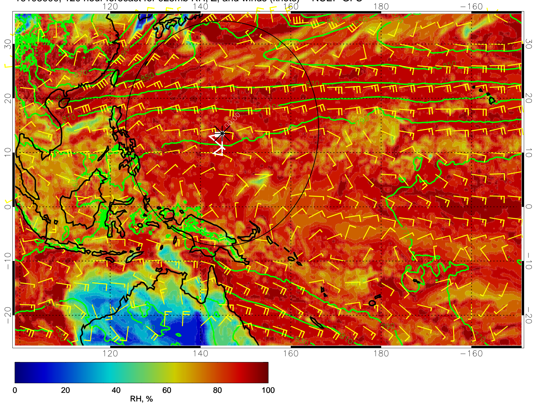
16103000, 120 hour forecast for 925mb RH, Z, and winds (knots) -- NCEP GFS
