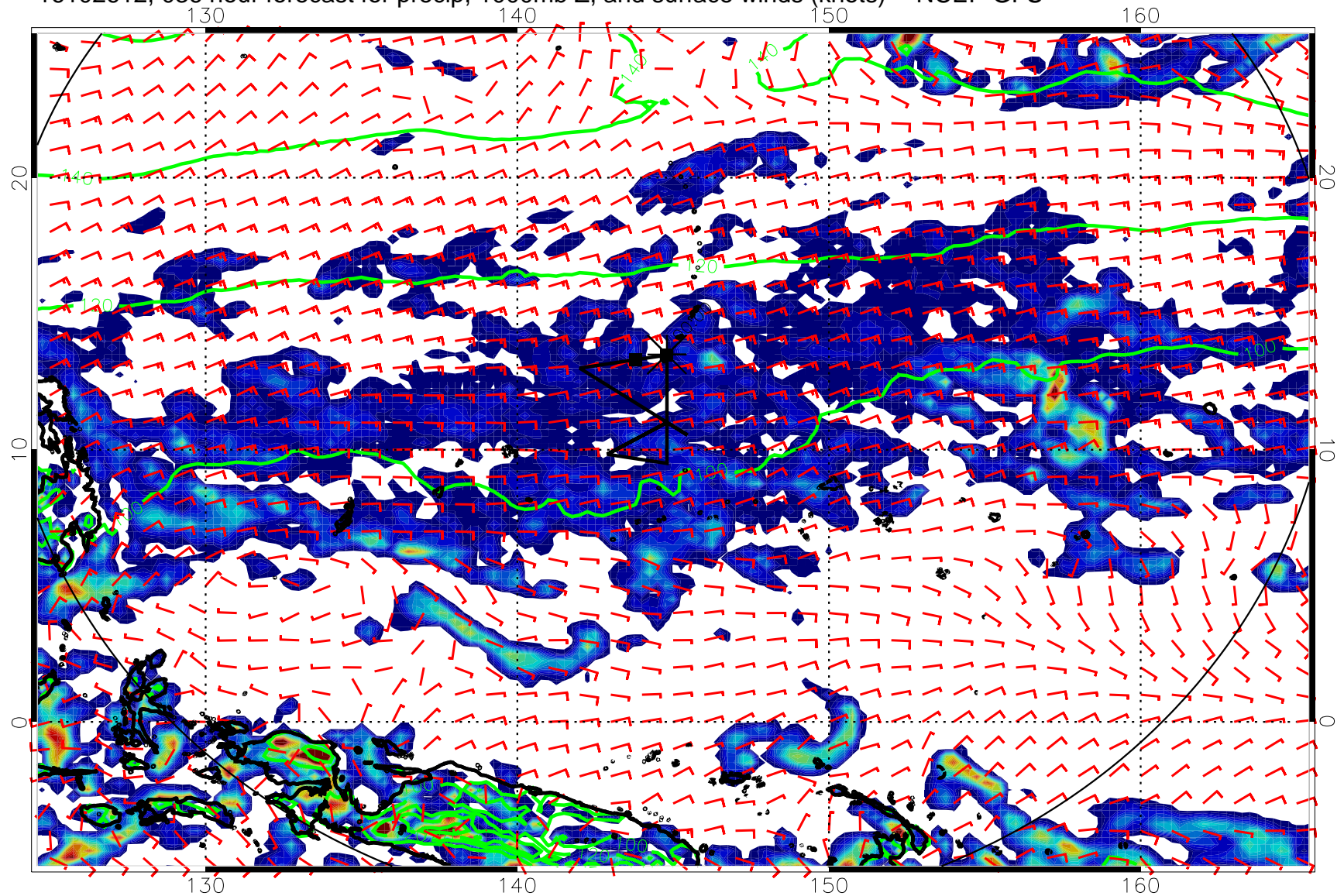
16102612, 036 hour forecast for precip, 1000mb Z, and surface winds (knots) -- NCEP GFS
