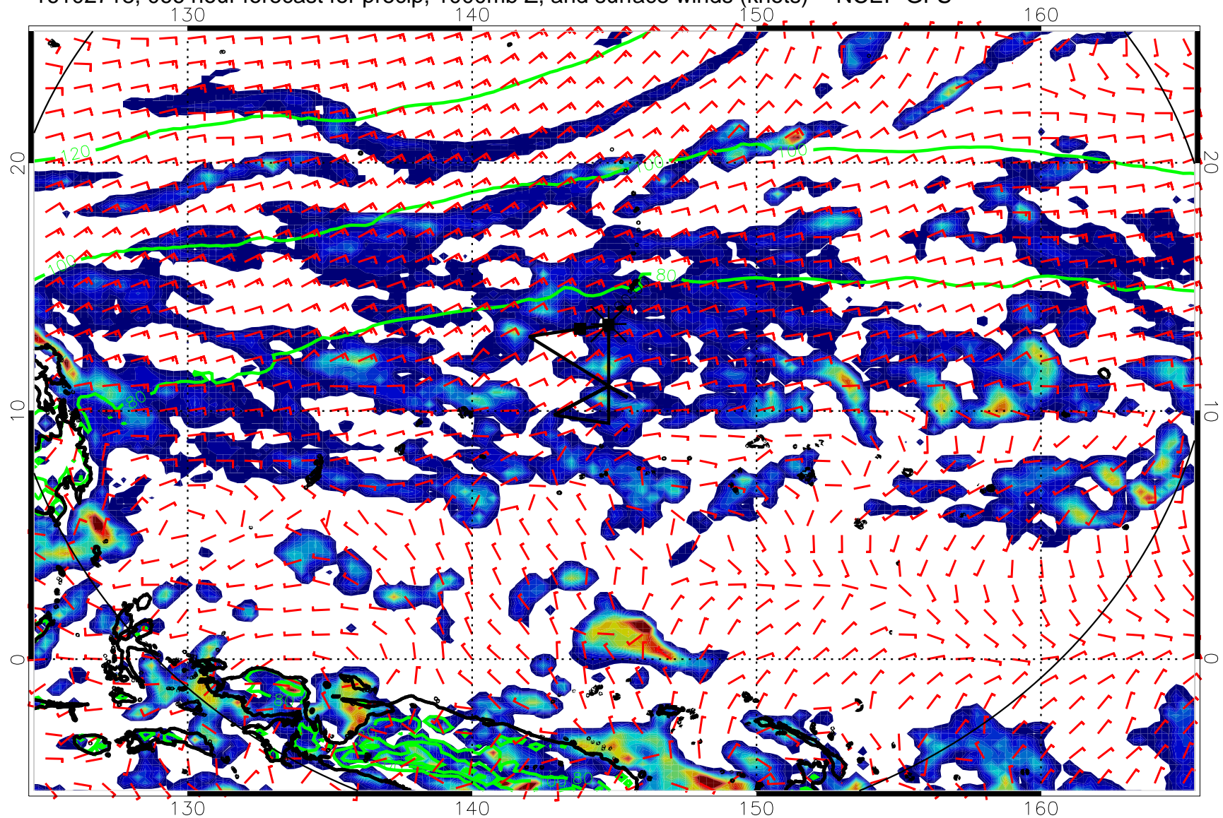
16102718, 066 hour forecast for precip, 1000mb Z, and surface winds (knots) -- NCEP GFS
