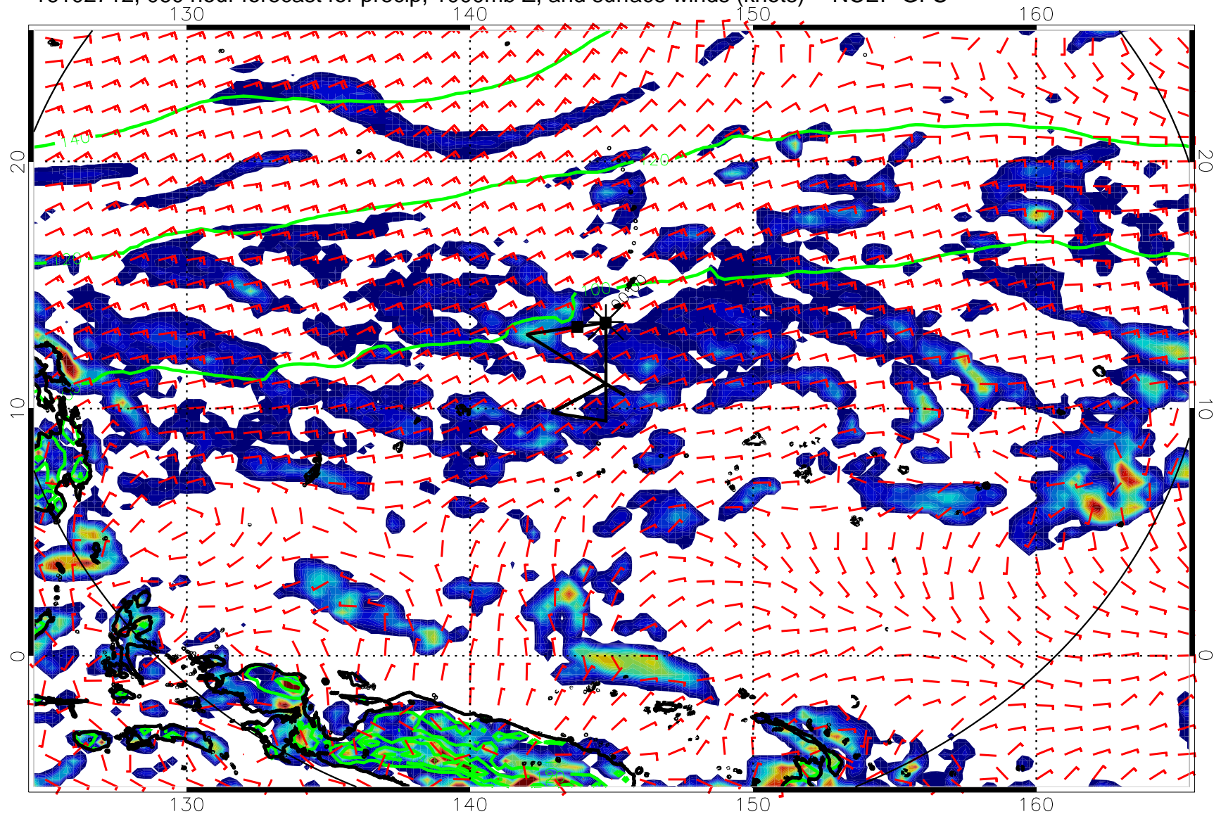
16102712, 060 hour forecast for precip, 1000mb Z, and surface winds (knots) -- NCEP GFS
