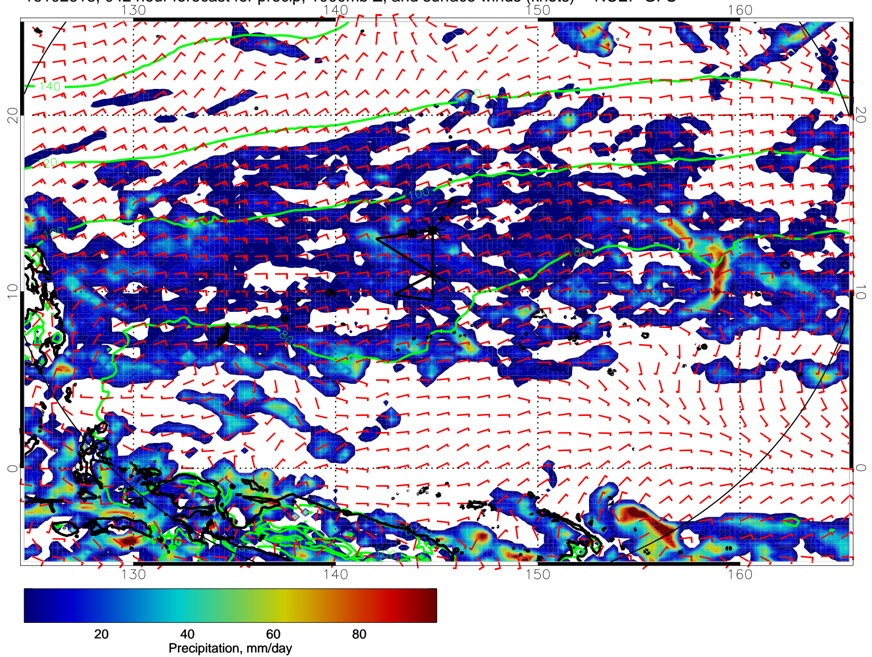
16102618, 042 hour forecast for precip, 1000mb Z, and surface winds (knots) -- NCEP GFS
