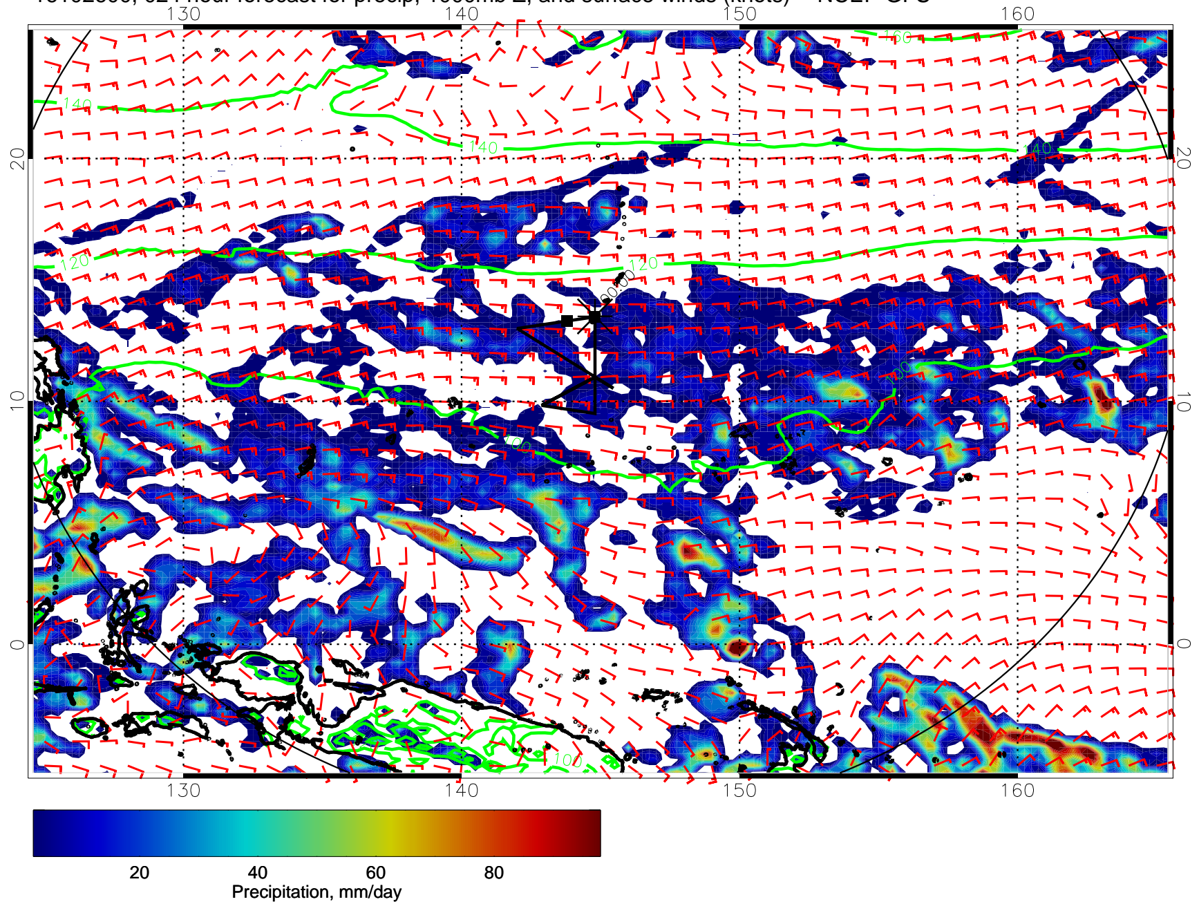
16102600, 024 hour forecast for precip, 1000mb Z, and surface winds (knots) -- NCEP GFS
