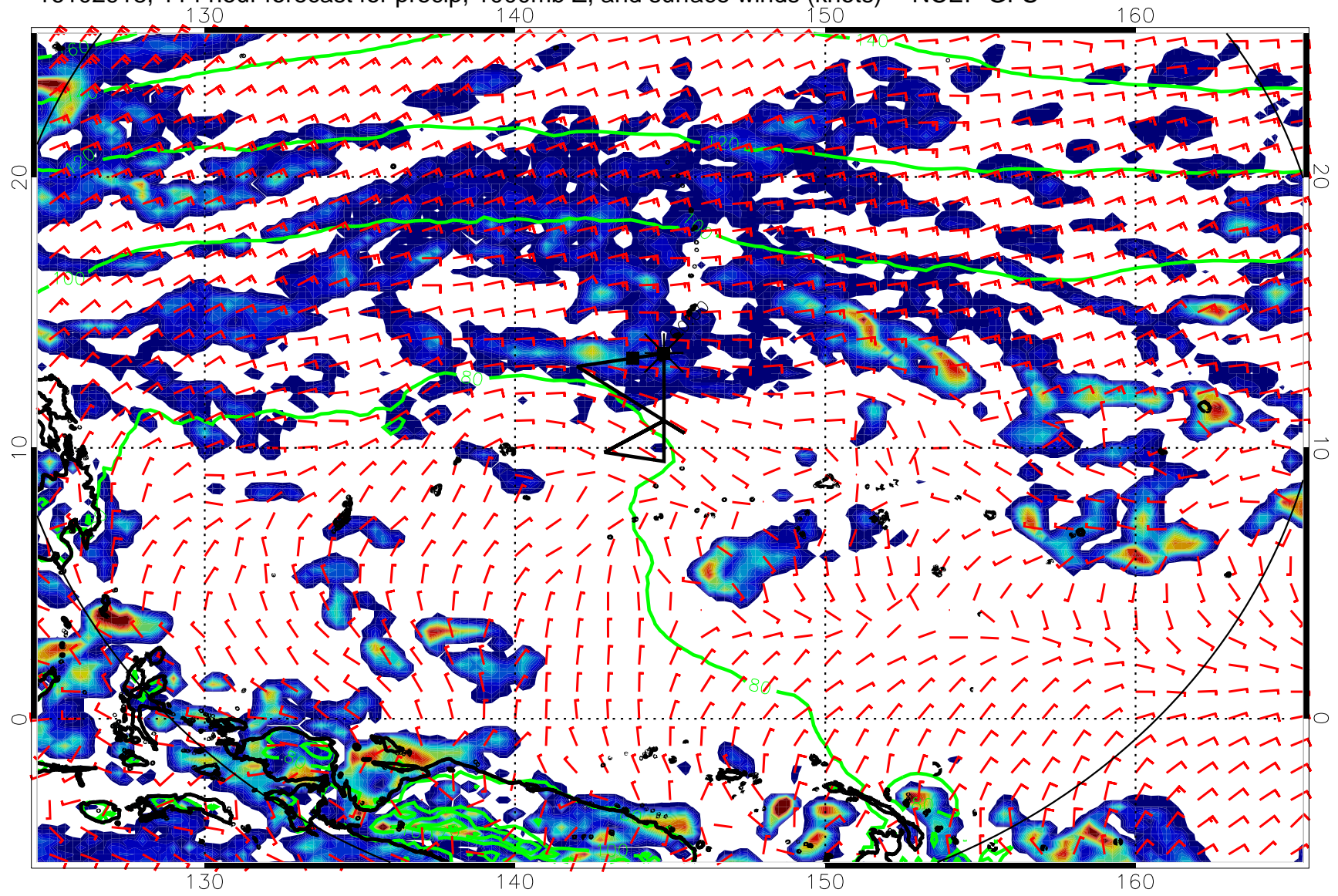
16102918, 114 hour forecast for precip, 1000mb Z, and surface winds (knots) -- NCEP GFS
