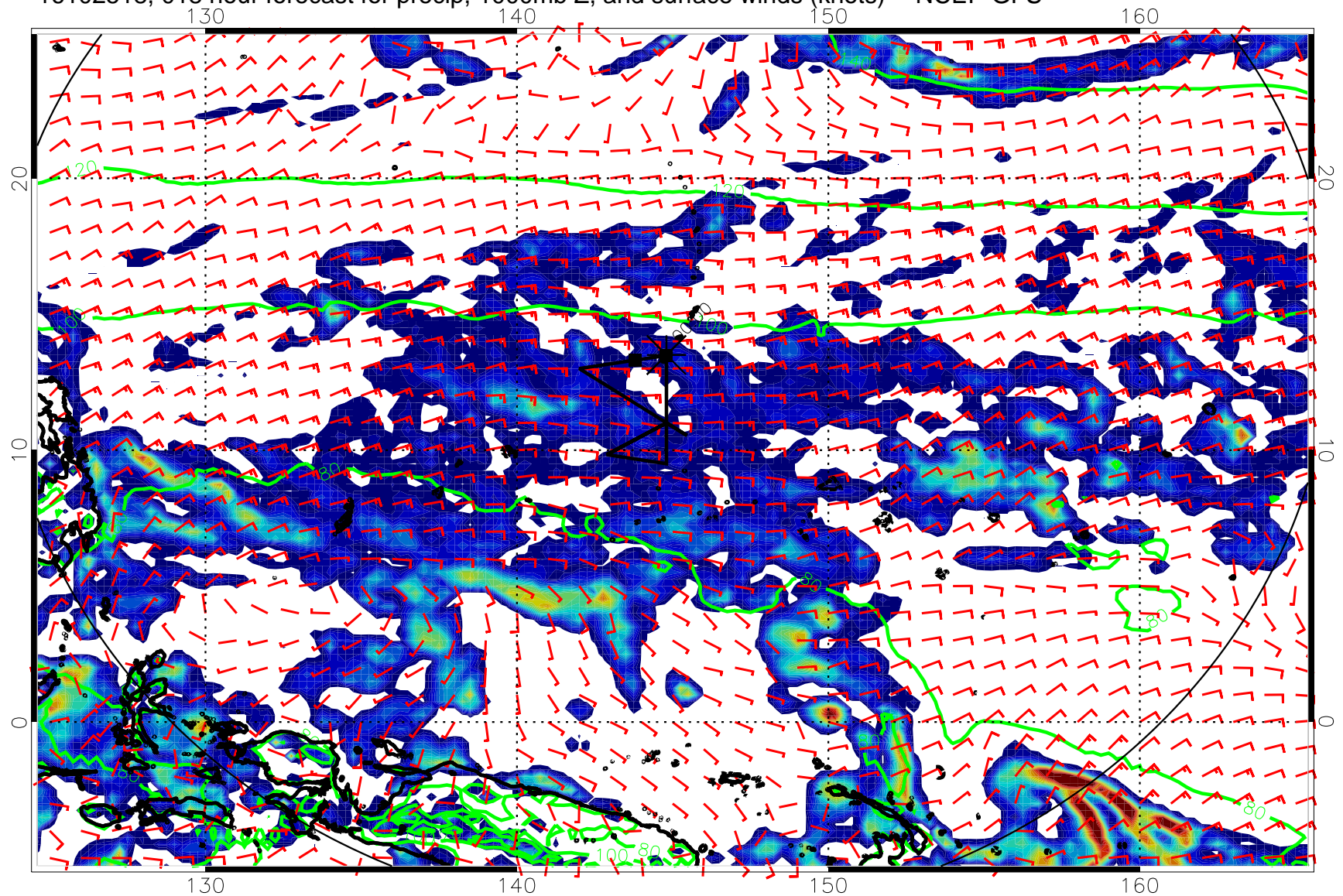
16102518, 018 hour forecast for precip, 1000mb Z, and surface winds (knots) -- NCEP GFS
