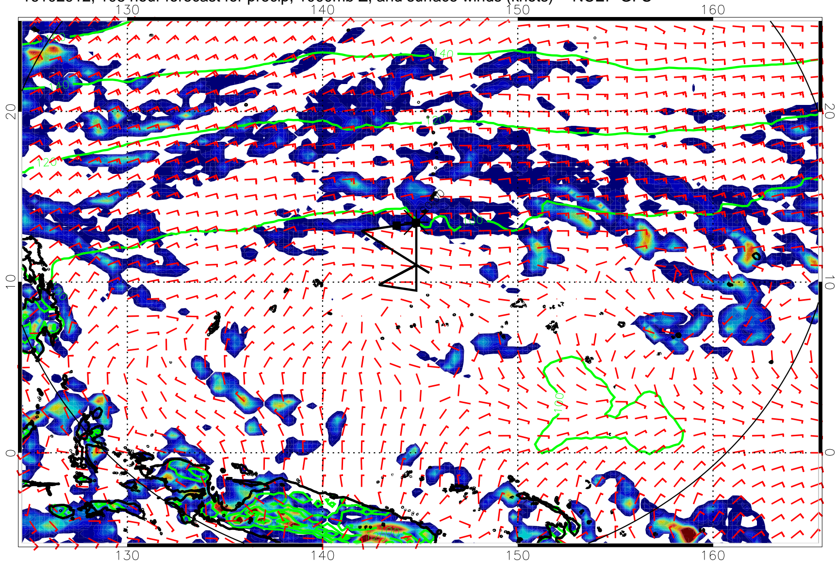
16102912, 108 hour forecast for precip, 1000mb Z, and surface winds (knots) -- NCEP GFS
