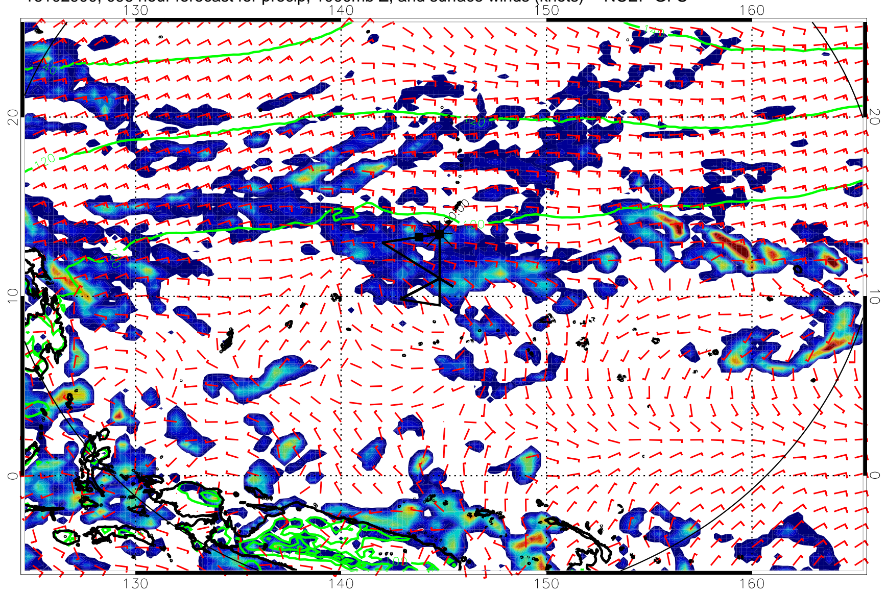
16102900, 096 hour forecast for precip, 1000mb Z, and surface winds (knots) -- NCEP GFS
