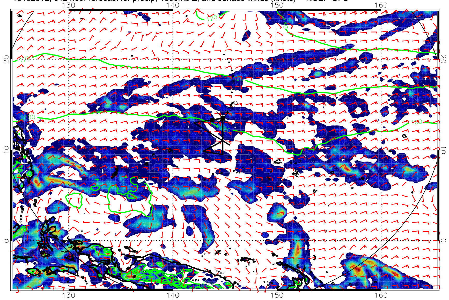
16102512, 012 hour forecast for precip, 1000mb Z, and surface winds (knots) -- NCEP GFS
