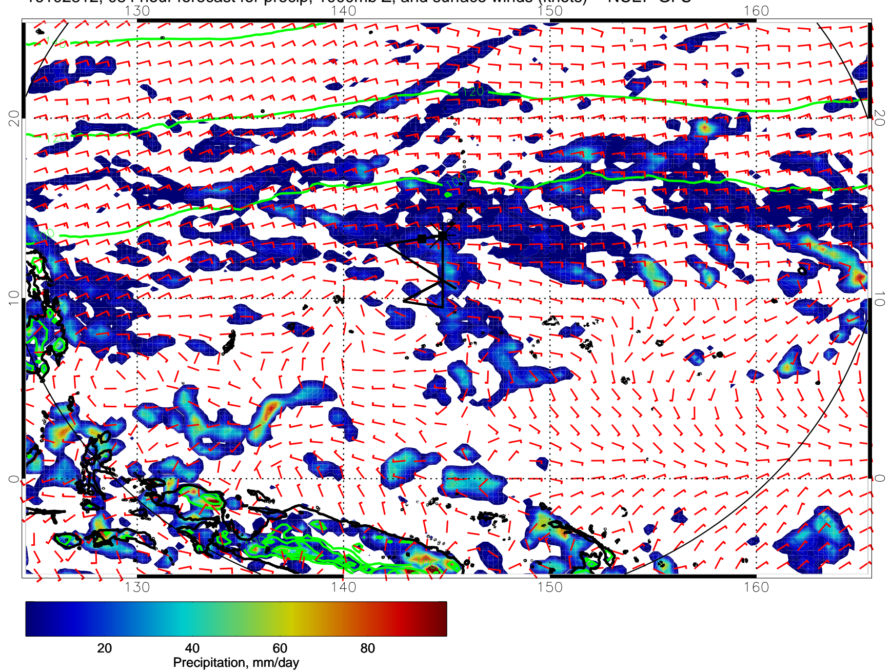
16102812, 084 hour forecast for precip, 1000mb Z, and surface winds (knots) -- NCEP GFS
