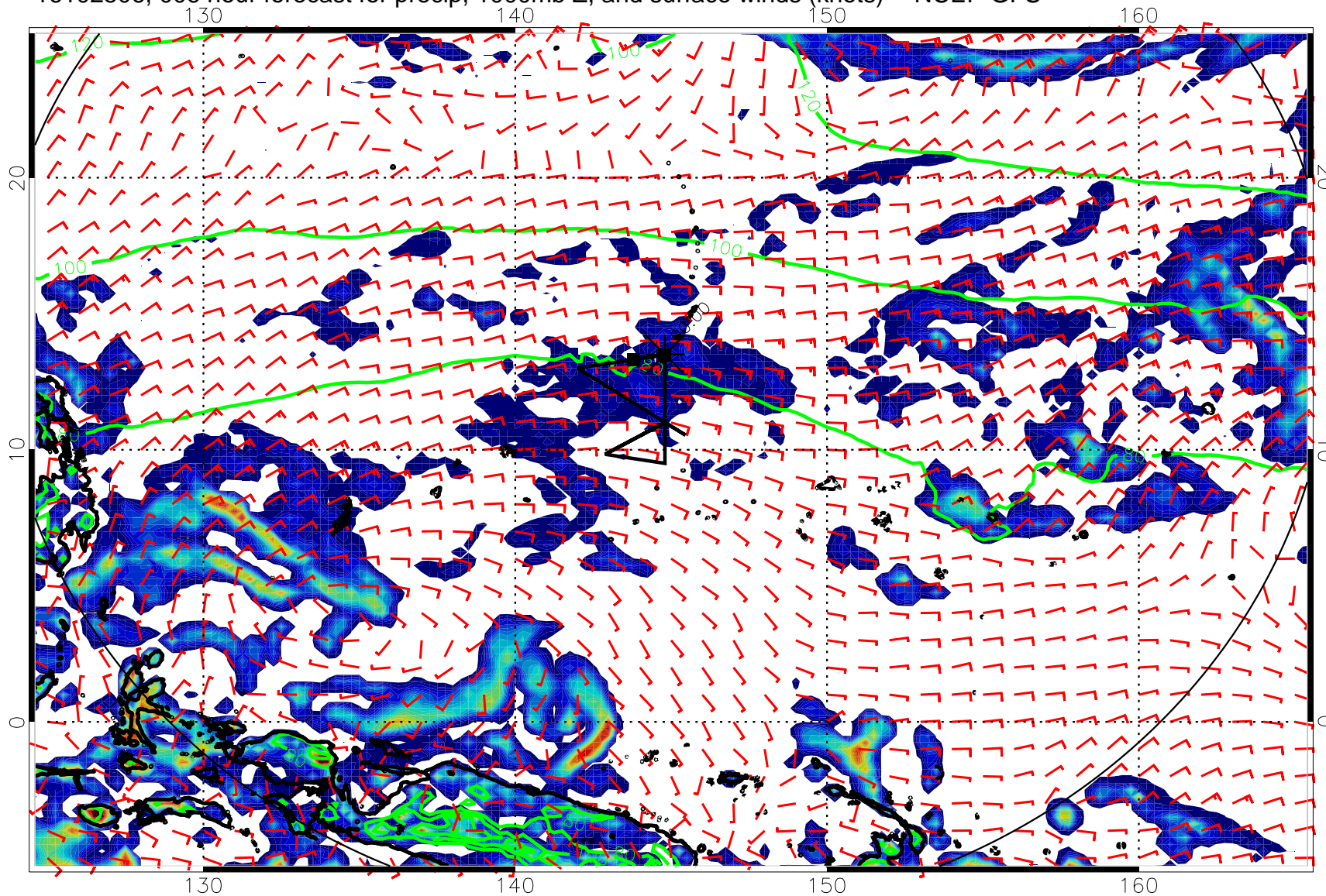
16102506, 006 hour forecast for precip, 1000mb Z, and surface winds (knots) -- NCEP GFS
