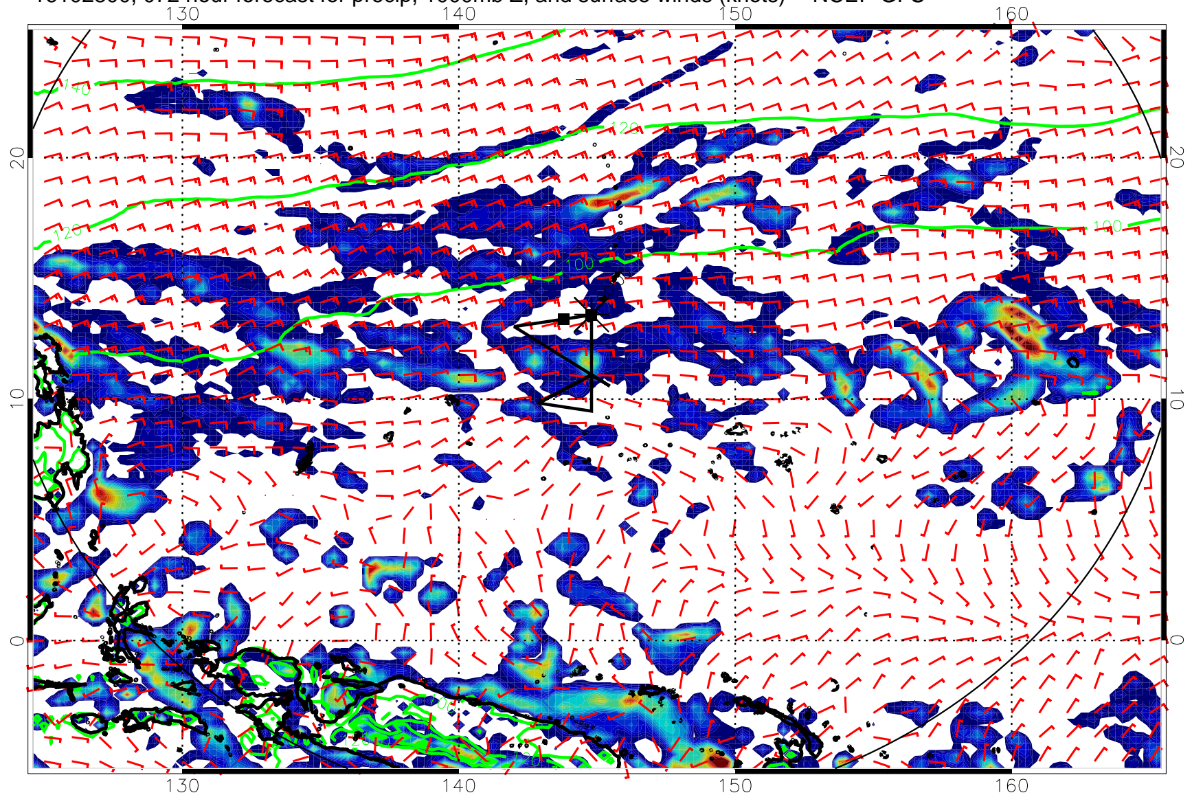
16102800, 072 hour forecast for precip, 1000mb Z, and surface winds (knots) -- NCEP GFS
