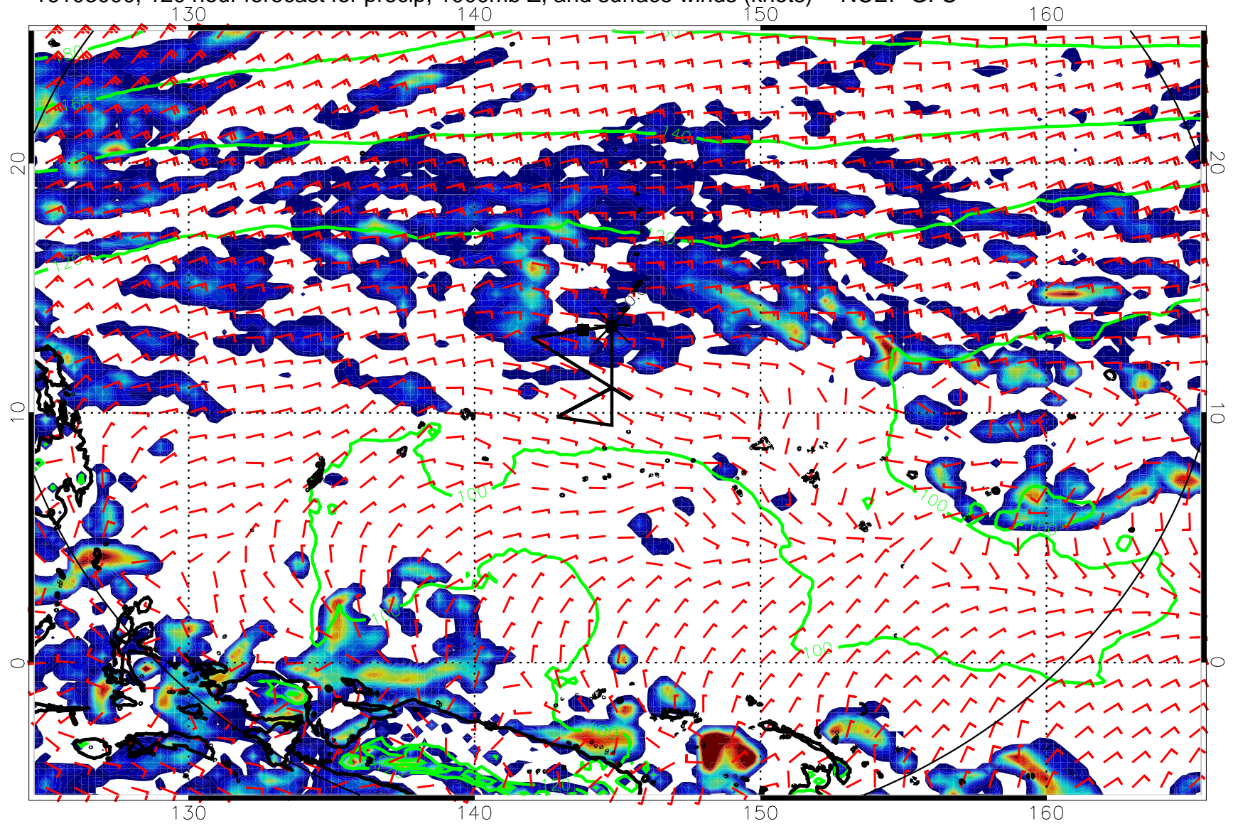
16103000, 120 hour forecast for precip, 1000mb Z, and surface winds (knots) -- NCEP GFS
