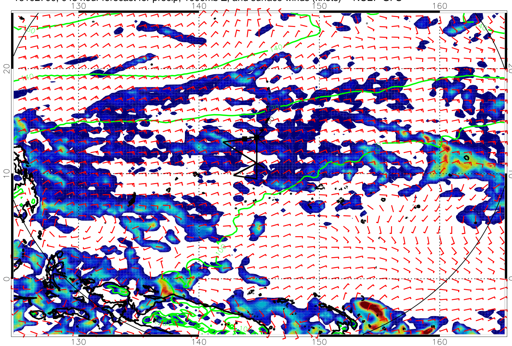
16102700, 048 hour forecast for precip, 1000mb Z, and surface winds (knots) -- NCEP GFS
