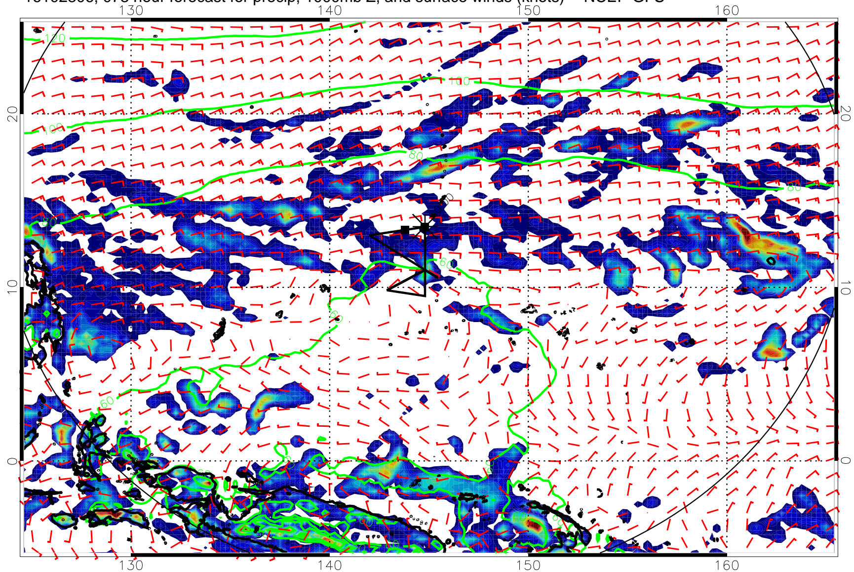
16102806, 078 hour forecast for precip, 1000mb Z, and surface winds (knots) -- NCEP GFS
