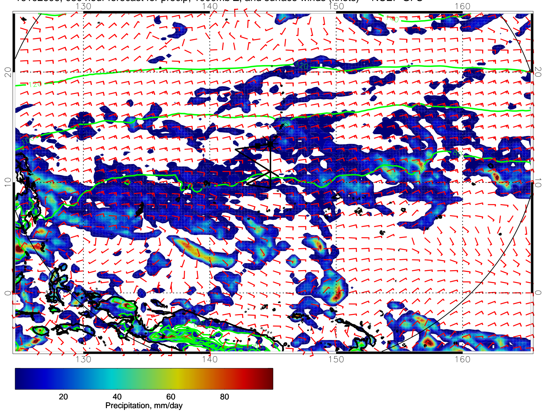
16102606, 030 hour forecast for precip, 1000mb Z, and surface winds (knots) -- NCEP GFS
