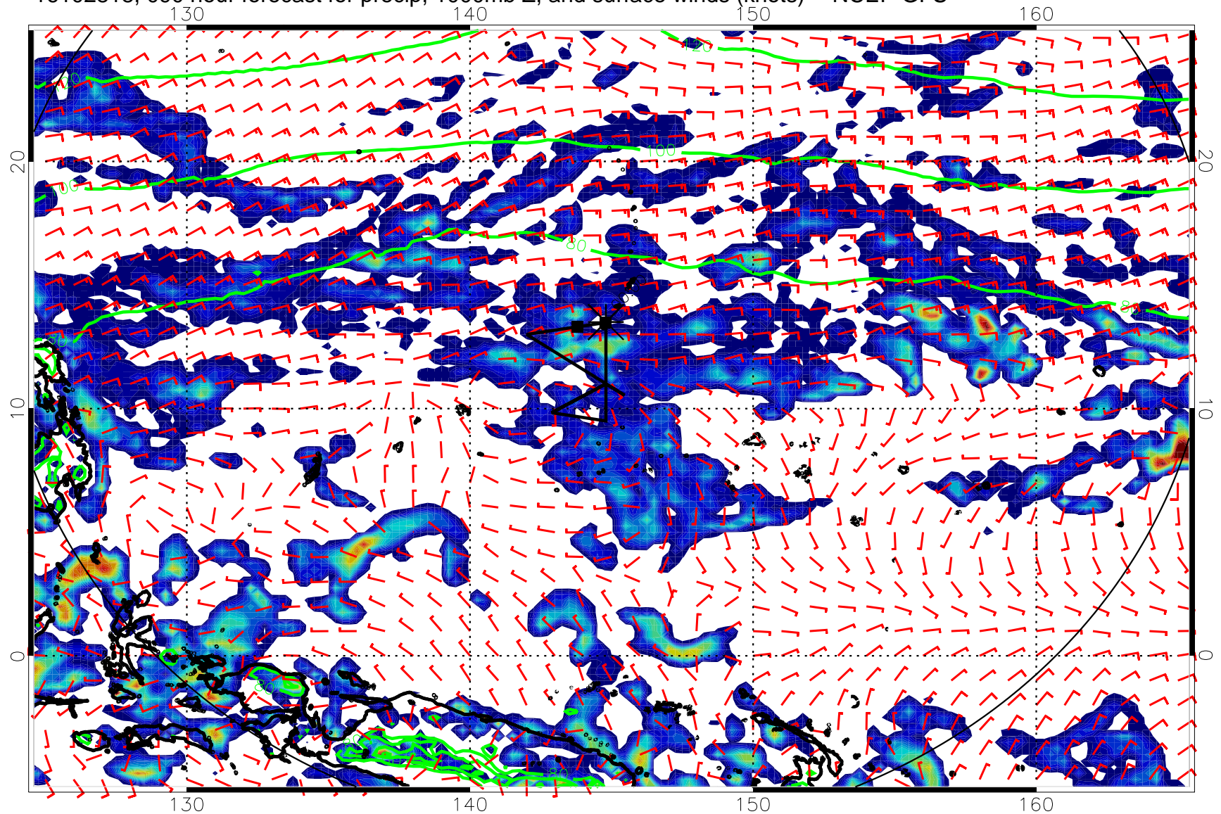
16102818, 090 hour forecast for precip, 1000mb Z, and surface winds (knots) -- NCEP GFS
