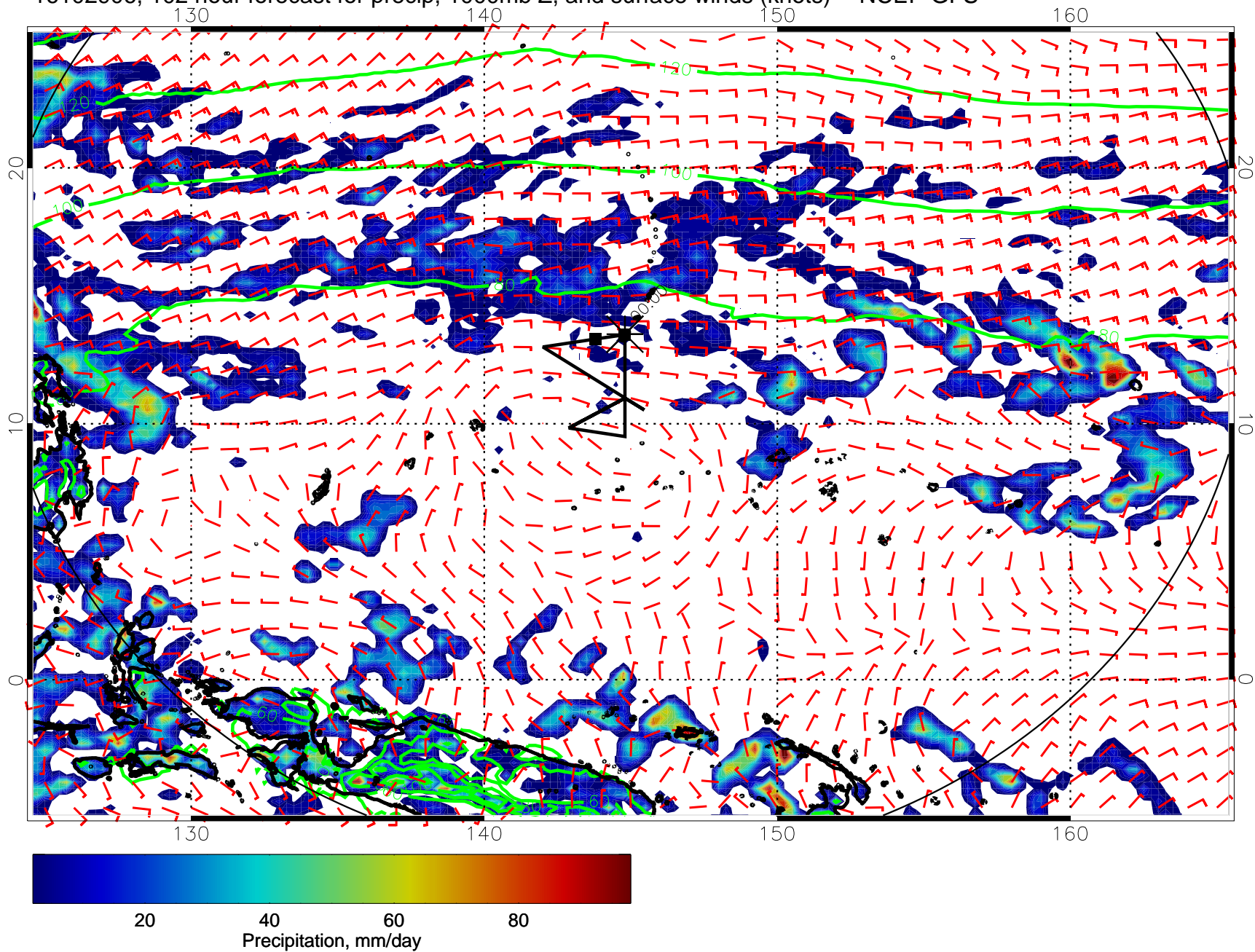
16102906, 102 hour forecast for precip, 1000mb Z, and surface winds (knots) -- NCEP GFS
