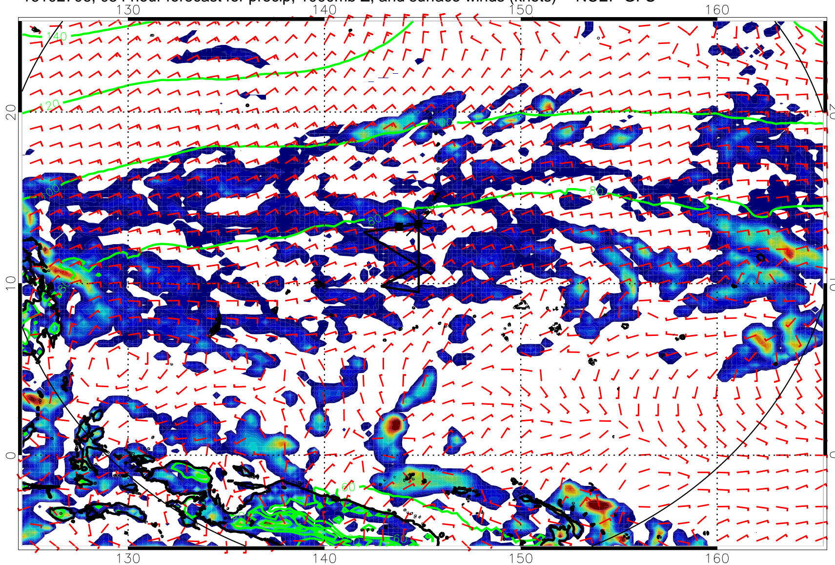
16102706, 054 hour forecast for precip, 1000mb Z, and surface winds (knots) -- NCEP GFS
