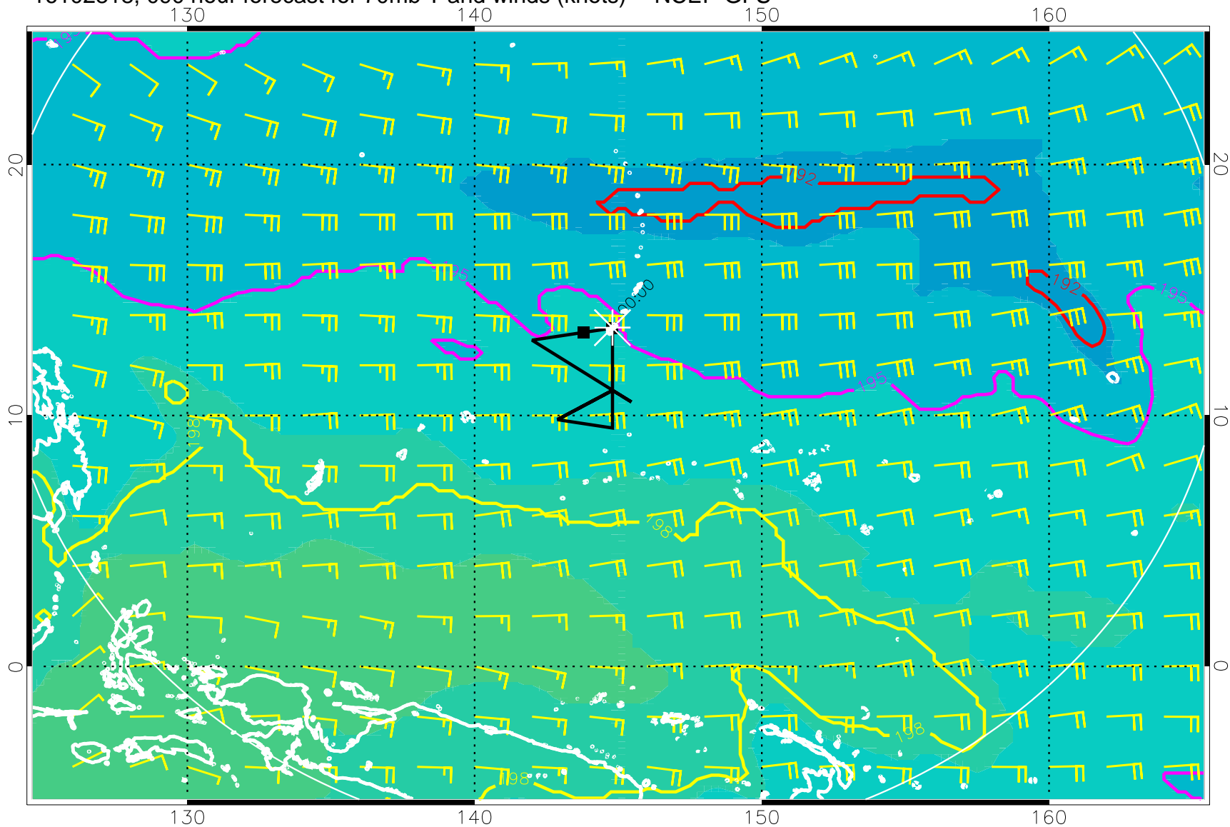
16102818, 090 hour forecast for 70mb T and winds (knots) -- NCEP GFS
