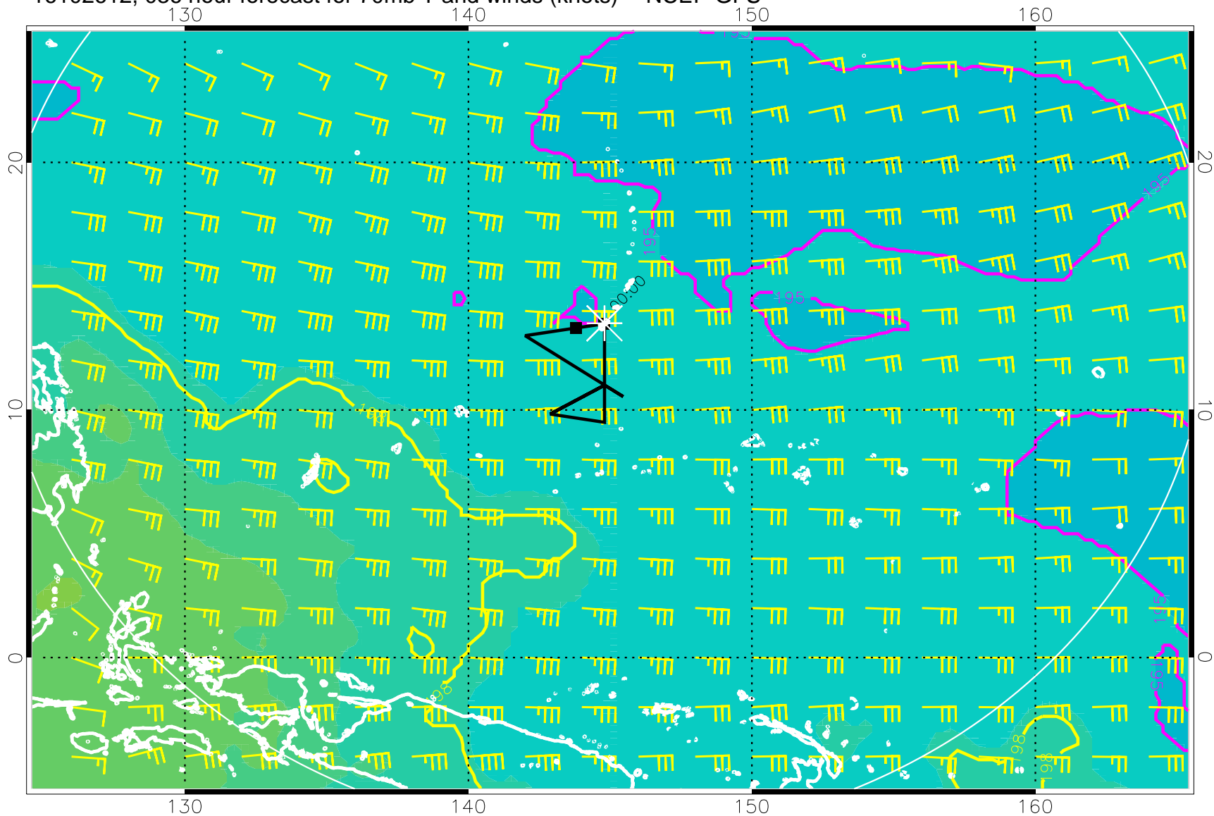
16102612, 036 hour forecast for 70mb T and winds (knots) -- NCEP GFS
