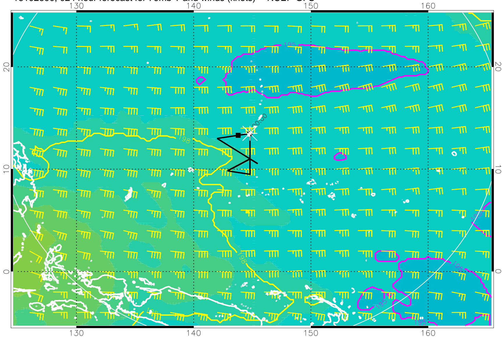
16102600, 024 hour forecast for 70mb T and winds (knots) -- NCEP GFS
