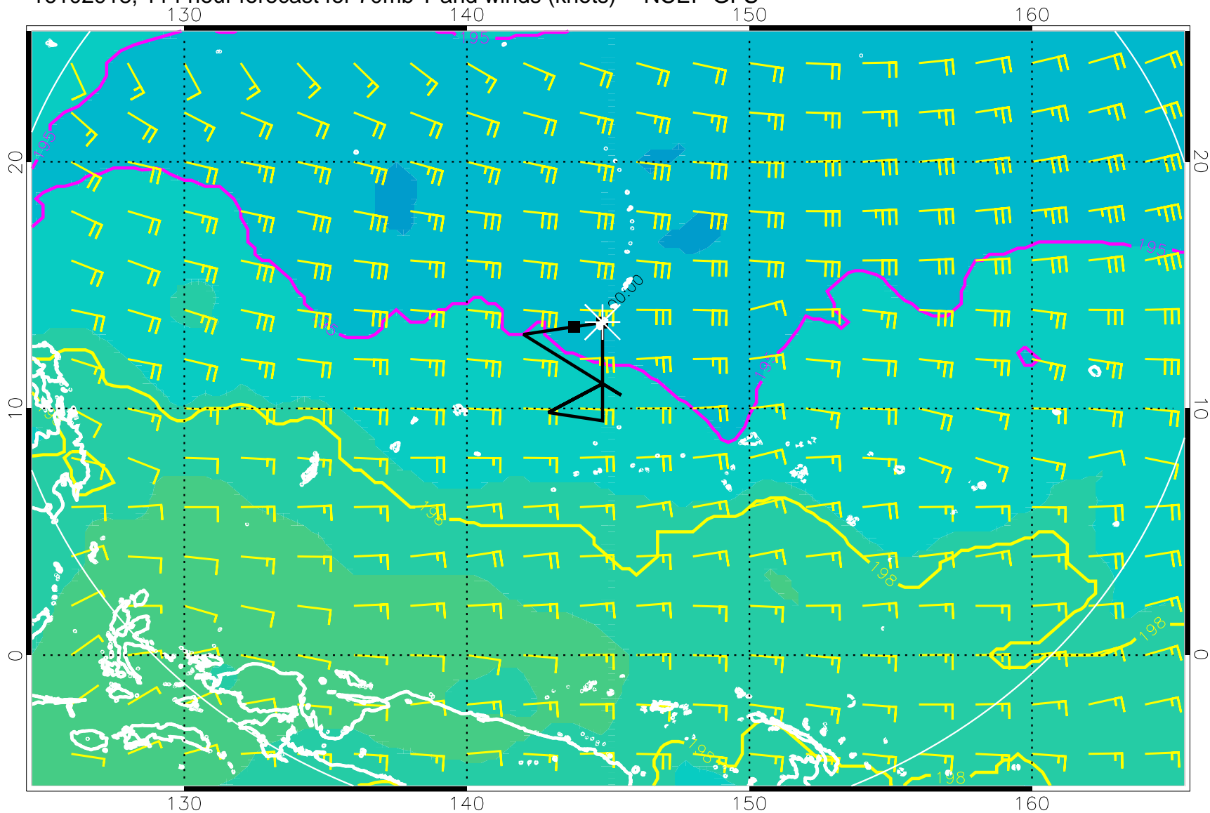
16102918, 114 hour forecast for 70mb T and winds (knots) -- NCEP GFS
