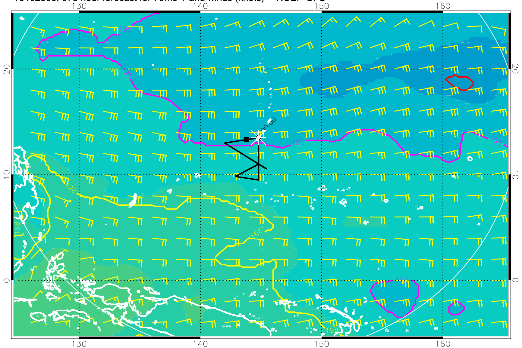
16102806, 078 hour forecast for 70mb T and winds (knots) -- NCEP GFS
