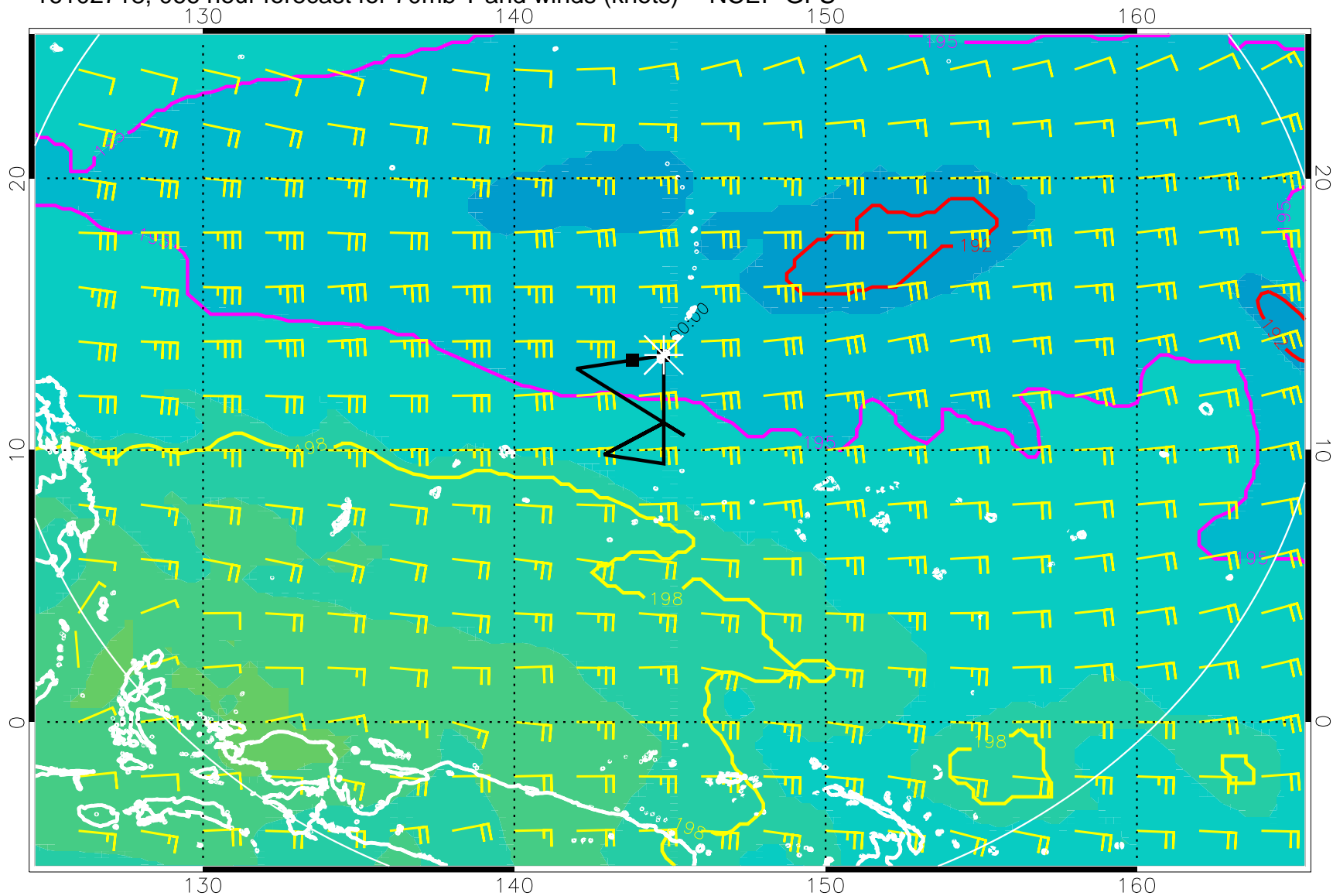
16102718, 066 hour forecast for 70mb T and winds (knots) -- NCEP GFS
