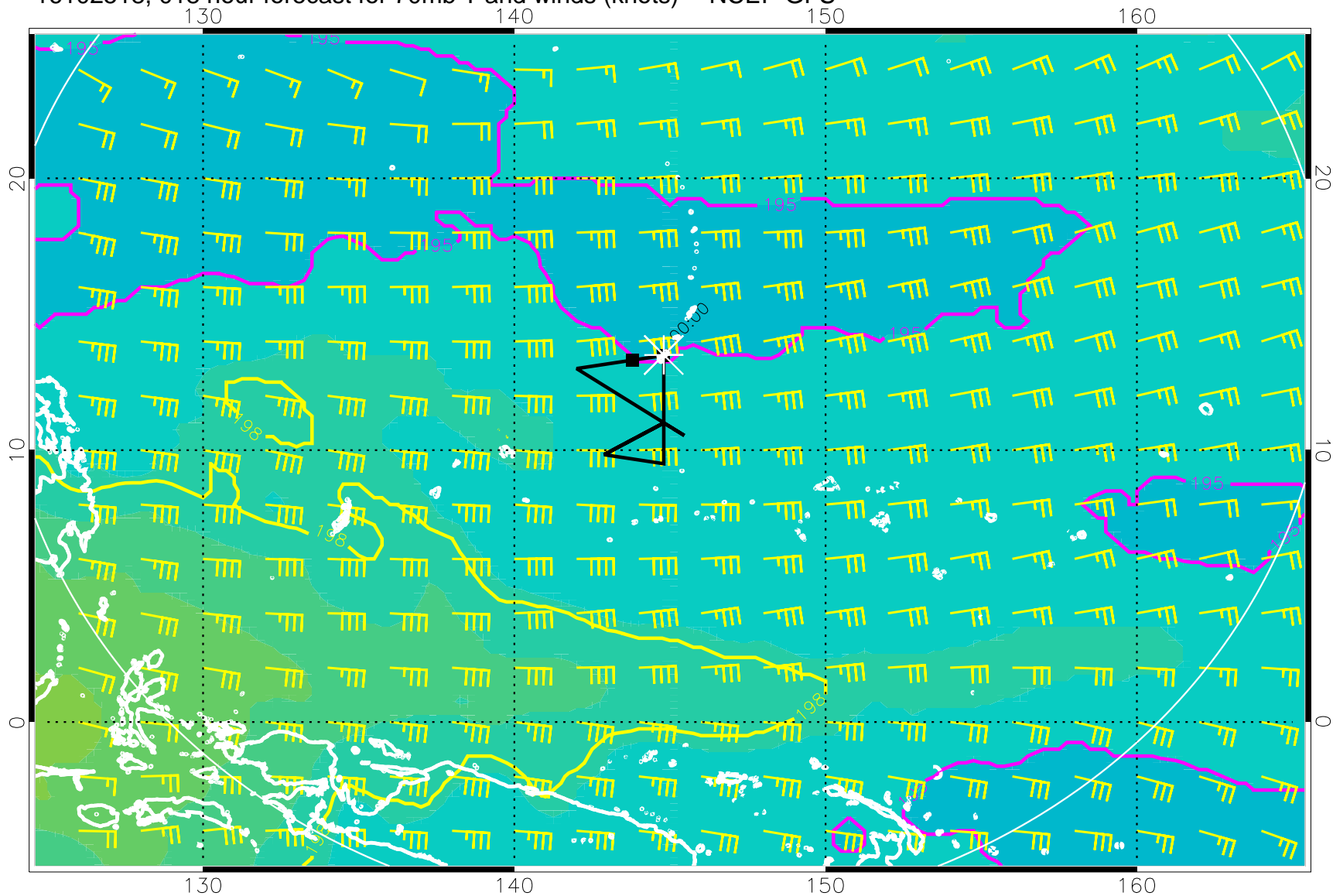
16102518, 018 hour forecast for 70mb T and winds (knots) -- NCEP GFS
