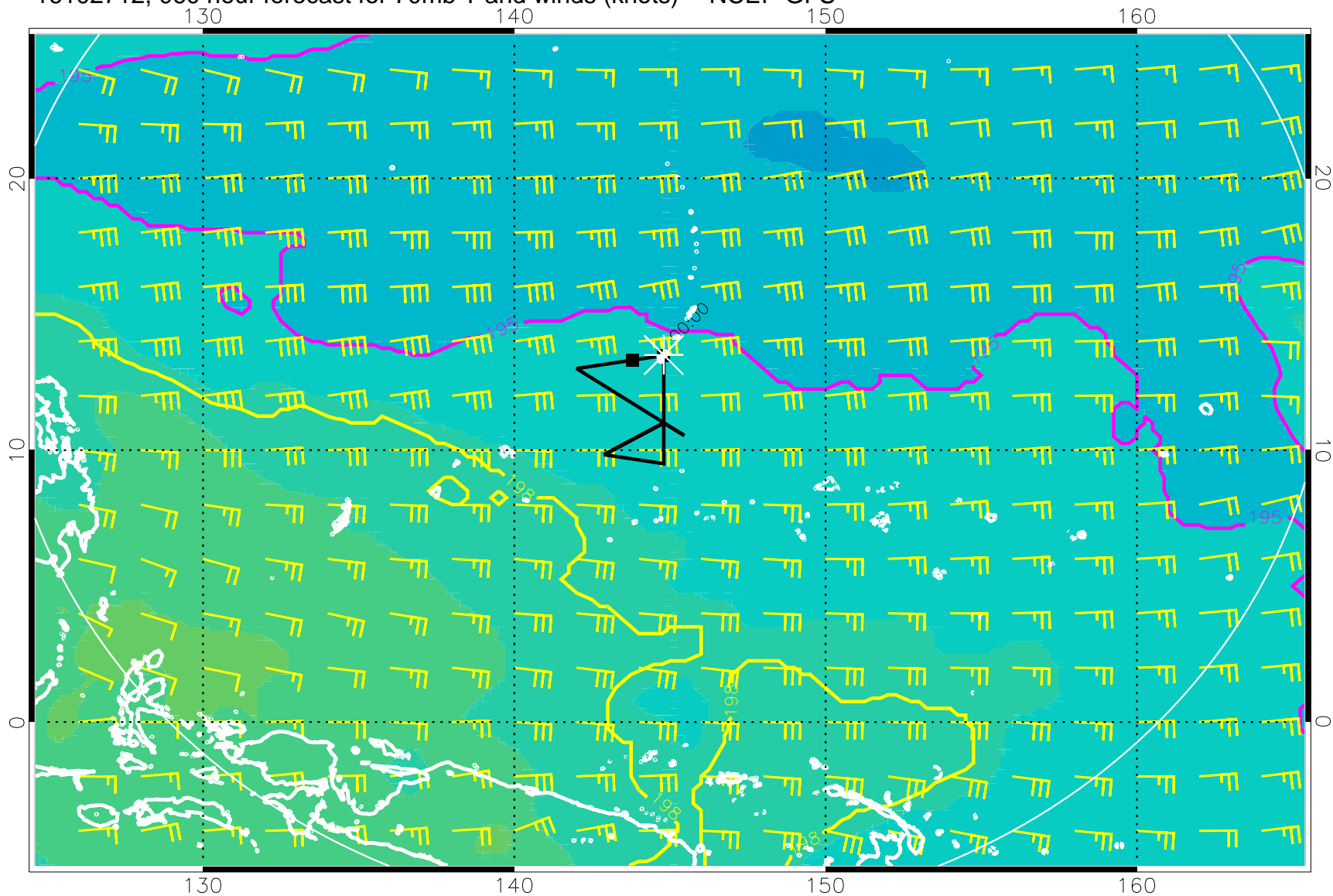
16102712, 060 hour forecast for 70mb T and winds (knots) -- NCEP GFS
