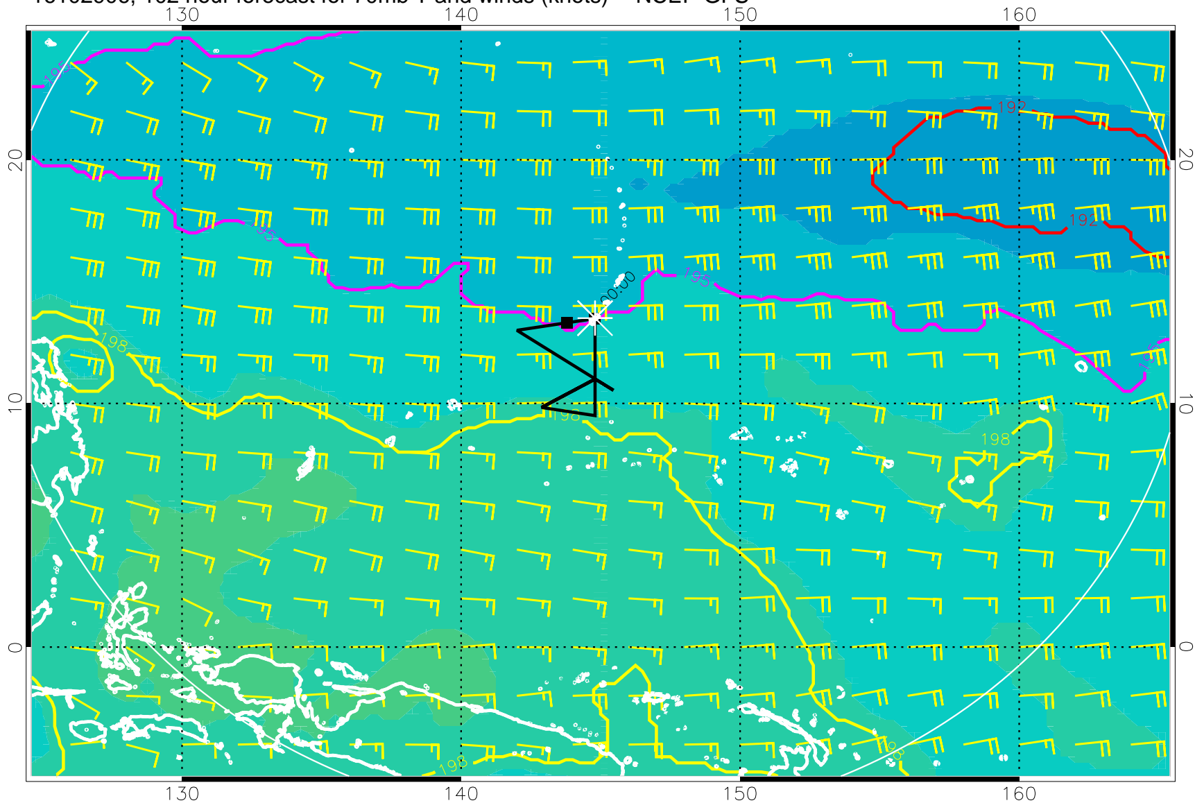
16102906, 102 hour forecast for 70mb T and winds (knots) -- NCEP GFS
