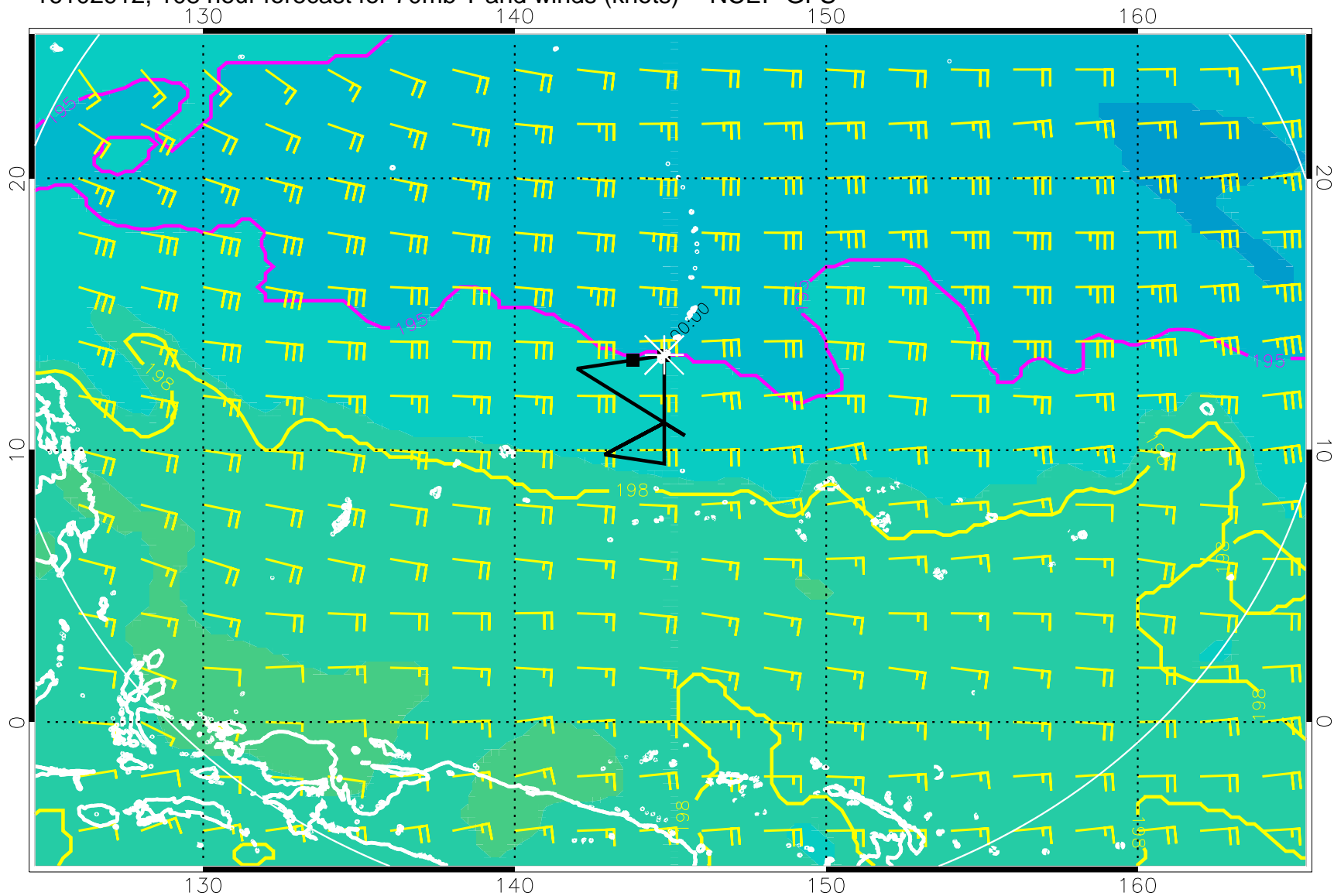
16102912, 108 hour forecast for 70mb T and winds (knots) -- NCEP GFS
