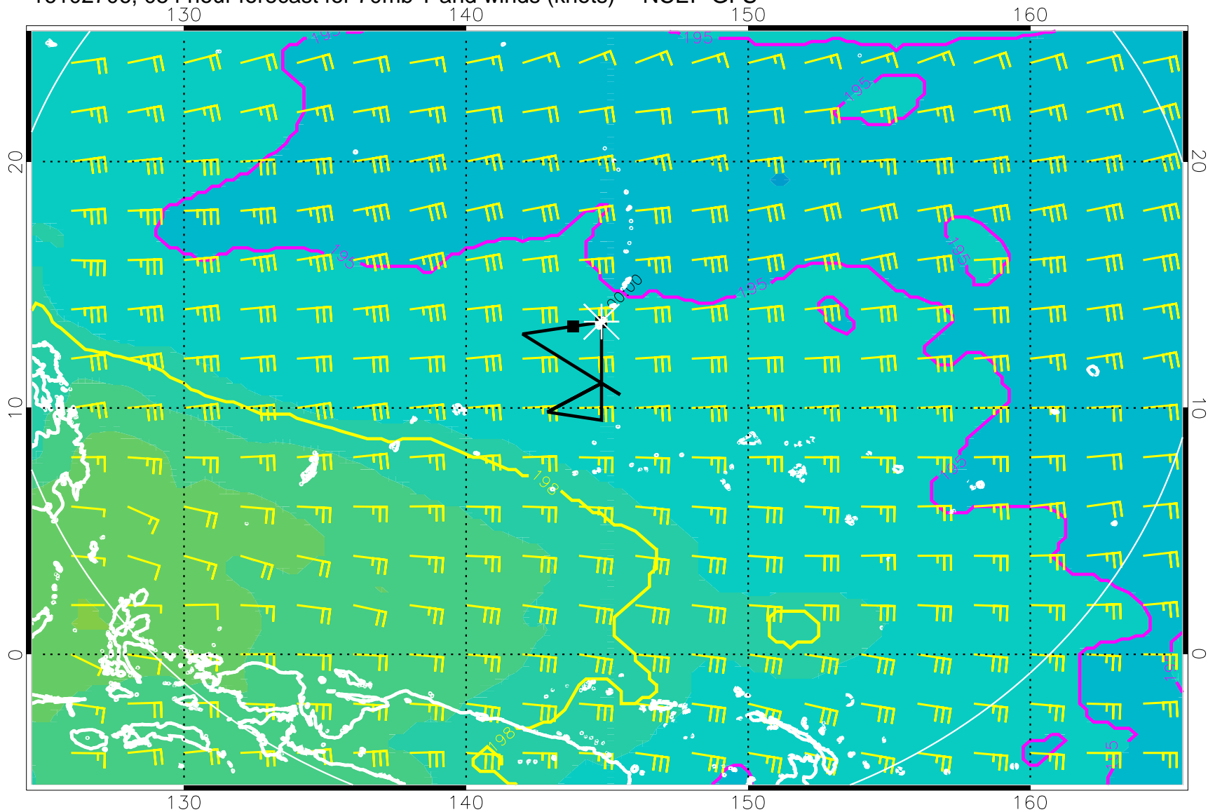
16102706, 054 hour forecast for 70mb T and winds (knots) -- NCEP GFS
