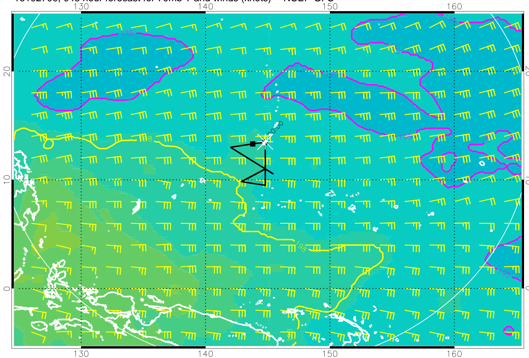
16102700, 048 hour forecast for 70mb T and winds (knots) -- NCEP GFS
