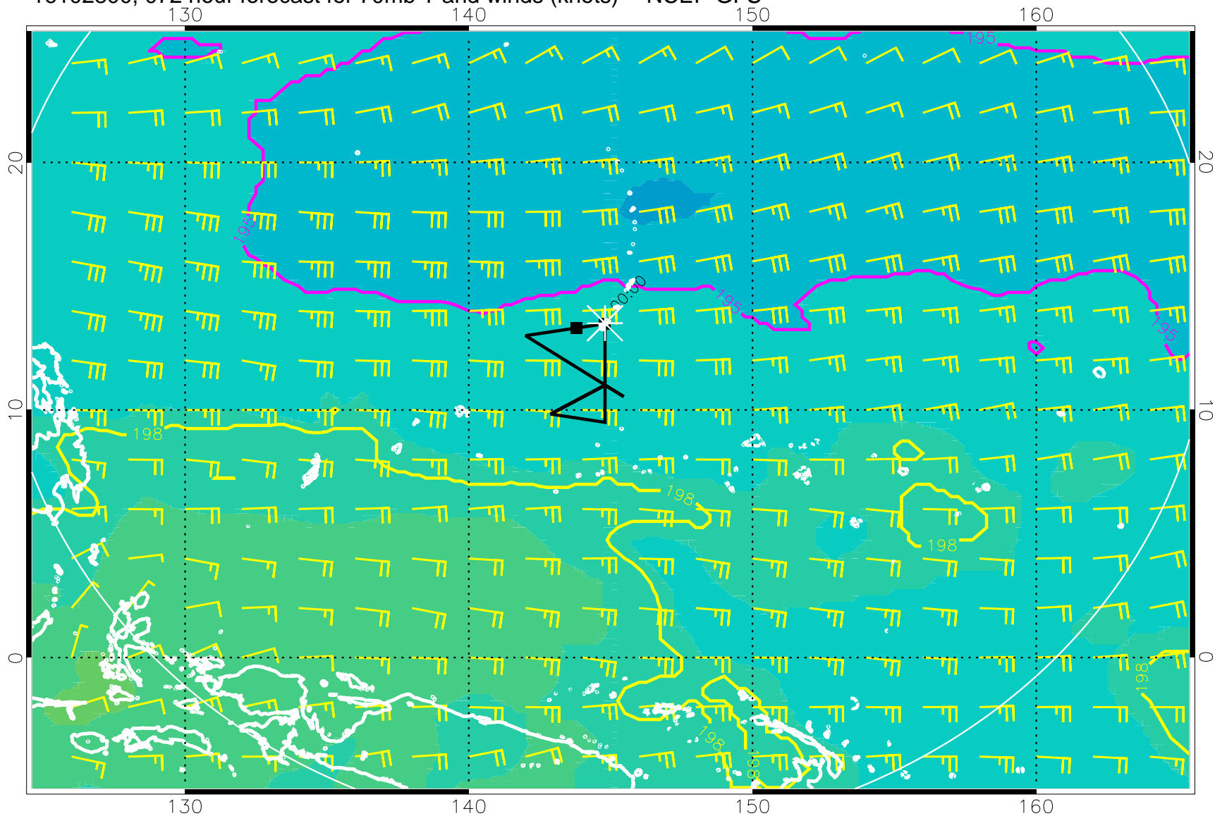
16102800, 072 hour forecast for 70mb T and winds (knots) -- NCEP GFS
