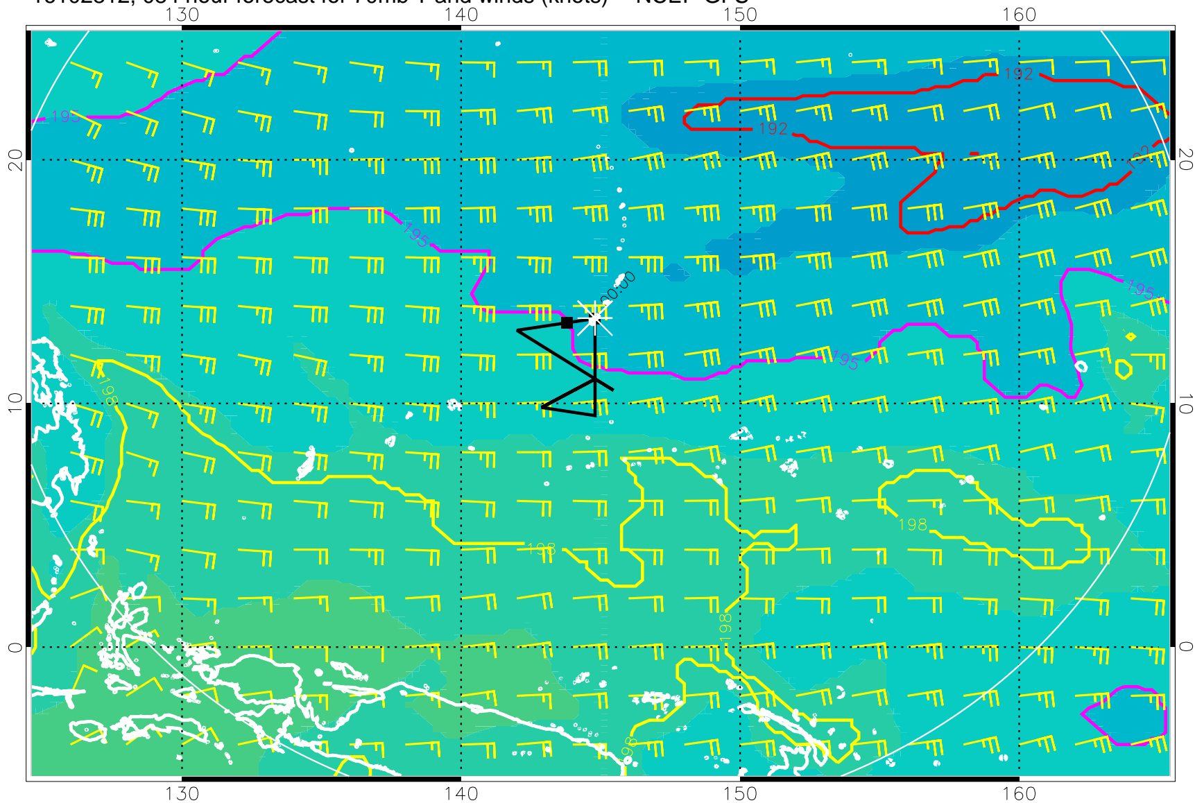
16102812, 084 hour forecast for 70mb T and winds (knots) -- NCEP GFS
