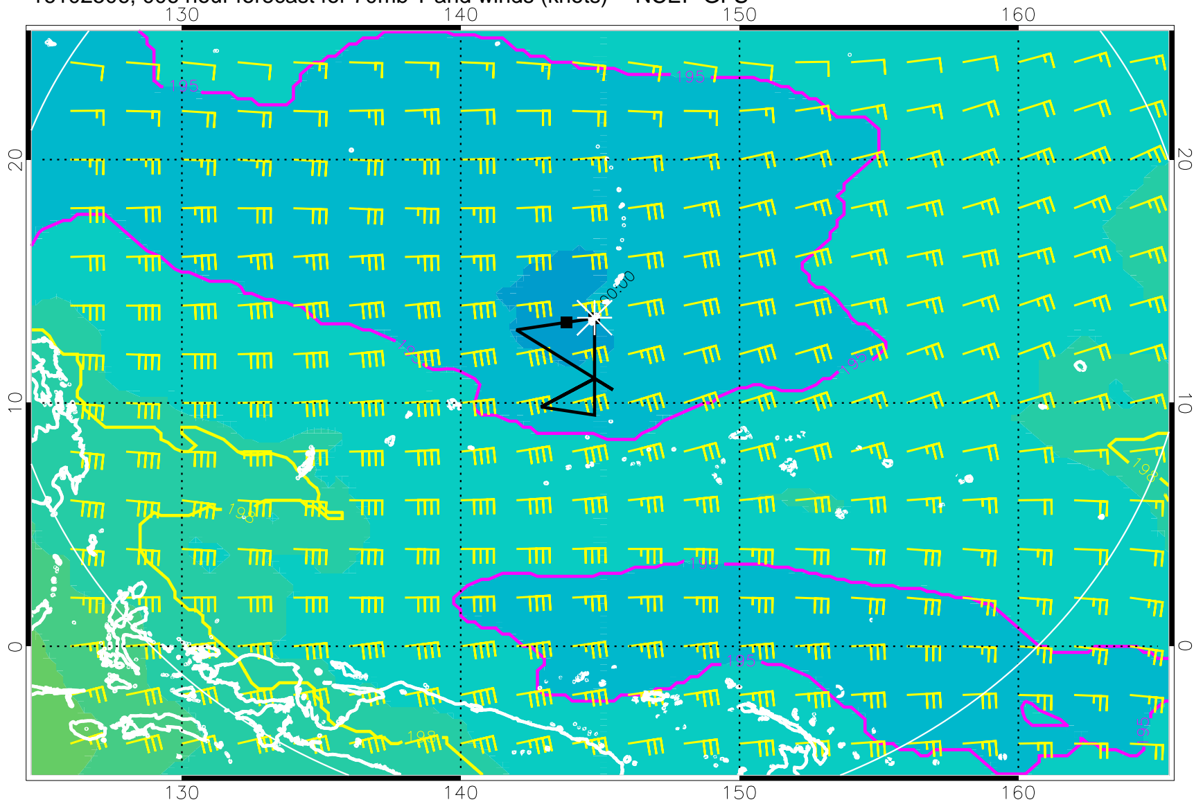
16102506, 006 hour forecast for 70mb T and winds (knots) -- NCEP GFS
