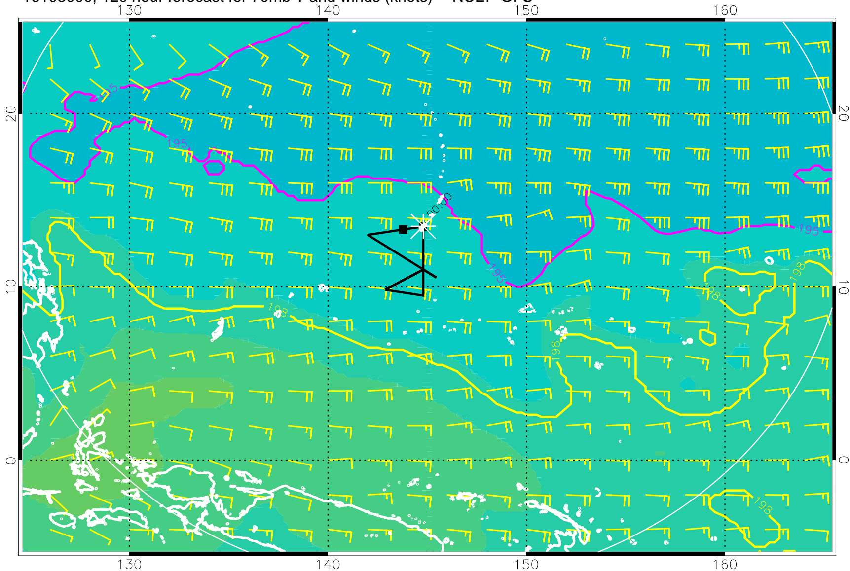
16103000, 120 hour forecast for 70mb T and winds (knots) -- NCEP GFS
