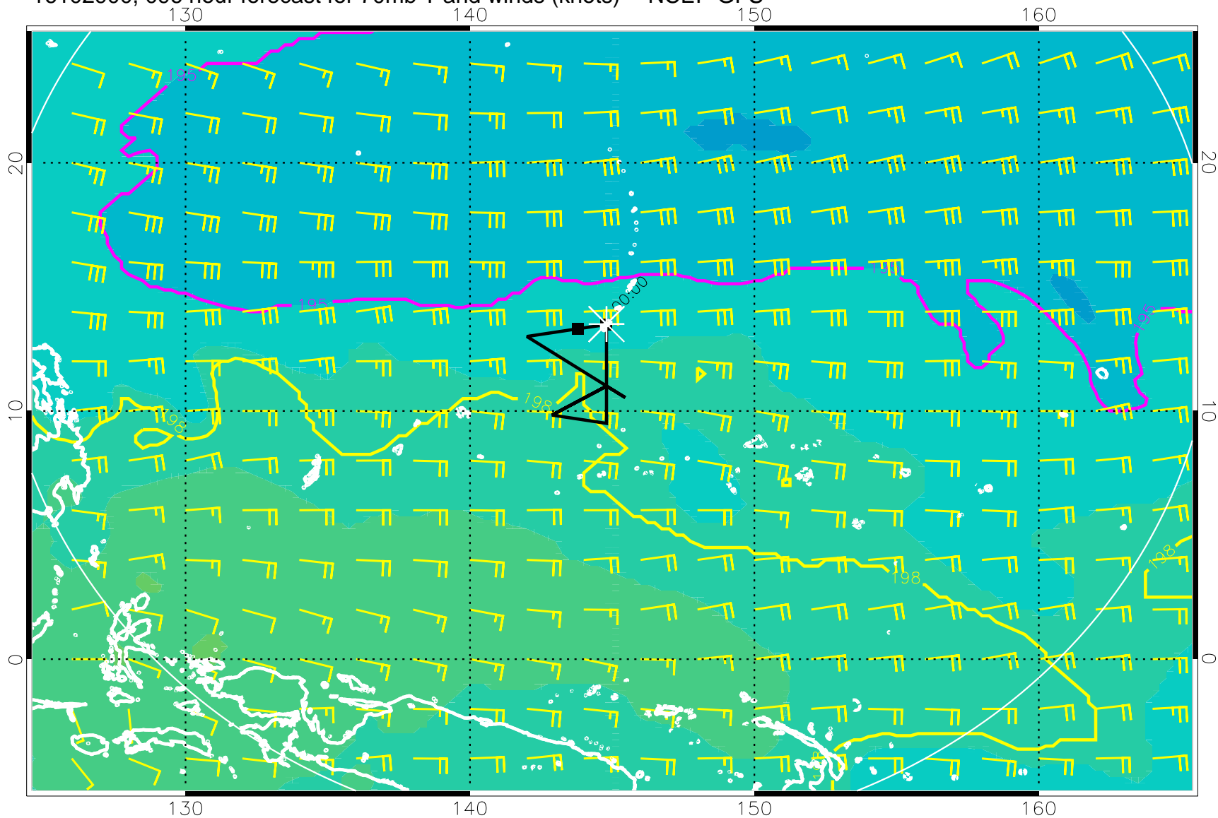
16102900, 096 hour forecast for 70mb T and winds (knots) -- NCEP GFS
