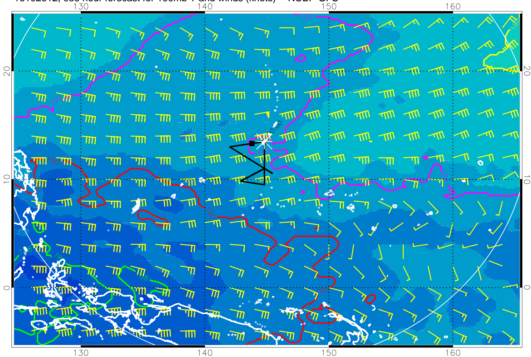
16102612, 036 hour forecast for 100mb T and winds (knots) -- NCEP GFS
