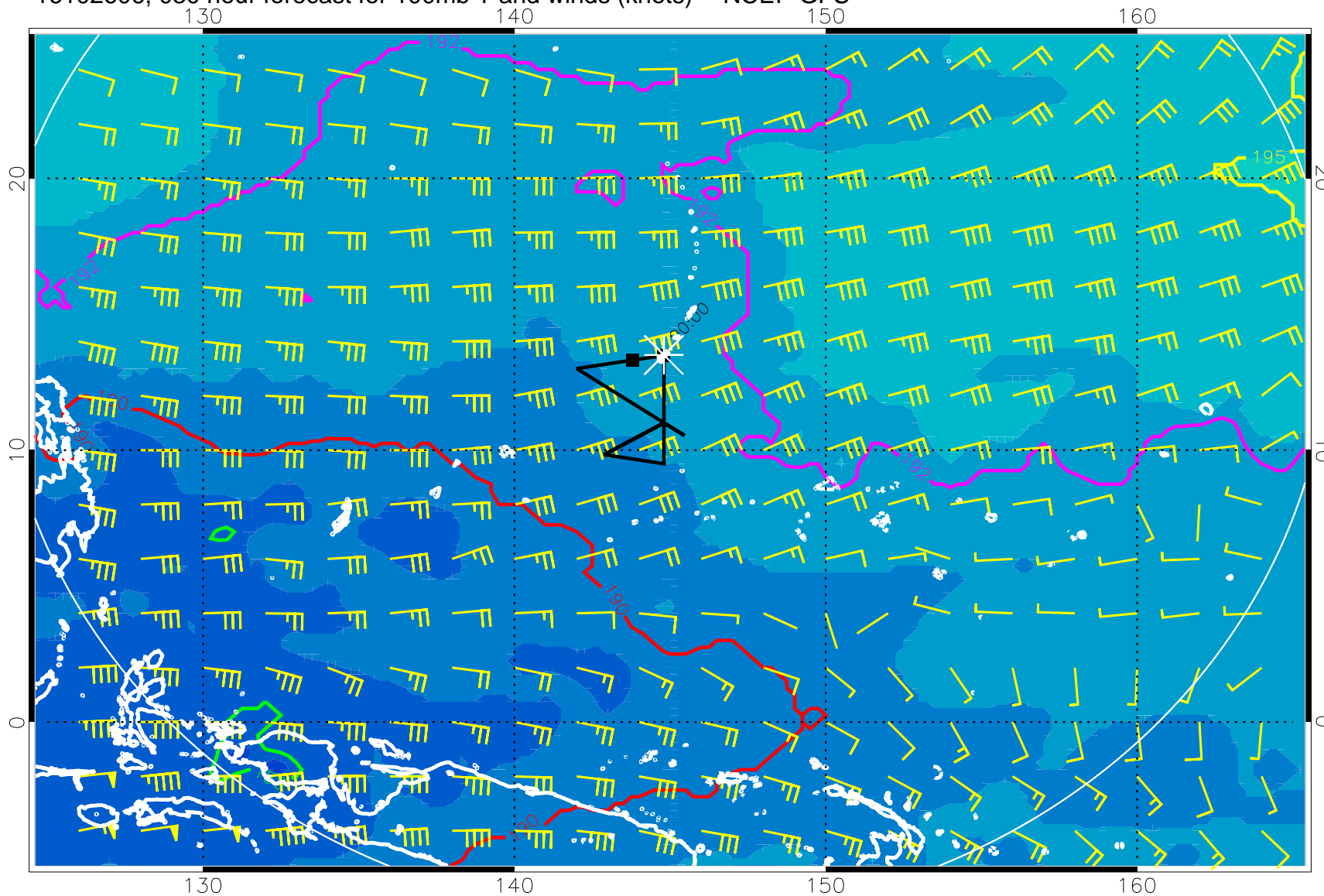
16102606, 030 hour forecast for 100mb T and winds (knots) -- NCEP GFS
