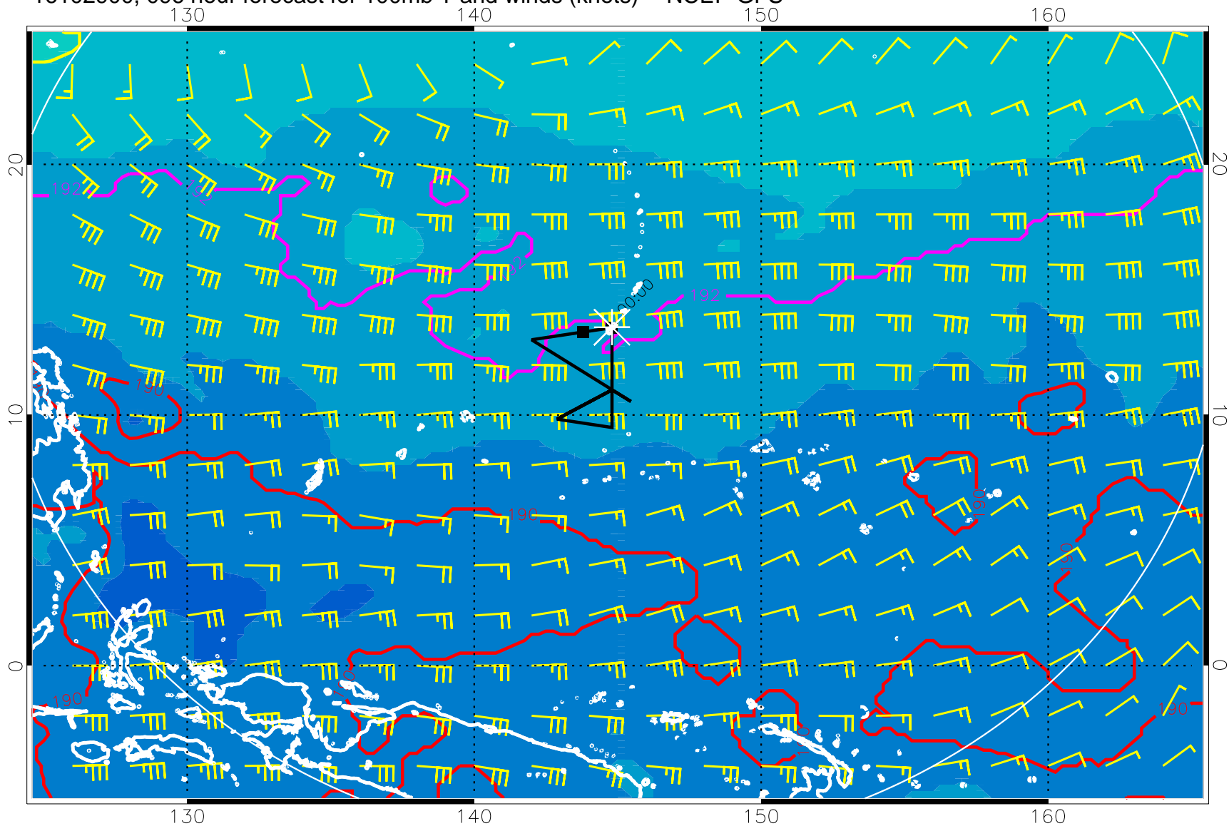
16102900, 096 hour forecast for 100mb T and winds (knots) -- NCEP GFS
