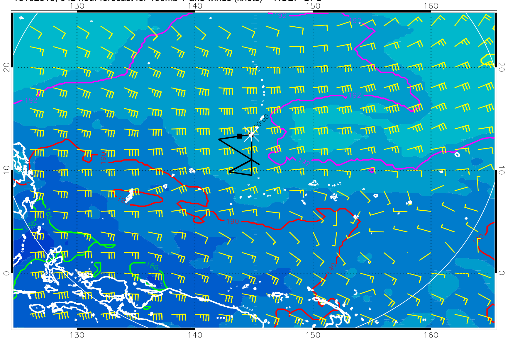
16102618, 042 hour forecast for 100mb T and winds (knots) -- NCEP GFS
