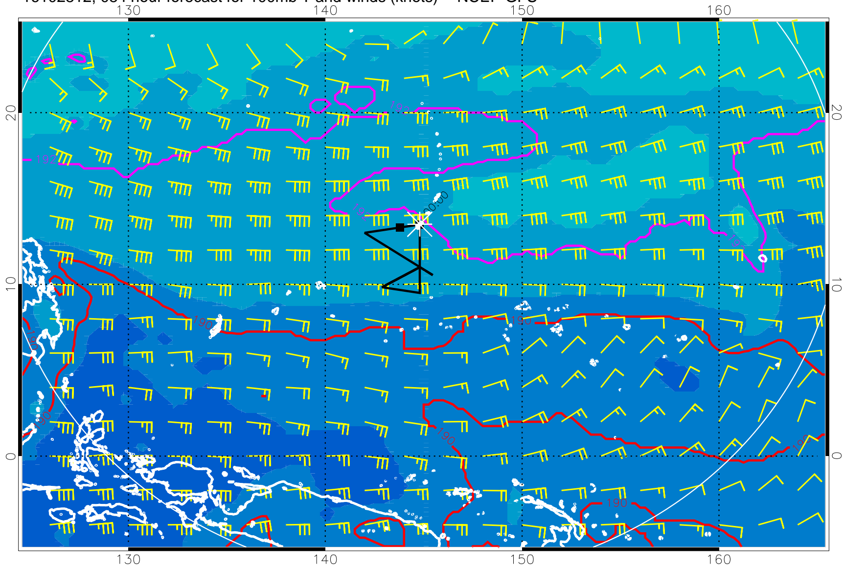
16102812, 084 hour forecast for 100mb T and winds (knots) -- NCEP GFS
