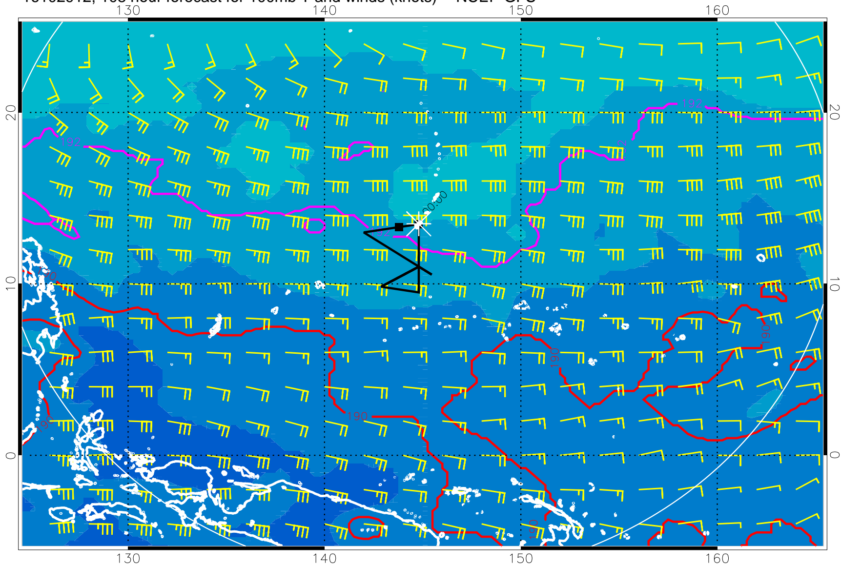
16102912, 108 hour forecast for 100mb T and winds (knots) -- NCEP GFS
