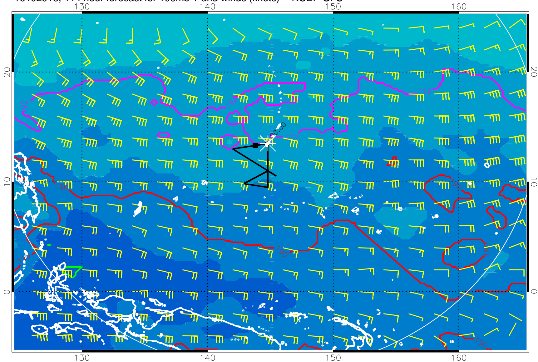
16102918, 114 hour forecast for 100mb T and winds (knots) -- NCEP GFS
