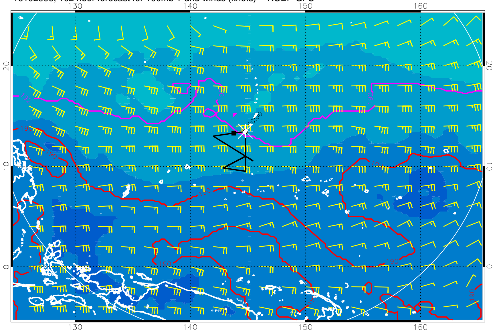
16102906, 102 hour forecast for 100mb T and winds (knots) -- NCEP GFS
