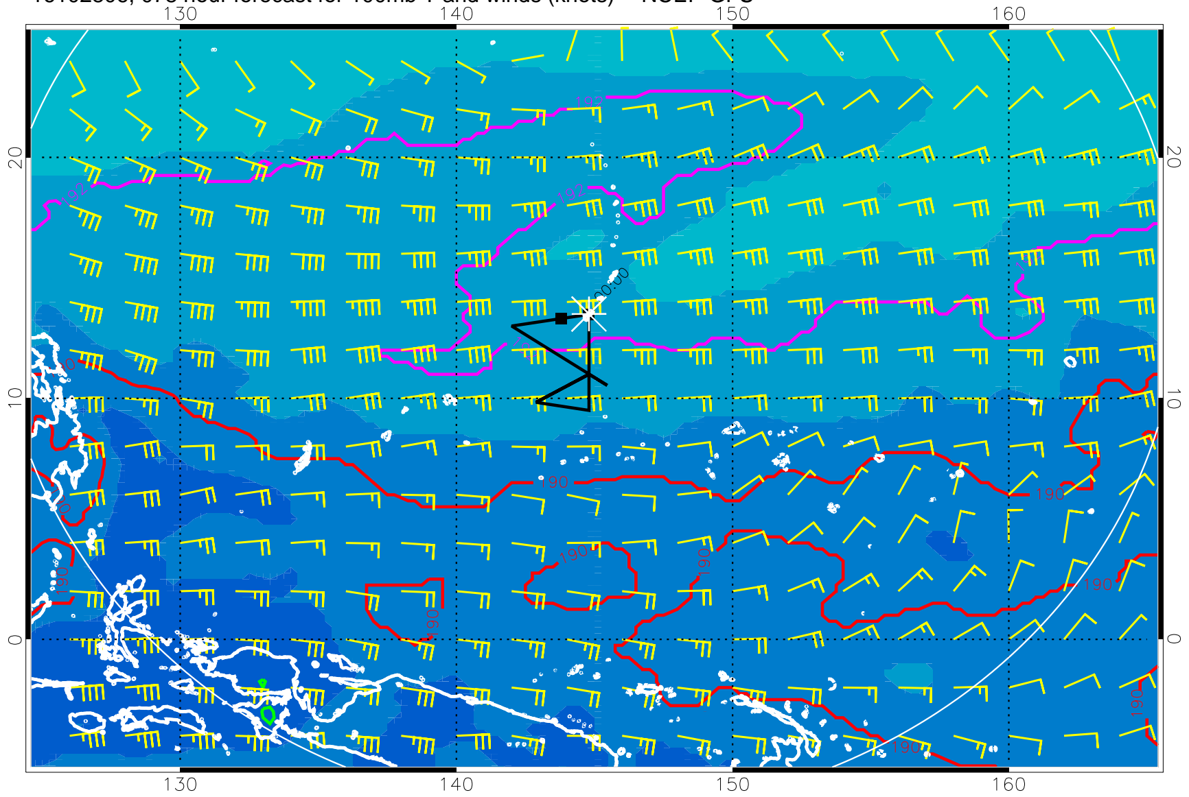
16102806, 078 hour forecast for 100mb T and winds (knots) -- NCEP GFS
