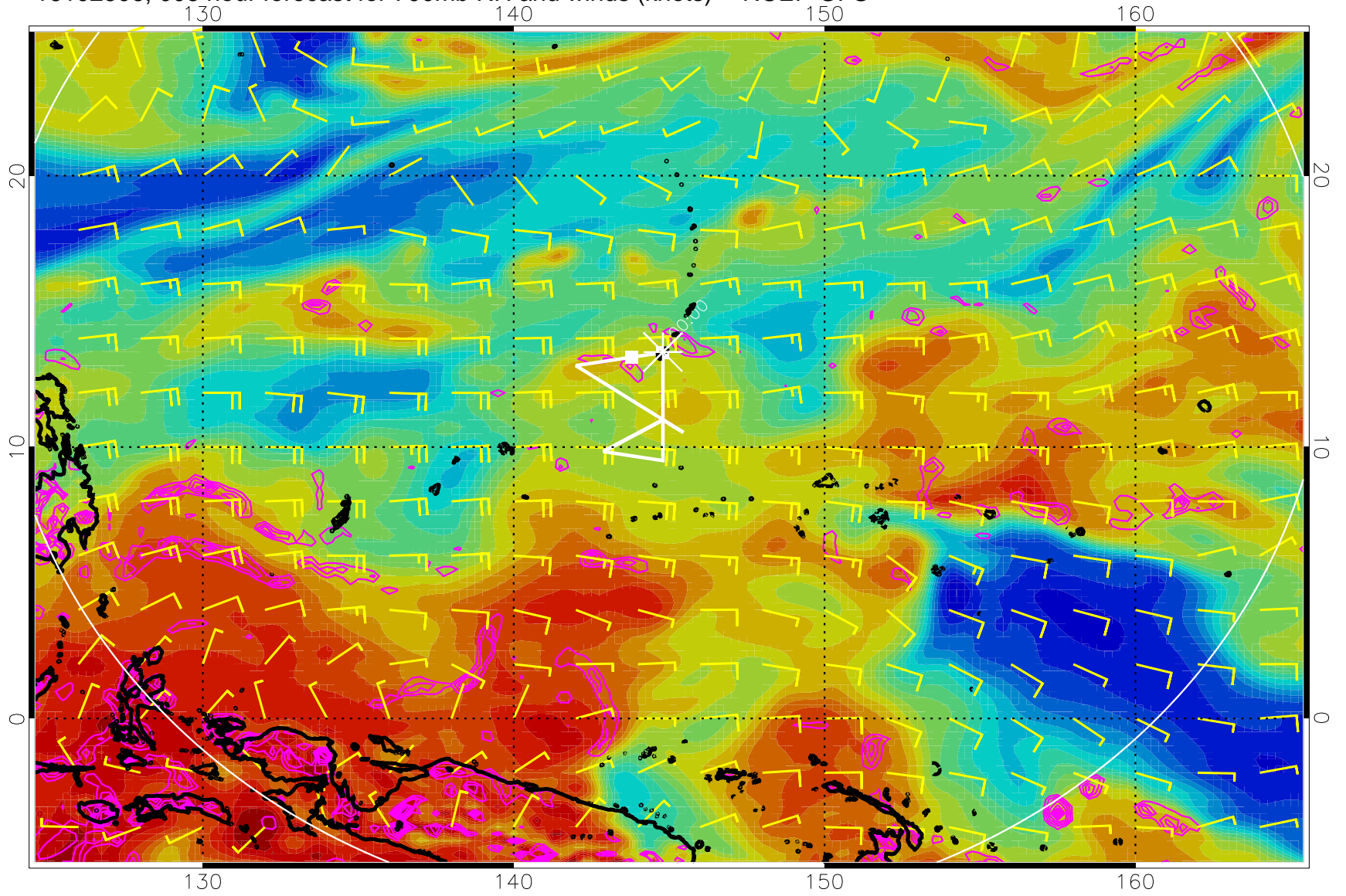
16102506, 006 hour forecast for 700mb RH and winds (knots) -- NCEP GFS
