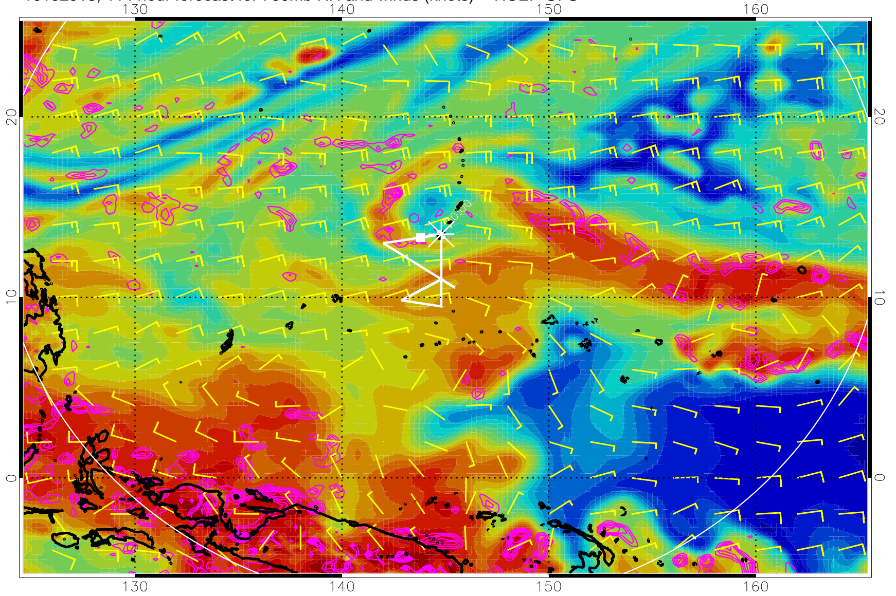
16102918, 114 hour forecast for 700mb RH and winds (knots) -- NCEP GFS
