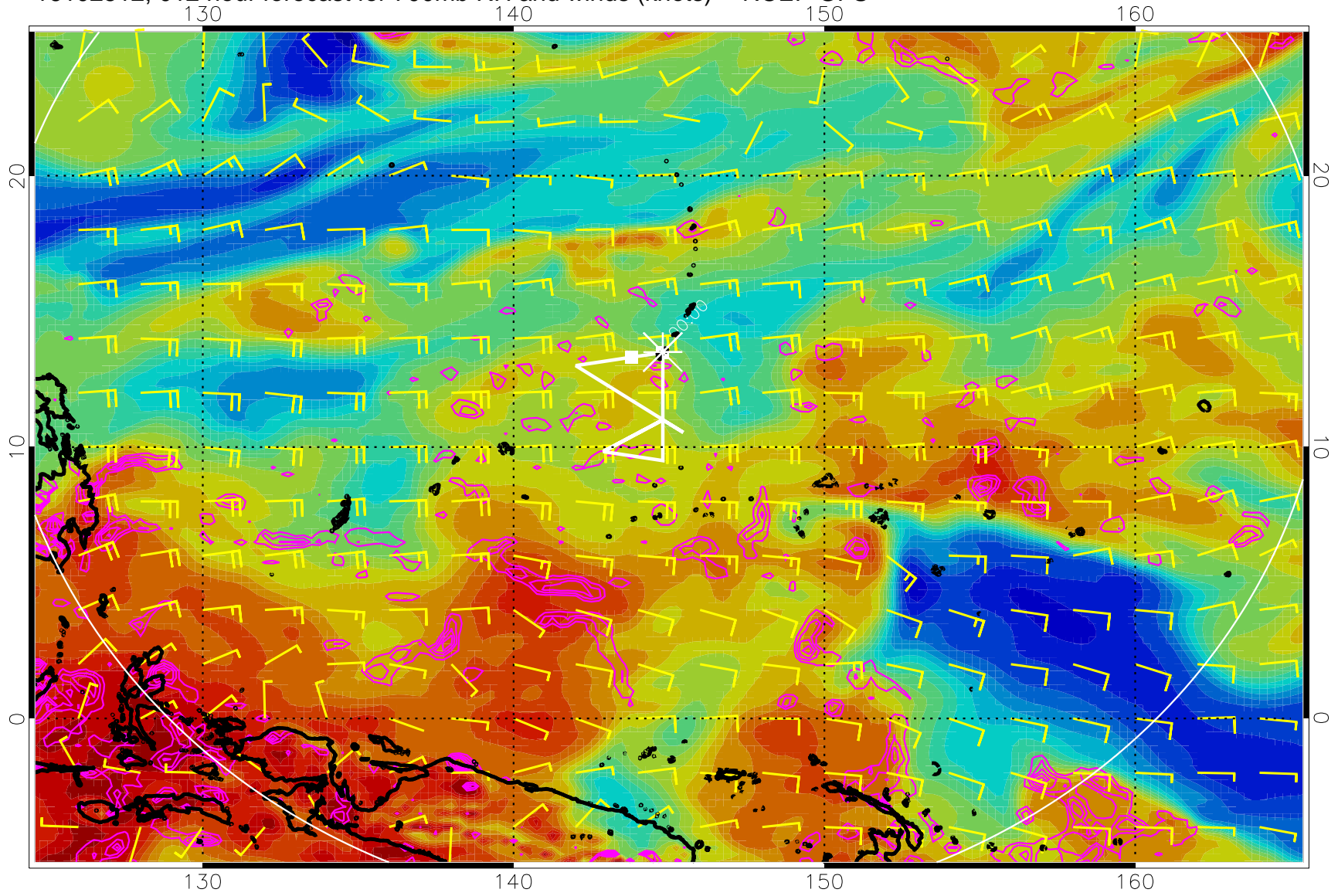
16102512, 012 hour forecast for 700mb RH and winds (knots) -- NCEP GFS
