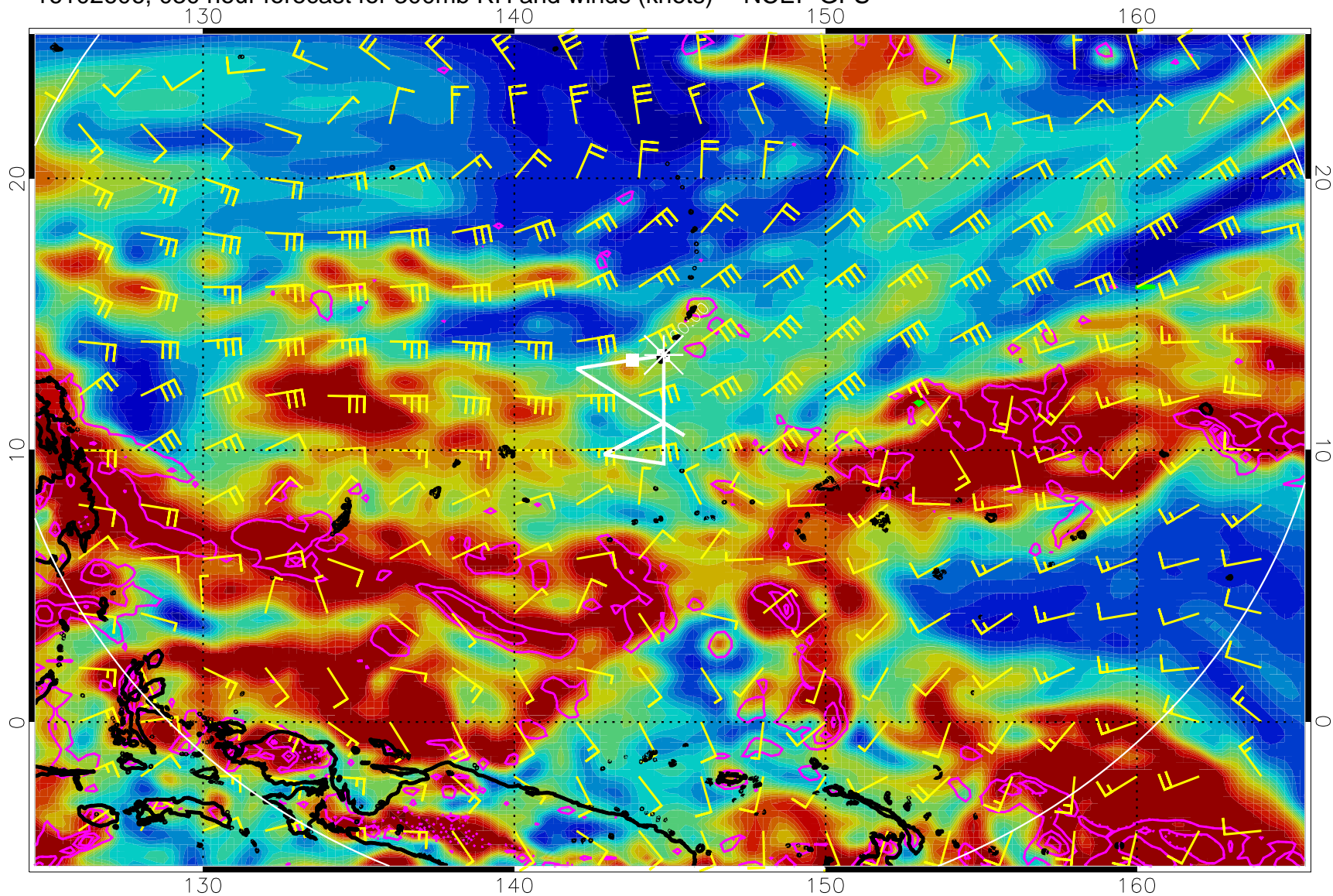
16102606, 030 hour forecast for 300mb RH and winds (knots) -- NCEP GFS
