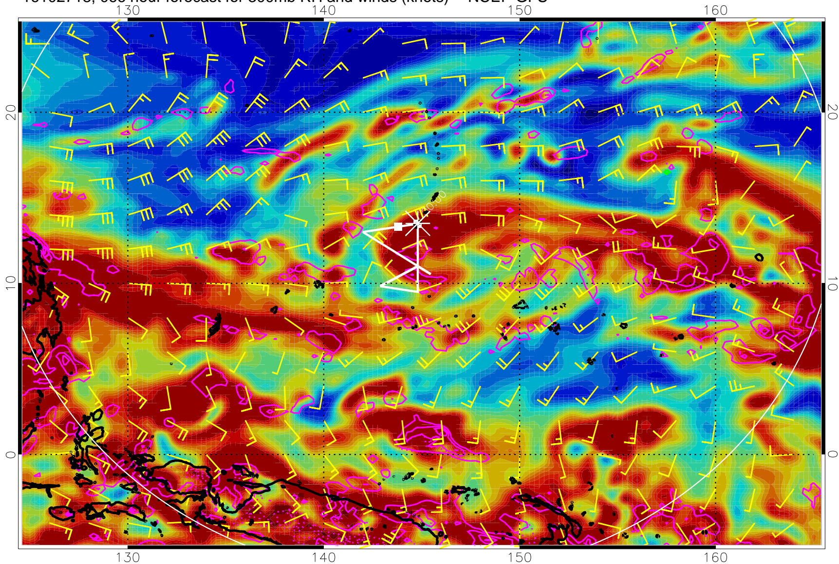
16102718, 066 hour forecast for 300mb RH and winds (knots) -- NCEP GFS
