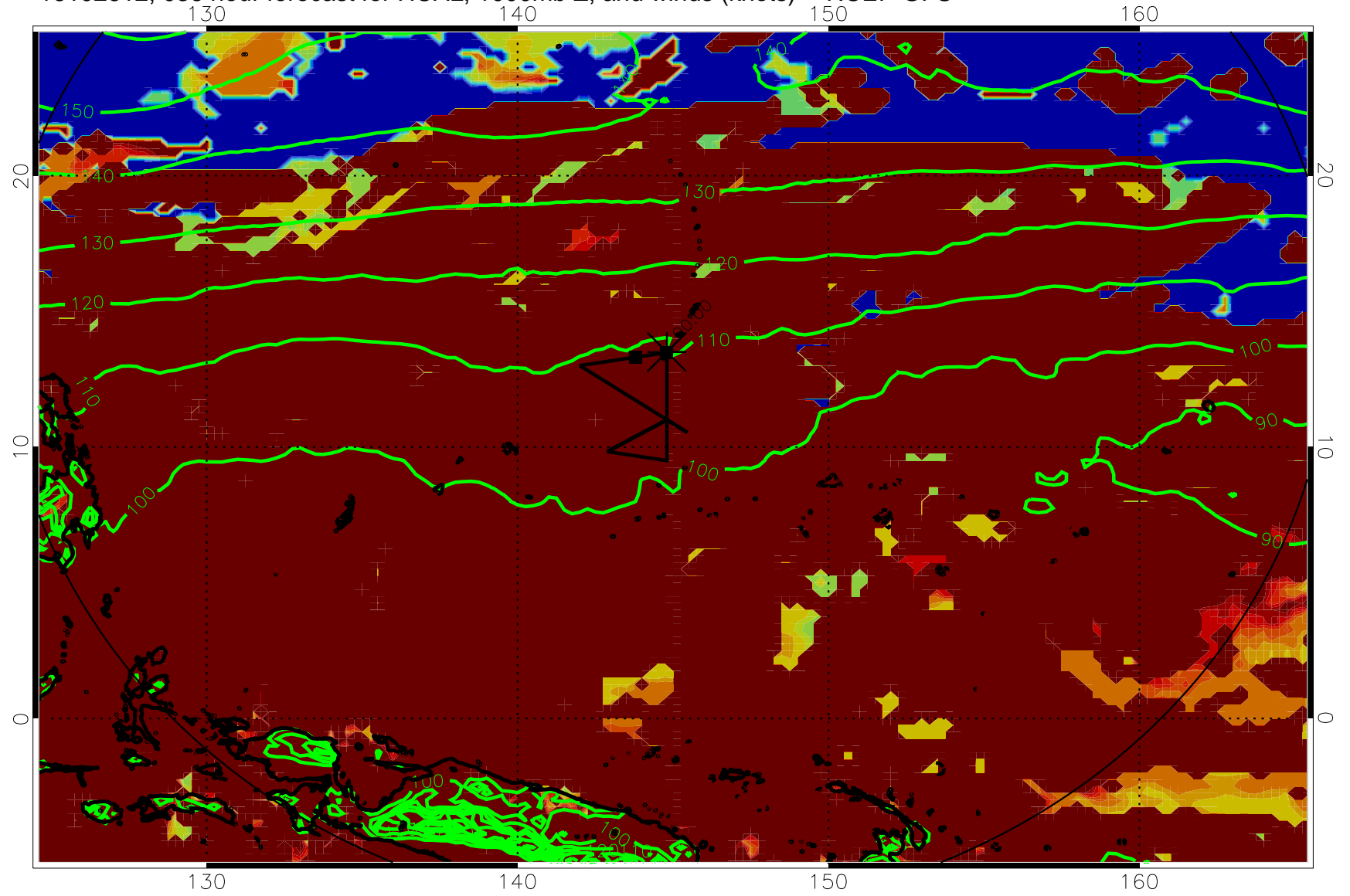
16102612, 036 hour forecast for HCAL, 1000mb Z, and winds (knots) -- NCEP GFS
