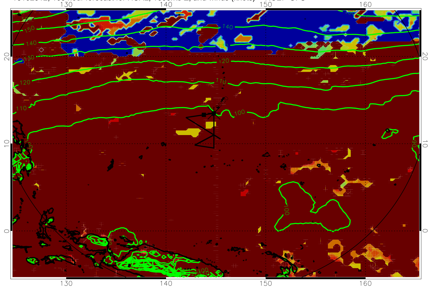
16102912, 108 hour forecast for HCAL, 1000mb Z, and winds (knots) -- NCEP GFS
