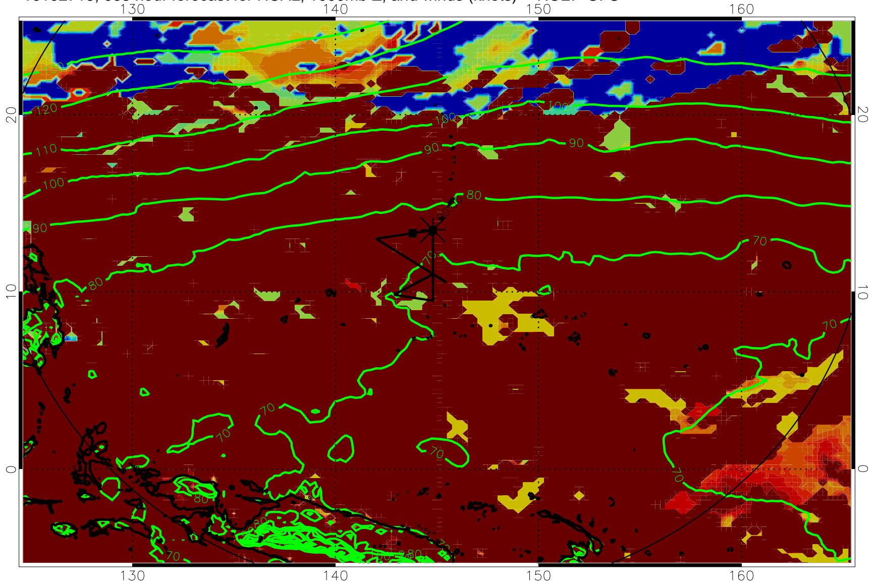
16102718, 066 hour forecast for HCAL, 1000mb Z, and winds (knots) -- NCEP GFS
