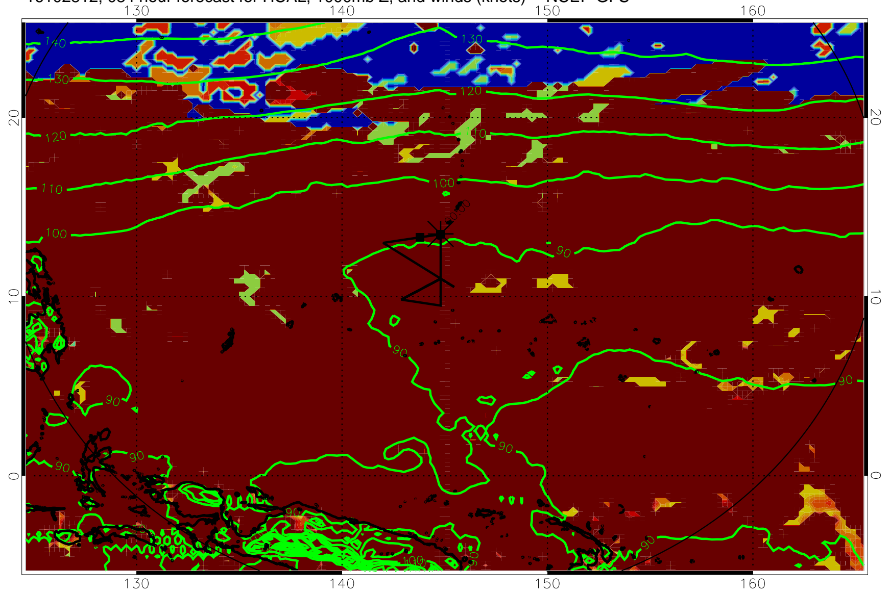
16102812, 084 hour forecast for HCAL, 1000mb Z, and winds (knots) -- NCEP GFS
