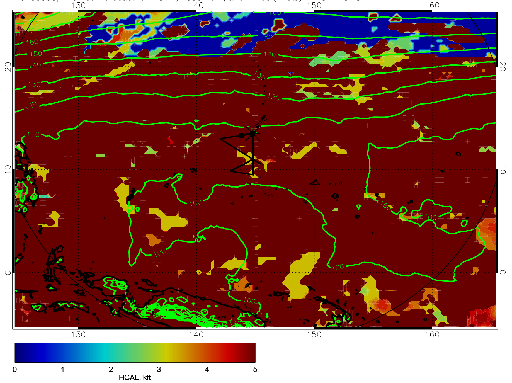
16103000, 120 hour forecast for HCAL, 1000mb Z, and winds (knots) -- NCEP GFS
