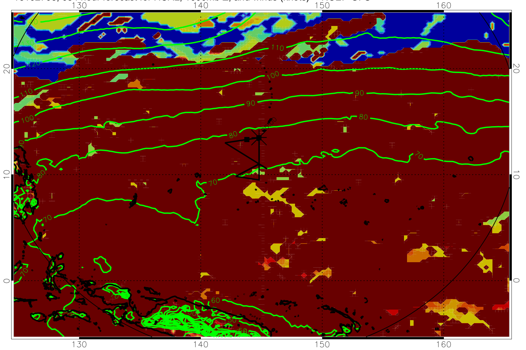
16102706, 054 hour forecast for HCAL, 1000mb Z, and winds (knots) -- NCEP GFS
