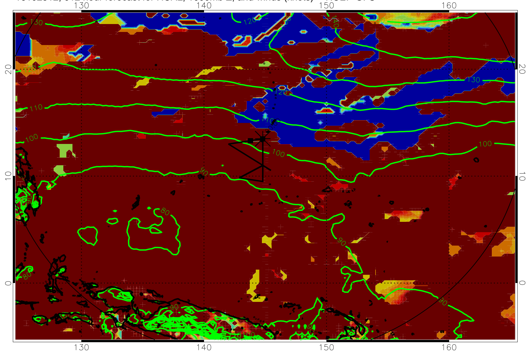
16102512, 012 hour forecast for HCAL, 1000mb Z, and winds (knots) -- NCEP GFS
