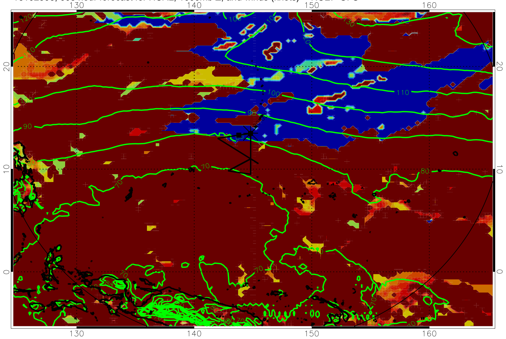
16102506, 006 hour forecast for HCAL, 1000mb Z, and winds (knots) -- NCEP GFS
