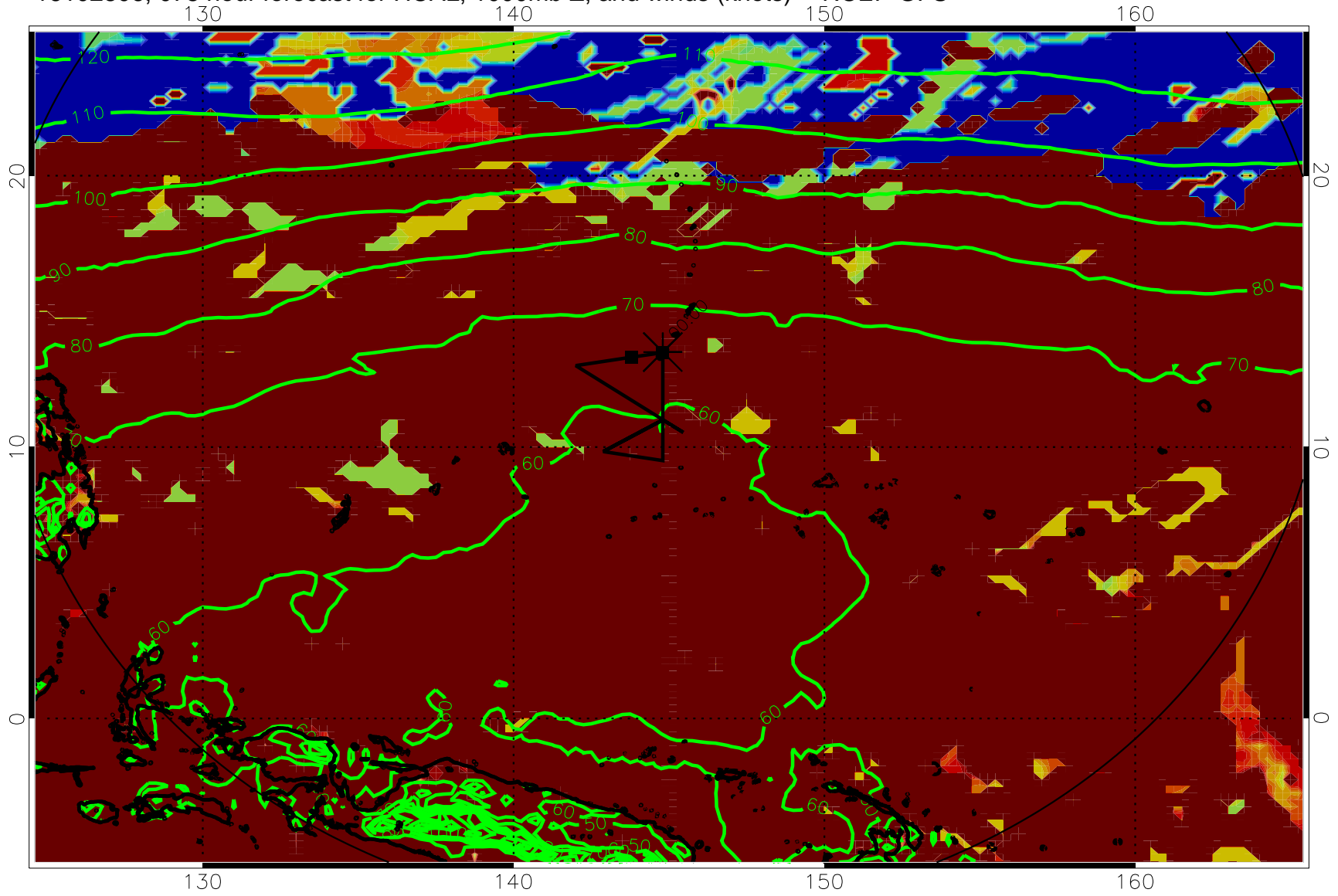
16102806, 078 hour forecast for HCAL, 1000mb Z, and winds (knots) -- NCEP GFS
