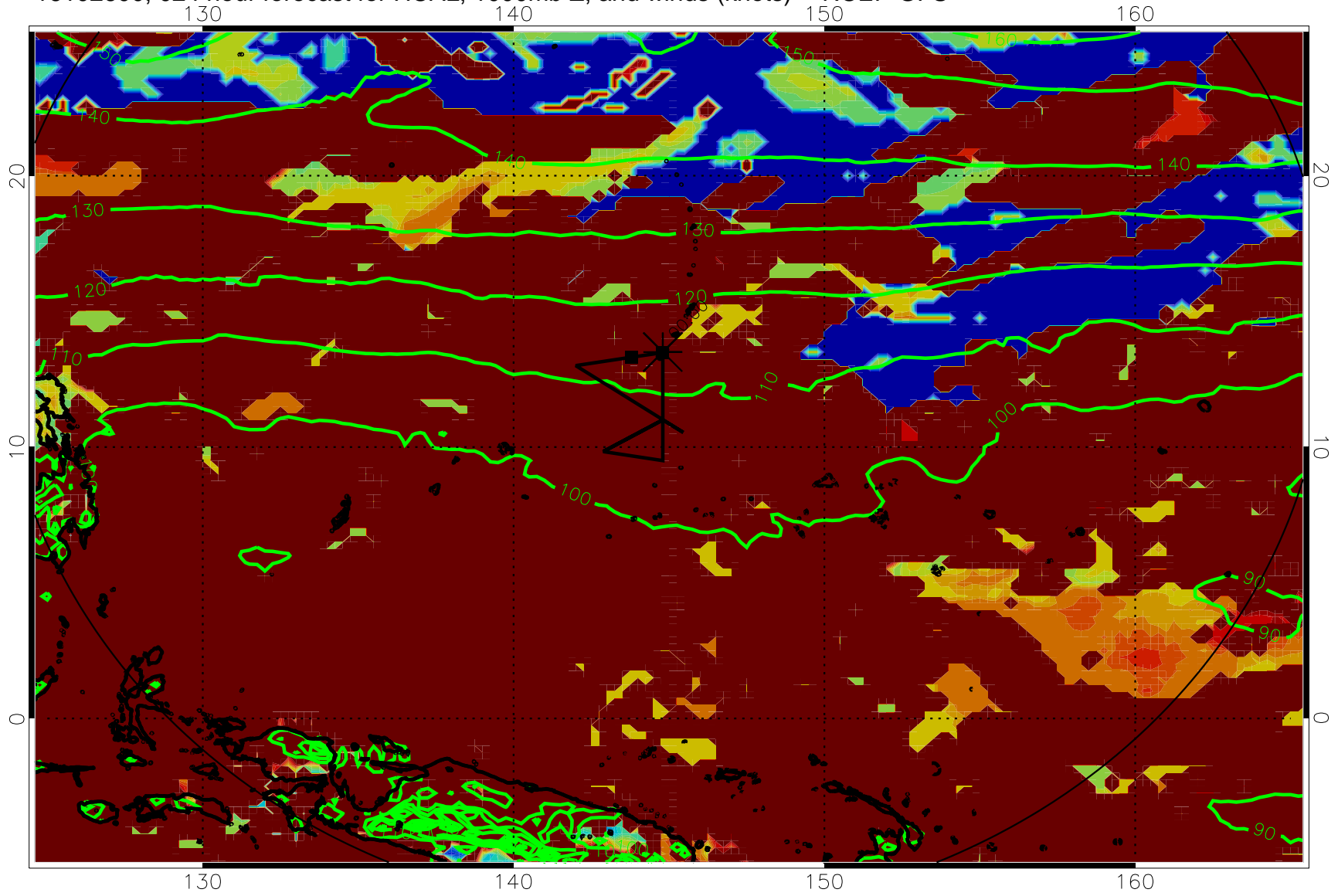
16102600, 024 hour forecast for HCAL, 1000mb Z, and winds (knots) -- NCEP GFS
