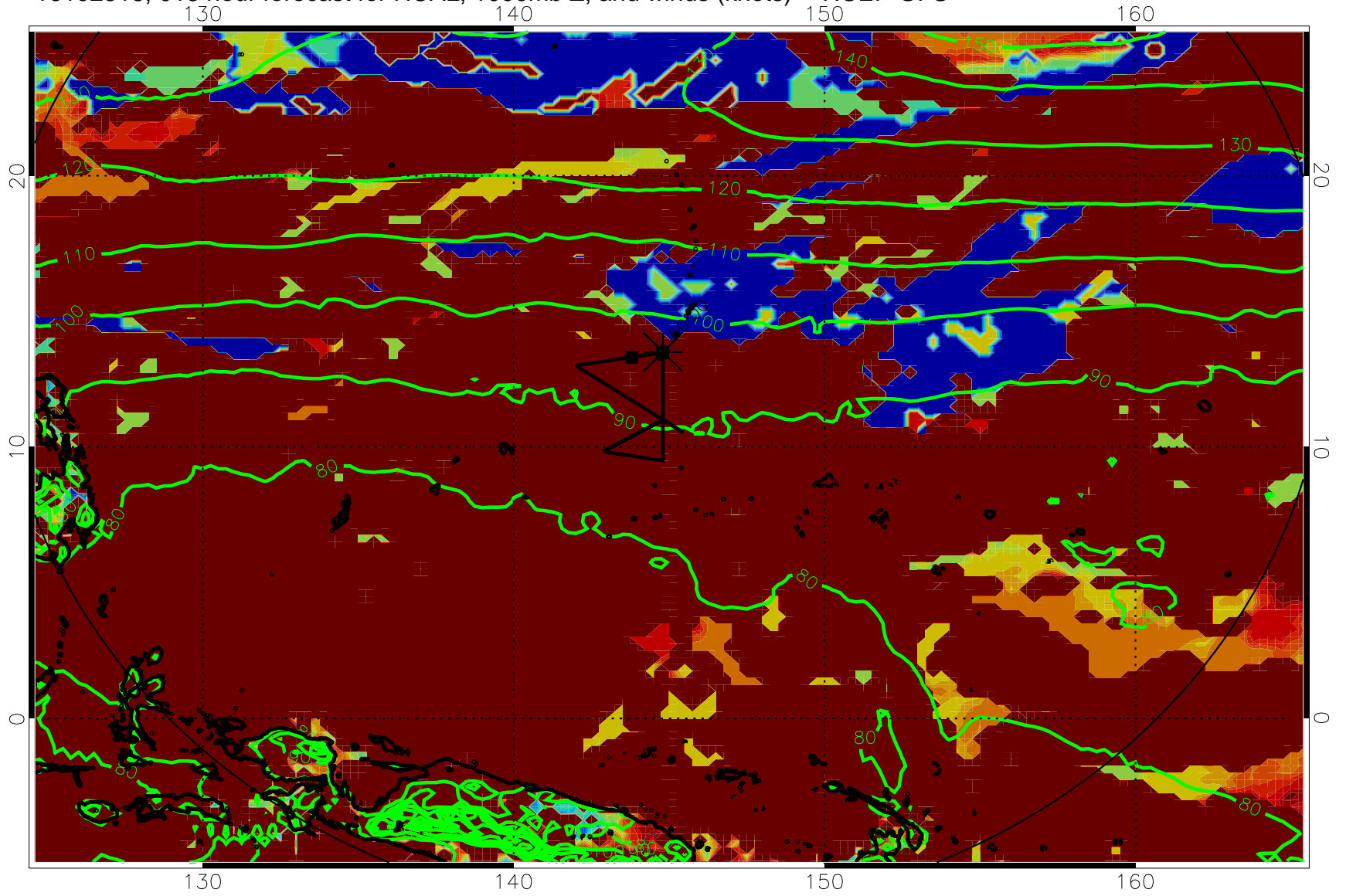
16102518, 018 hour forecast for HCAL, 1000mb Z, and winds (knots) -- NCEP GFS
