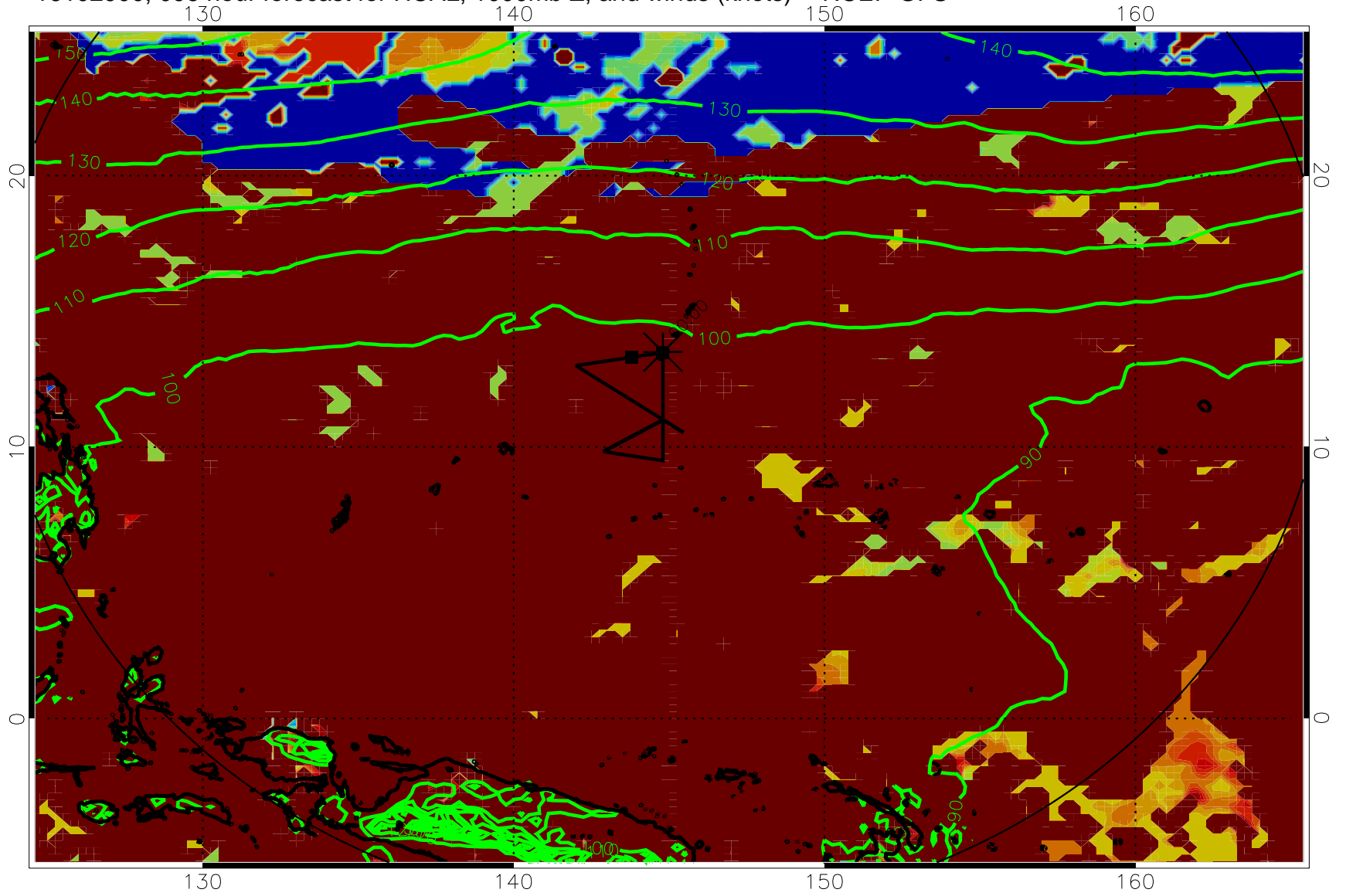
16102900, 096 hour forecast for HCAL, 1000mb Z, and winds (knots) -- NCEP GFS
