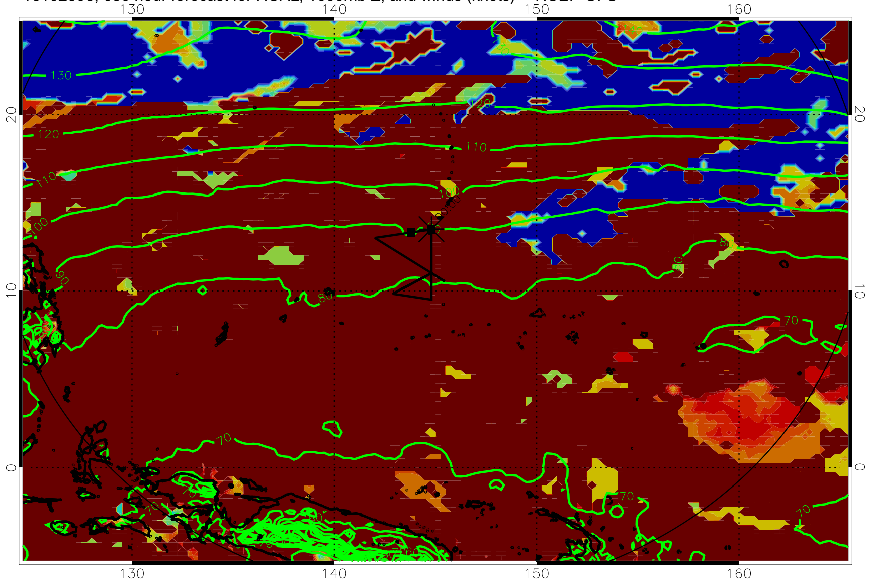
16102606, 030 hour forecast for HCAL, 1000mb Z, and winds (knots) -- NCEP GFS
