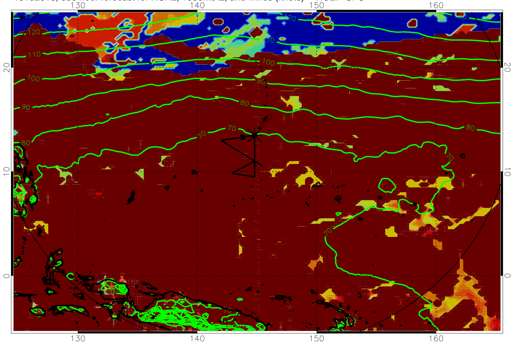
16102818, 090 hour forecast for HCAL, 1000mb Z, and winds (knots) -- NCEP GFS
