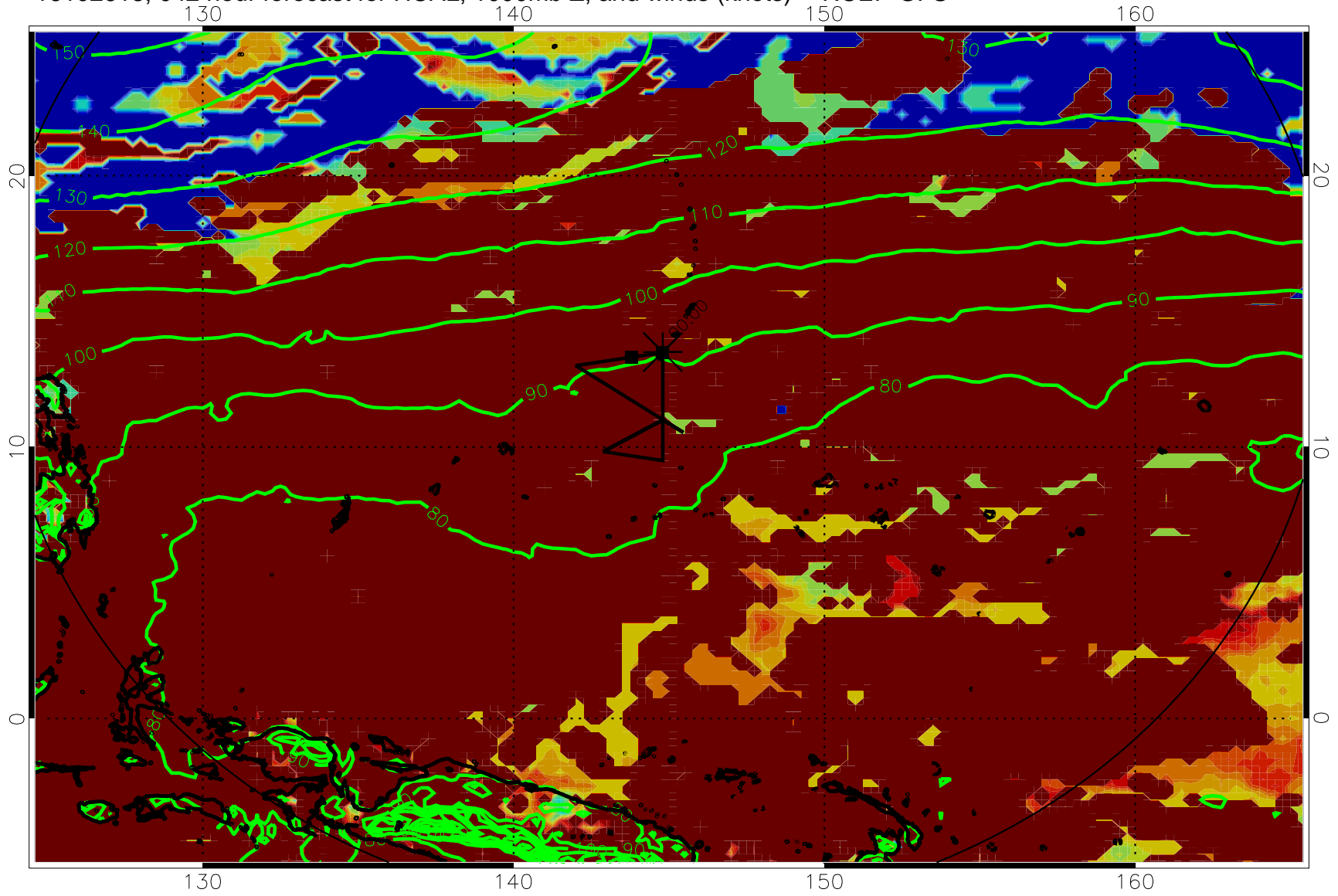
16102618, 042 hour forecast for HCAL, 1000mb Z, and winds (knots) -- NCEP GFS
