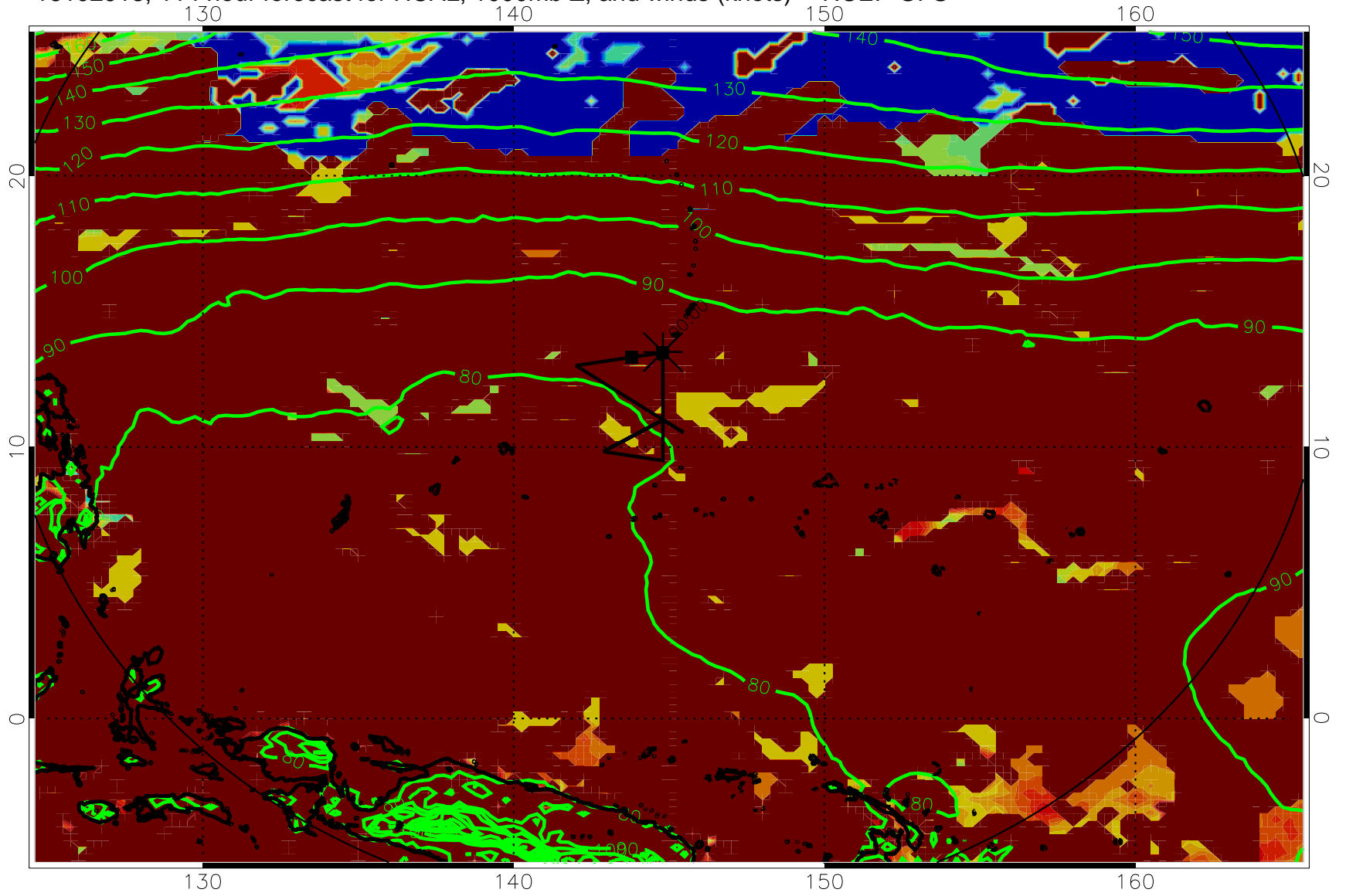
16102918, 114 hour forecast for HCAL, 1000mb Z, and winds (knots) -- NCEP GFS
