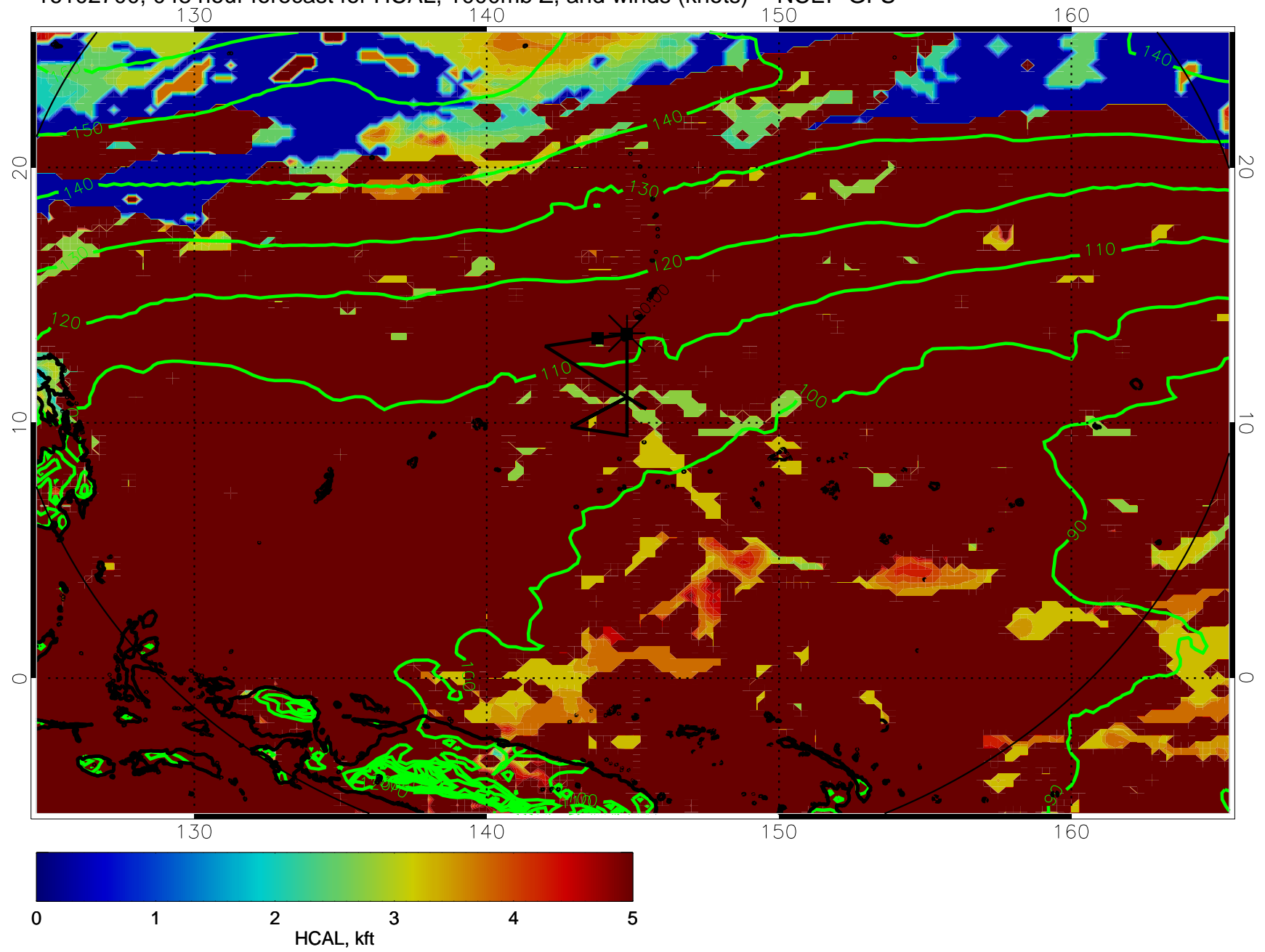
16102700, 048 hour forecast for HCAL, 1000mb Z, and winds (knots) -- NCEP GFS
