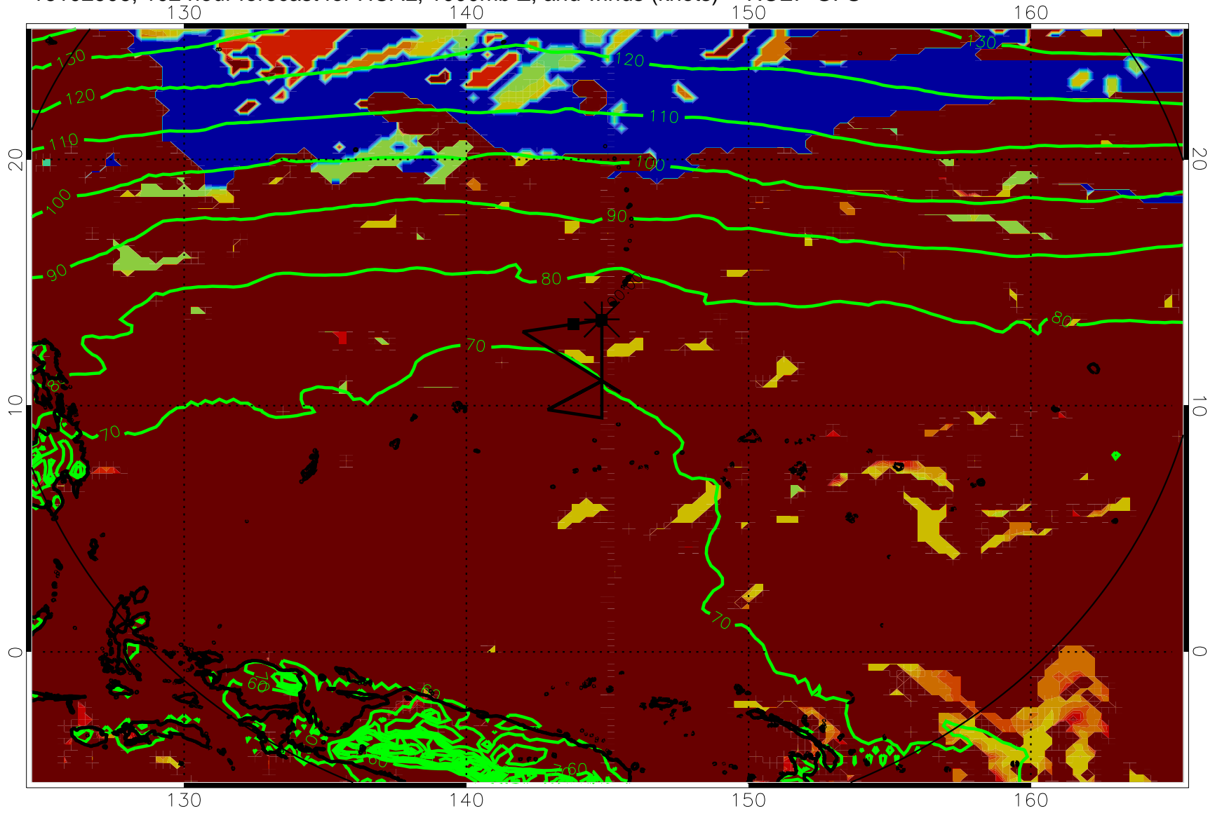
16102906, 102 hour forecast for HCAL, 1000mb Z, and winds (knots) -- NCEP GFS
