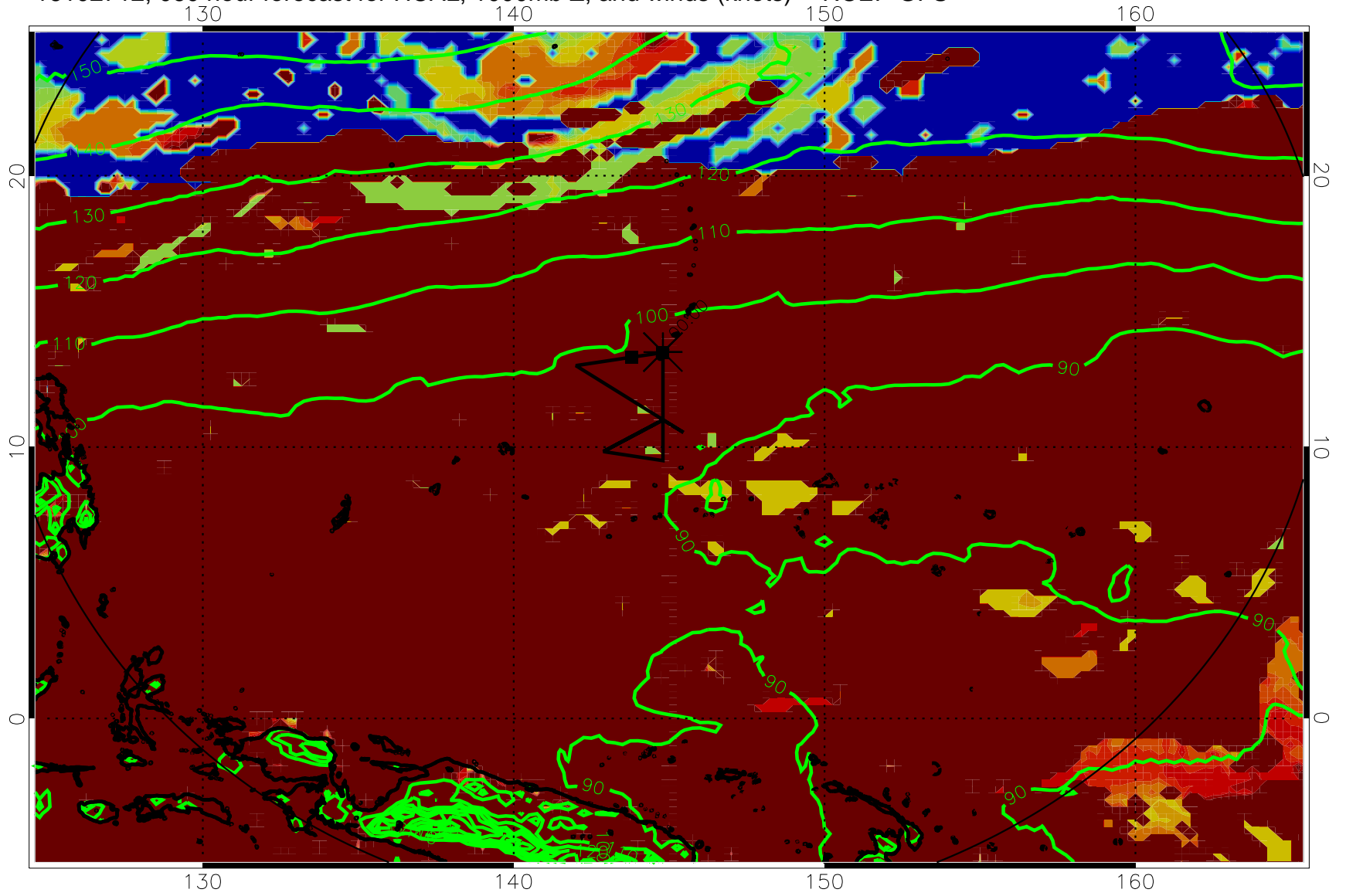
16102712, 060 hour forecast for HCAL, 1000mb Z, and winds (knots) -- NCEP GFS
