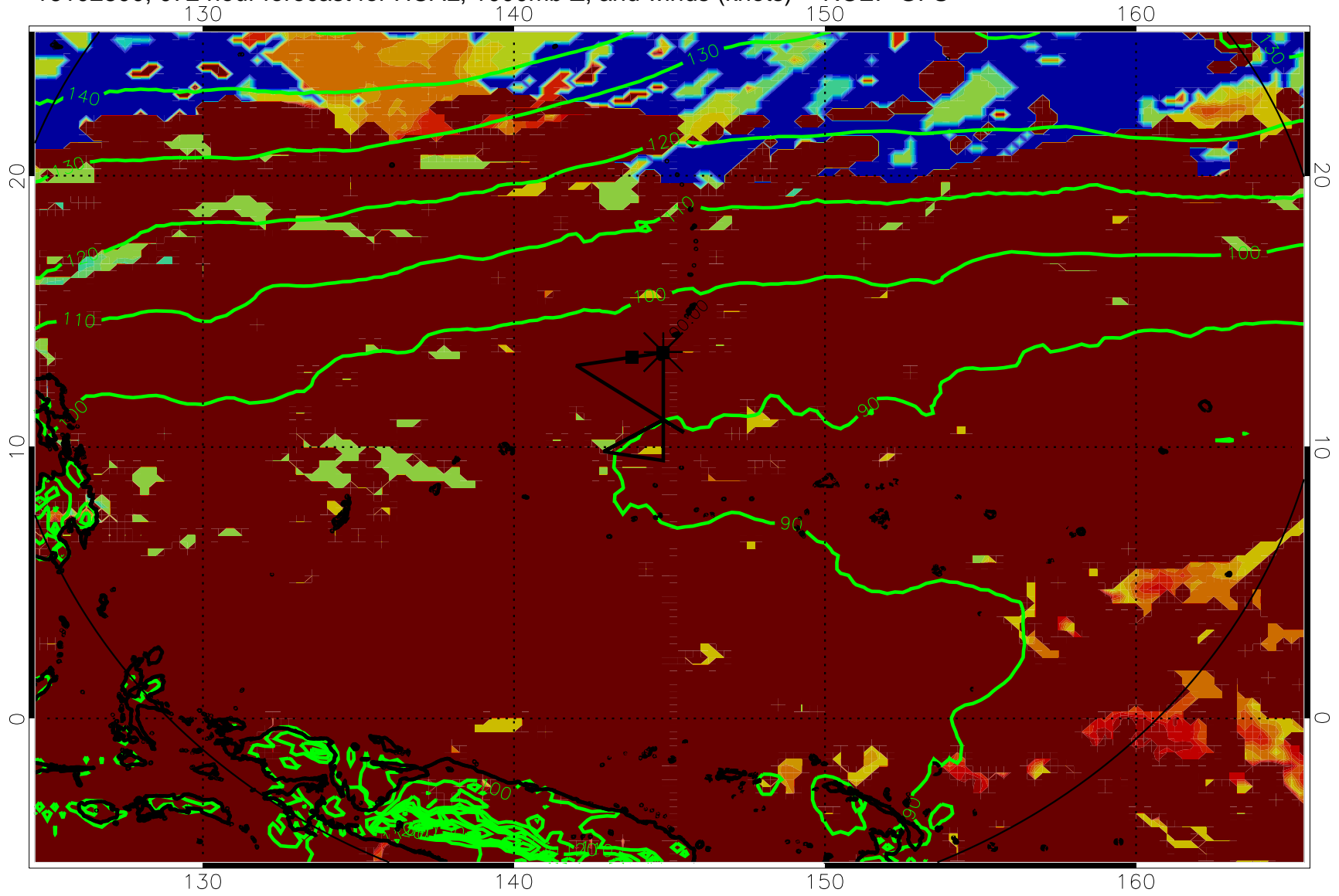
16102800, 072 hour forecast for HCAL, 1000mb Z, and winds (knots) -- NCEP GFS
