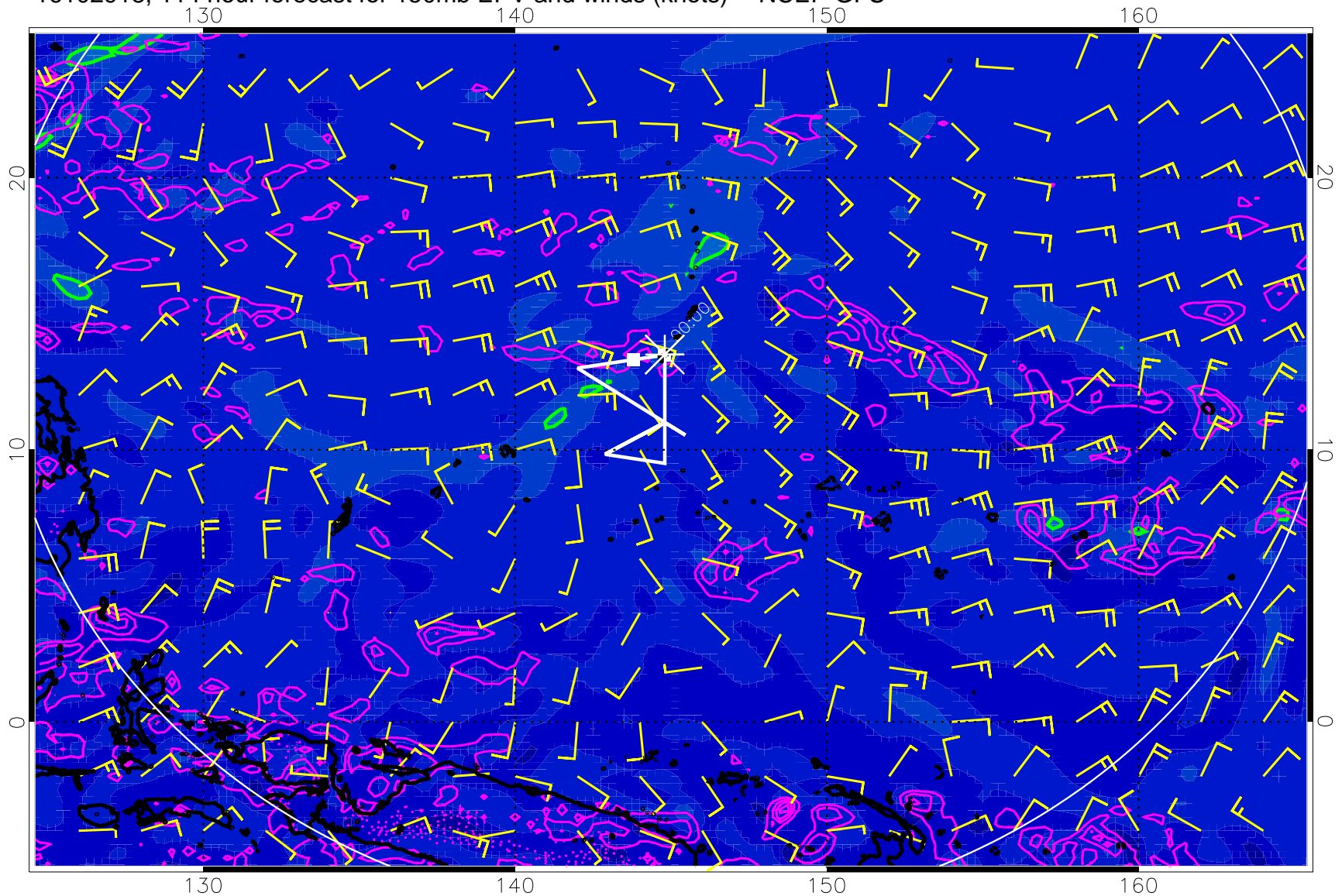
16102918, 114 hour forecast for 150mb EPV and winds (knots) -- NCEP GFS
