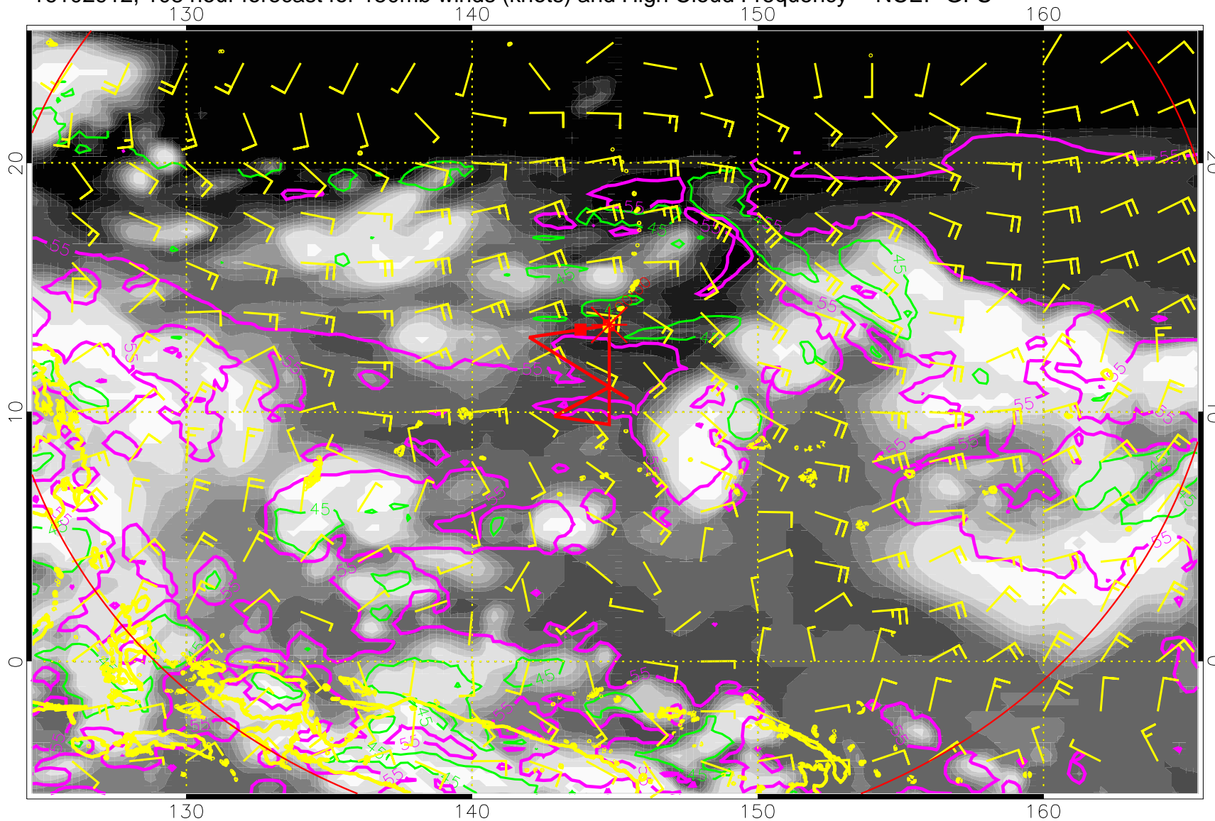
16102912, 108 hour forecast for 150mb winds (knots) and High Cloud Frequency -- NCEP GFS
