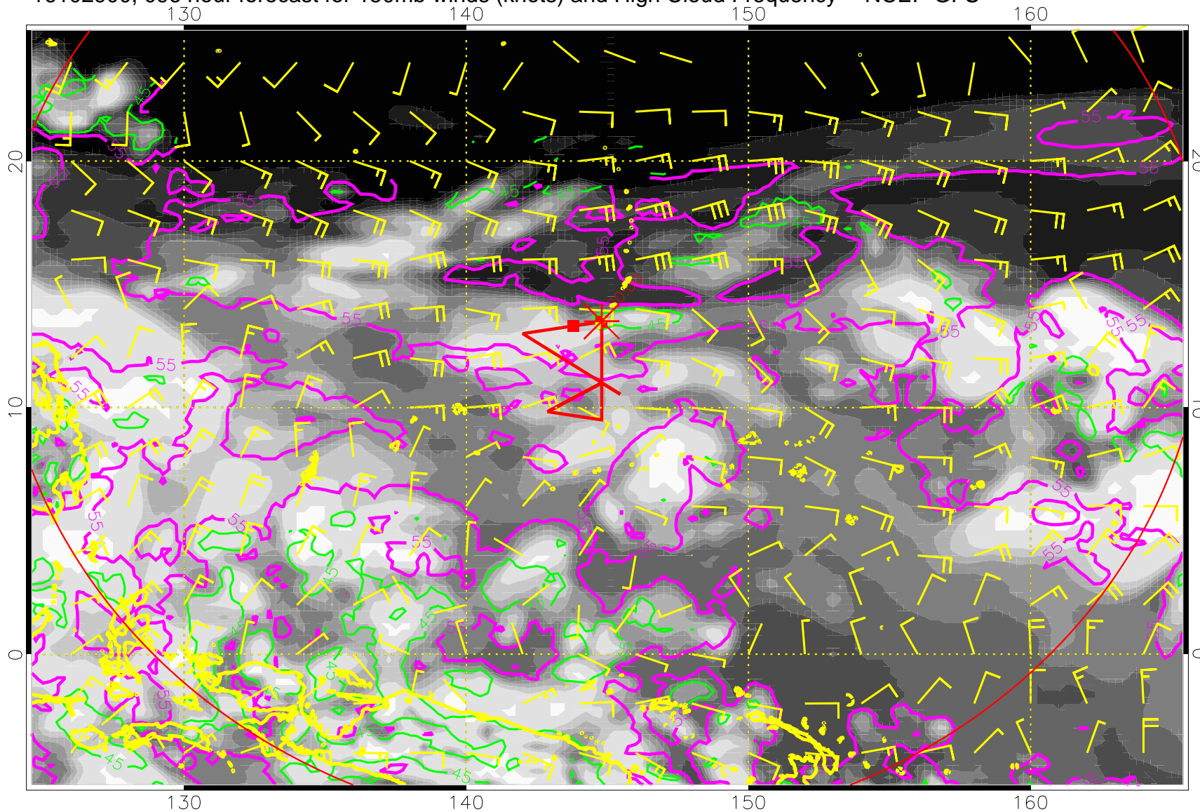
16102900, 096 hour forecast for 150mb winds (knots) and High Cloud Frequency -- NCEP GFS
