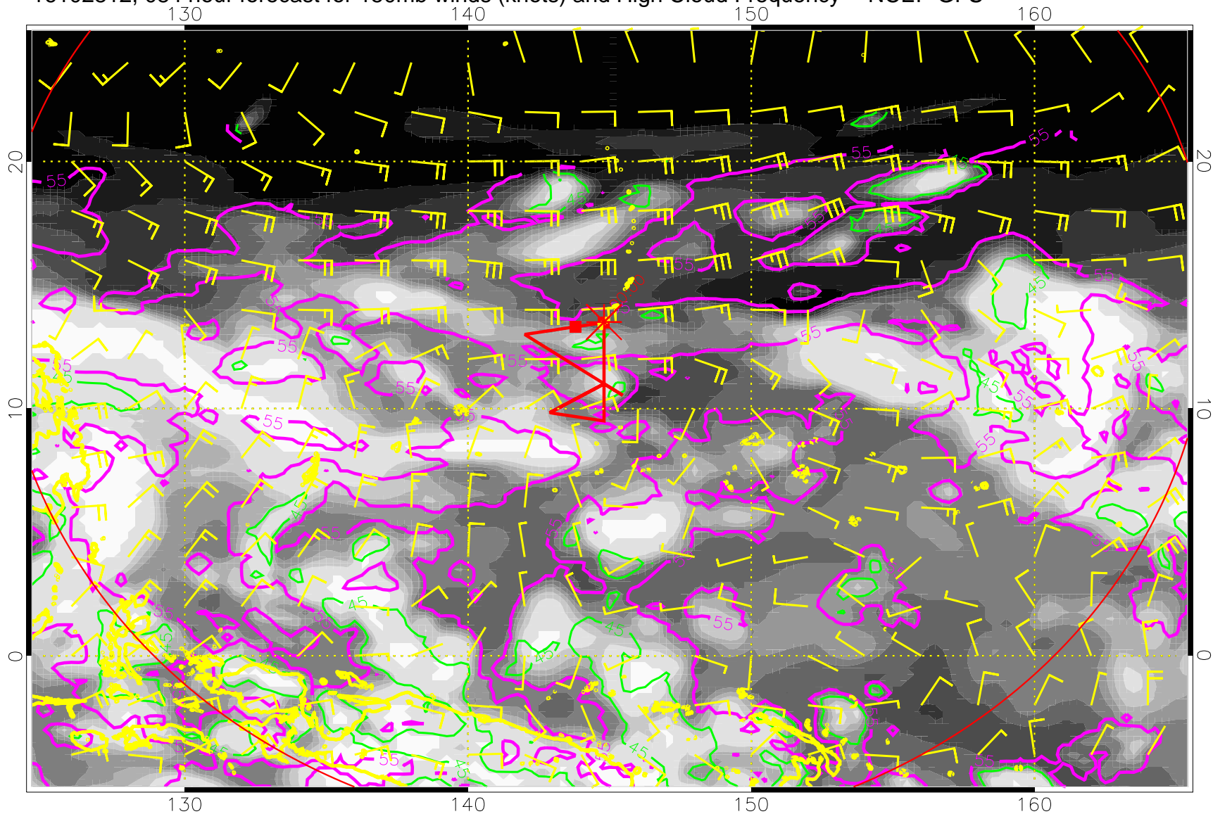
16102812, 084 hour forecast for 150mb winds (knots) and High Cloud Frequency -- NCEP GFS
