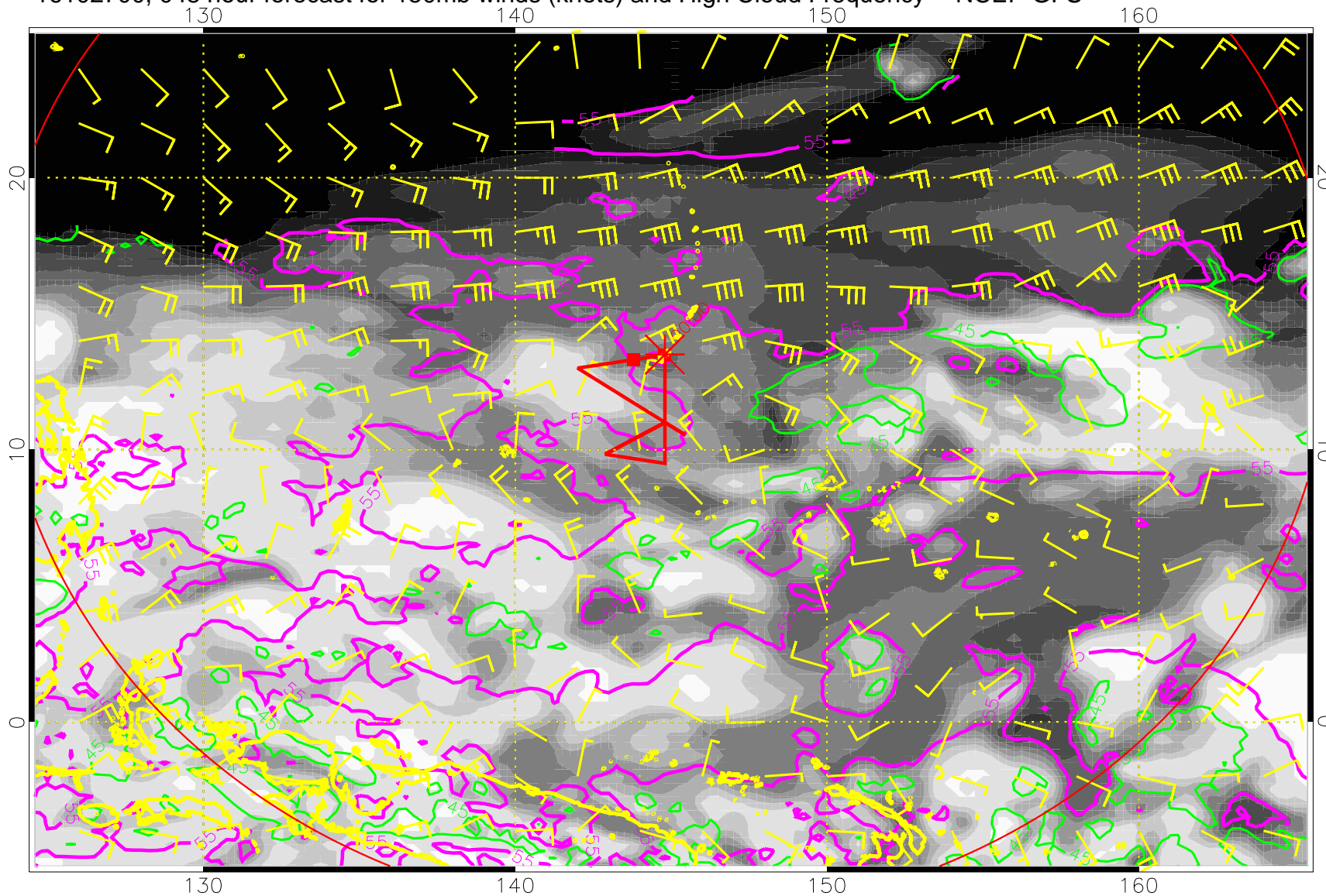
16102700, 048 hour forecast for 150mb winds (knots) and High Cloud Frequency -- NCEP GFS
