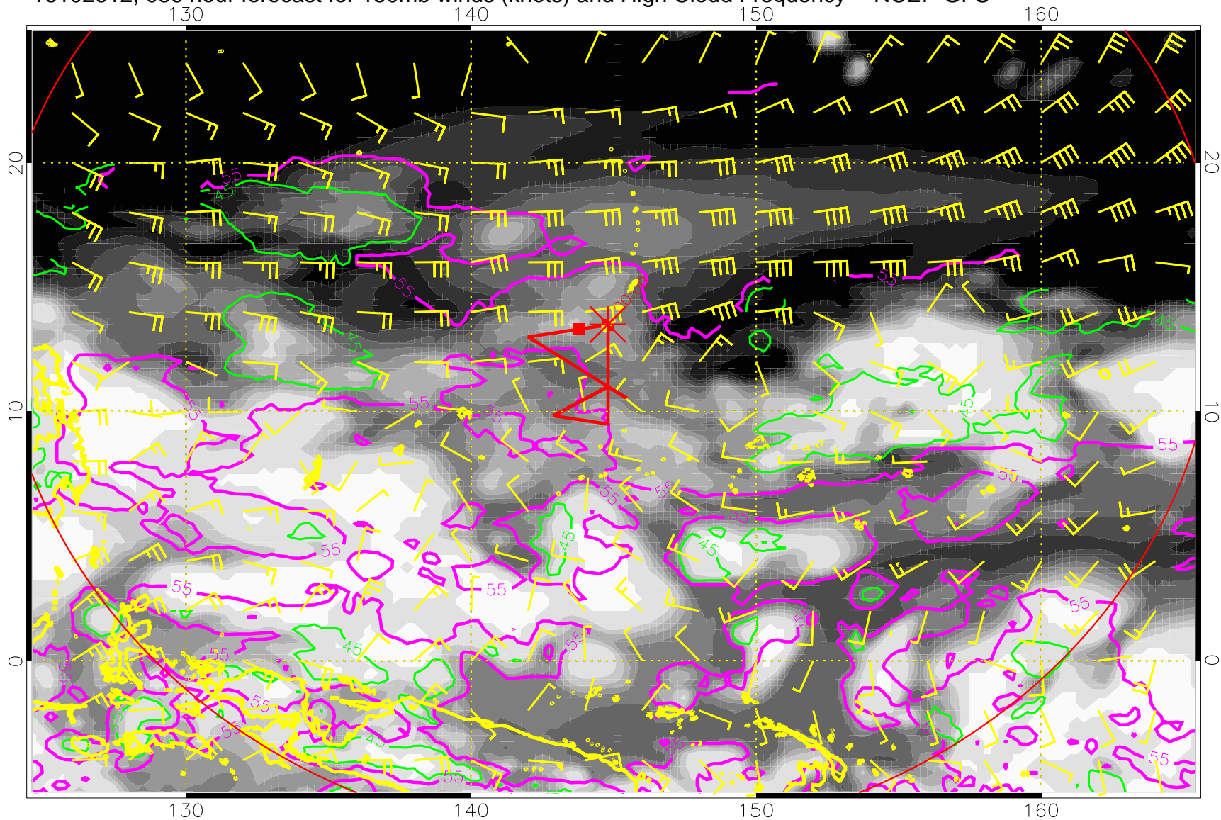
16102612, 036 hour forecast for 150mb winds (knots) and High Cloud Frequency -- NCEP GFS
