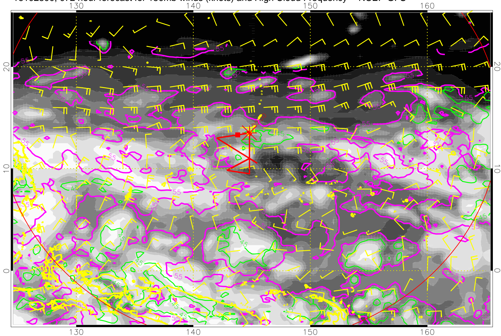
16102800, 07Z hour forecast for 150mb winds (knots) and High Cloud Frequency -- NCEP GFS
