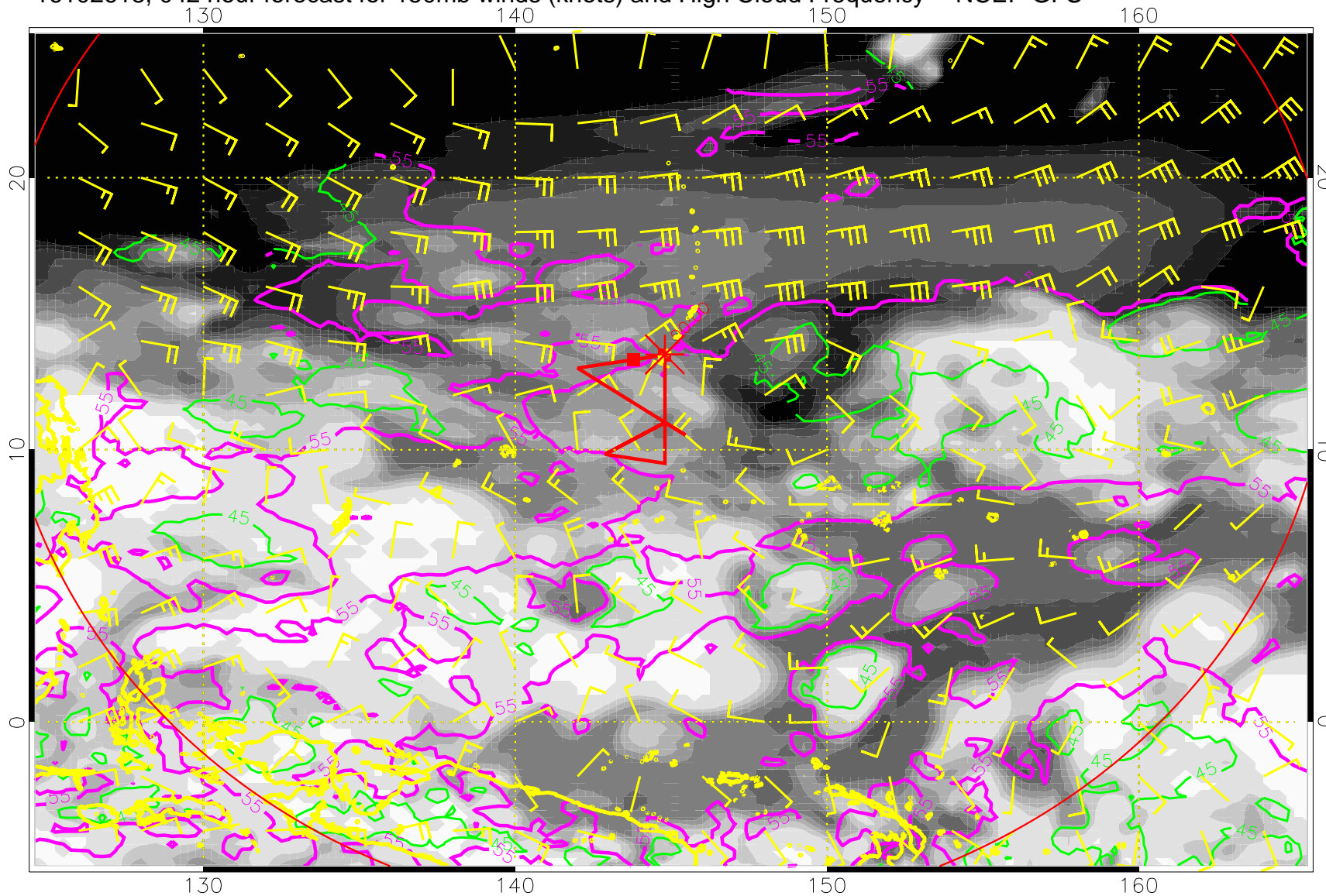
16102618, 042 hour forecast for 150mb winds (knots) and High Cloud Frequency -- NCEP GFS
