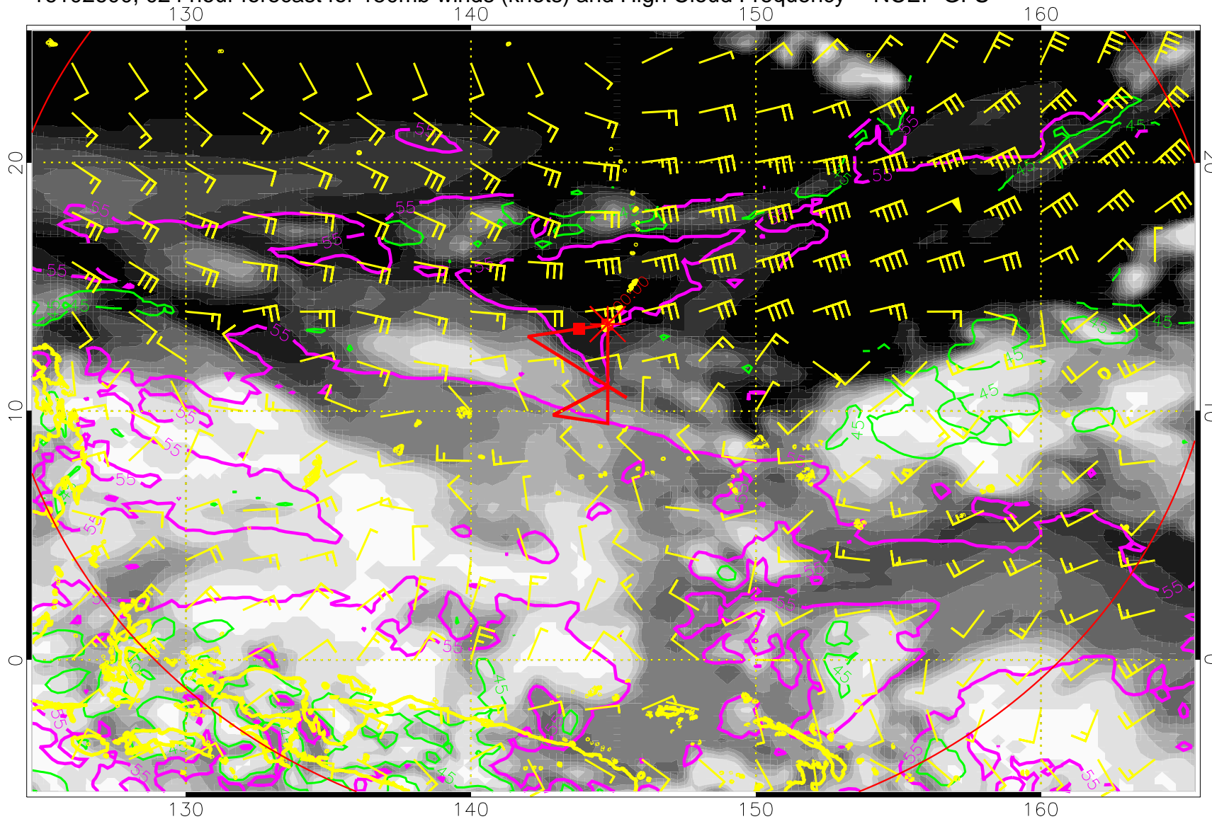
16102600, 024 hour forecast for 150mb winds (knots) and High Cloud Frequency -- NCEP GFS
