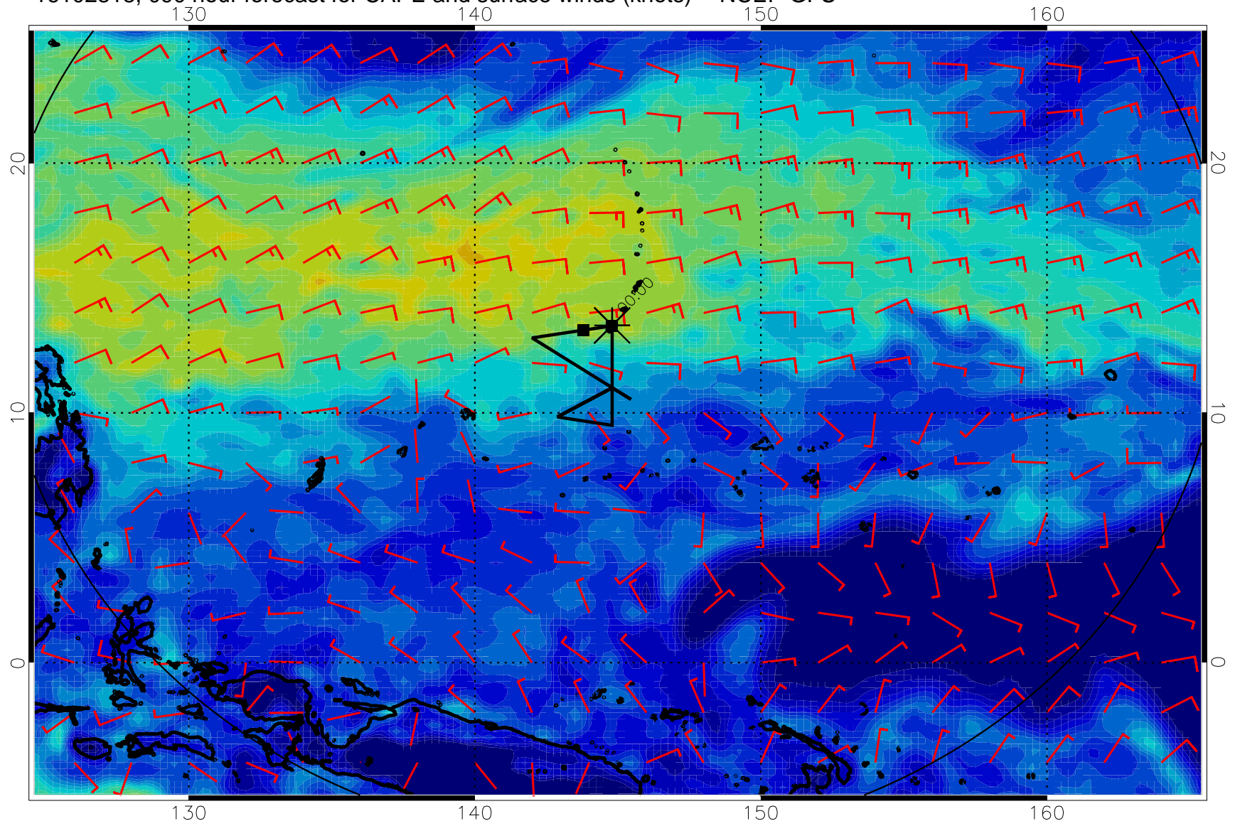
16102818, 090 hour forecast for CAPE and surface winds (knots) -- NCEP GFS
