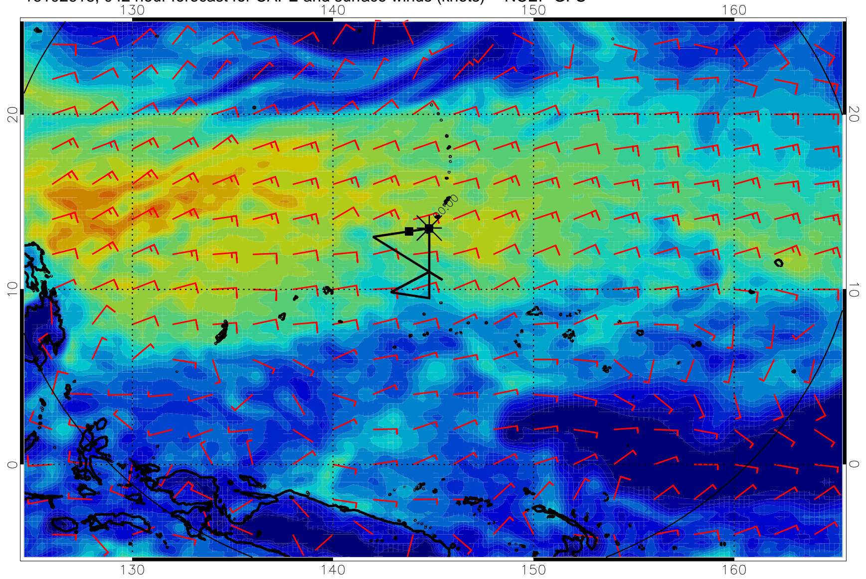
16102618, 042 hour forecast for CAPE and surface winds (knots) -- NCEP GFS
