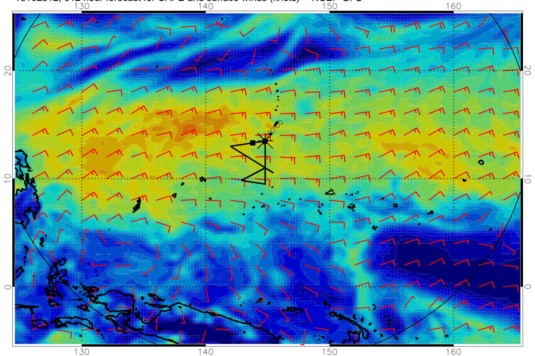
16102512, 012 hour forecast for CAPE and surface winds (knots) -- NCEP GFS
