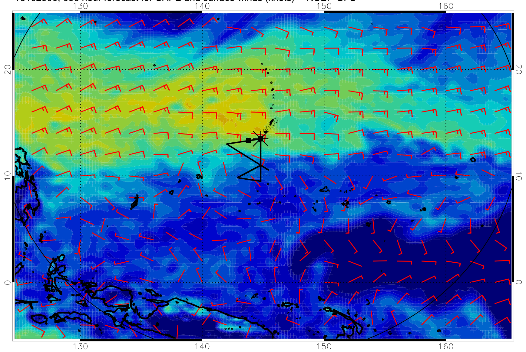
16102900, 096 hour forecast for CAPE and surface winds (knots) -- NCEP GFS
