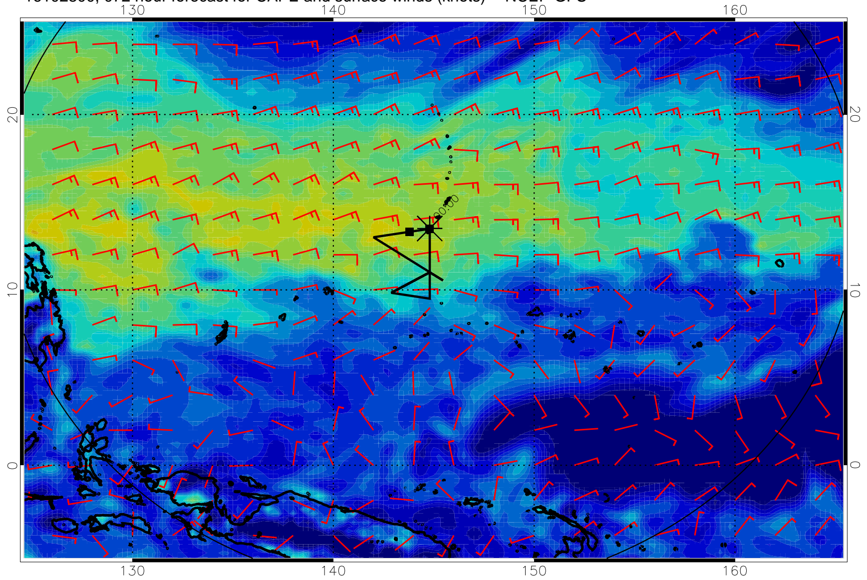
16102800, 072 hour forecast for CAPE and surface winds (knots) -- NCEP GFS
