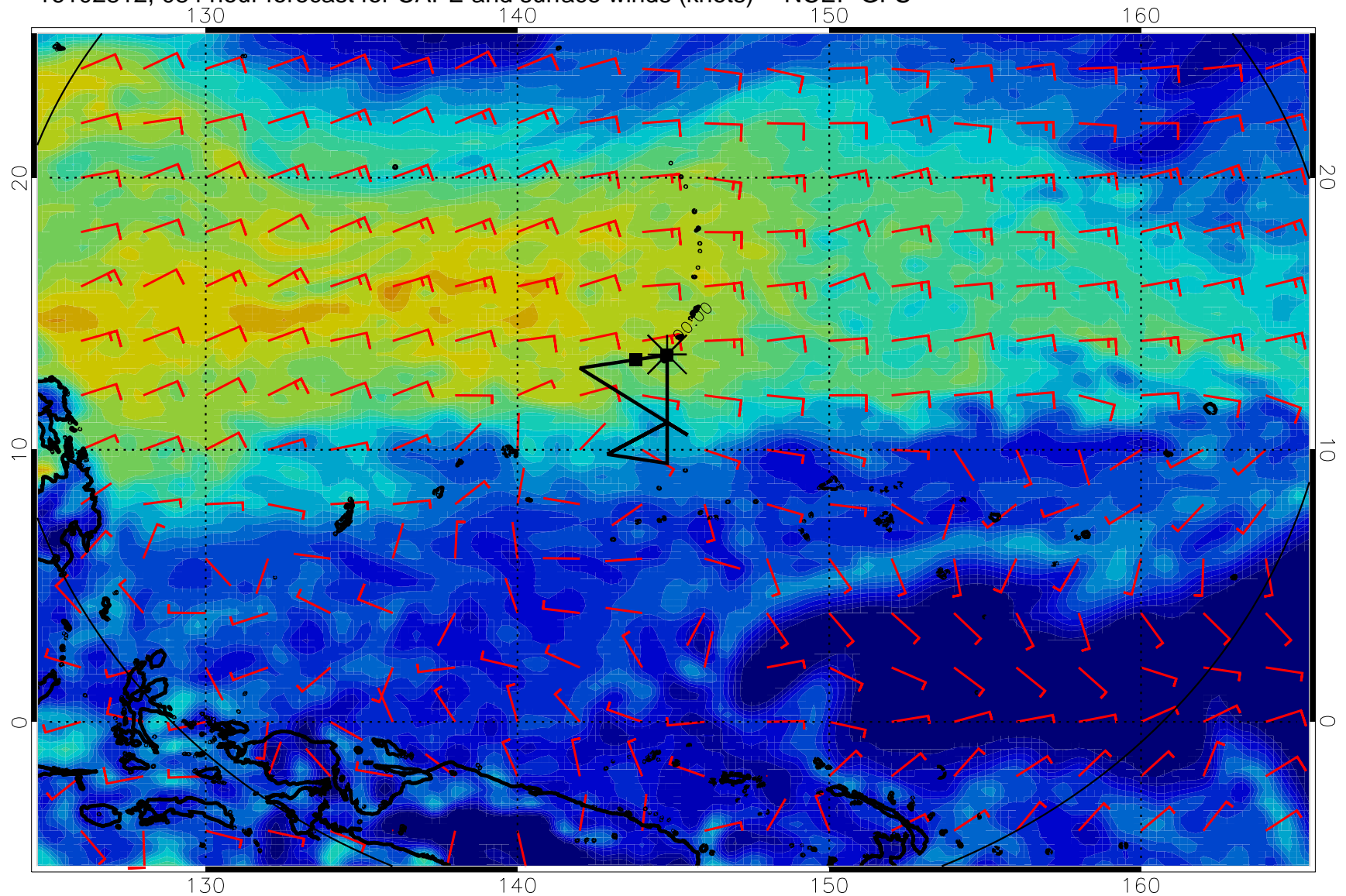
16102812, 084 hour forecast for CAPE and surface winds (knots) -- NCEP GFS
