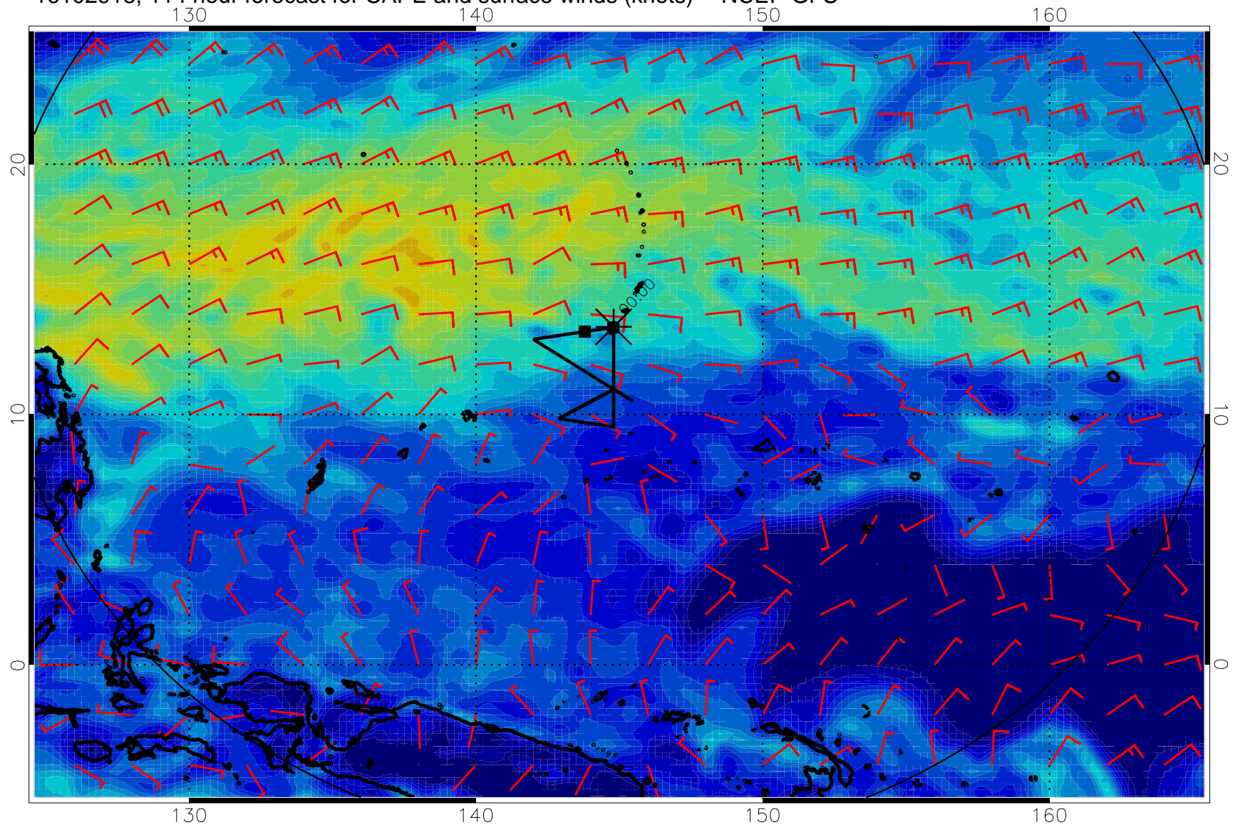
16102918, 114 hour forecast for CAPE and surface winds (knots) -- NCEP GFS
