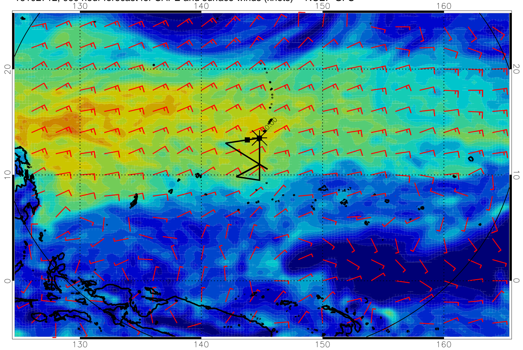
16102712, 060 hour forecast for CAPE and surface winds (knots) -- NCEP GFS
