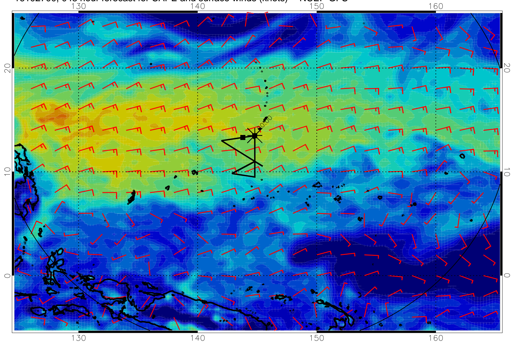
16102700, 048 hour forecast for CAPE and surface winds (knots) -- NCEP GFS
