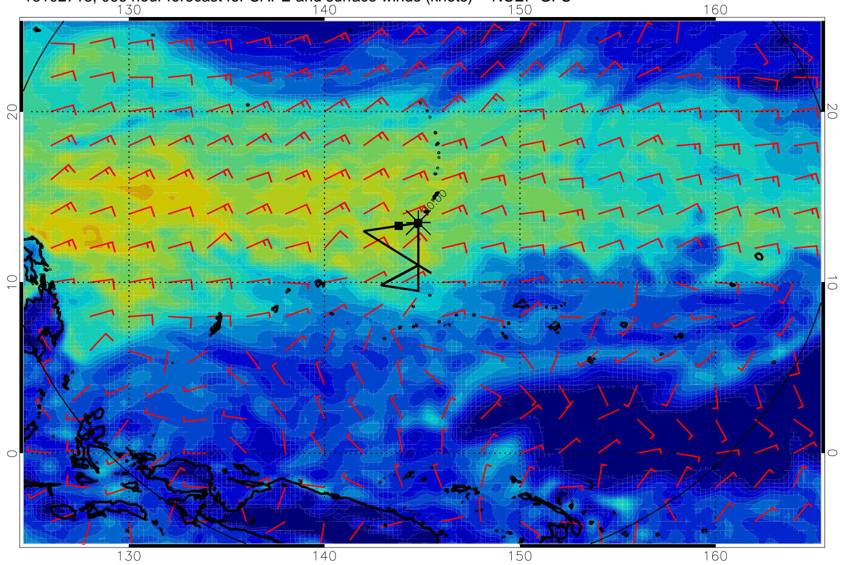
16102718, 066 hour forecast for CAPE and surface winds (knots) -- NCEP GFS
