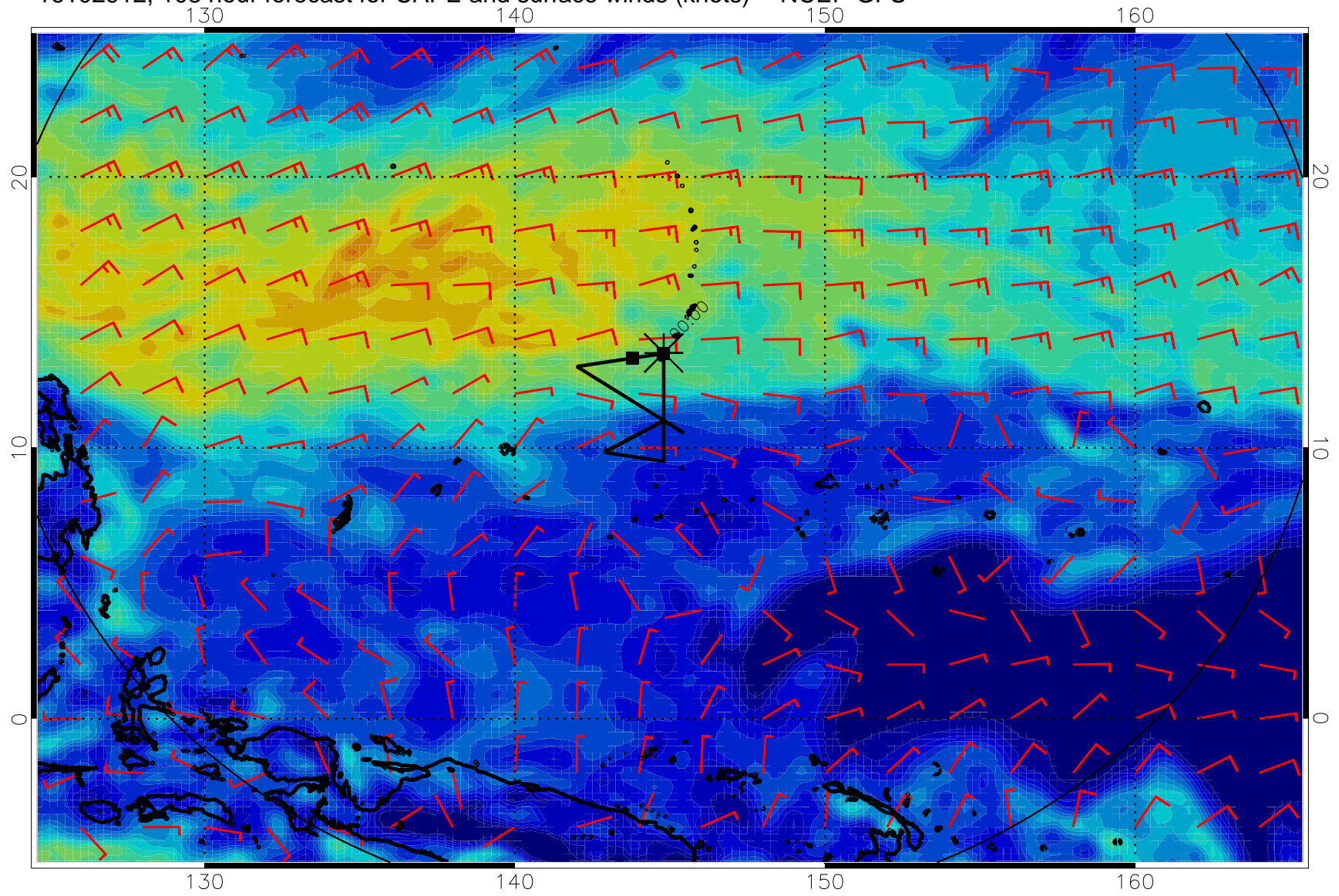
16102912, 108 hour forecast for CAPE and surface winds (knots) -- NCEP GFS
