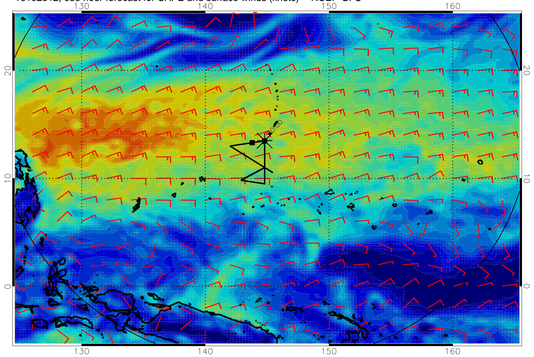
16102612, 036 hour forecast for CAPE and surface winds (knots) -- NCEP GFS
