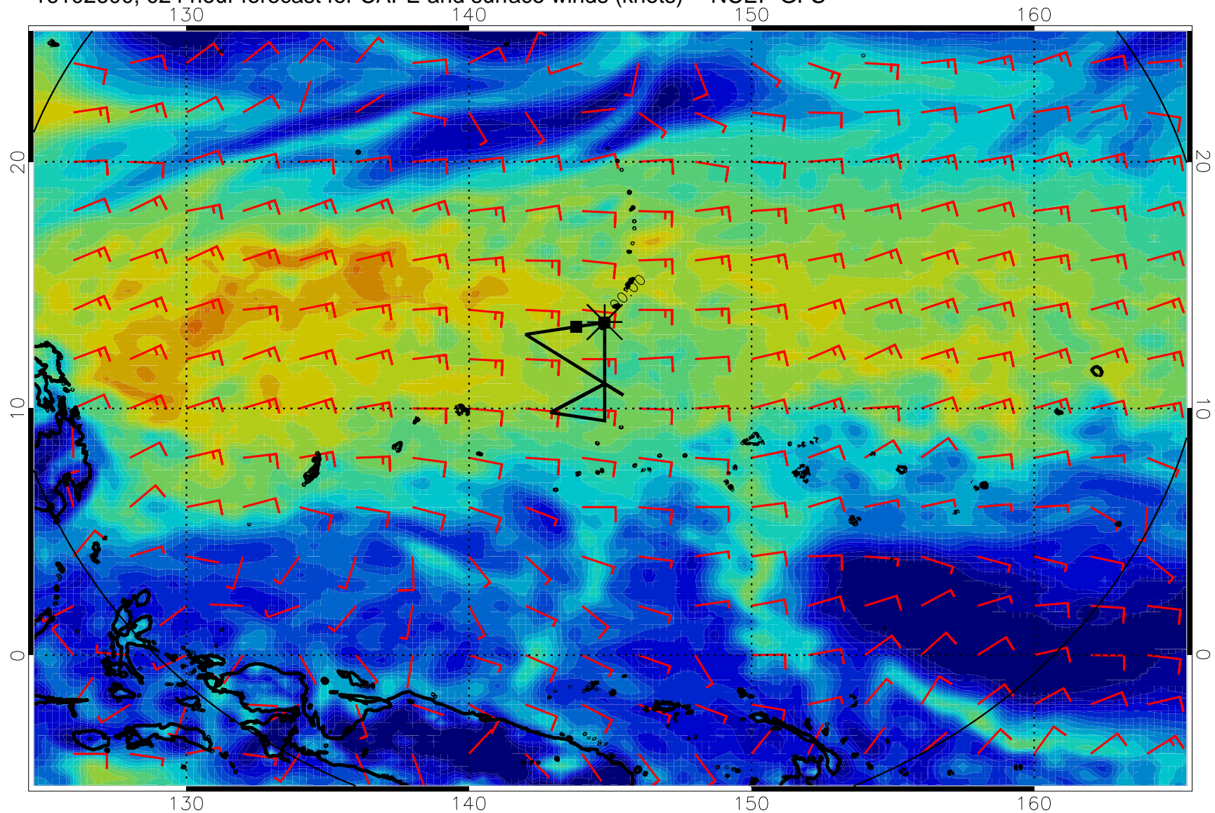
16102600, 024 hour forecast for CAPE and surface winds (knots) -- NCEP GFS
