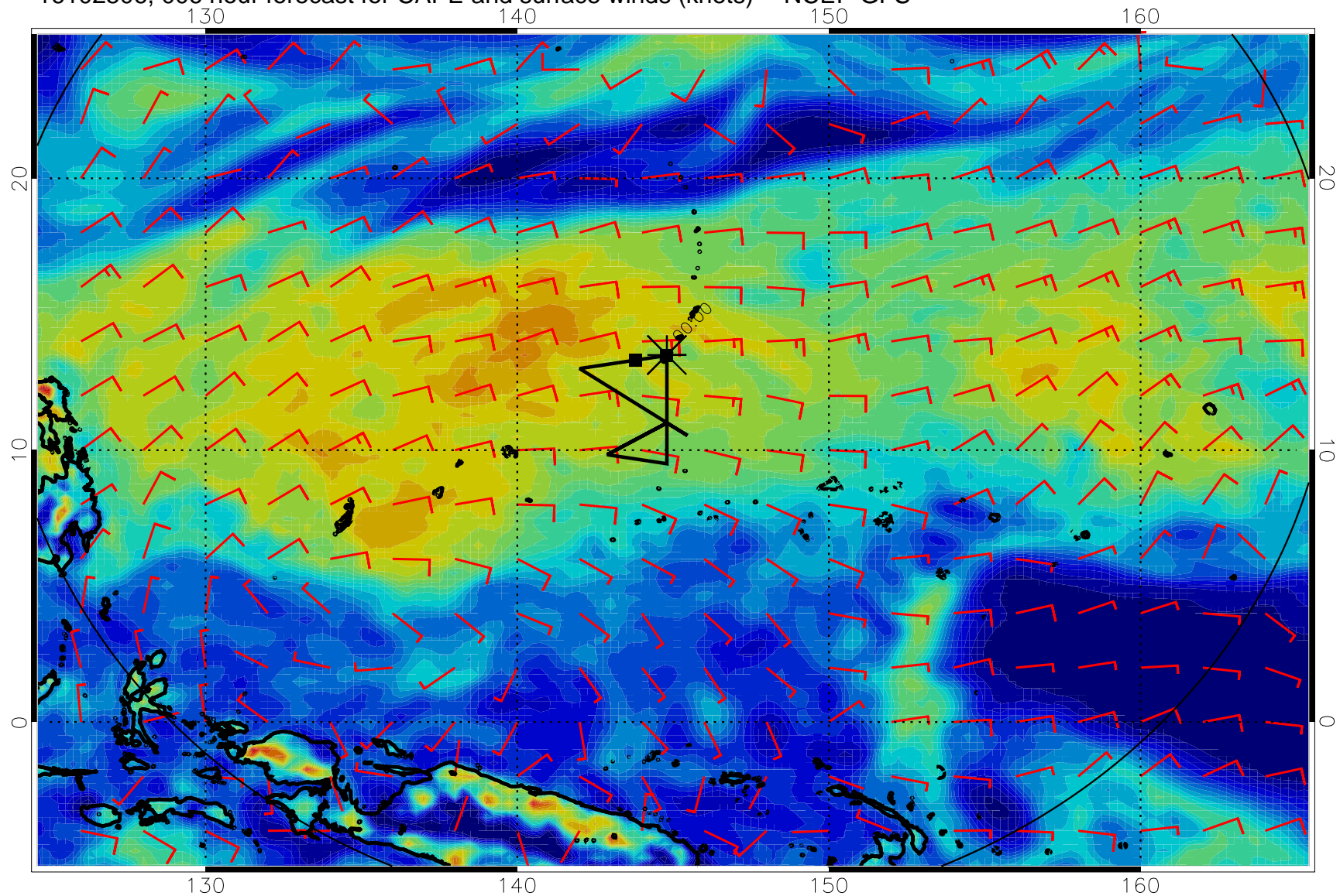
16102506, 006 hour forecast for CAPE and surface winds (knots) -- NCEP GFS
