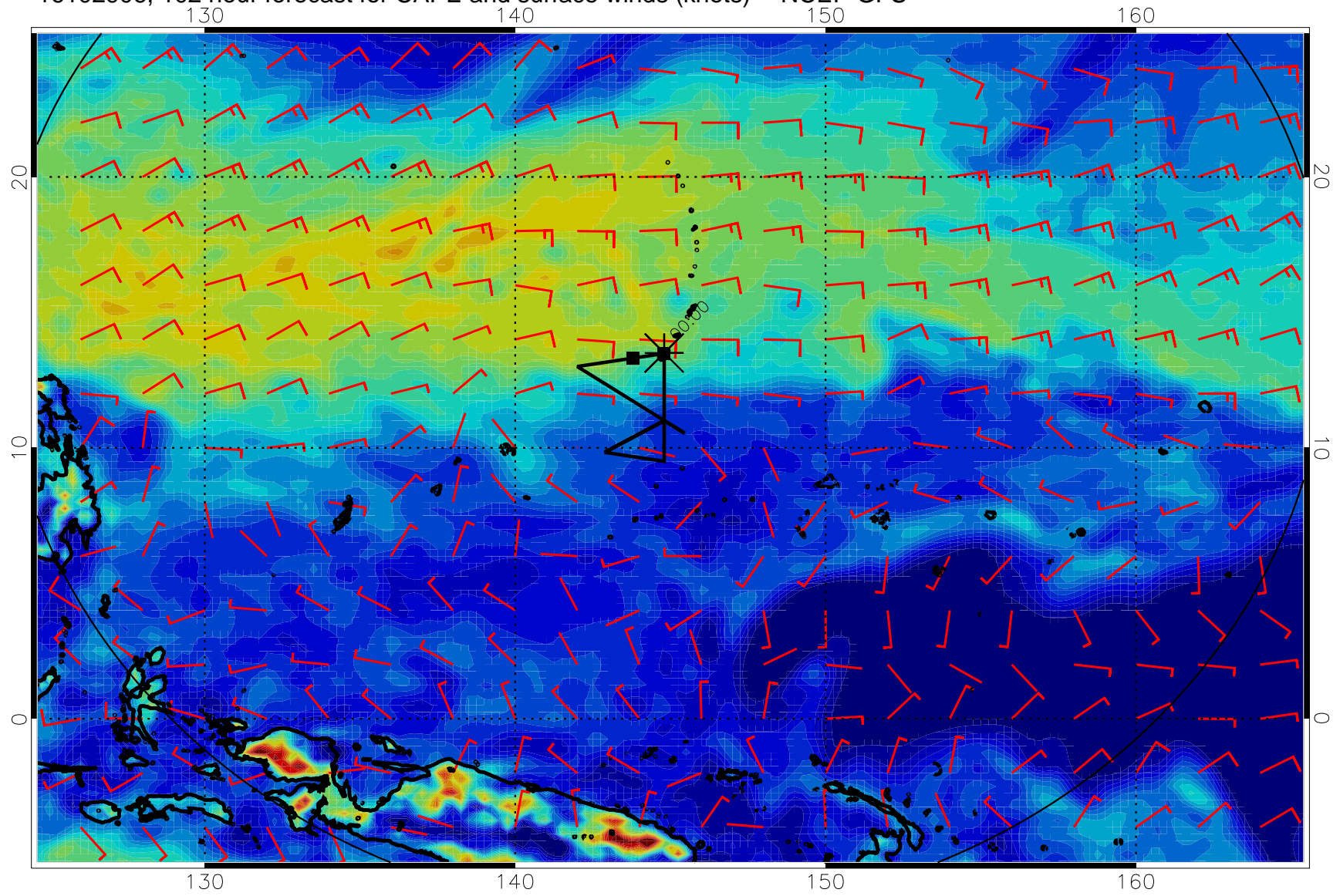
16102906, 102 hour forecast for CAPE and surface winds (knots) -- NCEP GFS
