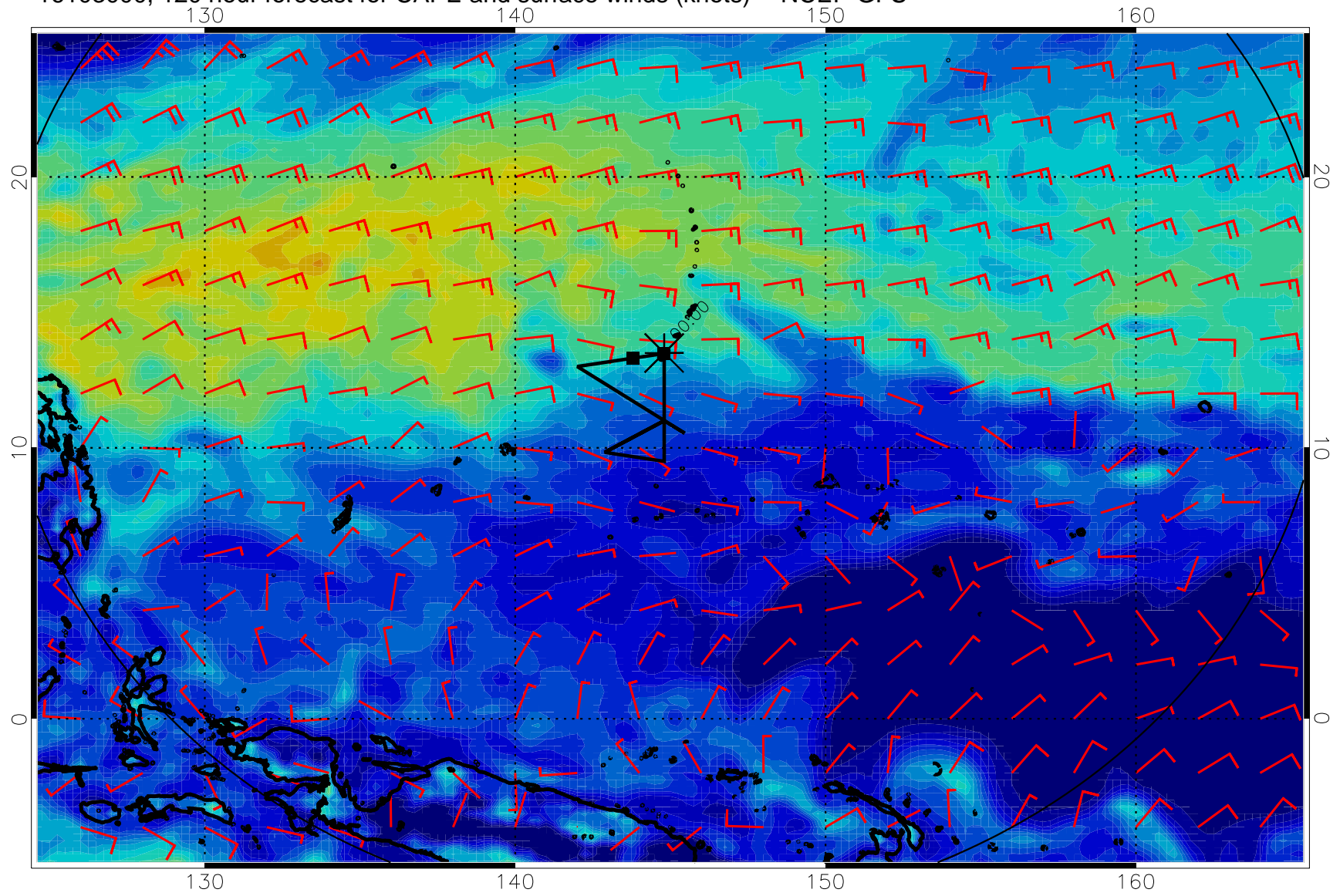
16103000, 120 hour forecast for CAPE and surface winds (knots) -- NCEP GFS
