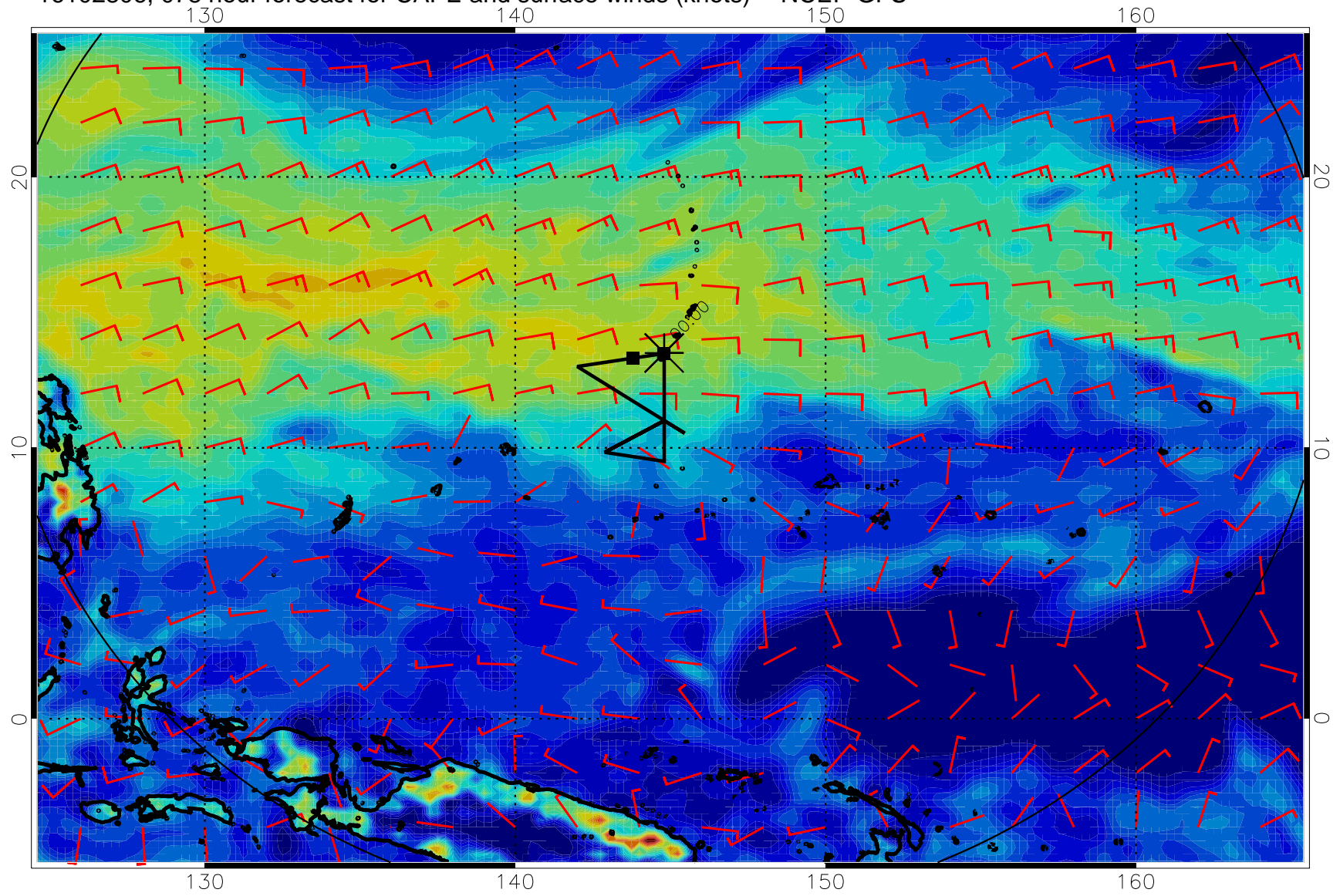
16102806, 078 hour forecast for CAPE and surface winds (knots) -- NCEP GFS
