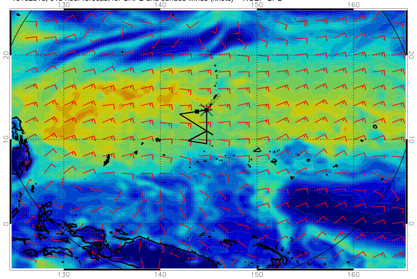
16102518, 018 hour forecast for CAPE and surface winds (knots) -- NCEP GFS
