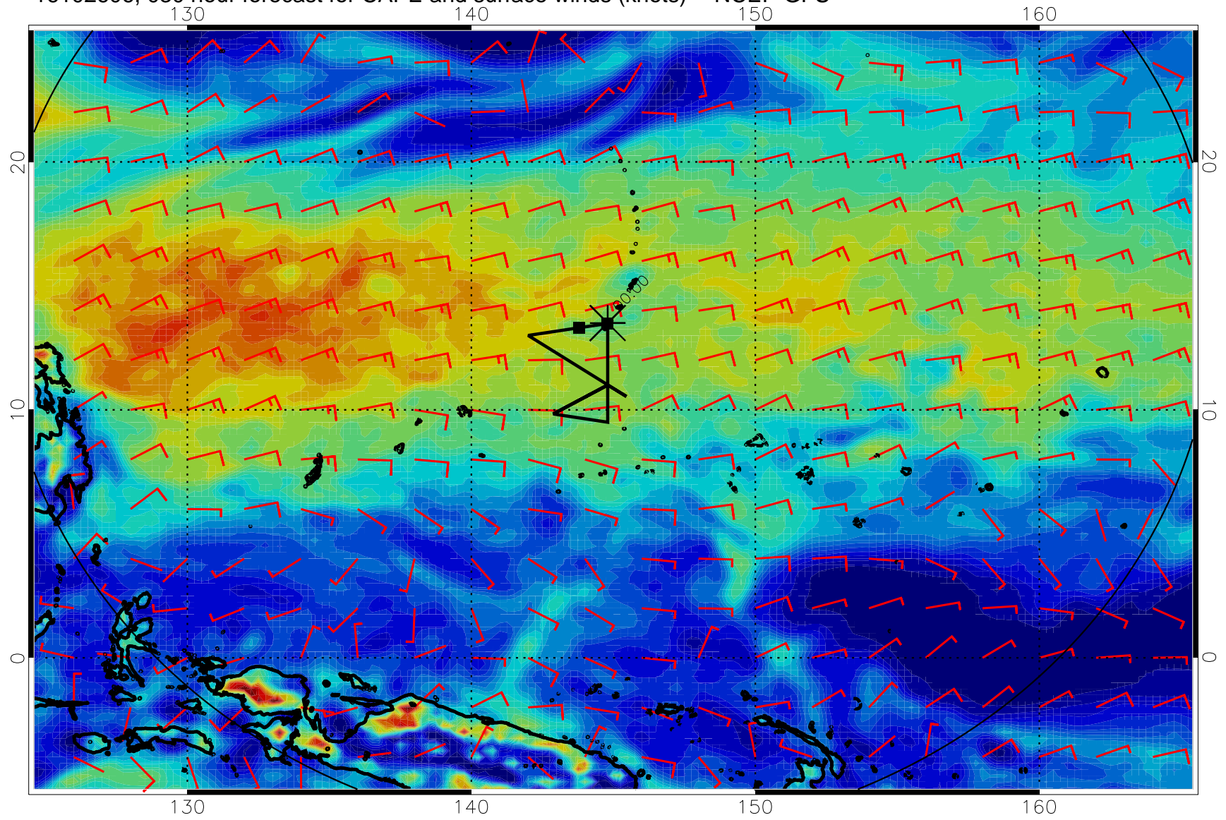
16102606, 030 hour forecast for CAPE and surface winds (knots) -- NCEP GFS
