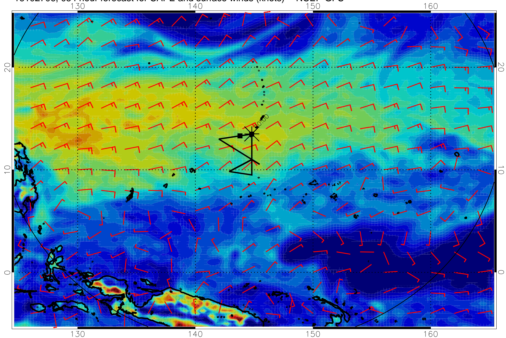
16102706, 054 hour forecast for CAPE and surface winds (knots) -- NCEP GFS
