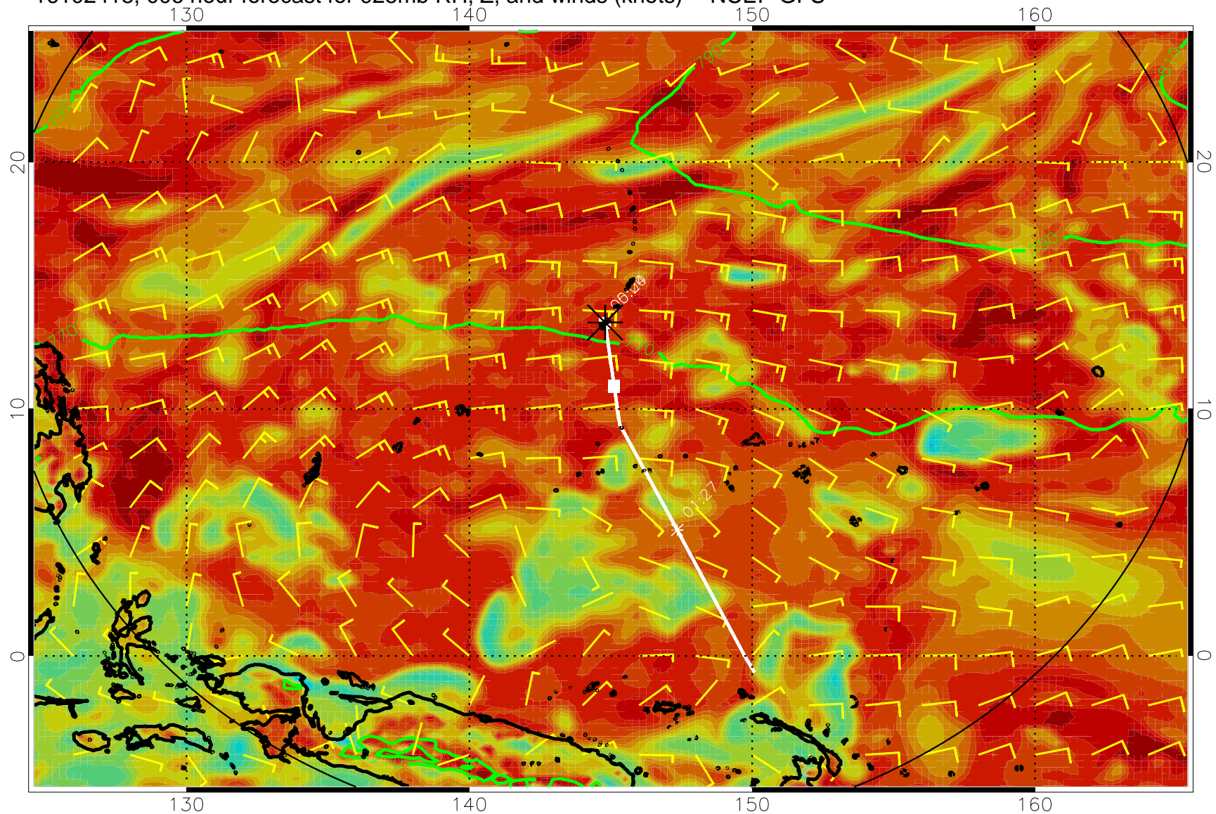
16102418, 006 hour forecast for 925mb RH, Z, and winds (knots) -- NCEP GFS
