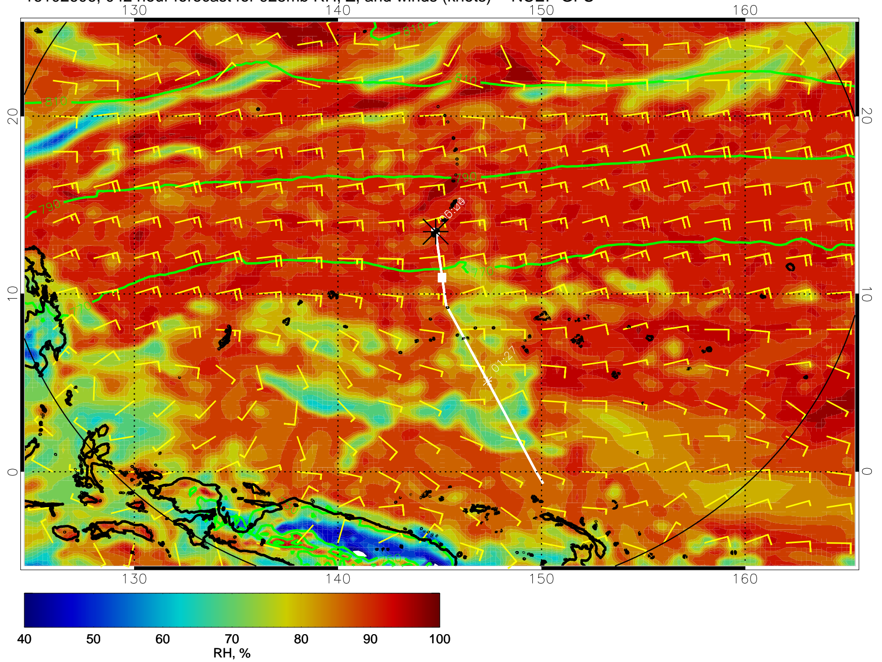
16102606, 042 hour forecast for 925mb RH, Z, and winds (knots) -- NCEP GFS
