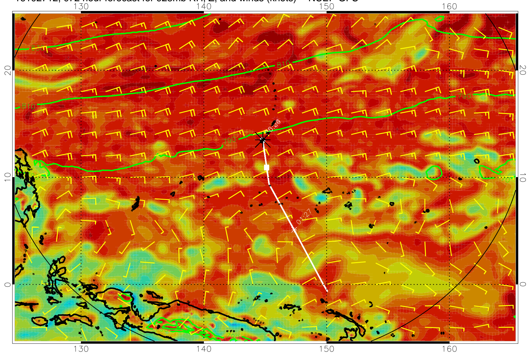
16102712, 072 hour forecast for 925mb RH, Z, and winds (knots) -- NCEP GFS
