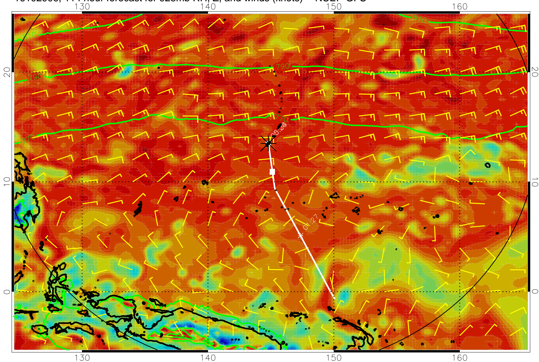
16102906, 114 hour forecast for 925mb RH, Z, and winds (knots) -- NCEP GFS
