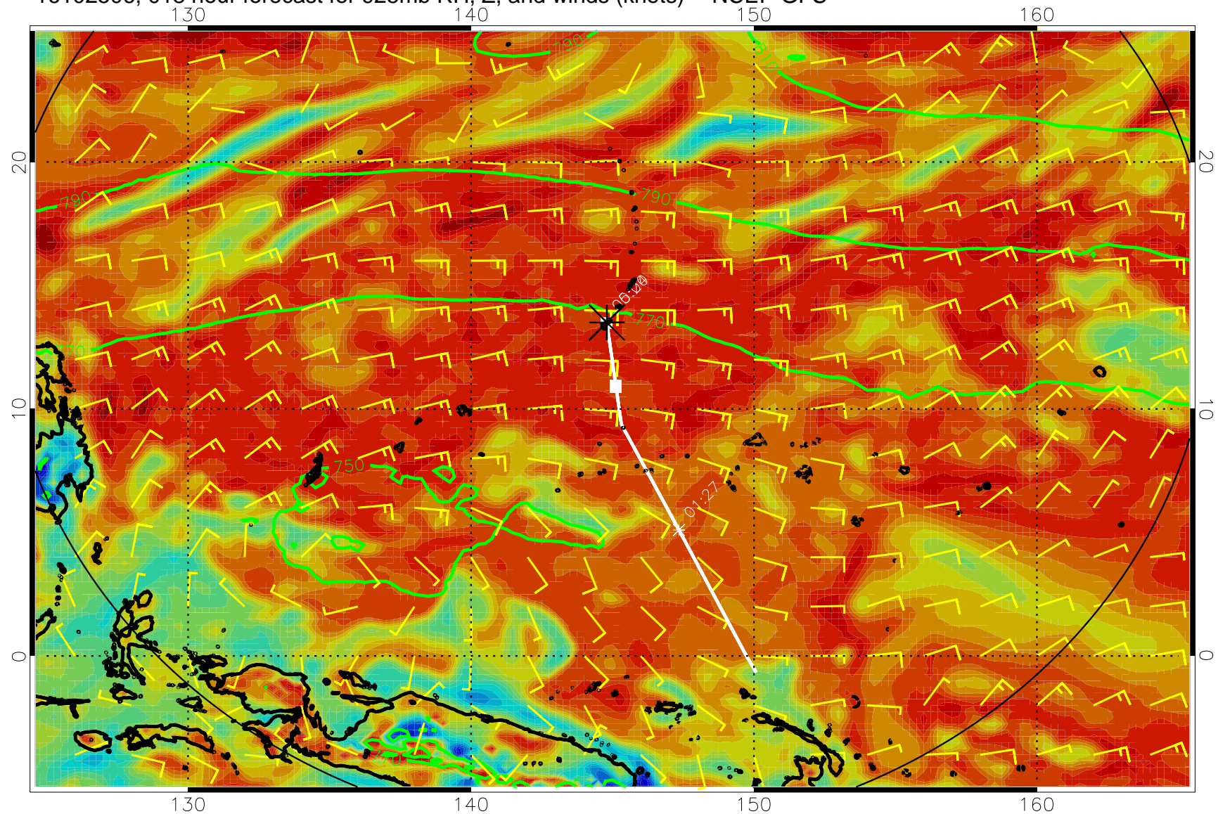
16102506, 018 hour forecast for 925mb RH, Z, and winds (knots) -- NCEP GFS
