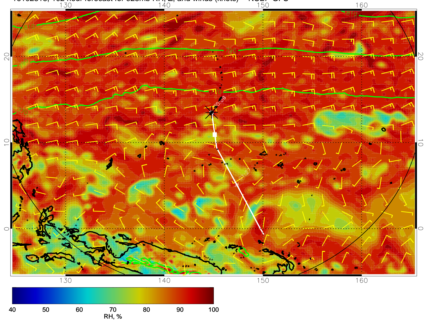
16102818, 102 hour forecast for 925mb RH, Z, and winds (knots) -- NCEP GFS
