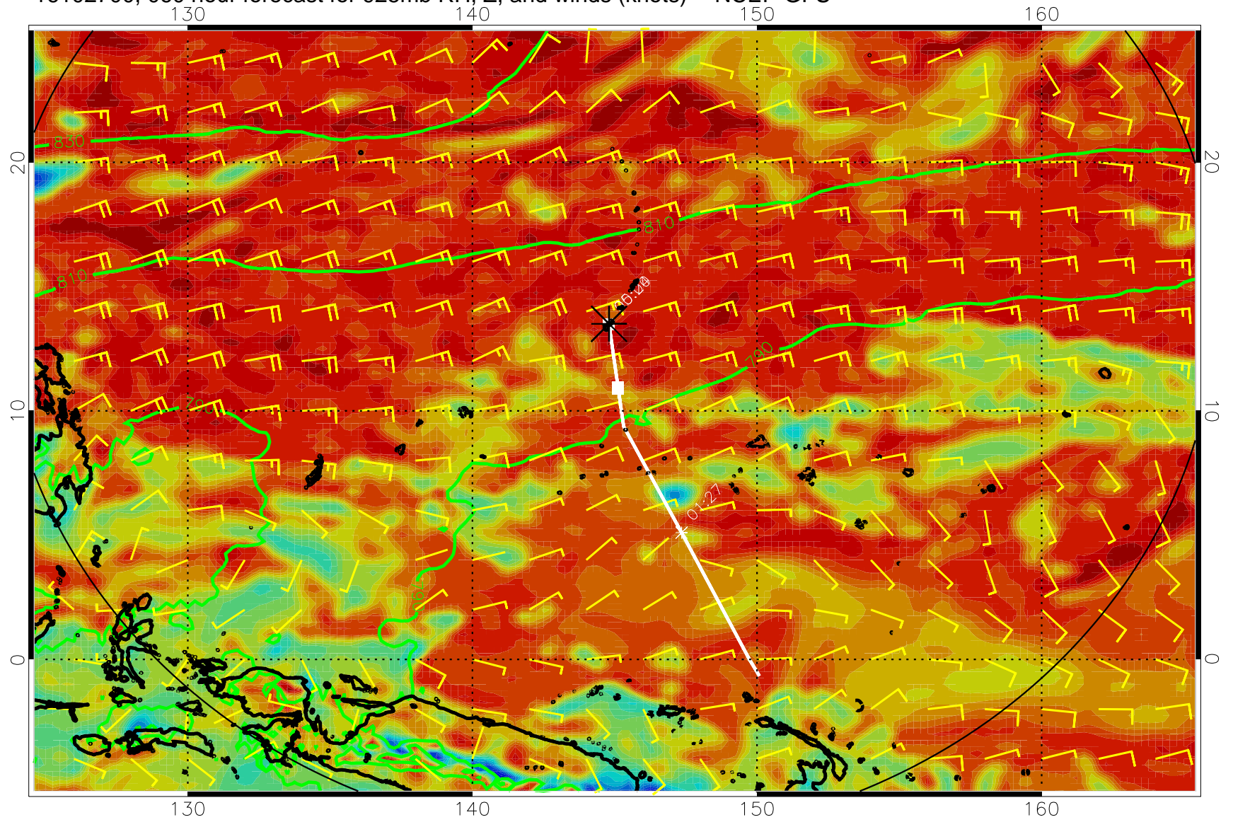
16102700, 060 hour forecast for 925mb RH, Z, and winds (knots) -- NCEP GFS
