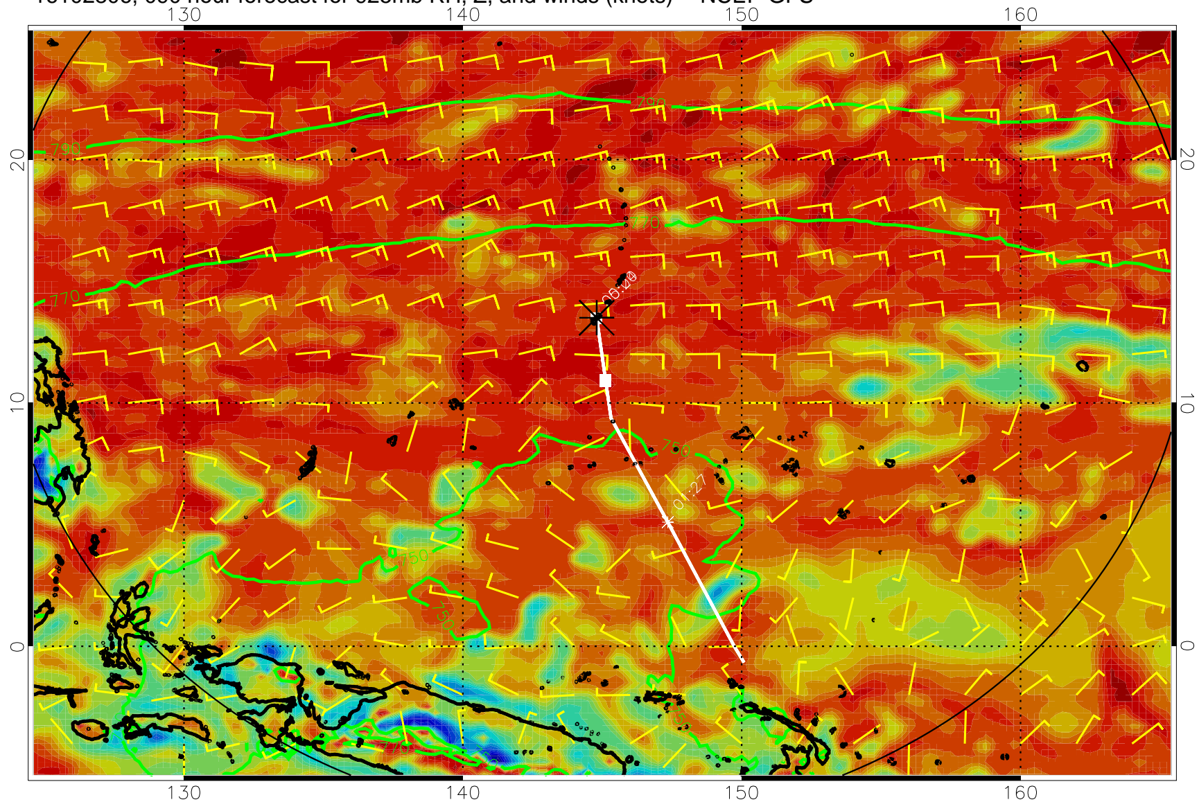
16102806, 090 hour forecast for 925mb RH, Z, and winds (knots) -- NCEP GFS
