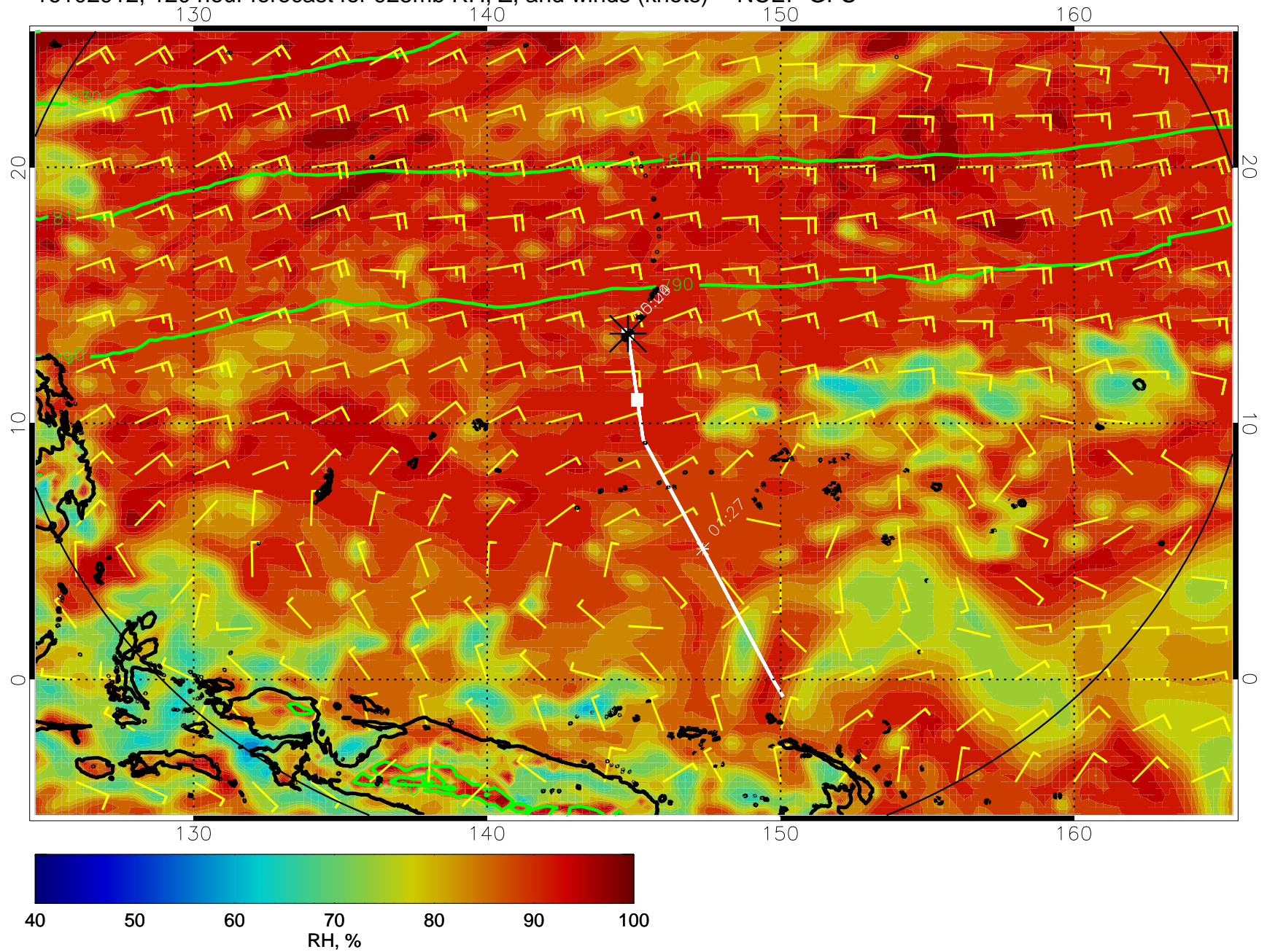
16102912, 120 hour forecast for 925mb RH, Z, and winds (knots) -- NCEP GFS
