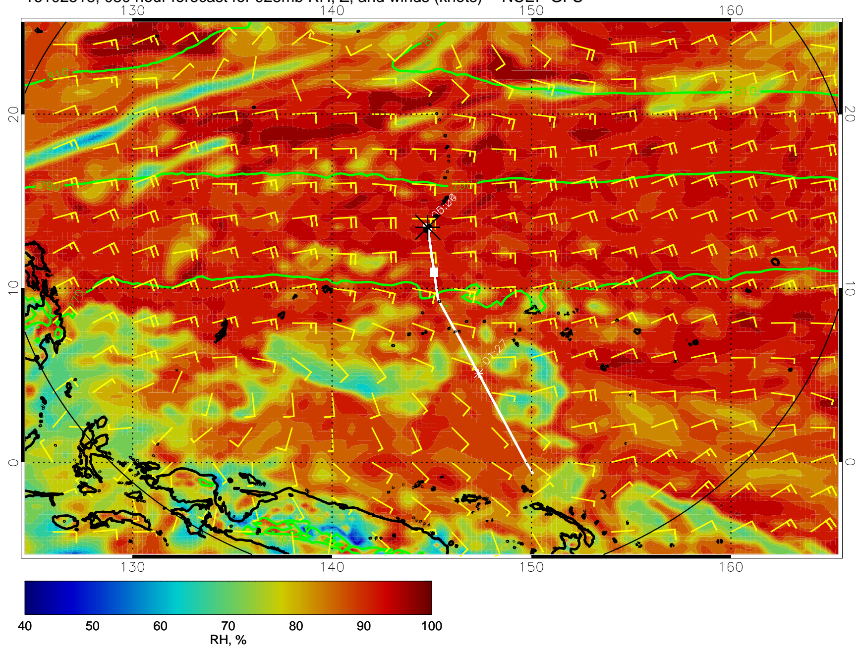
16102518, 030 hour forecast for 925mb RH, Z, and winds (knots) -- NCEP GFS
