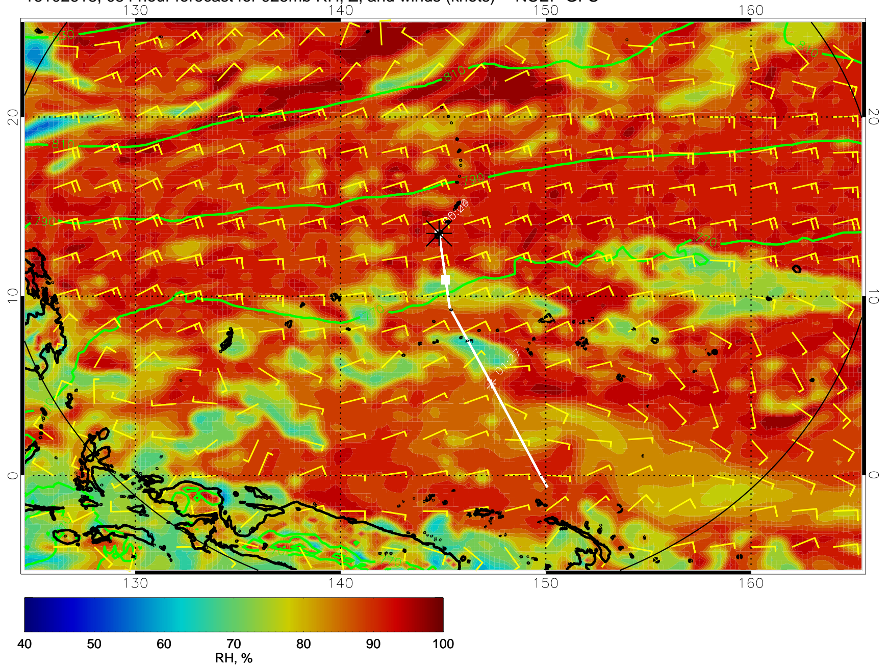
16102618, 054 hour forecast for 925mb RH, Z, and winds (knots) -- NCEP GFS
