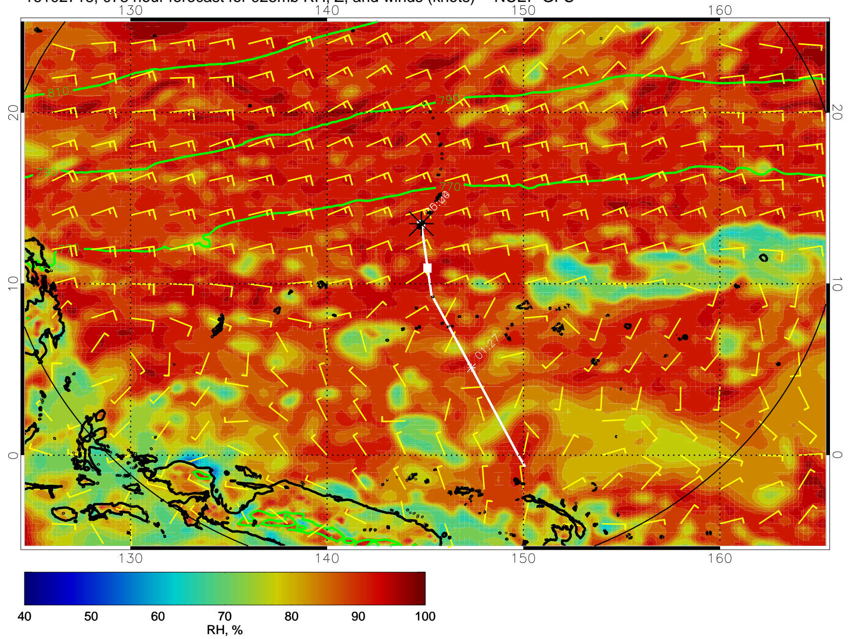
16102718, 078 hour forecast for 925mb RH, Z, and winds (knots) -- NCEP GFS
