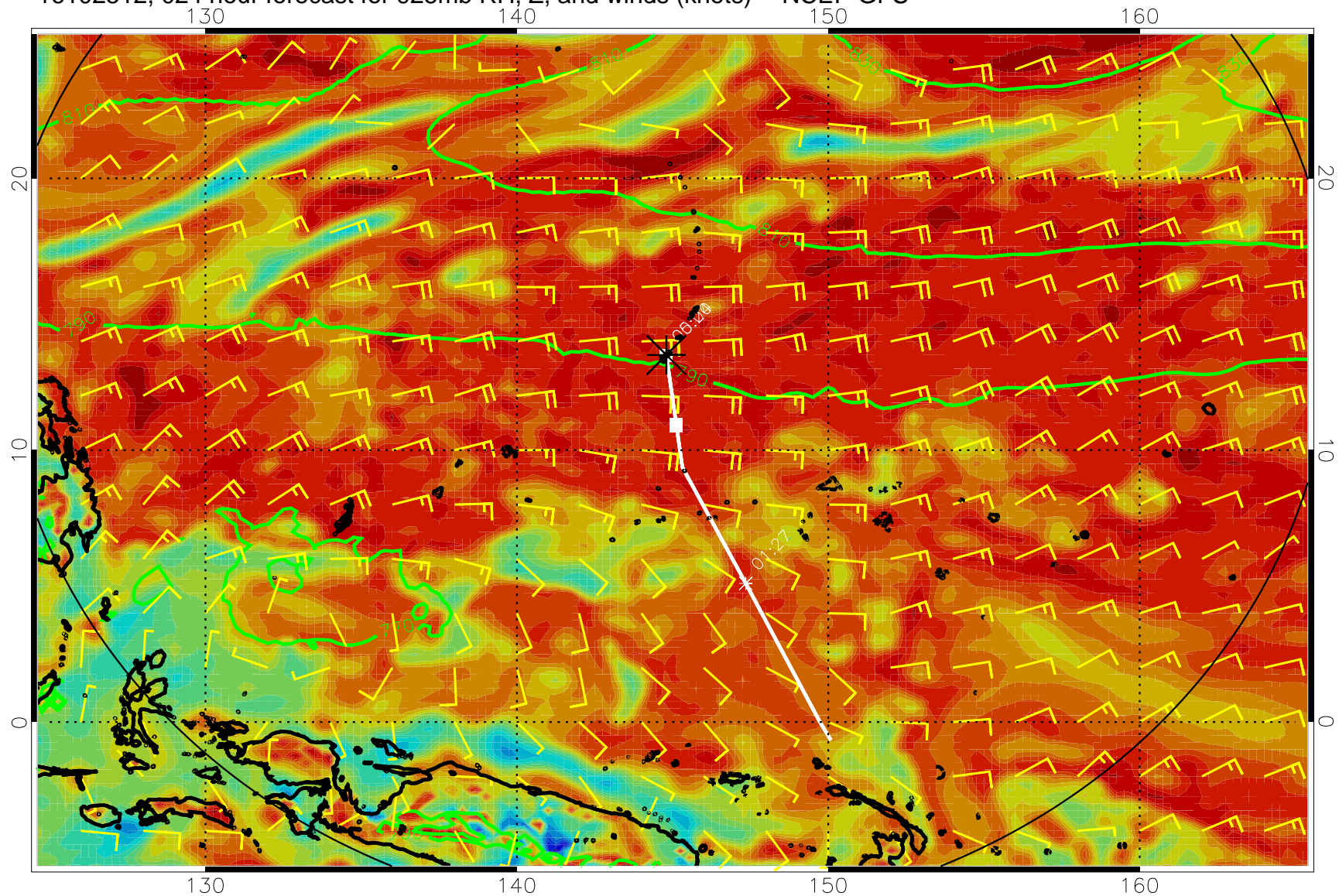
16102512, 024 hour forecast for 925mb RH, Z, and winds (knots) -- NCEP GFS
