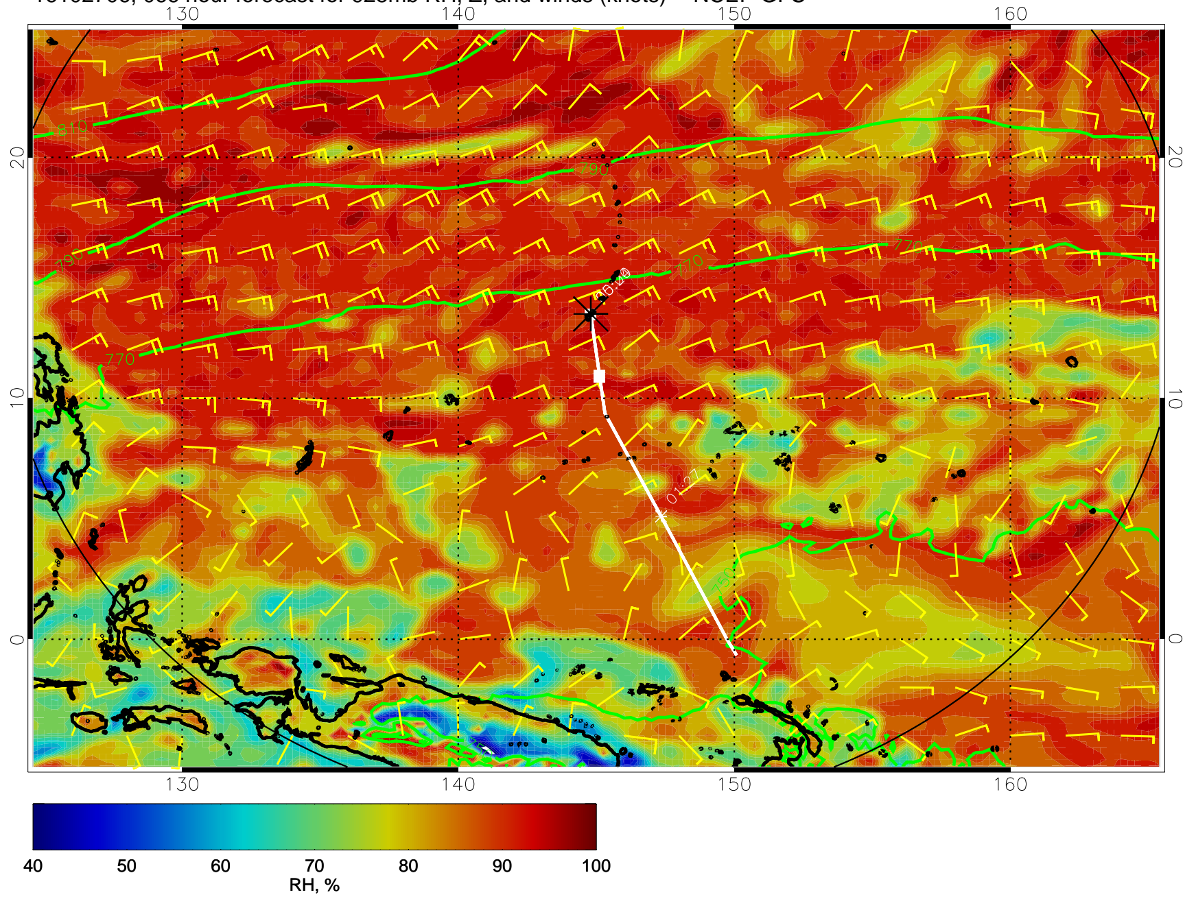
16102706, 066 hour forecast for 925mb RH, Z, and winds (knots) -- NCEP GFS
