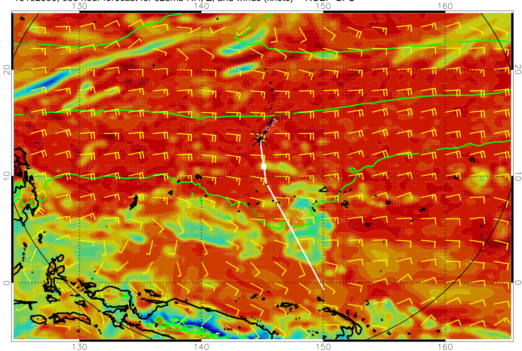
16102600, 036 hour forecast for 925mb RH, Z, and winds (knots) -- NCEP GFS
