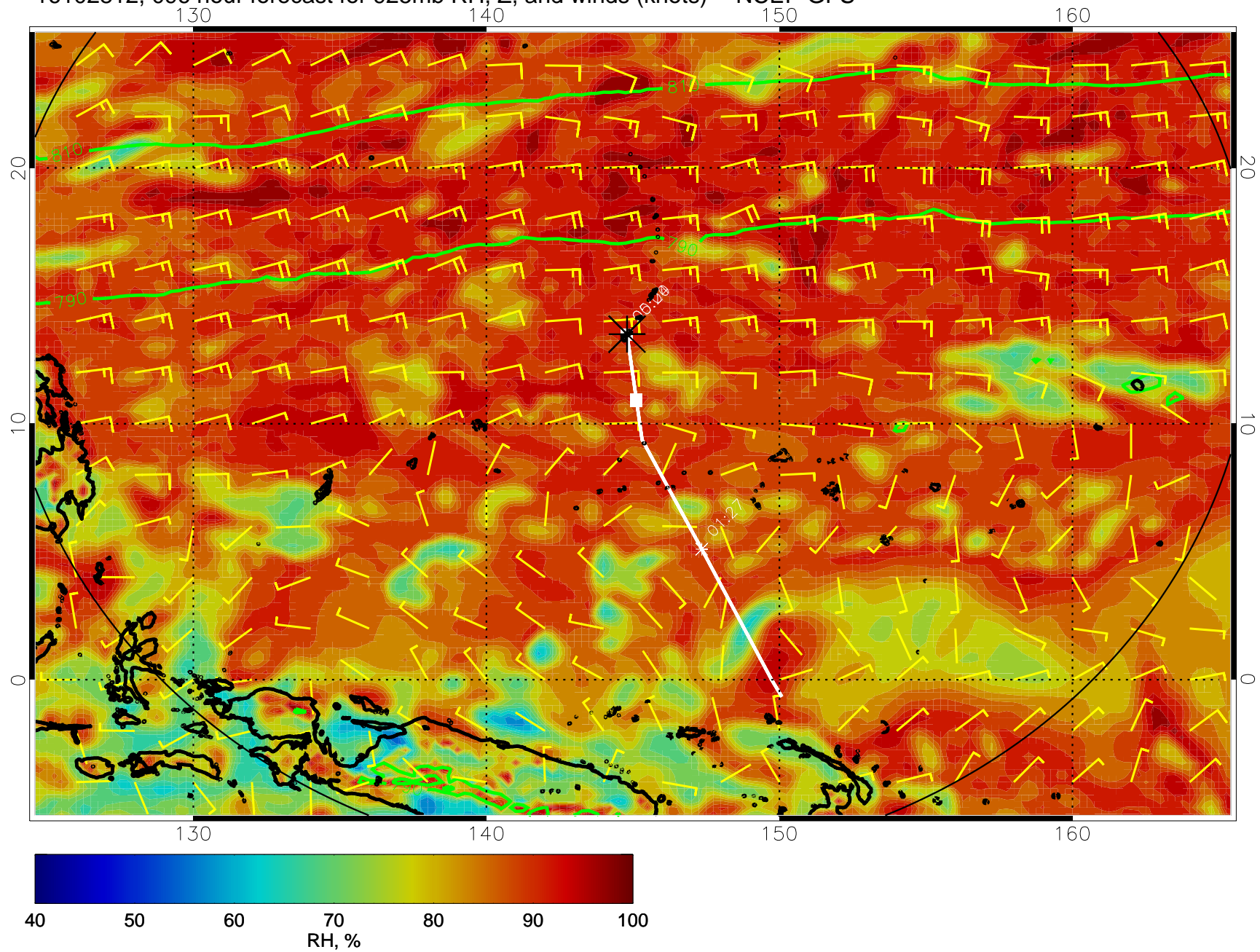
16102812, 096 hour forecast for 925mb RH, Z, and winds (knots) -- NCEP GFS
