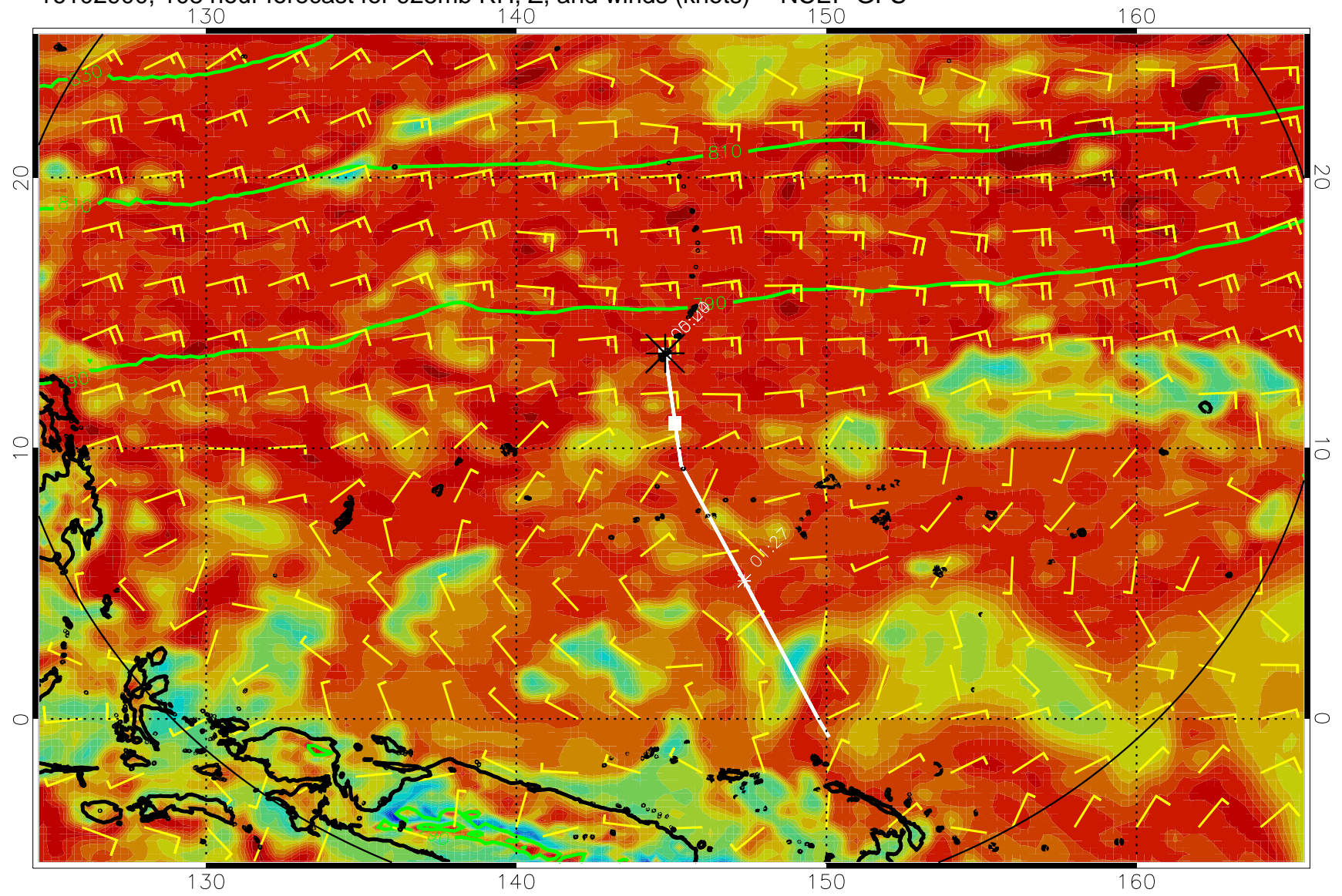
16102900, 108 hour forecast for 925mb RH, Z, and winds (knots) -- NCEP GFS
