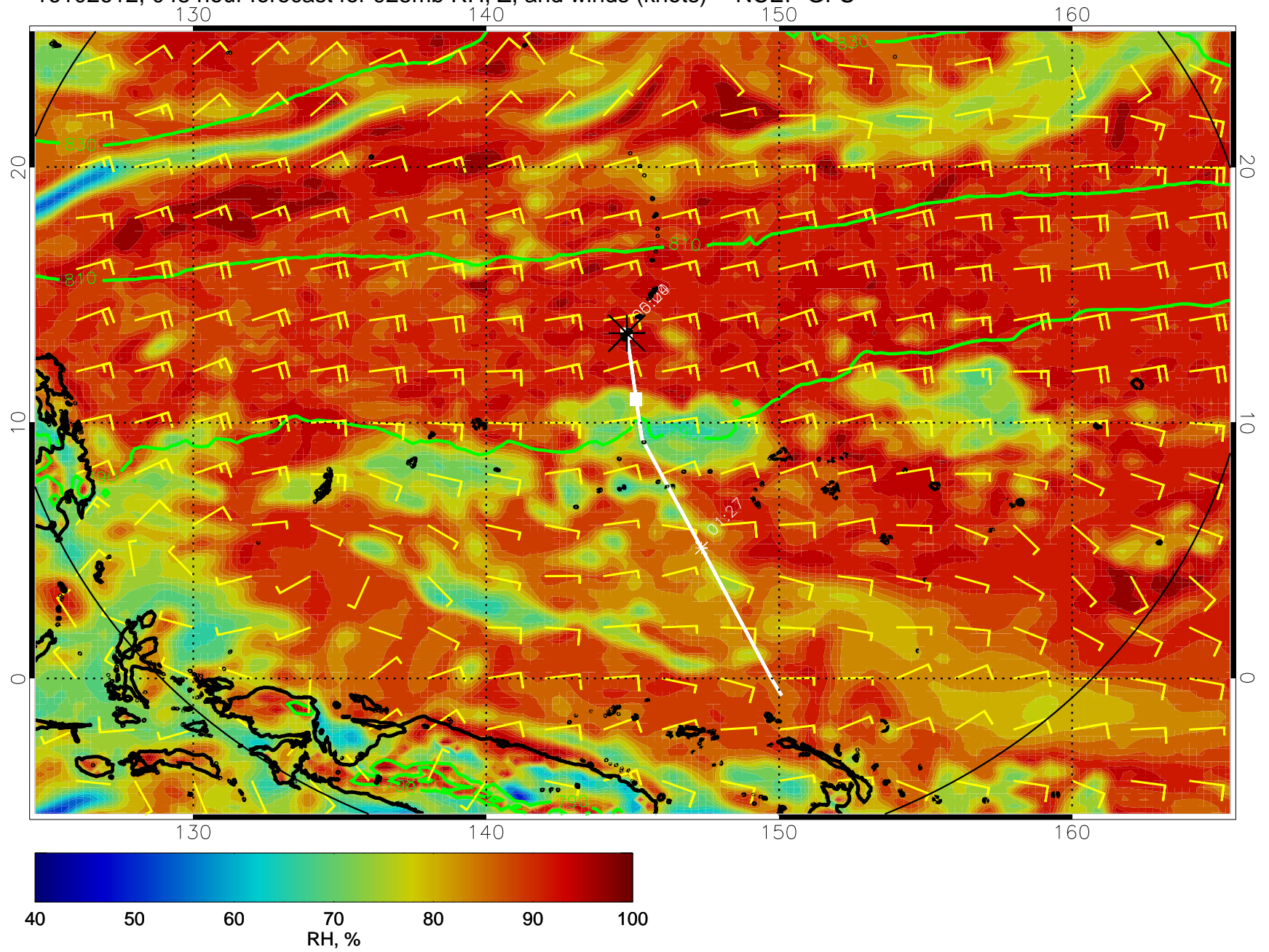
16102612, 048 hour forecast for 925mb RH, Z, and winds (knots) -- NCEP GFS
