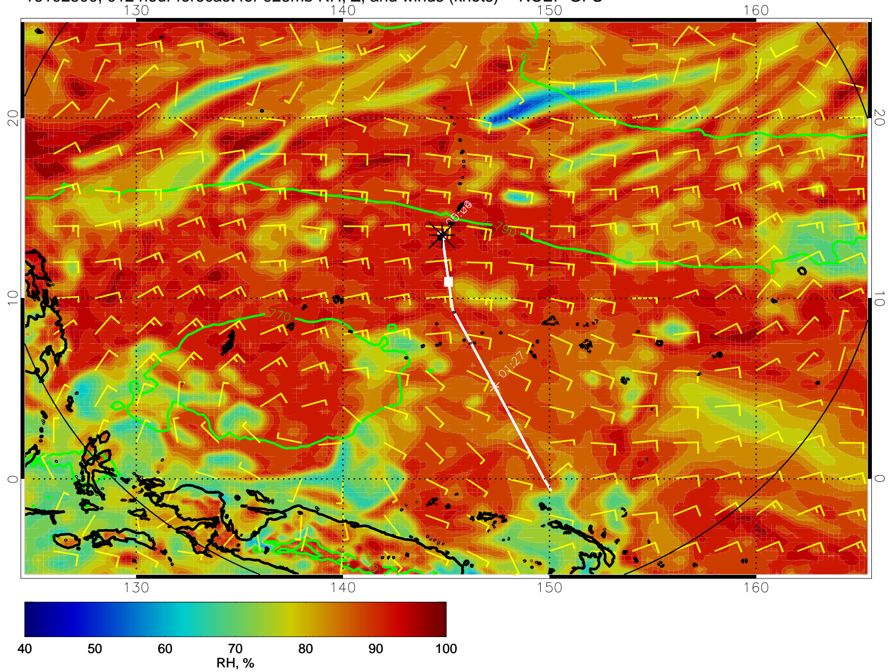
16102500, 012 hour forecast for 925mb RH, Z, and winds (knots) -- NCEP GFS
