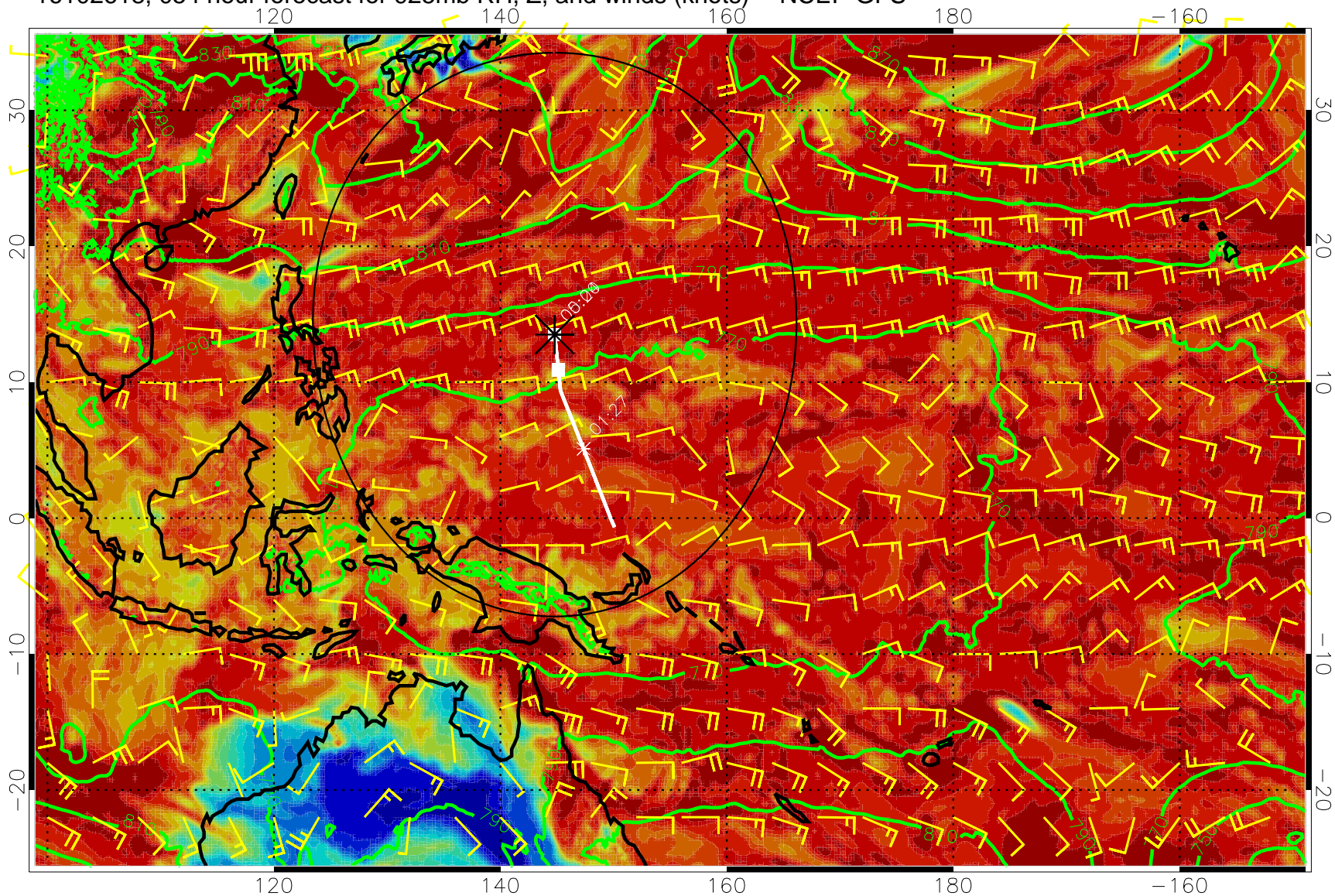
16102618, 054 hour forecast for 925mb RH, Z, and winds (knots) -- NCEP GFS
