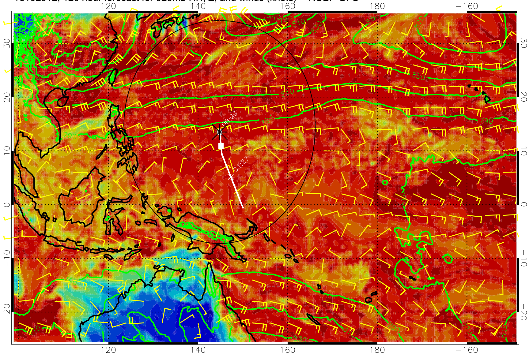
16102912, 120 hour forecast for 925mb RH, Z, and winds (knots) -- NCEP GFS
