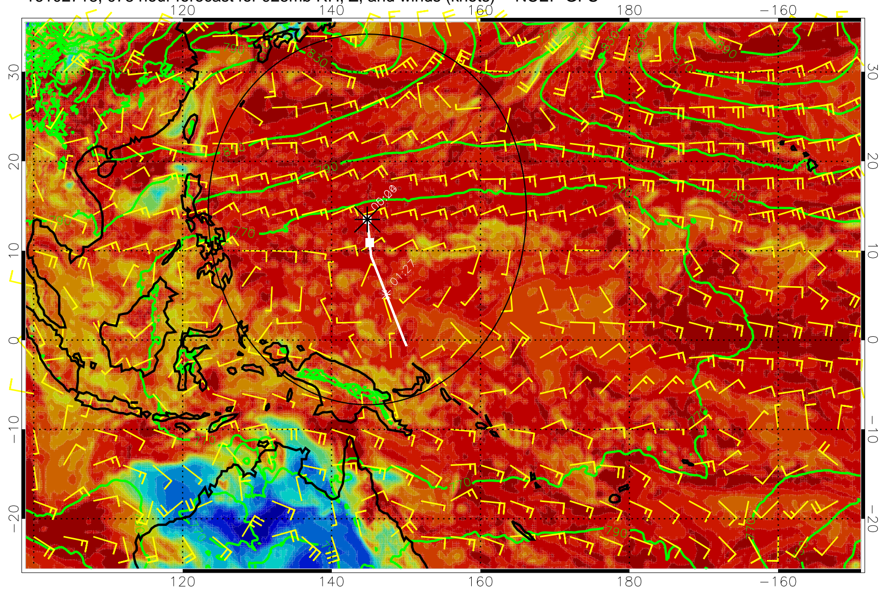
16102718, 078 hour forecast for 925mb RH, Z, and winds (knots) -- NCEP GFS
