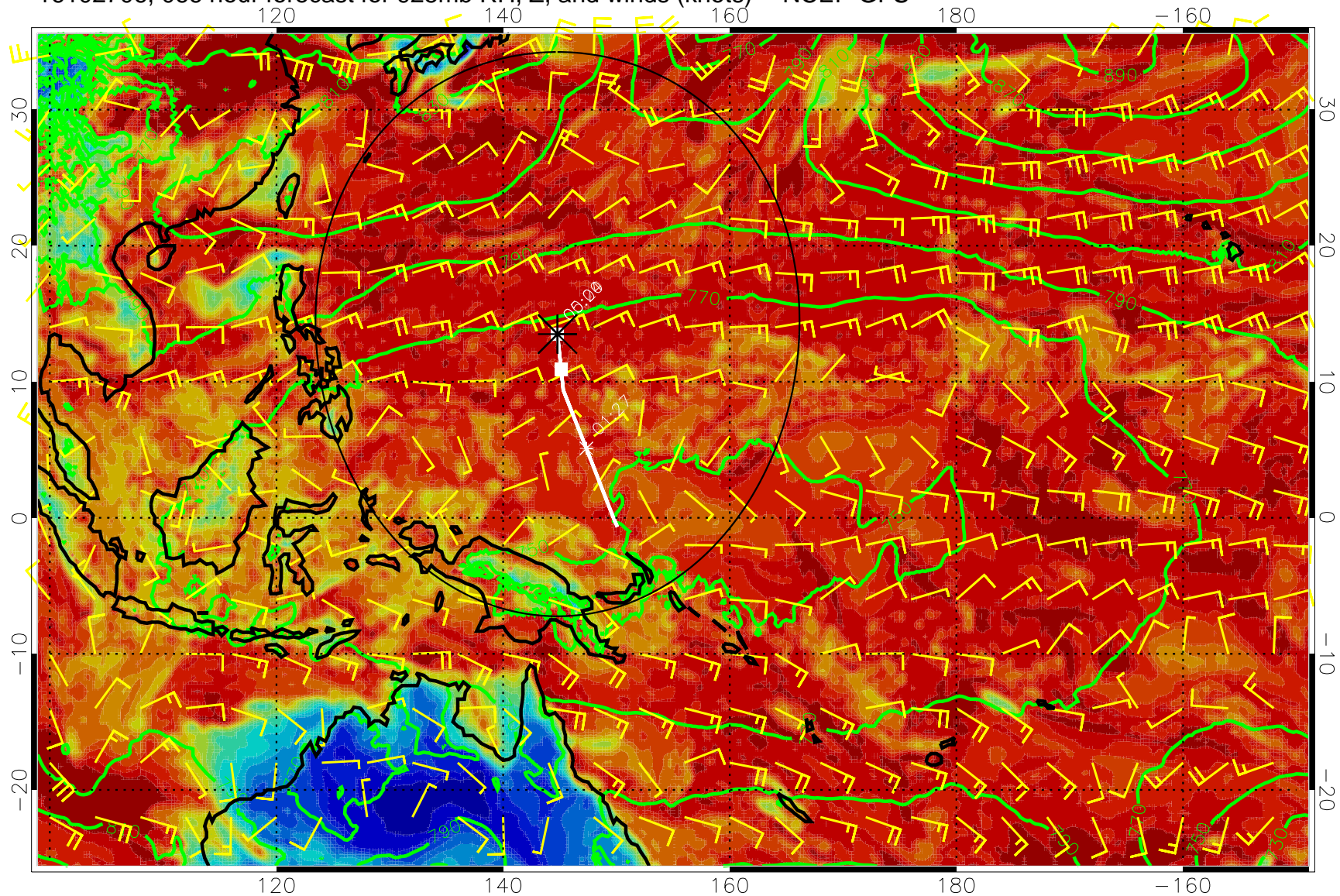
16102706, 066 hour forecast for 925mb RH, Z, and winds (knots) -- NCEP GFS
