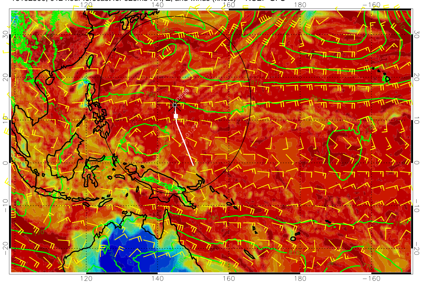
16102500, 012 hour forecast for 925mb RH, Z, and winds (knots) -- NCEP GFS
