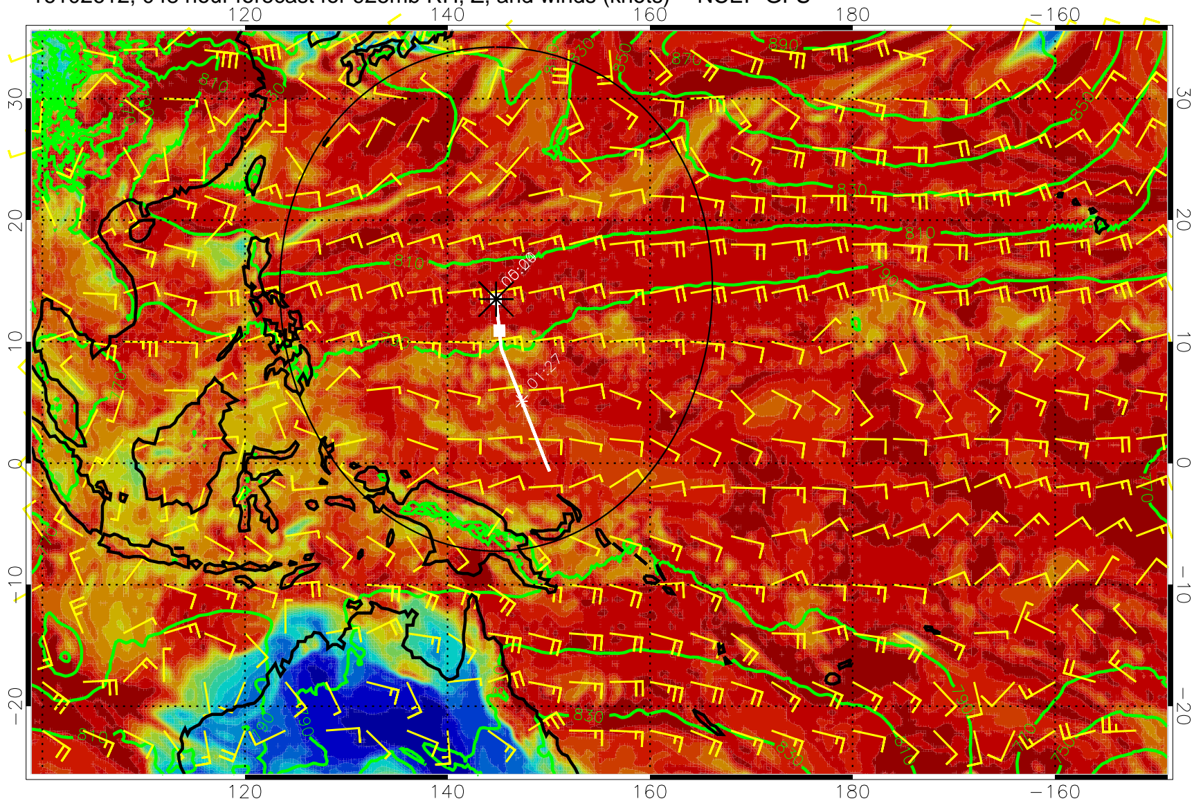
16102612, 048 hour forecast for 925mb RH, Z, and winds (knots) -- NCEP GFS
