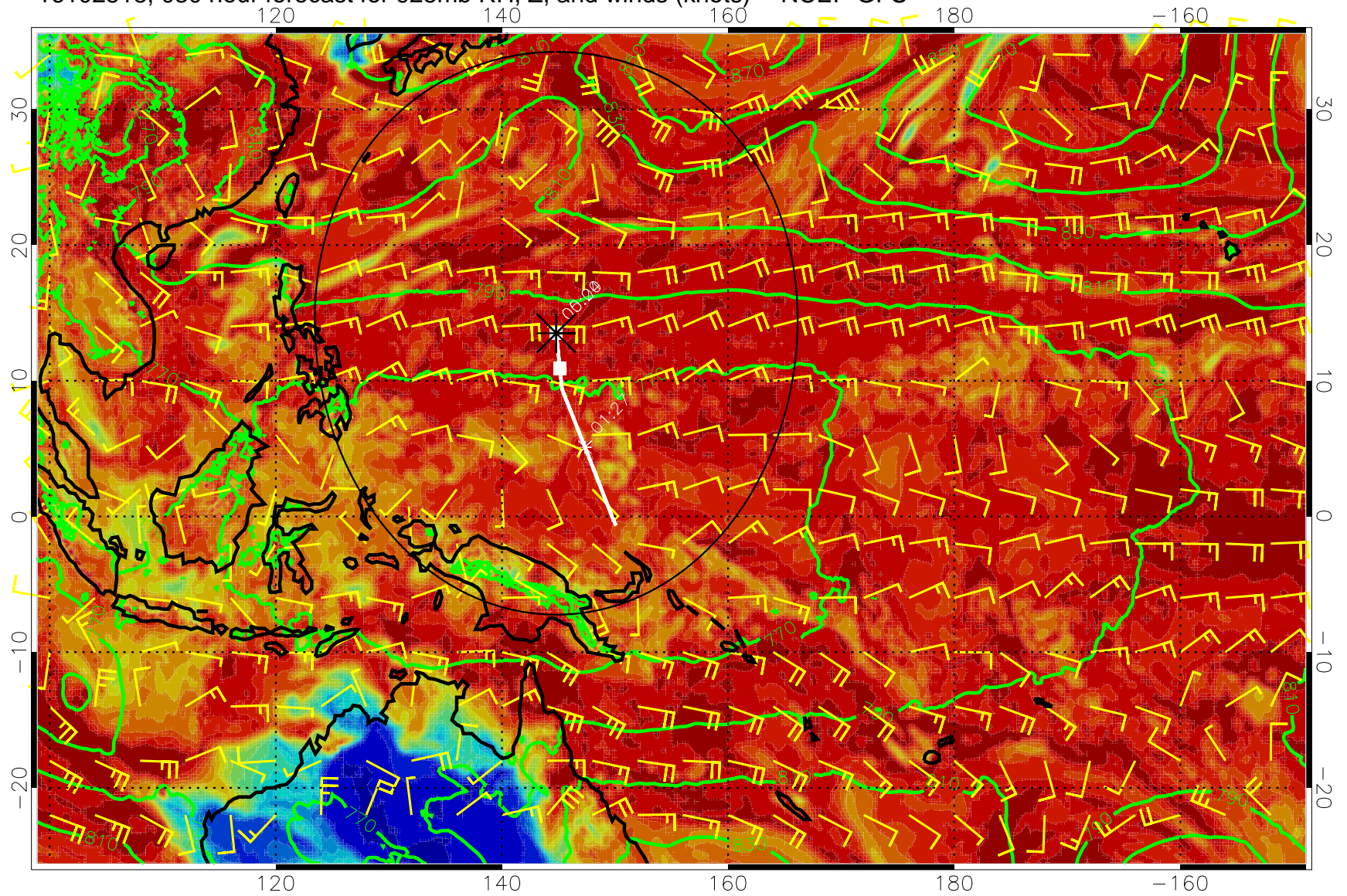
16102518, 030 hour forecast for 925mb RH, Z, and winds (knots) -- NCEP GFS
