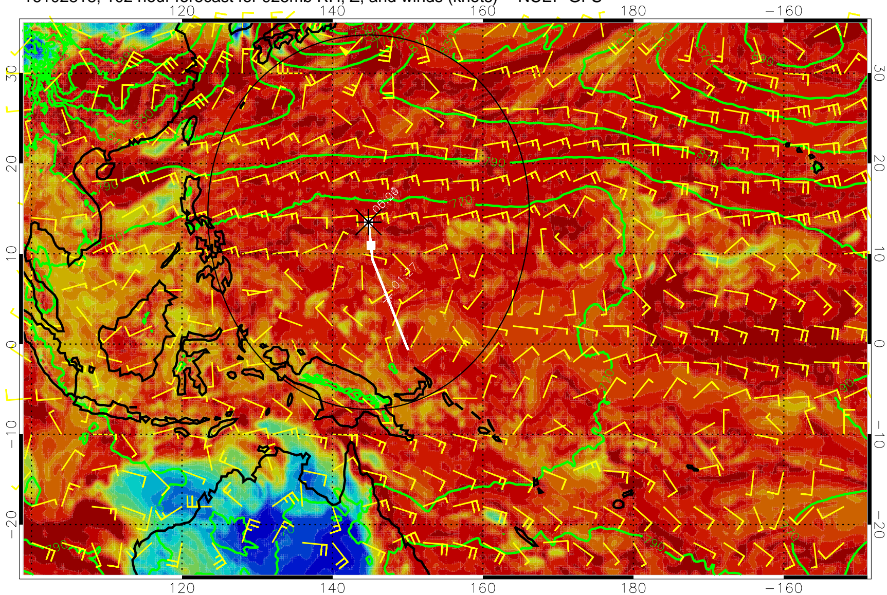
16102818, 102 hour forecast for 925mb RH, Z, and winds (knots) -- NCEP GFS
