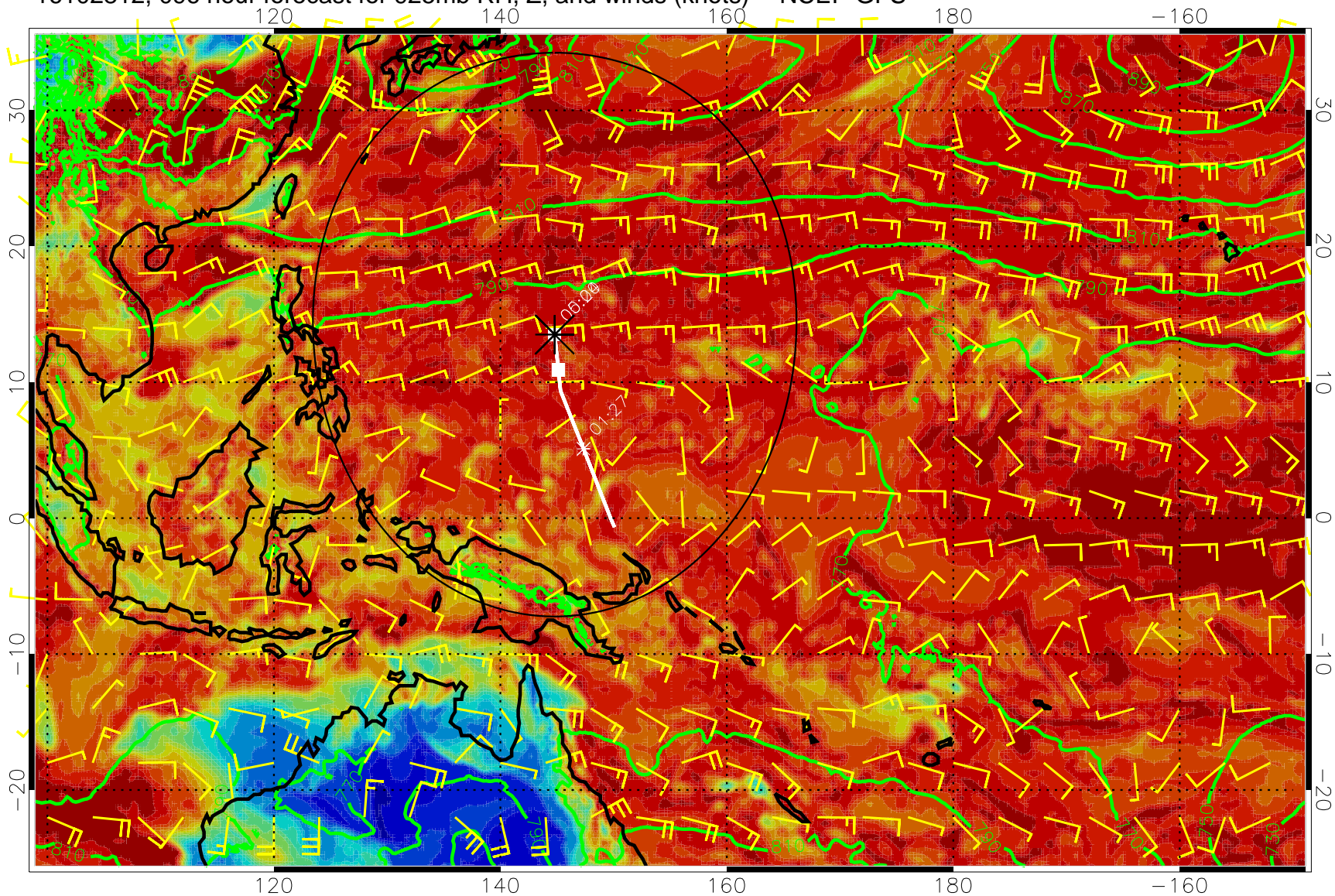
16102812, 096 hour forecast for 925mb RH, Z, and winds (knots) -- NCEP GFS
