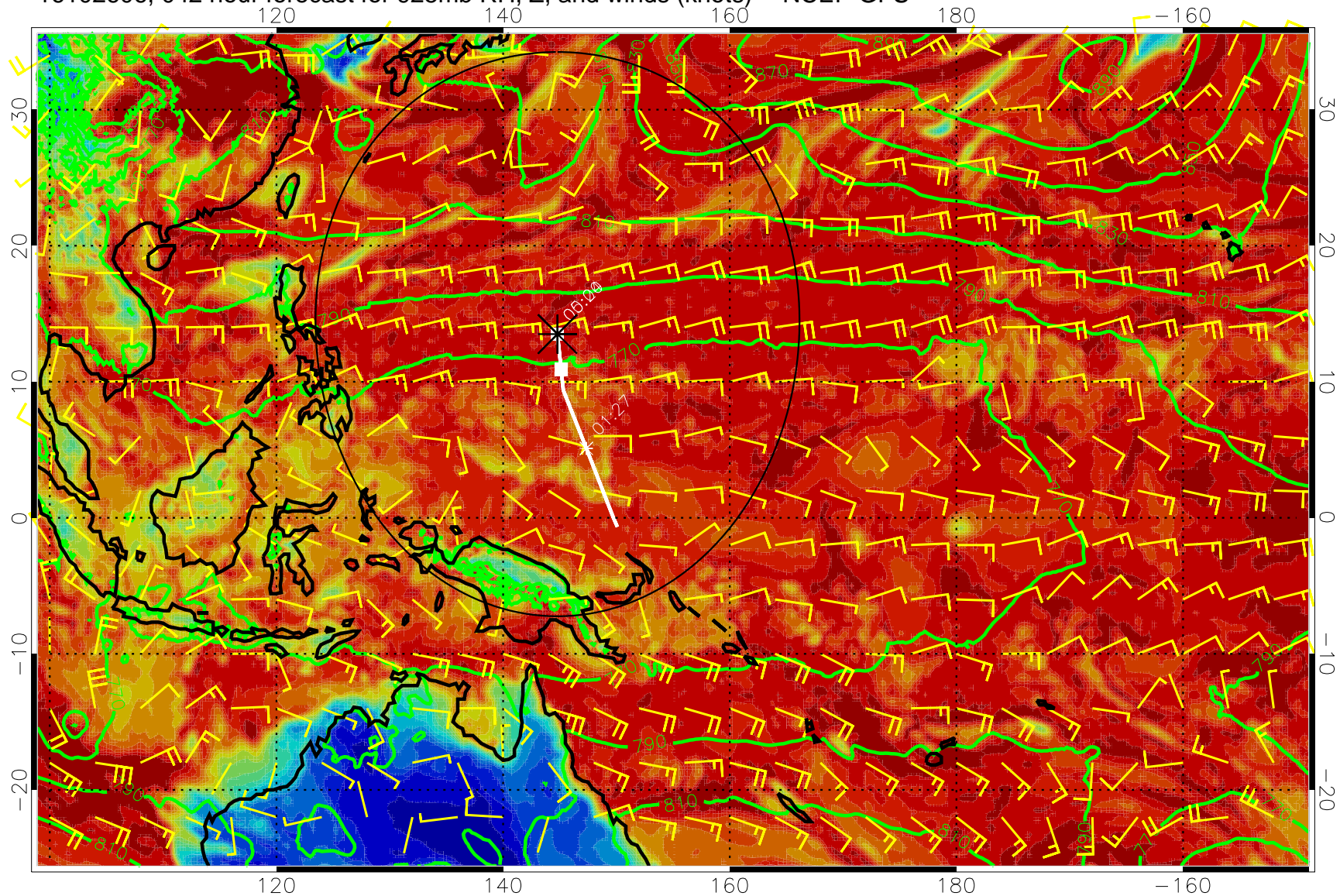
16102606, 042 hour forecast for 925mb RH, Z, and winds (knots) -- NCEP GFS
