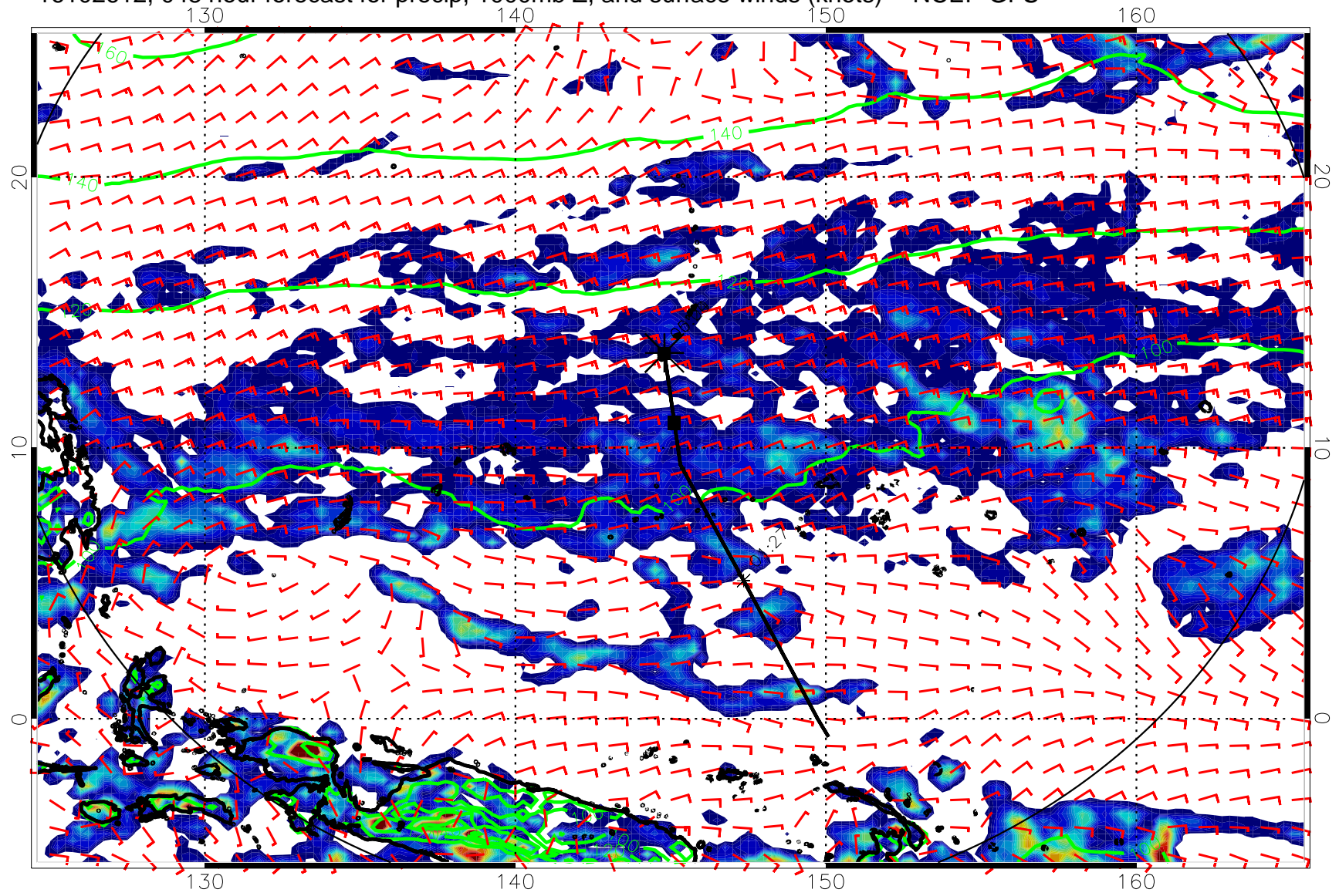
16102612, 048 hour forecast for precip, 1000mb Z, and surface winds (knots) -- NCEP GFS
