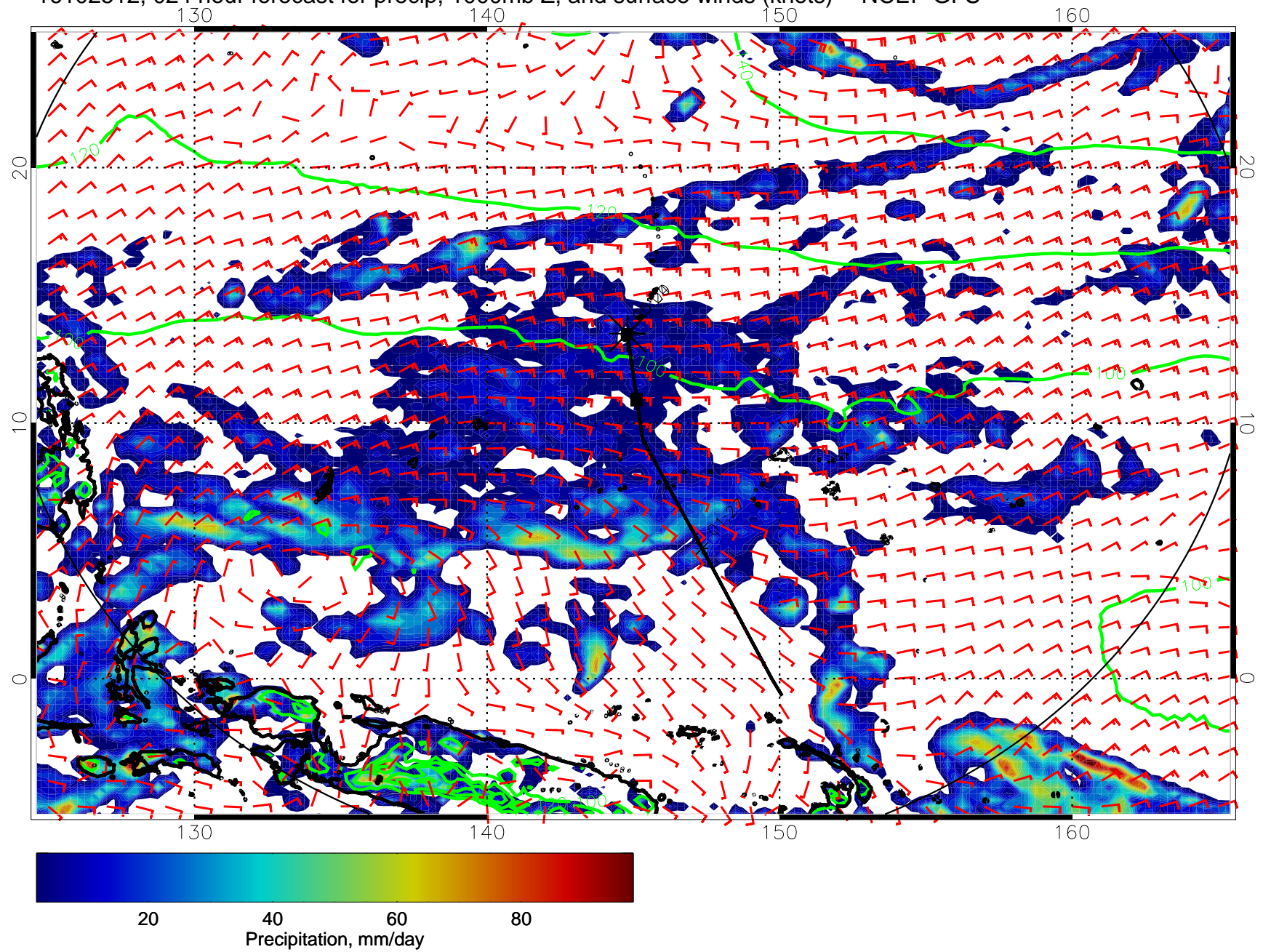
16102512, 024 hour forecast for precip, 1000mb Z, and surface winds (knots) -- NCEP GFS
