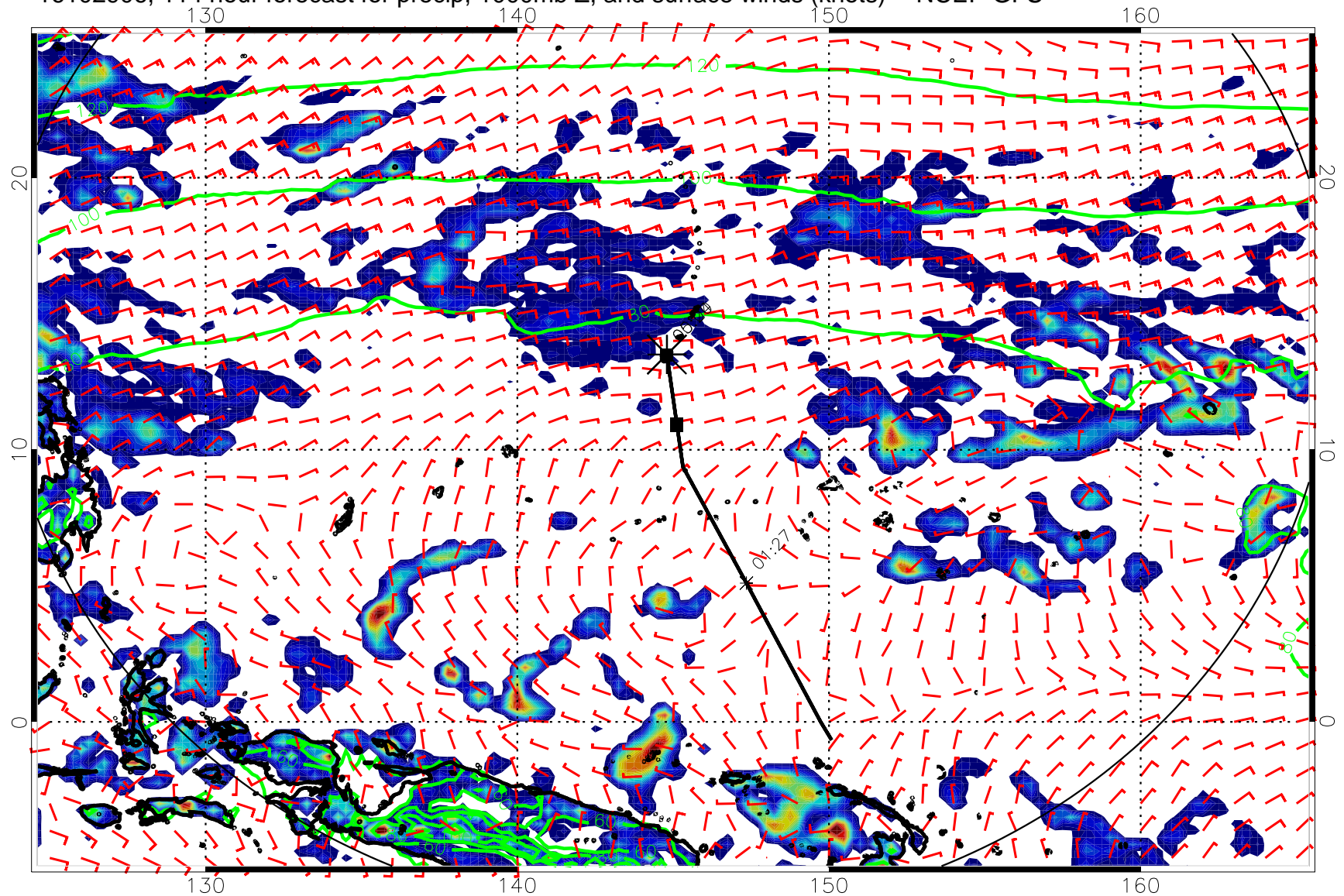
16102906, 114 hour forecast for precip, 1000mb Z, and surface winds (knots) -- NCEP GFS
