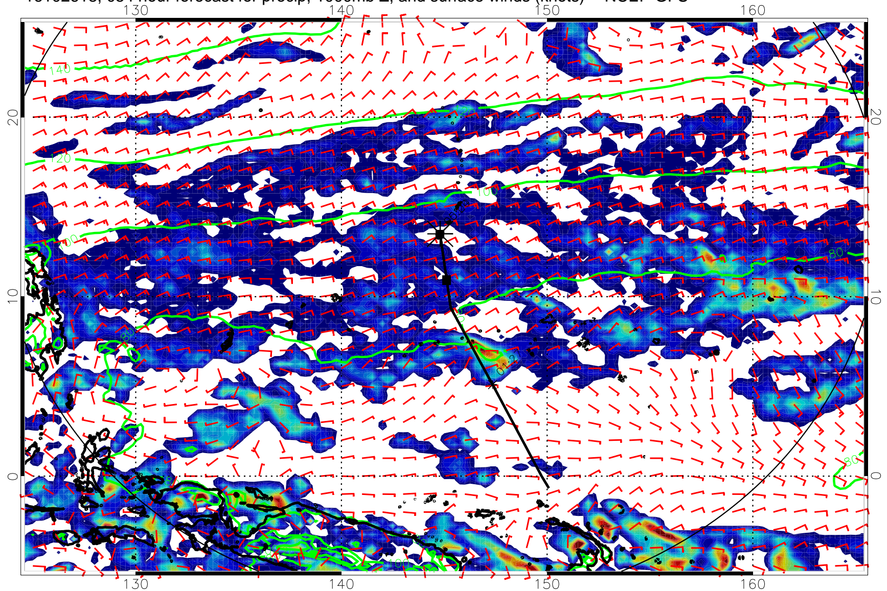
16102618, 054 hour forecast for precip, 1000mb Z, and surface winds (knots) -- NCEP GFS
