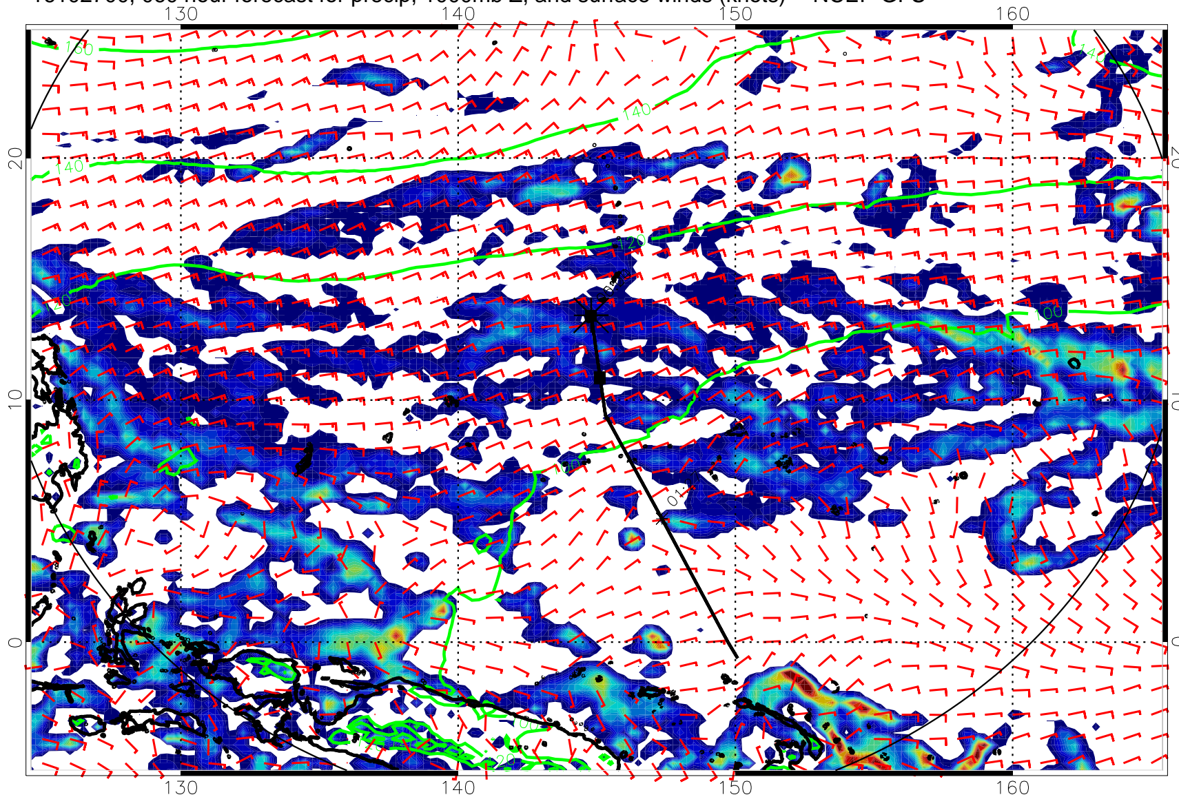
16102700, 060 hour forecast for precip, 1000mb Z, and surface winds (knots) -- NCEP GFS
