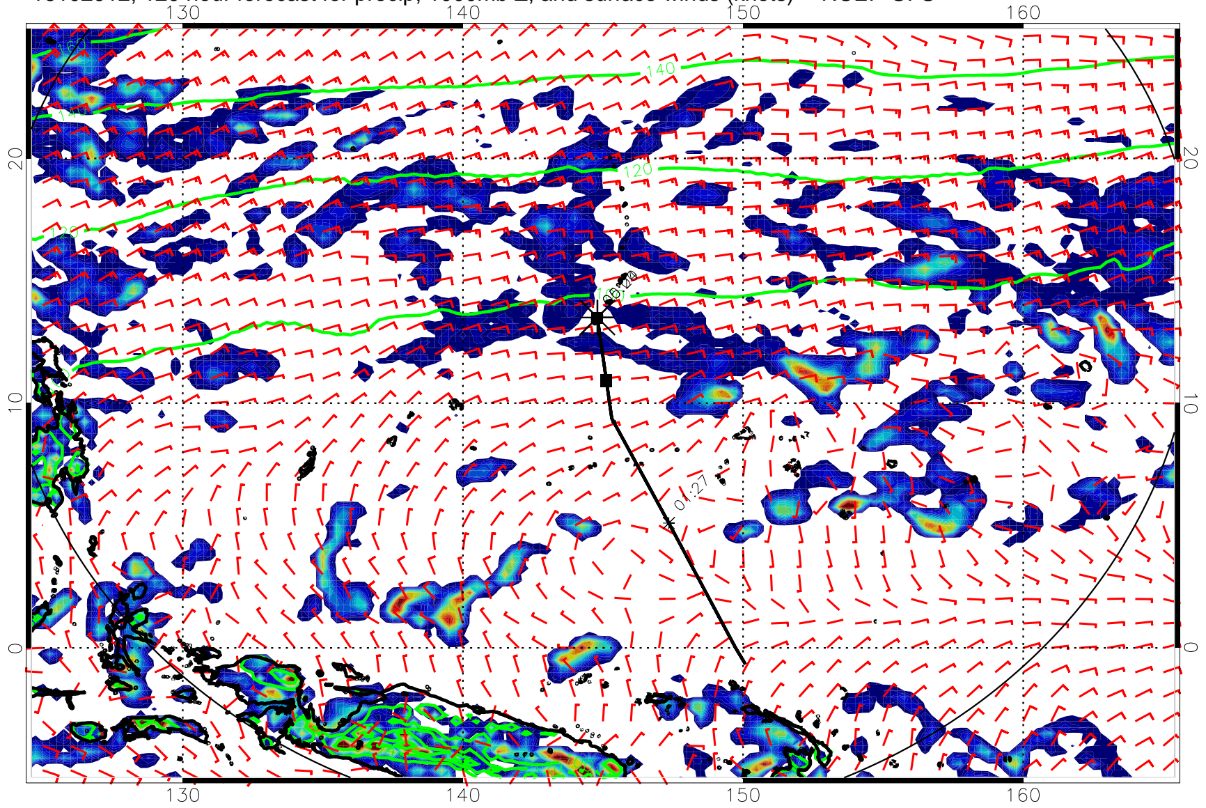
16102912, 120 hour forecast for precip, 1000mb Z, and surface winds (knots) -- NCEP GFS
