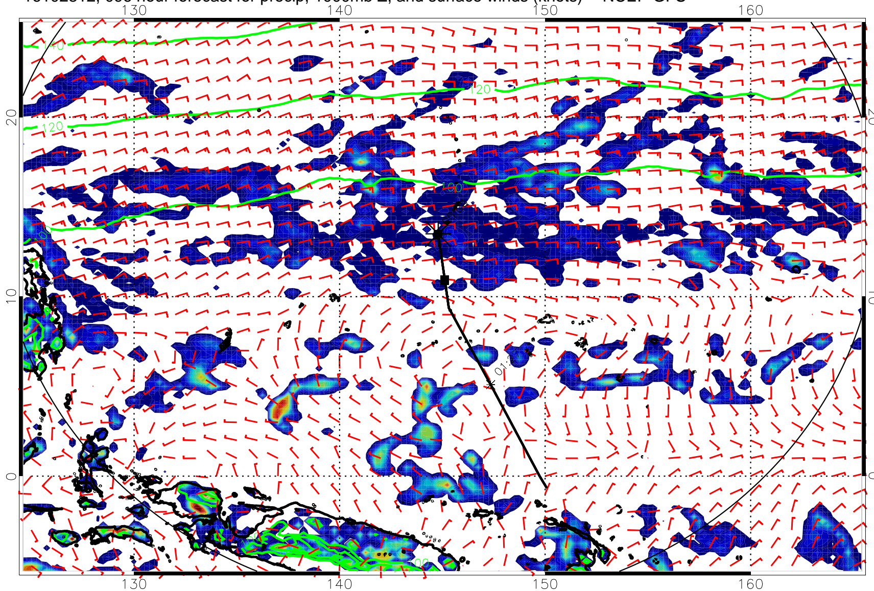
16102812, 096 hour forecast for precip, 1000mb Z, and surface winds (knots) -- NCEP GFS
