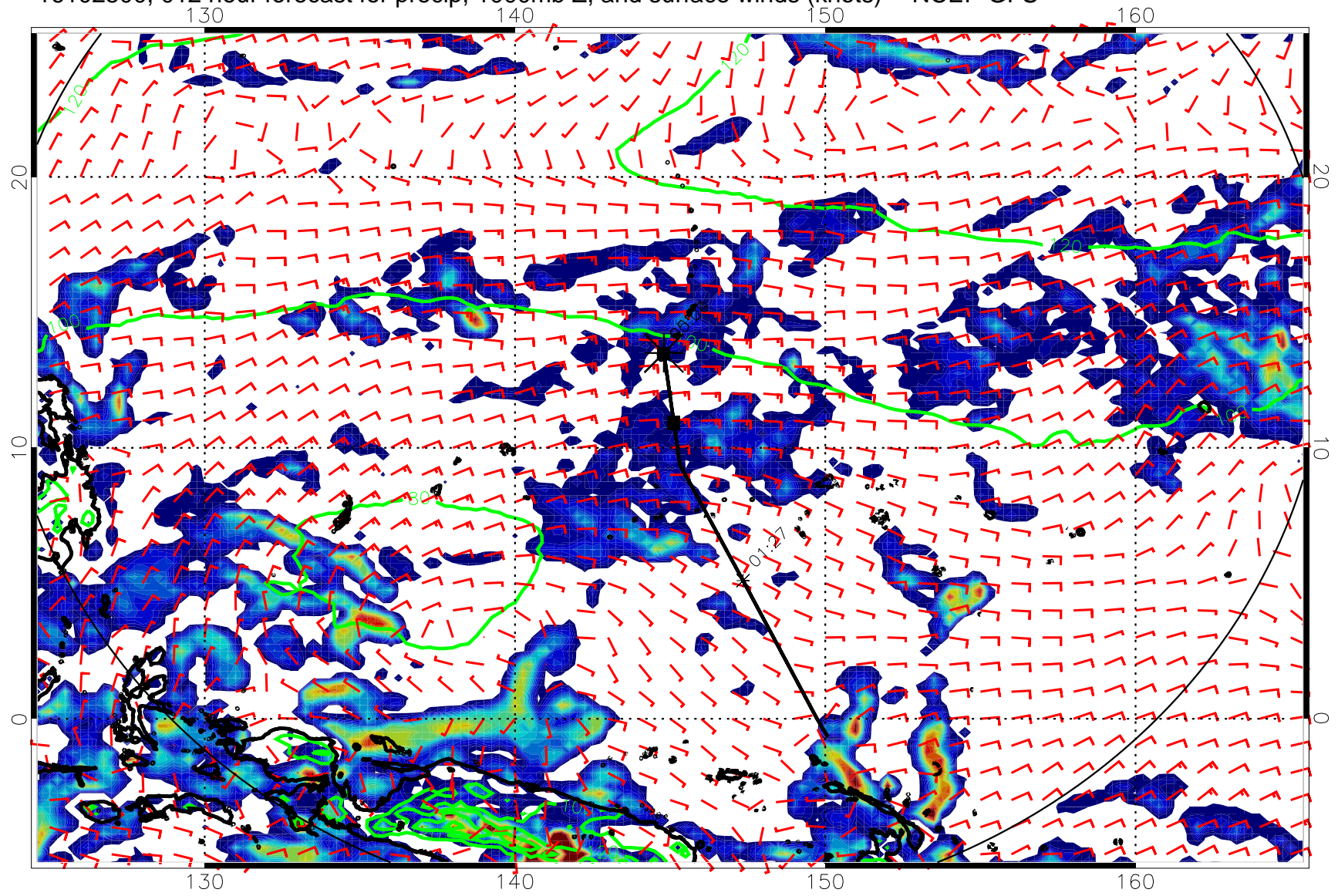
16102500, 012 hour forecast for precip, 1000mb Z, and surface winds (knots) -- NCEP GFS
