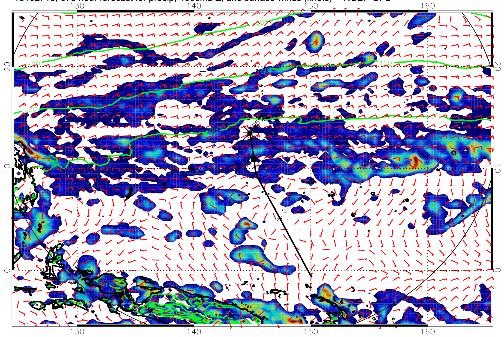
16102718, 078 hour forecast for precip, 1000mb Z, and surface winds (knots) -- NCEP GFS
