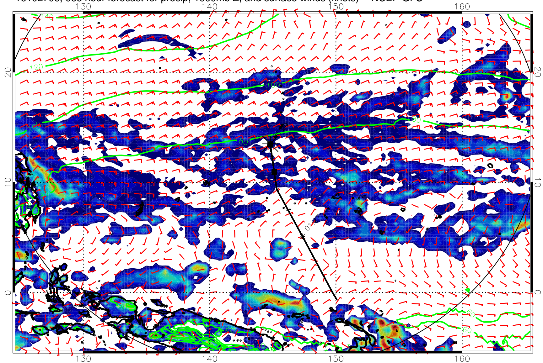
16102706, 066 hour forecast for precip, 1000mb Z, and surface winds (knots) -- NCEP GFS
