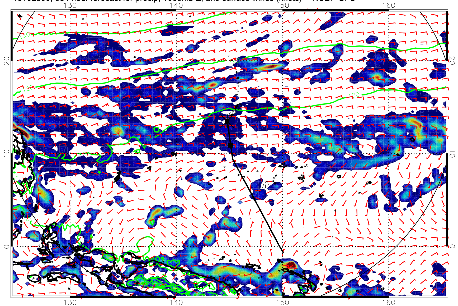
16102800, 084 hour forecast for precip, 1000mb Z, and surface winds (knots) -- NCEP GFS
