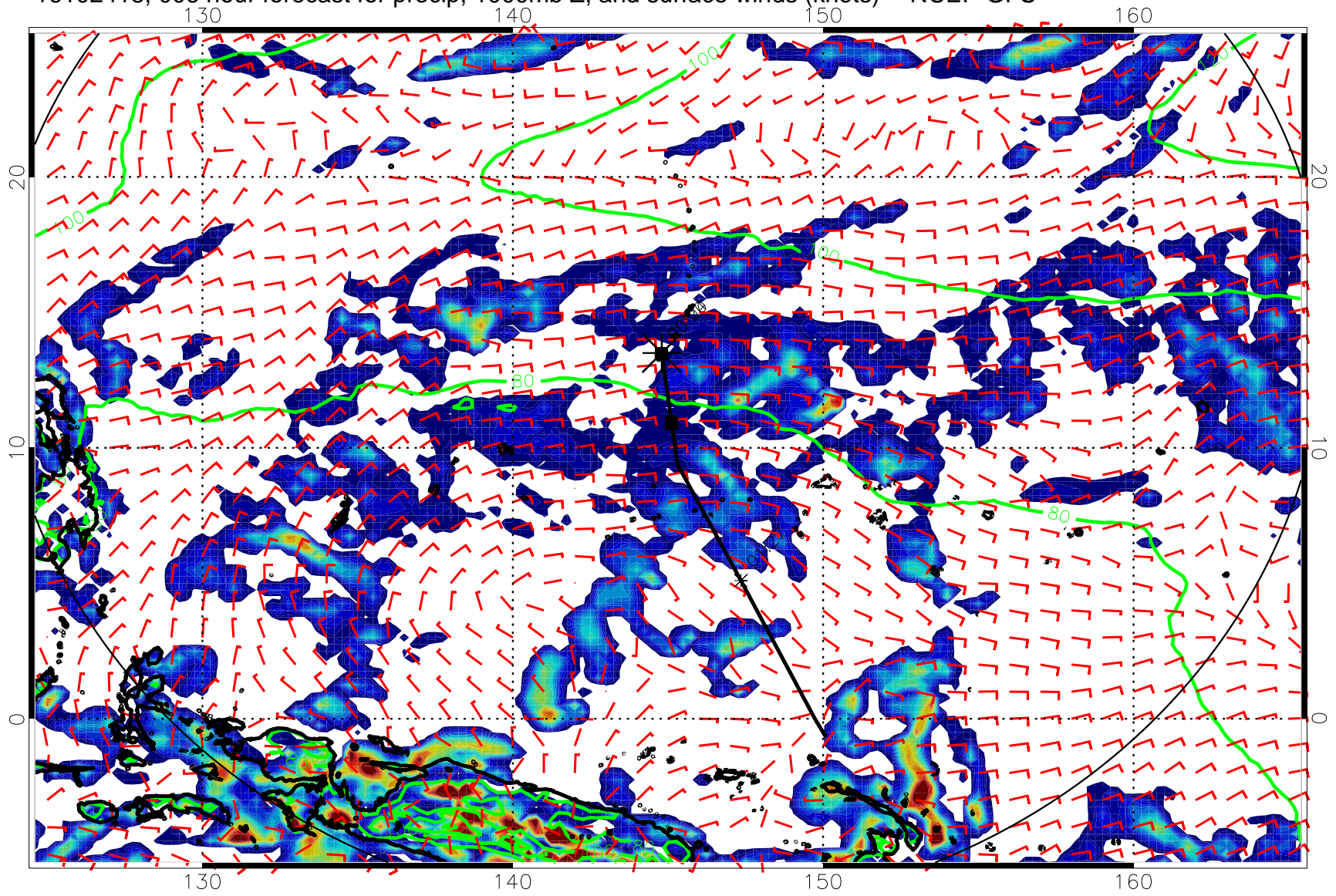
16102418, 006 hour forecast for precip, 1000mb Z, and surface winds (knots) -- NCEP GFS
