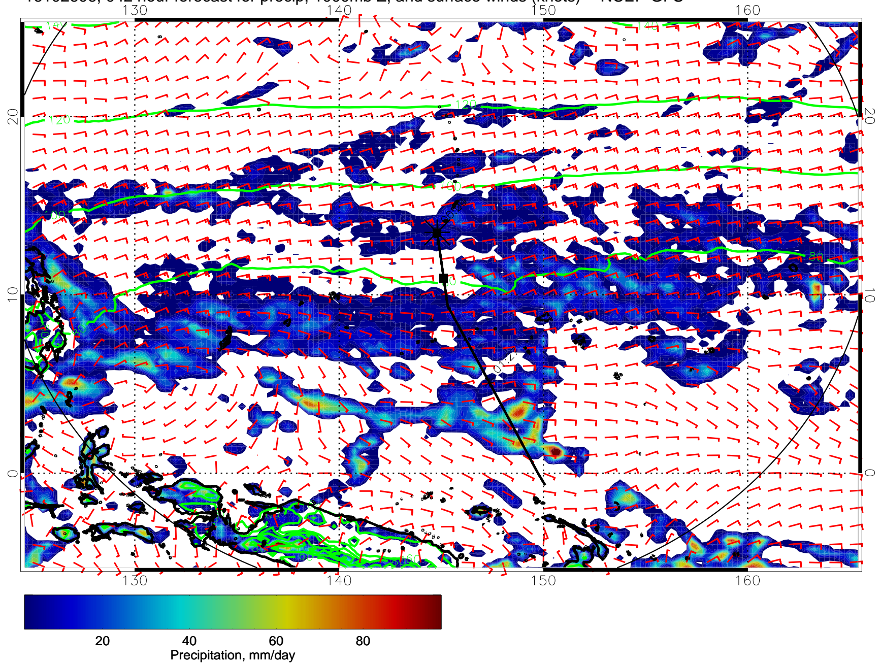
16102606, 042 hour forecast for precip, 1000mb Z, and surface winds (knots) -- NCEP GFS
