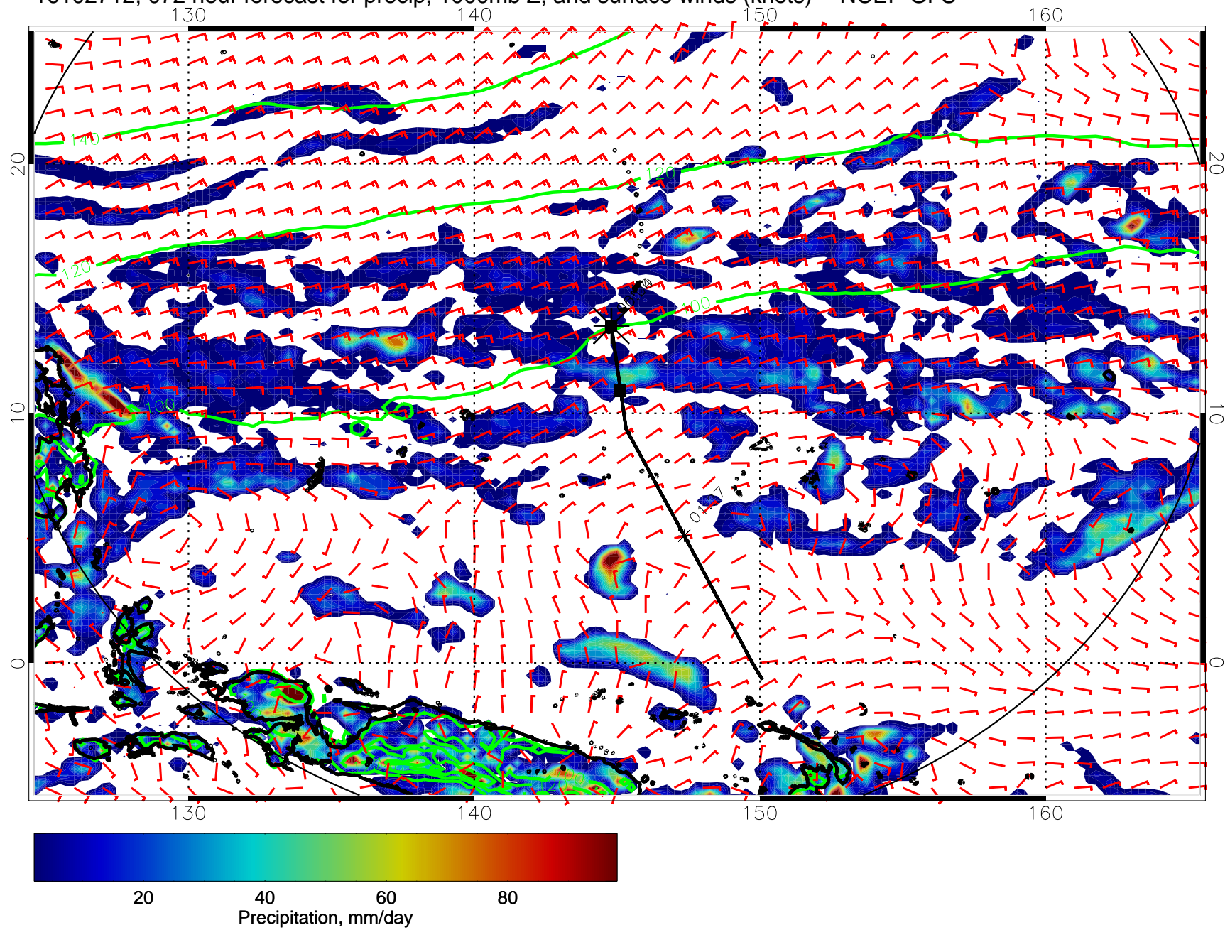
16102712, 072 hour forecast for precip, 1000mb Z, and surface winds (knots) -- NCEP GFS
