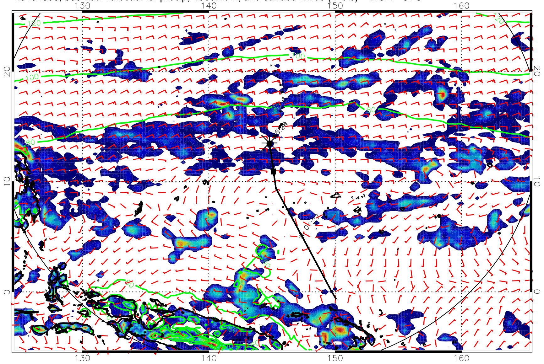
16102806, 090 hour forecast for precip, 1000mb Z, and surface winds (knots) -- NCEP GFS
