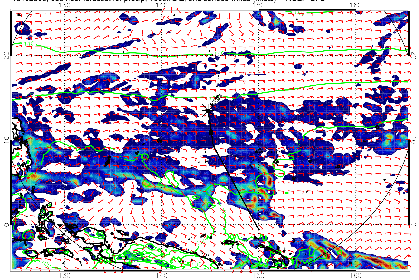
16102600, 036 hour forecast for precip, 1000mb Z, and surface winds (knots) -- NCEP GFS
