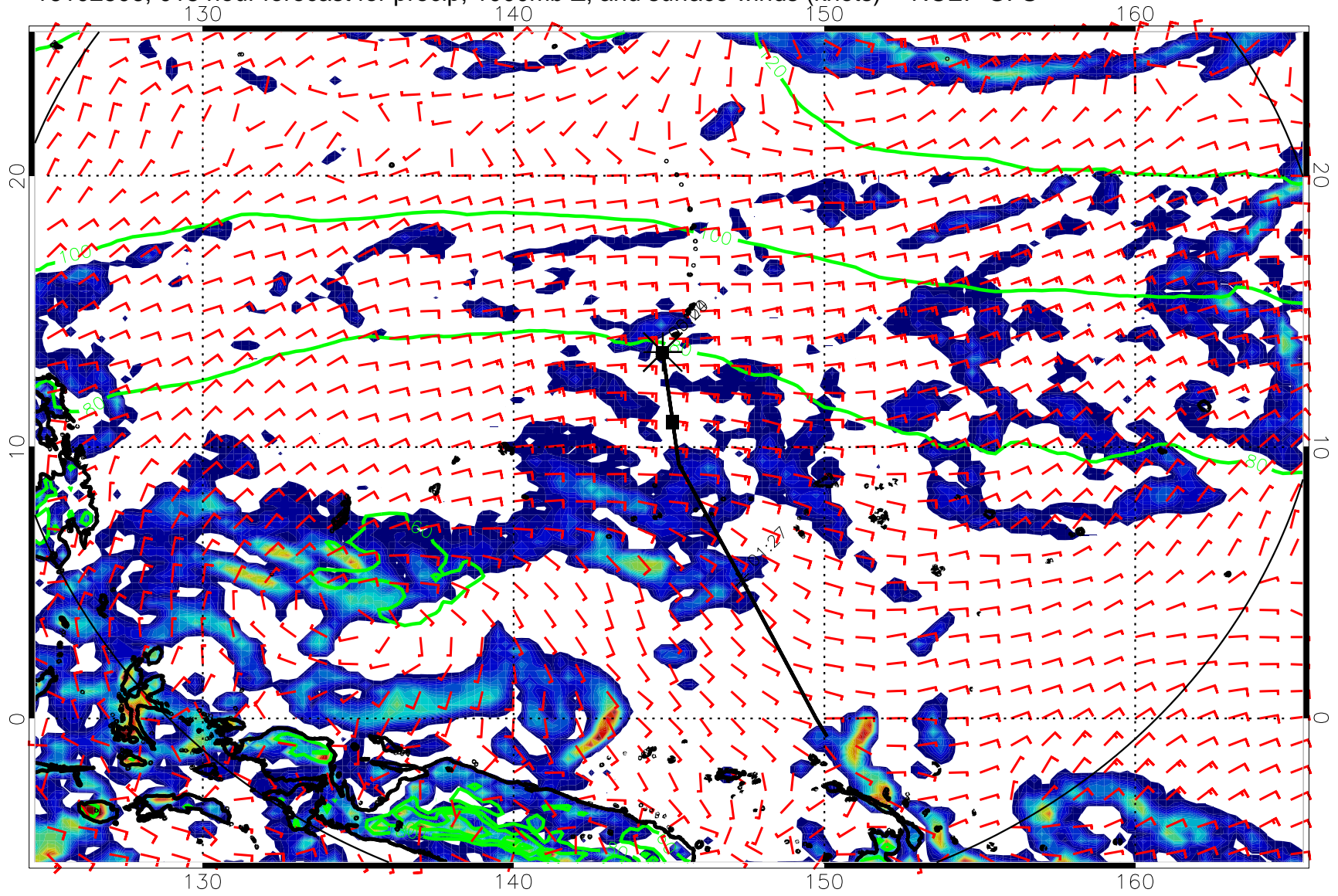
16102506, 018 hour forecast for precip, 1000mb Z, and surface winds (knots) -- NCEP GFS
