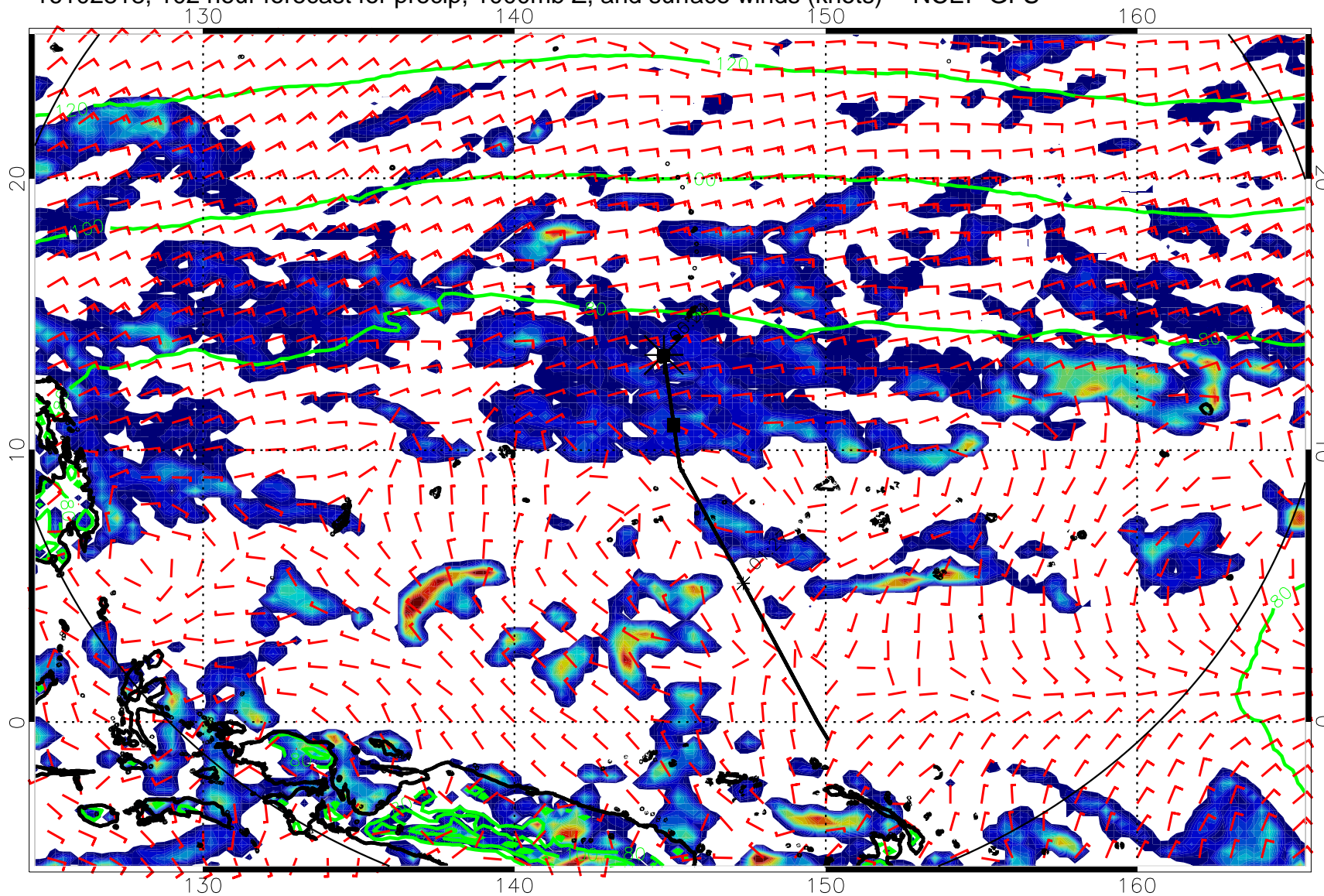
16102818, 102 hour forecast for precip, 1000mb Z, and surface winds (knots) -- NCEP GFS
