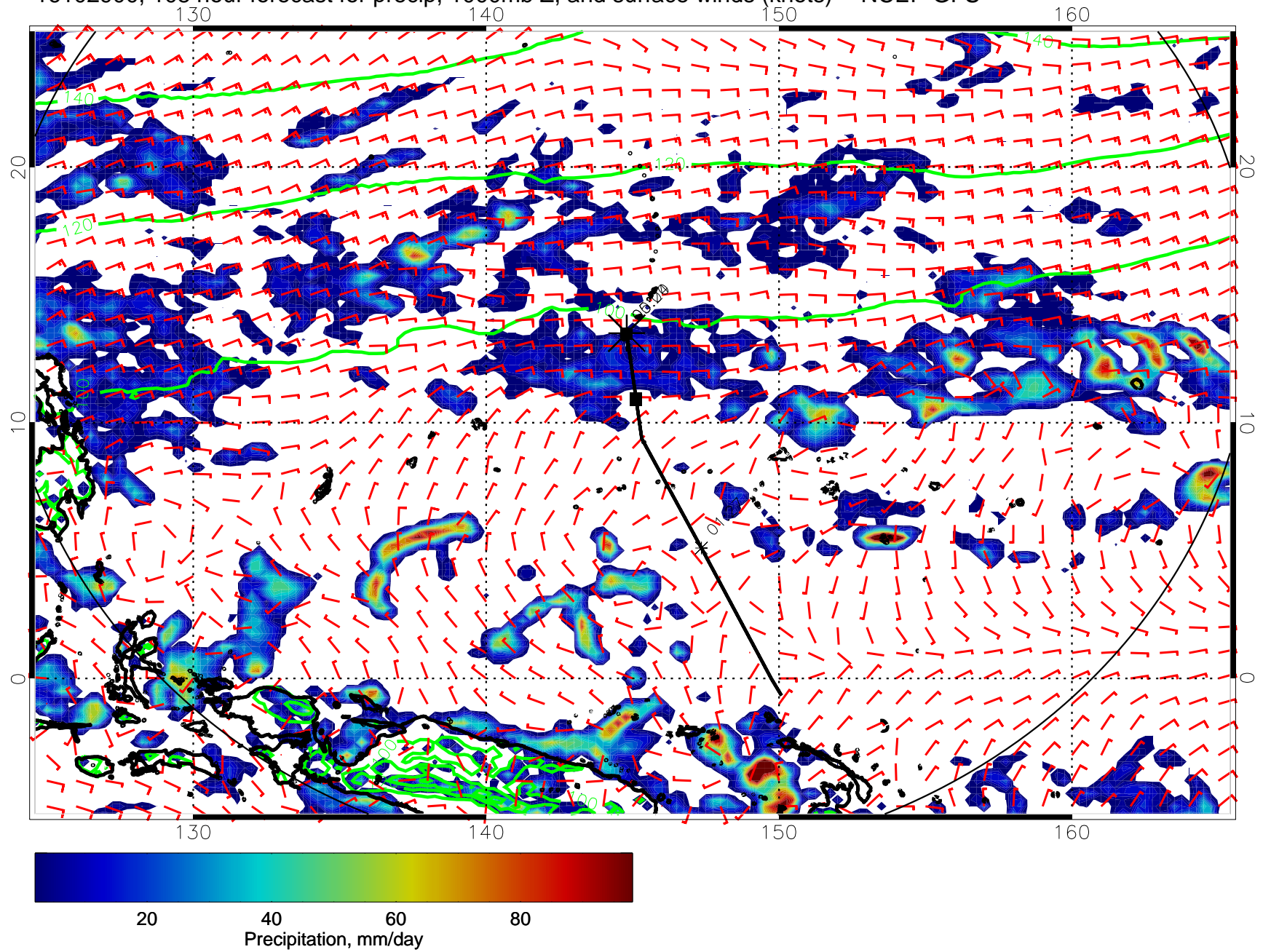
16102900, 108 hour forecast for precip, 1000mb Z, and surface winds (knots) -- NCEP GFS
