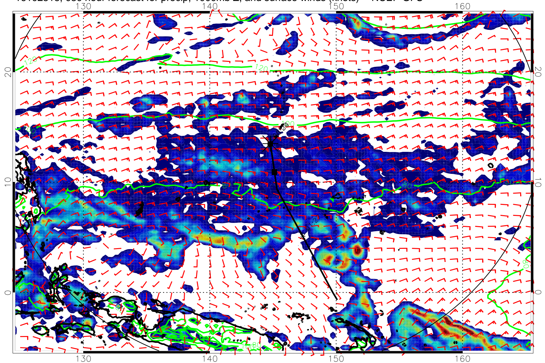
16102518, 030 hour forecast for precip, 1000mb Z, and surface winds (knots) -- NCEP GFS
