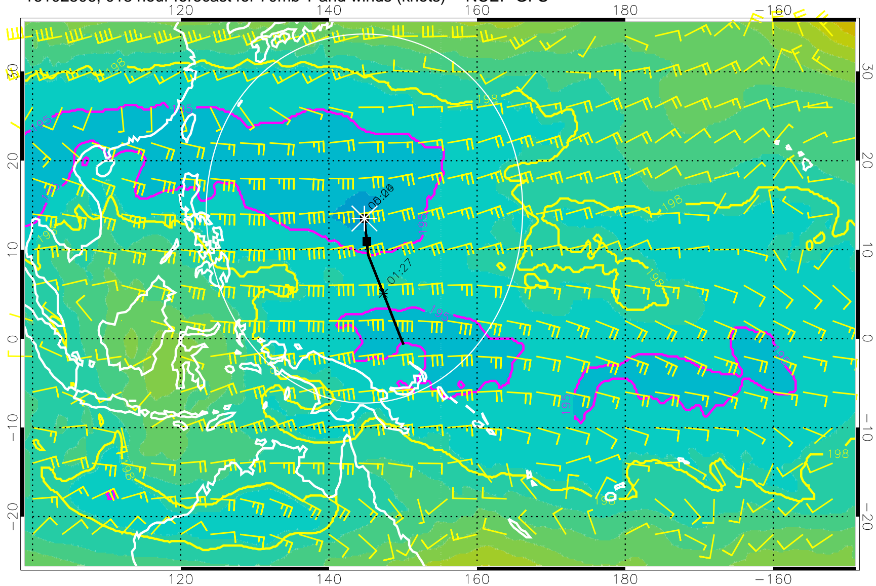
16102506, 018 hour forecast for 70mb T and winds (knots) -- NCEP GFS
