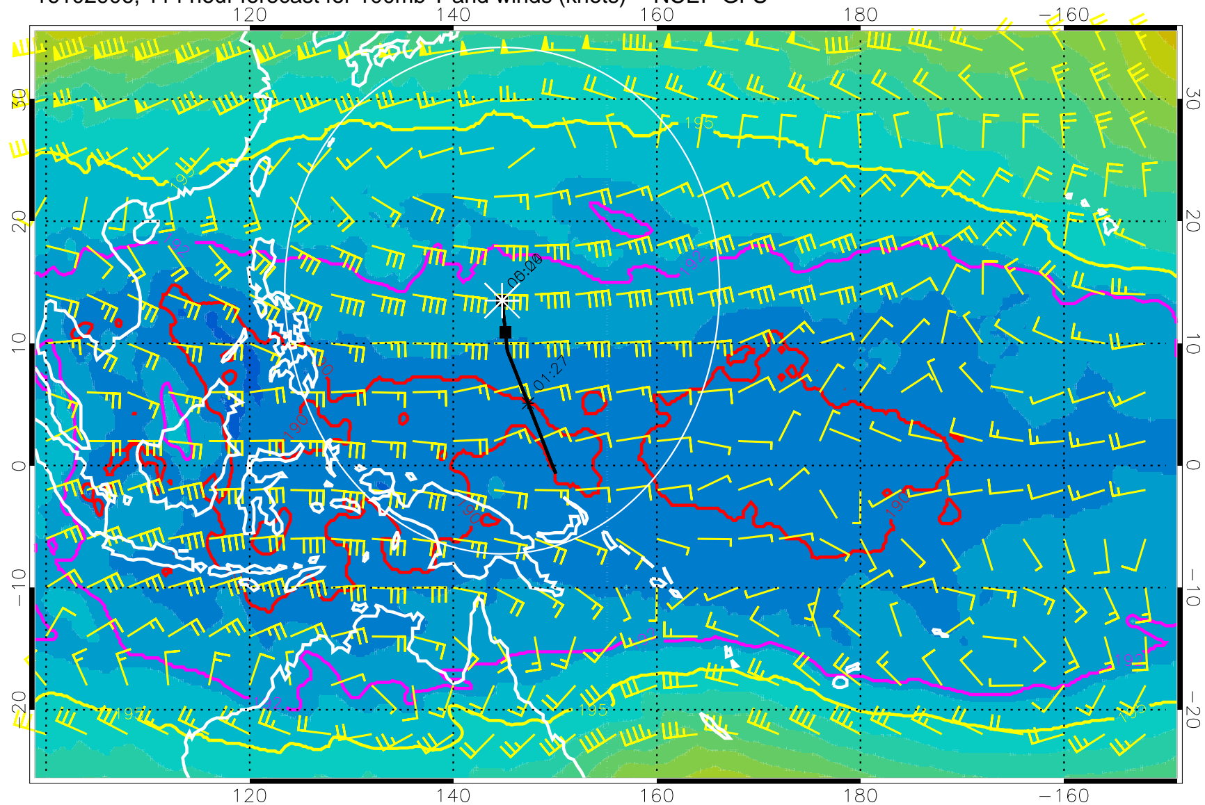
16102906, 114 hour forecast for 100mb T and winds (knots) -- NCEP GFS
