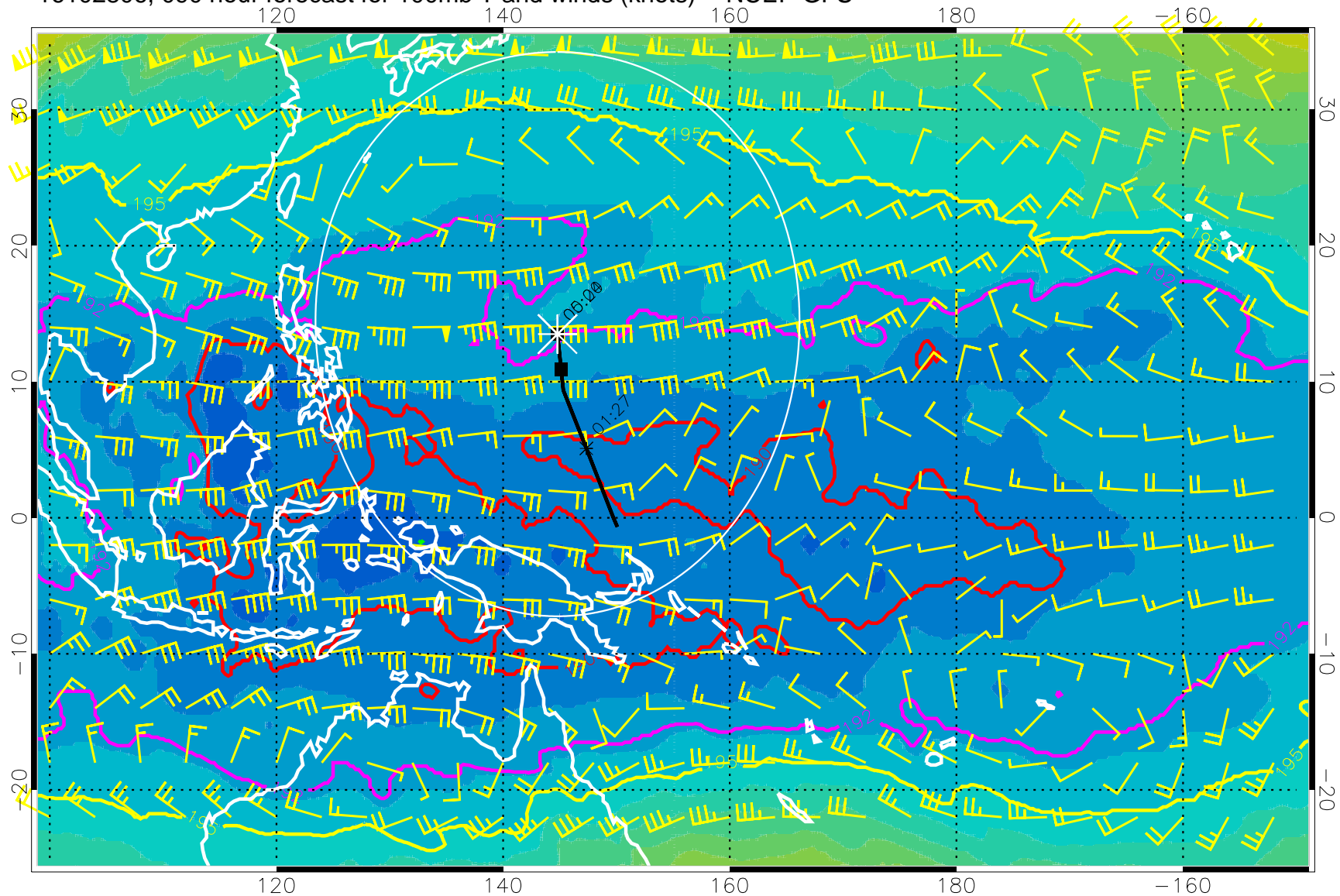
16102806, 090 hour forecast for 100mb T and winds (knots) -- NCEP GFS
