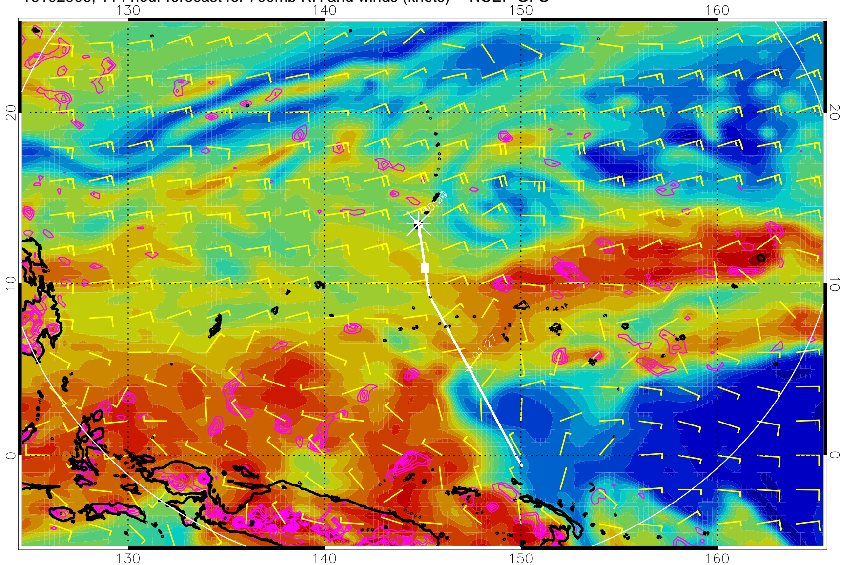
16102906, 114 hour forecast for 700mb RH and winds (knots) -- NCEP GFS
