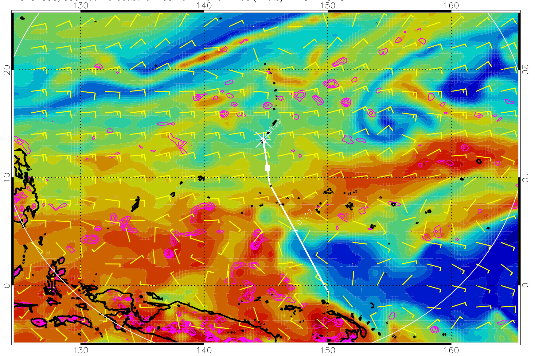
16102806, 090 hour forecast for 700mb RH and winds (knots) -- NCEP GFS
