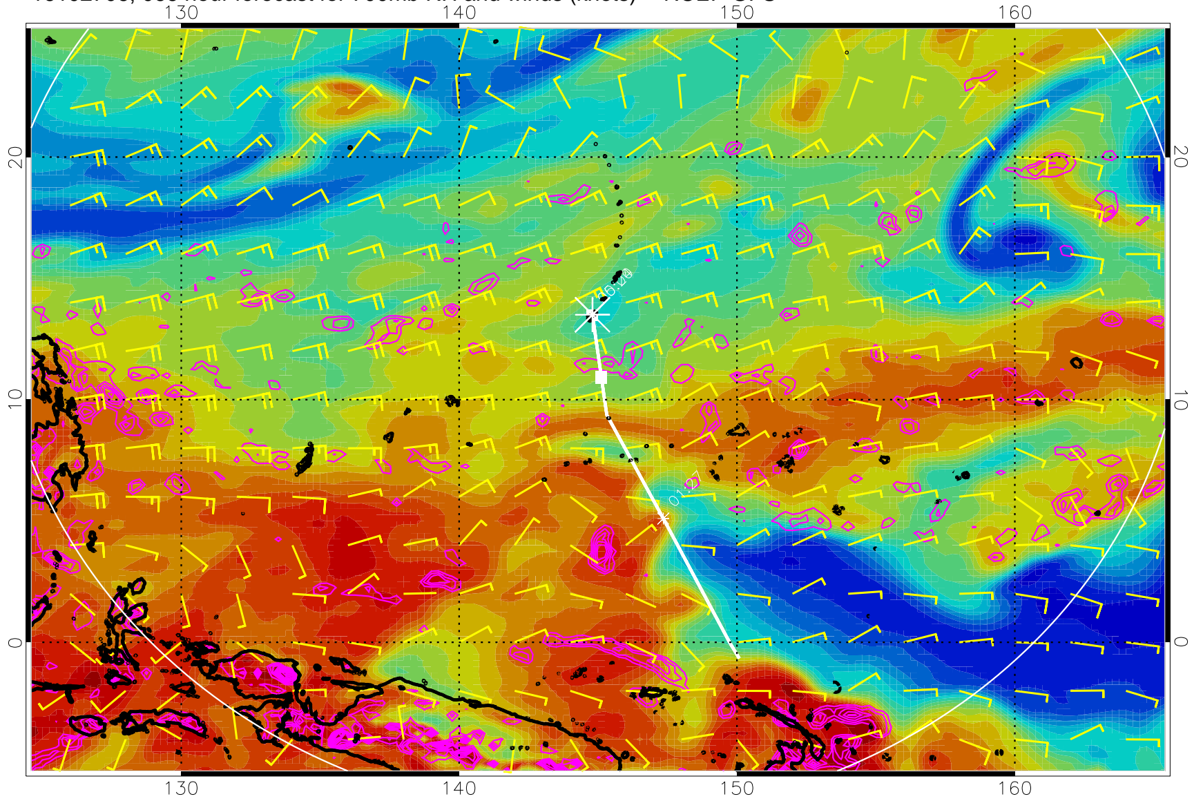
16102706, 066 hour forecast for 700mb RH and winds (knots) -- NCEP GFS
