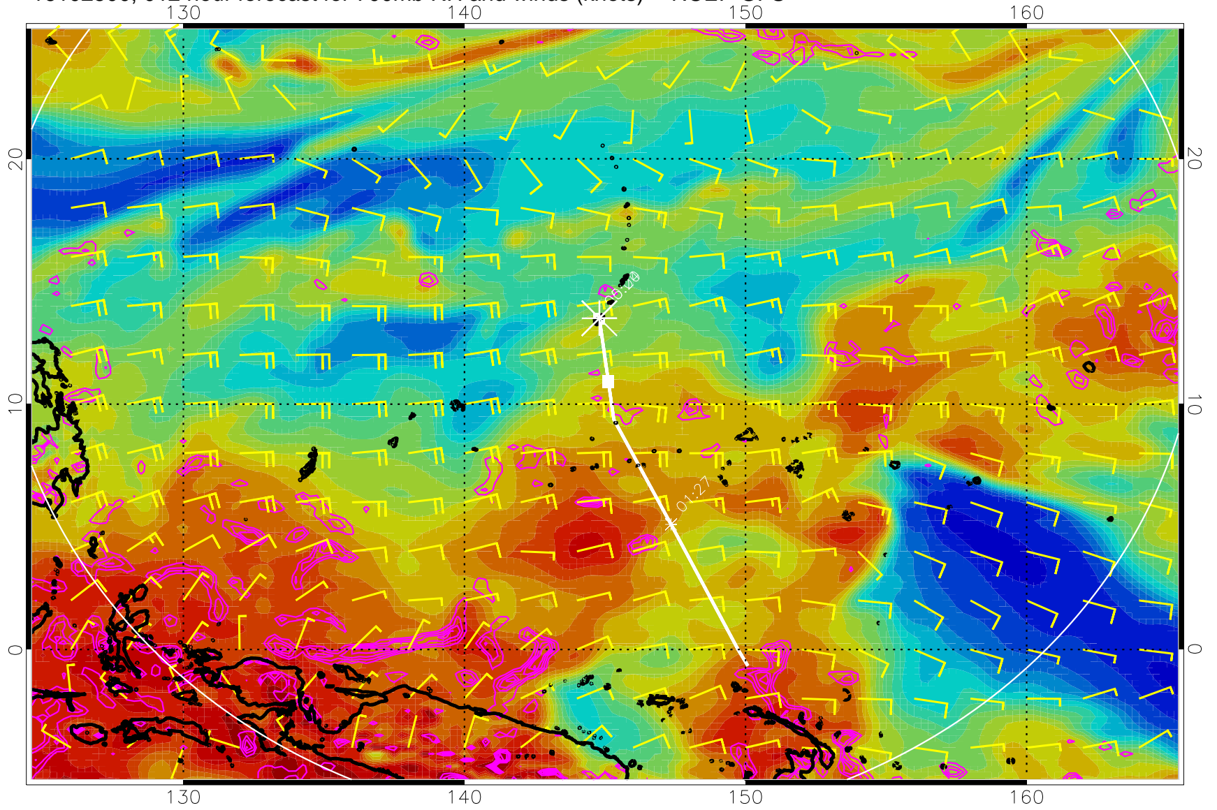
16102500, 012 hour forecast for 700mb RH and winds (knots) -- NCEP GFS
