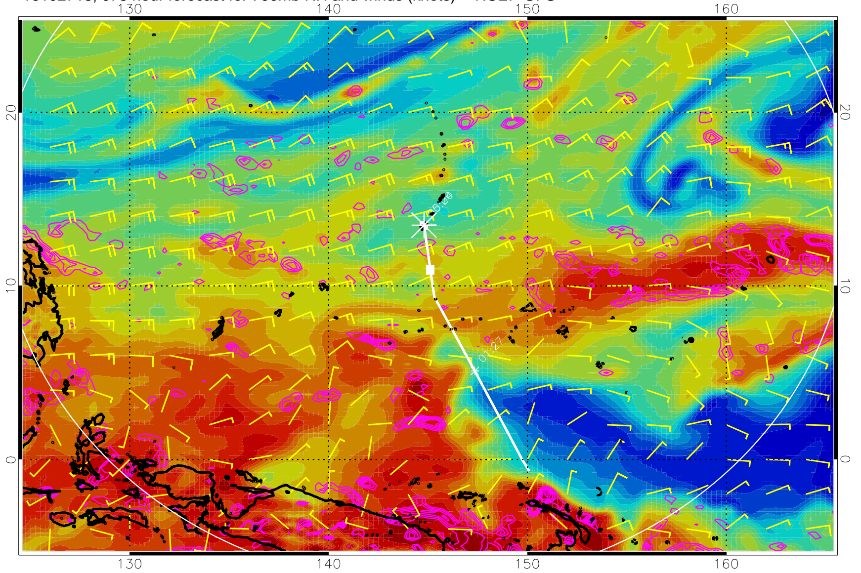
16102718, 078 hour forecast for 700mb RH and winds (knots) -- NCEP GFS
