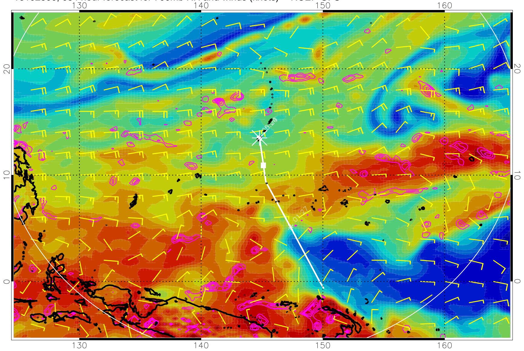
16102800, 084 hour forecast for 700mb RH and winds (knots) -- NCEP GFS
