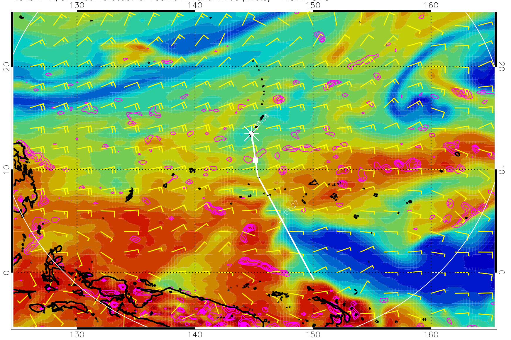
16102712, 072 hour forecast for 700mb RH and winds (knots) -- NCEP GFS
