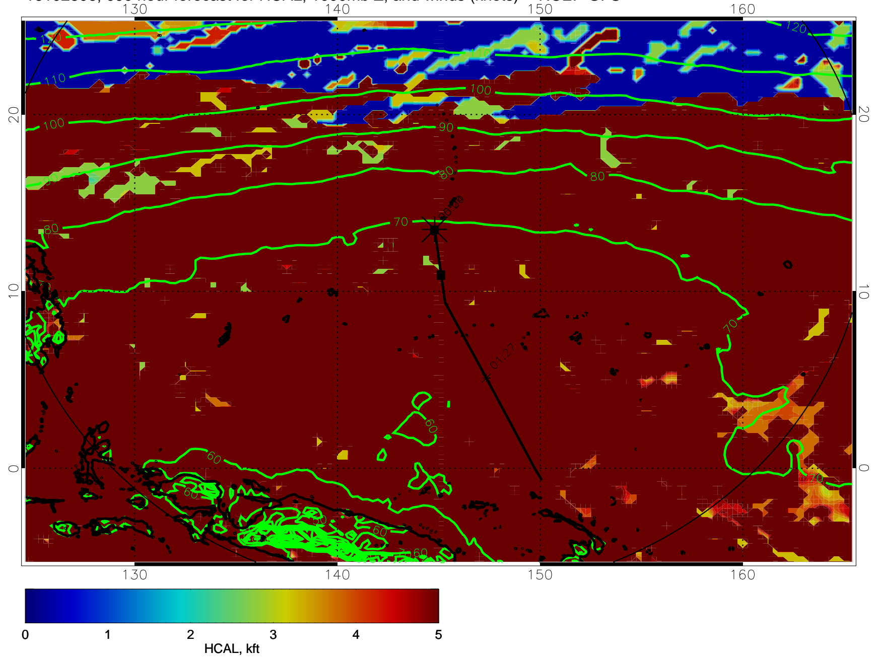
16102806, 090 hour forecast for HCAL, 1000mb Z, and winds (knots) -- NCEP GFS
