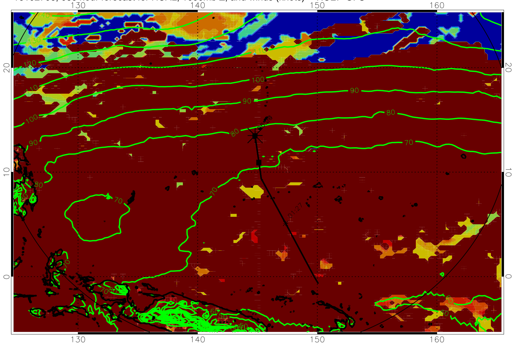
16102706, 066 hour forecast for HCAL, 1000mb Z, and winds (knots) -- NCEP GFS
