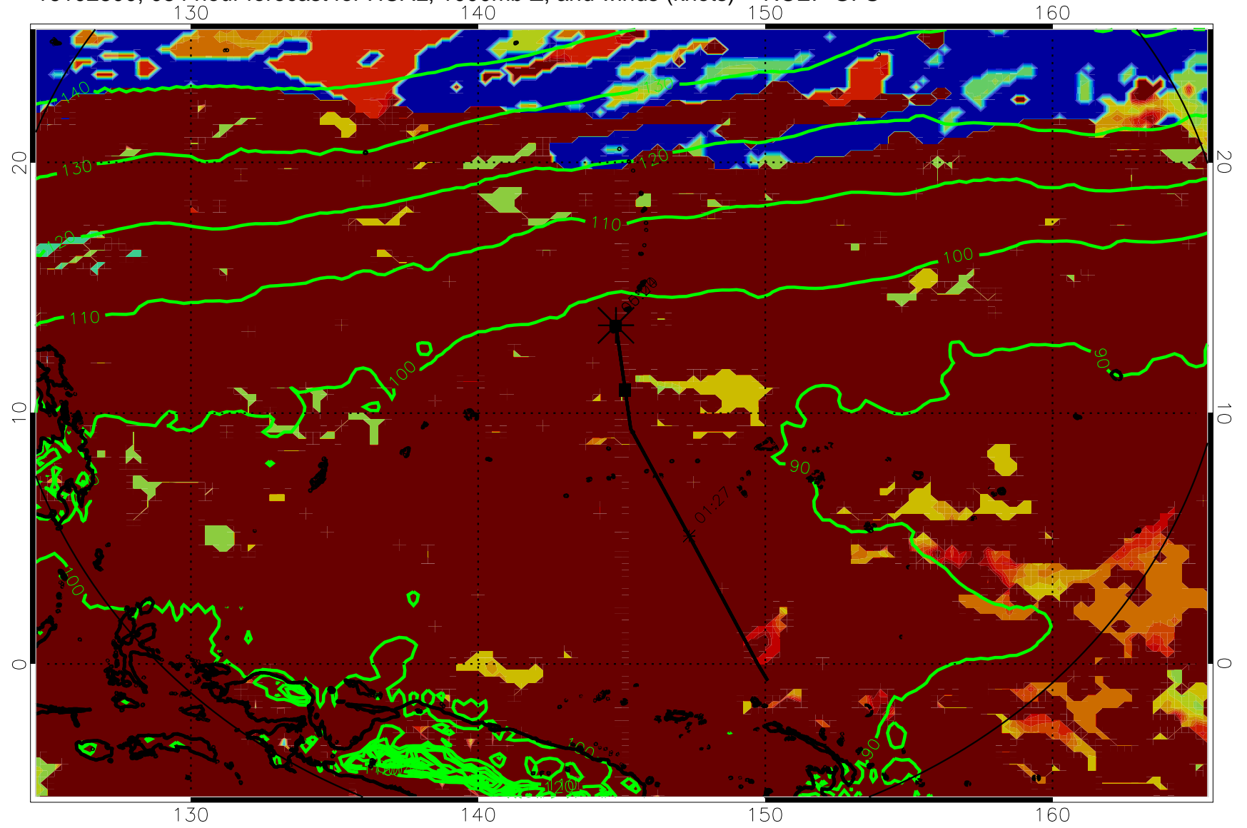
16102800, 084 hour forecast for HCAL, 1000mb Z, and winds (knots) -- NCEP GFS
