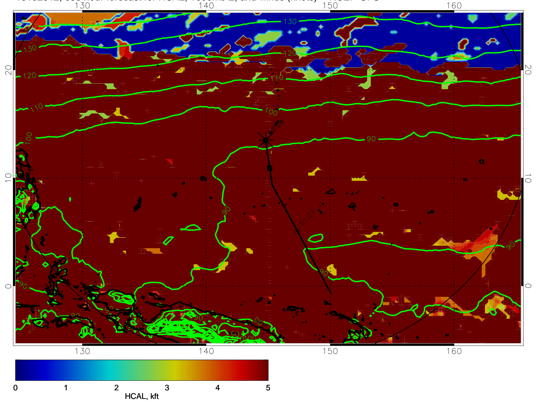
16102812, 096 hour forecast for HCAL, 1000mb Z, and winds (knots) -- NCEP GFS
