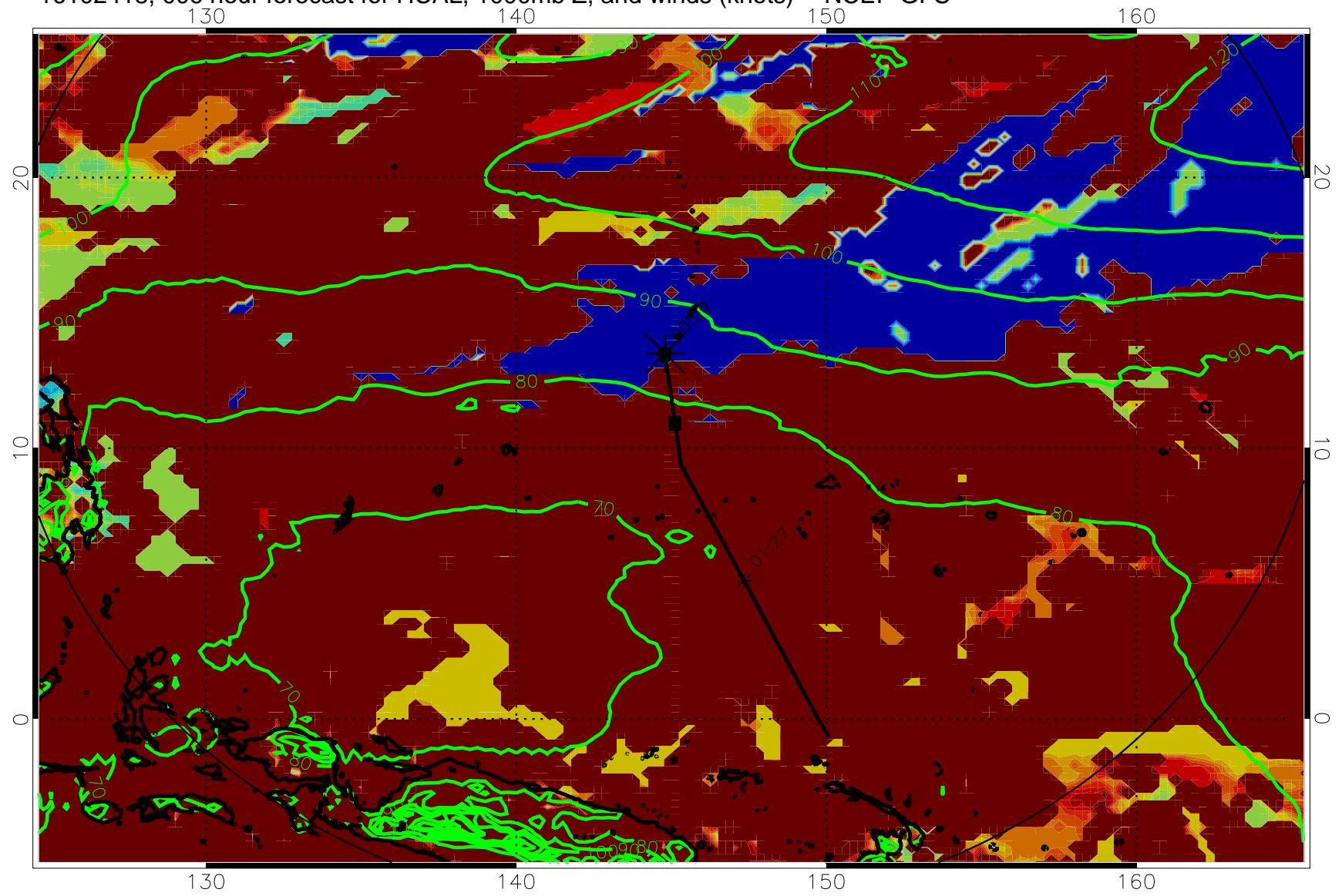
16102418, 006 hour forecast for HCAL, 1000mb Z, and winds (knots) -- NCEP GFS
