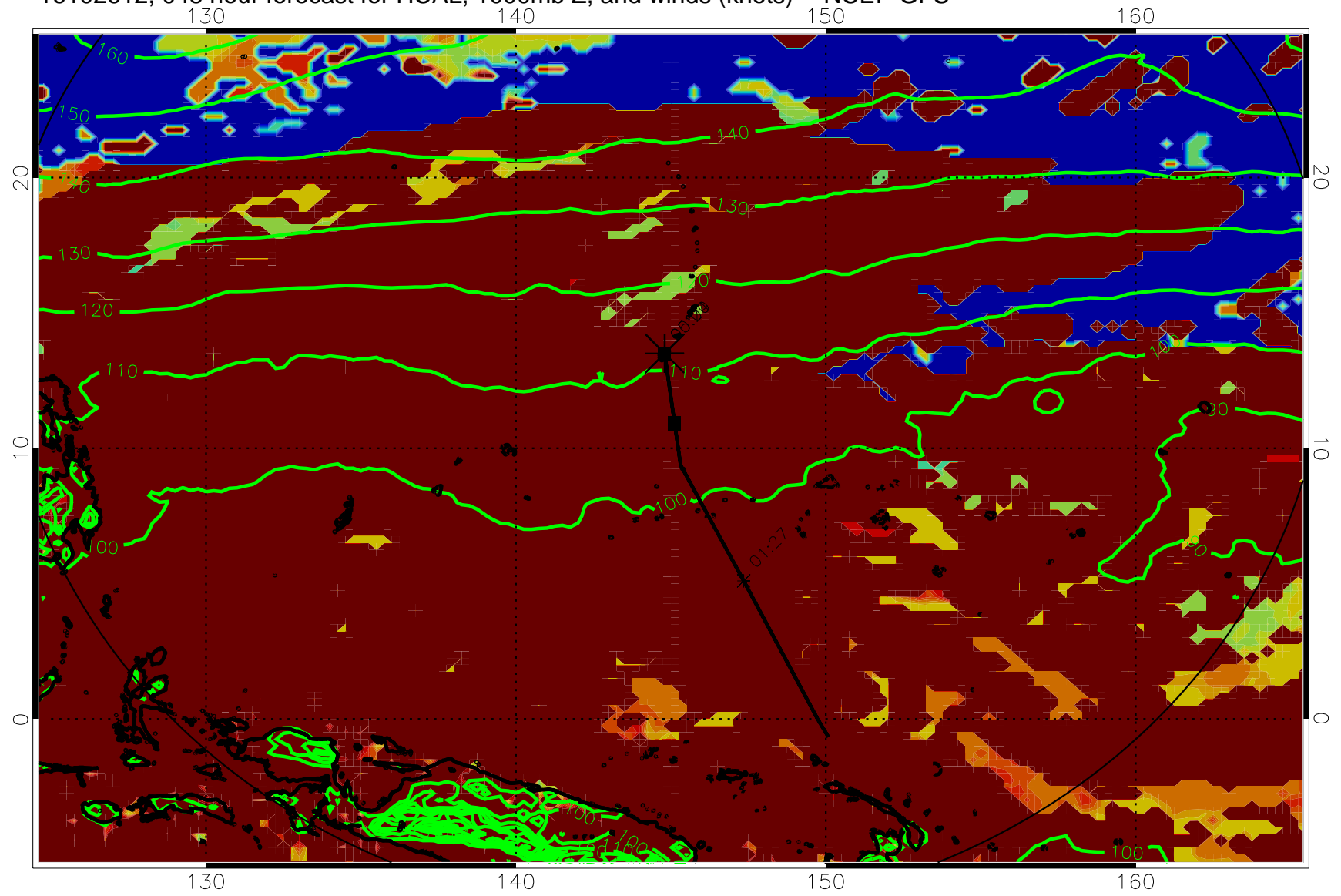
16102612, 048 hour forecast for HCAL, 1000mb Z, and winds (knots) -- NCEP GFS
