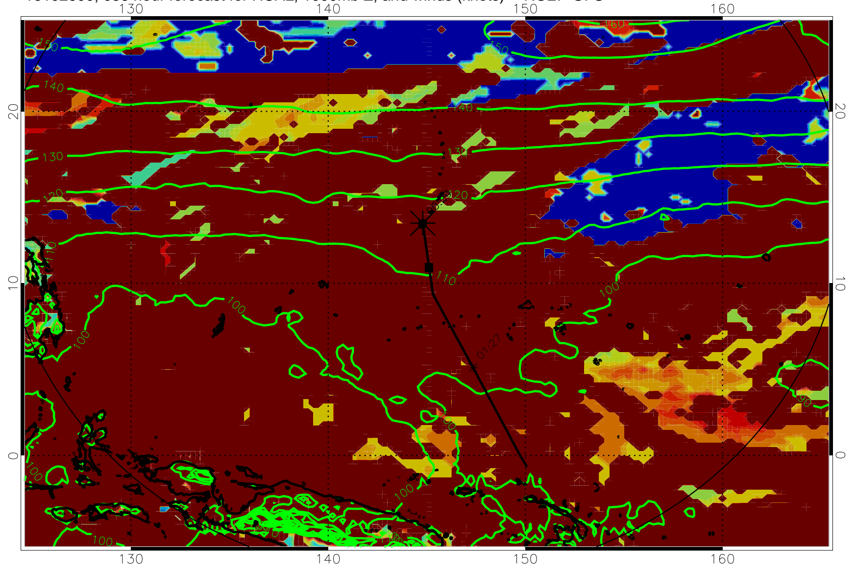
16102600, 036 hour forecast for HCAL, 1000mb Z, and winds (knots) -- NCEP GFS
