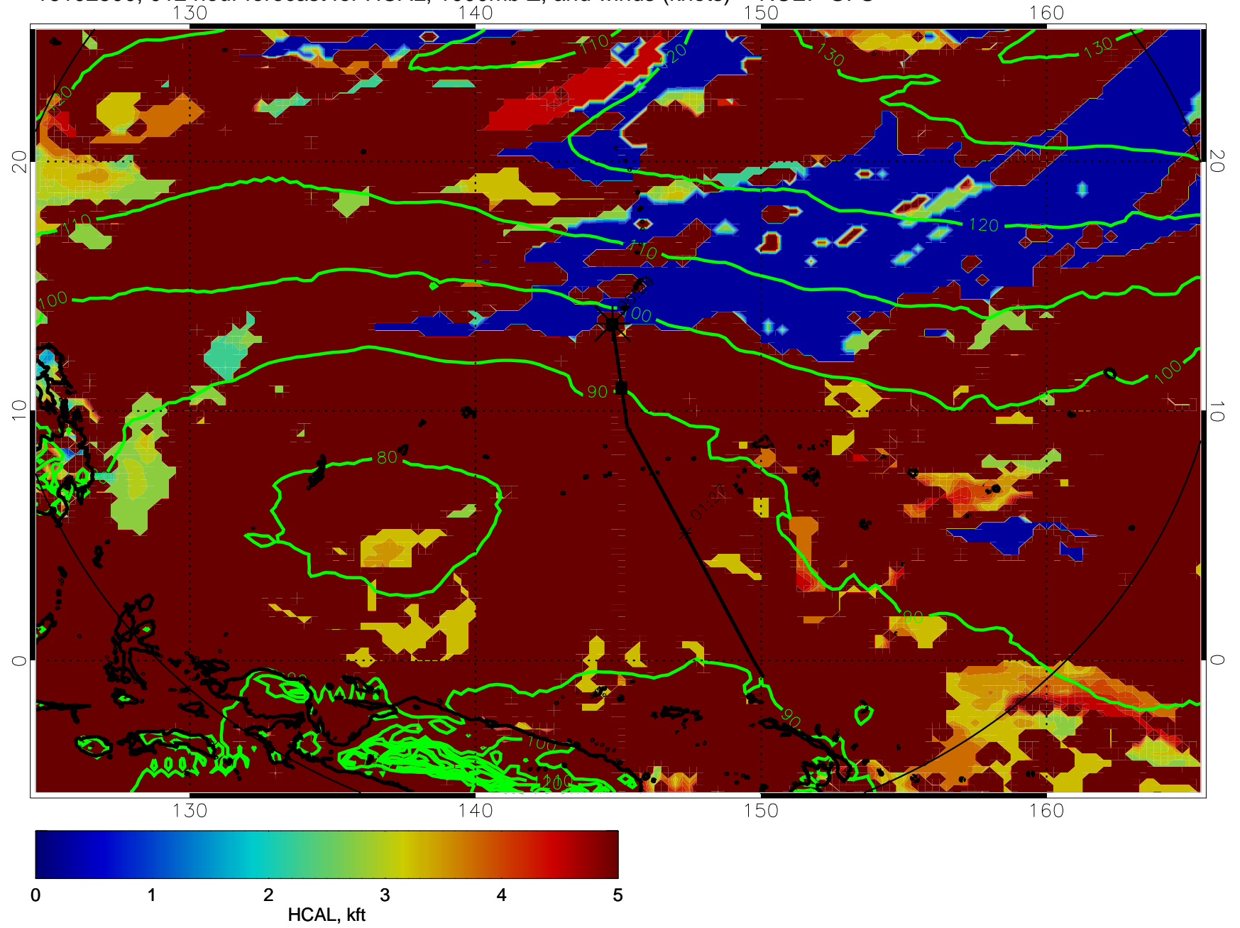
16102500, 012 hour forecast for HCAL, 1000mb Z, and winds (knots) -- NCEP GFS
