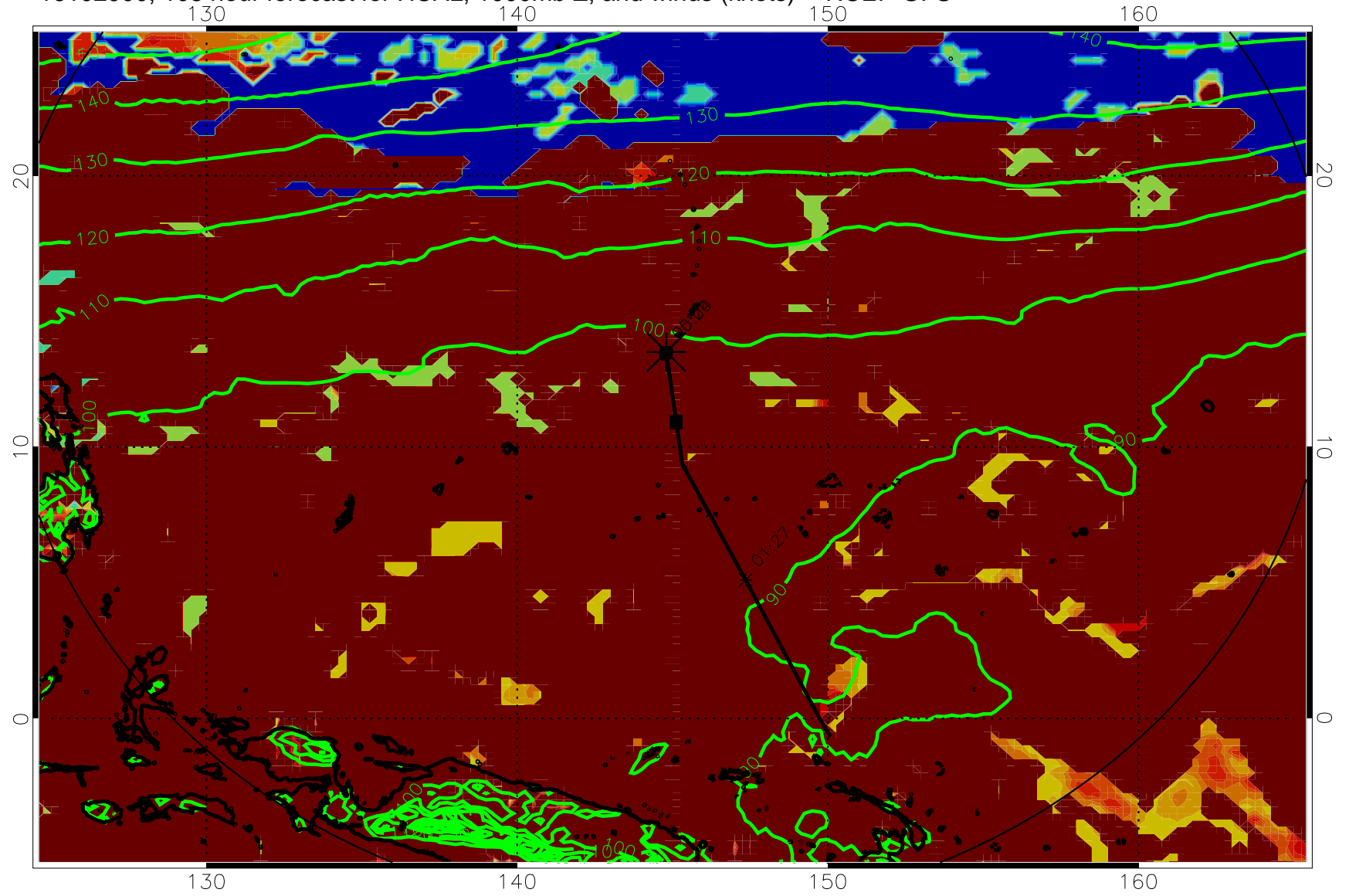
16102900, 108 hour forecast for HCAL, 1000mb Z, and winds (knots) -- NCEP GFS
