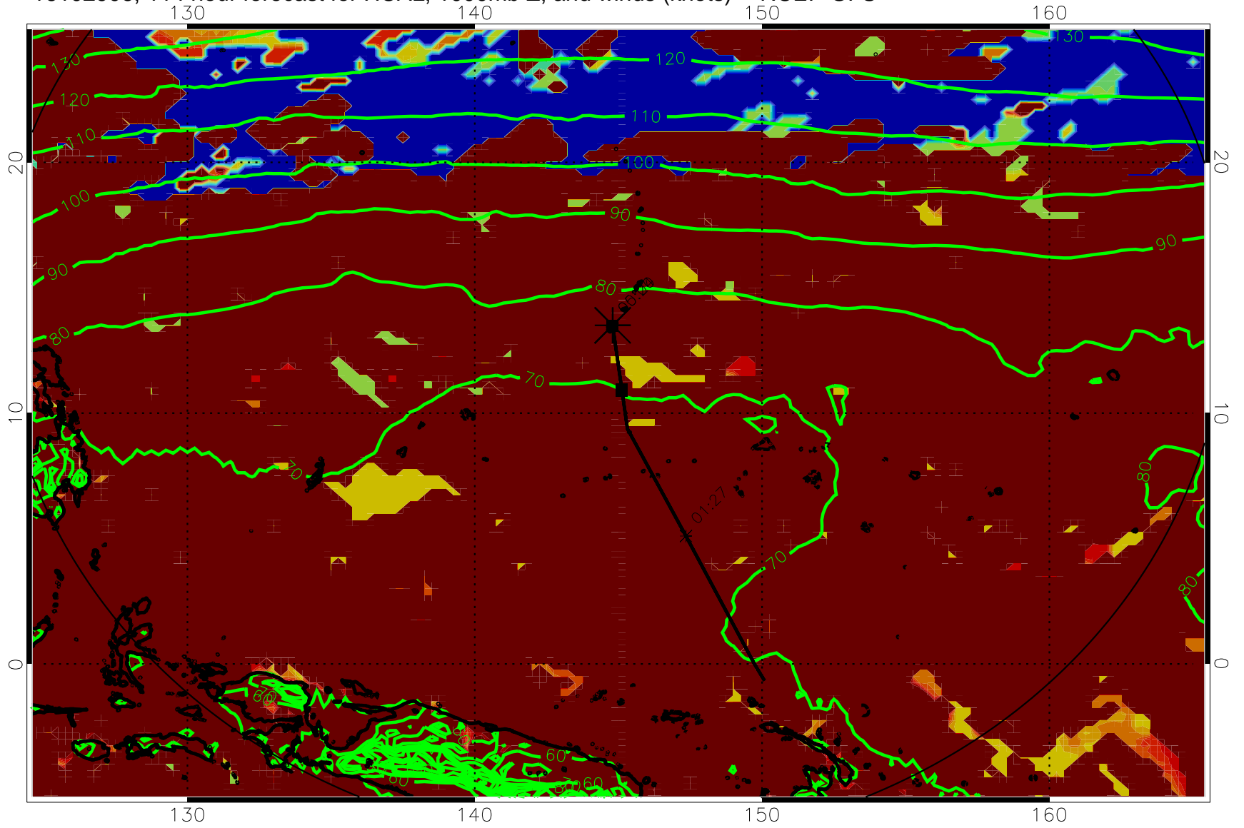
16102906, 114 hour forecast for HCAL, 1000mb Z, and winds (knots) -- NCEP GFS
