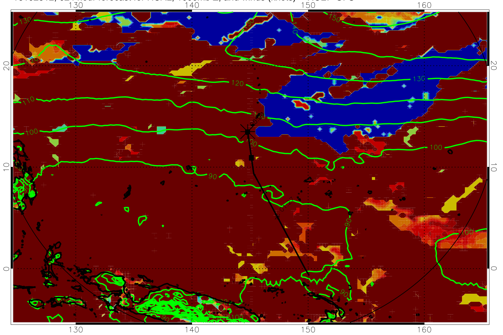
16102512, 024 hour forecast for HCAL, 1000mb Z, and winds (knots) -- NCEP GFS
