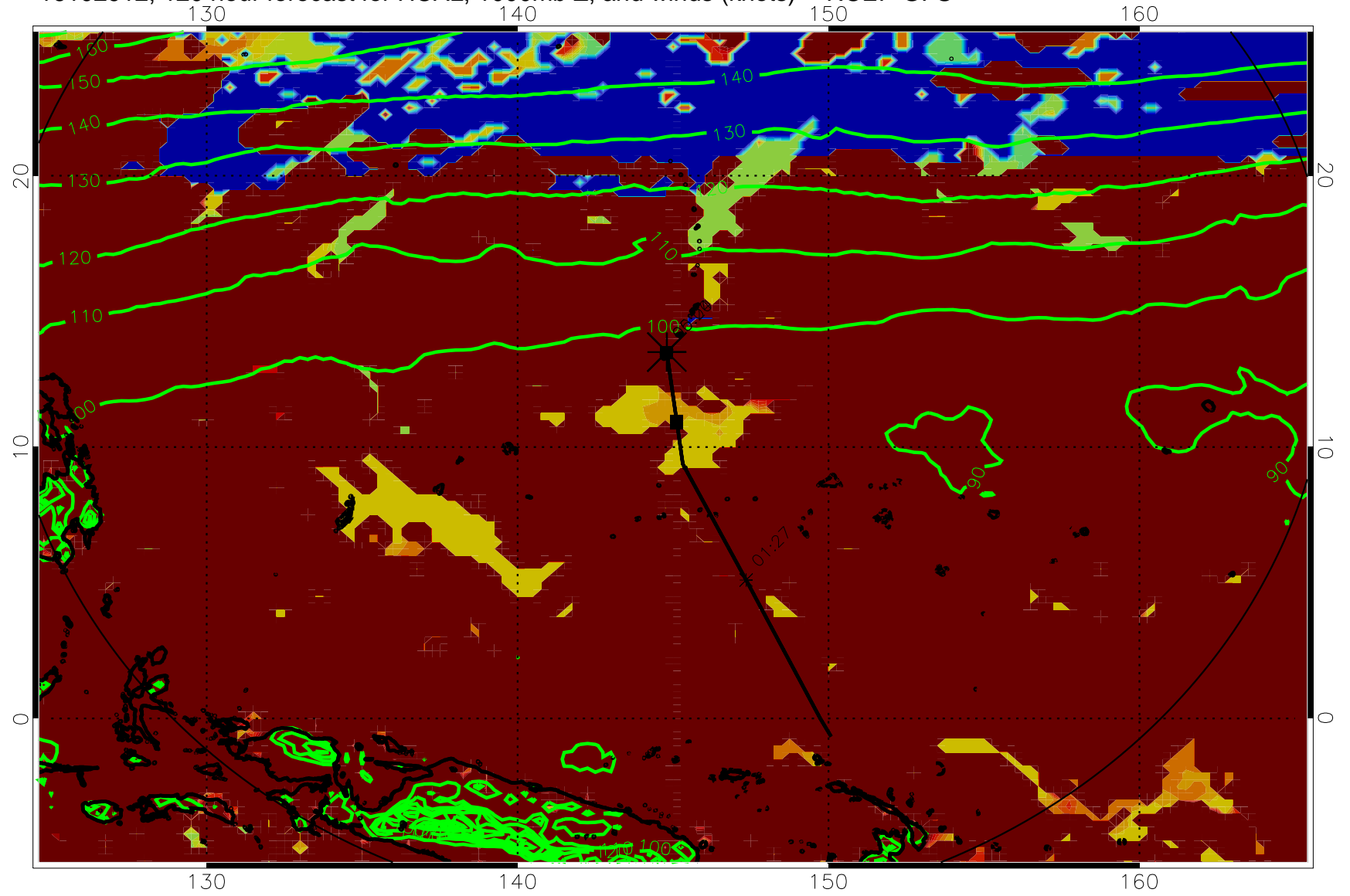
16102912, 120 hour forecast for HCAL, 1000mb Z, and winds (knots) -- NCEP GFS
