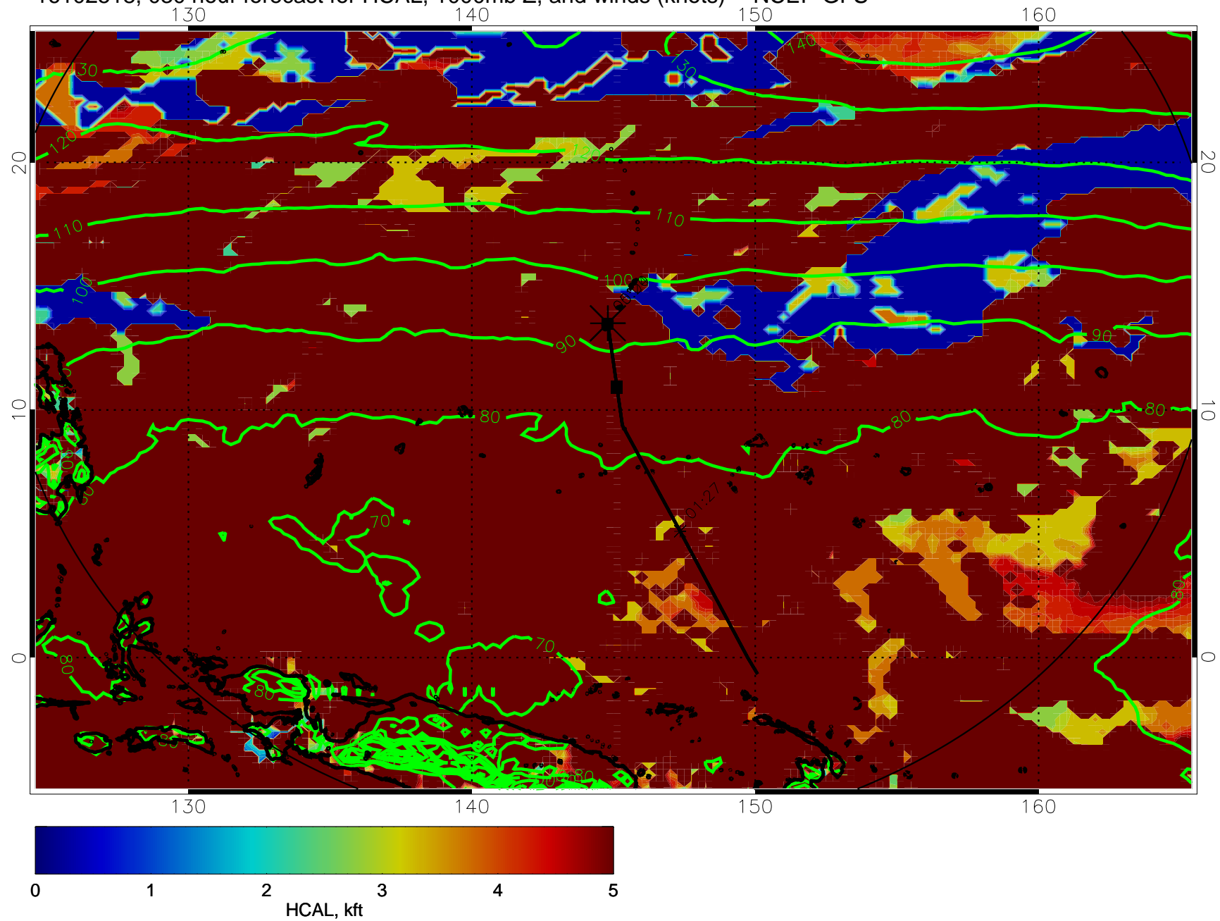
16102518, 030 hour forecast for HCAL, 1000mb Z, and winds (knots) -- NCEP GFS
