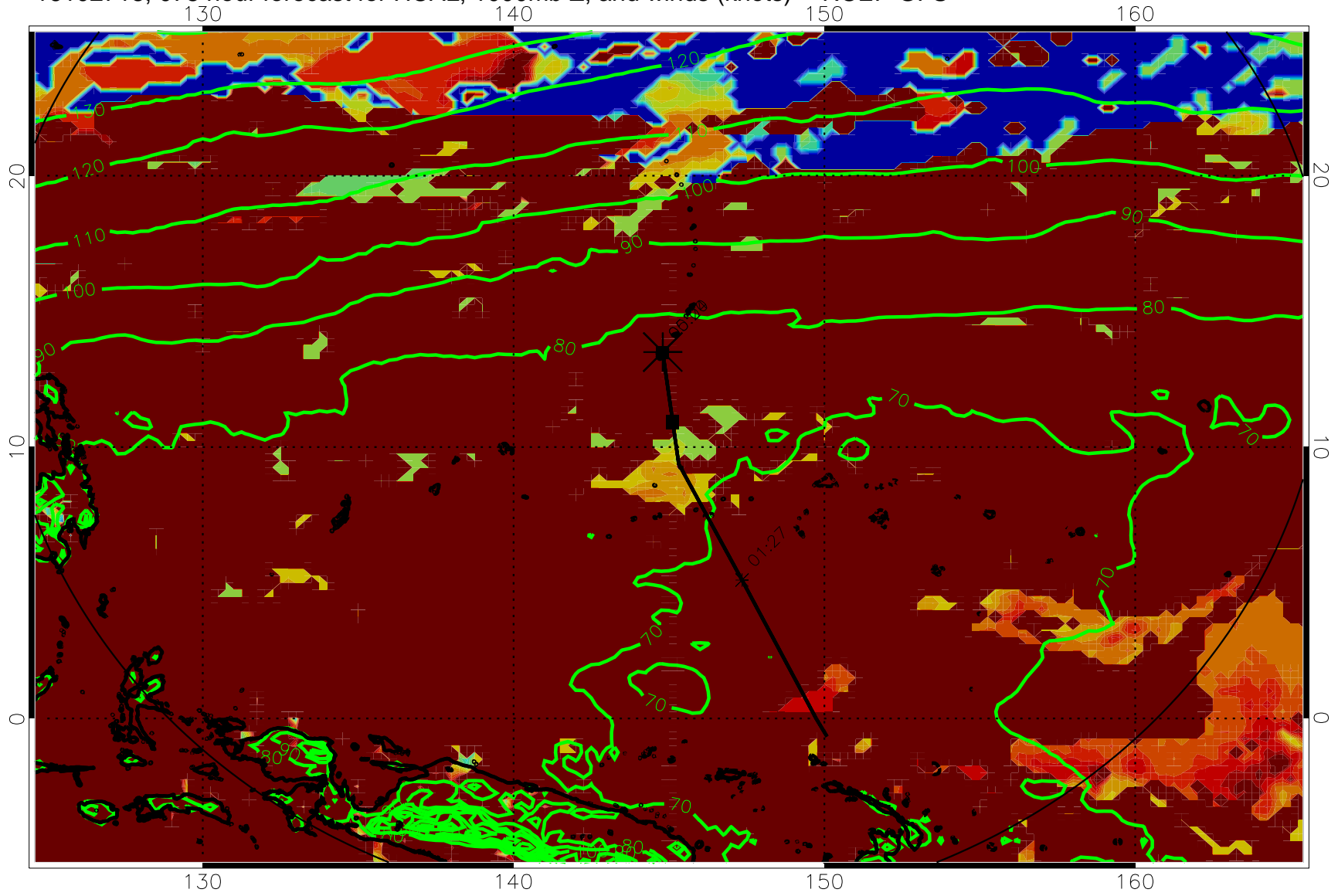
16102718, 078 hour forecast for HCAL, 1000mb Z, and winds (knots) -- NCEP GFS
