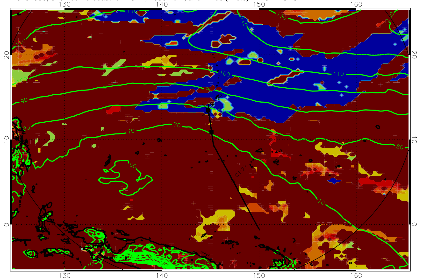
16102506, 018 hour forecast for HCAL, 1000mb Z, and winds (knots) -- NCEP GFS
