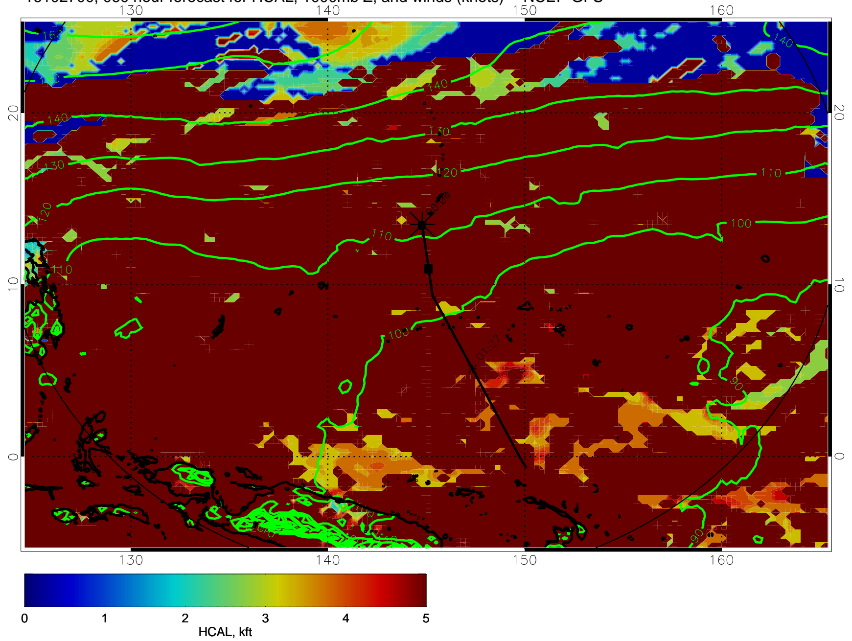
16102700, 060 hour forecast for HCAL, 1000mb Z, and winds (knots) -- NCEP GFS
