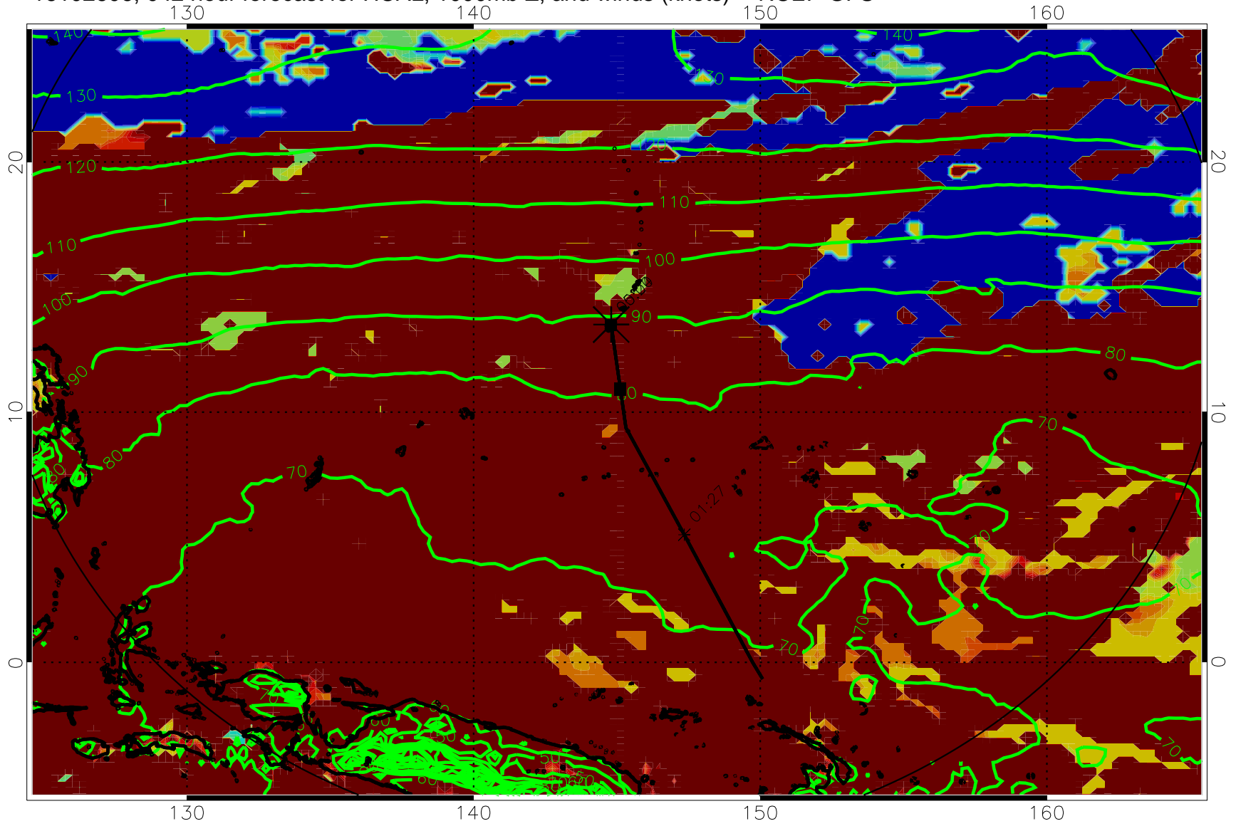
16102606, 042 hour forecast for HCAL, 1000mb Z, and winds (knots) -- NCEP GFS
