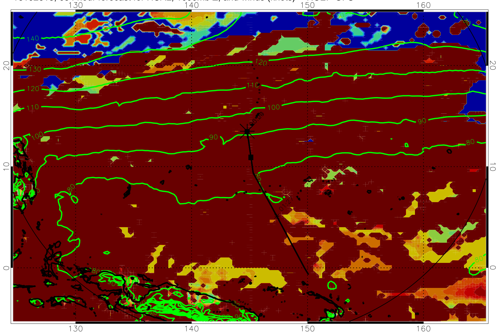
16102618, 054 hour forecast for HCAL, 1000mb Z, and winds (knots) -- NCEP GFS
