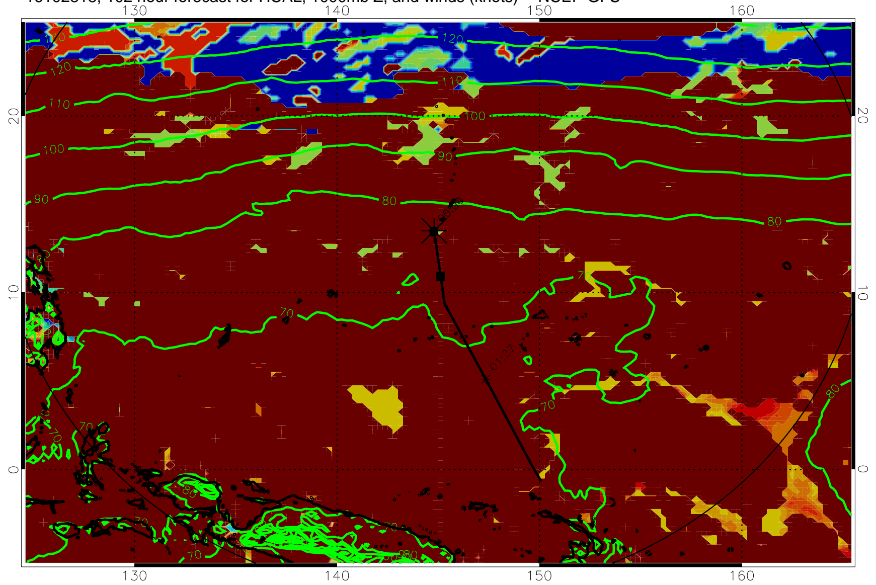
16102818, 102 hour forecast for HCAL, 1000mb Z, and winds (knots) -- NCEP GFS
