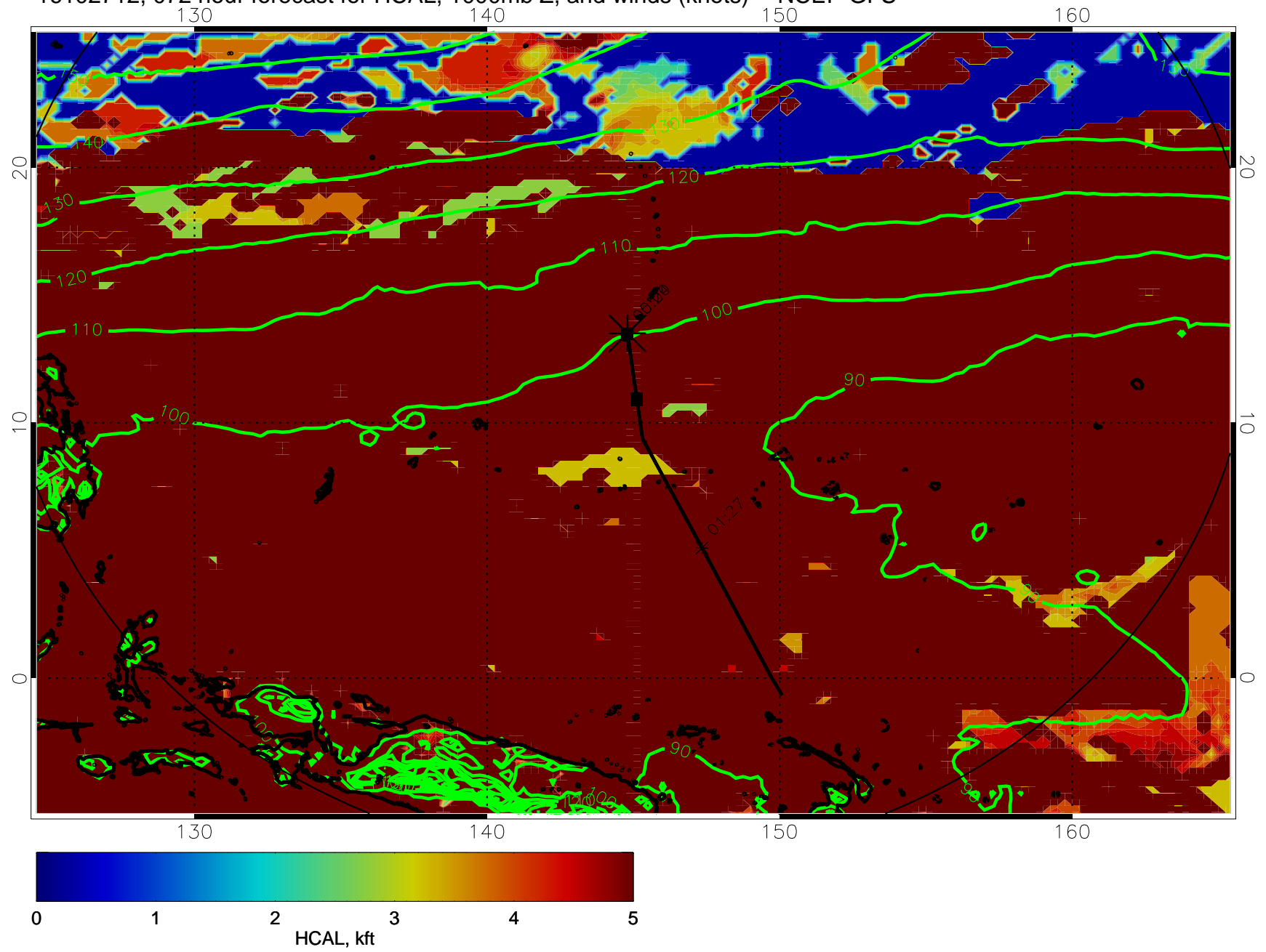
16102712, 072 hour forecast for HCAL, 1000mb Z, and winds (knots) -- NCEP GFS
