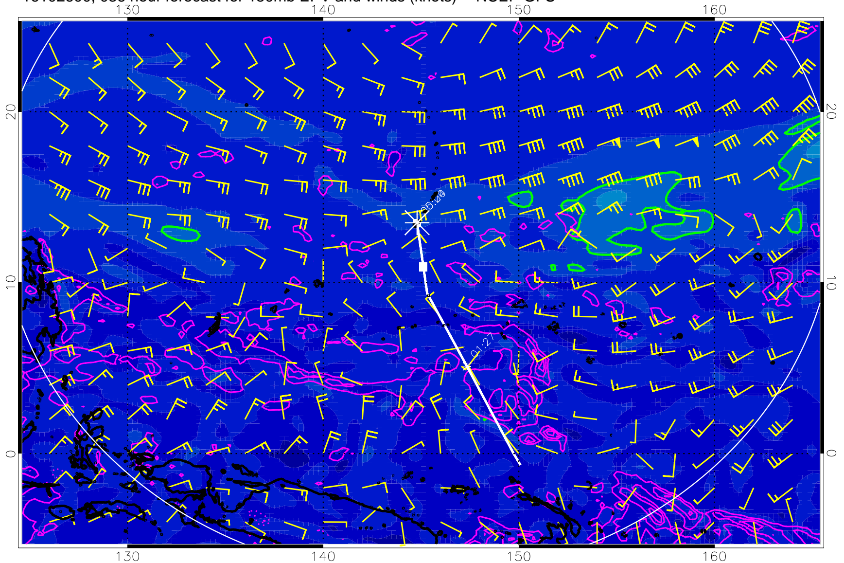
16102600, 036 hour forecast for 150mb EPV and winds (knots) -- NCEP GFS
