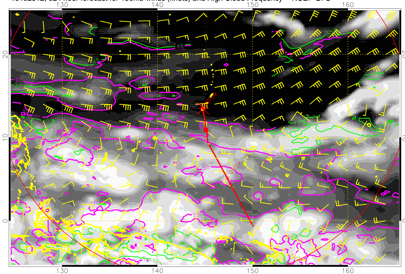
16102512, 024 hour forecast for 150mb winds (knots) and High Cloud Frequency -- NCEP GFS
