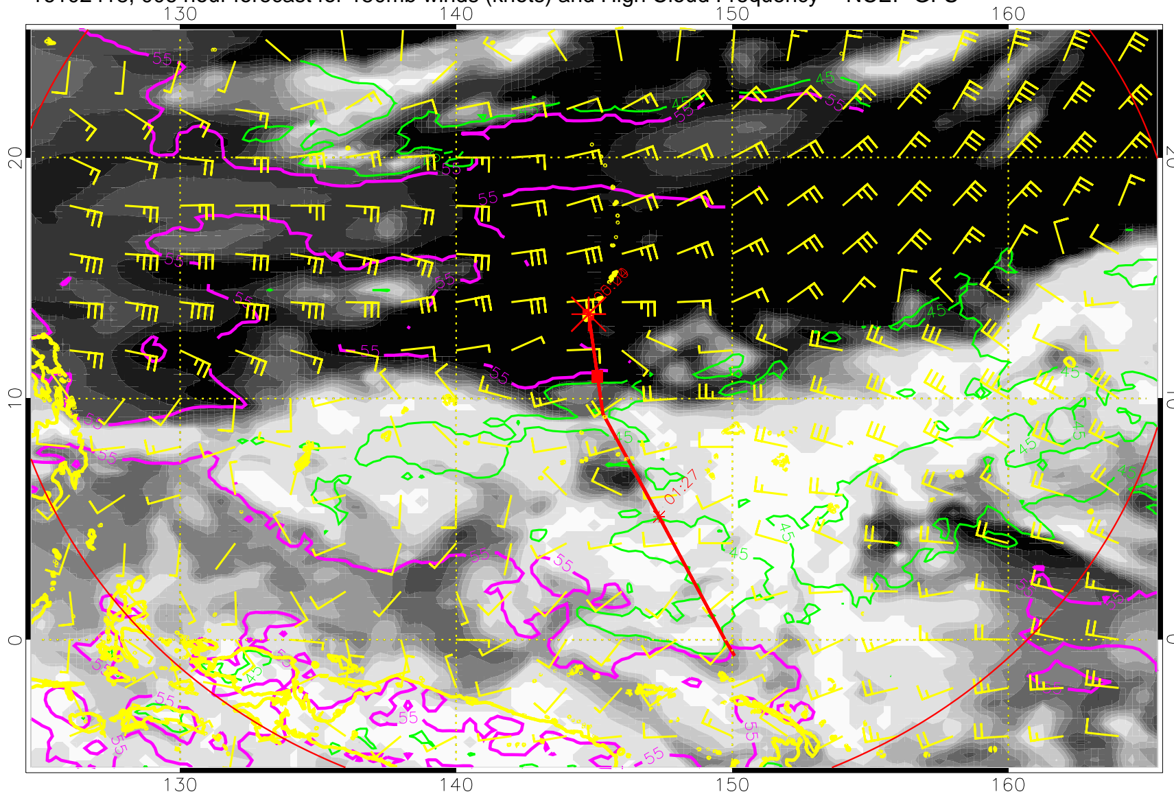
16102418, 006 hour forecast for 150mb winds (knots) and High Cloud Frequency -- NCEP GFS
