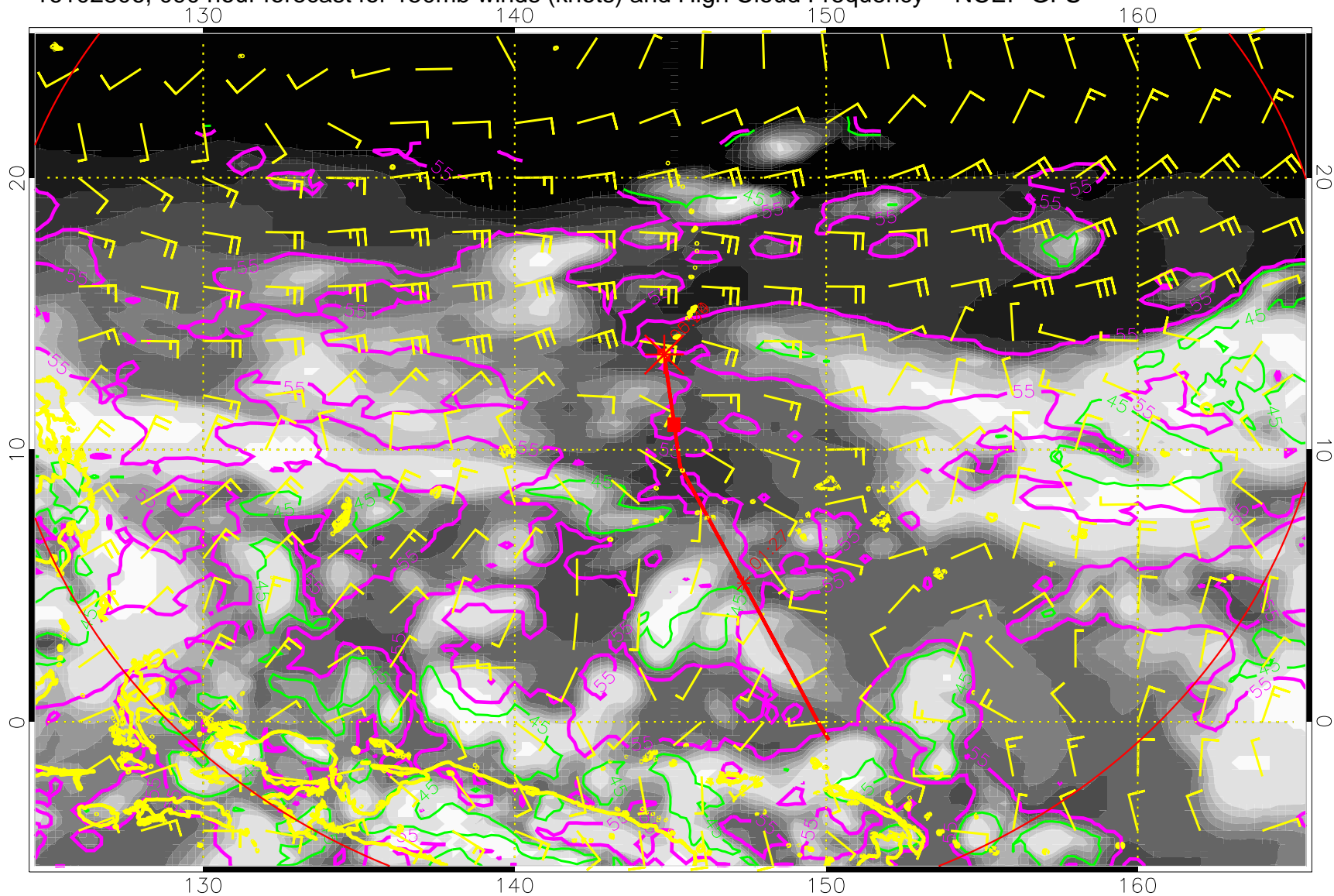
16102806, 090 hour forecast for 150mb winds (knots) and High Cloud Frequency -- NCEP GFS
