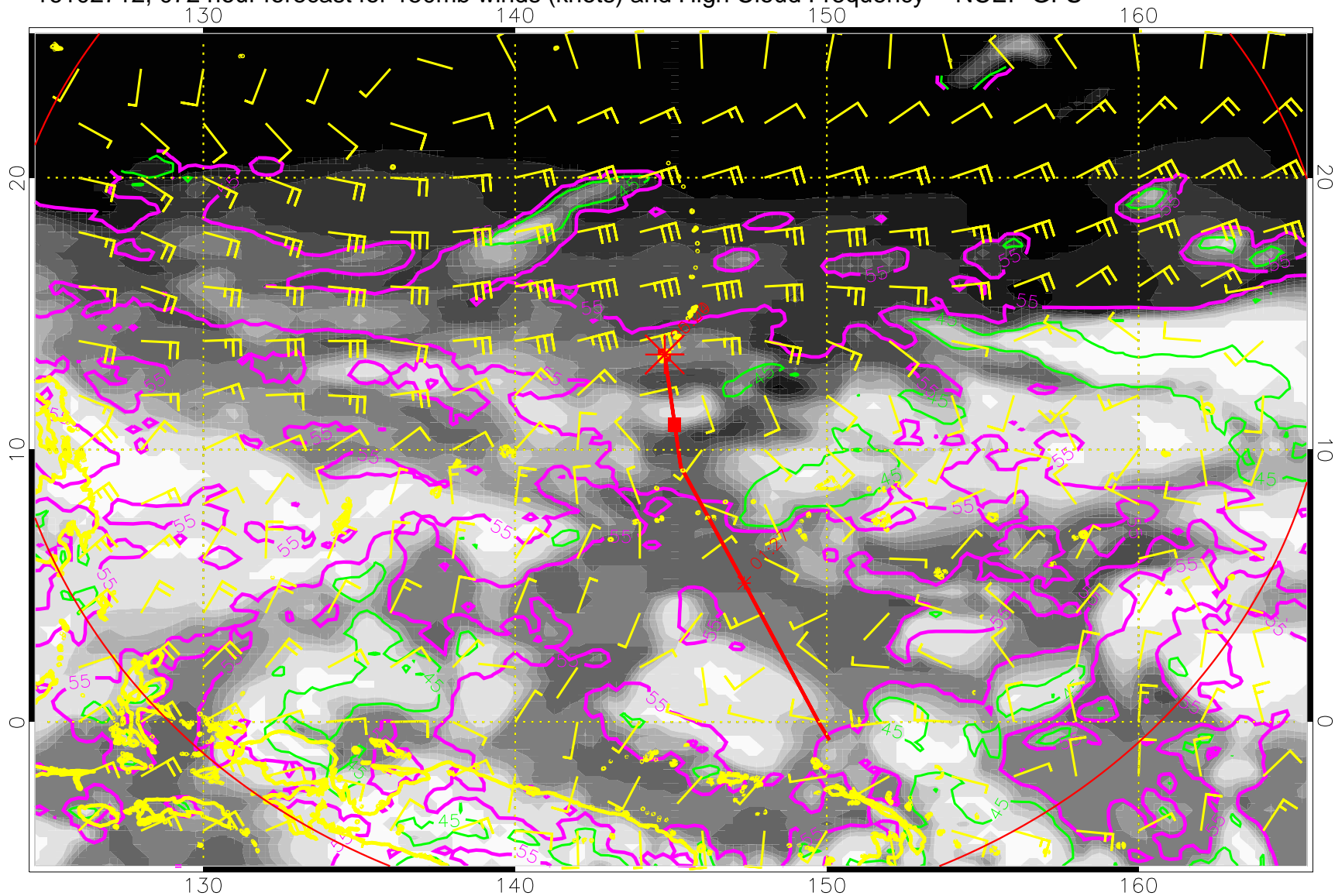
16102712, 072 hour forecast for 150mb winds (knots) and High Cloud Frequency -- NCEP GFS
