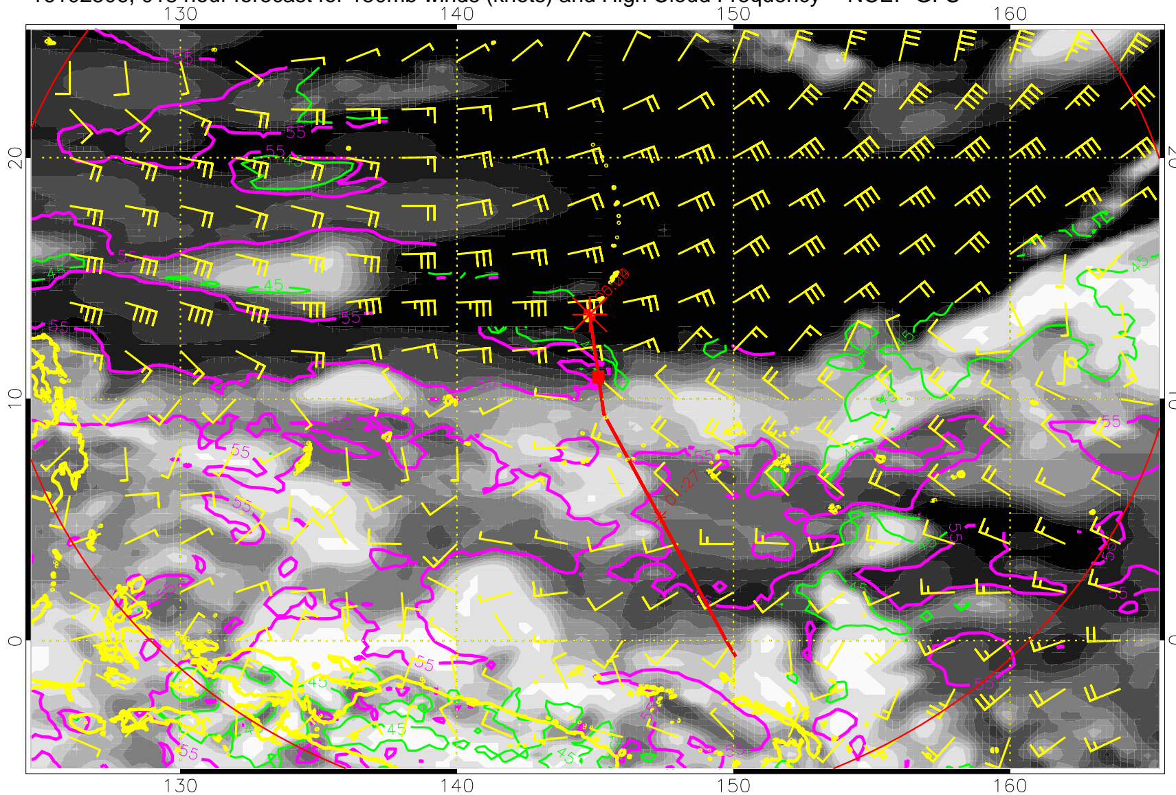
16102506, 018 hour forecast for 150mb winds (knots) and High Cloud Frequency -- NCEP GFS
