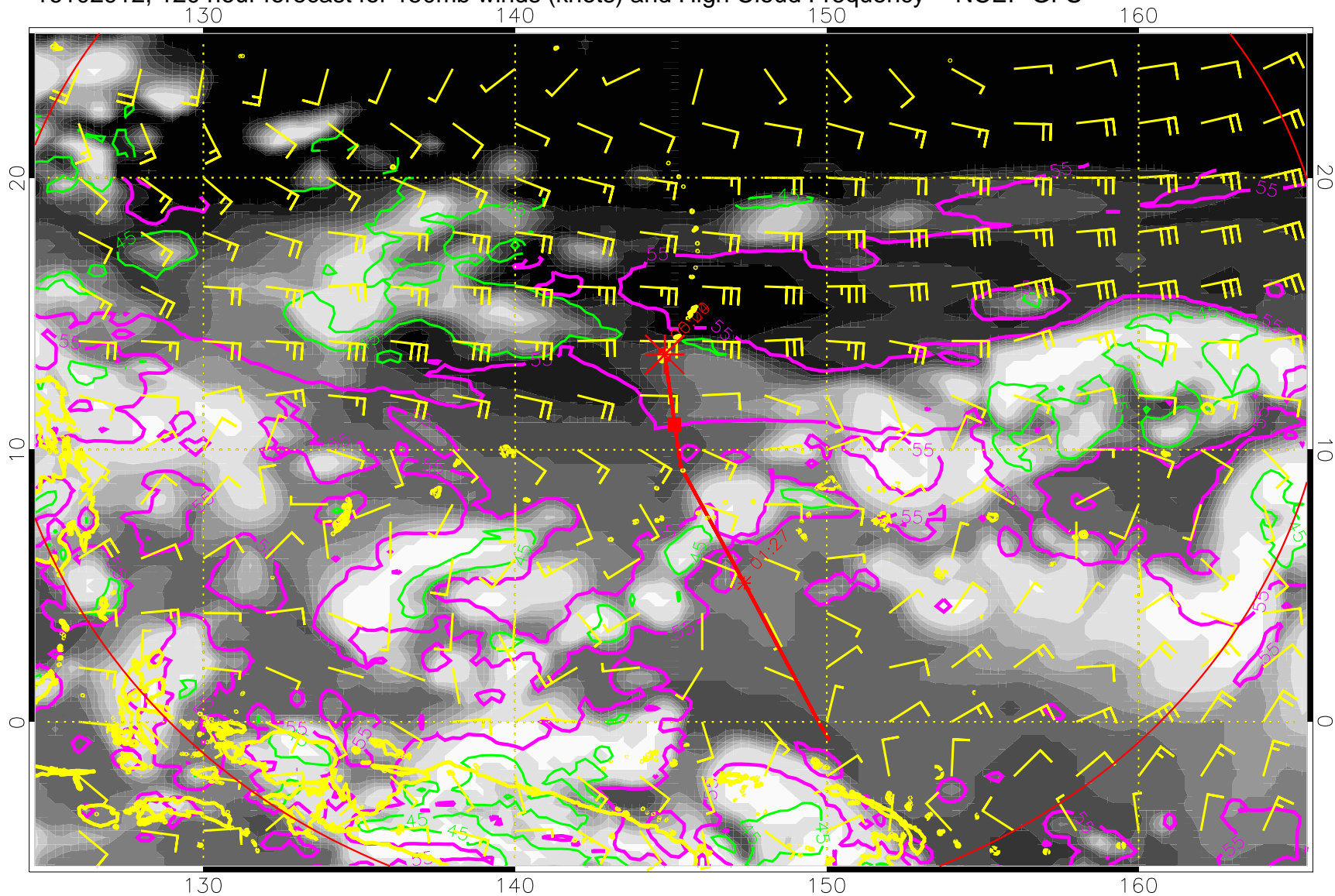
16102912, 120 hour forecast for 150mb winds (knots) and High Cloud Frequency -- NCEP GFS
