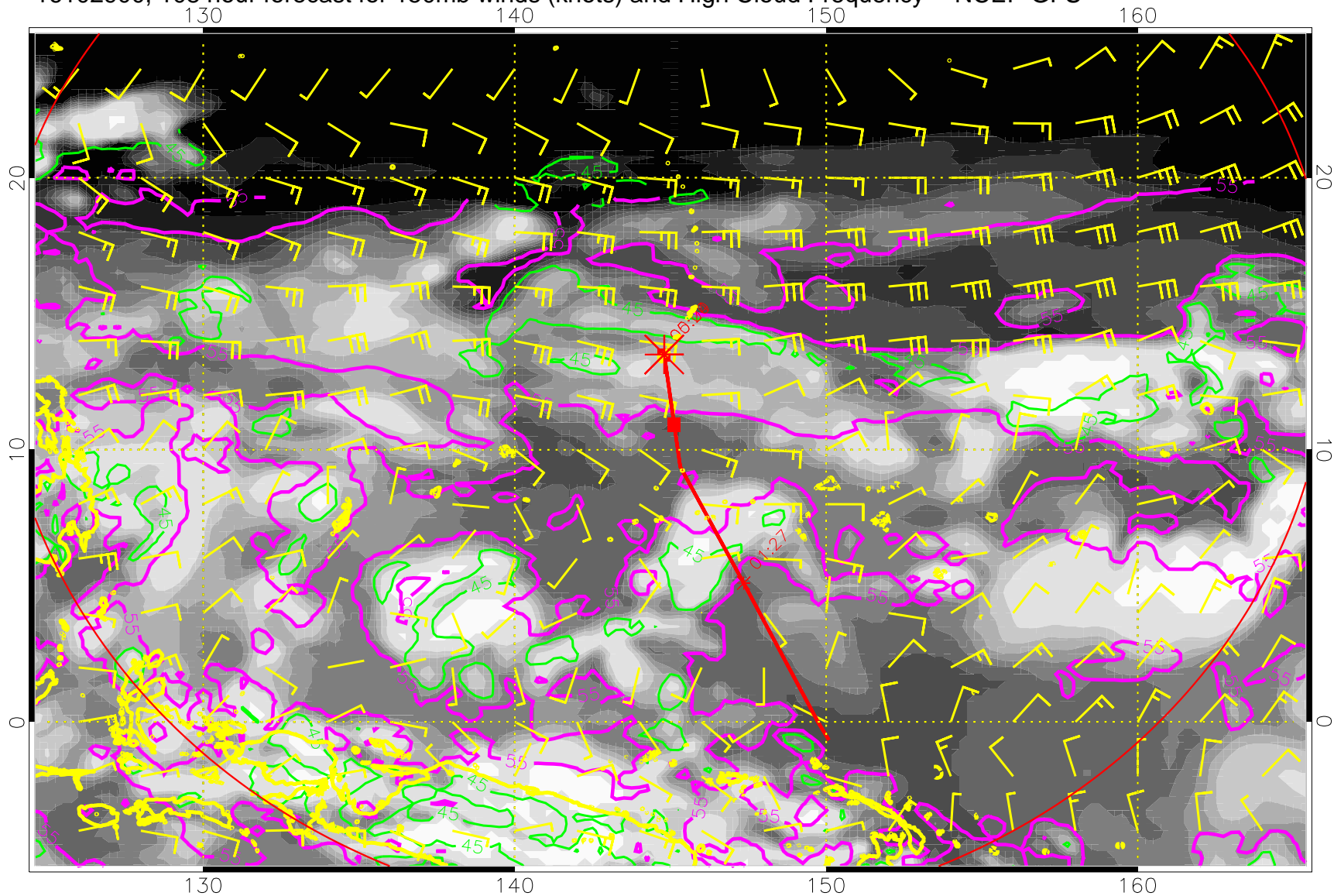
16102900, 108 hour forecast for 150mb winds (knots) and High Cloud Frequency -- NCEP GFS
