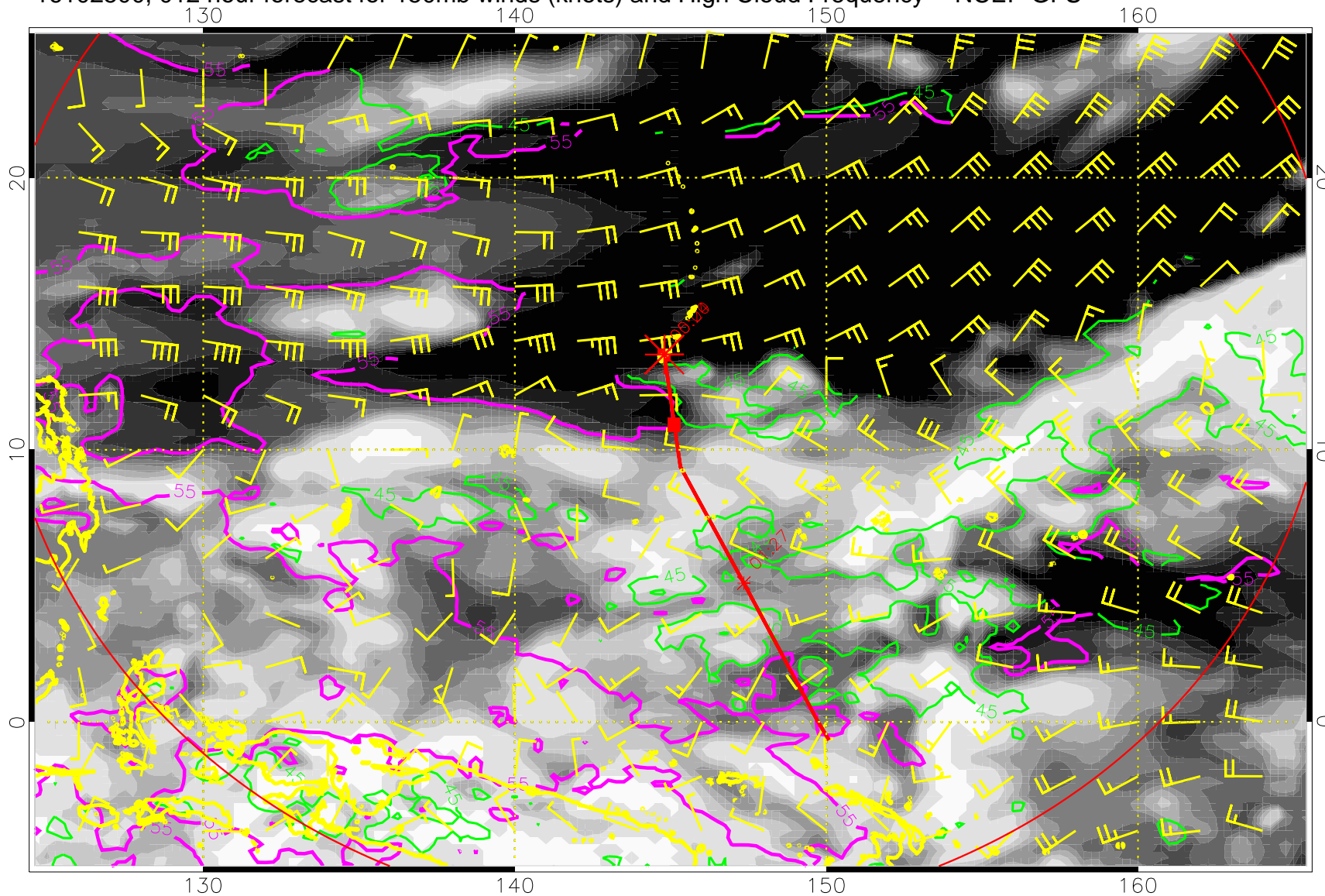
16102500, 012 hour forecast for 150mb winds (knots) and High Cloud Frequency -- NCEP GFS
