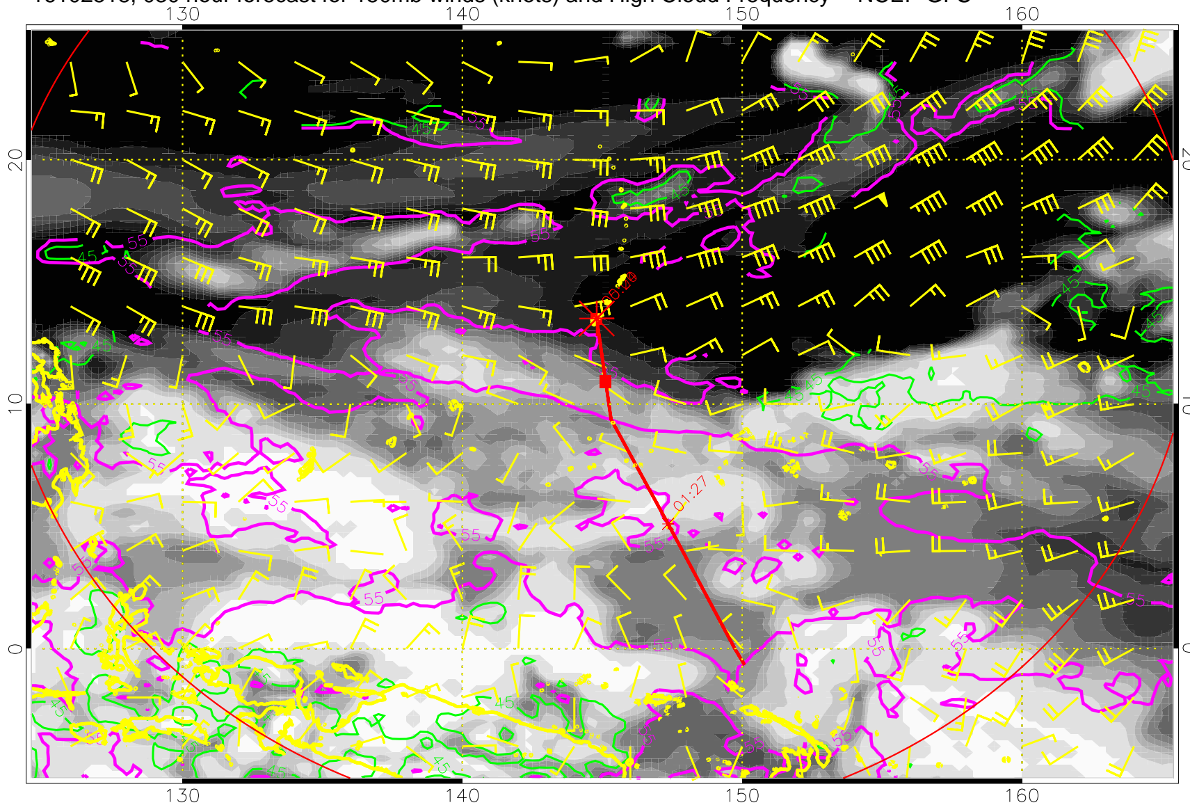
16102518, 030 hour forecast for 150mb winds (knots) and High Cloud Frequency -- NCEP GFS
