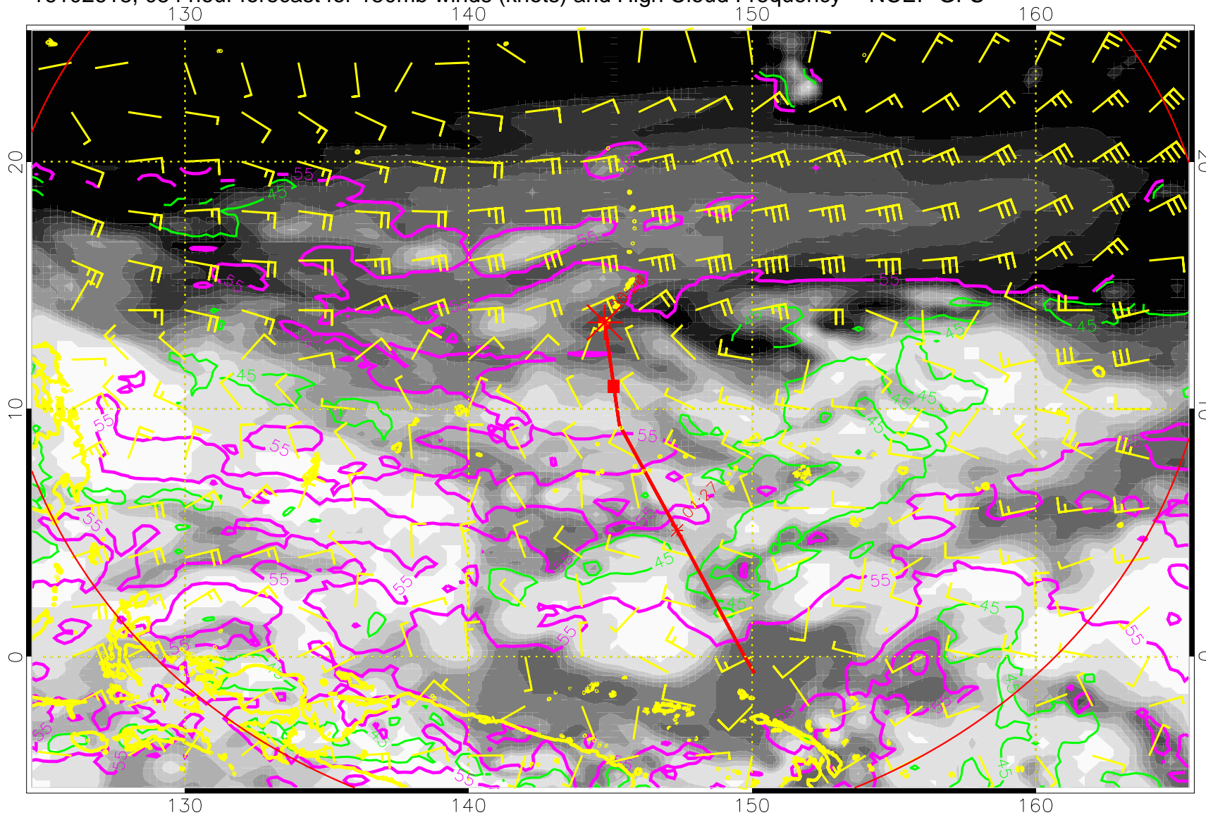
16102618, 054 hour forecast for 150mb winds (knots) and High Cloud Frequency -- NCEP GFS
