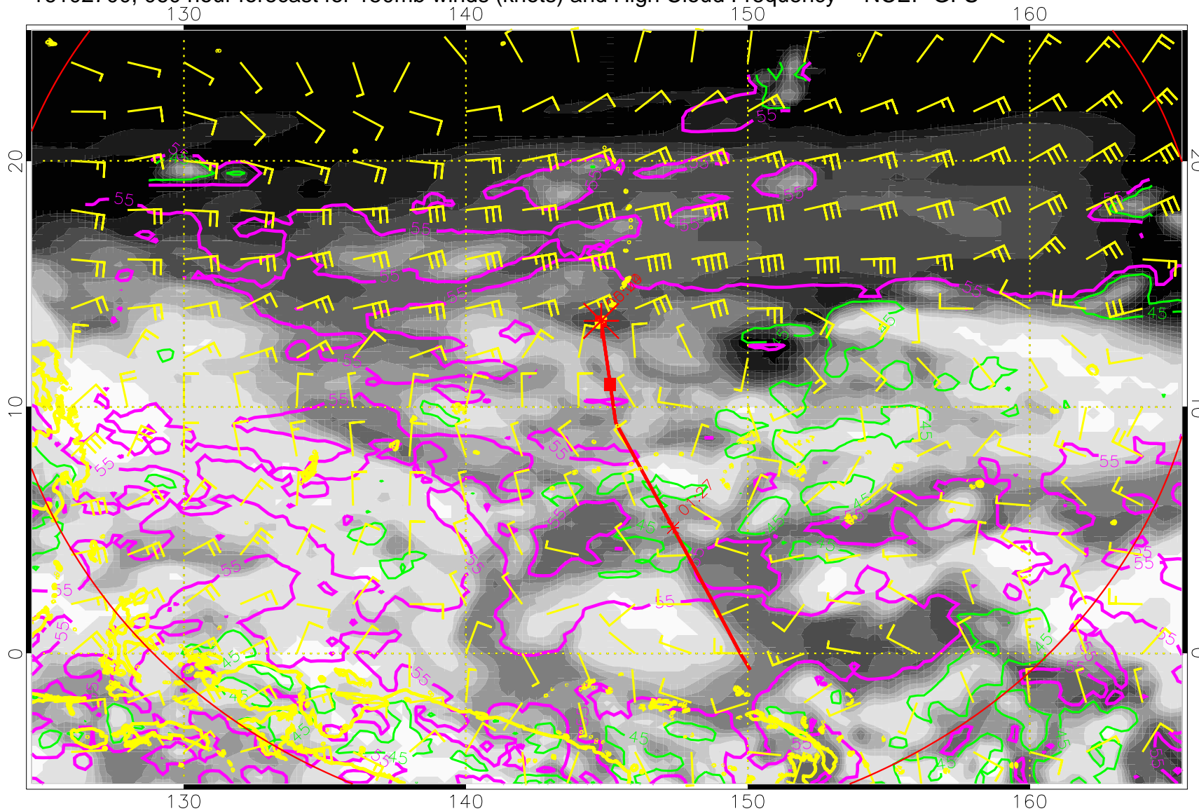
16102700, 060 hour forecast for 150mb winds (knots) and High Cloud Frequency -- NCEP GFS
