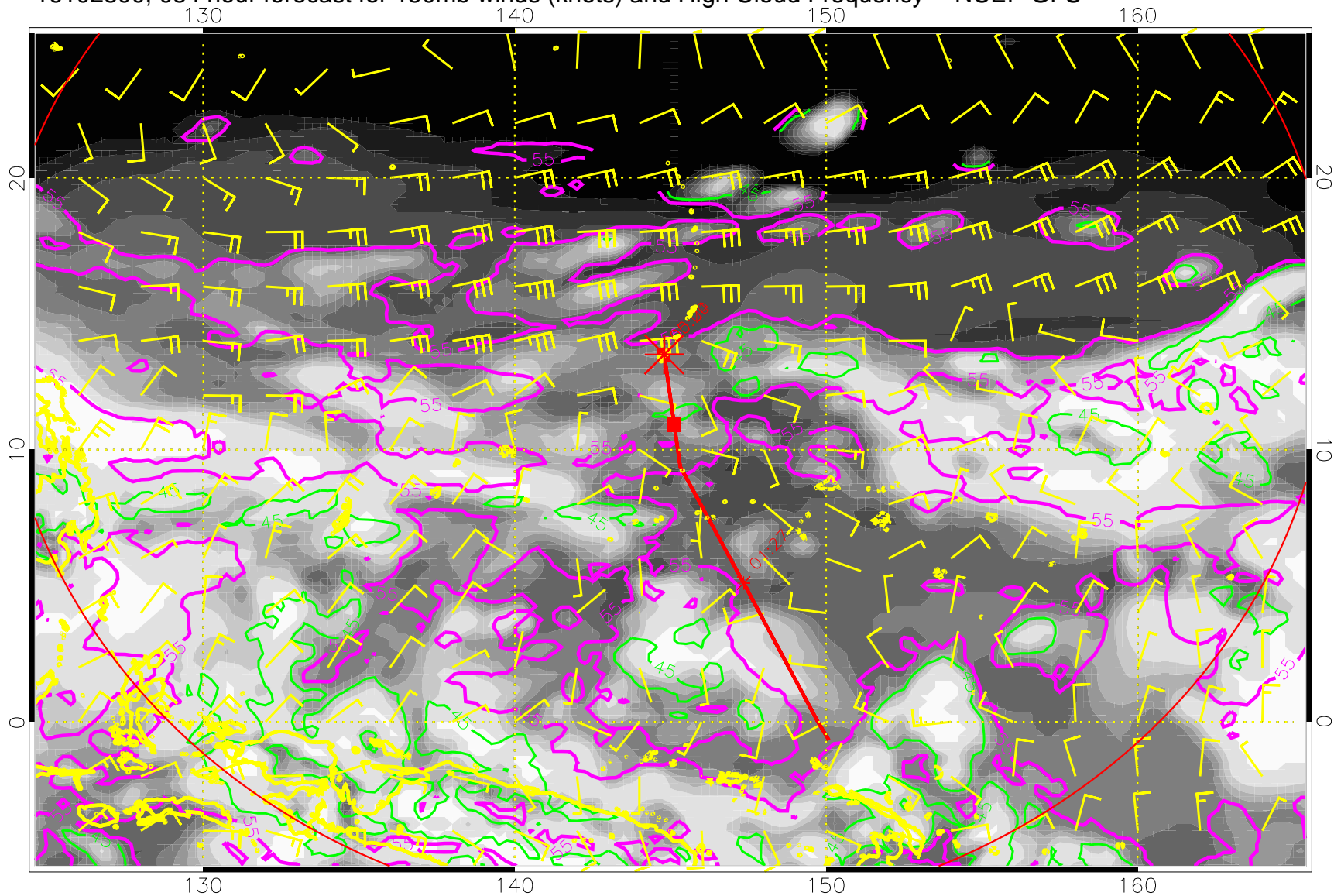
16102800, 084 hour forecast for 150mb winds (knots) and High Cloud Frequency -- NCEP GFS
