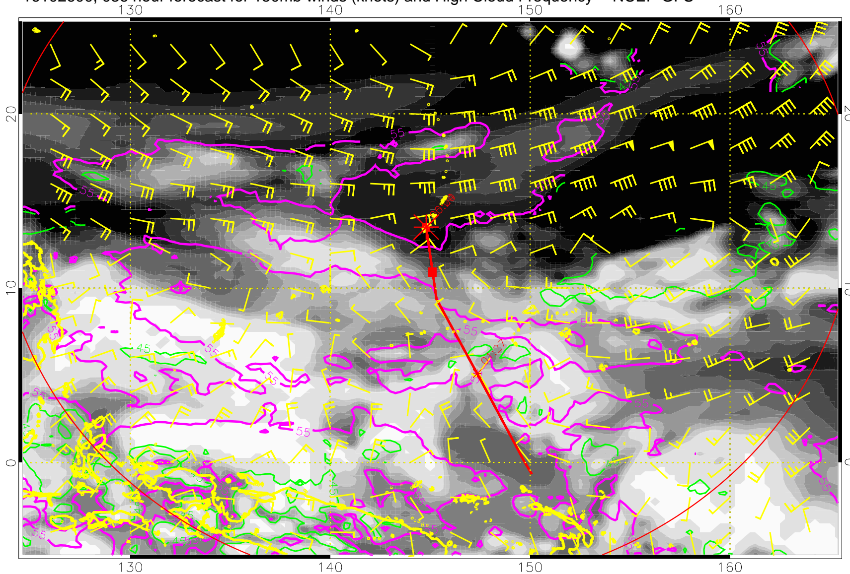
16102600, 036 hour forecast for 150mb winds (knots) and High Cloud Frequency -- NCEP GFS
