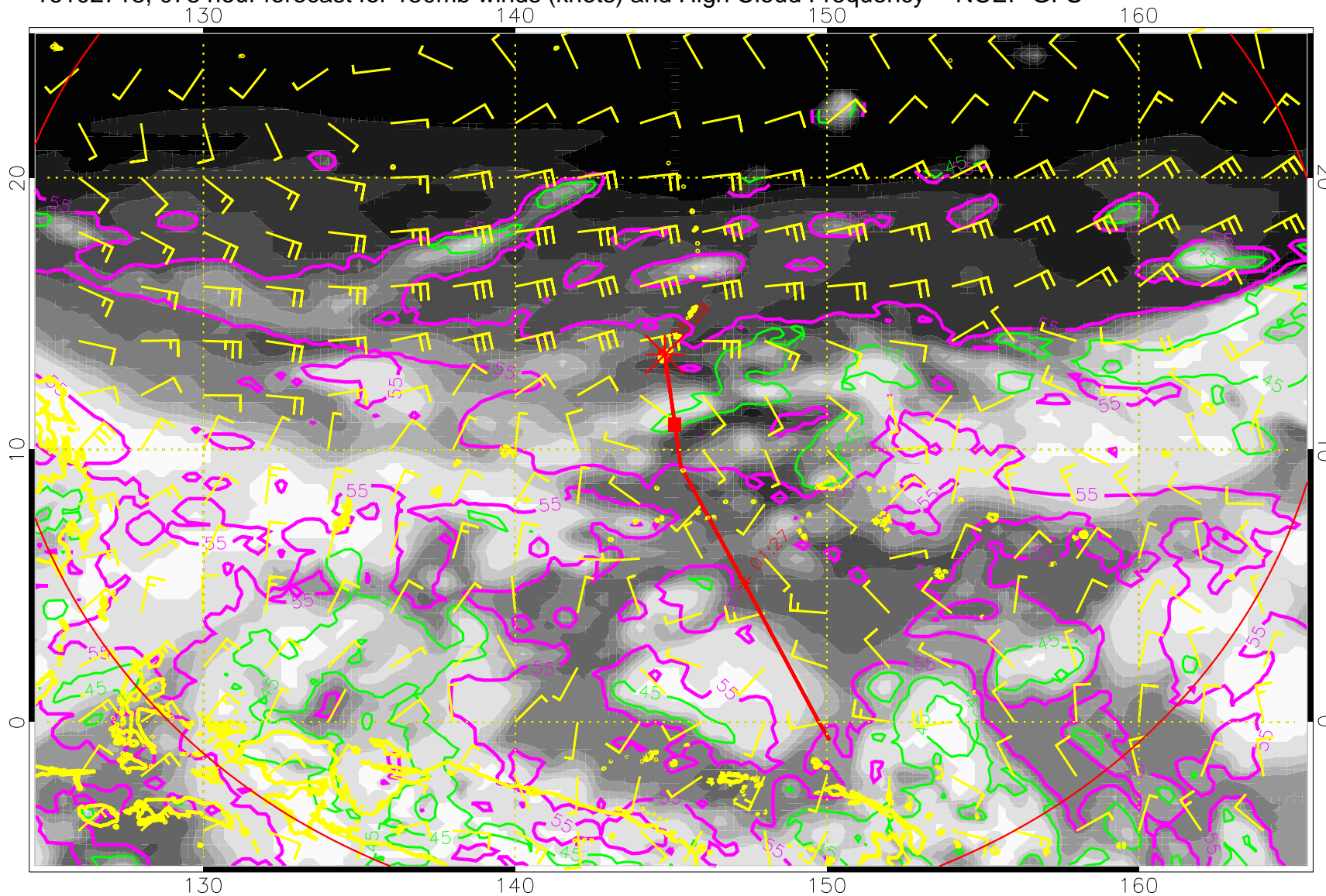
16102718, 078 hour forecast for 150mb winds (knots) and High Cloud Frequency -- NCEP GFS
