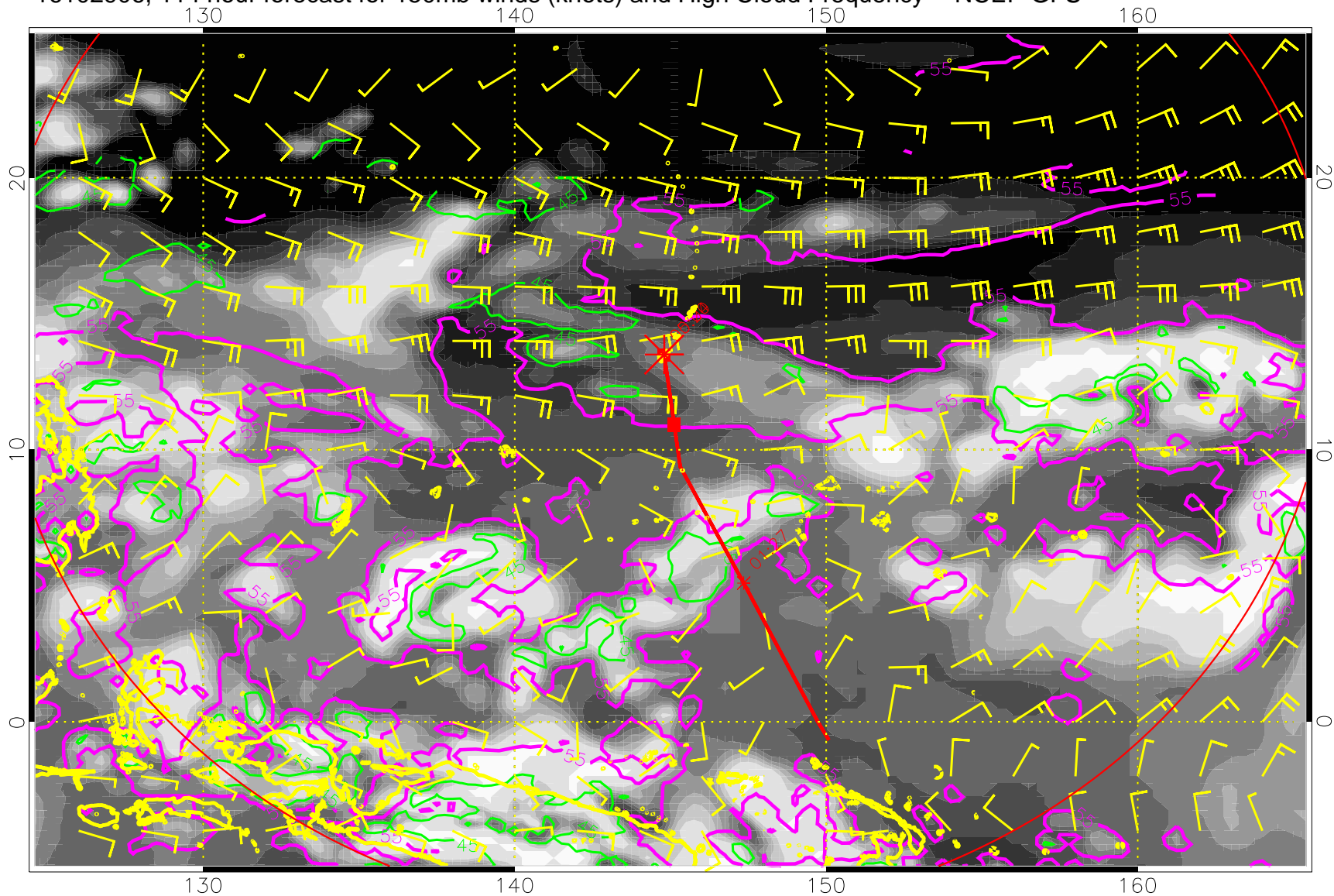
16102906, 114 hour forecast for 150mb winds (knots) and High Cloud Frequency -- NCEP GFS
