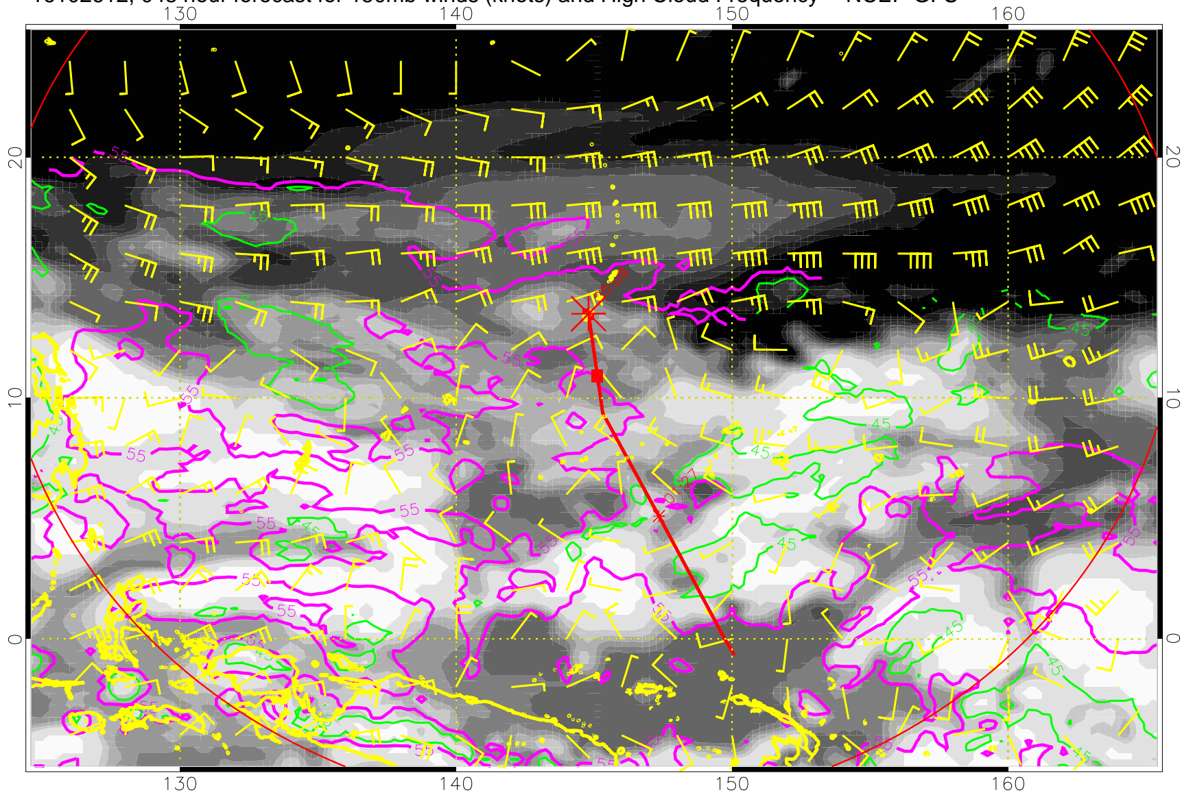
16102612, 048 hour forecast for 150mb winds (knots) and High Cloud Frequency -- NCEP GFS
