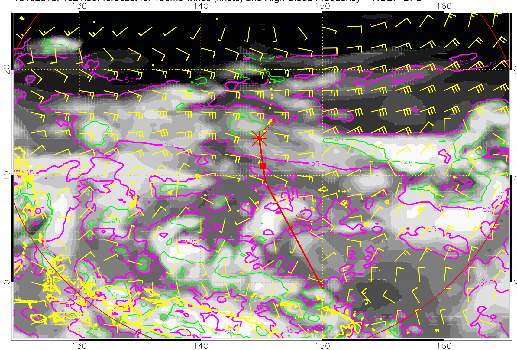
16102818, 102 hour forecast for 150mb winds (knots) and High Cloud Frequency -- NCEP GFS
