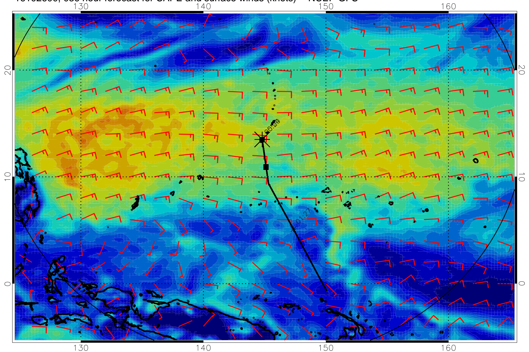
16102600, 036 hour forecast for CAPE and surface winds (knots) -- NCEP GFS
