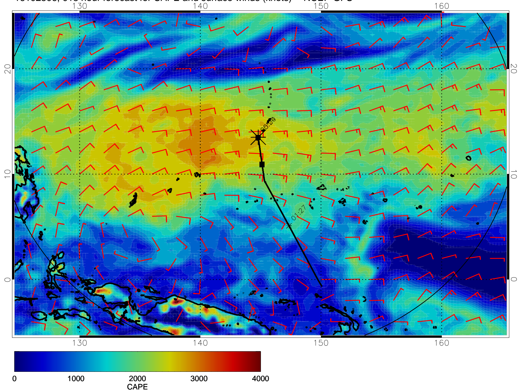
16102506, 018 hour forecast for CAPE and surface winds (knots) -- NCEP GFS
