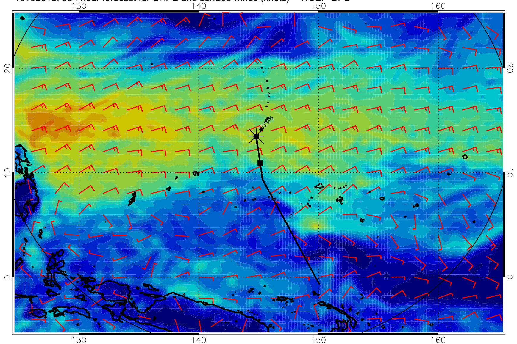
16102618, 054 hour forecast for CAPE and surface winds (knots) -- NCEP GFS
