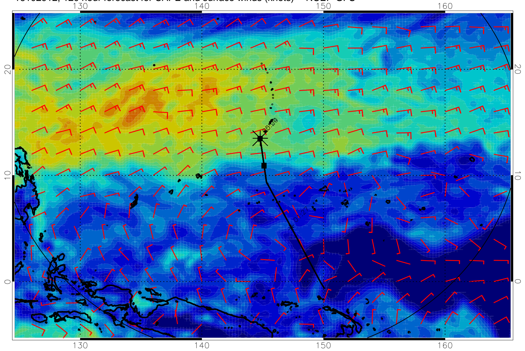
16102912, 120 hour forecast for CAPE and surface winds (knots) -- NCEP GFS
