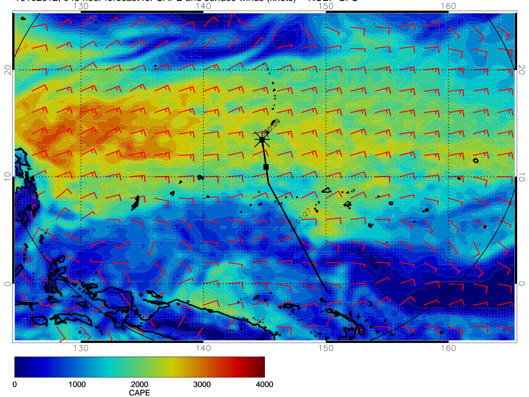
16102612, 048 hour forecast for CAPE and surface winds (knots) -- NCEP GFS
