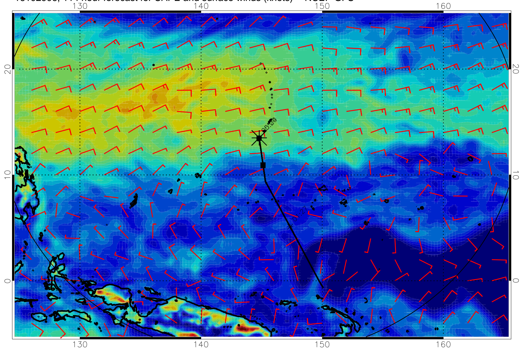
16102906, 114 hour forecast for CAPE and surface winds (knots) -- NCEP GFS
