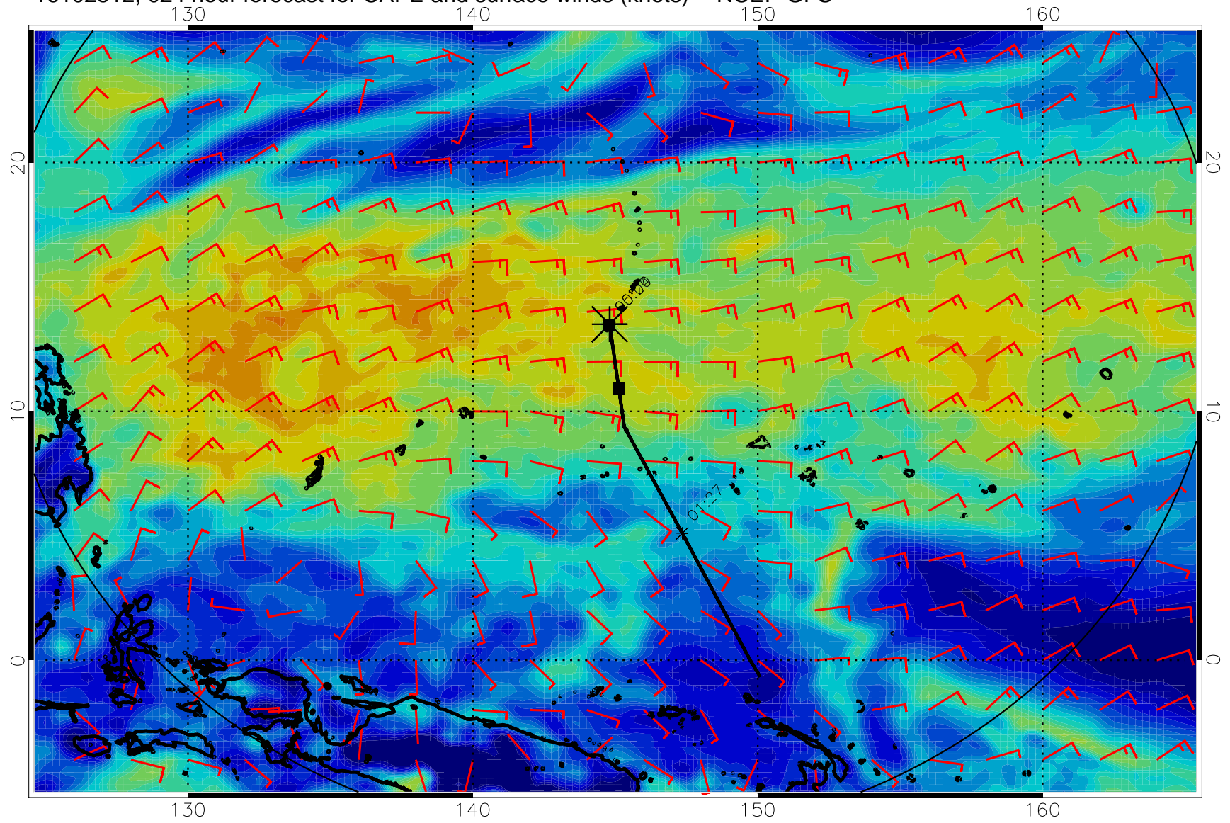
16102512, 024 hour forecast for CAPE and surface winds (knots) -- NCEP GFS
