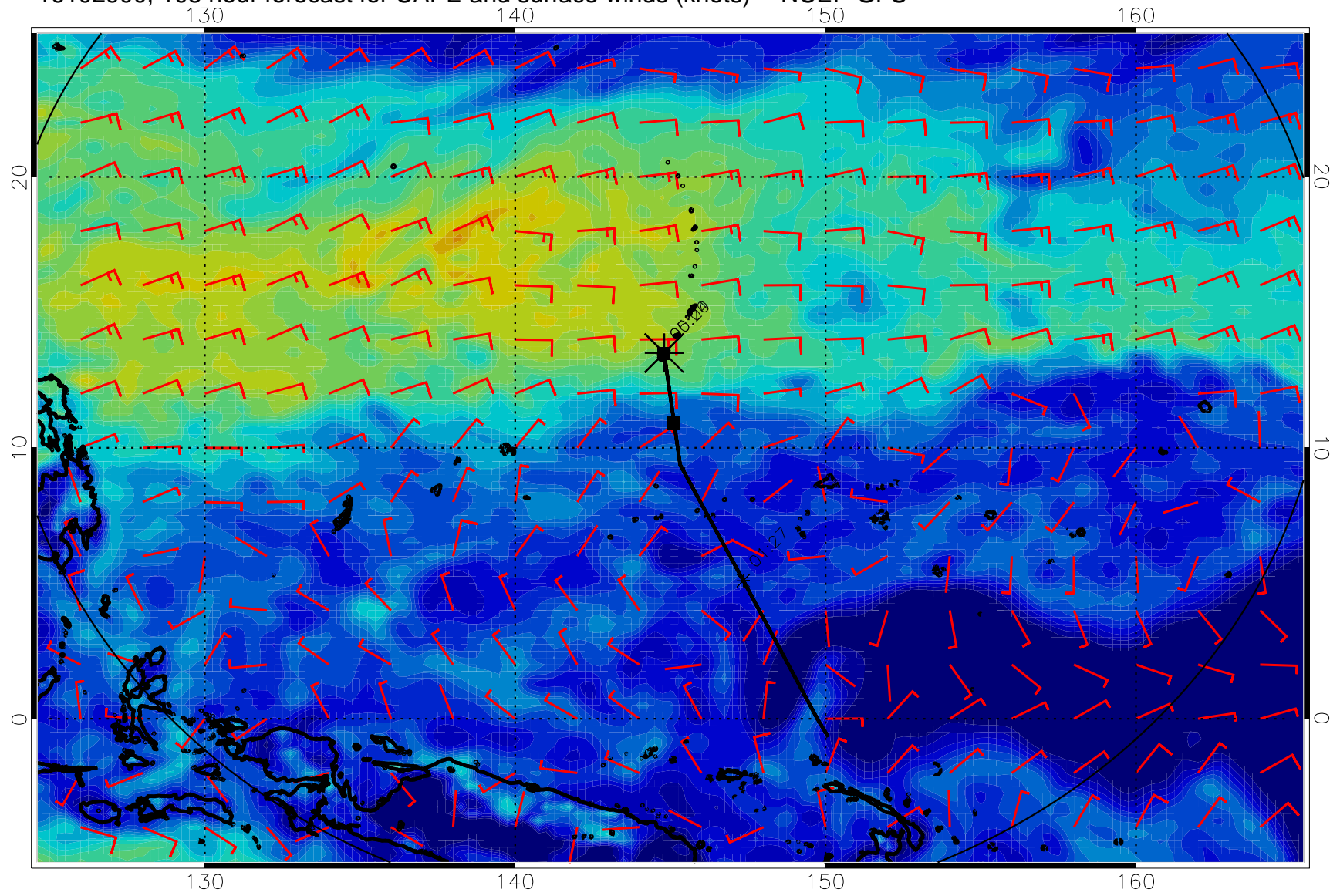
16102900, 108 hour forecast for CAPE and surface winds (knots) -- NCEP GFS
