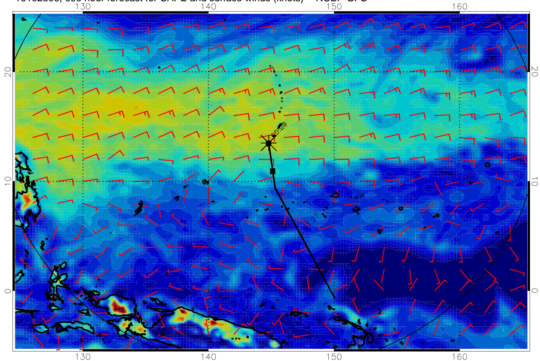
16102806, 090 hour forecast for CAPE and surface winds (knots) -- NCEP GFS
