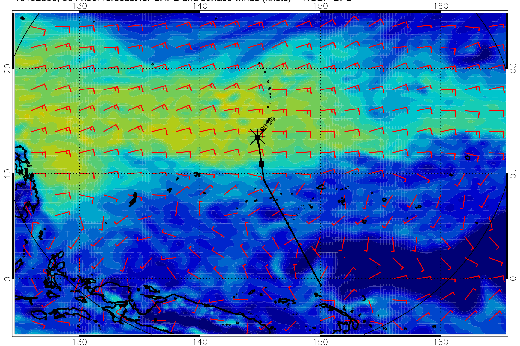
16102800, 084 hour forecast for CAPE and surface winds (knots) -- NCEP GFS
