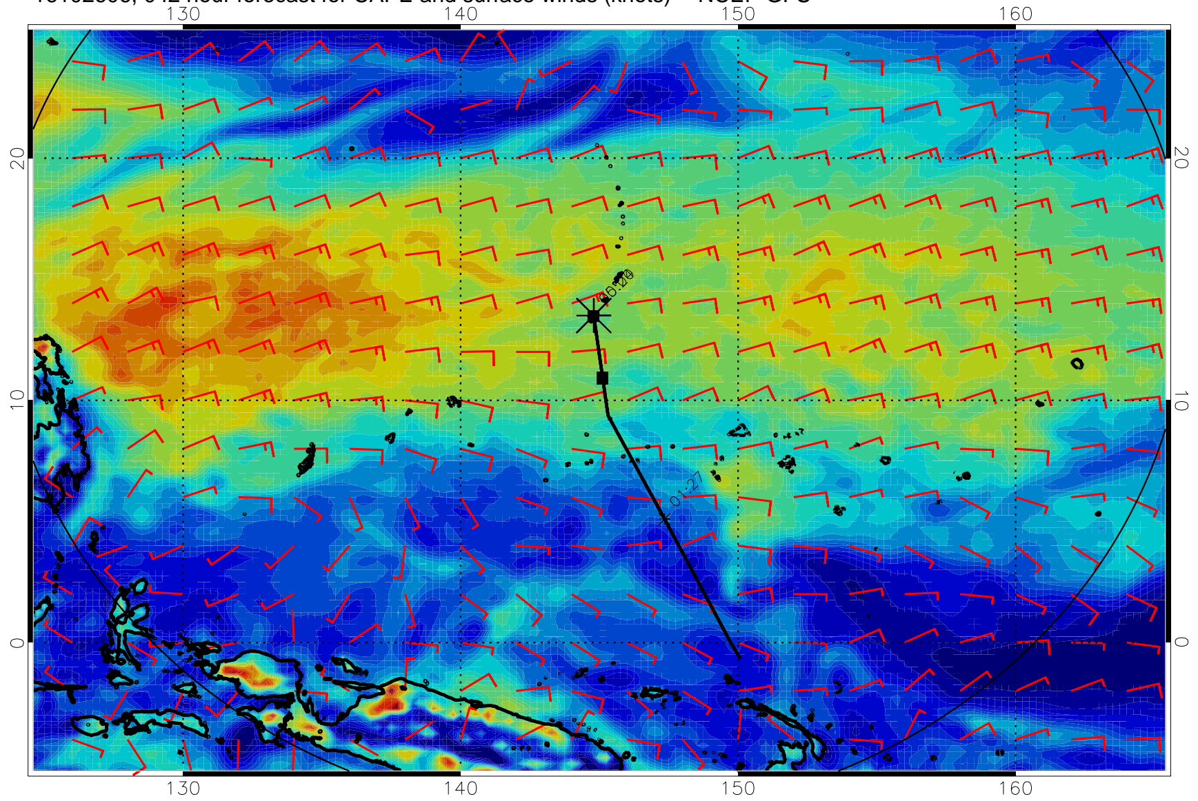
16102606, 042 hour forecast for CAPE and surface winds (knots) -- NCEP GFS
