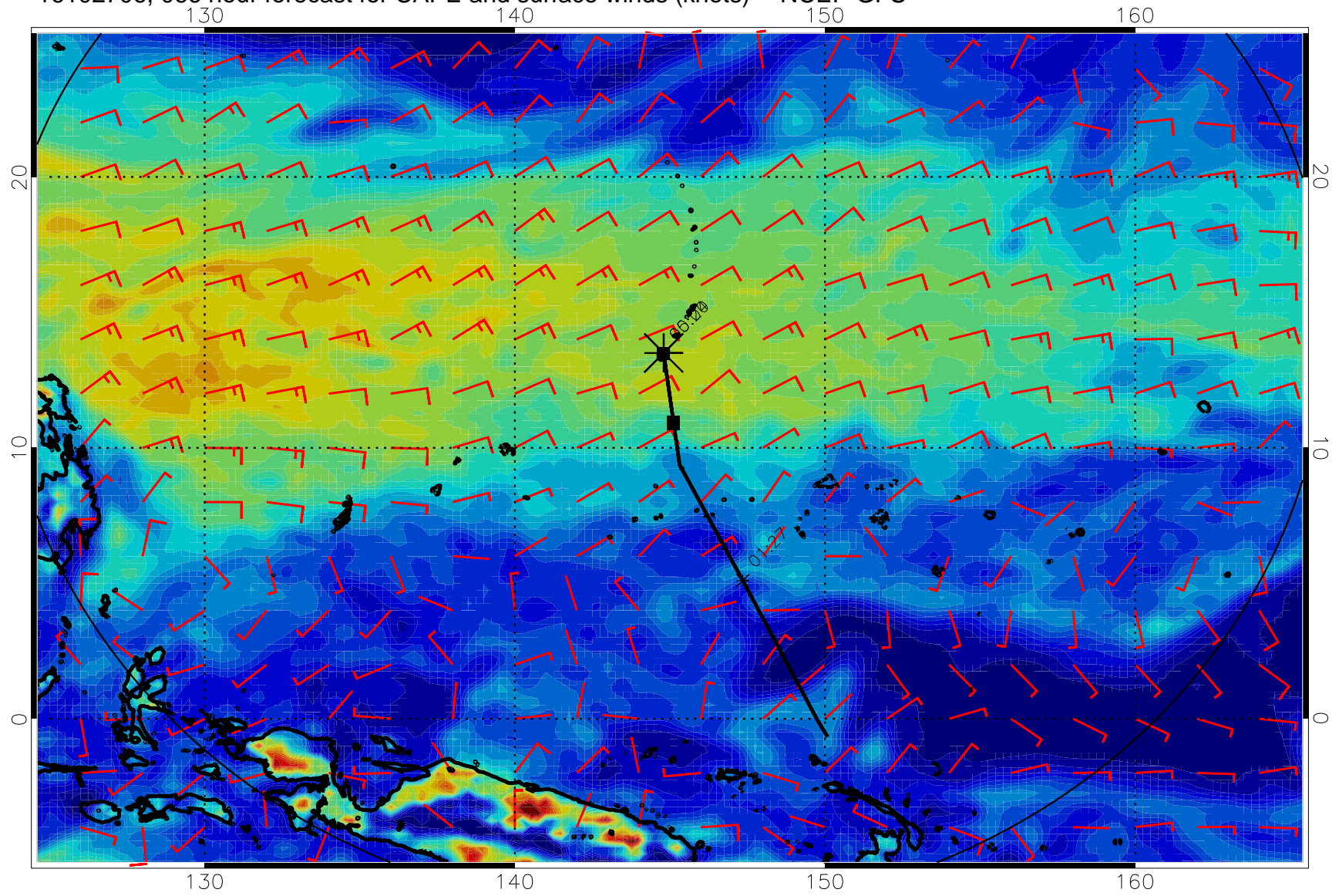
16102706, 066 hour forecast for CAPE and surface winds (knots) -- NCEP GFS
