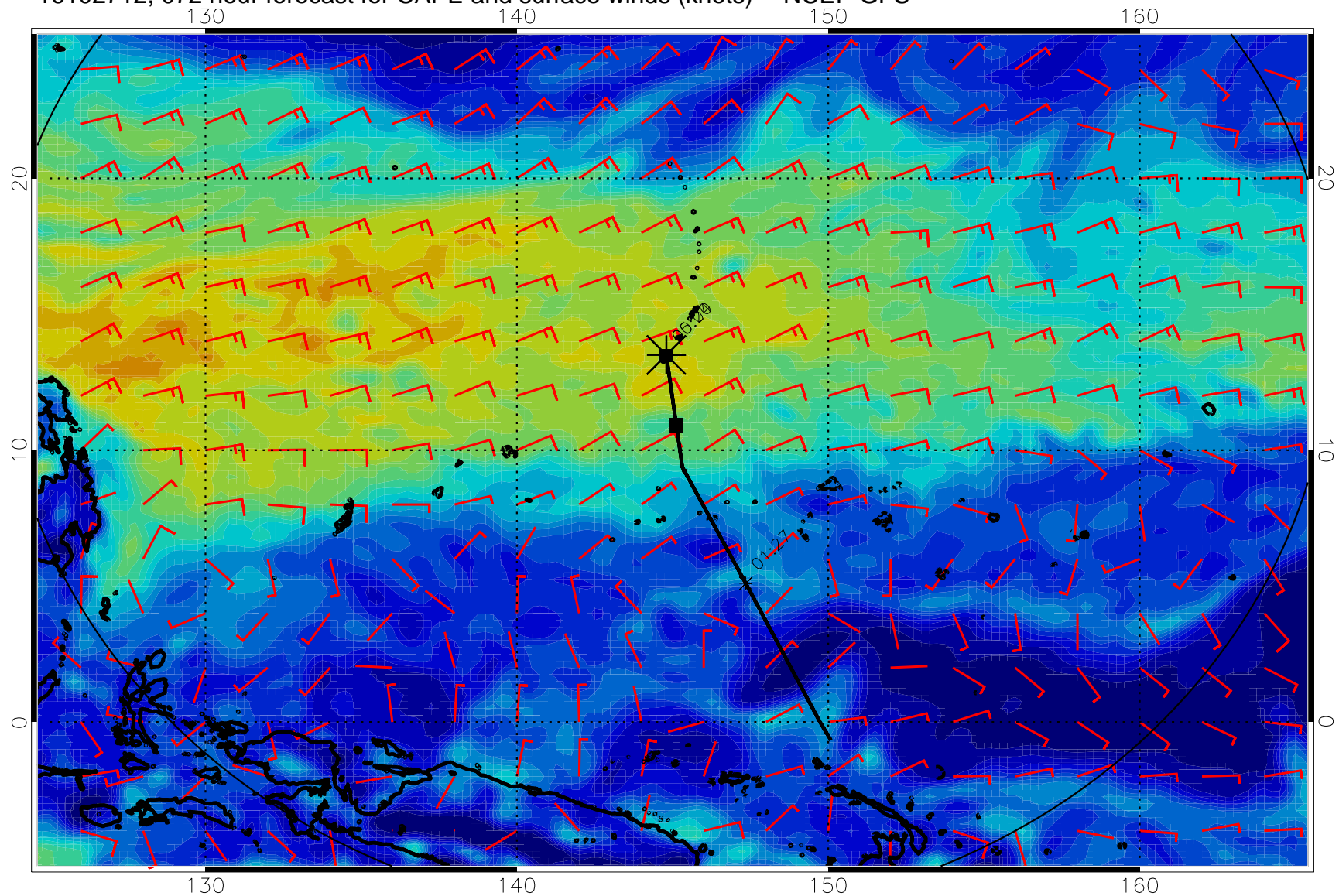
16102712, 072 hour forecast for CAPE and surface winds (knots) -- NCEP GFS
