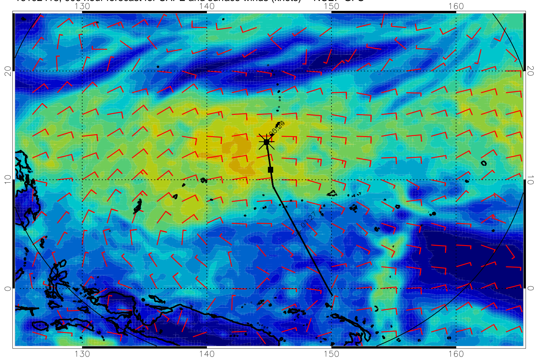
16102418, 006 hour forecast for CAPE and surface winds (knots) -- NCEP GFS
