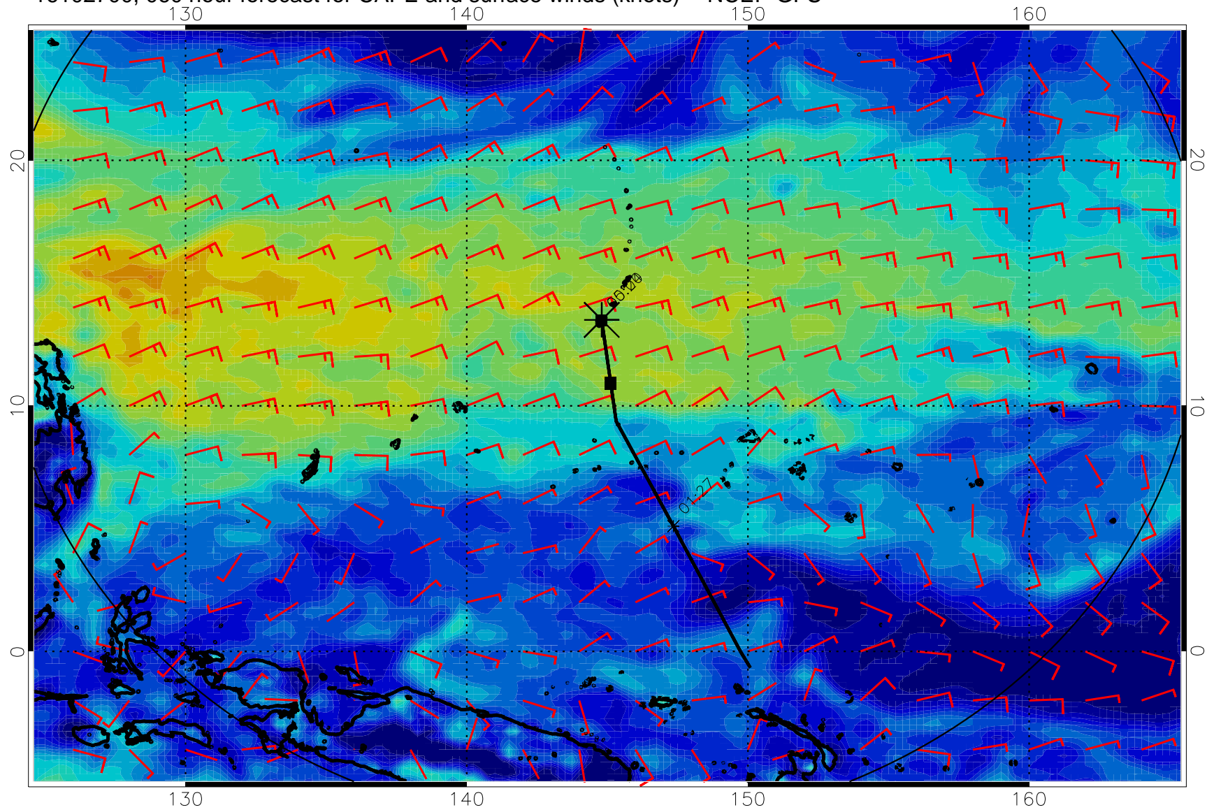
16102700, 060 hour forecast for CAPE and surface winds (knots) -- NCEP GFS
