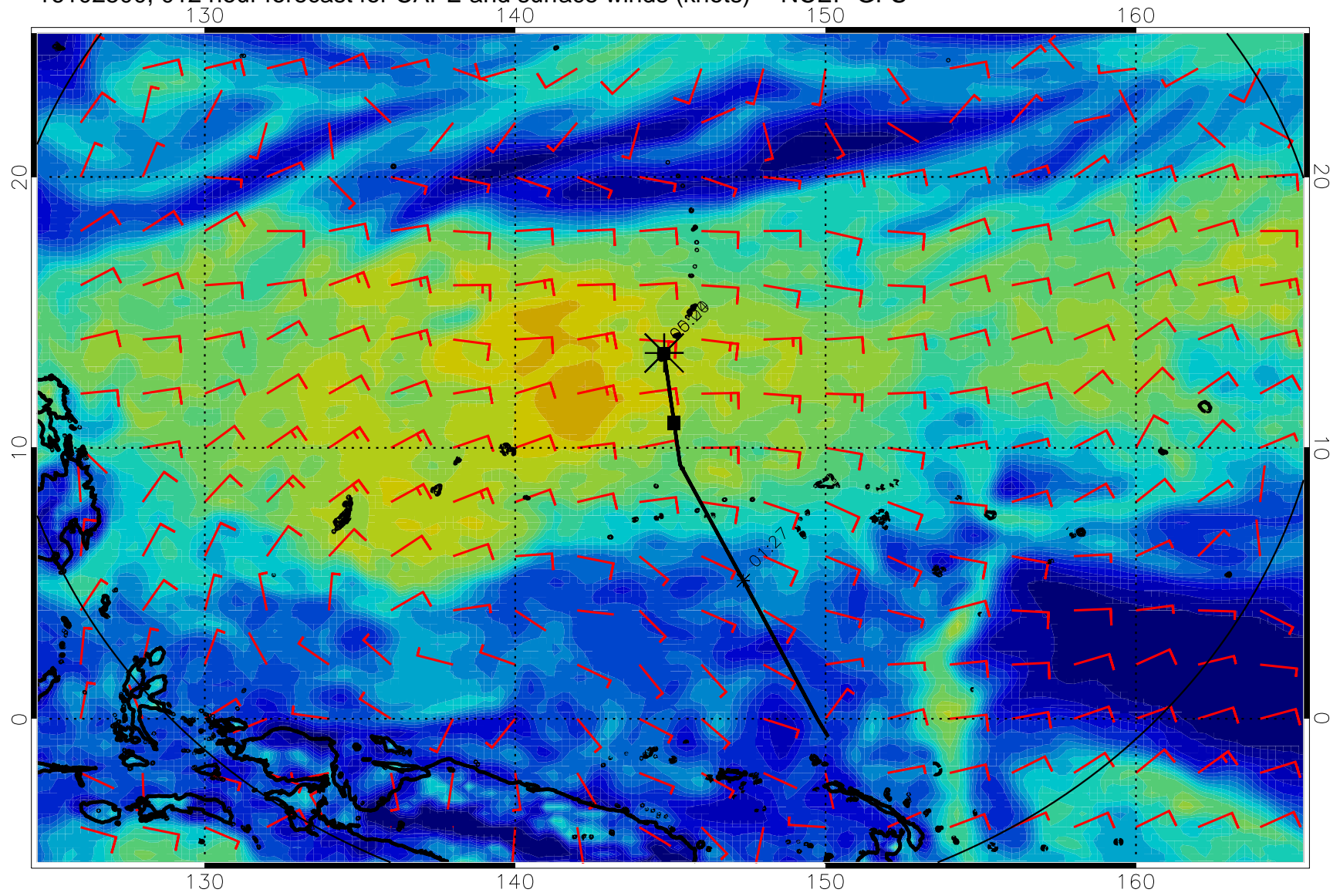
16102500, 012 hour forecast for CAPE and surface winds (knots) -- NCEP GFS
