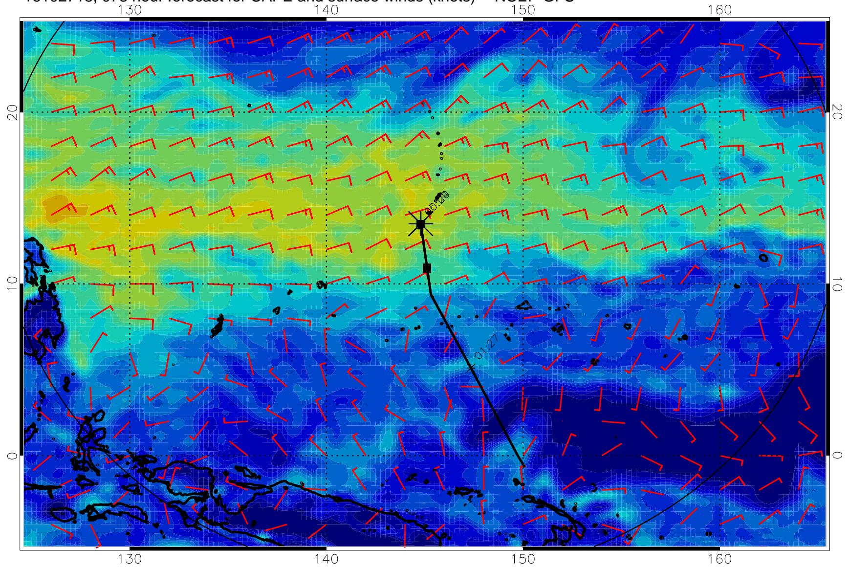
16102718, 078 hour forecast for CAPE and surface winds (knots) -- NCEP GFS
