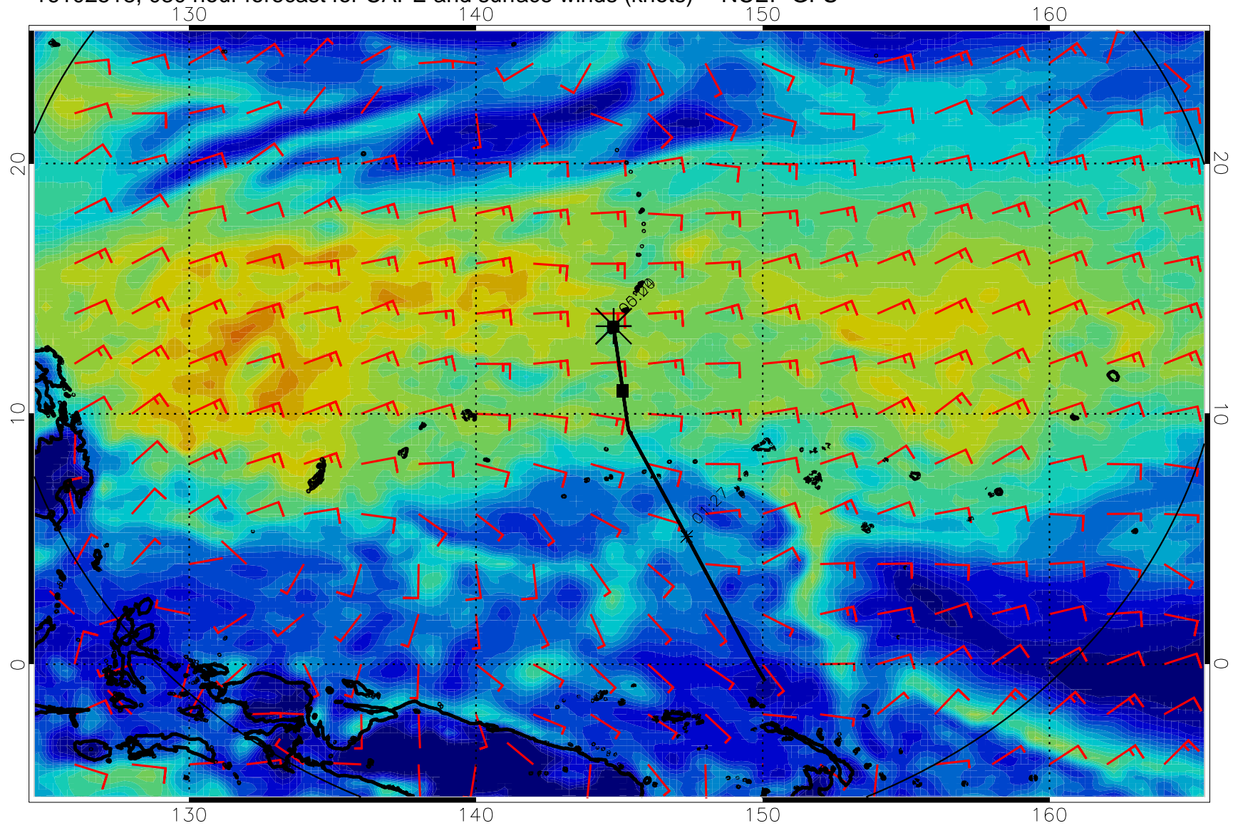
16102518, 030 hour forecast for CAPE and surface winds (knots) -- NCEP GFS
