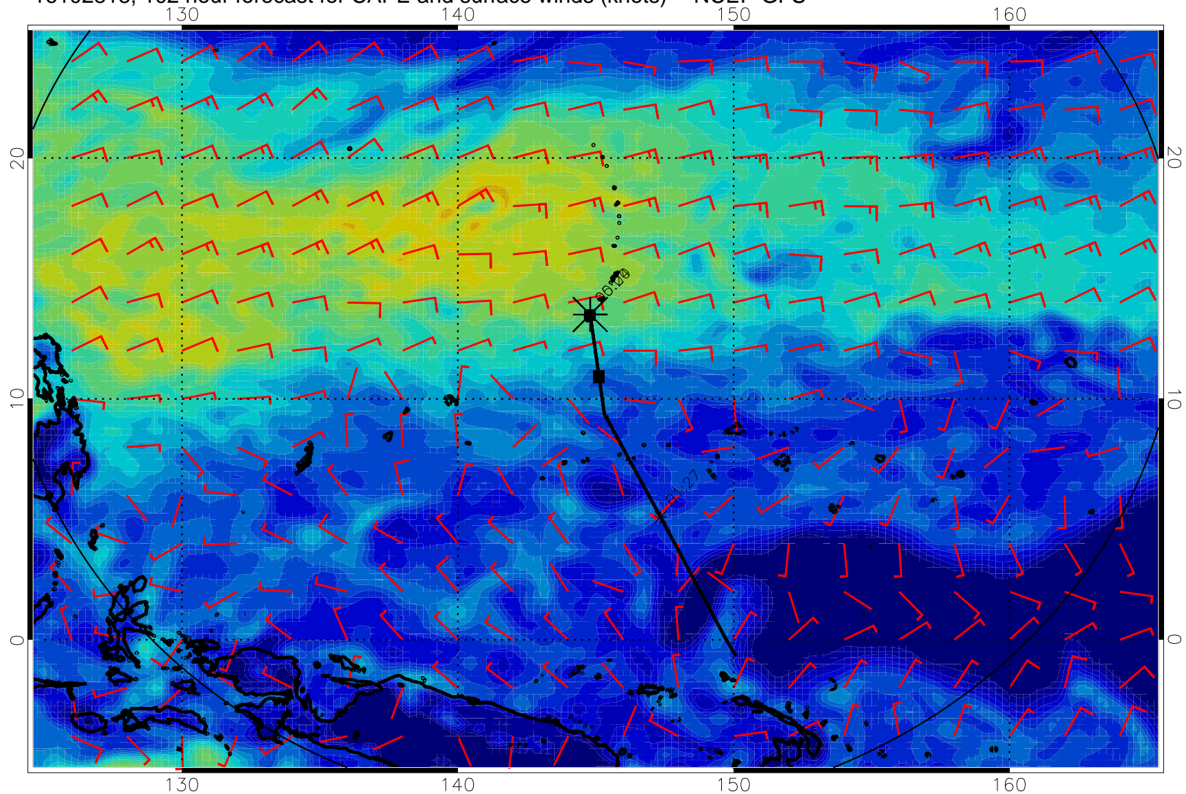
16102818, 102 hour forecast for CAPE and surface winds (knots) -- NCEP GFS
