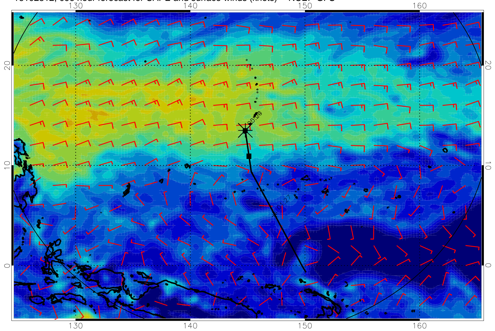
16102812, 096 hour forecast for CAPE and surface winds (knots) -- NCEP GFS
