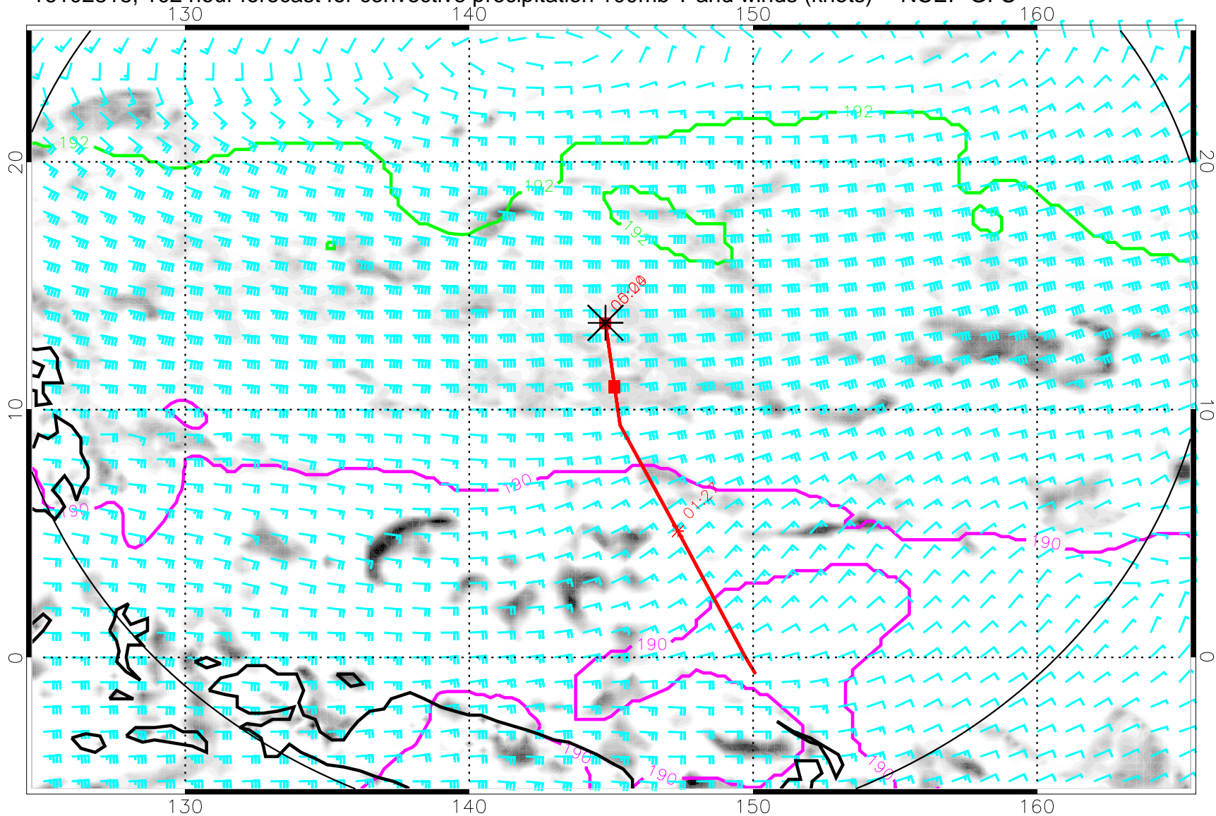
16102818, 102 hour forecast for convective precipitation 100mb T and winds (knots) -- NCEP GFS
