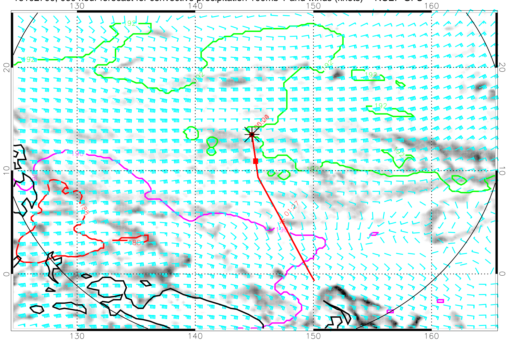
16102700, 060 hour forecast for convective precipitation 100mb T and winds (knots) -- NCEP GFS
