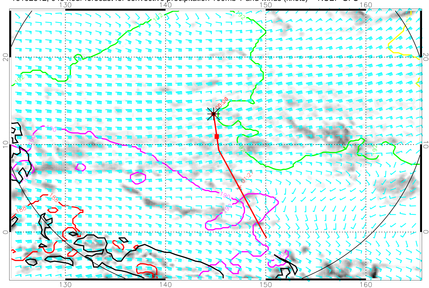
16102612, 048 hour forecast for convective precipitation 100mb T and winds (knots) -- NCEP GFS
