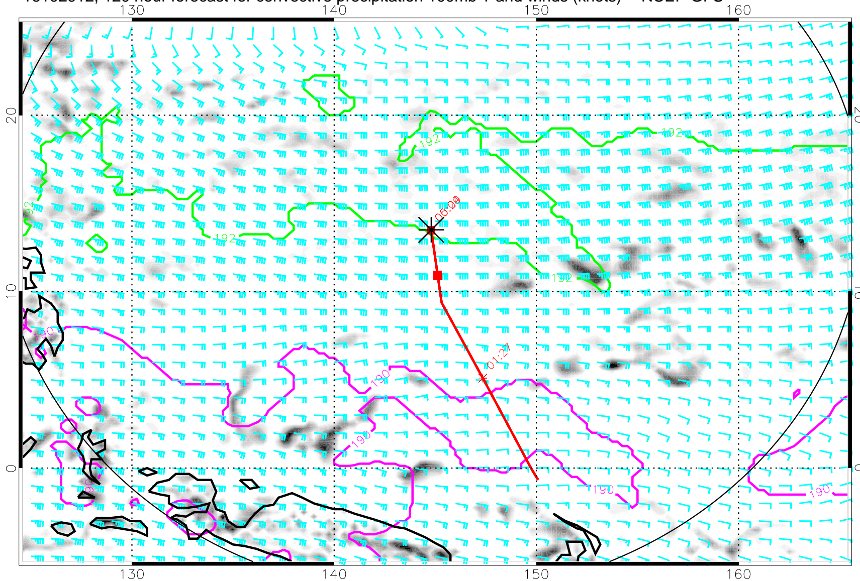
16102912, 120 hour forecast for convective precipitation 100mb T and winds (knots) -- NCEP GFS
