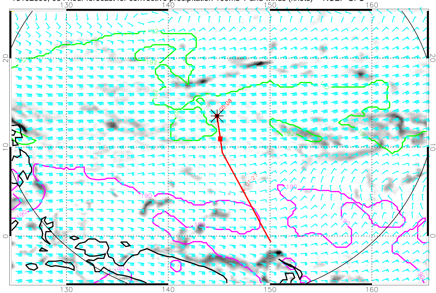
16102800, 084 hour forecast for convective precipitation 100mb T and winds (knots) -- NCEP GFS
