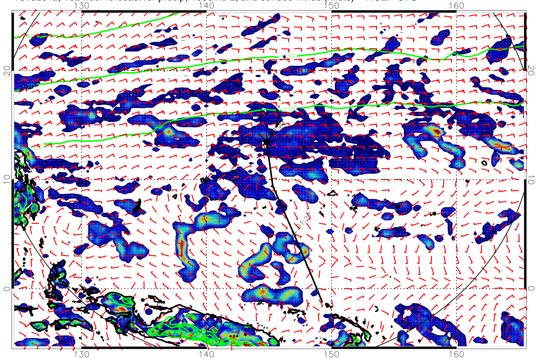
16102812, 102 hour forecast for precip, 1000mb Z, and surface winds (knots) -- NCEP GFS
