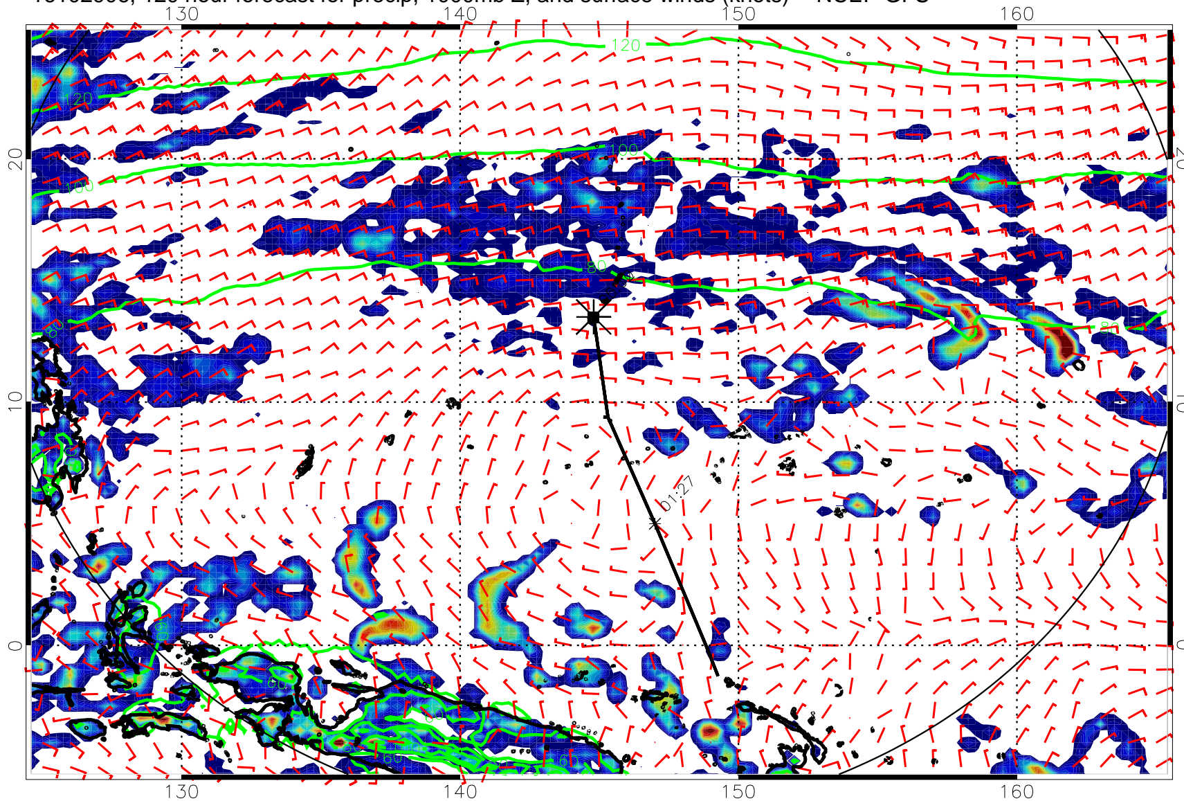
16102906, 120 hour forecast for precip, 1000mb Z, and surface winds (knots) -- NCEP GFS
