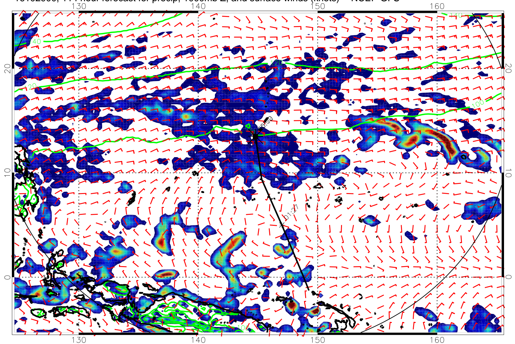
16102900, 114 hour forecast for precip, 1000mb Z, and surface winds (knots) -- NCEP GFS
