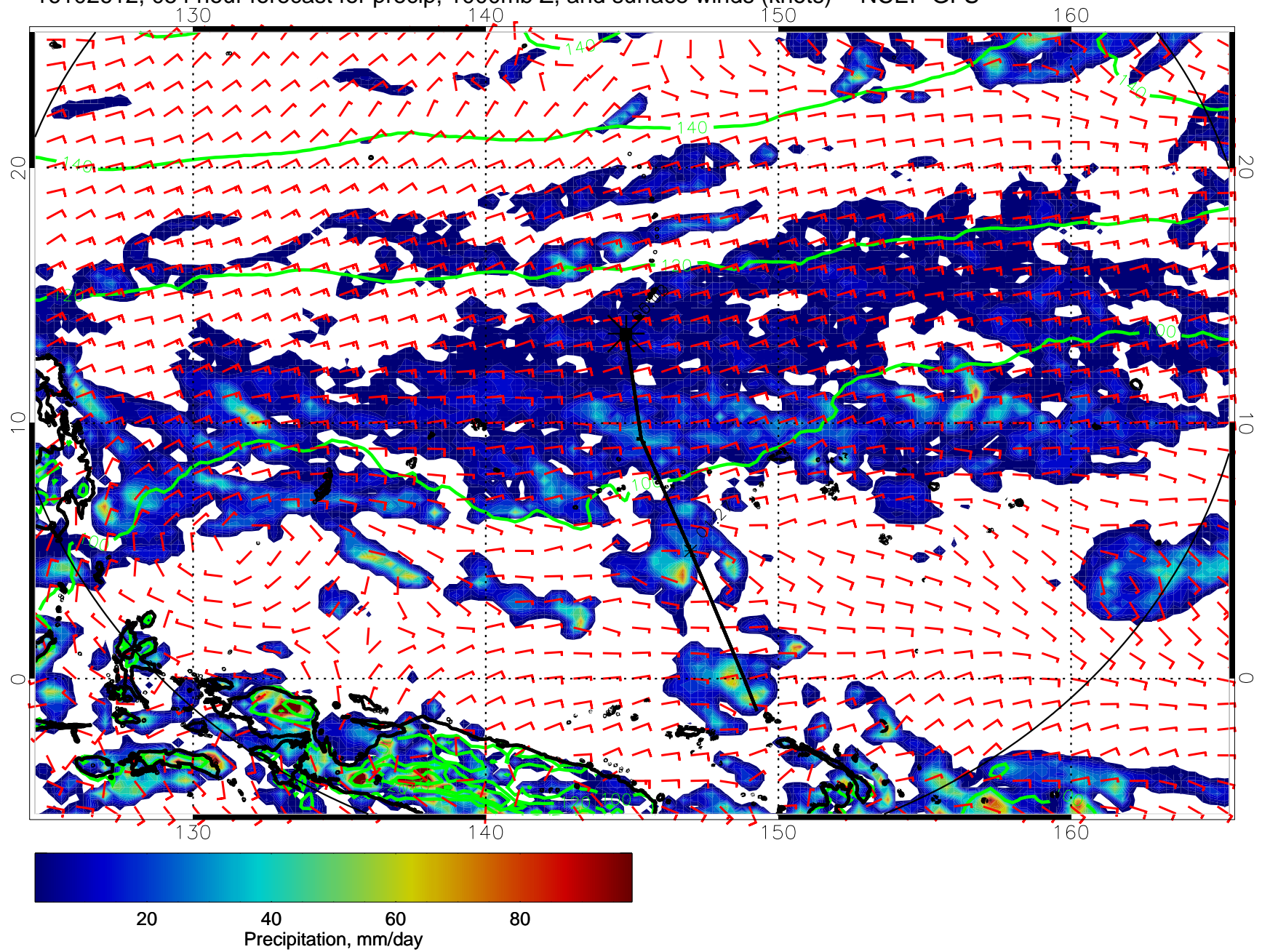
16102612, 054 hour forecast for precip, 1000mb Z, and surface winds (knots) -- NCEP GFS
