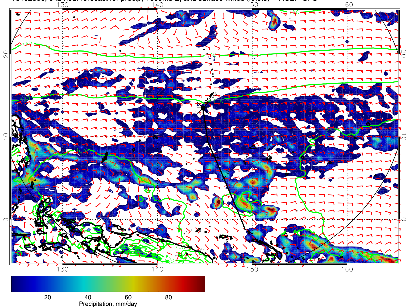
16102600, 042 hour forecast for precip, 1000mb Z, and surface winds (knots) -- NCEP GFS
