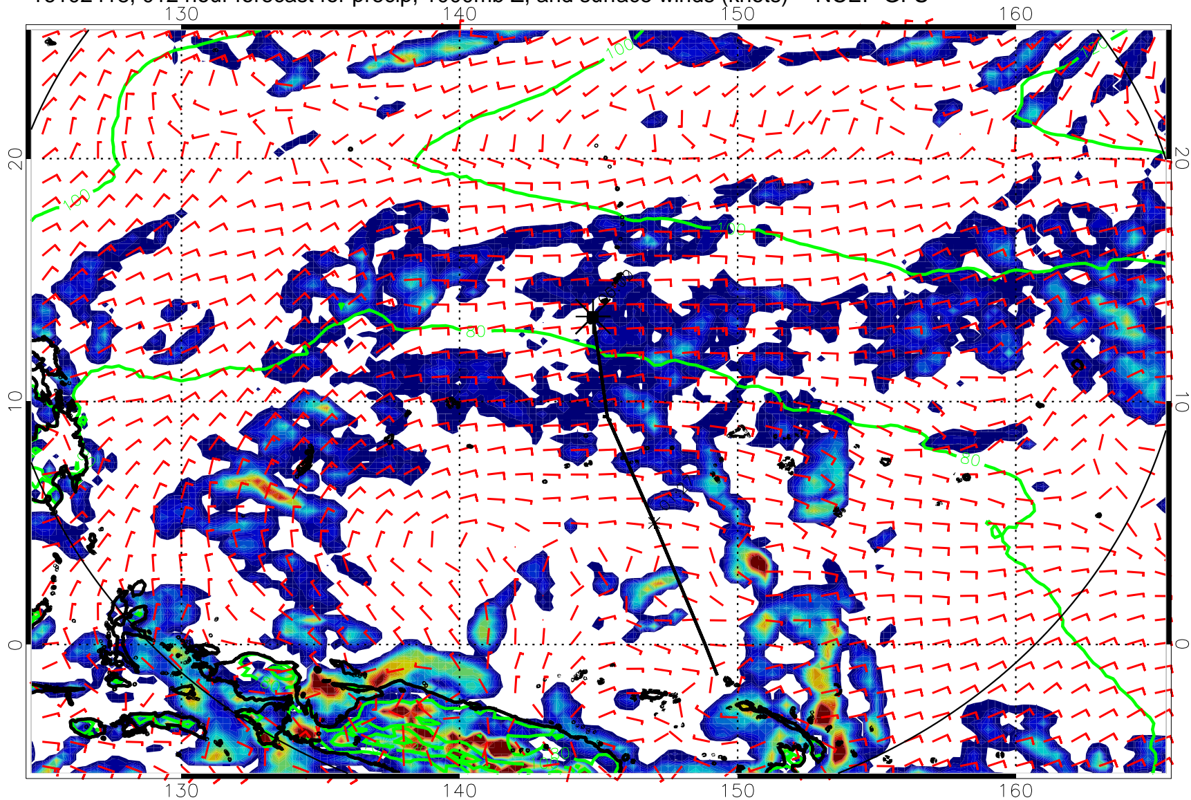
16102418, 012 hour forecast for precip, 1000mb Z, and surface winds (knots) -- NCEP GFS
