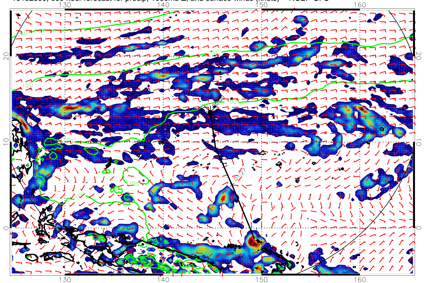
16102800, 090 hour forecast for precip, 1000mb Z, and surface winds (knots) -- NCEP GFS
