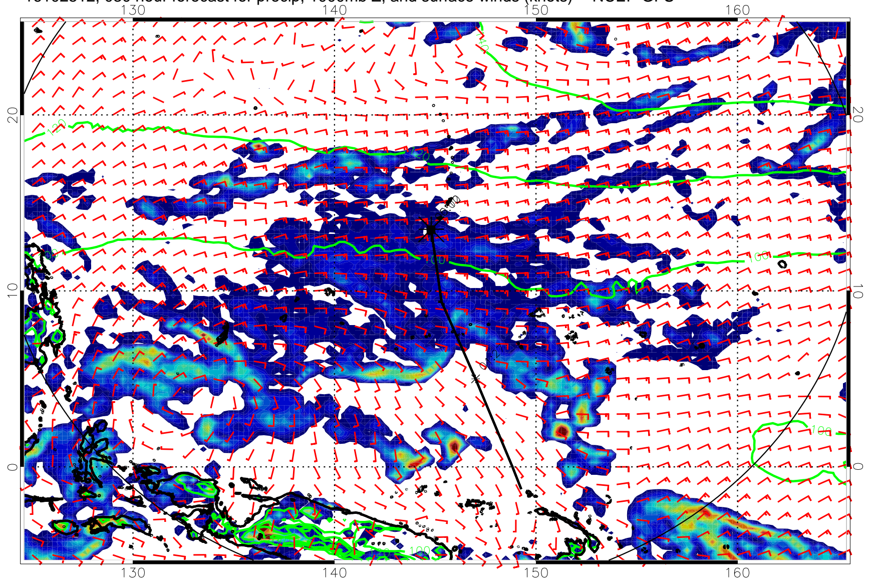
16102512, 030 hour forecast for precip, 1000mb Z, and surface winds (knots) -- NCEP GFS
