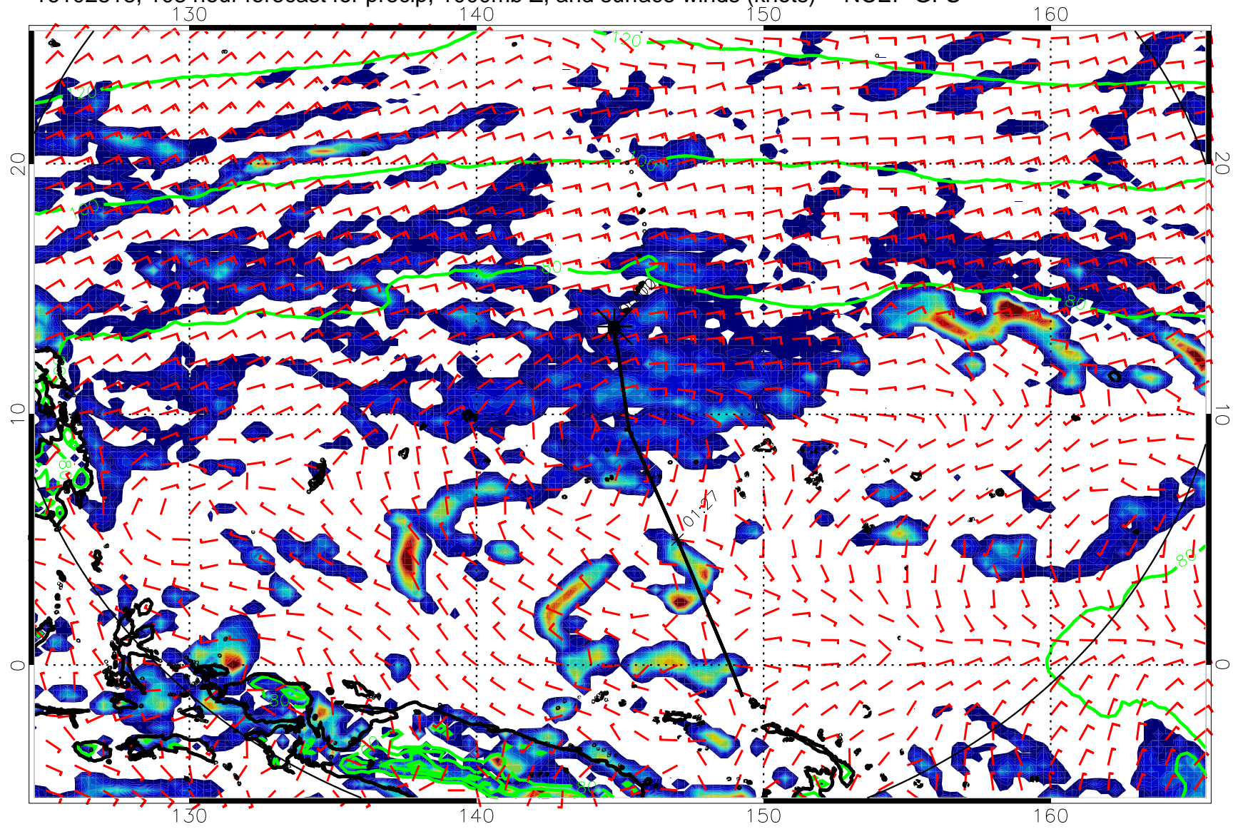
16102818, 108 hour forecast for precip, 1000mb Z, and surface winds (knots) -- NCEP GFS
