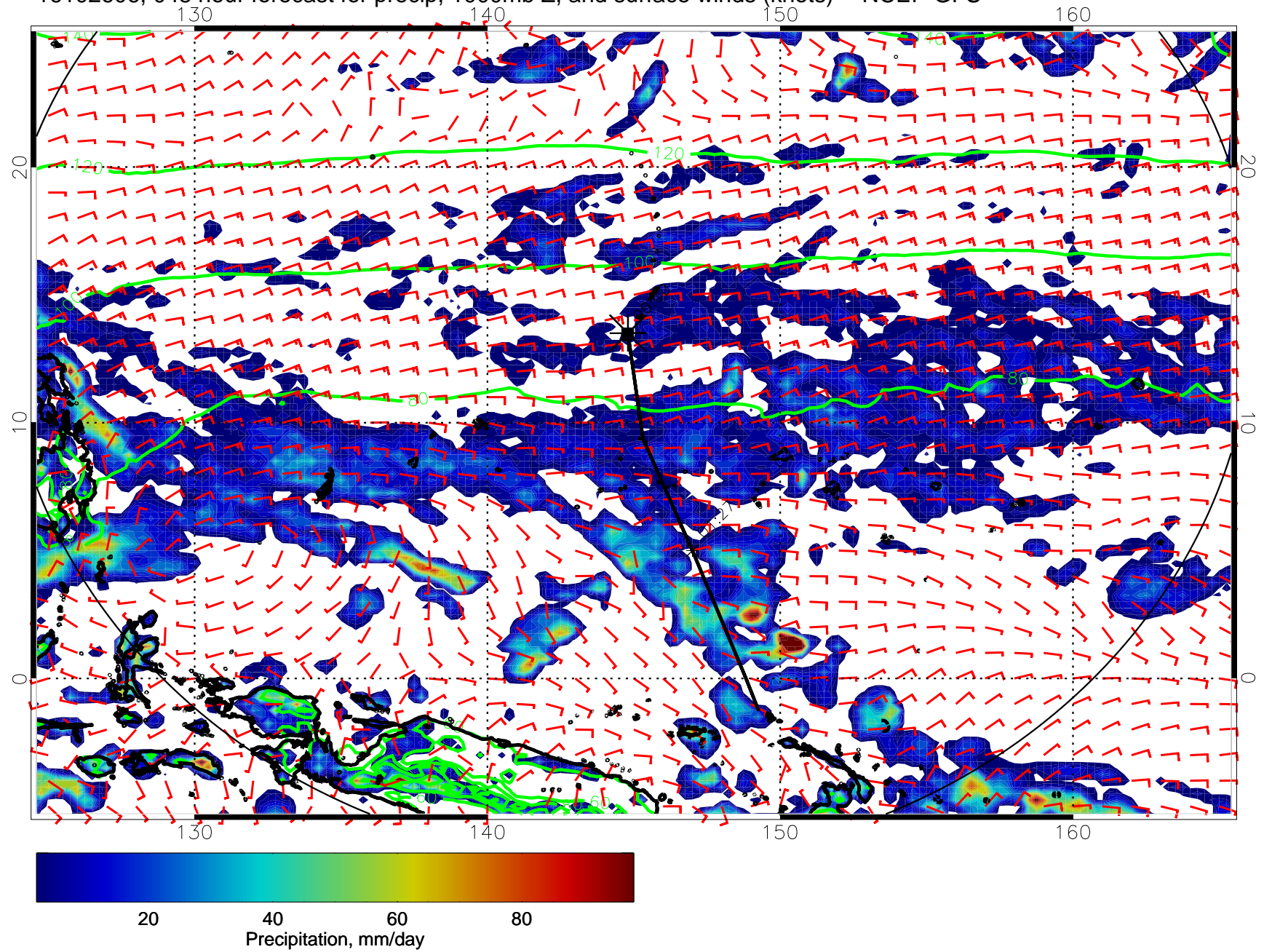
16102606, 048 hour forecast for precip, 1000mb Z, and surface winds (knots) -- NCEP GFS
