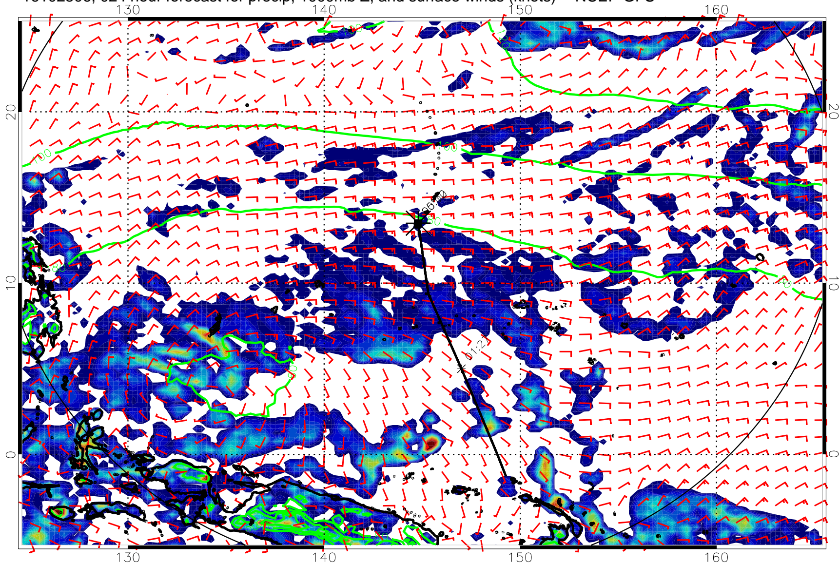
16102506, 024 hour forecast for precip, 1000mb Z, and surface winds (knots) -- NCEP GFS
