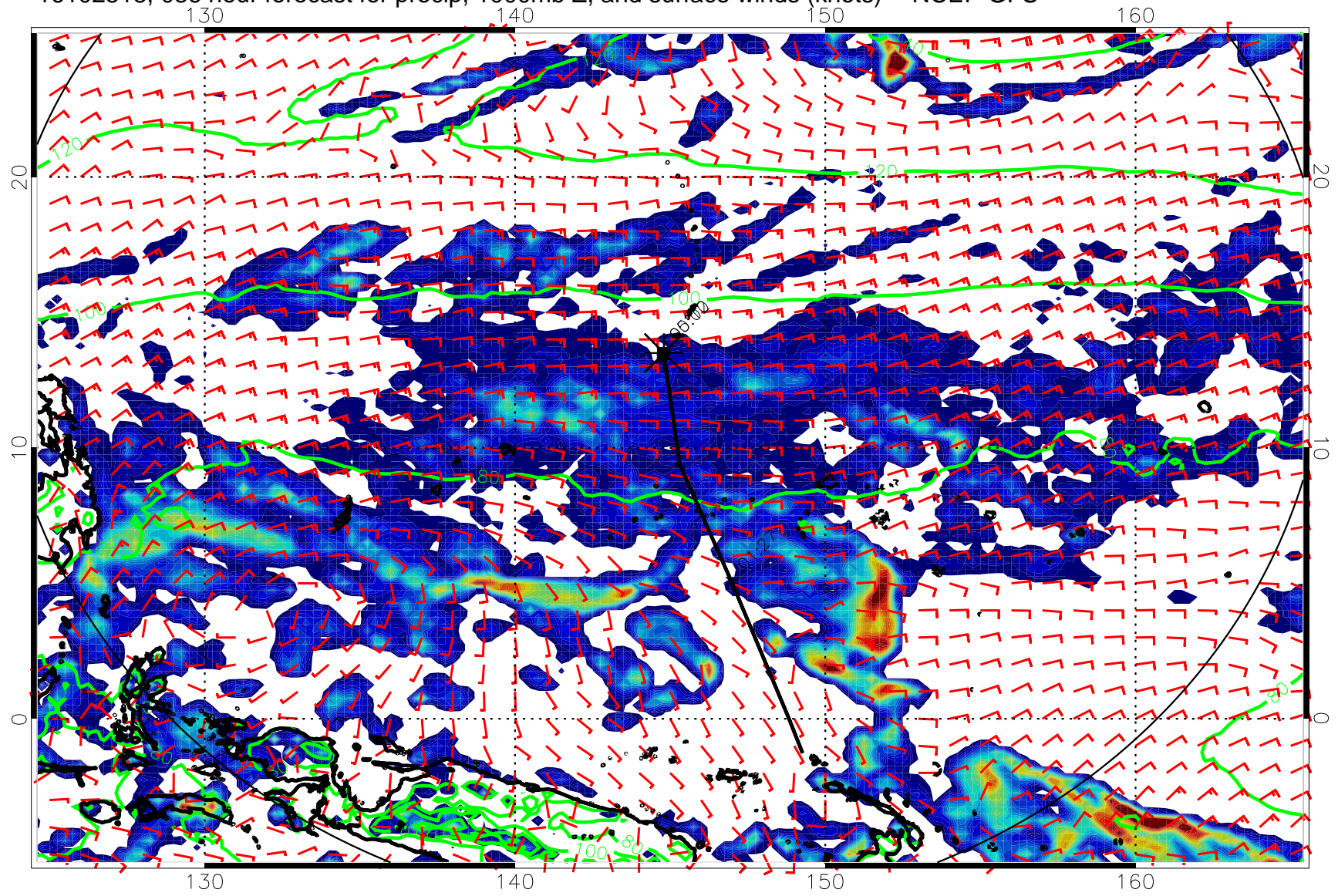
16102518, 036 hour forecast for precip, 1000mb Z, and surface winds (knots) -- NCEP GFS
