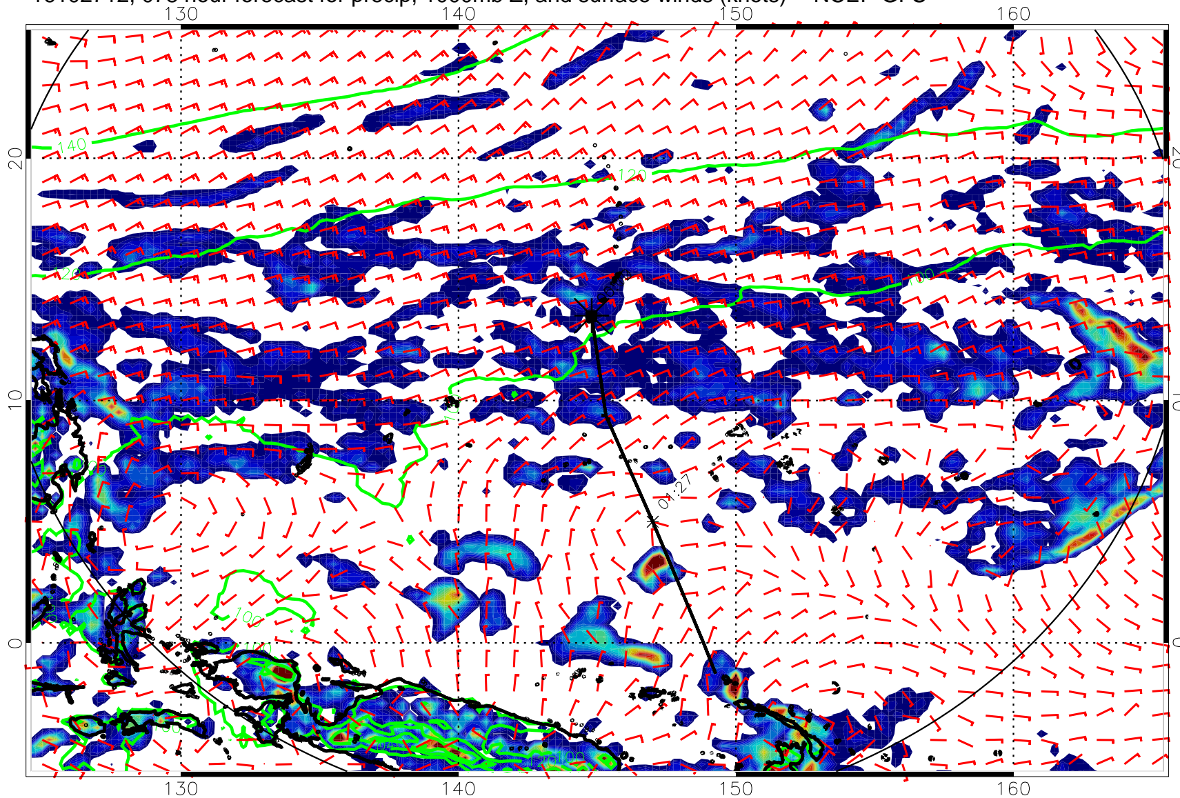
16102712, 078 hour forecast for precip, 1000mb Z, and surface winds (knots) -- NCEP GFS
