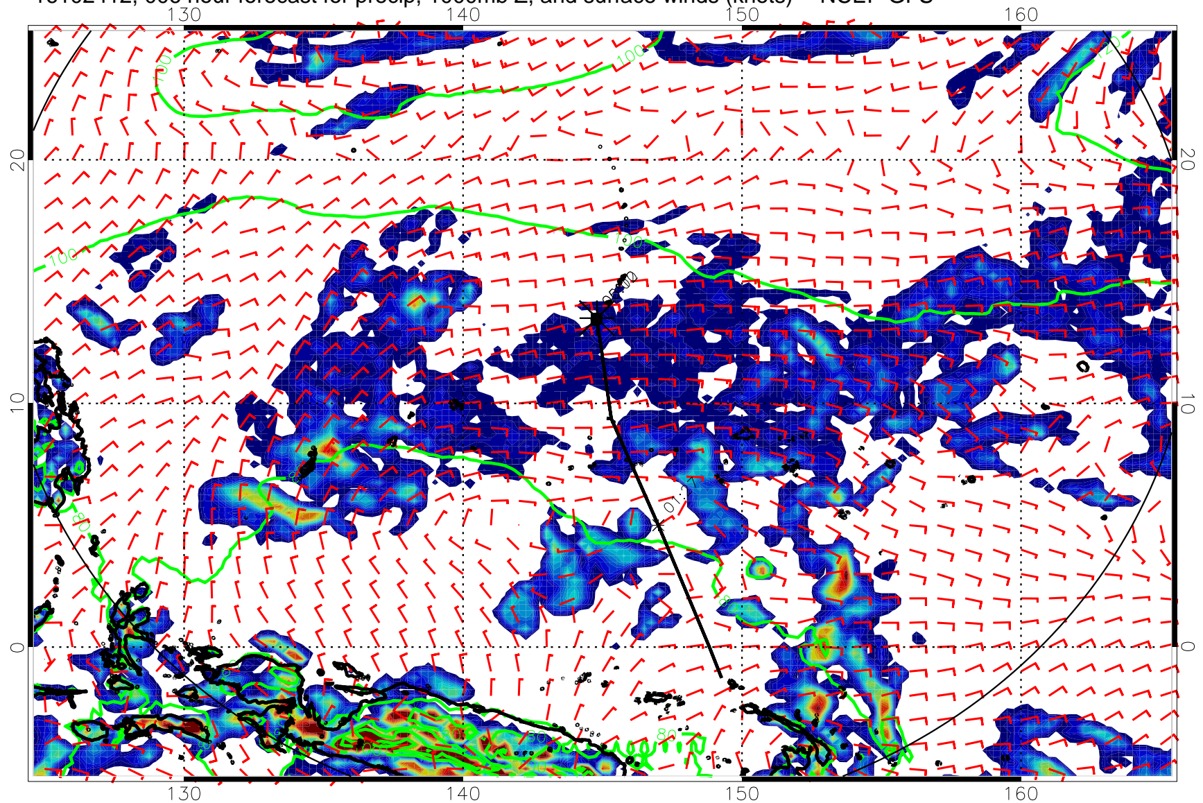
16102412, 006 hour forecast for precip, 1000mb Z, and surface winds (knots) -- NCEP GFS
