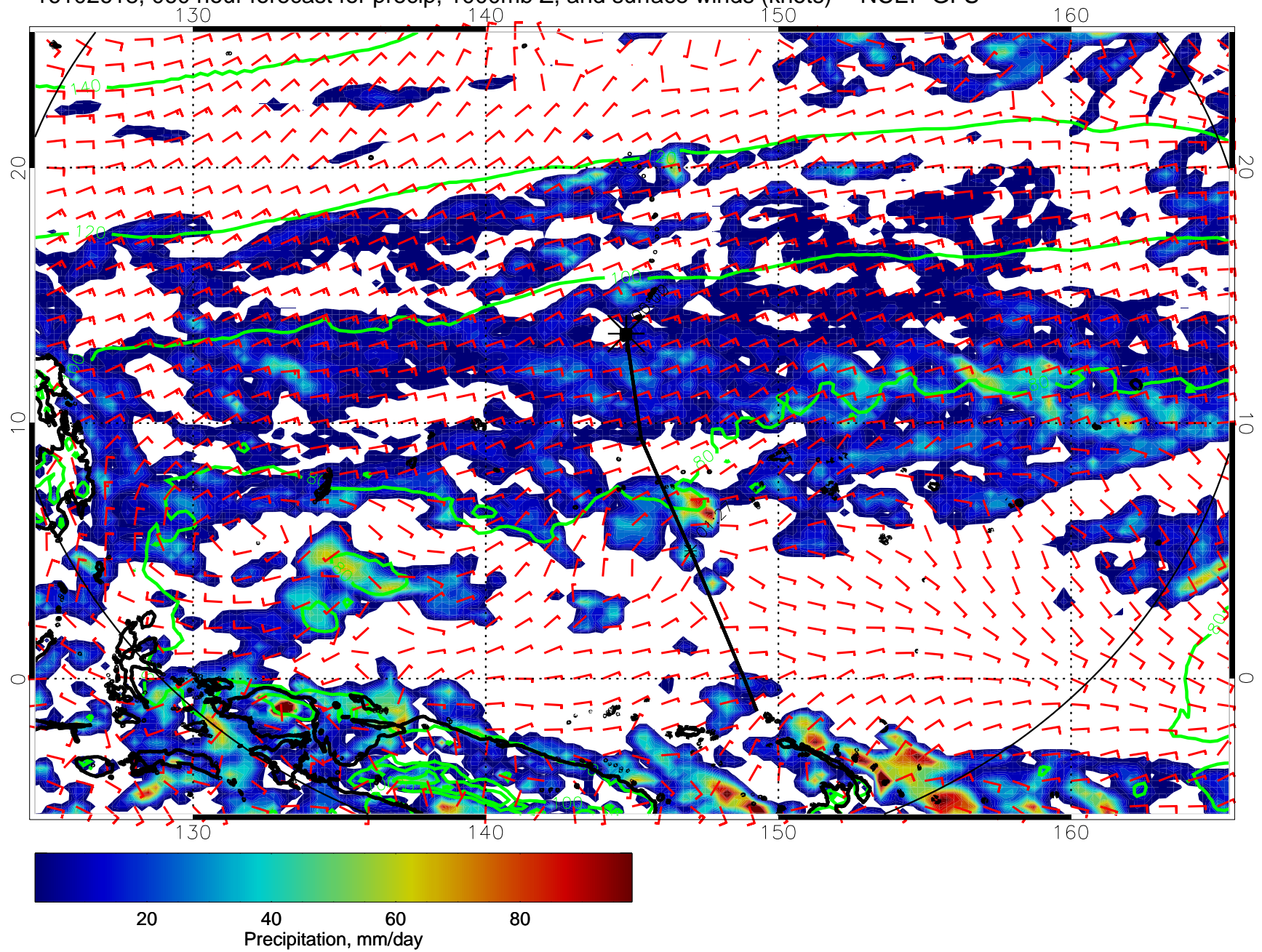
16102618, 060 hour forecast for precip, 1000mb Z, and surface winds (knots) -- NCEP GFS
