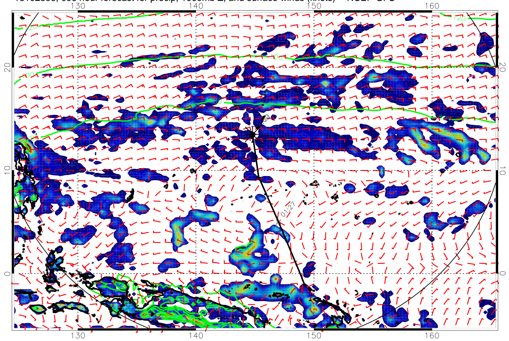
16102806, 096 hour forecast for precip, 1000mb Z, and surface winds (knots) -- NCEP GFS
