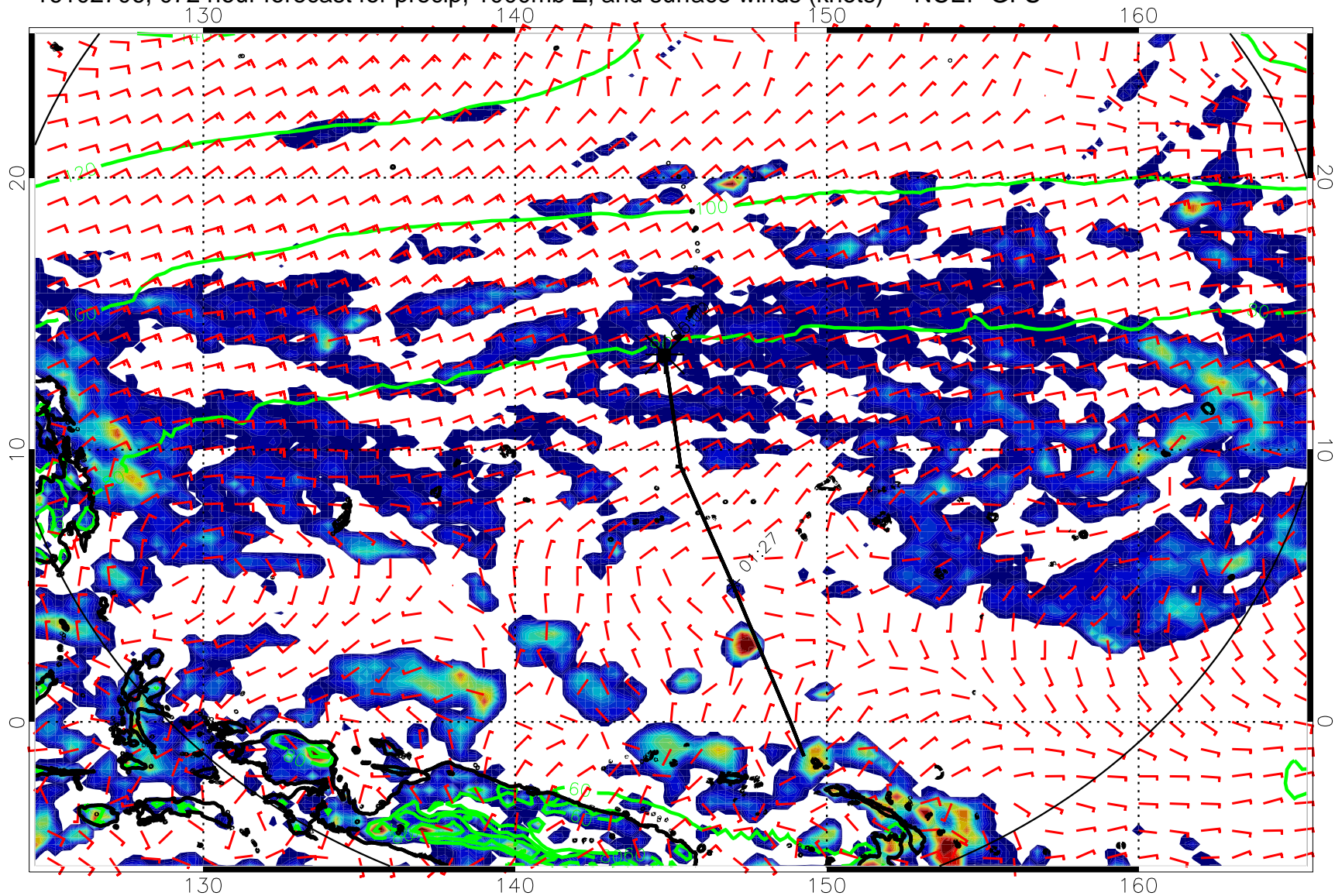
16102706, 072 hour forecast for precip, 1000mb Z, and surface winds (knots) -- NCEP GFS
