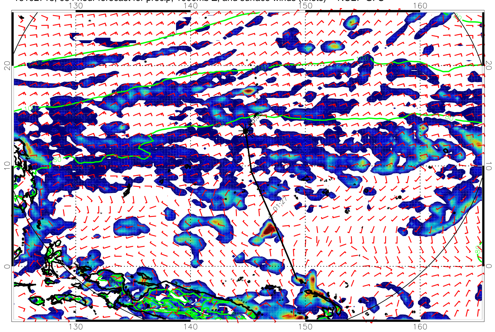
16102718, 084 hour forecast for precip, 1000mb Z, and surface winds (knots) -- NCEP GFS
