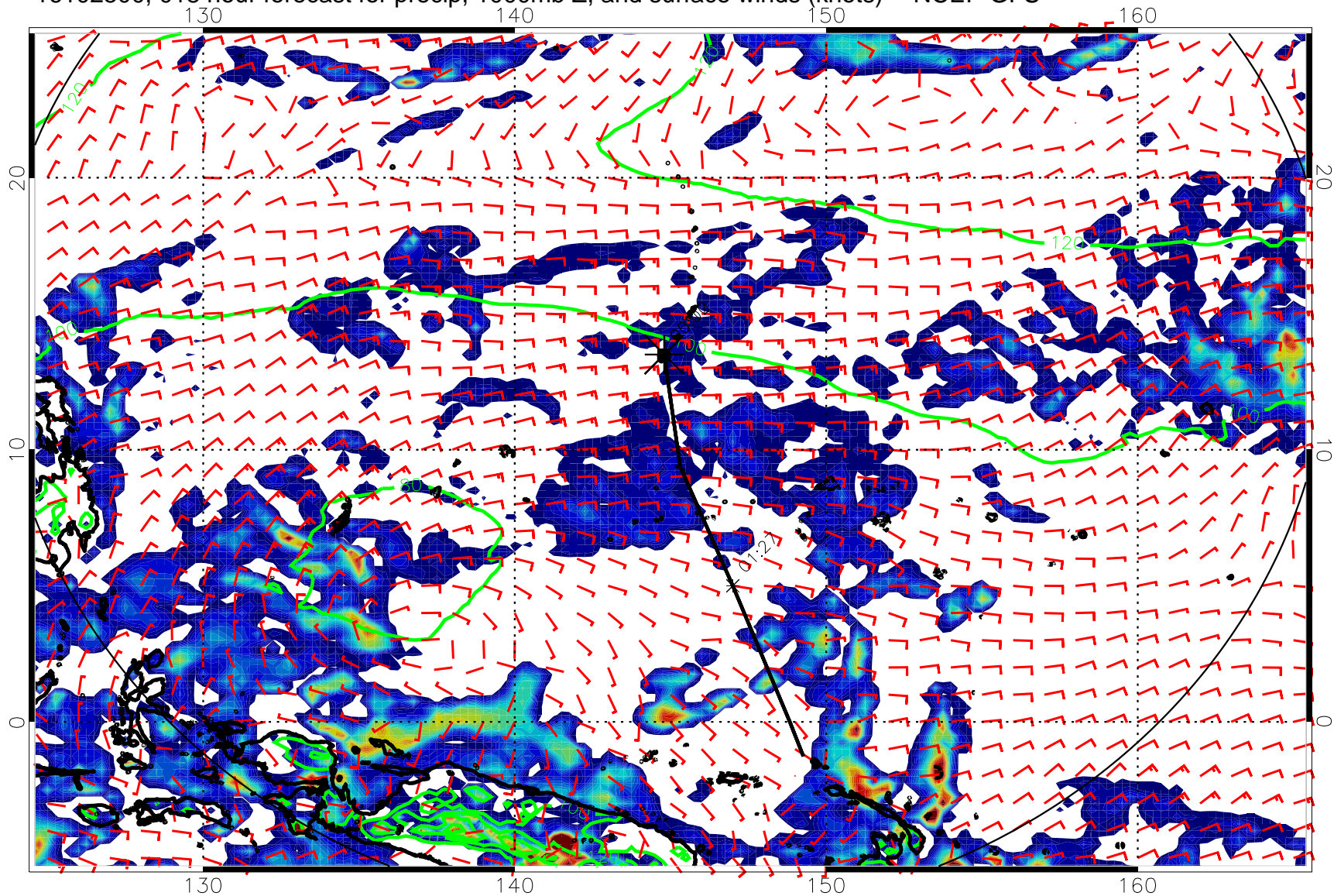
16102500, 018 hour forecast for precip, 1000mb Z, and surface winds (knots) -- NCEP GFS
