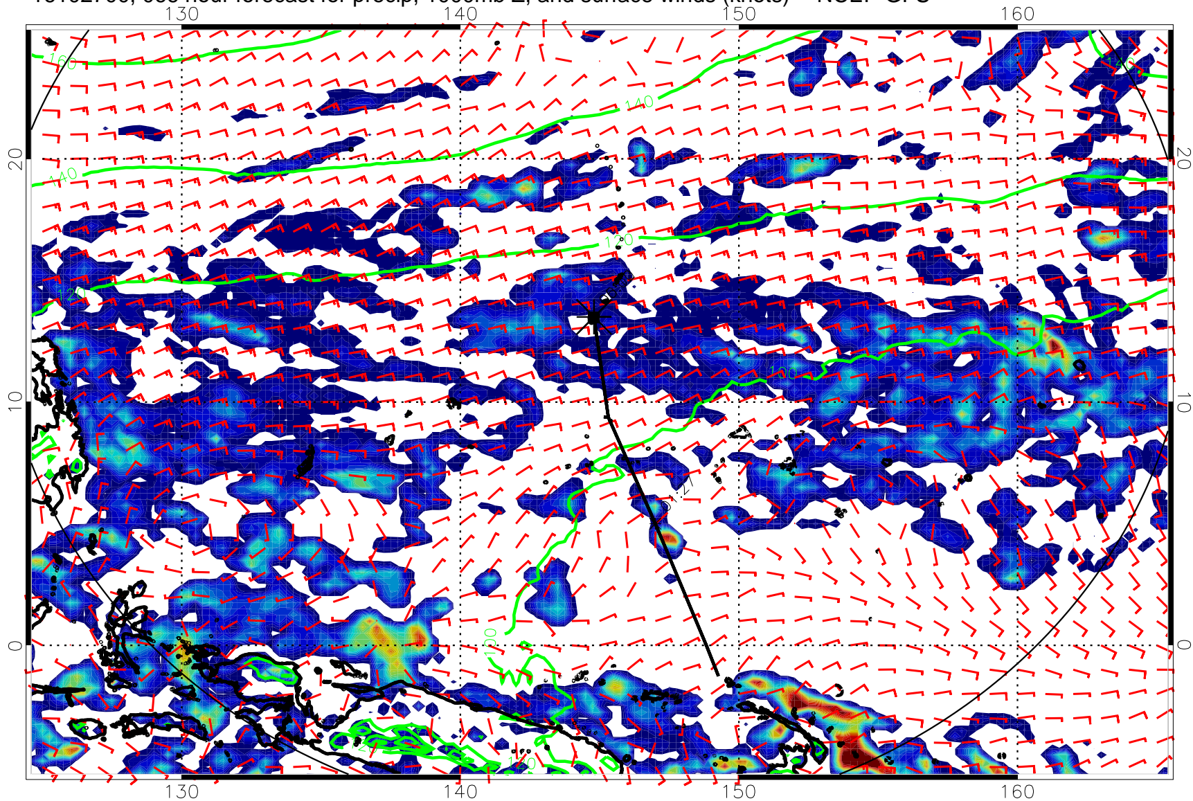
16102700, 066 hour forecast for precip, 1000mb Z, and surface winds (knots) -- NCEP GFS
