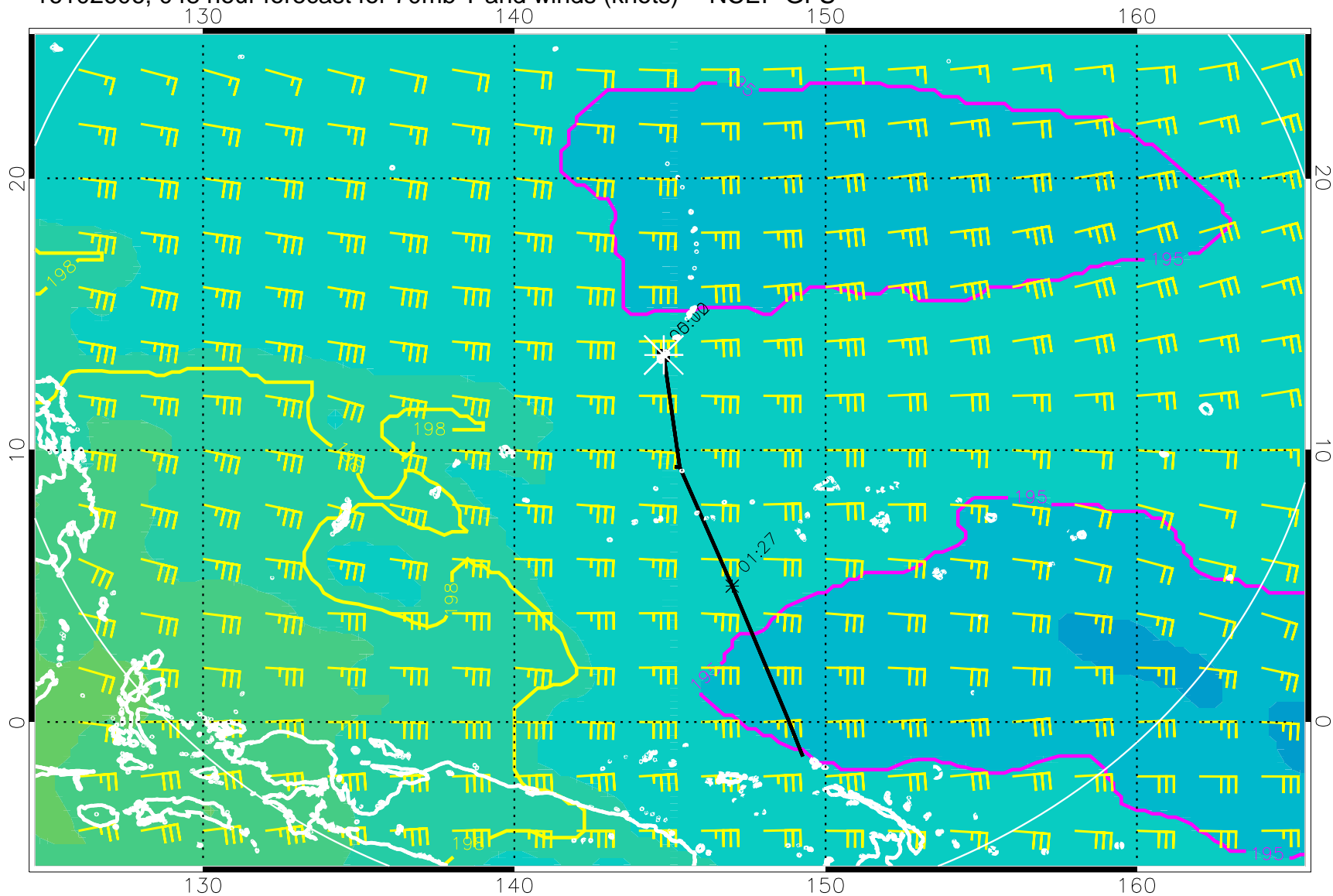
16102606, 048 hour forecast for 70mb T and winds (knots) -- NCEP GFS
