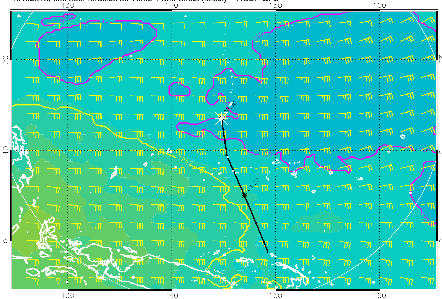
16102618, 060 hour forecast for 70mb T and winds (knots) -- NCEP GFS
