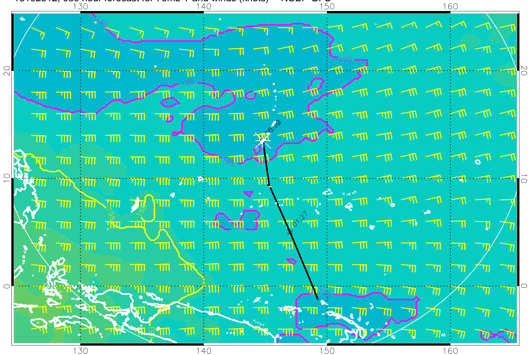
16102512, 030 hour forecast for 70mb T and winds (knots) -- NCEP GFS
