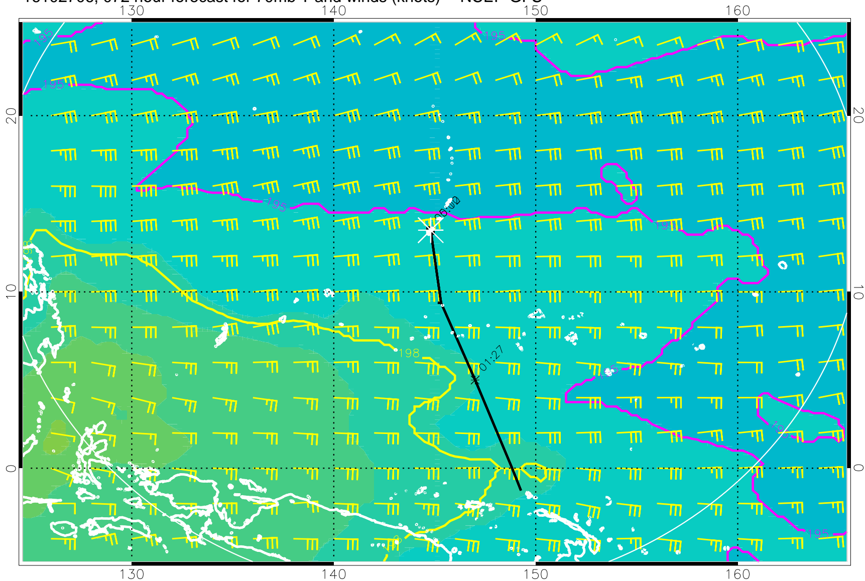
16102706, 072 hour forecast for 70mb T and winds (knots) -- NCEP GFS
