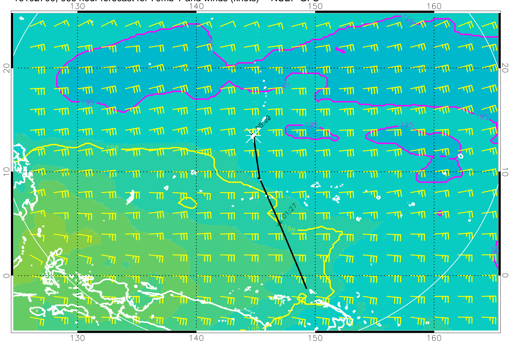
16102700, 066 hour forecast for 70mb T and winds (knots) -- NCEP GFS
