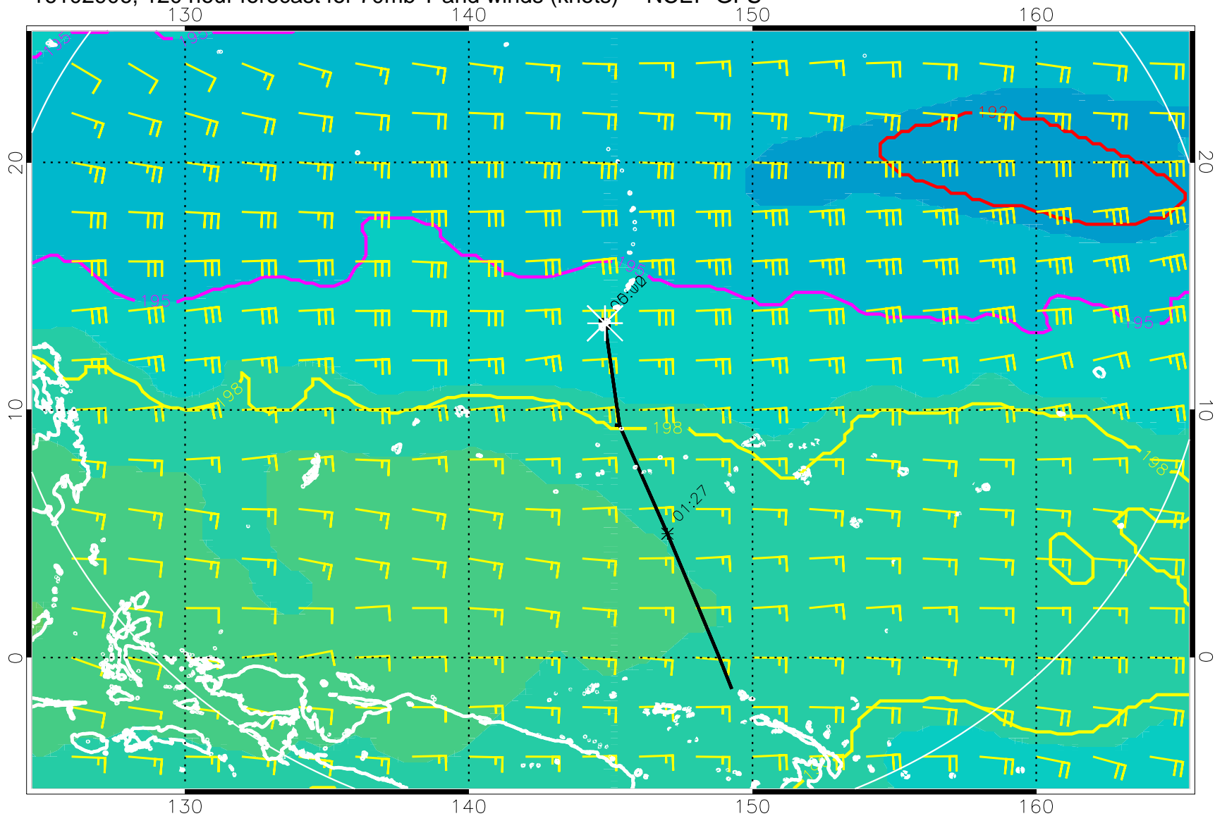
16102906, 120 hour forecast for 70mb T and winds (knots) -- NCEP GFS
