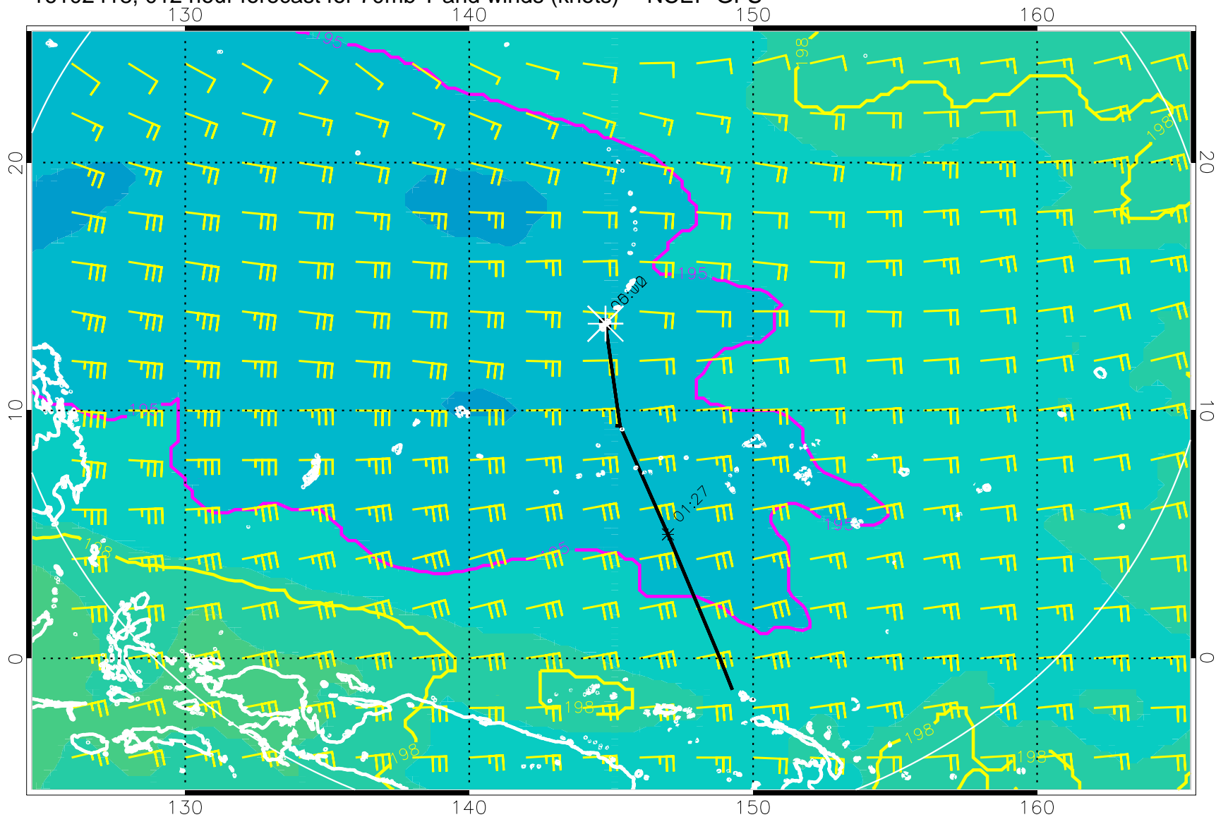
16102418, 012 hour forecast for 70mb T and winds (knots) -- NCEP GFS
