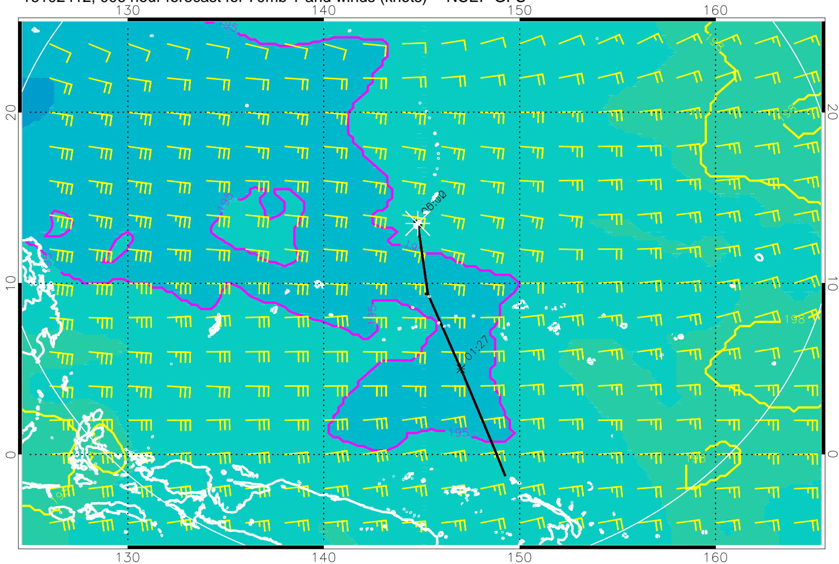
16102412, 006 hour forecast for 70mb T and winds (knots) -- NCEP GFS
