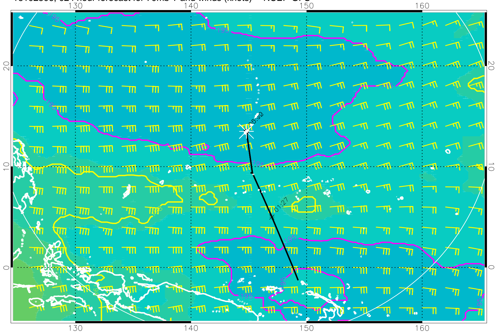
16102506, 024 hour forecast for 70mb T and winds (knots) -- NCEP GFS
