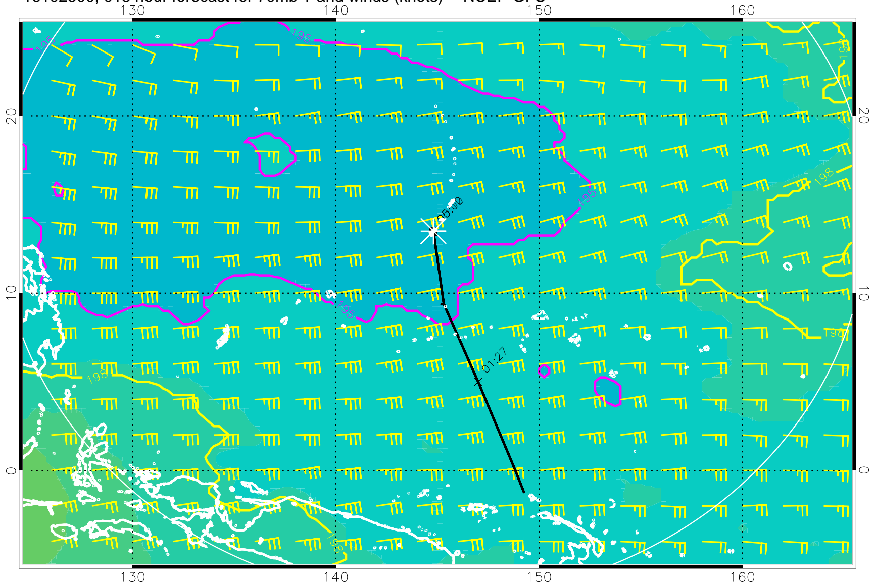
16102500, 018 hour forecast for 70mb T and winds (knots) -- NCEP GFS
