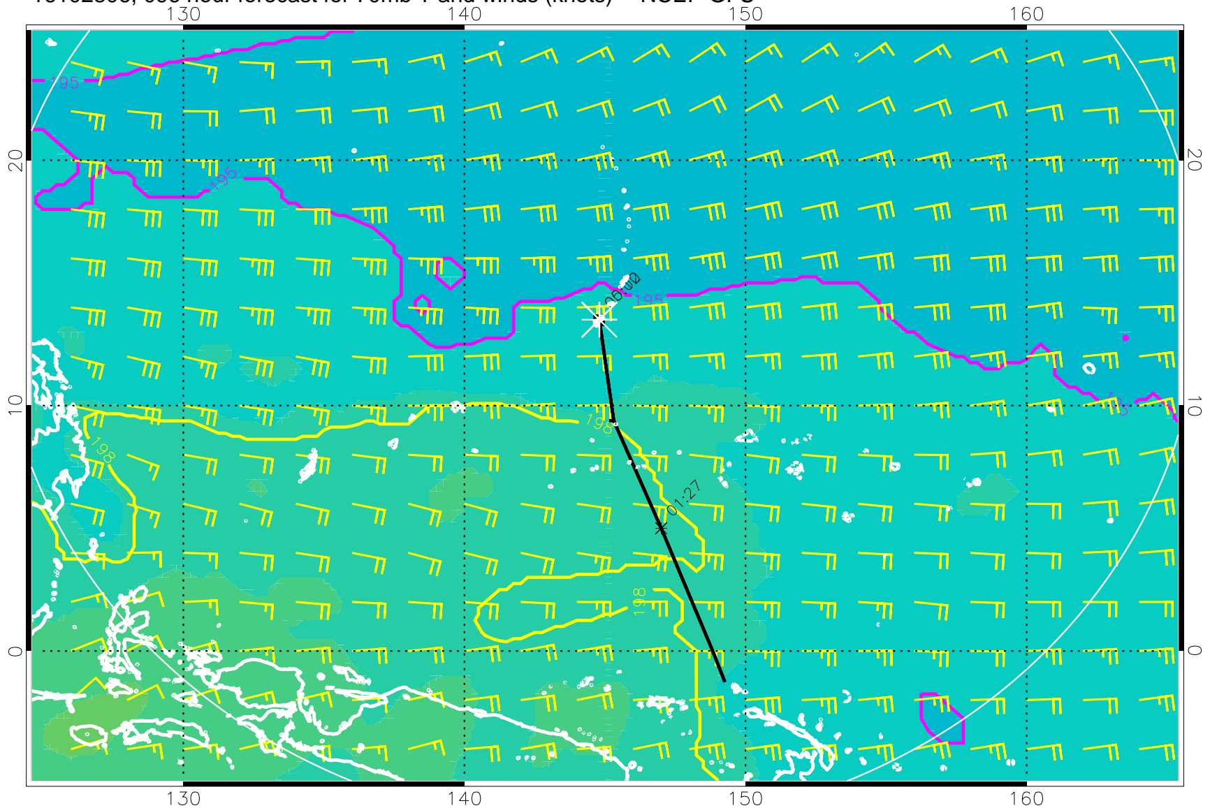
16102806, 096 hour forecast for 70mb T and winds (knots) -- NCEP GFS
