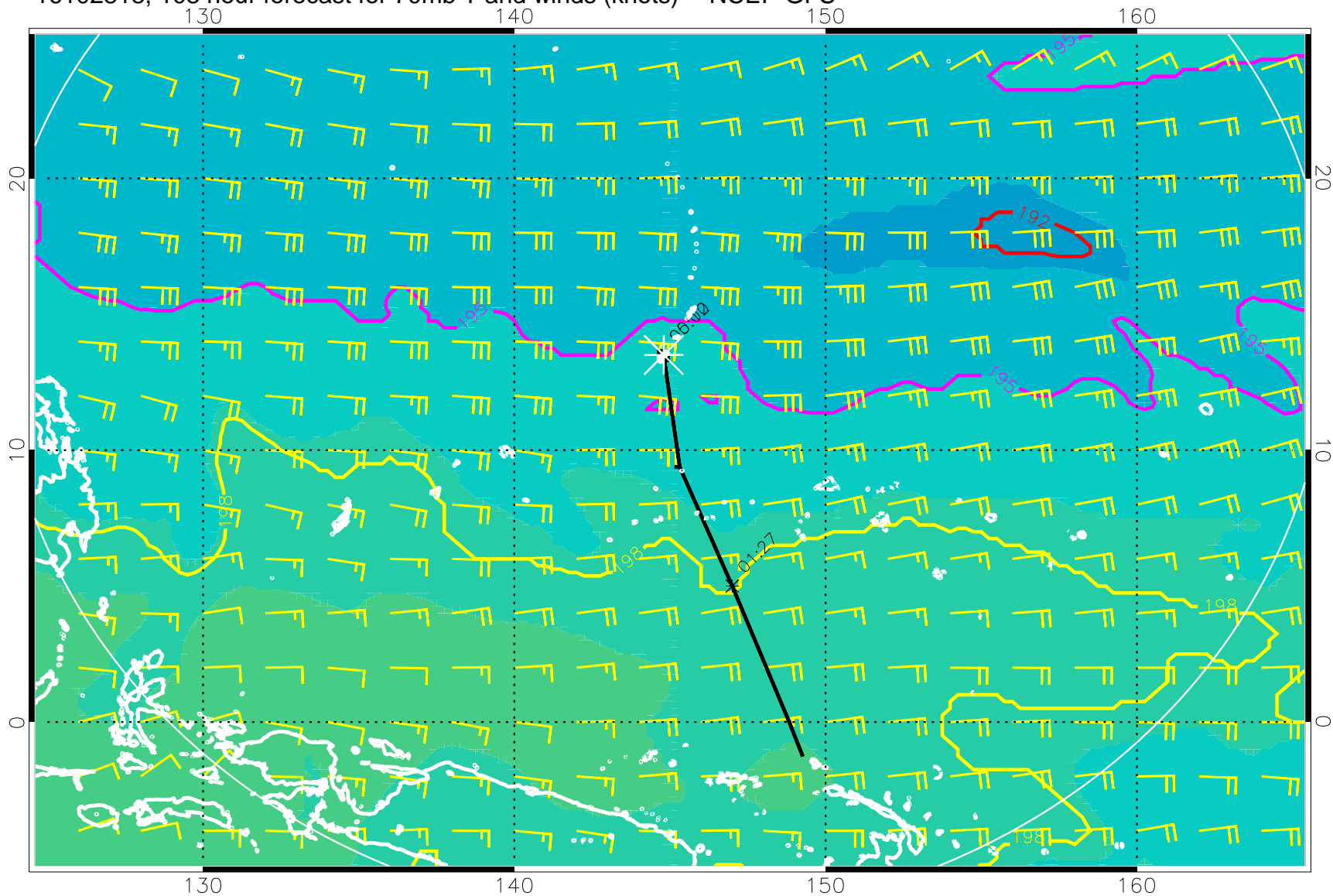
16102818, 108 hour forecast for 70mb T and winds (knots) -- NCEP GFS
