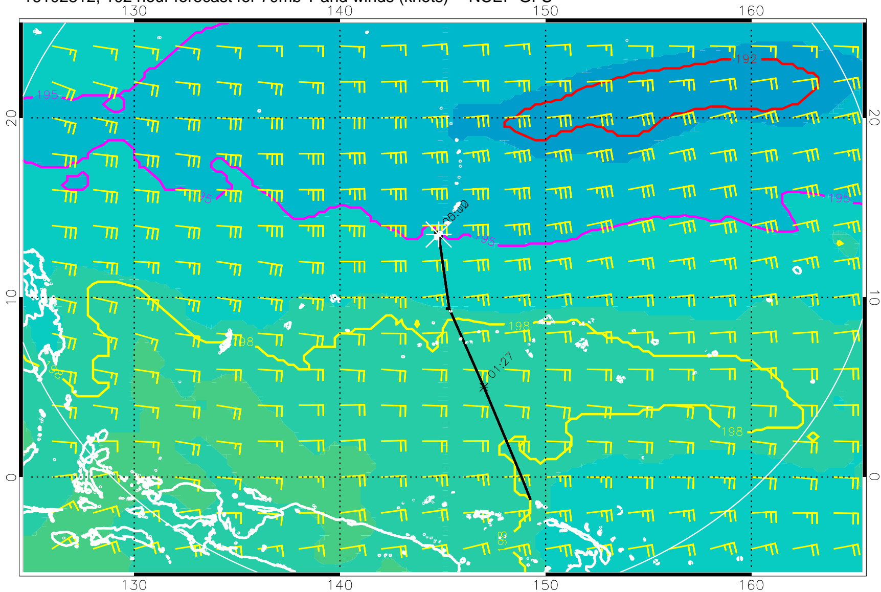
16102812, 102 hour forecast for 70mb T and winds (knots) -- NCEP GFS
