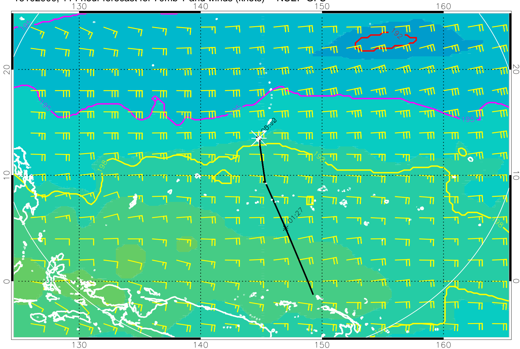
16102900, 114 hour forecast for 70mb T and winds (knots) -- NCEP GFS
