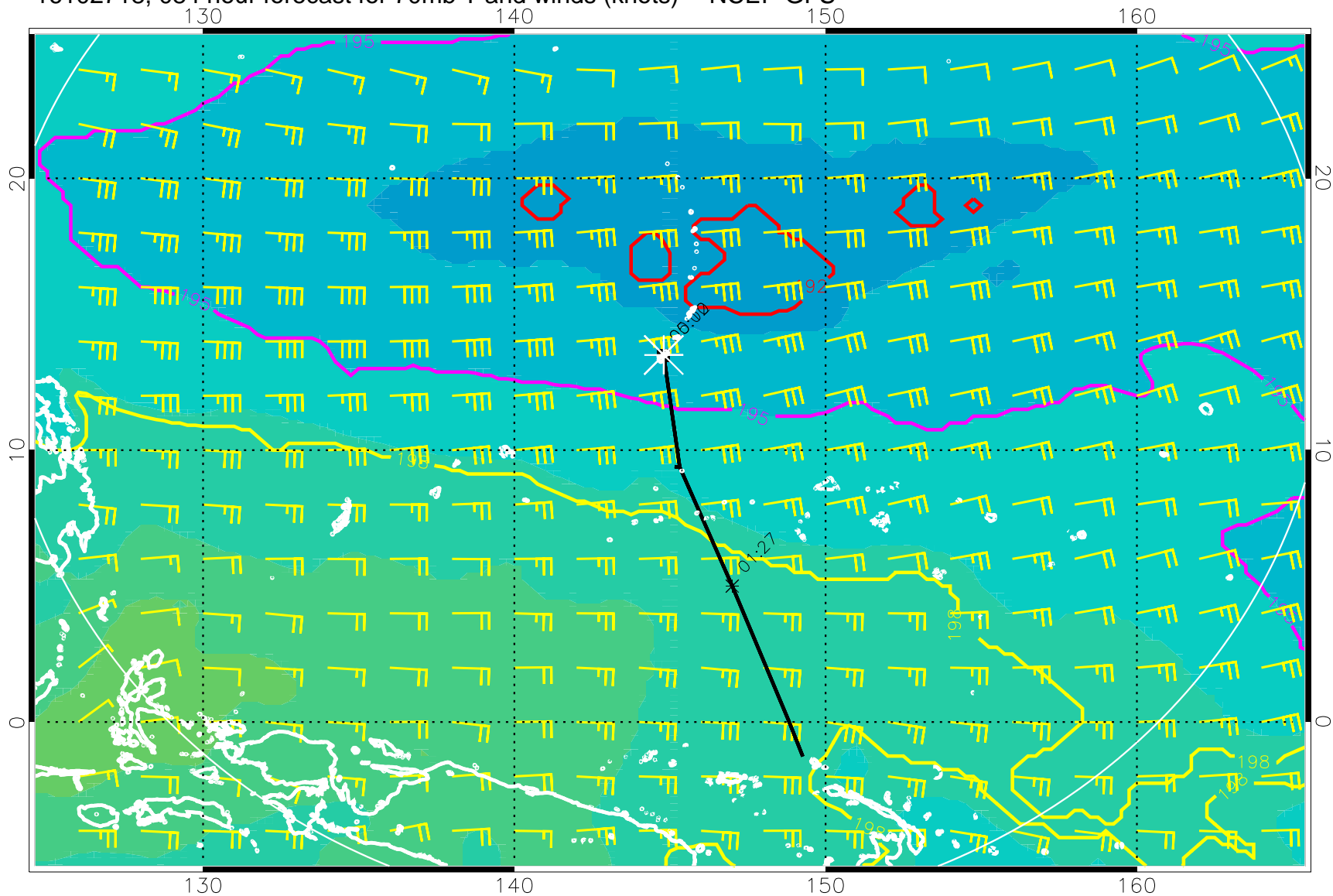
16102718, 084 hour forecast for 70mb T and winds (knots) -- NCEP GFS
