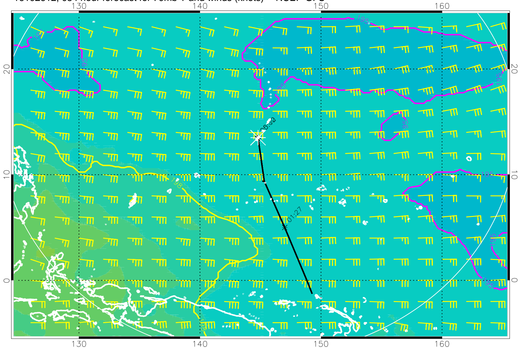
16102612, 054 hour forecast for 70mb T and winds (knots) -- NCEP GFS
