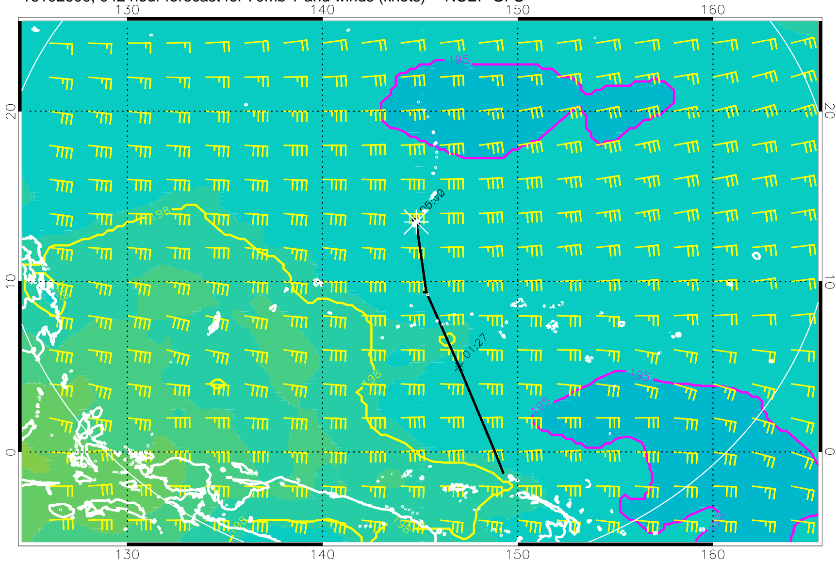
16102600, 042 hour forecast for 70mb T and winds (knots) -- NCEP GFS
