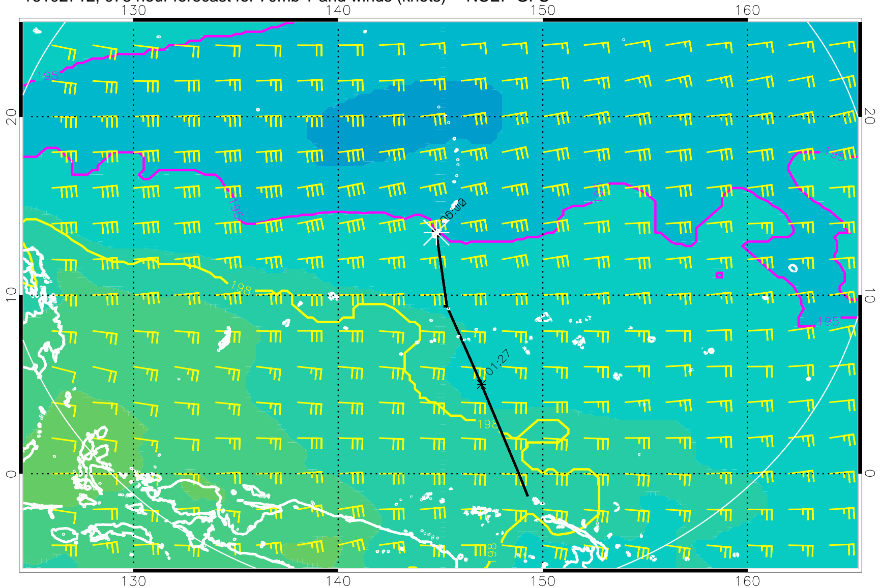
16102712, 078 hour forecast for 70mb T and winds (knots) -- NCEP GFS
