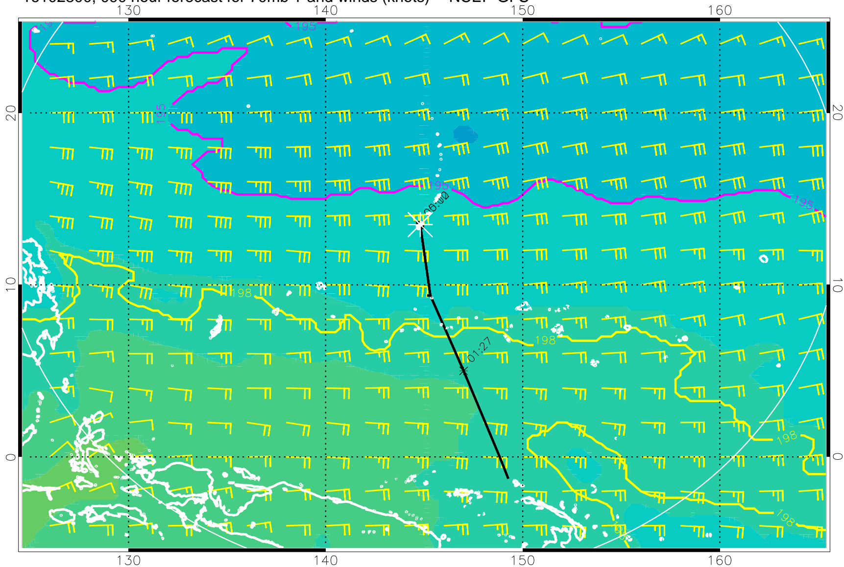
16102800, 090 hour forecast for 70mb T and winds (knots) -- NCEP GFS
