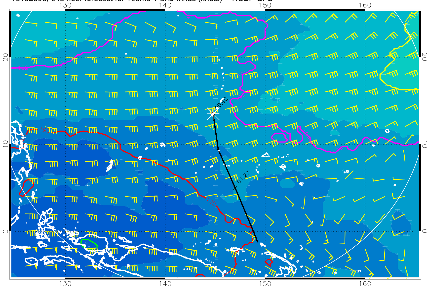
16102606, 048 hour forecast for 100mb T and winds (knots) -- NCEP GFS
