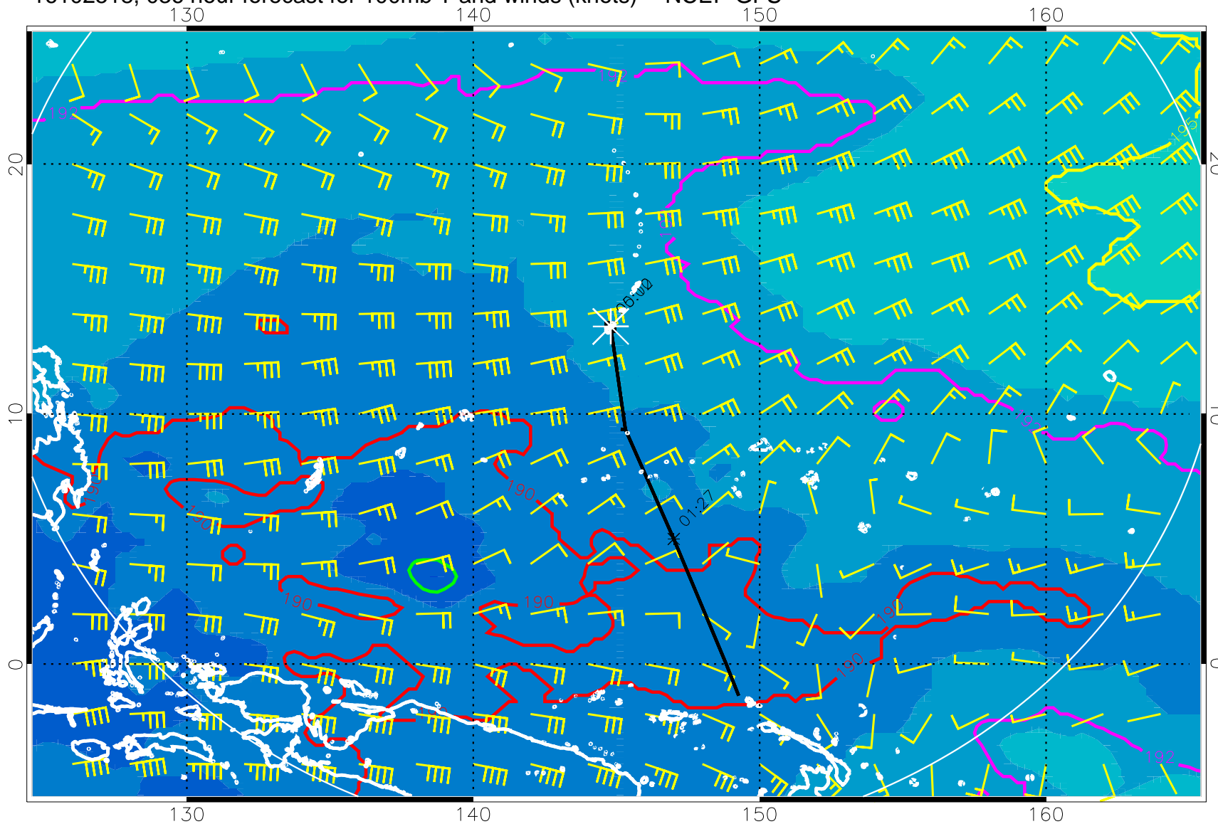
16102518, 036 hour forecast for 100mb T and winds (knots) -- NCEP GFS
