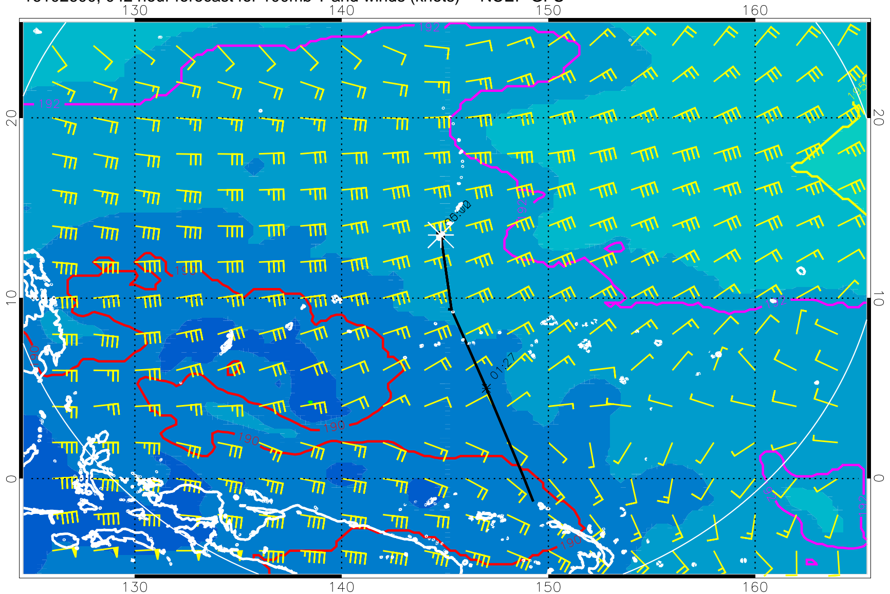
16102600, 042 hour forecast for 100mb T and winds (knots) -- NCEP GFS
