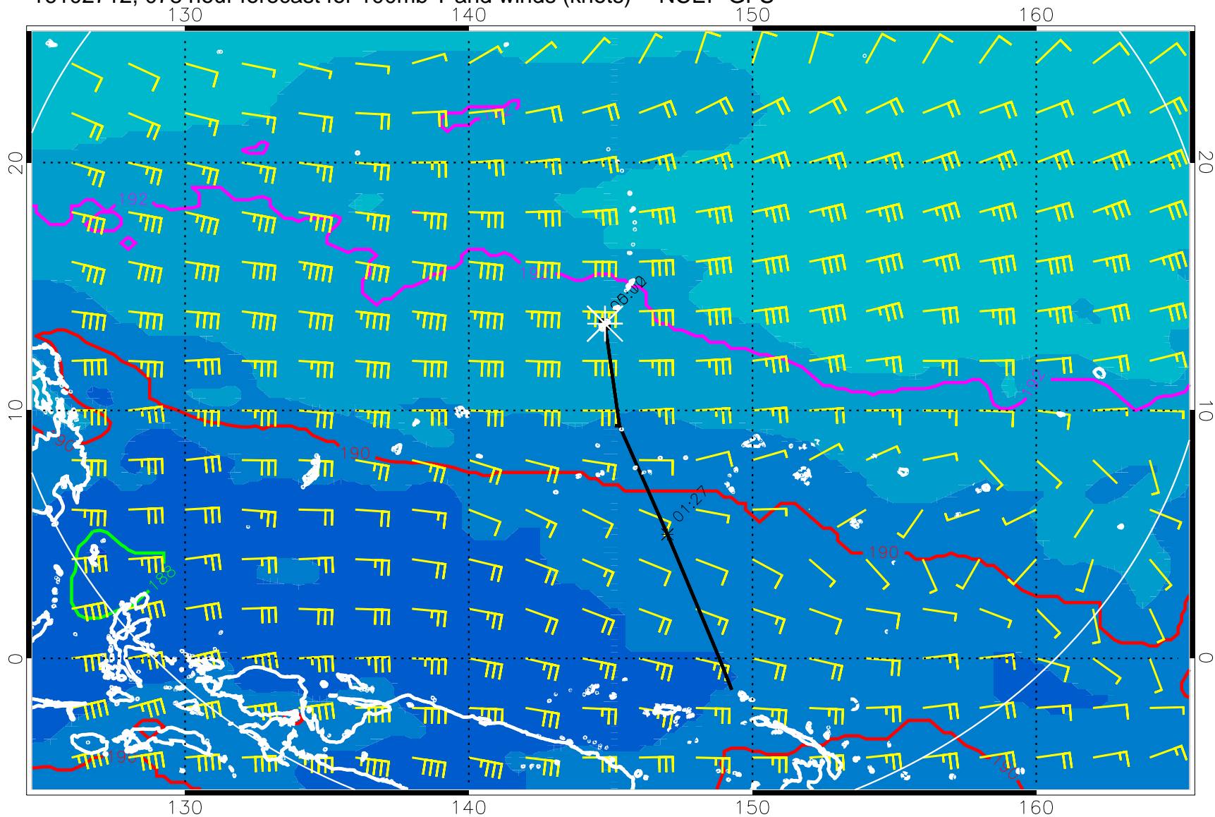
16102712, 078 hour forecast for 100mb T and winds (knots) -- NCEP GFS
