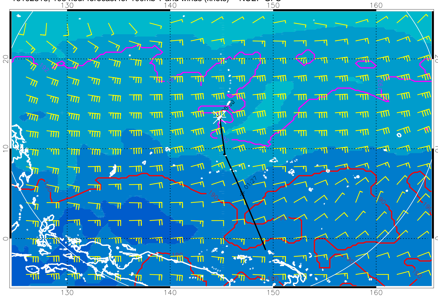
16102818, 108 hour forecast for 100mb T and winds (knots) -- NCEP GFS
