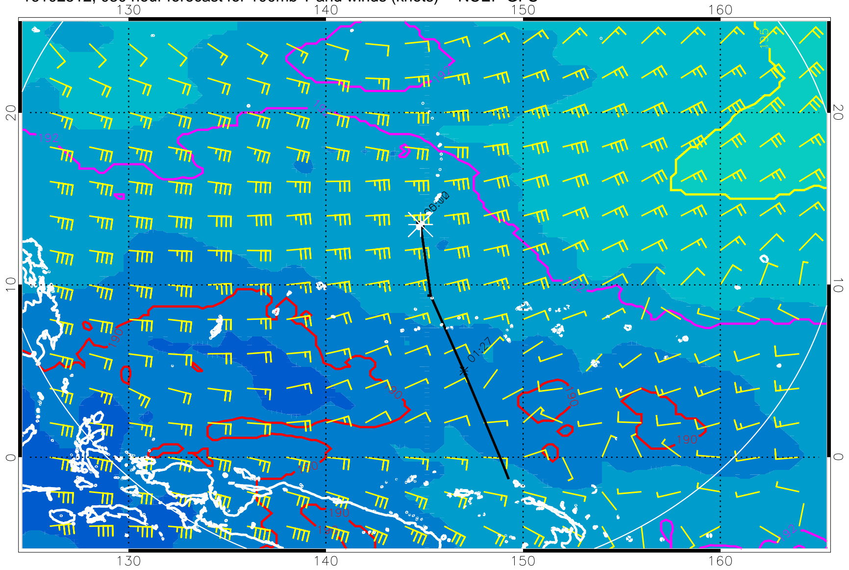
16102512, 030 hour forecast for 100mb T and winds (knots) -- NCEP GFS
