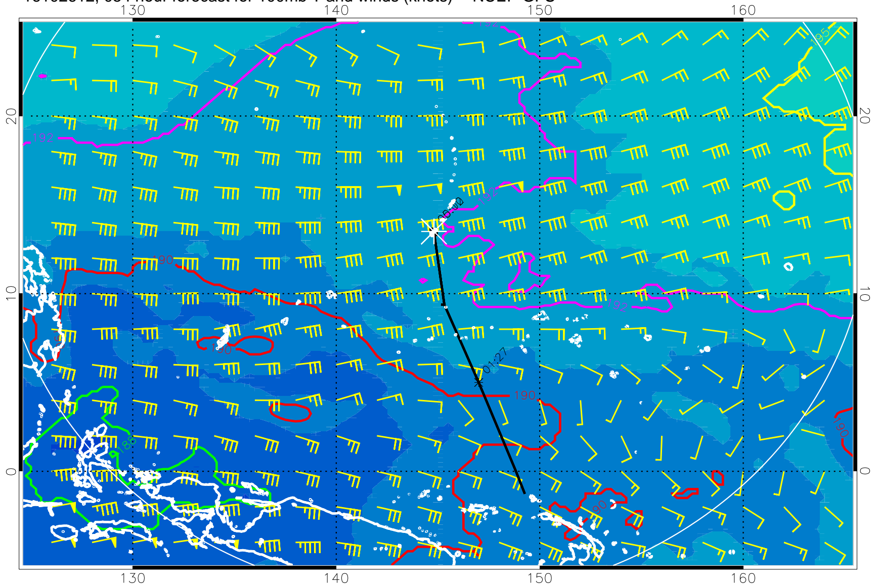
16102612, 054 hour forecast for 100mb T and winds (knots) -- NCEP GFS
