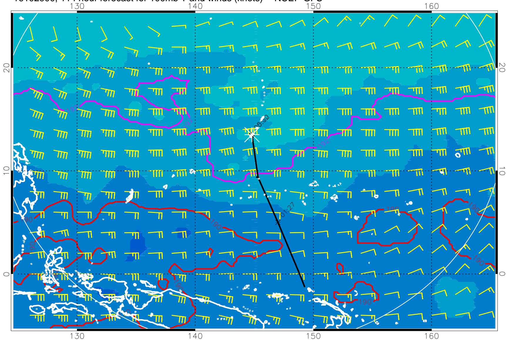
16102900, 114 hour forecast for 100mb T and winds (knots) -- NCEP GFS
