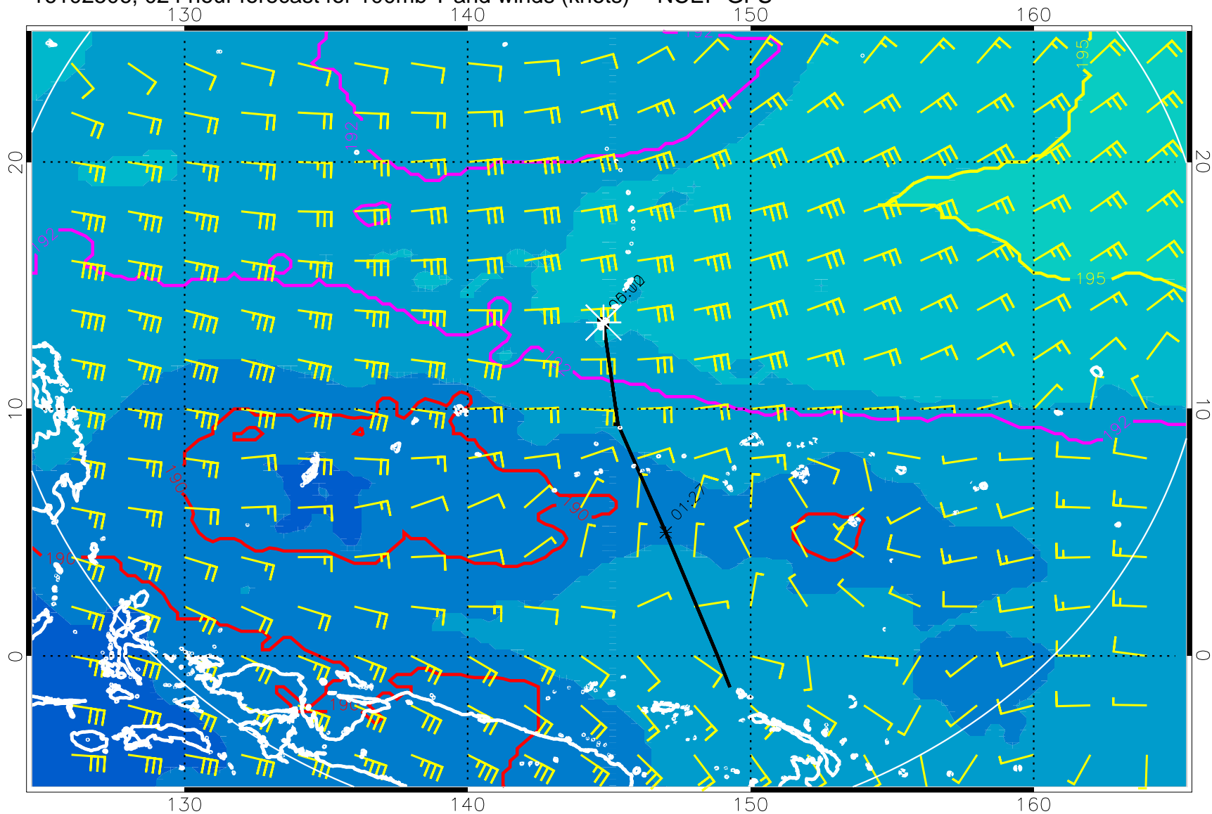
16102506, 024 hour forecast for 100mb T and winds (knots) -- NCEP GFS
