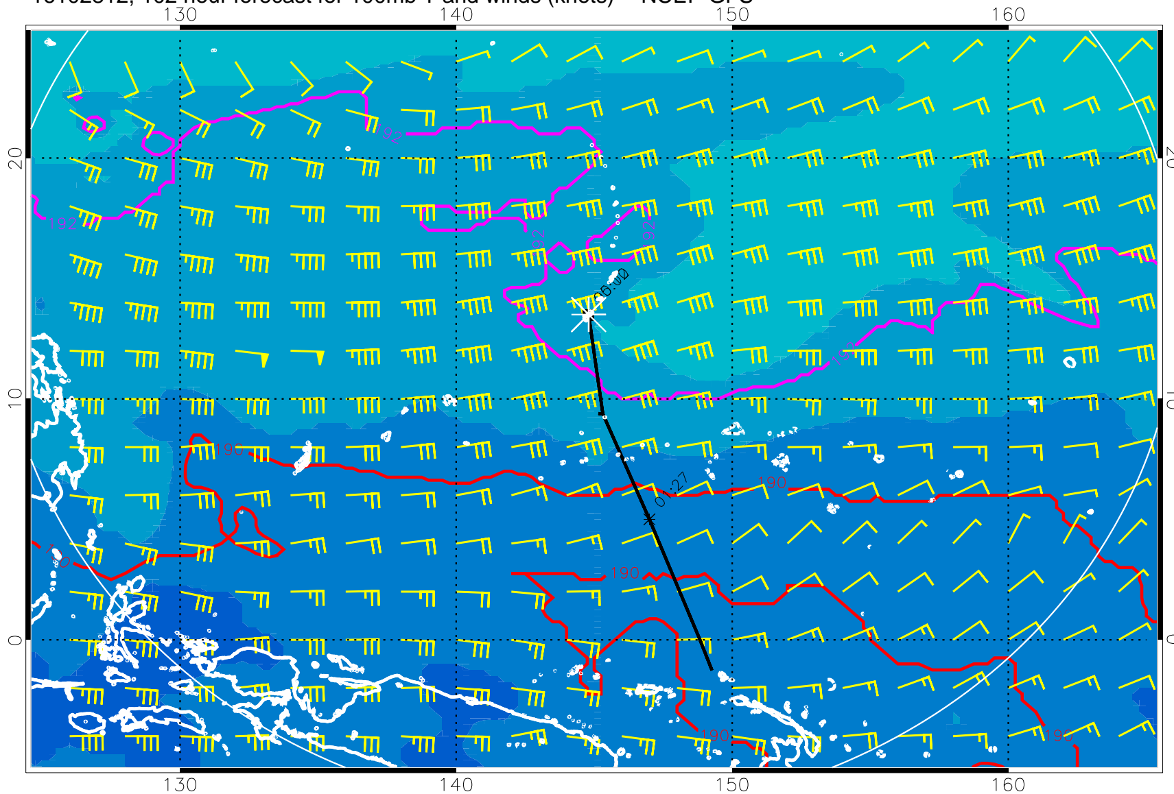
16102812, 102 hour forecast for 100mb T and winds (knots) -- NCEP GFS
