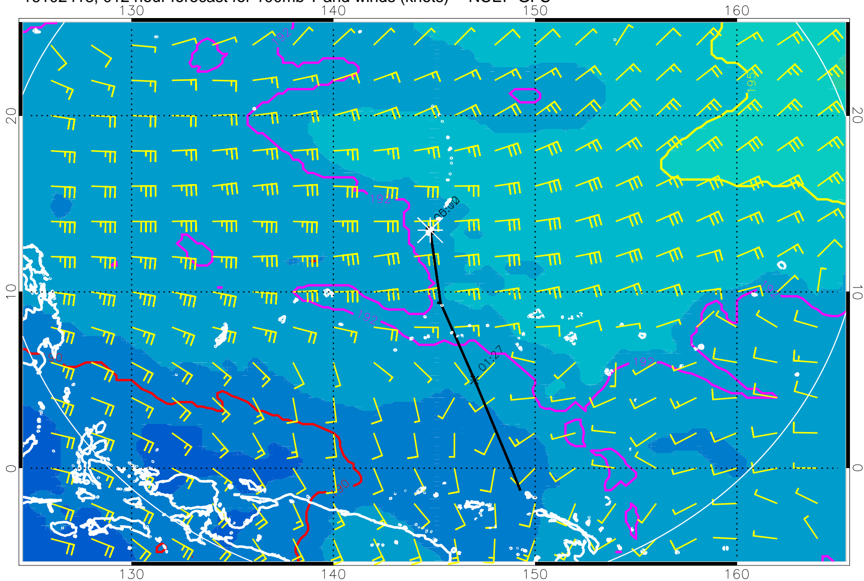
16102418, 012 hour forecast for 100mb T and winds (knots) -- NCEP GFS
