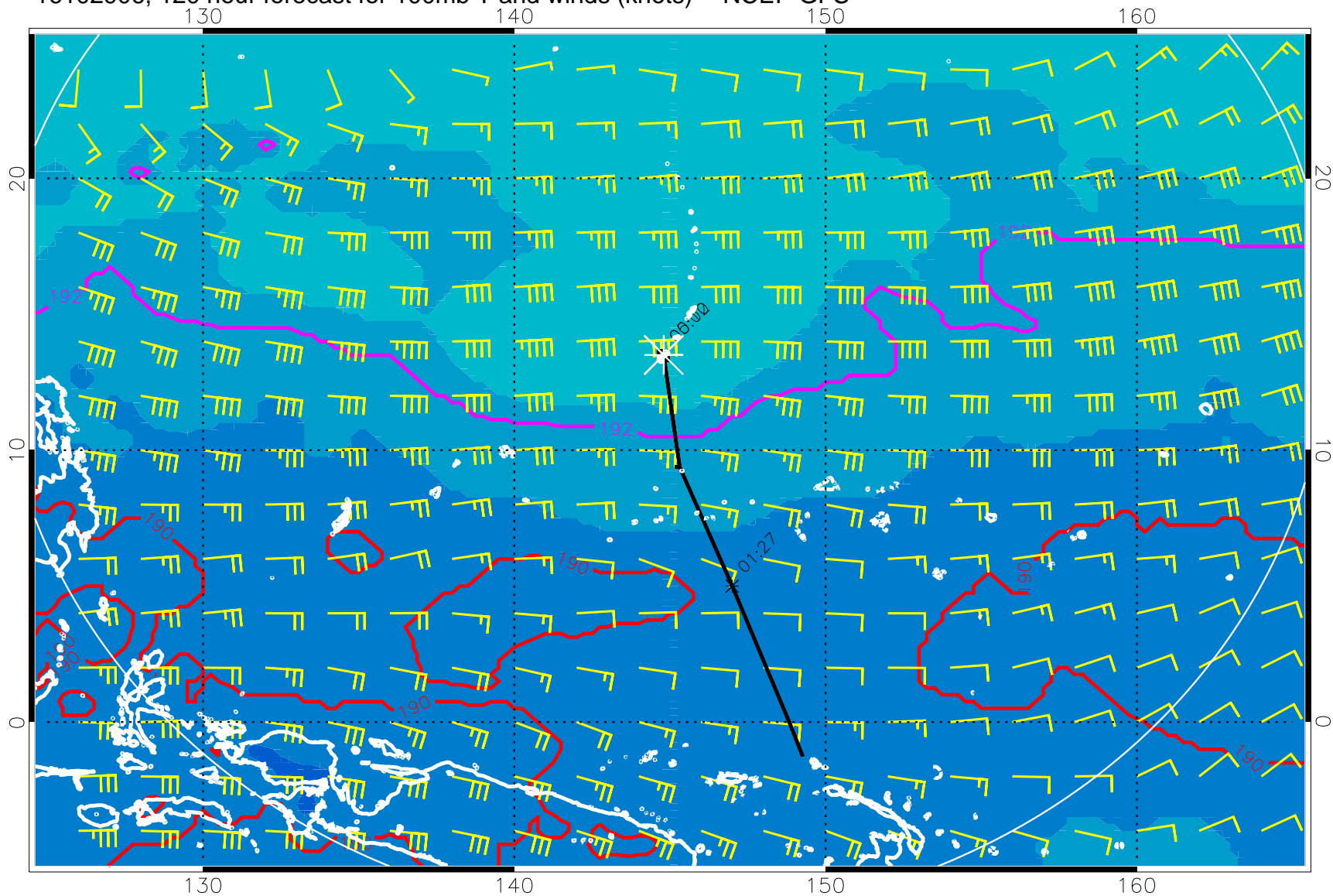
16102906, 120 hour forecast for 100mb T and winds (knots) -- NCEP GFS
