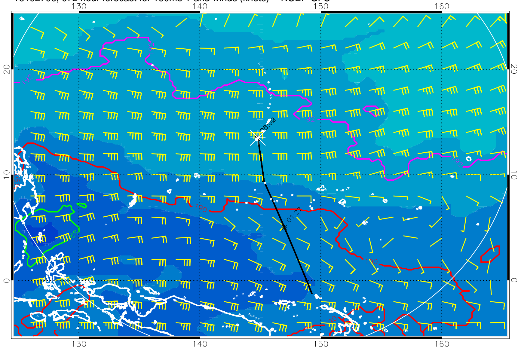
16102706, 072 hour forecast for 100mb T and winds (knots) -- NCEP GFS
