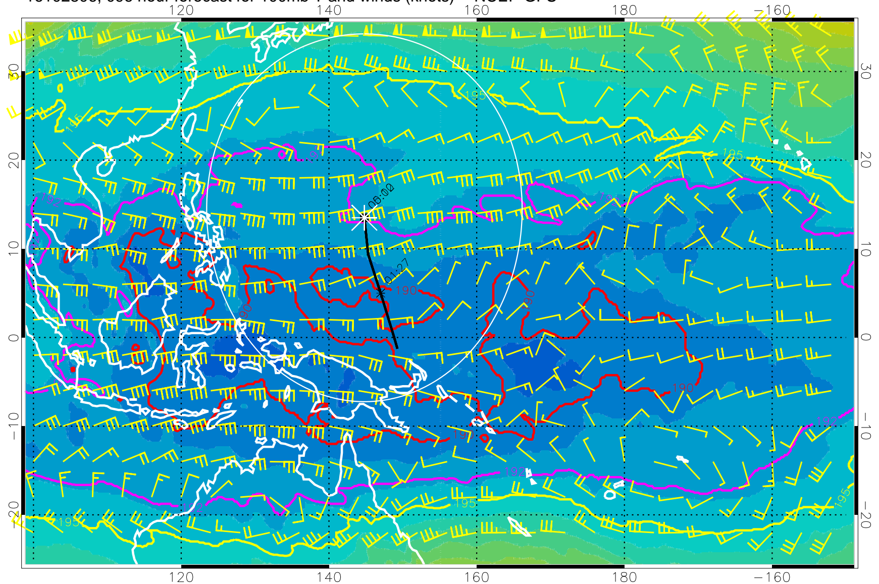
16102806, 096 hour forecast for 100mb T and winds (knots) -- NCEP GFS
