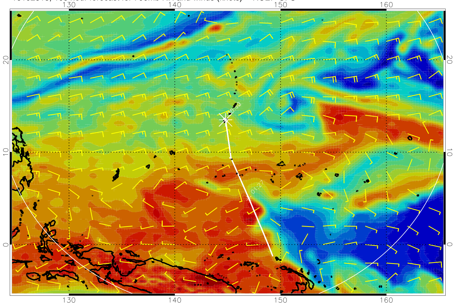
16102818, 108 hour forecast for 700mb RH and winds (knots) -- NCEP GFS
