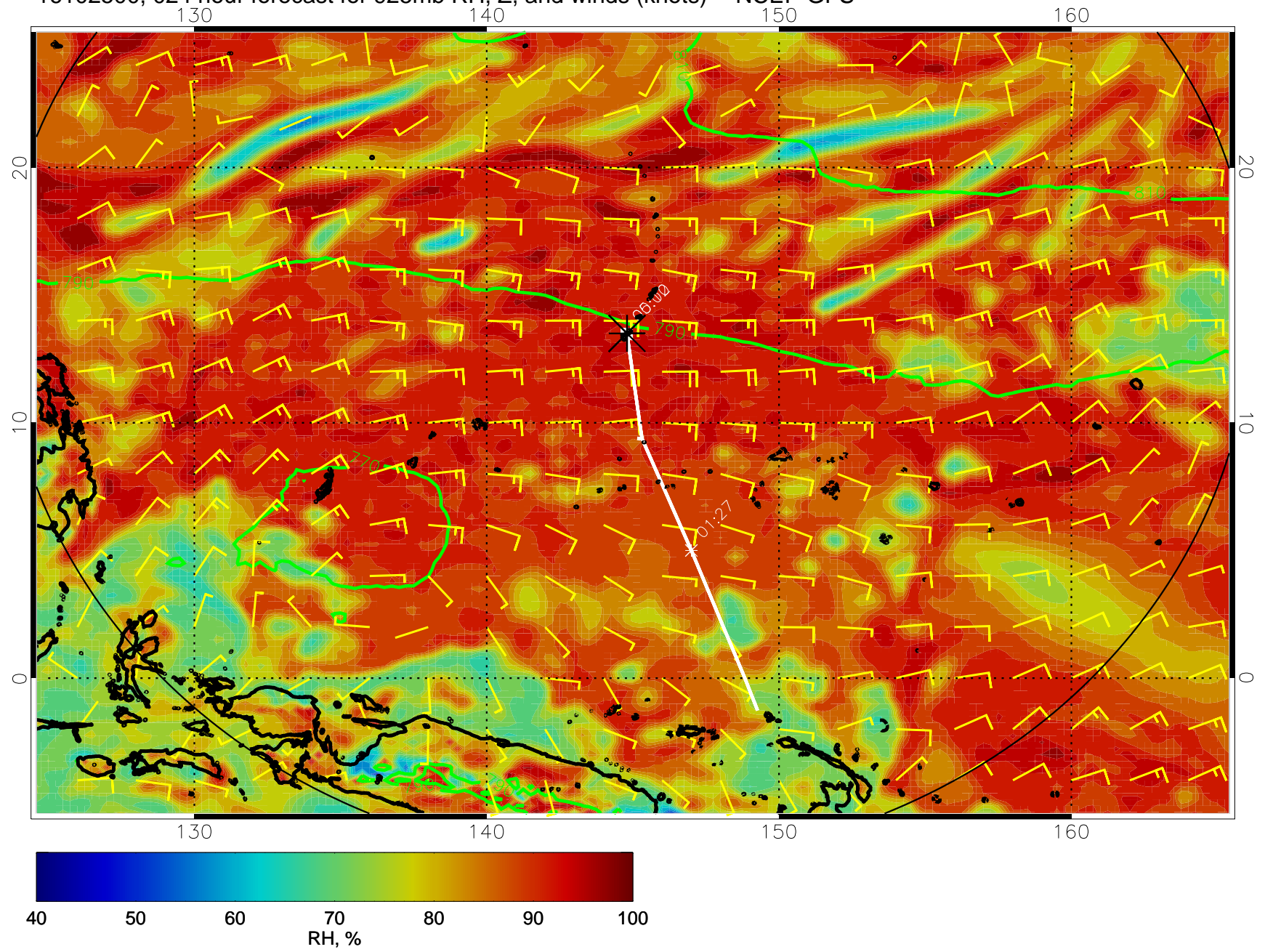
16102500, 024 hour forecast for 925mb RH, Z, and winds (knots) -- NCEP GFS
