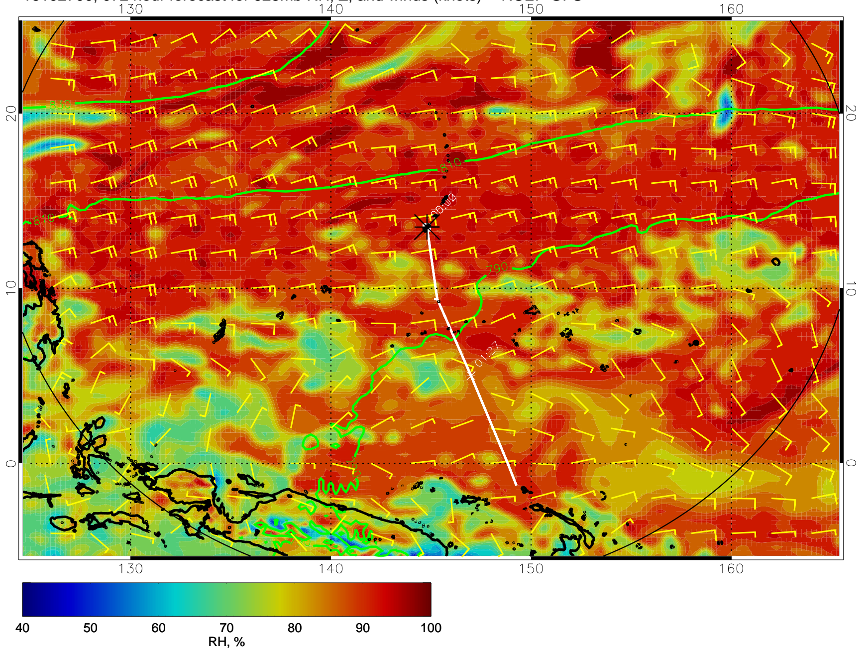
16102700, 072 hour forecast for 925mb RH, Z, and winds (knots) -- NCEP GFS
