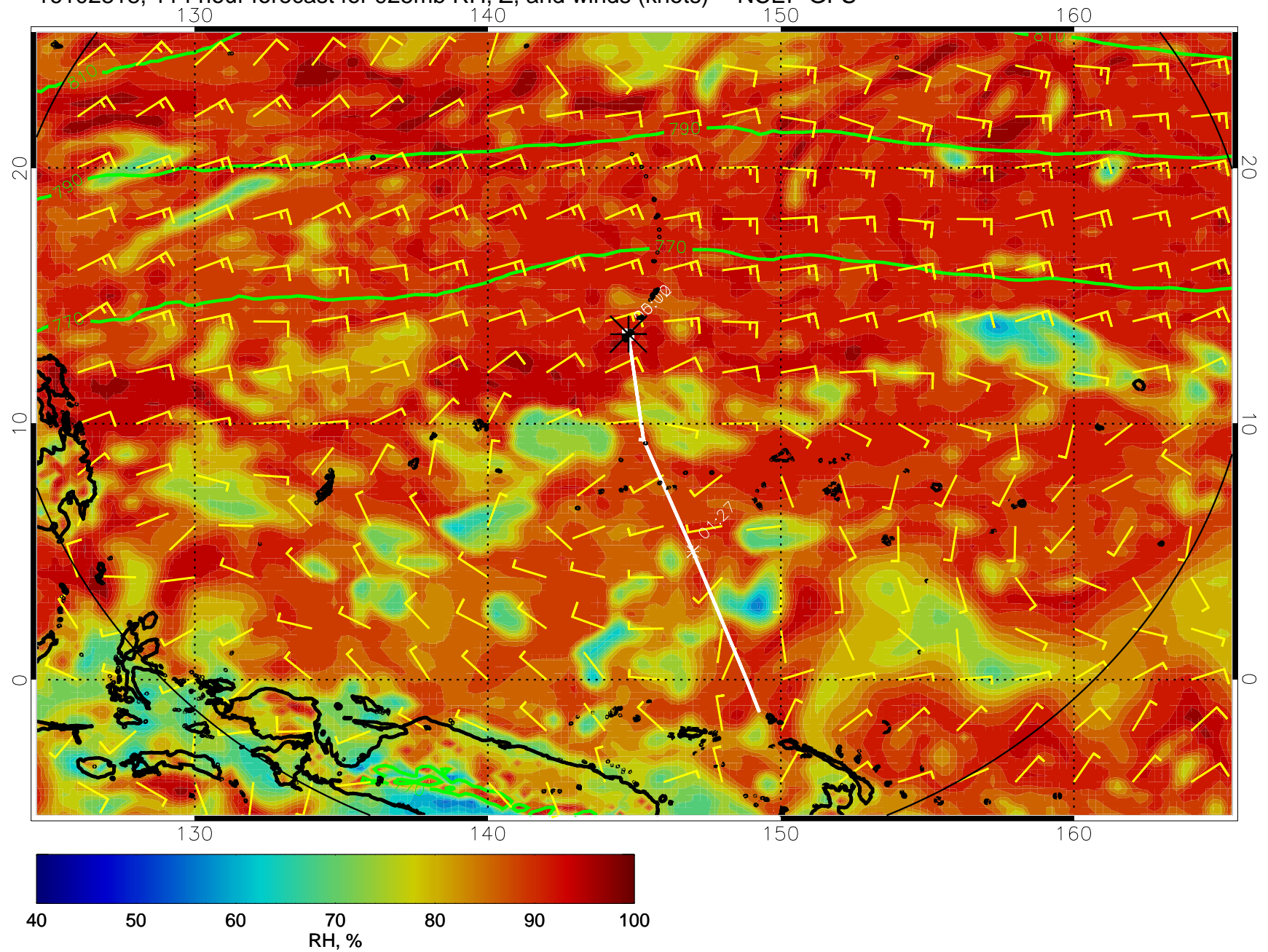
16102818, 114 hour forecast for 925mb RH, Z, and winds (knots) -- NCEP GFS
