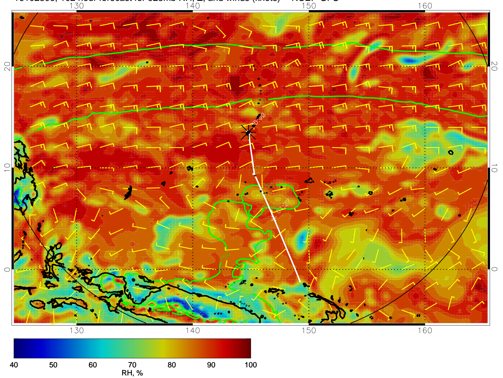
16102806, 102 hour forecast for 925mb RH, Z, and winds (knots) -- NCEP GFS
