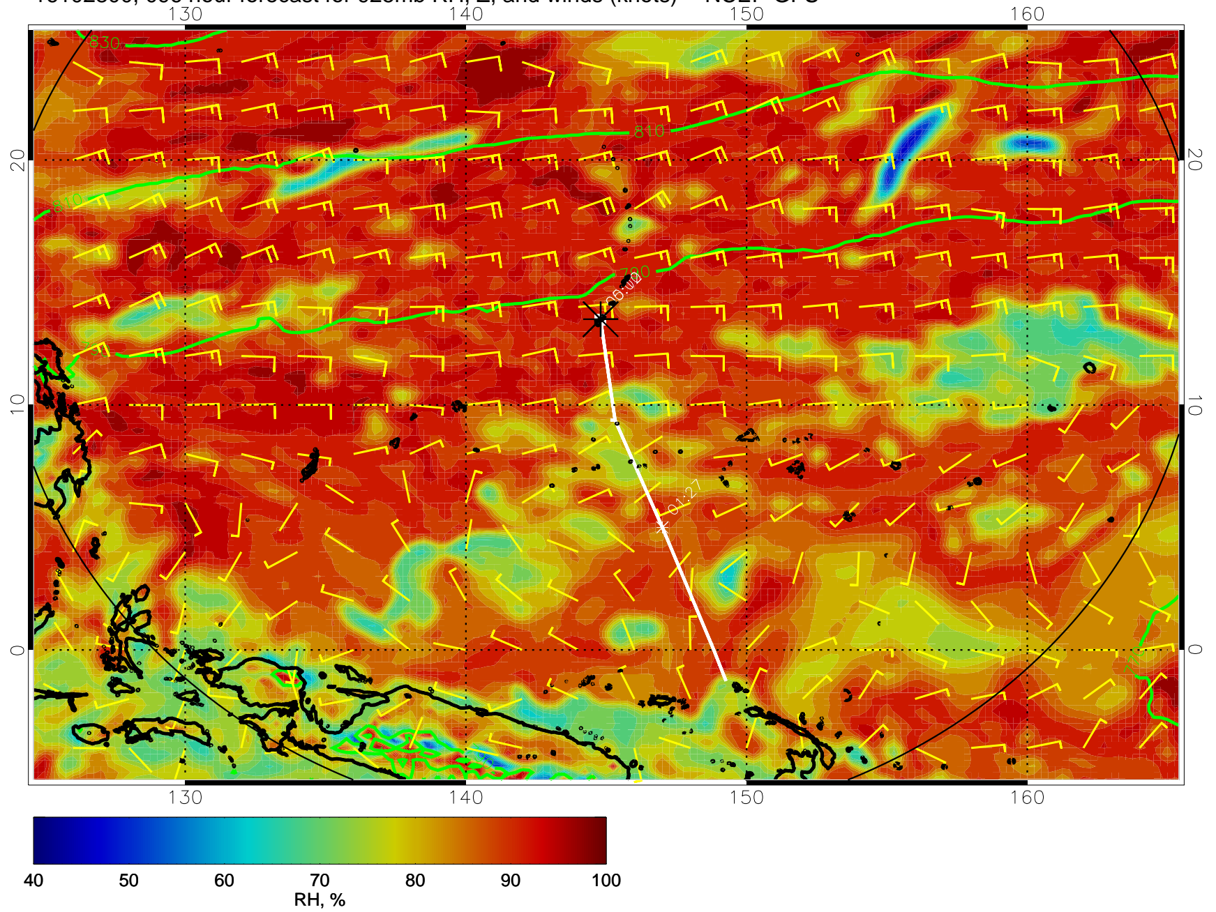
16102800, 096 hour forecast for 925mb RH, Z, and winds (knots) -- NCEP GFS
