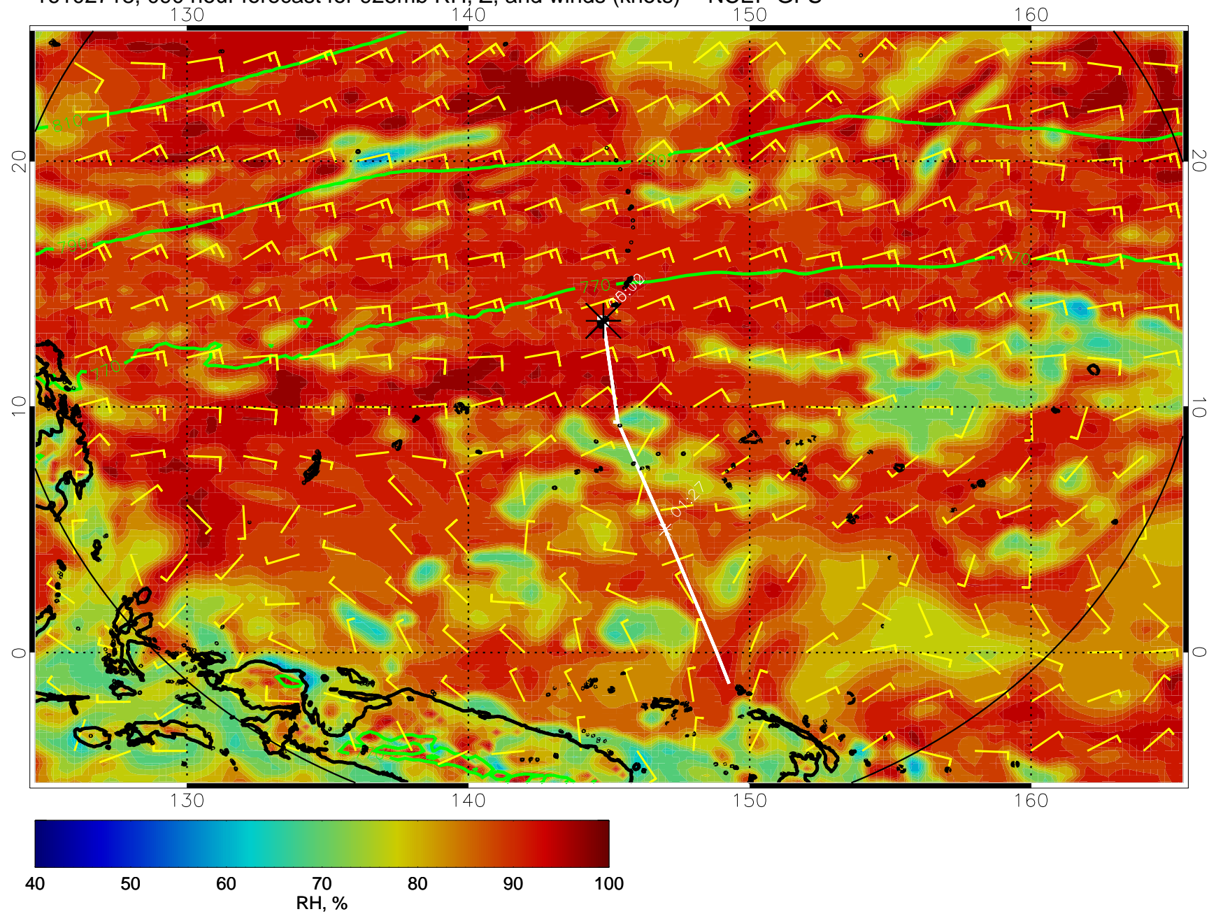
16102718, 090 hour forecast for 925mb RH, Z, and winds (knots) -- NCEP GFS
