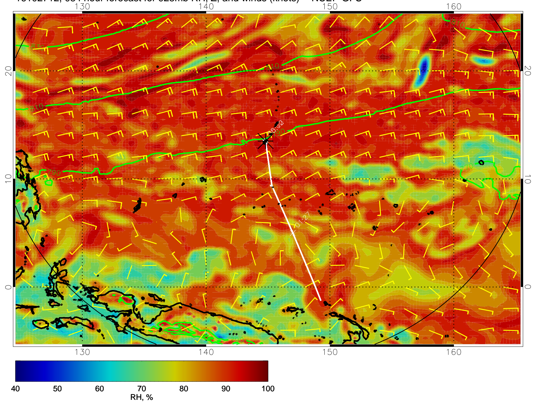
16102712, 084 hour forecast for 925mb RH, Z, and winds (knots) -- NCEP GFS
