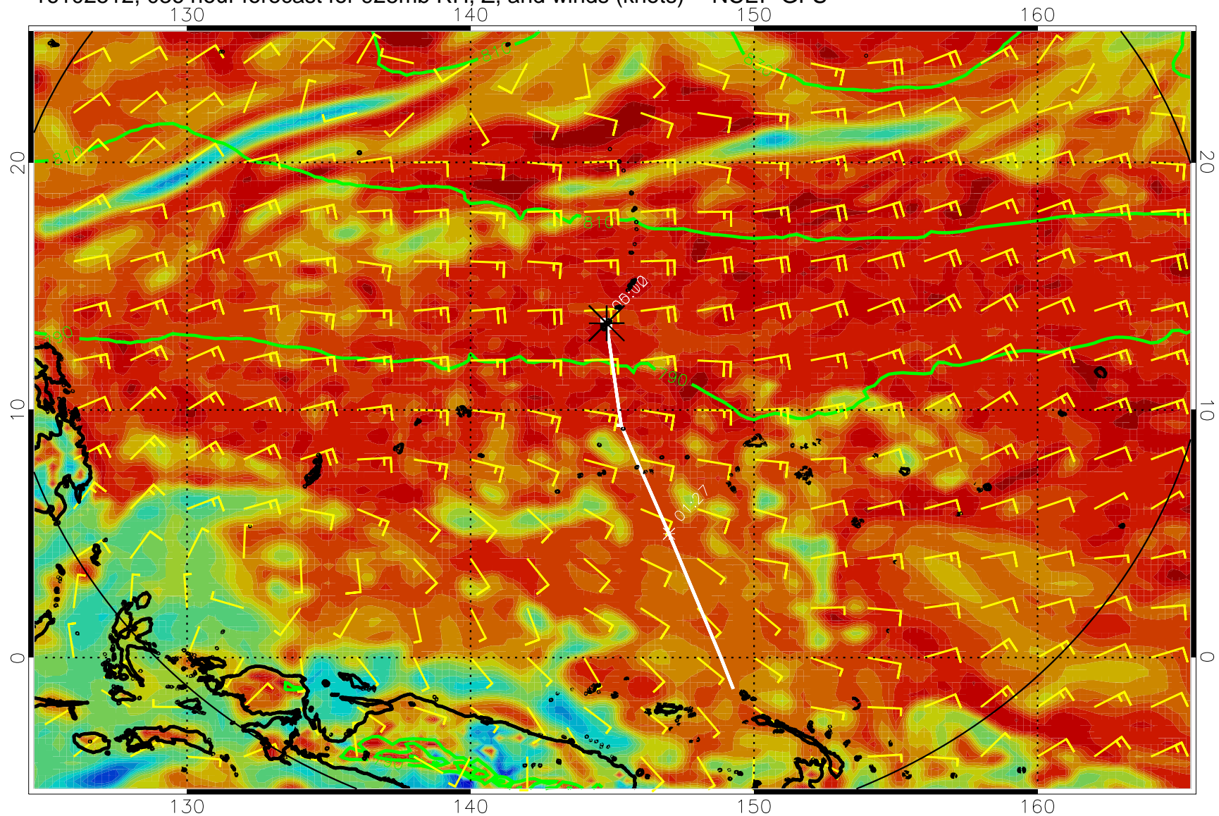
16102512, 036 hour forecast for 925mb RH, Z, and winds (knots) -- NCEP GFS
