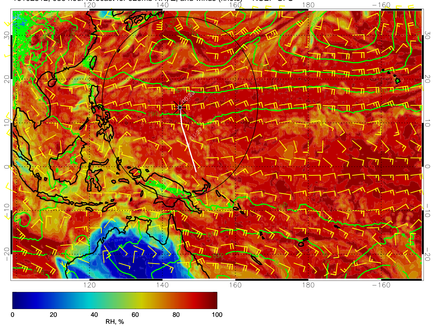
16102512, 036 hour forecast for 925mb RH, Z, and winds (knots) -- NCEP GFS
