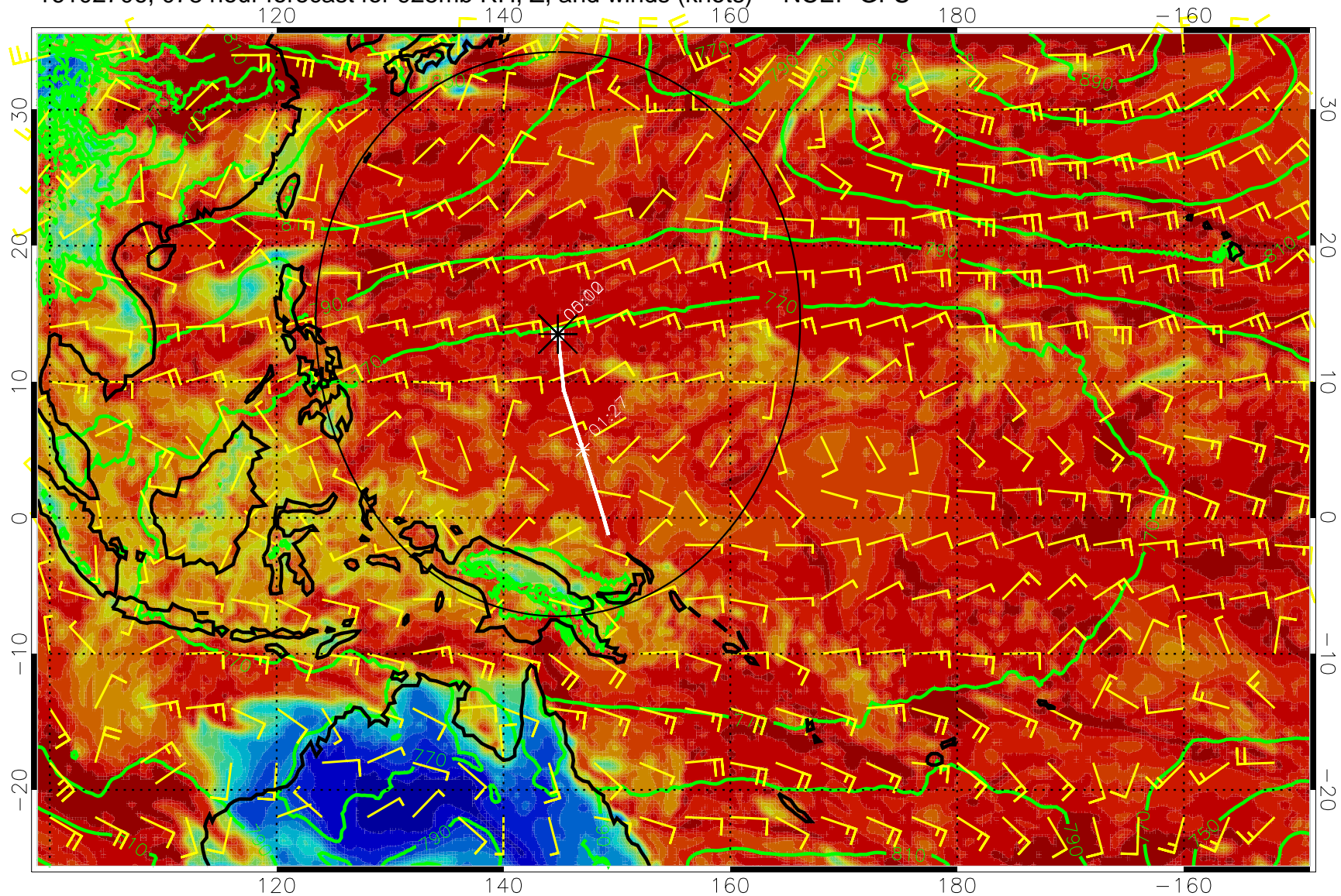
16102706, 078 hour forecast for 925mb RH, Z, and winds (knots) -- NCEP GFS
