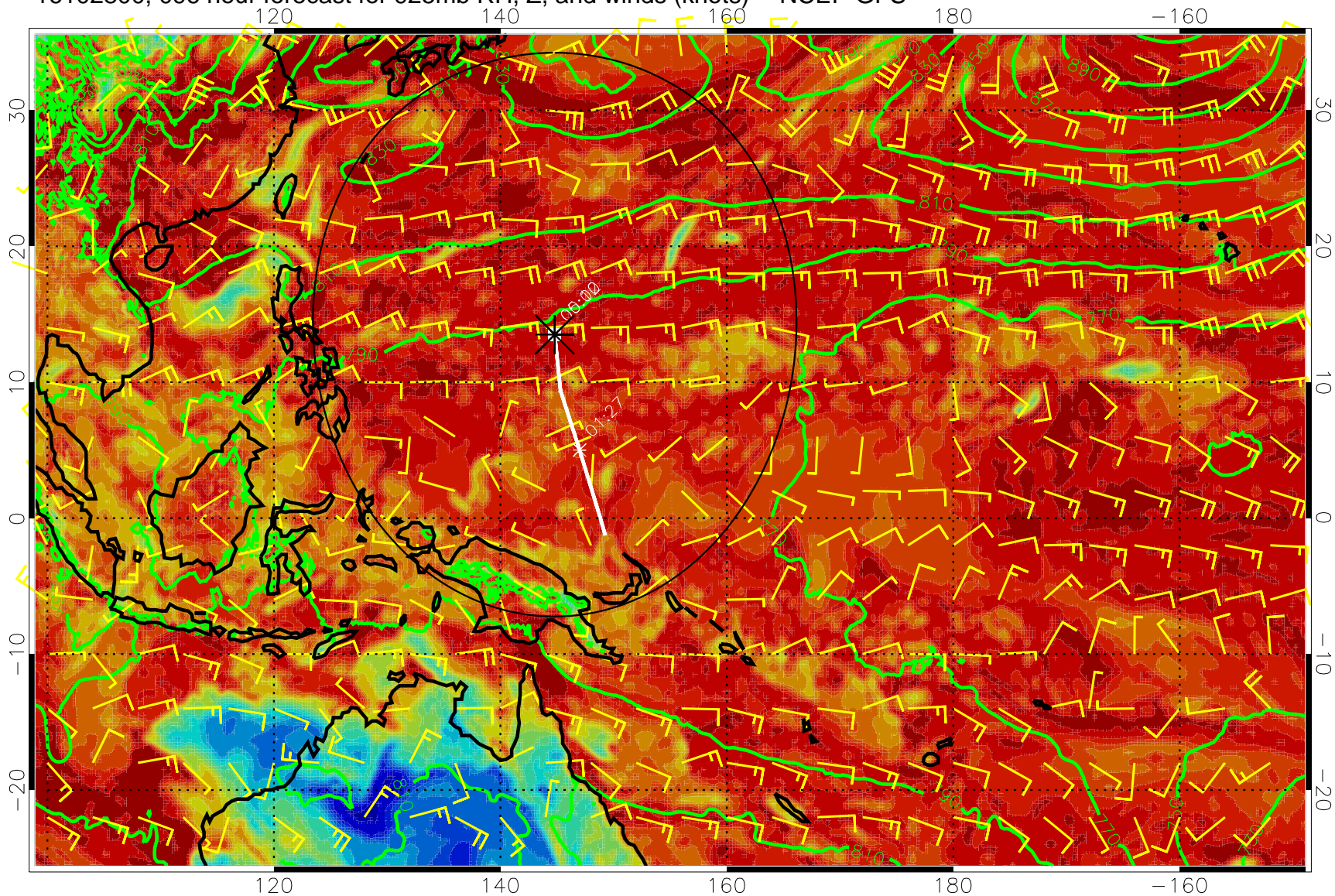
16102800, 096 hour forecast for 925mb RH, Z, and winds (knots) -- NCEP GFS
