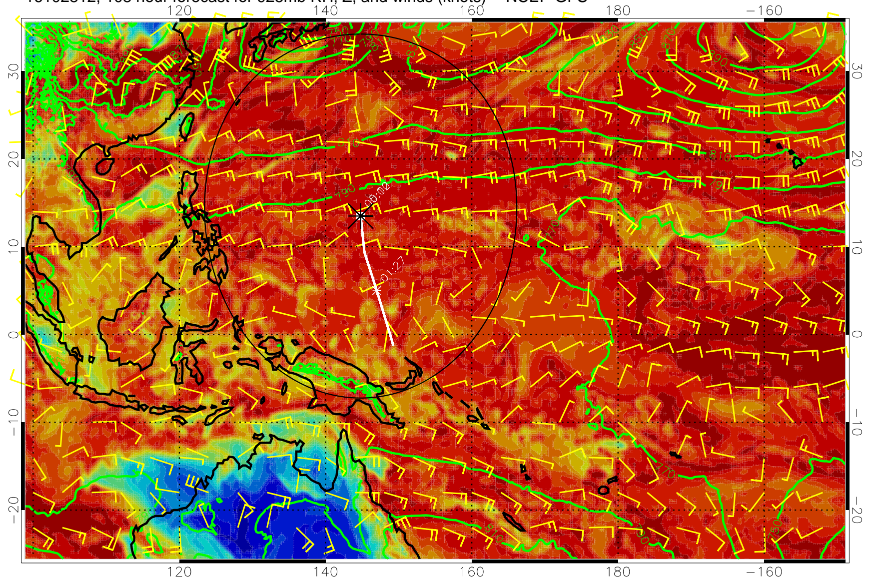
16102812, 108 hour forecast for 925mb RH, Z, and winds (knots) -- NCEP GFS
