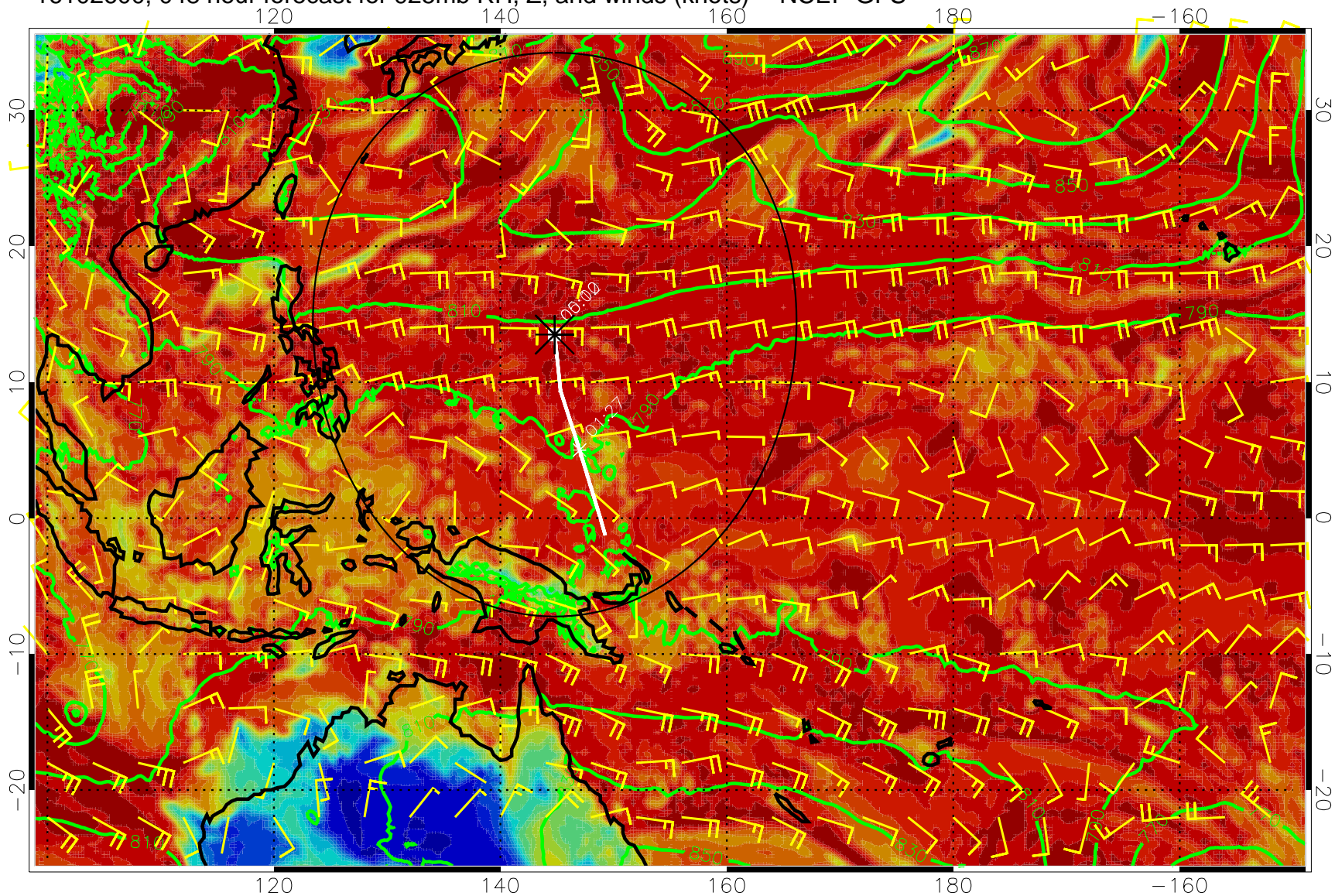
16102600, 048 hour forecast for 925mb RH, Z, and winds (knots) -- NCEP GFS
