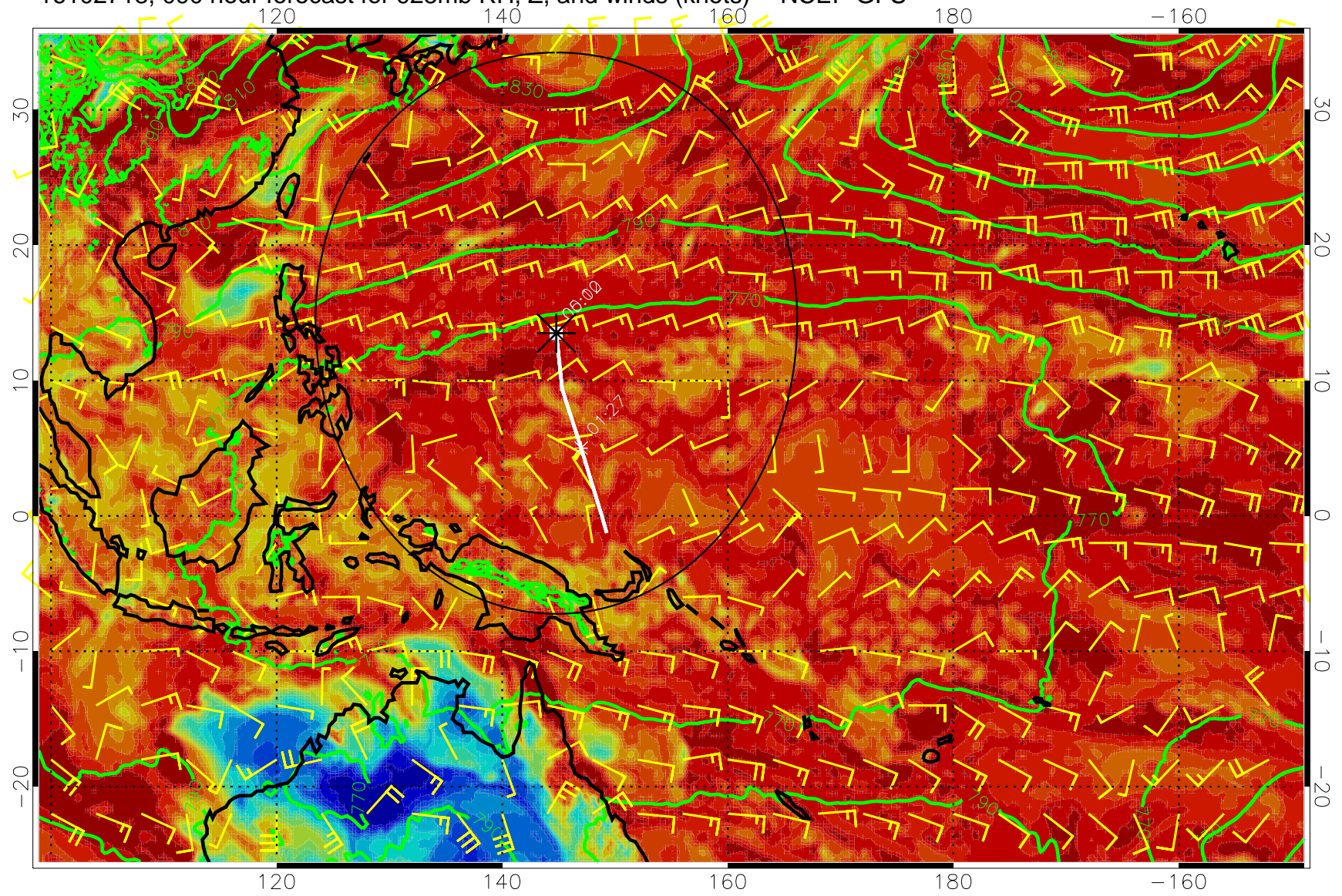
16102718, 090 hour forecast for 925mb RH, Z, and winds (knots) -- NCEP GFS
