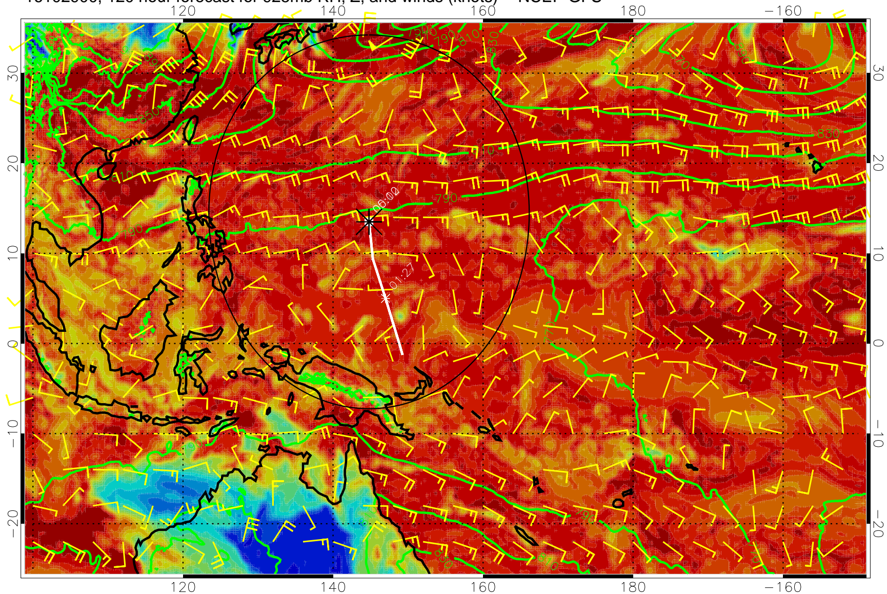
16102900, 120 hour forecast for 925mb RH, Z, and winds (knots) -- NCEP GFS
