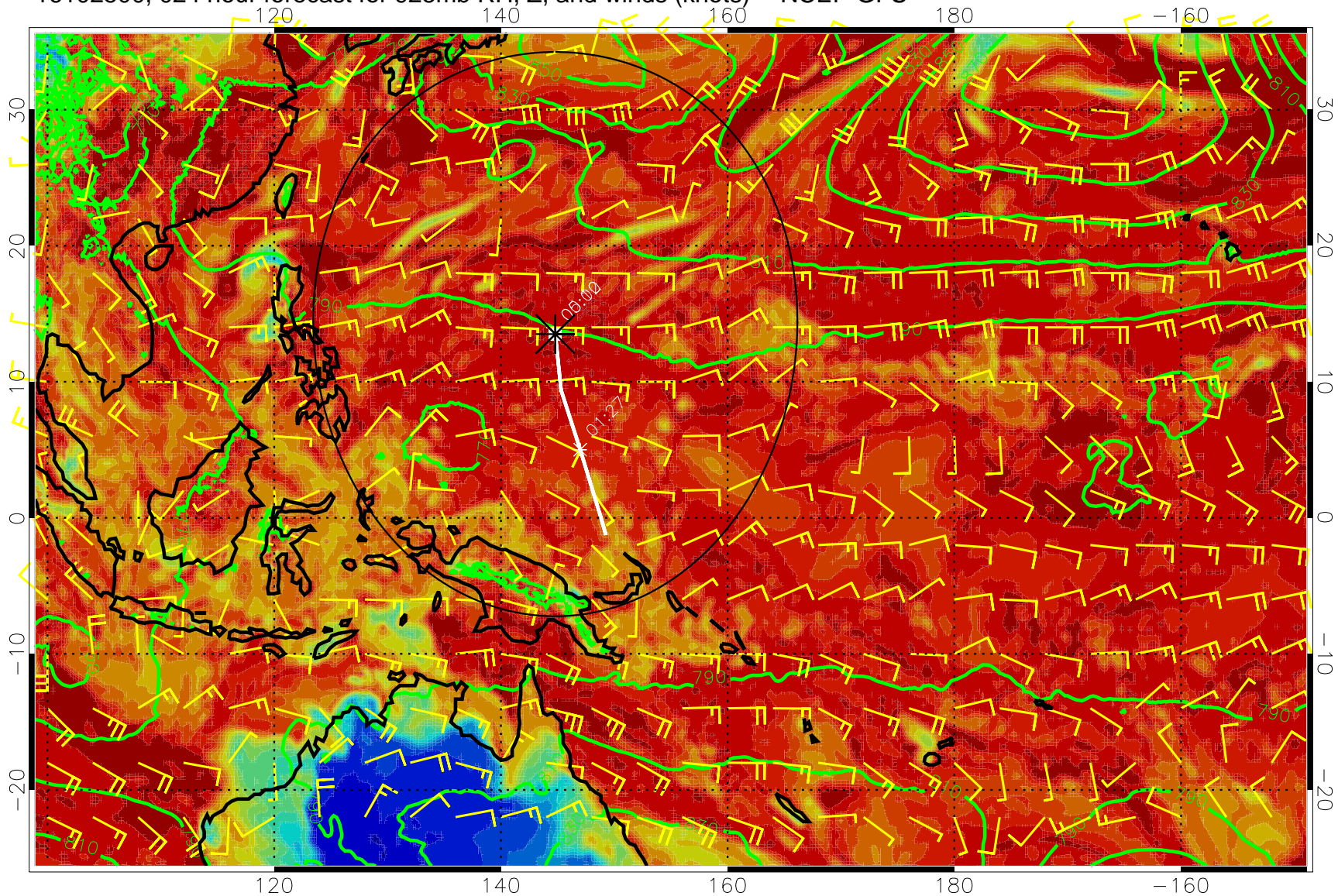
16102500, 024 hour forecast for 925mb RH, Z, and winds (knots) -- NCEP GFS
