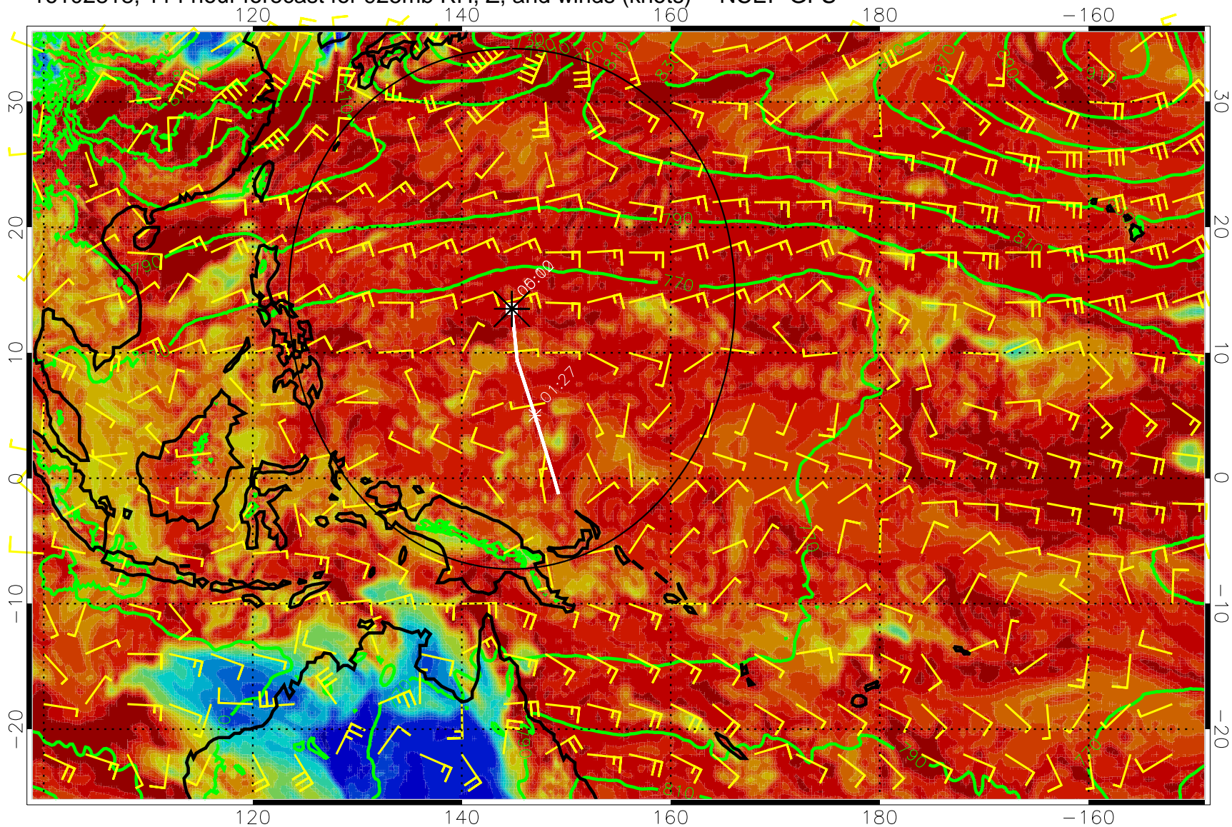
16102818, 114 hour forecast for 925mb RH, Z, and winds (knots) -- NCEP GFS
