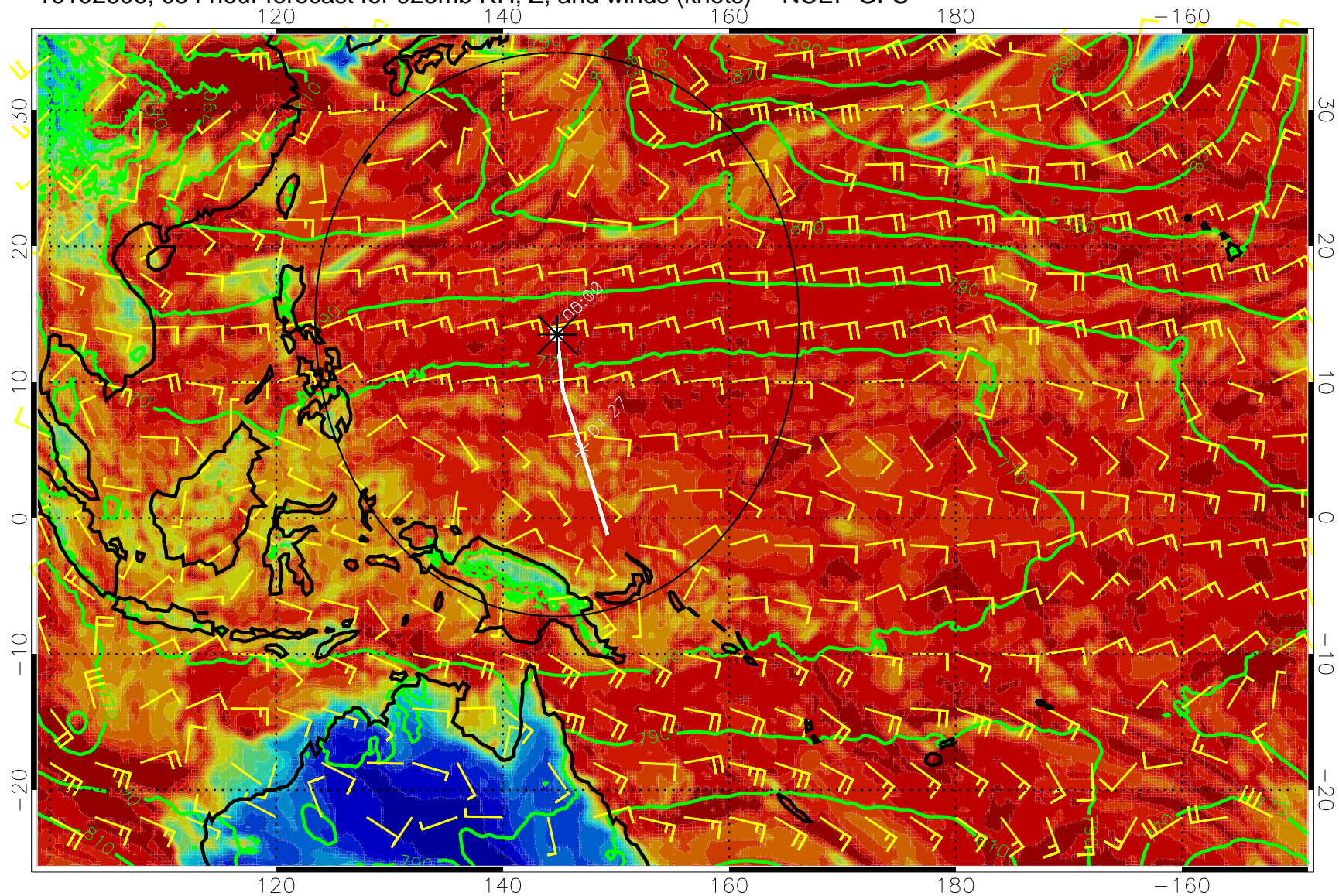
16102606, 054 hour forecast for 925mb RH, Z, and winds (knots) -- NCEP GFS
