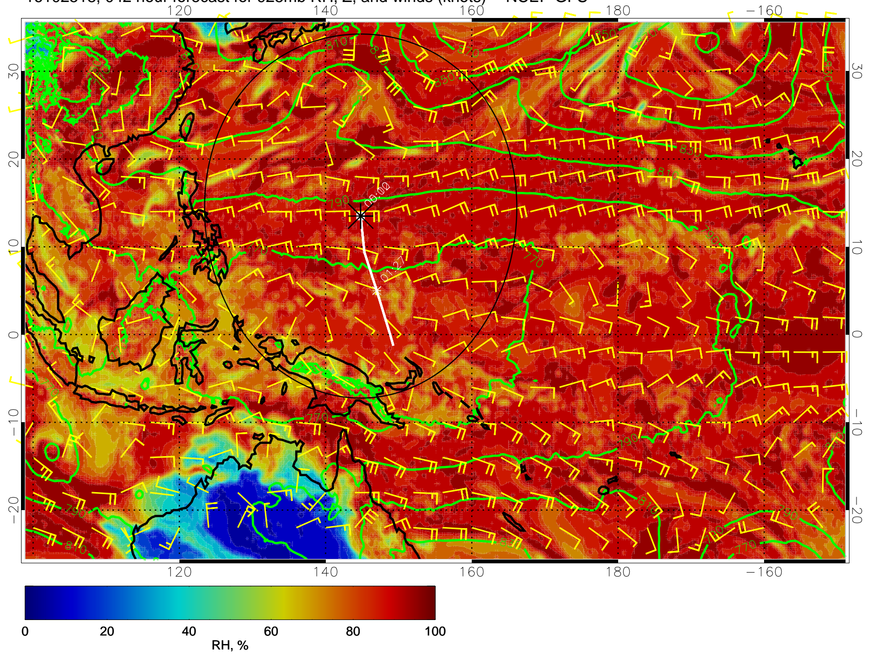
16102518, 042 hour forecast for 925mb RH, Z, and winds (knots) -- NCEP GFS
