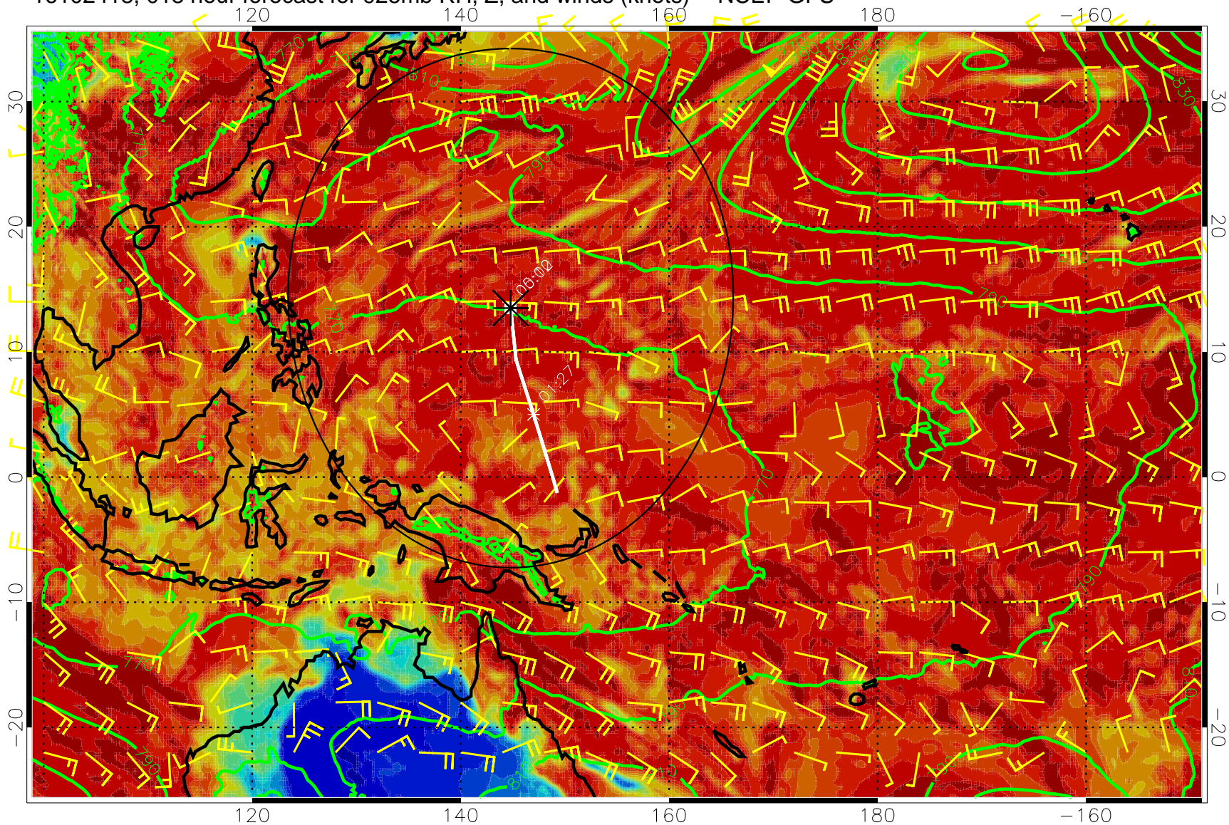
16102418, 018 hour forecast for 925mb RH, Z, and winds (knots) -- NCEP GFS
