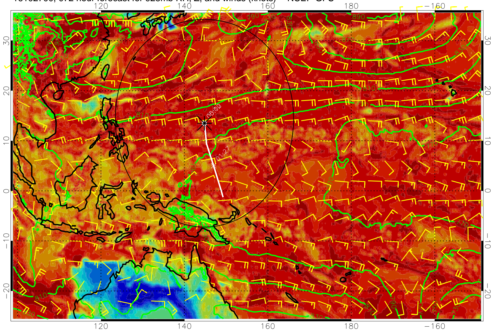
16102700, 072 hour forecast for 925mb RH, Z, and winds (knots) -- NCEP GFS
