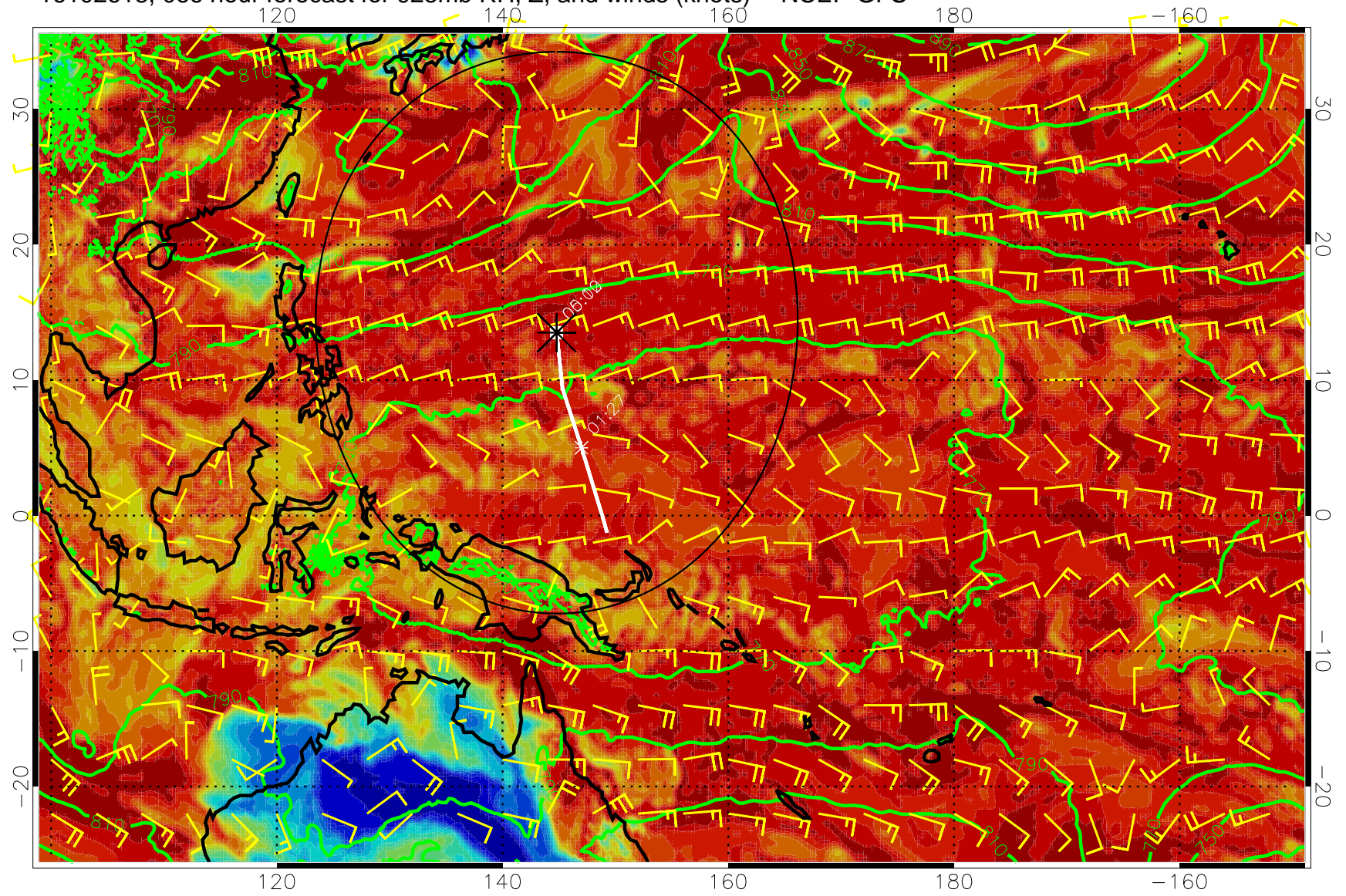
16102618, 066 hour forecast for 925mb RH, Z, and winds (knots) -- NCEP GFS
