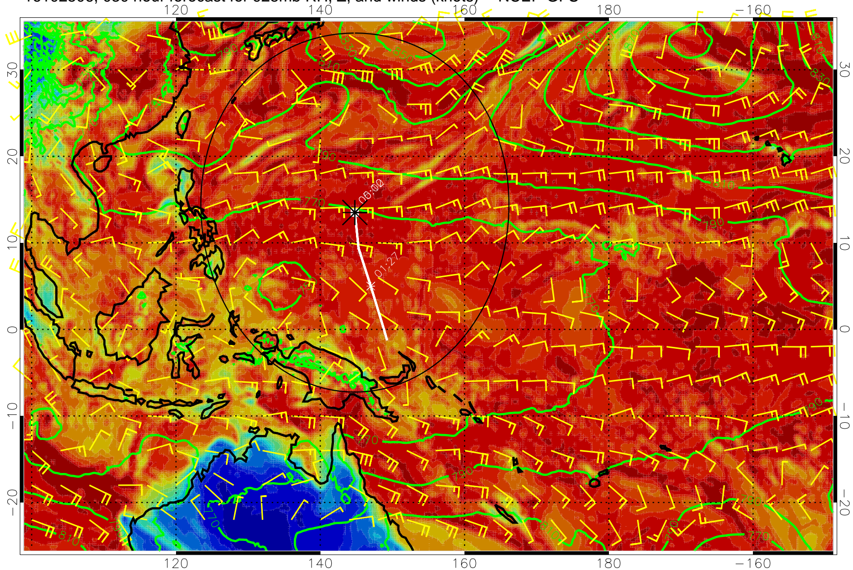
16102506, 030 hour forecast for 925mb RH, Z, and winds (knots) -- NCEP GFS
