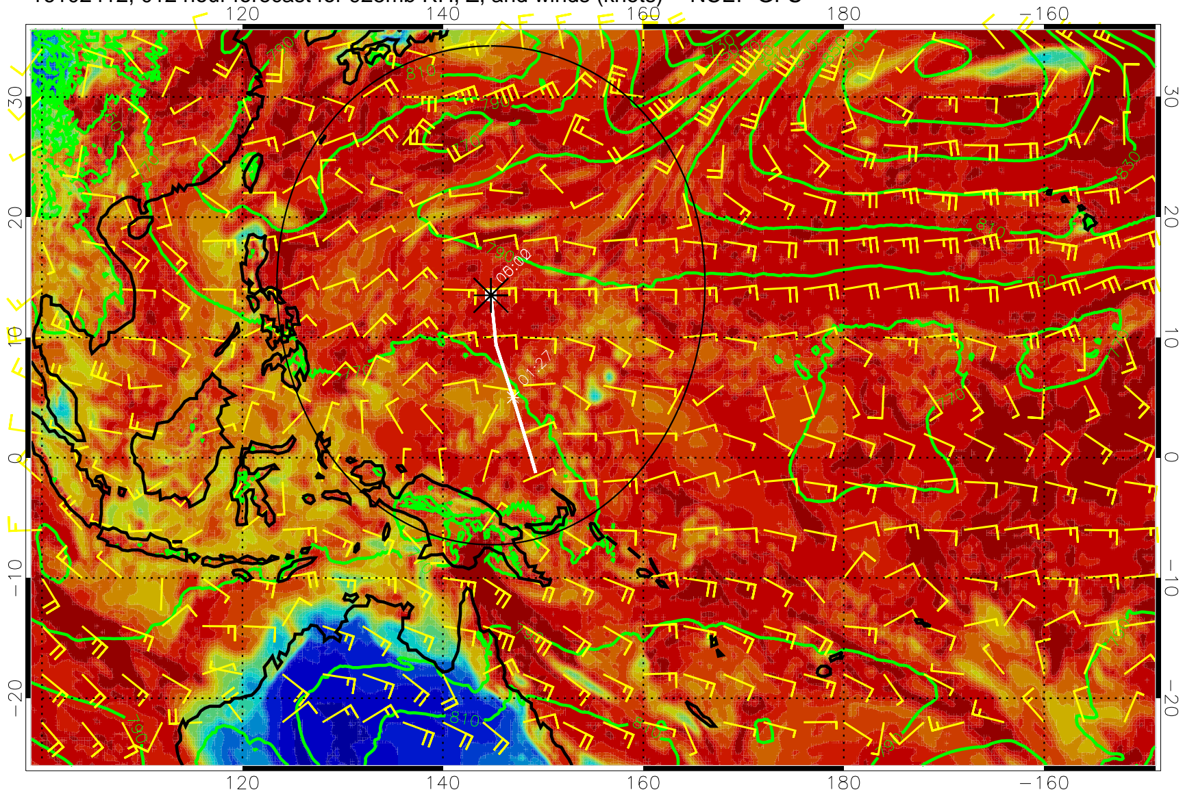
16102412, 012 hour forecast for 925mb RH, Z, and winds (knots) -- NCEP GFS
