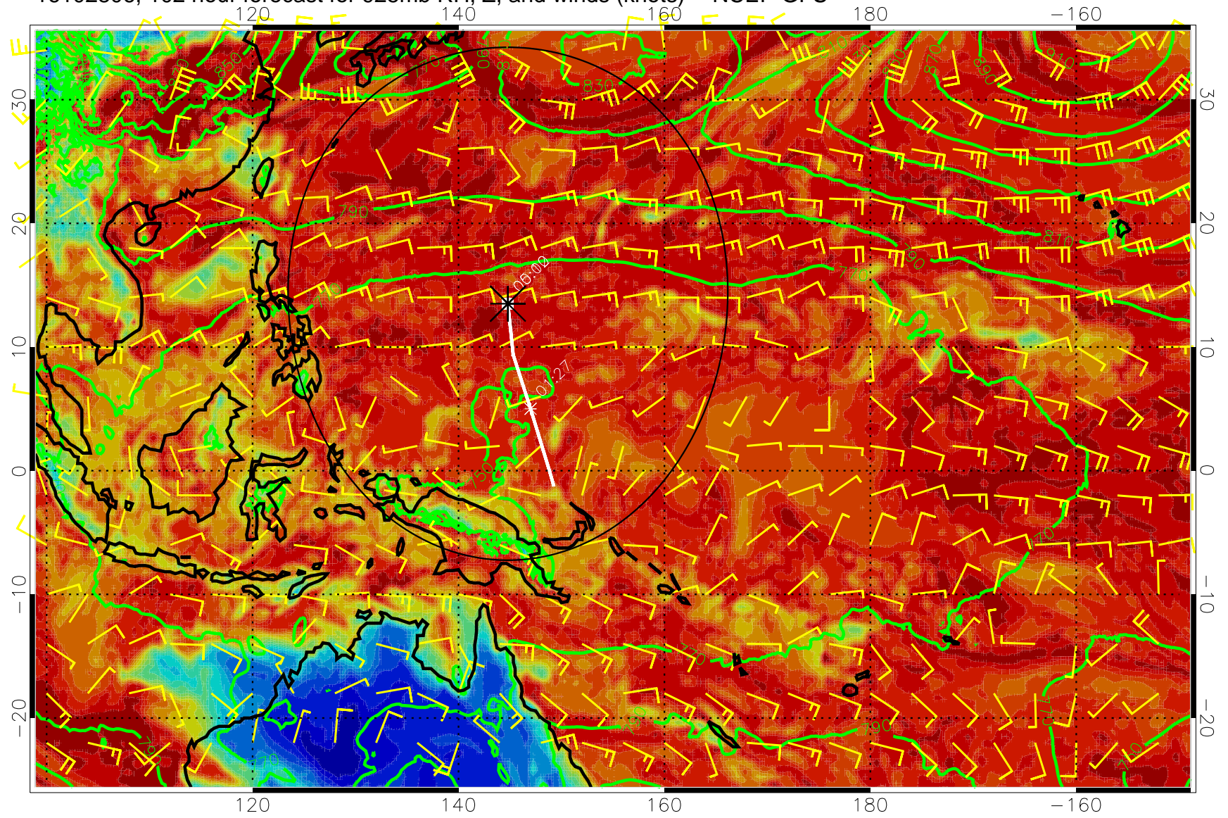
16102806, 102 hour forecast for 925mb RH, Z, and winds (knots) -- NCEP GFS
