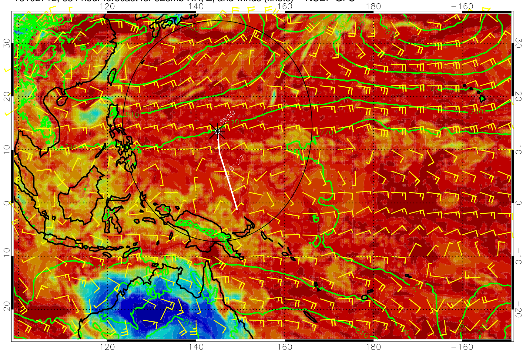
16102712, 084 hour forecast for 925mb RH, Z, and winds (knots) -- NCEP GFS
