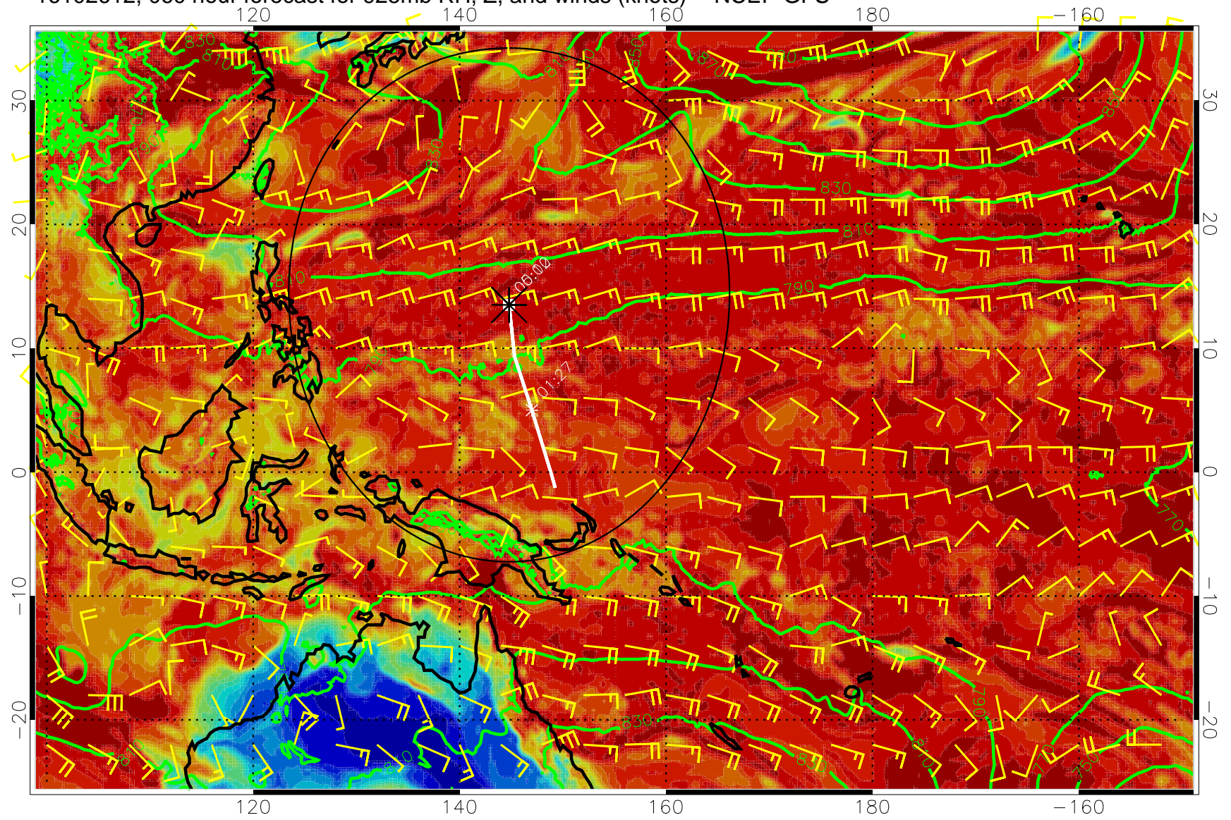
16102612, 060 hour forecast for 925mb RH, Z, and winds (knots) -- NCEP GFS
