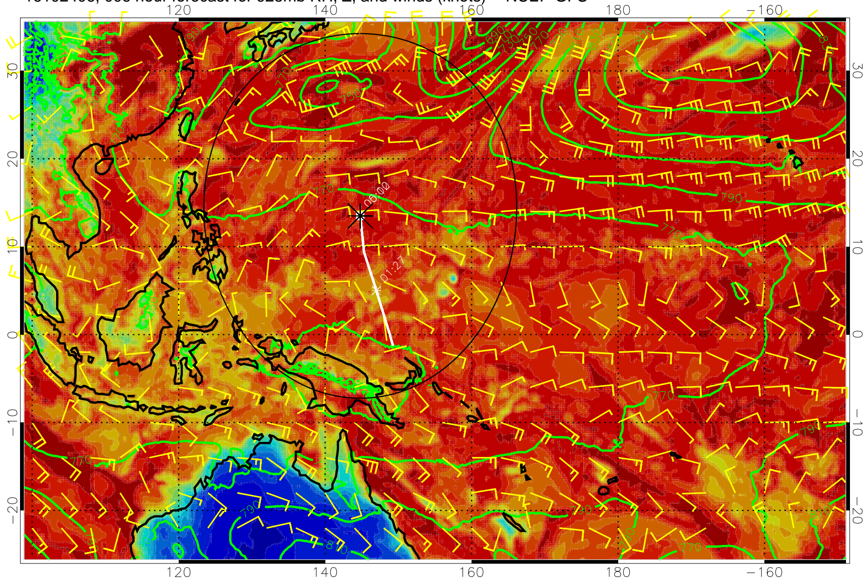
16102406, 006 hour forecast for 925mb RH, Z, and winds (knots) -- NCEP GFS
