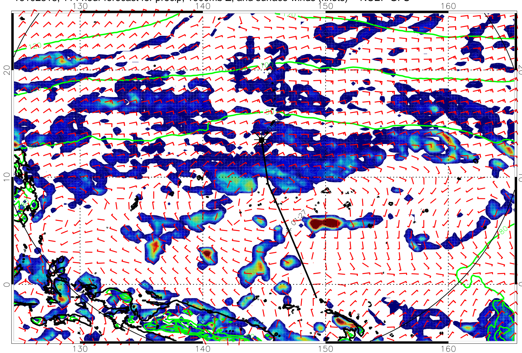
16102818, 114 hour forecast for precip, 1000mb Z, and surface winds (knots) -- NCEP GFS
