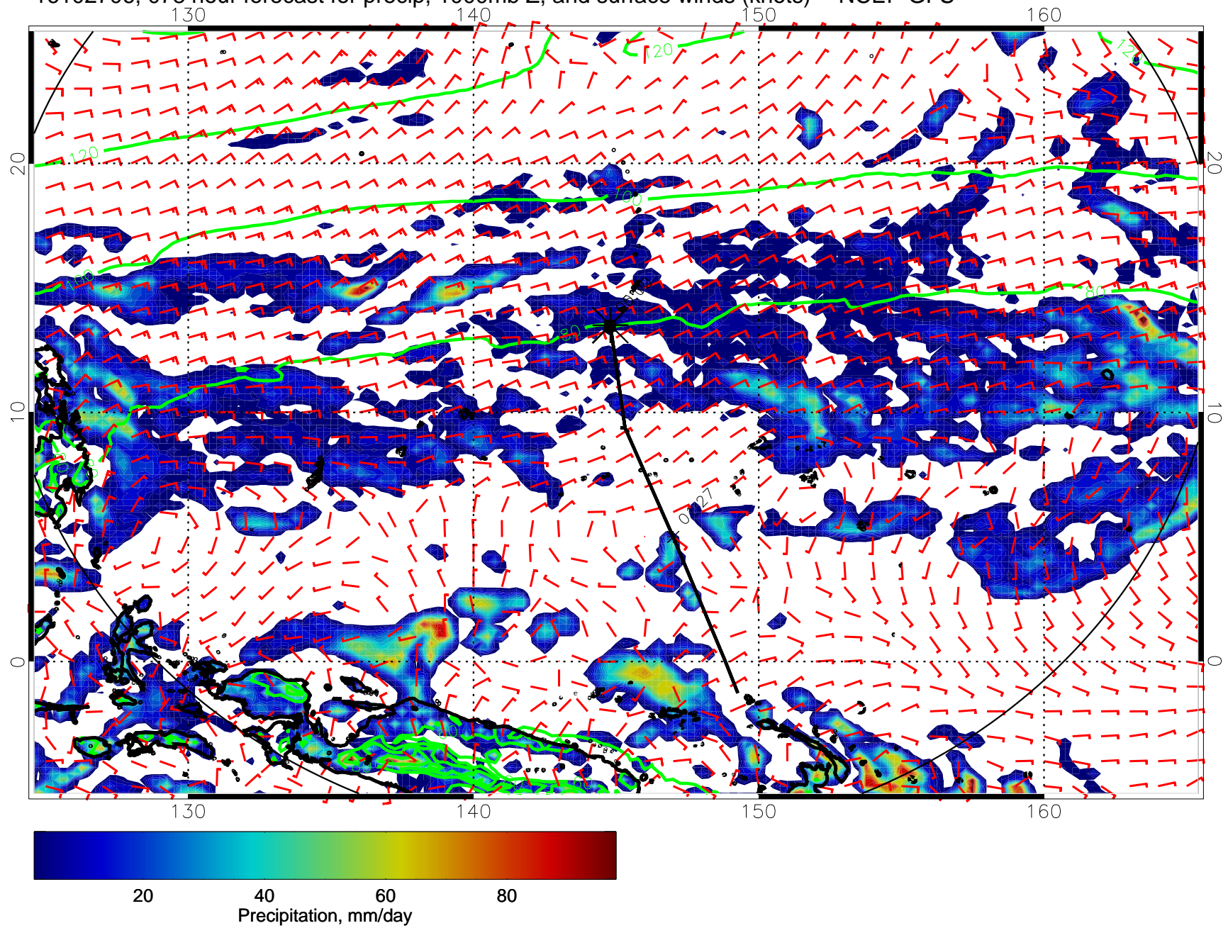
16102706, 078 hour forecast for precip, 1000mb Z, and surface winds (knots) -- NCEP GFS
