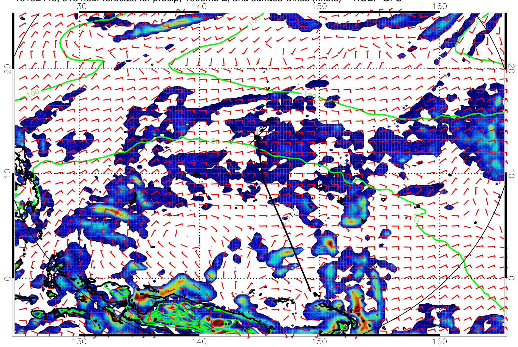
16102418, 018 hour forecast for precip, 1000mb Z, and surface winds (knots) -- NCEP GFS
