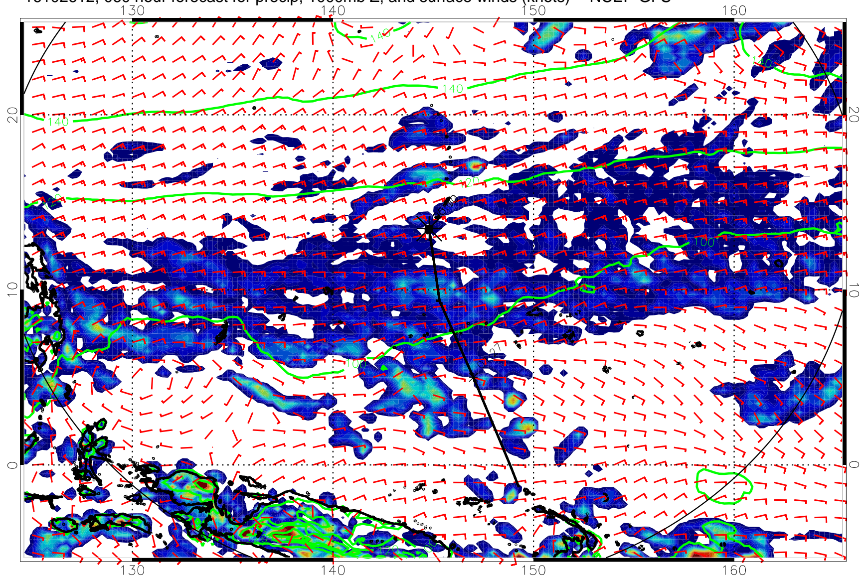
16102612, 060 hour forecast for precip, 1000mb Z, and surface winds (knots) -- NCEP GFS
