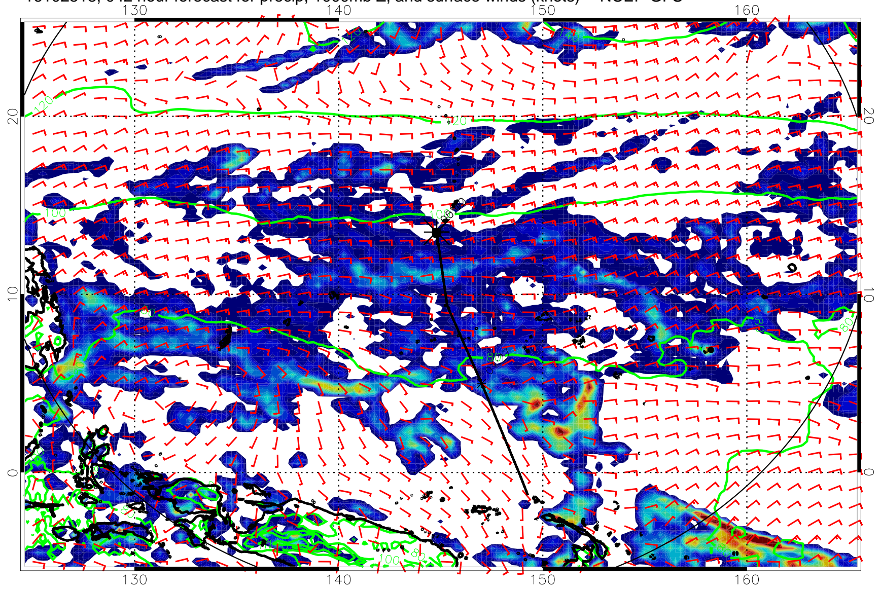
16102518, 042 hour forecast for precip, 1000mb Z, and surface winds (knots) -- NCEP GFS
