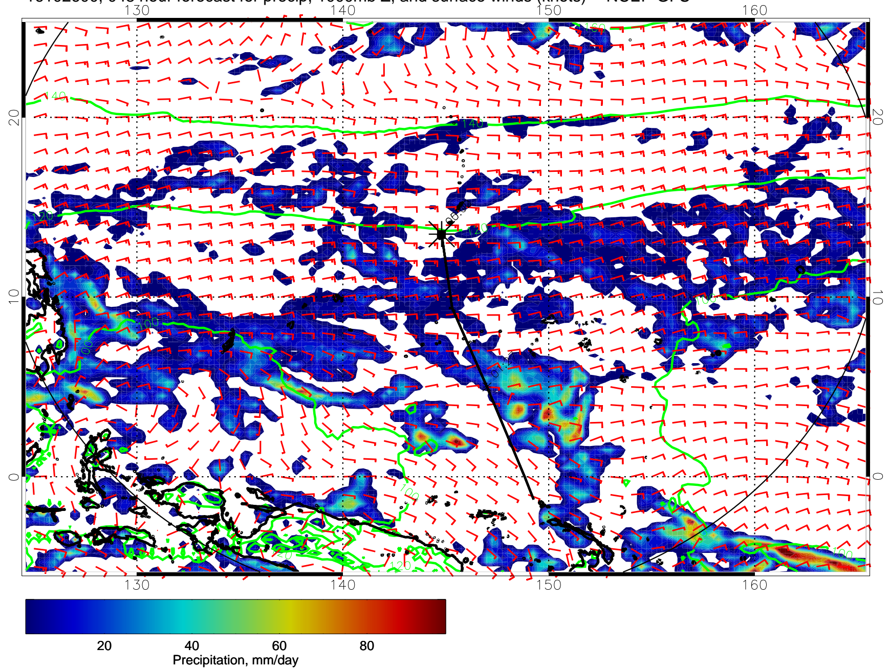
16102600, 048 hour forecast for precip, 1000mb Z, and surface winds (knots) -- NCEP GFS
