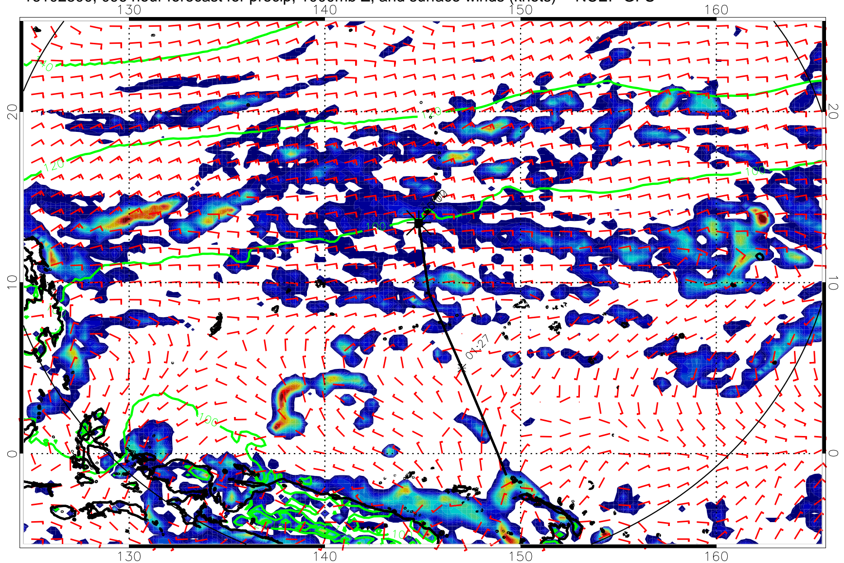
16102800, 096 hour forecast for precip, 1000mb Z, and surface winds (knots) -- NCEP GFS
