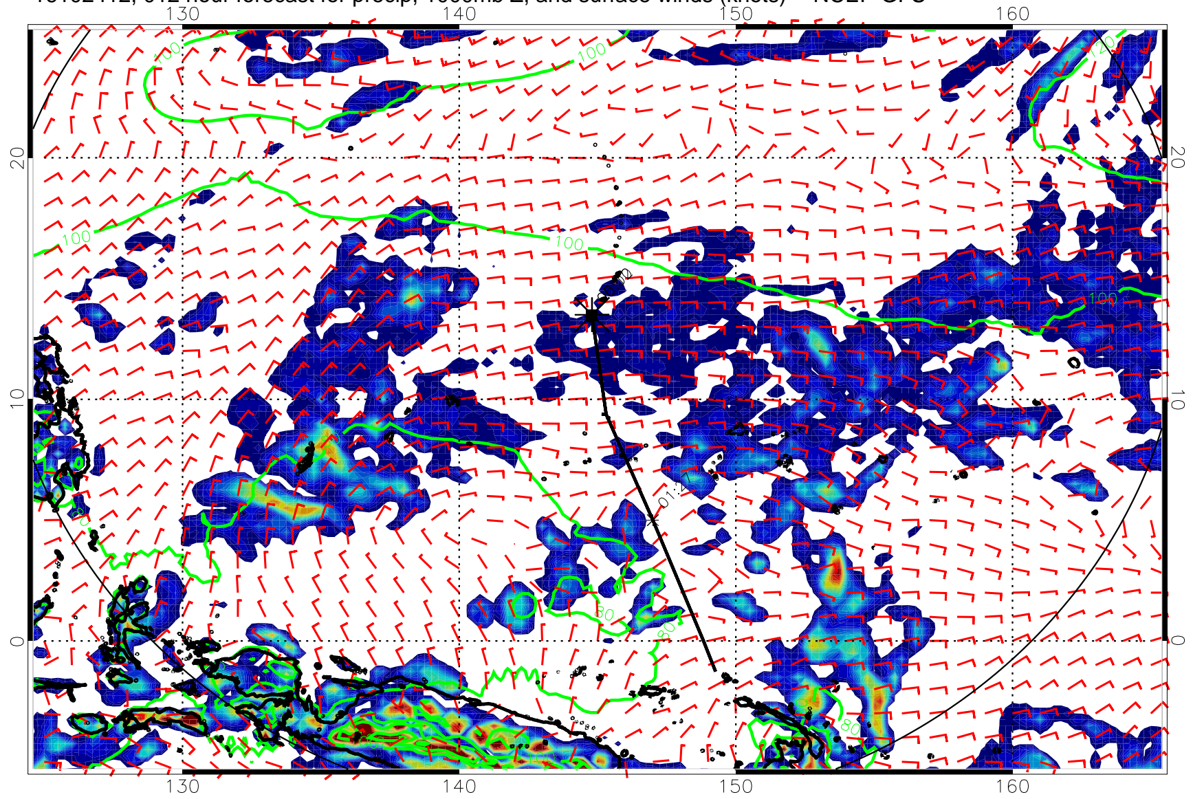
16102412, 012 hour forecast for precip, 1000mb Z, and surface winds (knots) -- NCEP GFS
