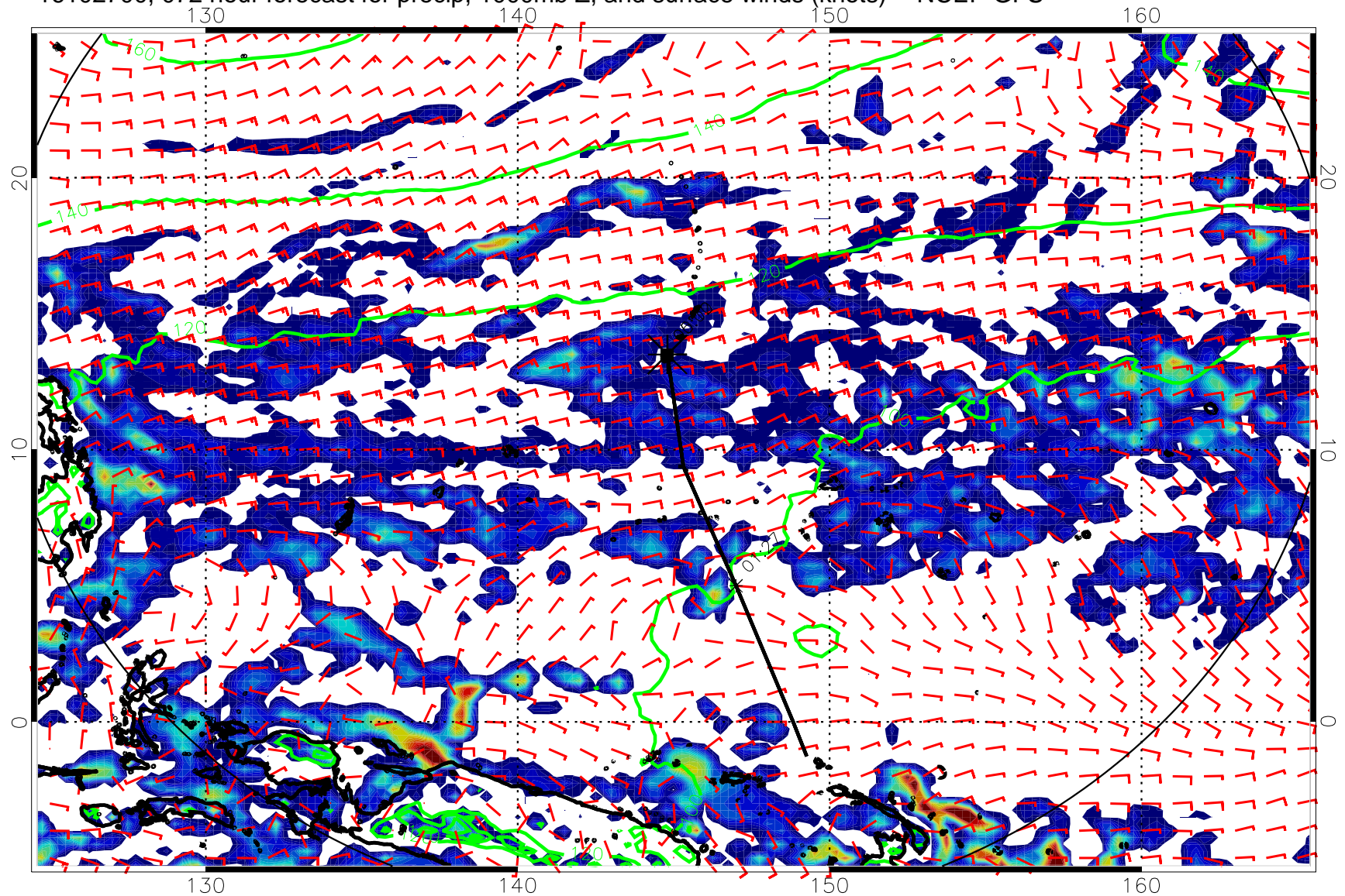
16102700, 072 hour forecast for precip, 1000mb Z, and surface winds (knots) -- NCEP GFS
