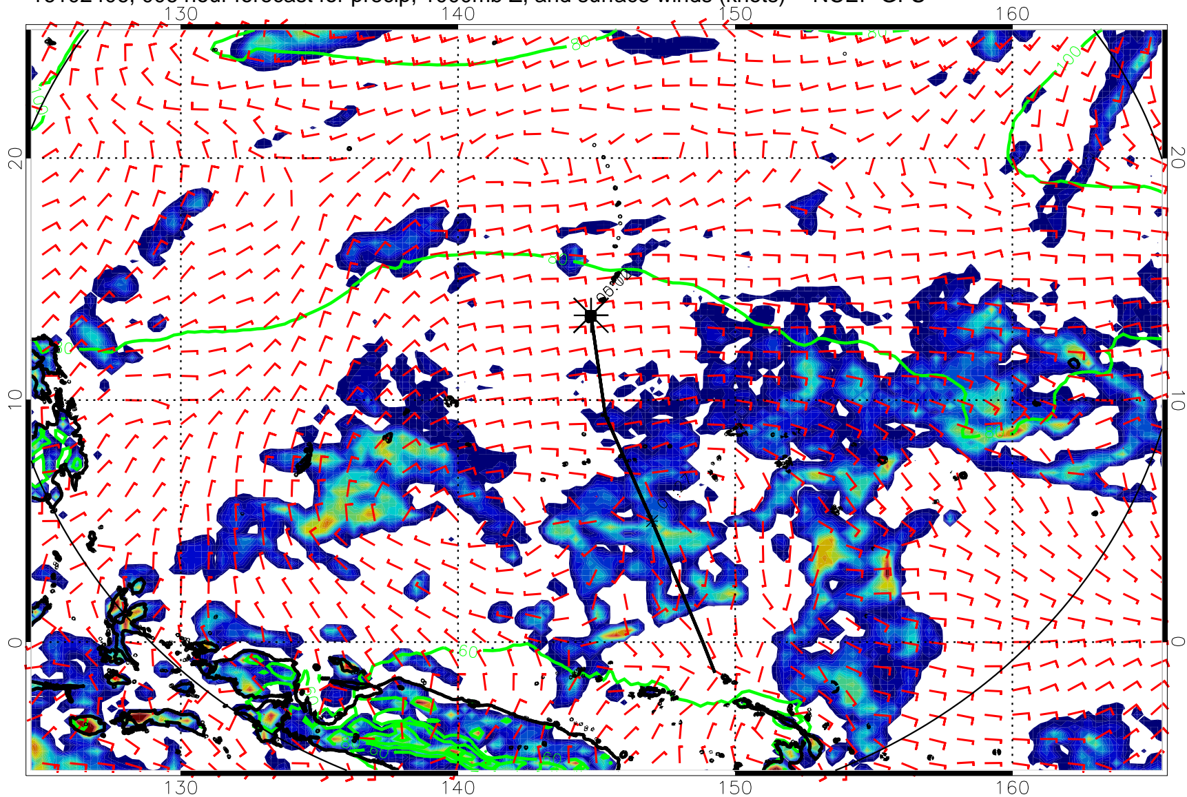
16102406, 006 hour forecast for precip, 1000mb Z, and surface winds (knots) -- NCEP GFS
