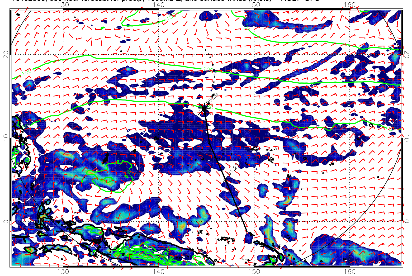
16102506, 030 hour forecast for precip, 1000mb Z, and surface winds (knots) -- NCEP GFS
