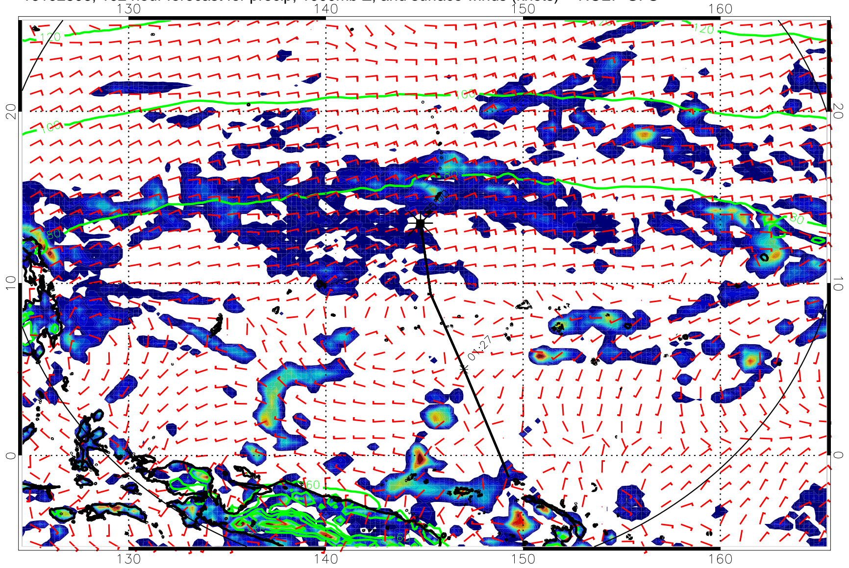
16102806, 102 hour forecast for precip, 1000mb Z, and surface winds (knots) -- NCEP GFS
