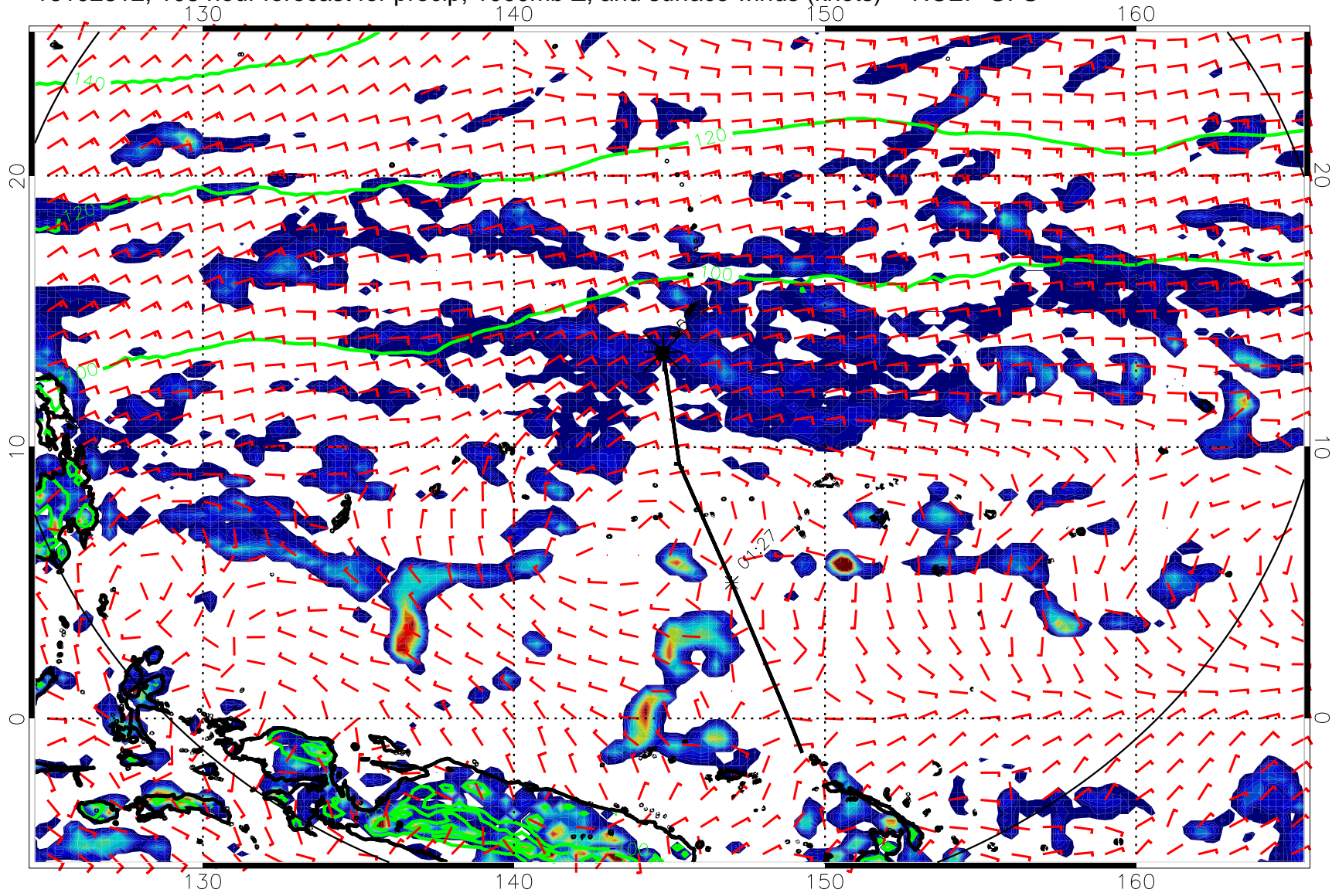
16102812, 108 hour forecast for precip, 1000mb Z, and surface winds (knots) -- NCEP GFS
