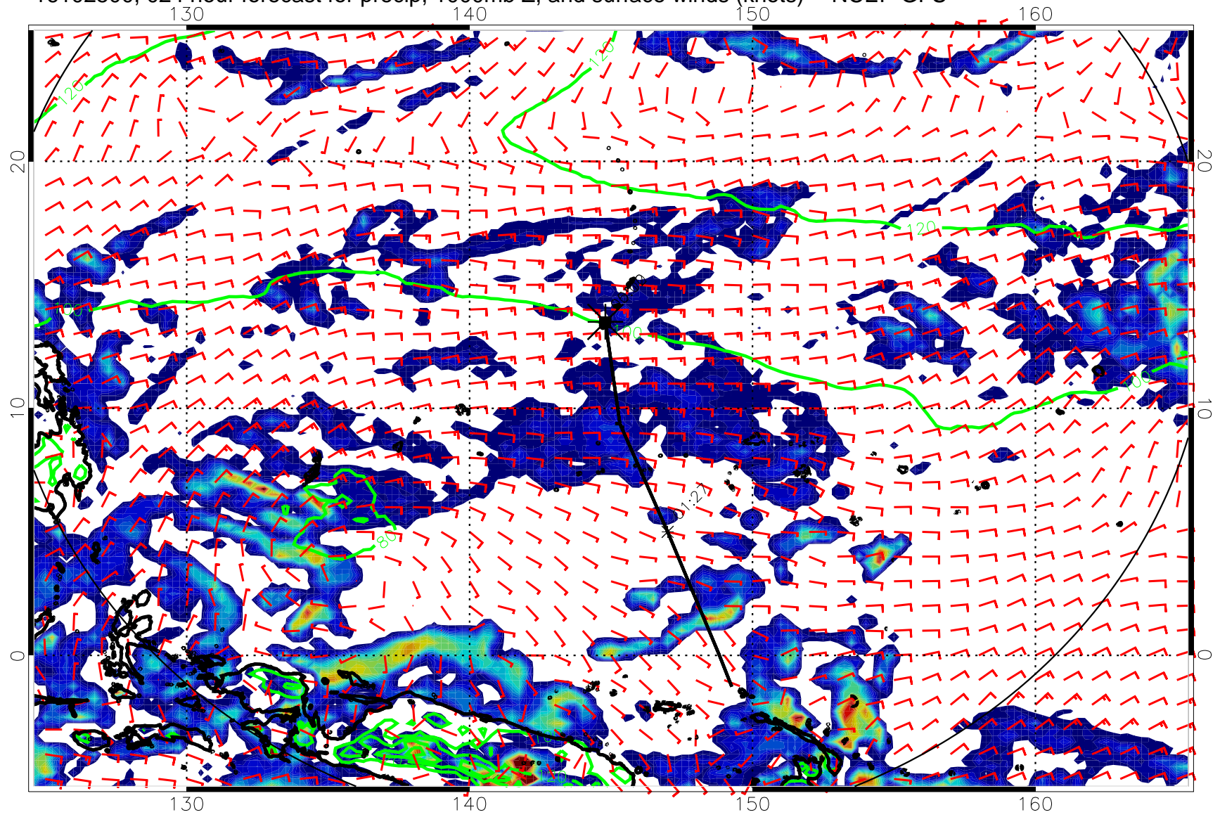
16102500, 024 hour forecast for precip, 1000mb Z, and surface winds (knots) -- NCEP GFS
