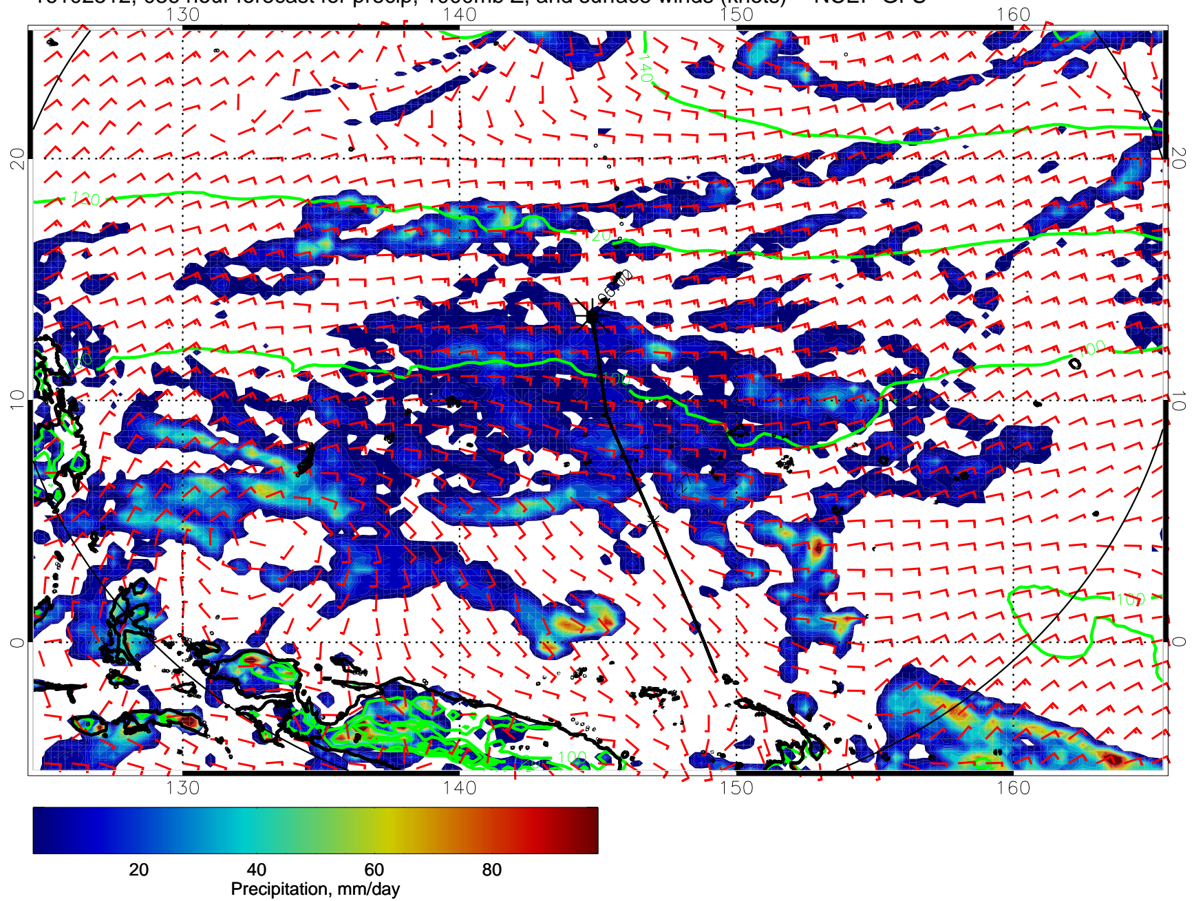
16102512, 036 hour forecast for precip, 1000mb Z, and surface winds (knots) -- NCEP GFS
