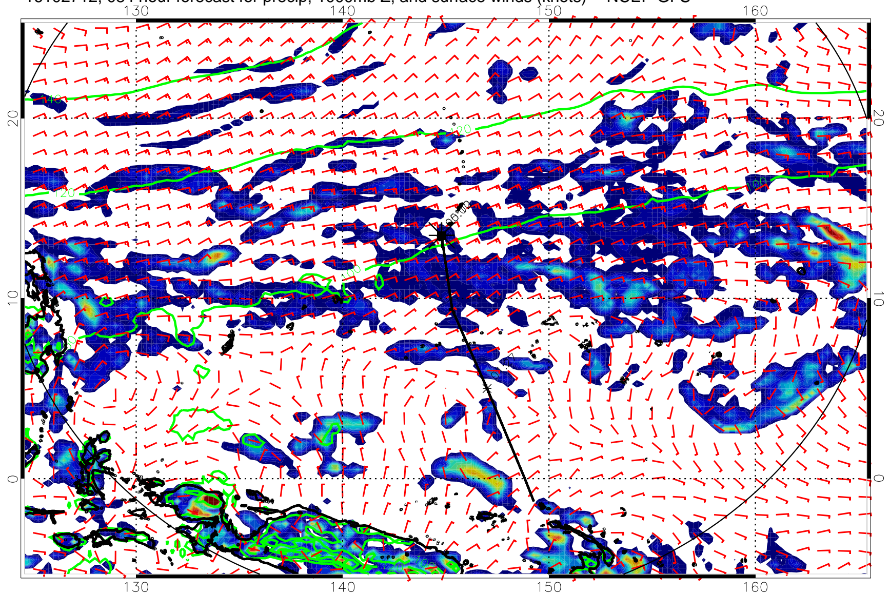
16102712, 084 hour forecast for precip, 1000mb Z, and surface winds (knots) -- NCEP GFS
