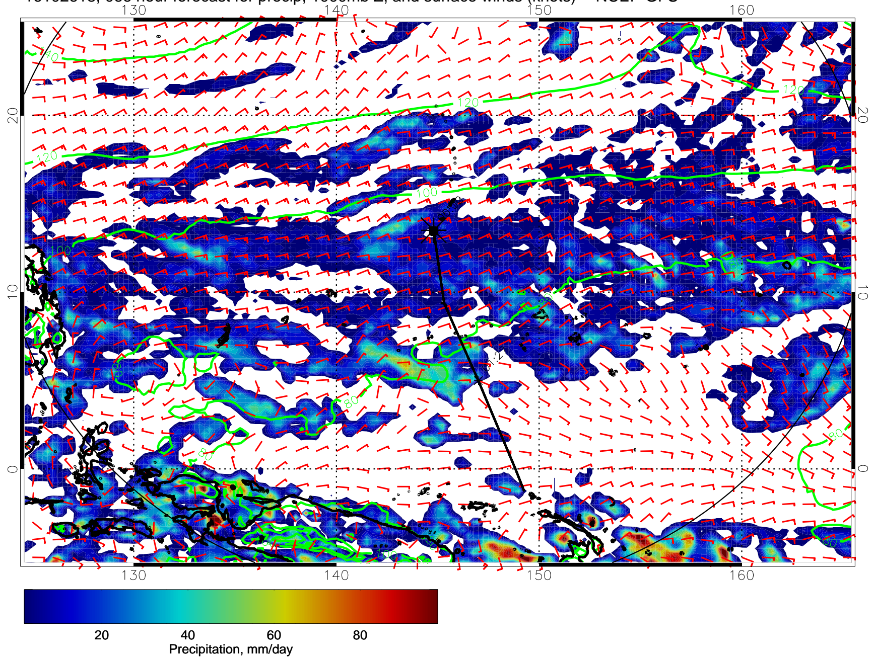
16102618, 066 hour forecast for precip, 1000mb Z, and surface winds (knots) -- NCEP GFS
