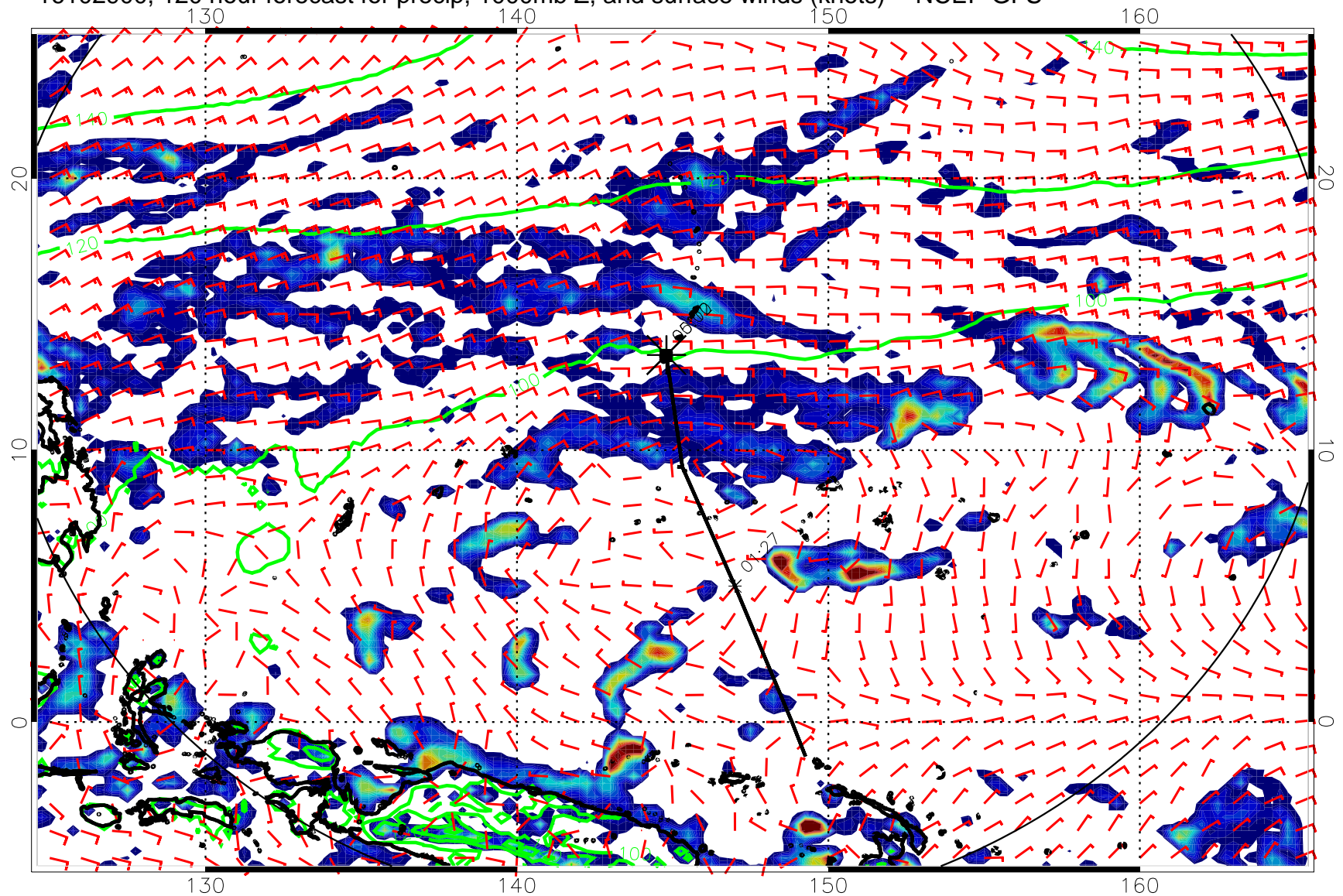
16102900, 120 hour forecast for precip, 1000mb Z, and surface winds (knots) -- NCEP GFS
