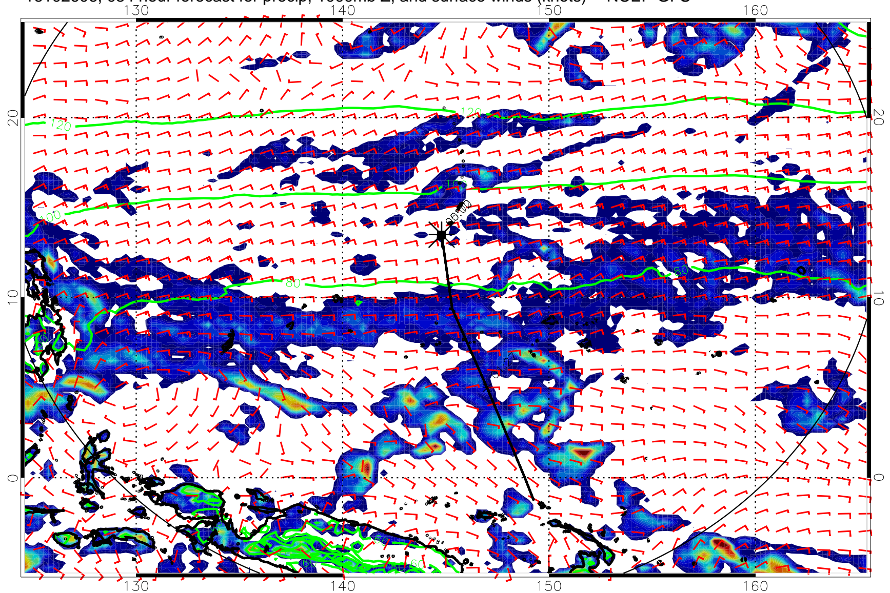
16102606, 054 hour forecast for precip, 1000mb Z, and surface winds (knots) -- NCEP GFS
