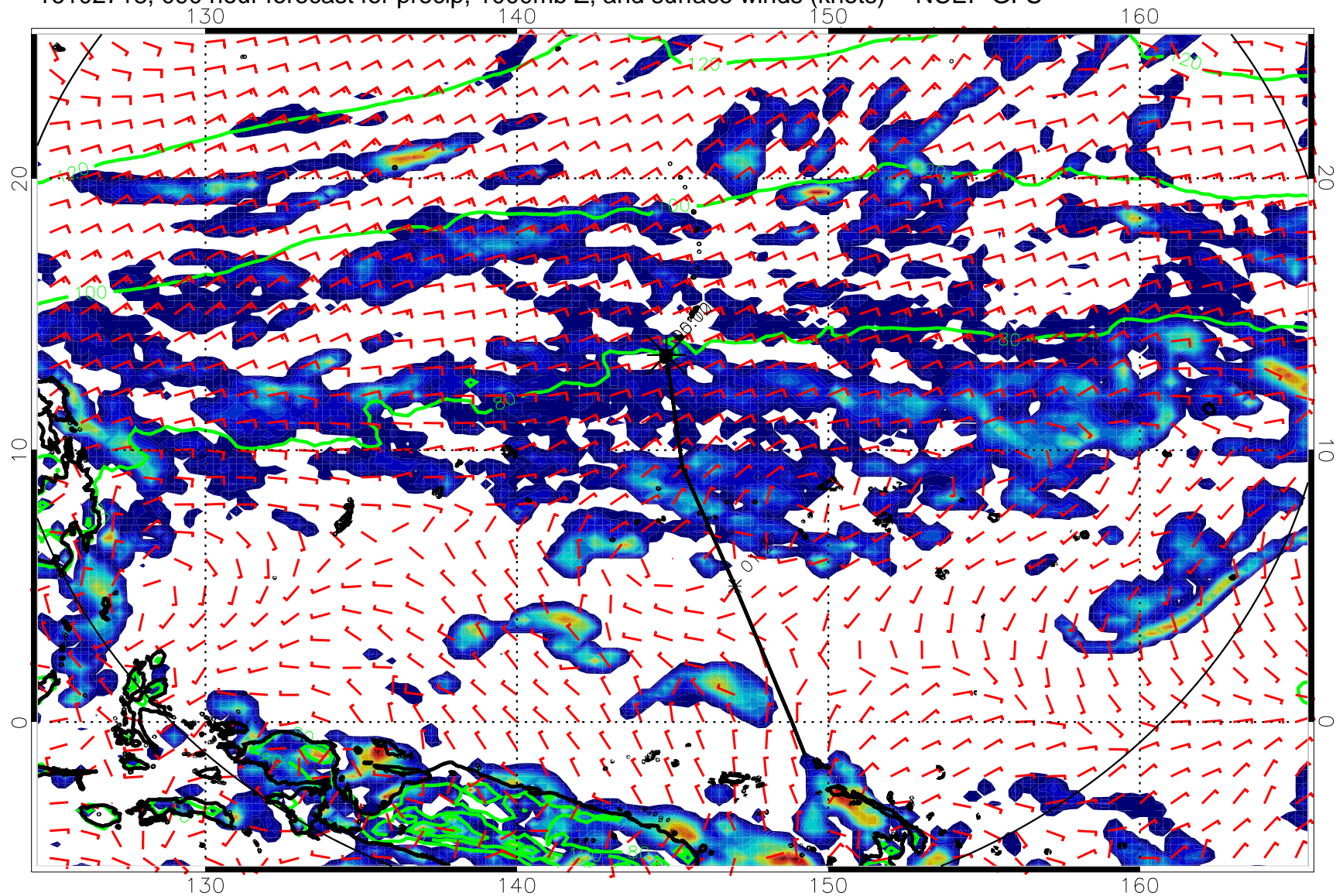
16102718, 090 hour forecast for precip, 1000mb Z, and surface winds (knots) -- NCEP GFS
