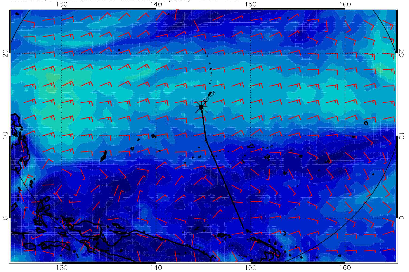
16102700, 072 hour forecast for surface winds (knots) -- NCEP GFS
