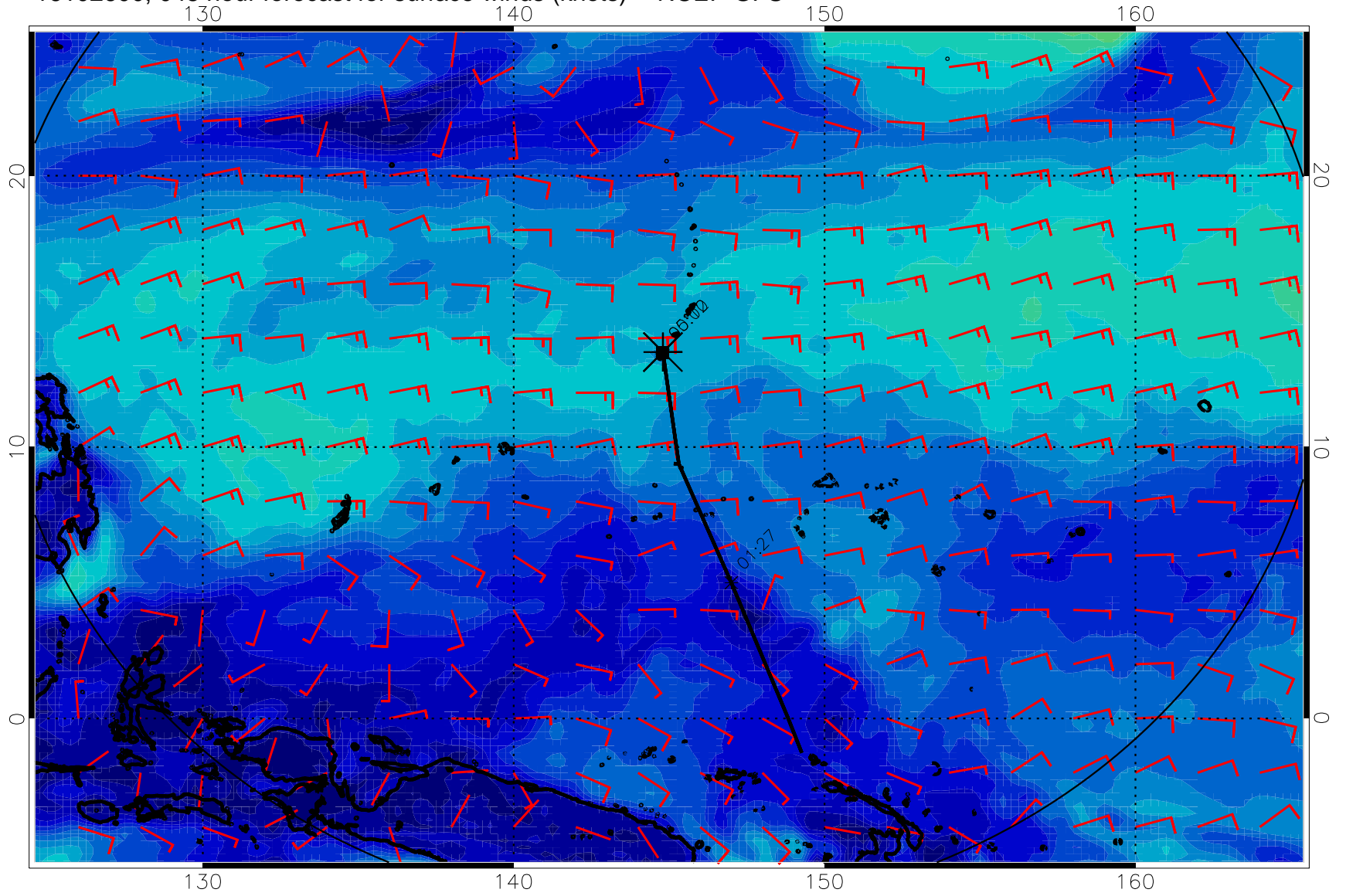
16102600, 048 hour forecast for surface winds (knots) -- NCEP GFS
