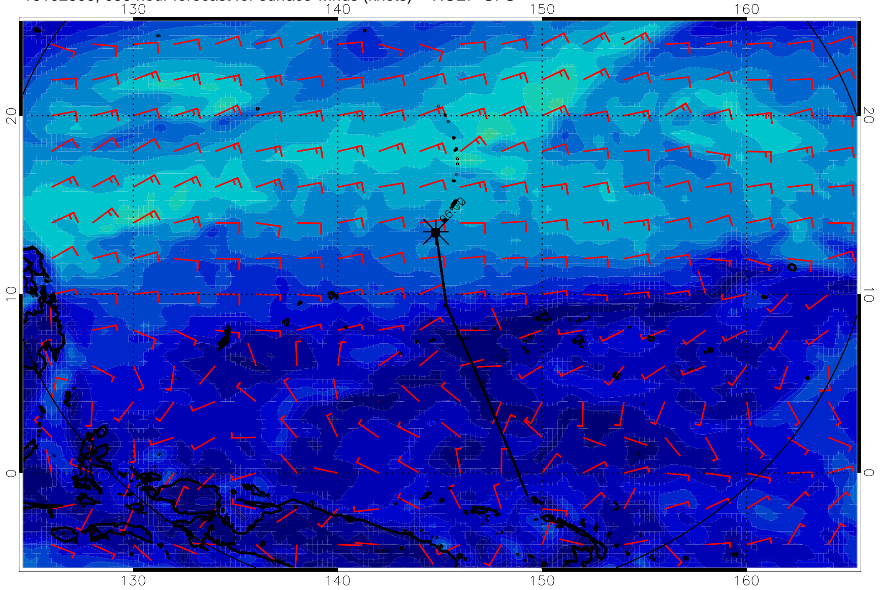
16102800, 096 hour forecast for surface winds (knots) -- NCEP GFS
