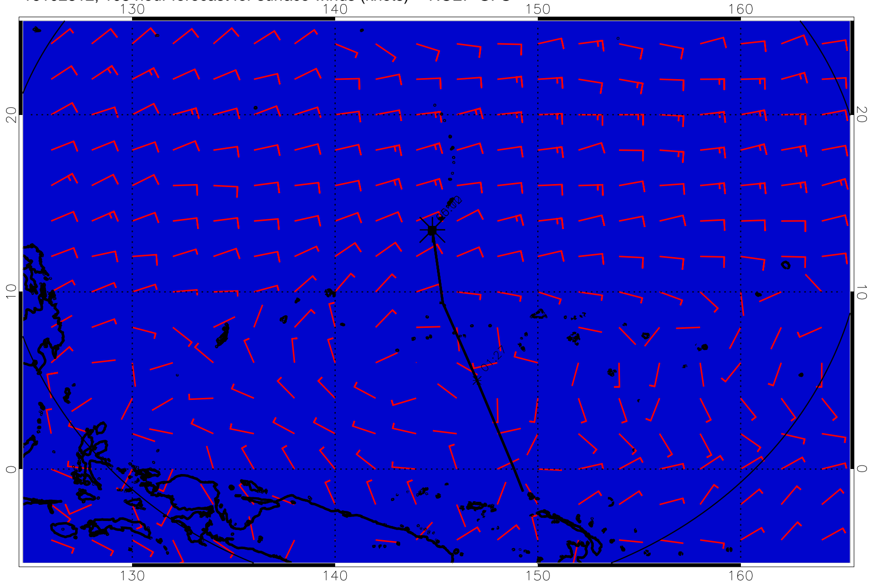
16102812, 108 hour forecast for surface winds (knots) -- NCEP GFS
