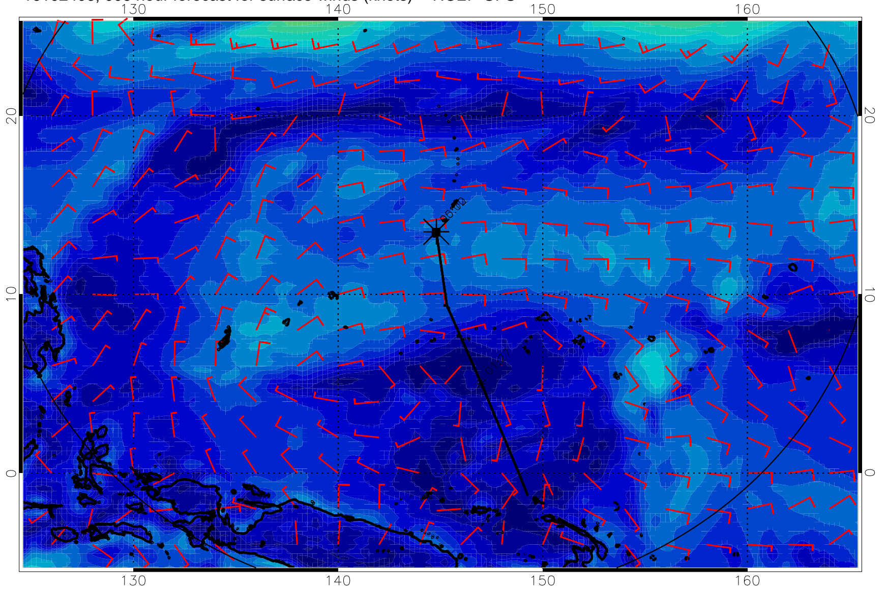
16102406, 006 hour forecast for surface winds (knots) -- NCEP GFS
