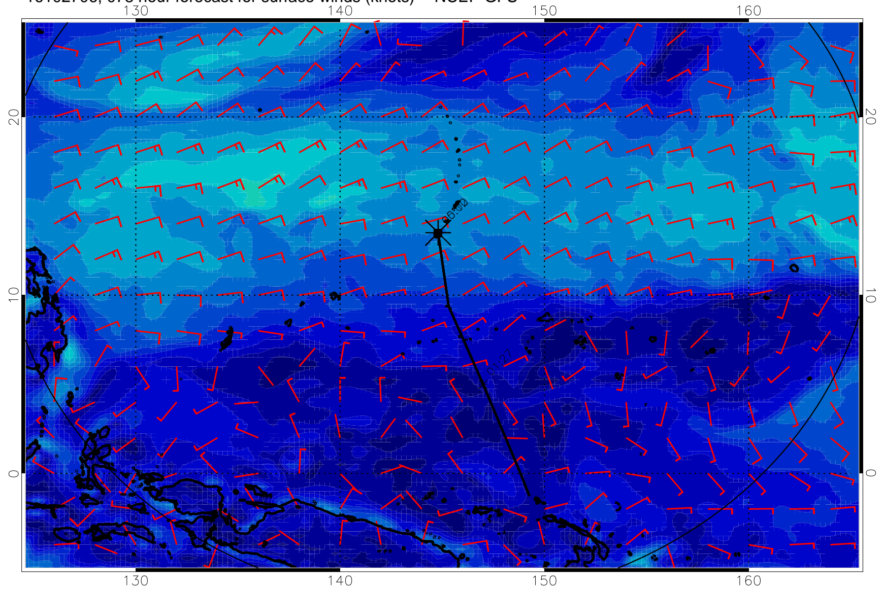
16102706, 078 hour forecast for surface winds (knots) -- NCEP GFS
