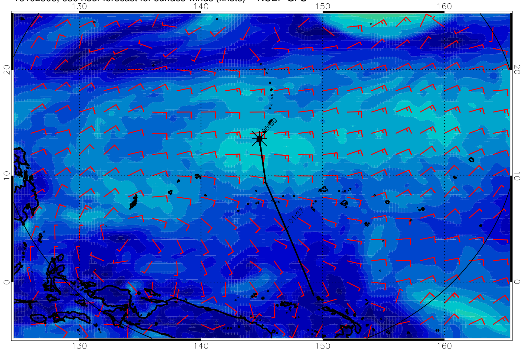
16102506, 030 hour forecast for surface winds (knots) -- NCEP GFS
