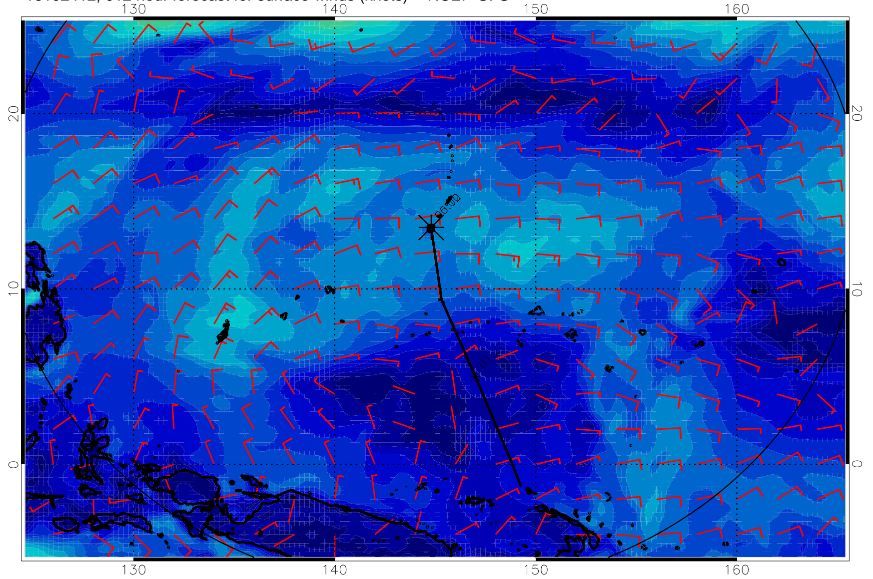
16102412, 012 hour forecast for surface winds (knots) -- NCEP GFS
