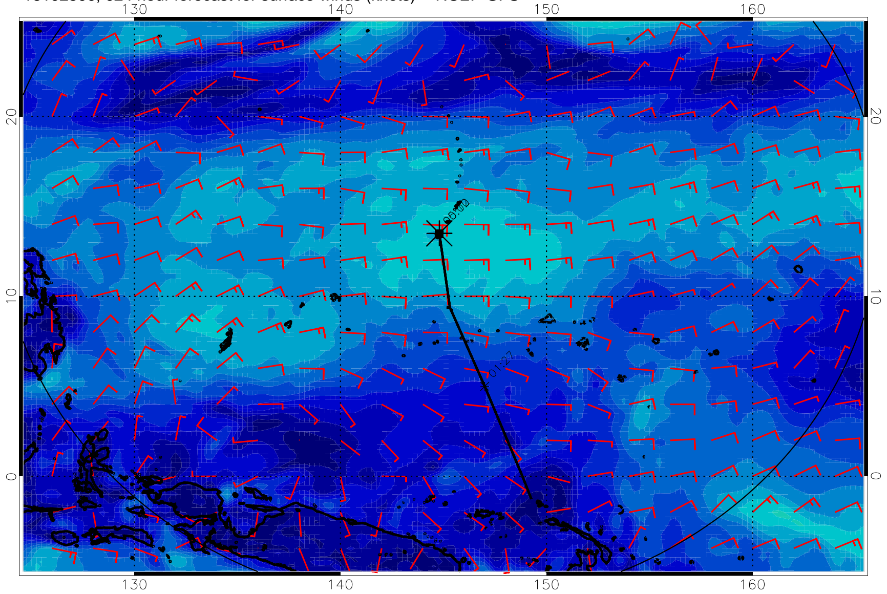
16102500, 024 hour forecast for surface winds (knots) -- NCEP GFS
