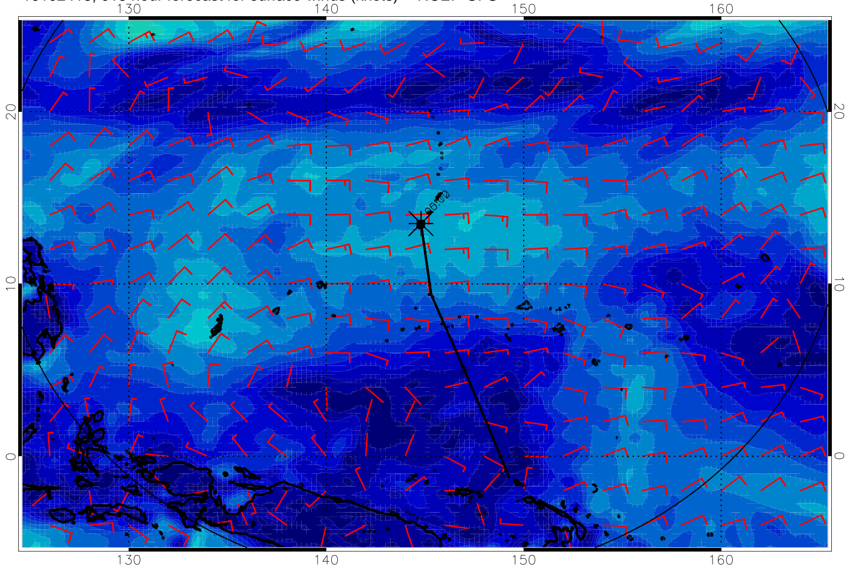
16102418, 018 hour forecast for surface winds (knots) -- NCEP GFS
