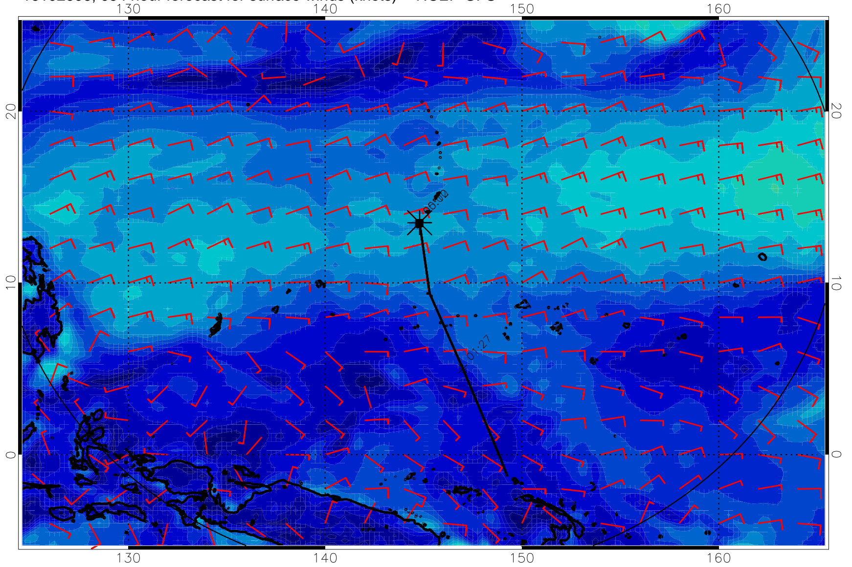
16102606, 054 hour forecast for surface winds (knots) -- NCEP GFS
