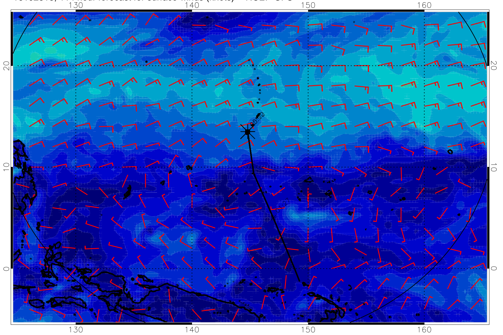
16102818, 114 hour forecast for surface winds (knots) -- NCEP GFS
