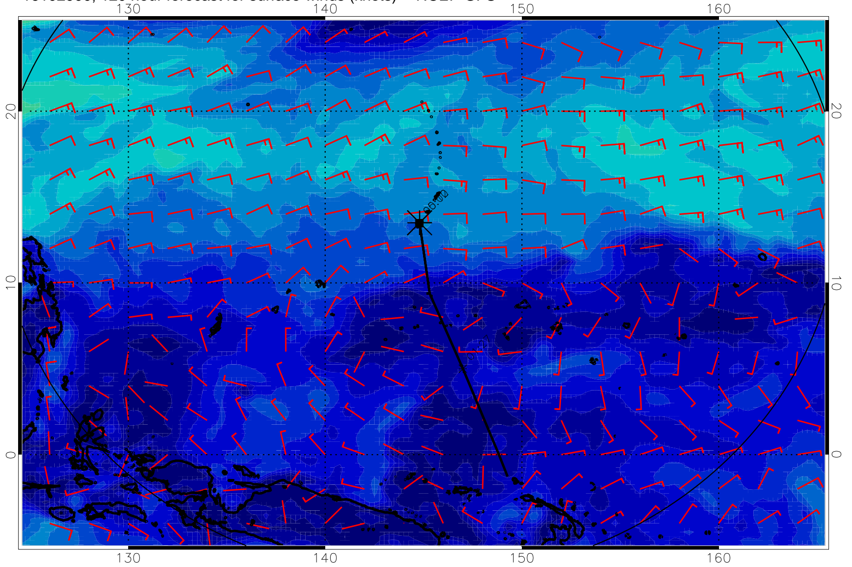
16102900, 120 hour forecast for surface winds (knots) -- NCEP GFS
