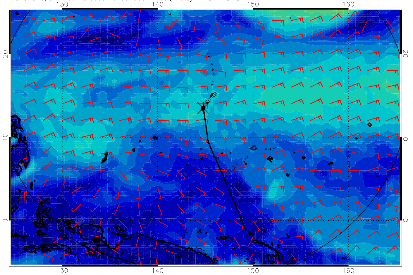
16102518, 042 hour forecast for surface winds (knots) -- NCEP GFS
