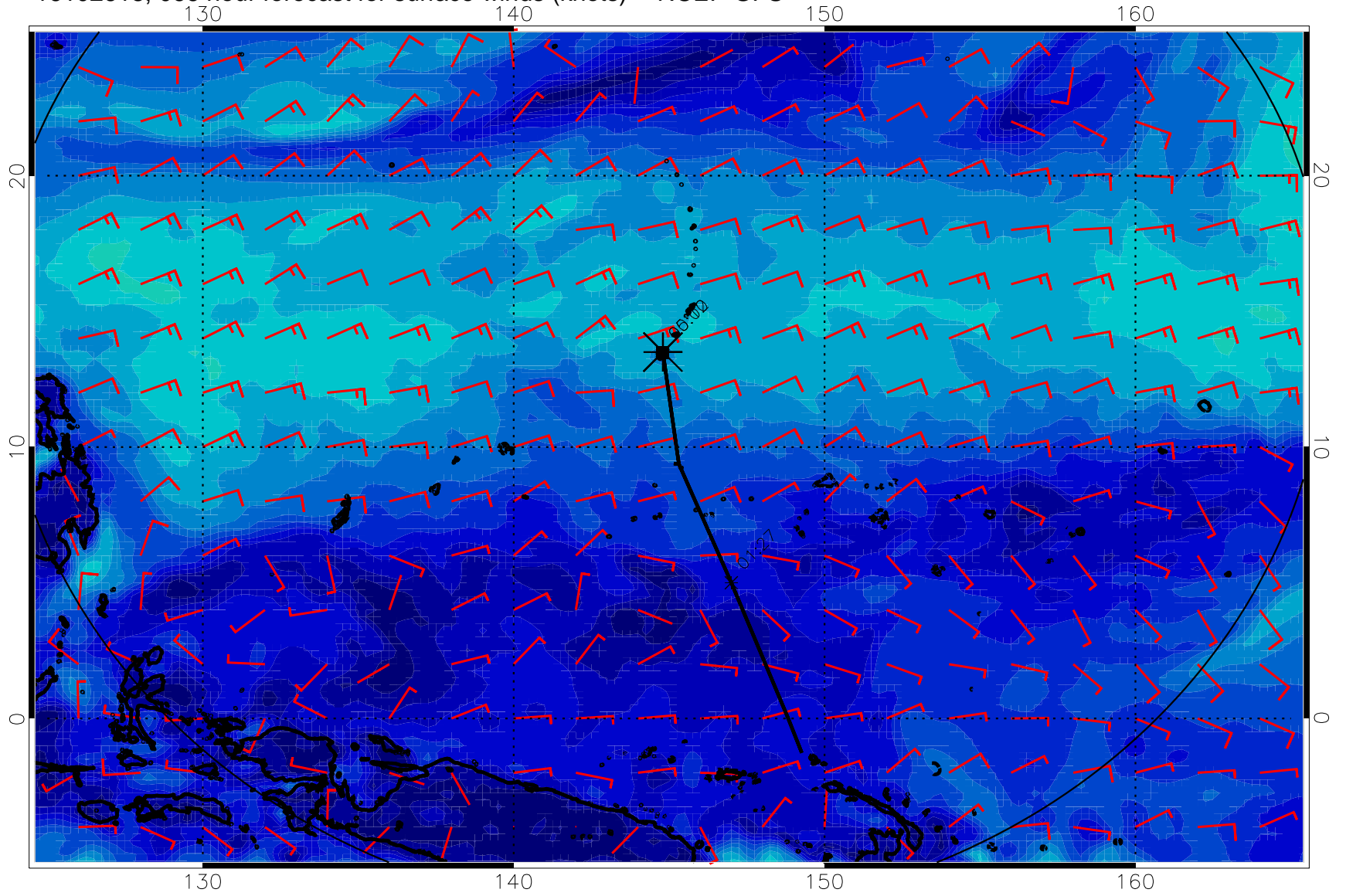
16102618, 066 hour forecast for surface winds (knots) -- NCEP GFS
