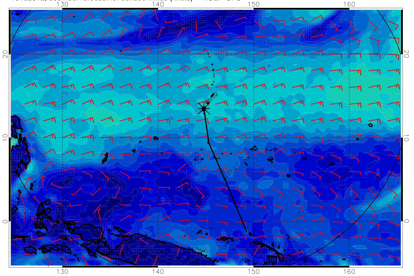
16102612, 060 hour forecast for surface winds (knots) -- NCEP GFS
