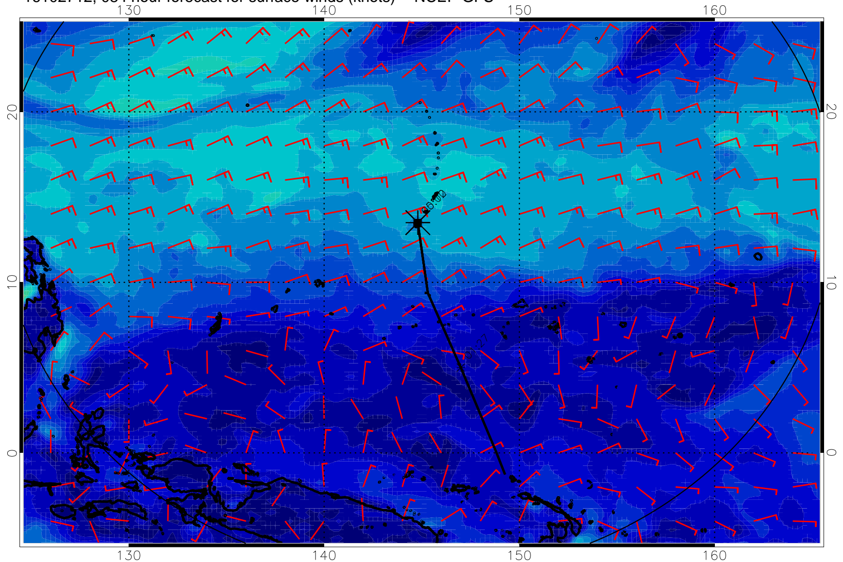
16102712, 084 hour forecast for surface winds (knots) -- NCEP GFS
