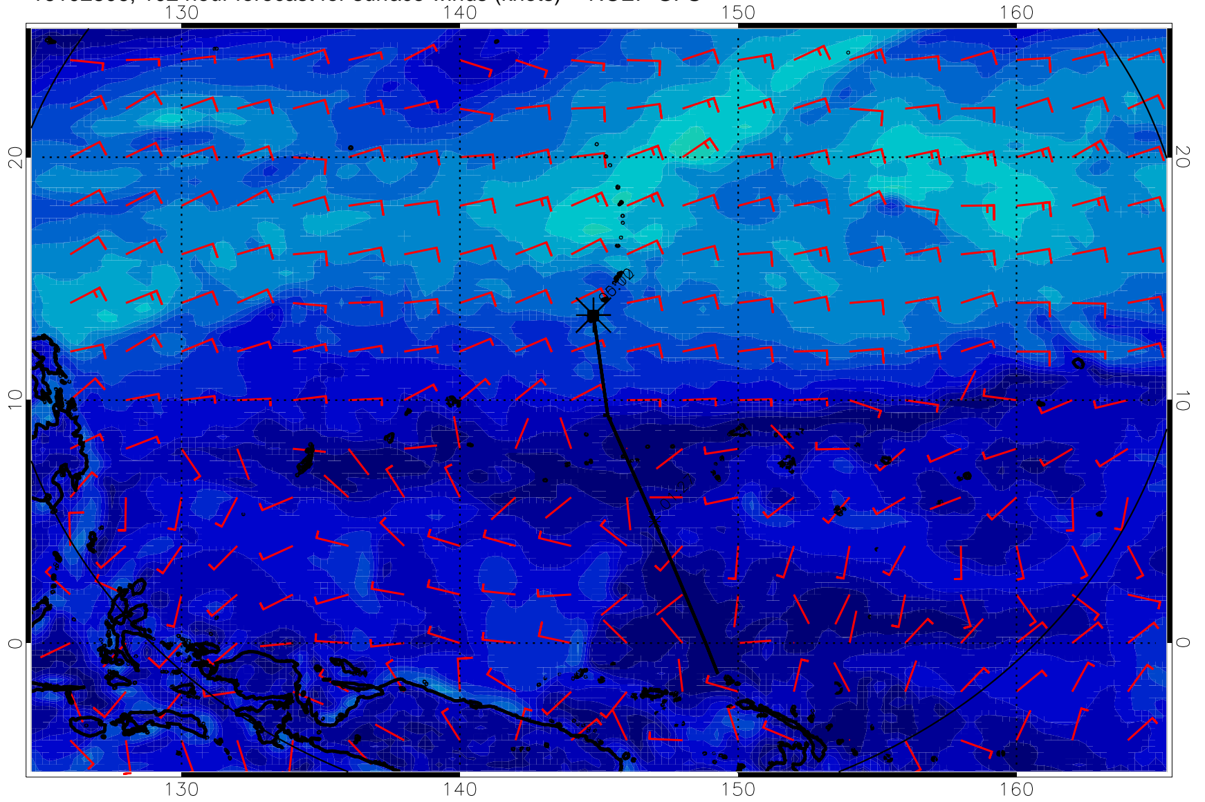
16102806, 102 hour forecast for surface winds (knots) -- NCEP GFS
