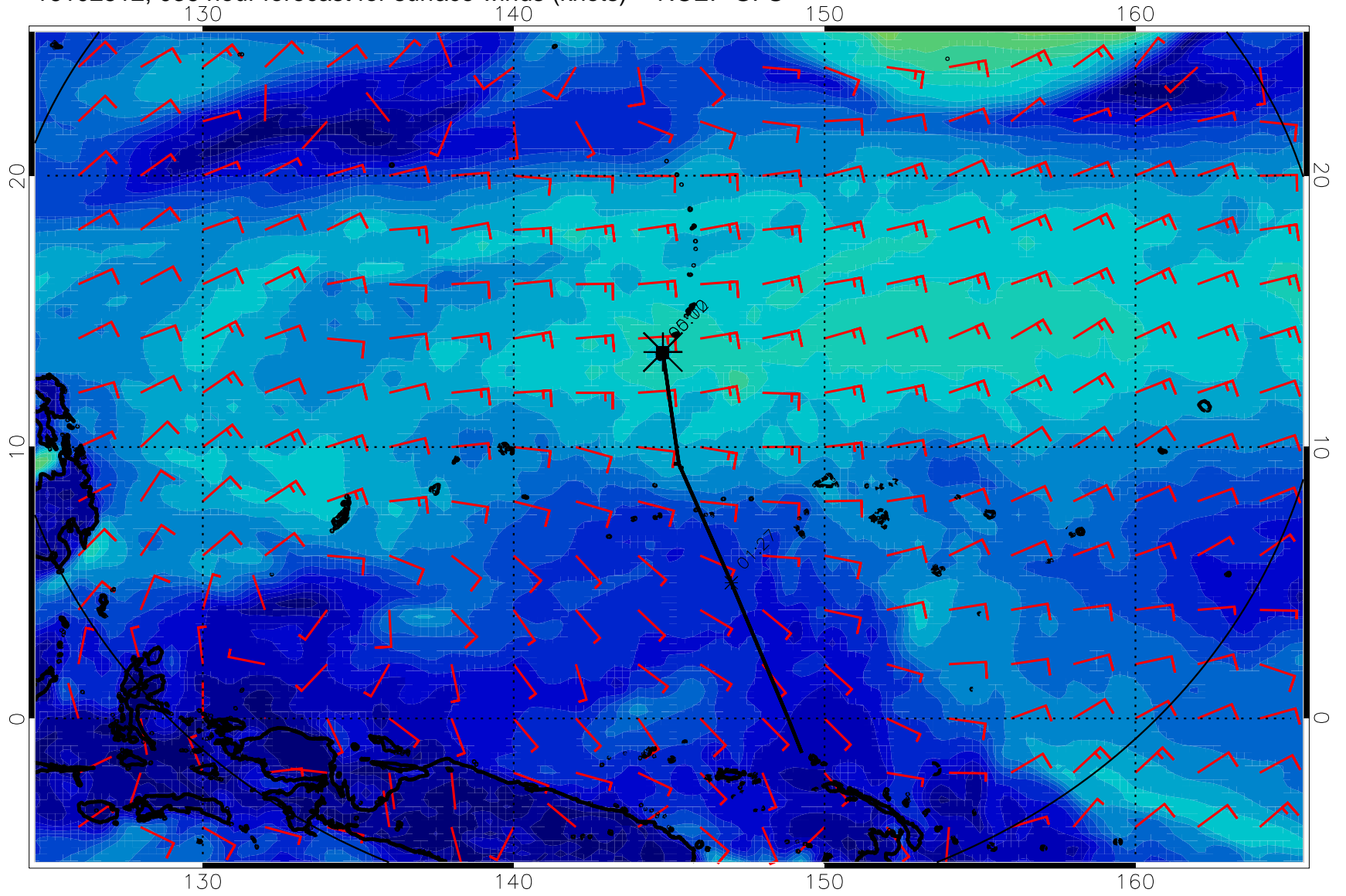
16102512, 036 hour forecast for surface winds (knots) -- NCEP GFS
