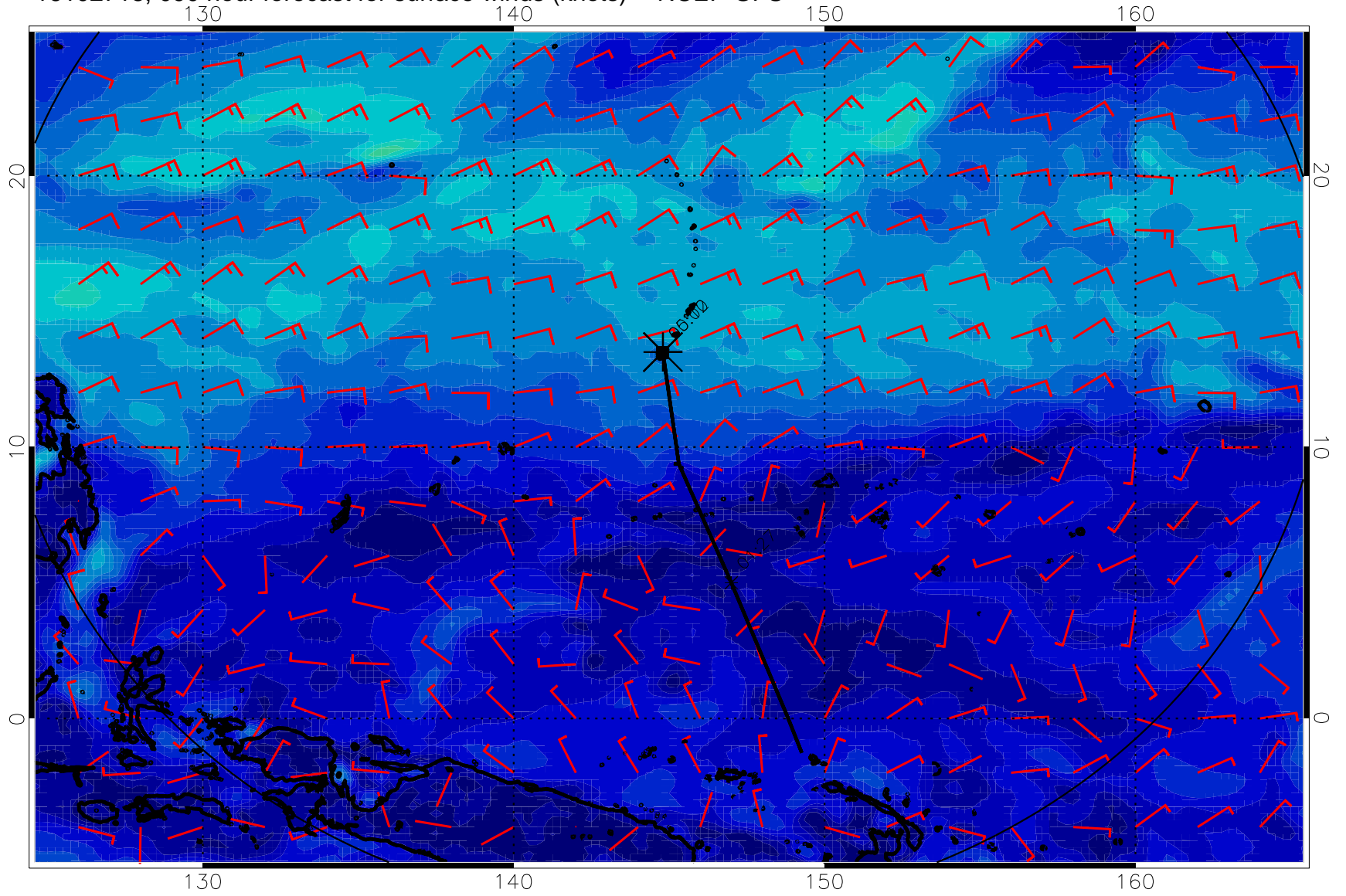
16102718, 090 hour forecast for surface winds (knots) -- NCEP GFS
