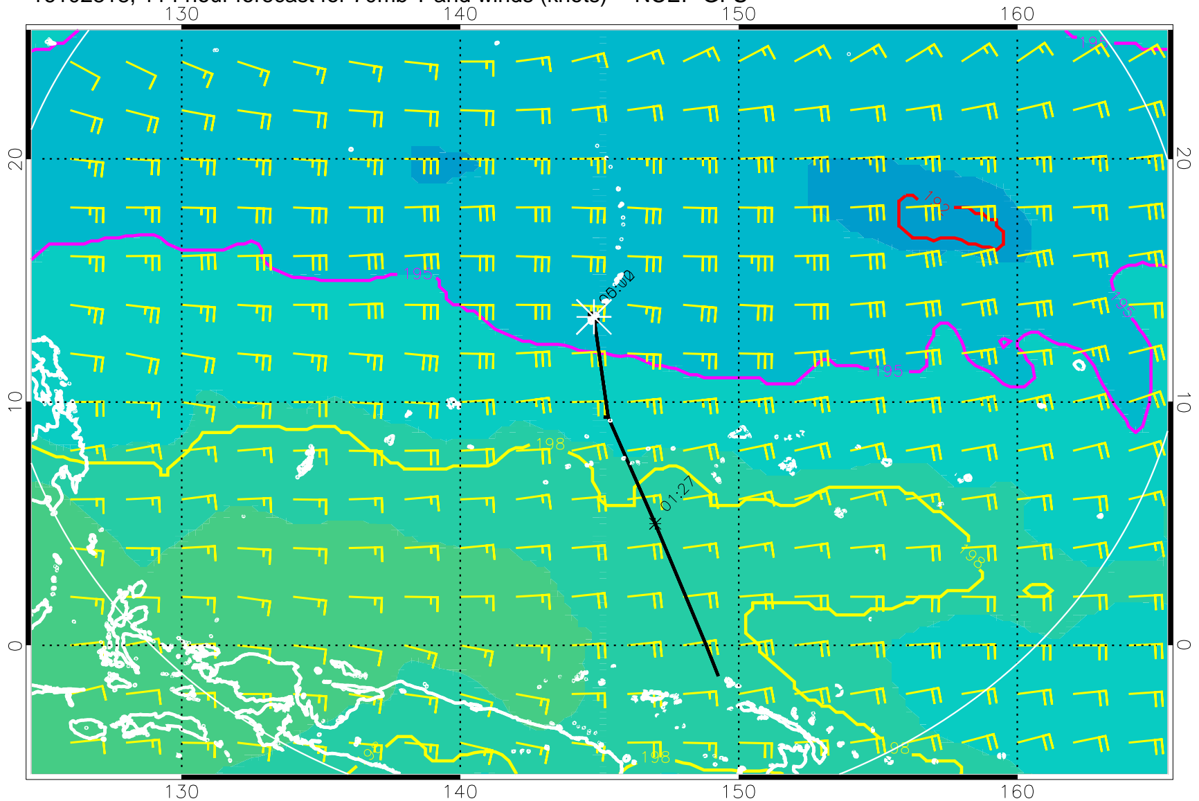
16102818, 114 hour forecast for 70mb T and winds (knots) -- NCEP GFS
