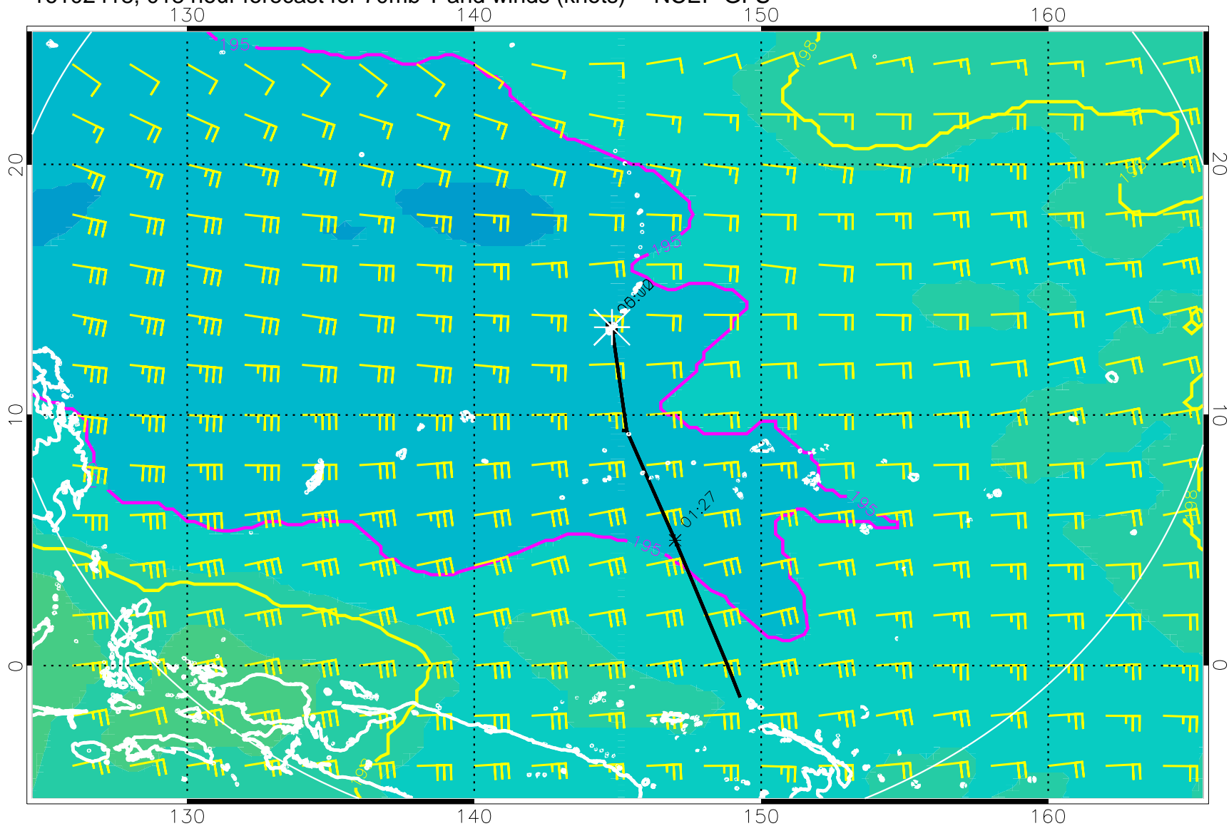
16102418, 018 hour forecast for 70mb T and winds (knots) -- NCEP GFS
