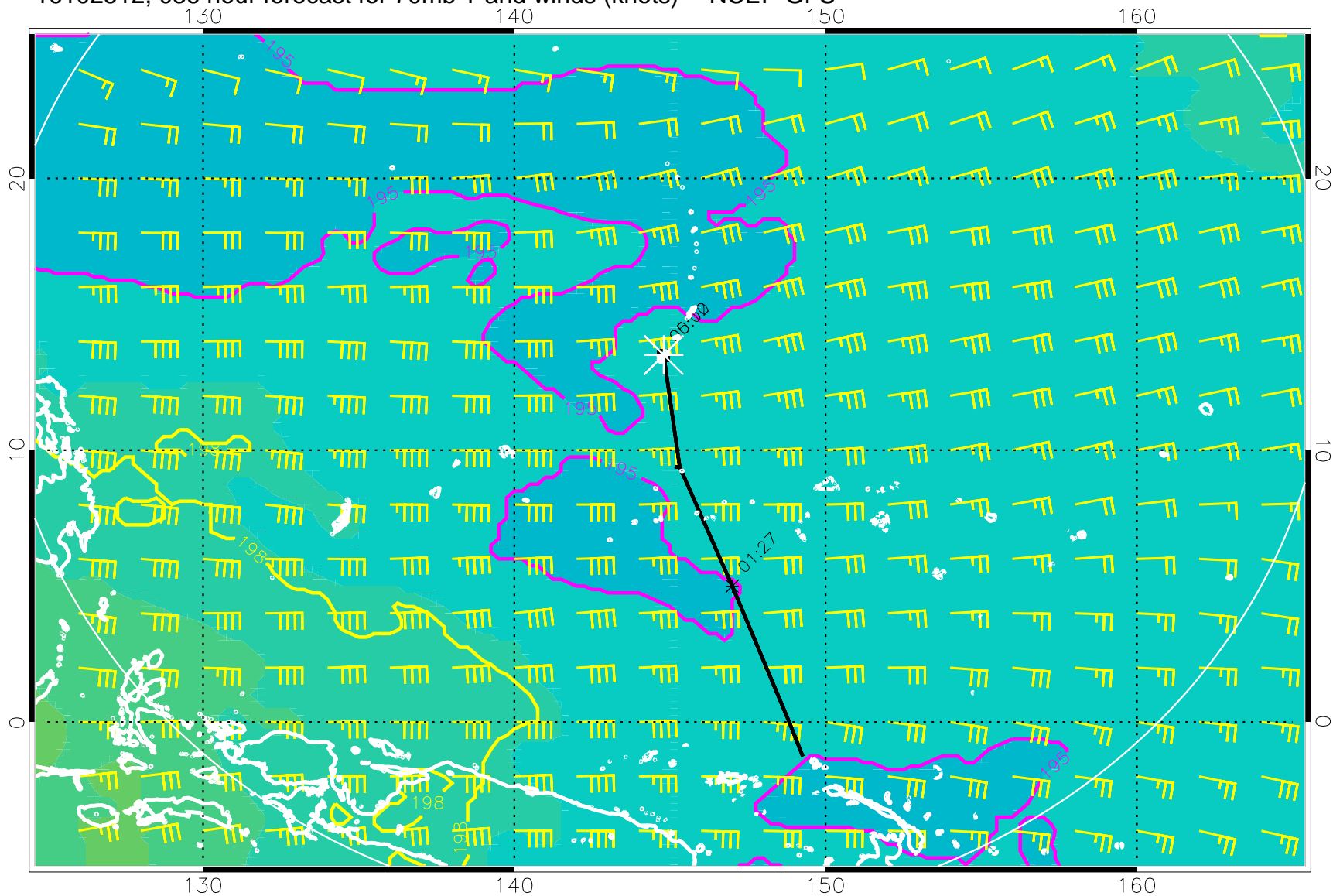
16102512, 036 hour forecast for 70mb T and winds (knots) -- NCEP GFS
