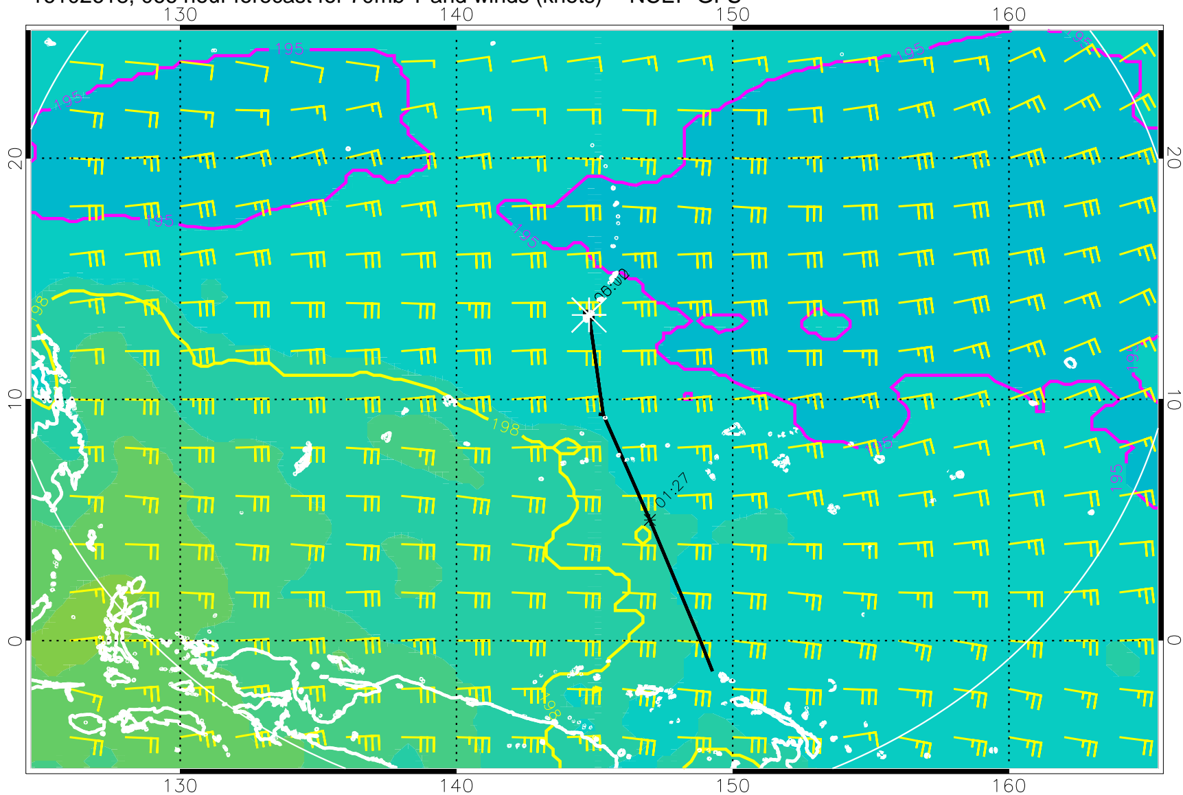
16102618, 066 hour forecast for 70mb T and winds (knots) -- NCEP GFS
