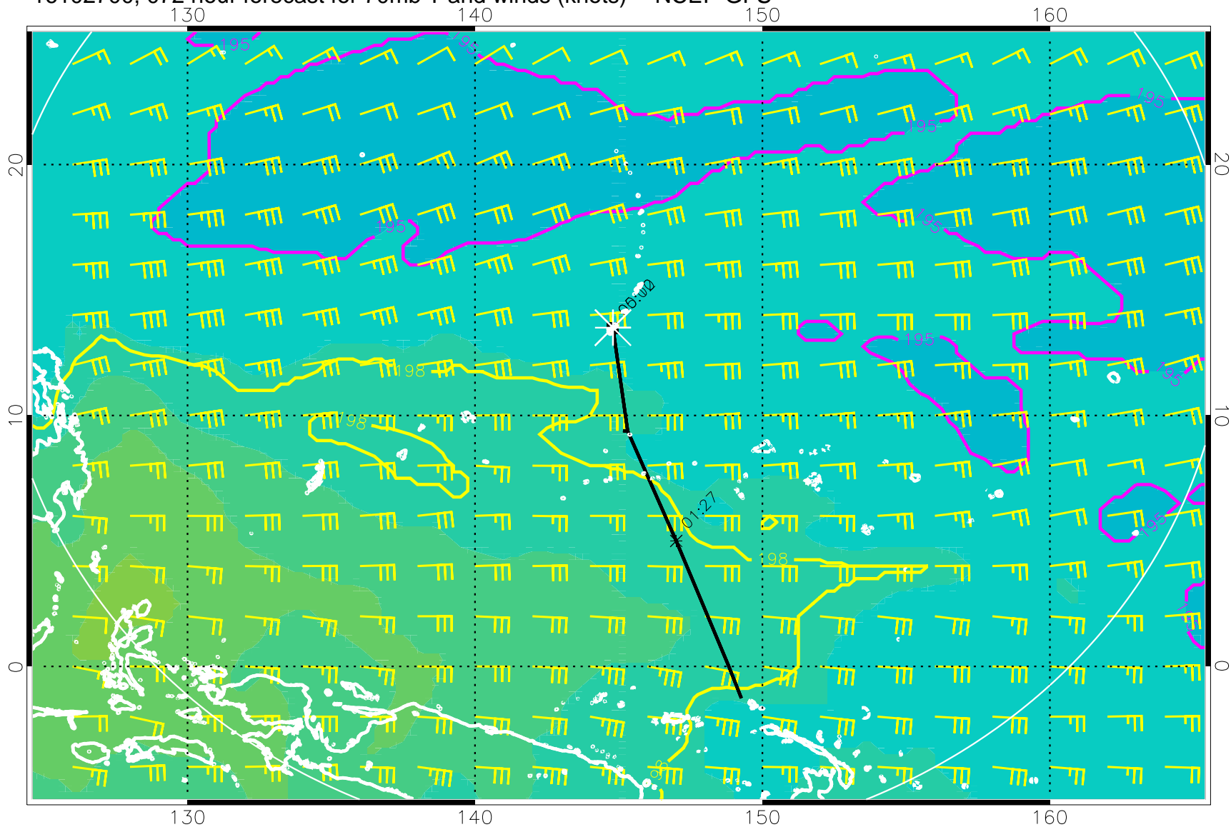
16102700, 072 hour forecast for 70mb T and winds (knots) -- NCEP GFS
