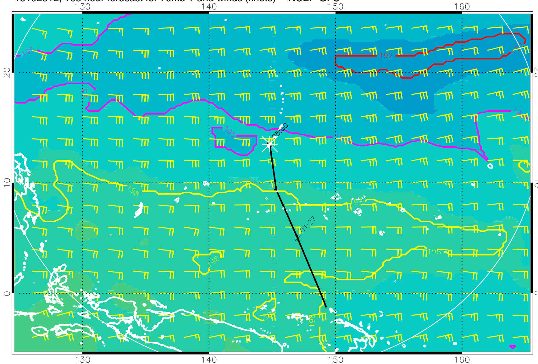
16102812, 108 hour forecast for 70mb T and winds (knots) -- NCEP GFS
