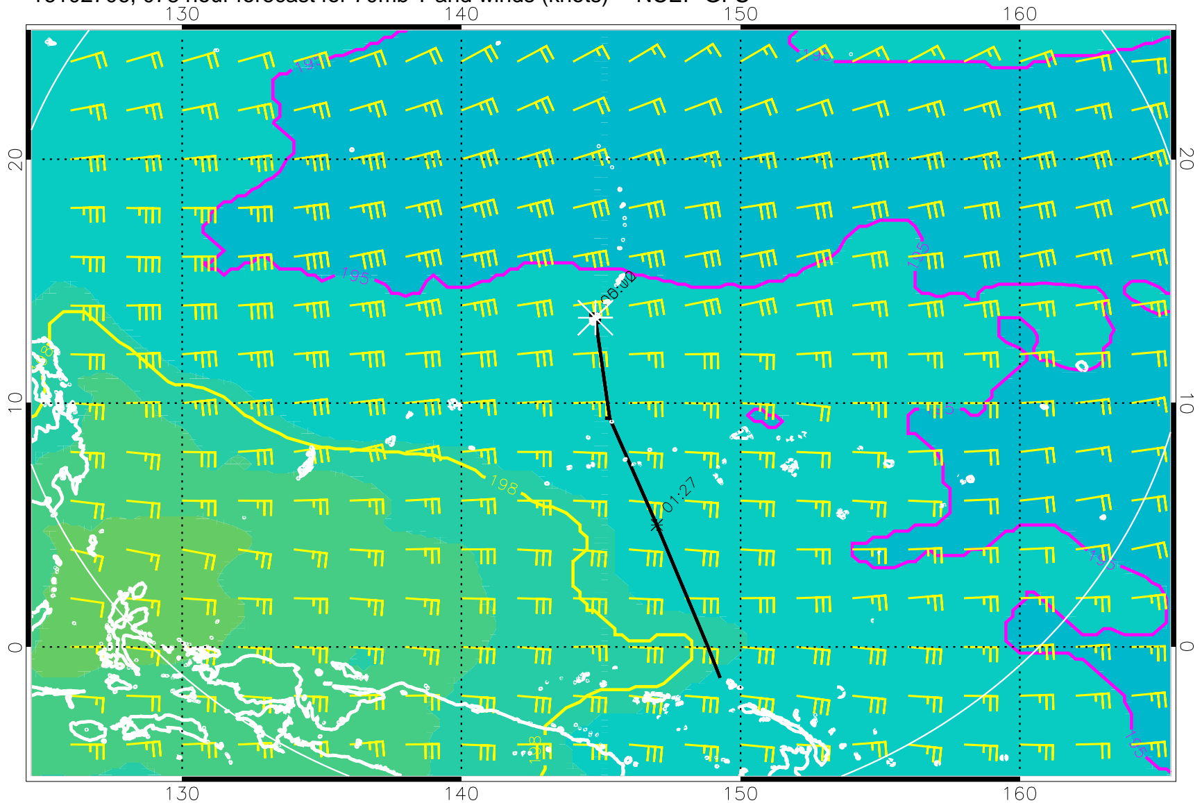
16102706, 078 hour forecast for 70mb T and winds (knots) -- NCEP GFS
