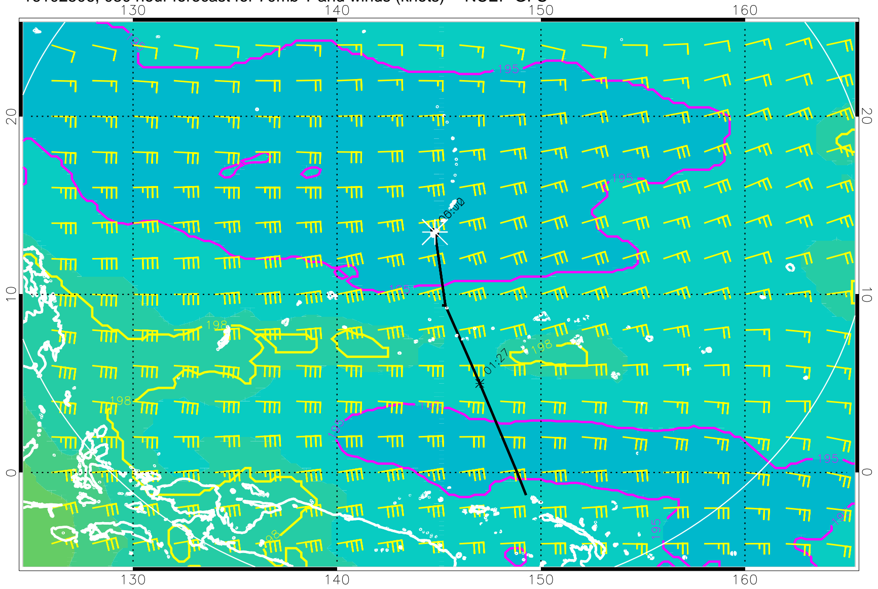
16102506, 030 hour forecast for 70mb T and winds (knots) -- NCEP GFS
