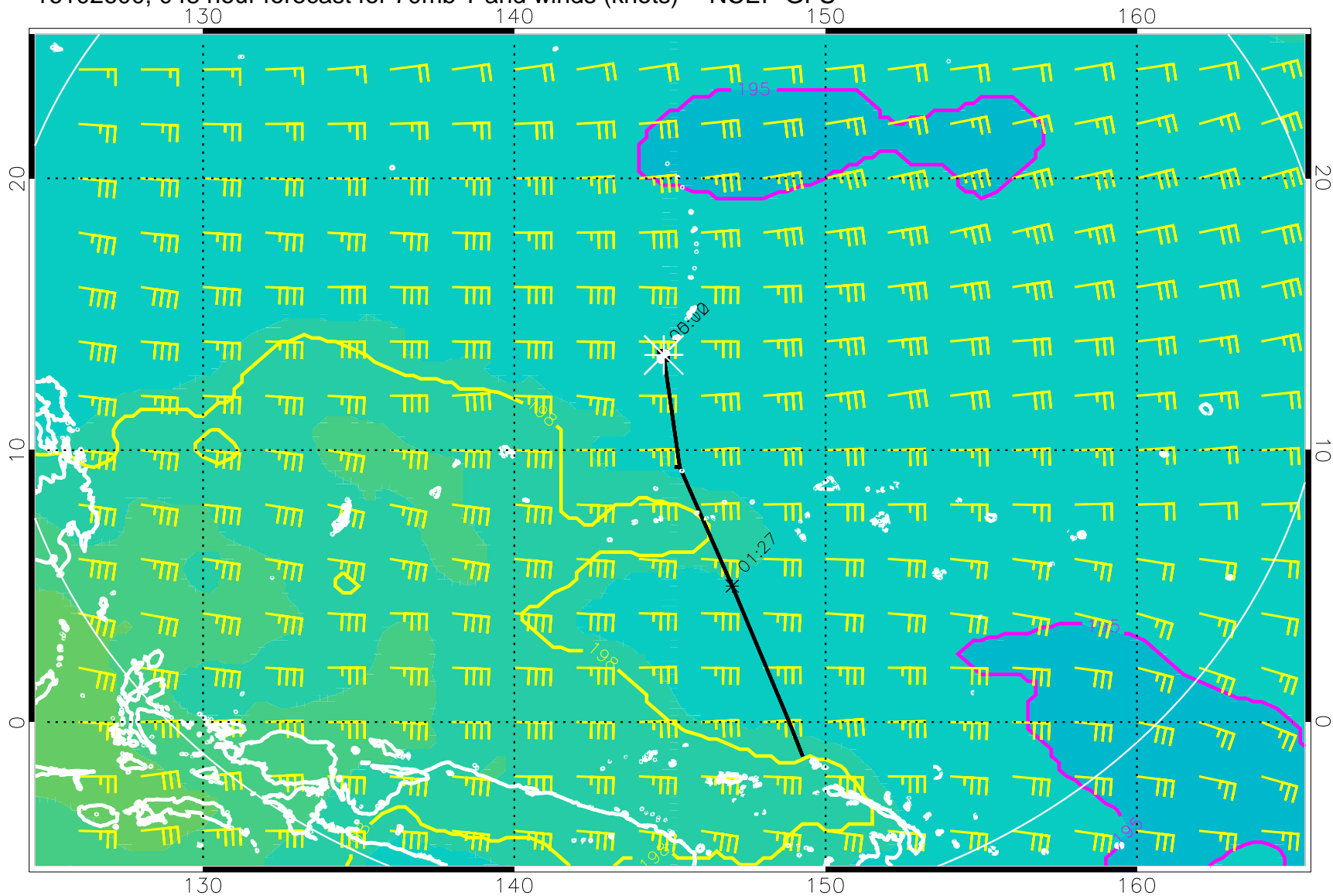
16102600, 048 hour forecast for 70mb T and winds (knots) -- NCEP GFS
