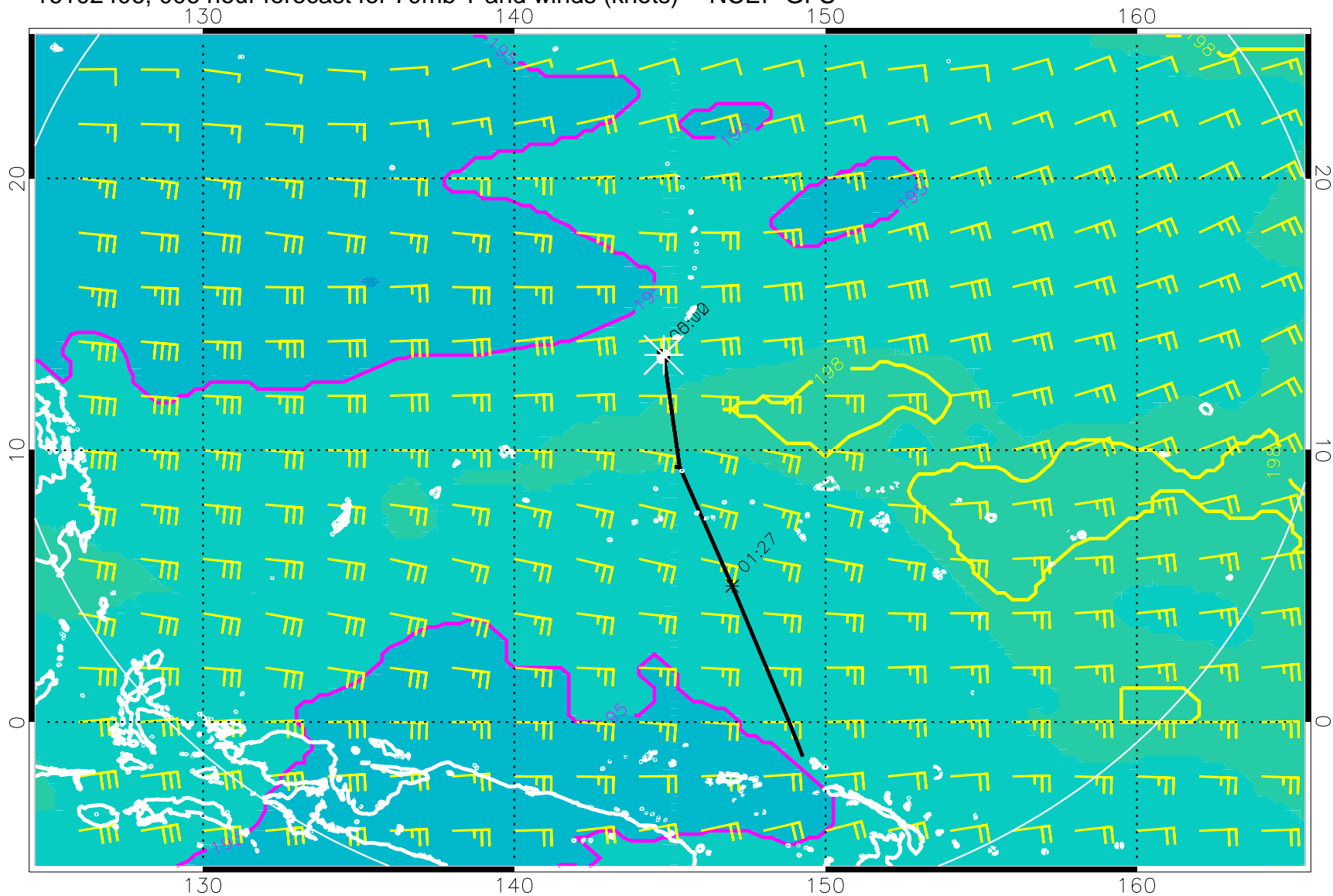
16102406, 006 hour forecast for 70mb T and winds (knots) -- NCEP GFS
