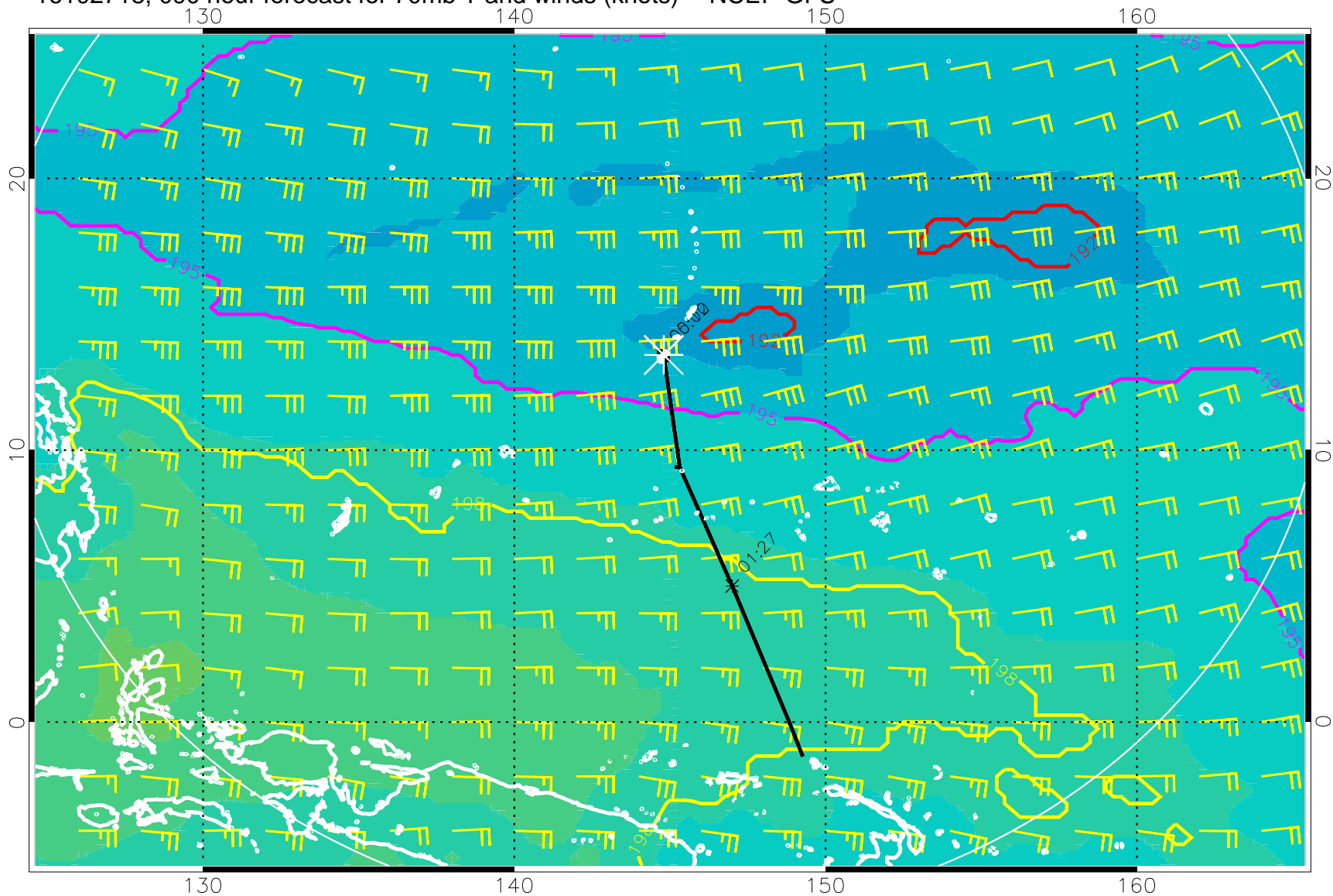
16102718, 090 hour forecast for 70mb T and winds (knots) -- NCEP GFS
