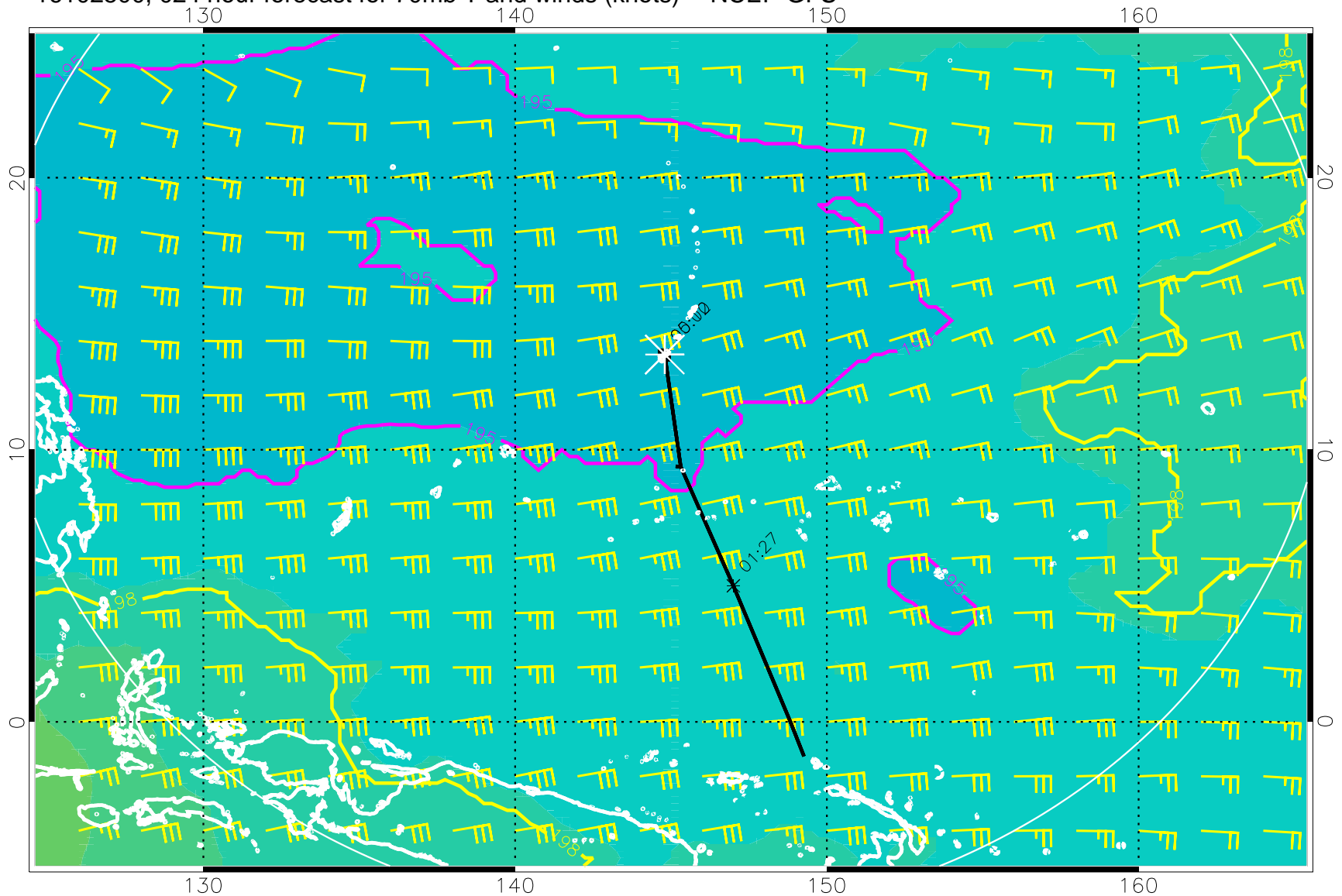
16102500, 024 hour forecast for 70mb T and winds (knots) -- NCEP GFS
