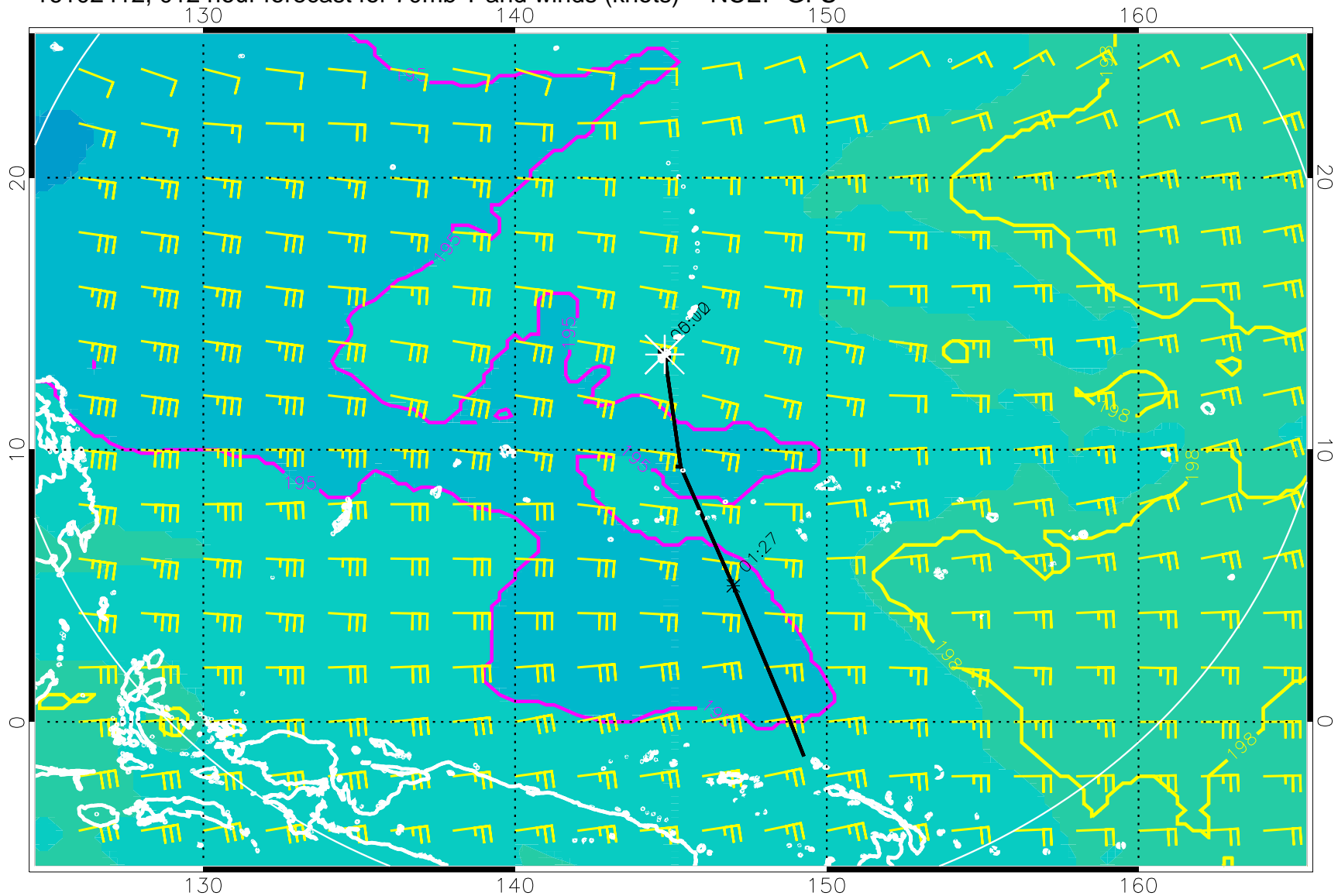
16102412, 012 hour forecast for 70mb T and winds (knots) -- NCEP GFS
