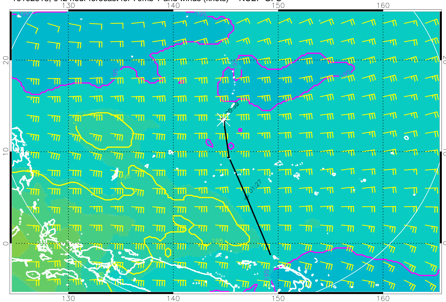
16102518, 042 hour forecast for 70mb T and winds (knots) -- NCEP GFS
