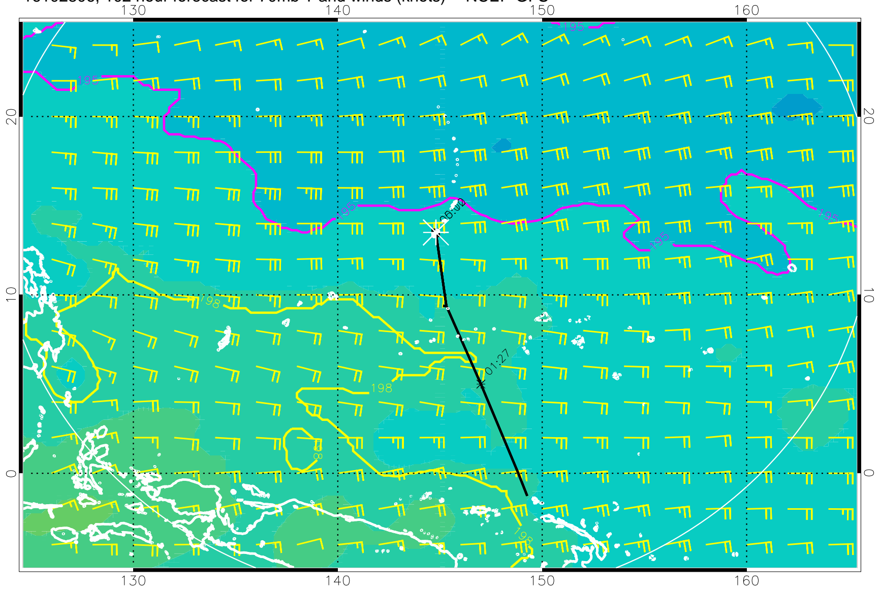
16102806, 102 hour forecast for 70mb T and winds (knots) -- NCEP GFS
