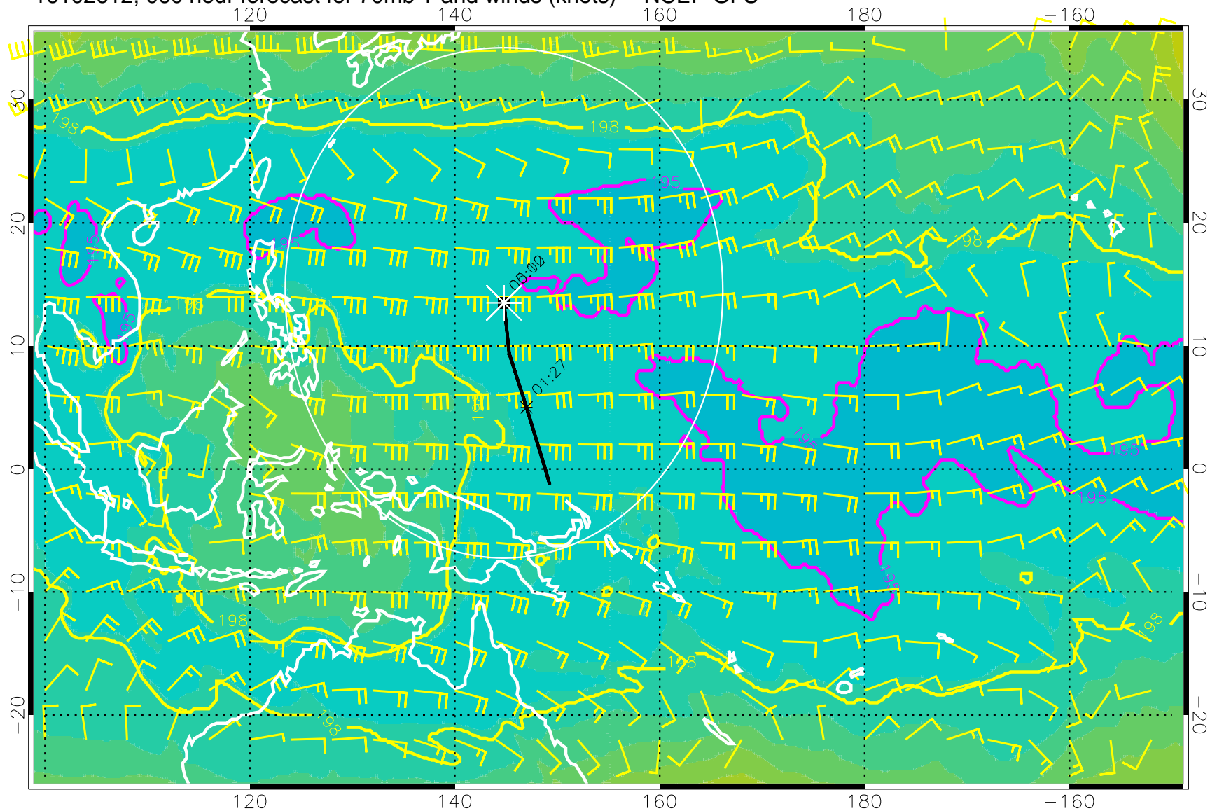
16102612, 060 hour forecast for 70mb T and winds (knots) -- NCEP GFS
