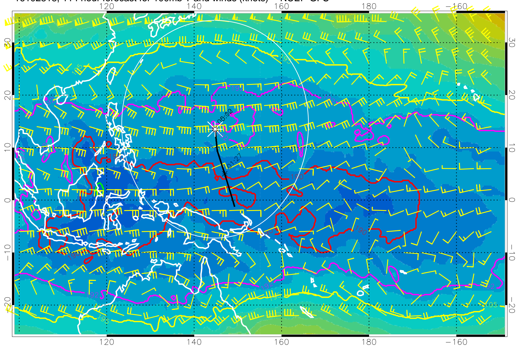
16102818, 114 hour forecast for 100mb T and winds (knots) -- NCEP GFS
