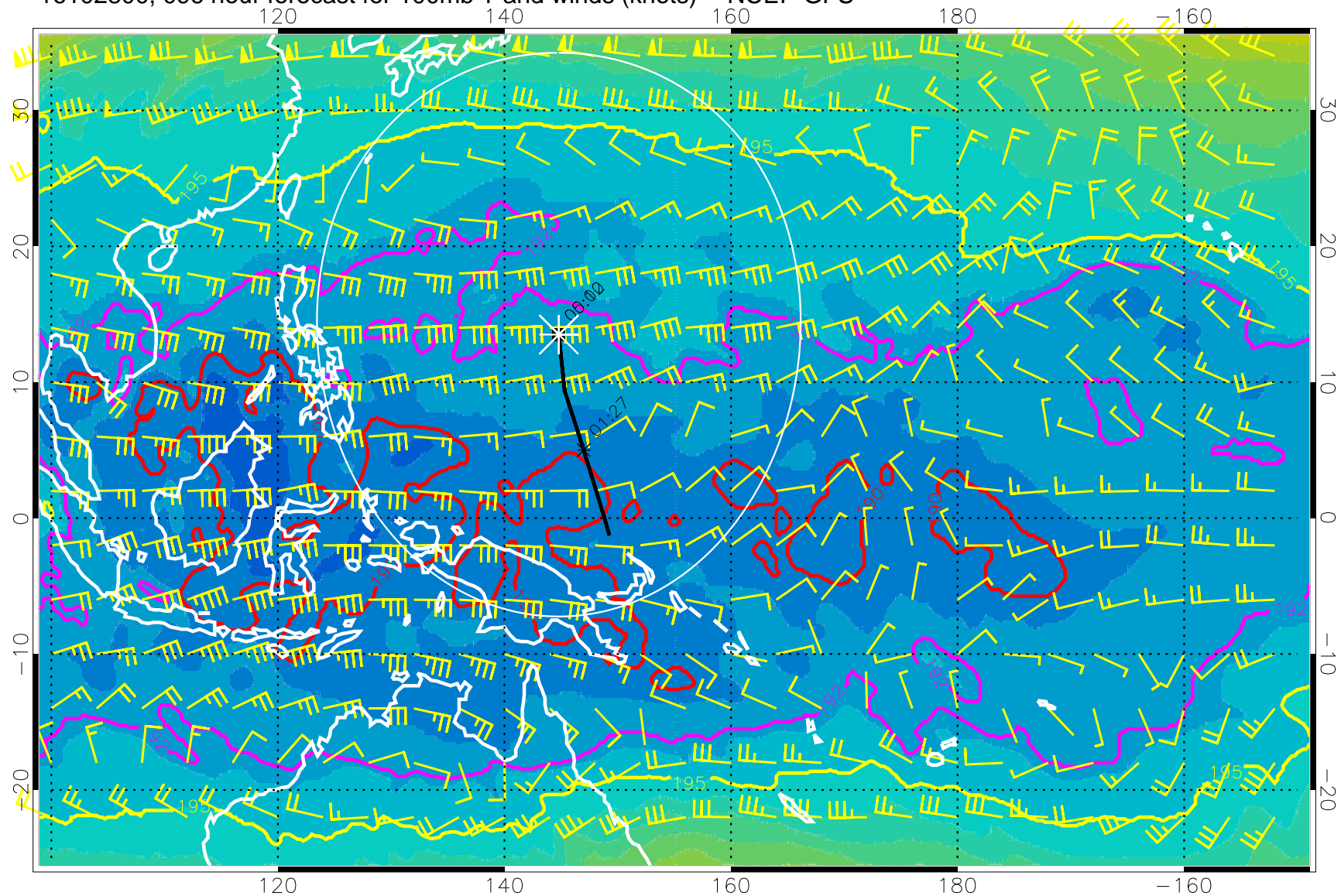
16102800, 096 hour forecast for 100mb T and winds (knots) -- NCEP GFS
