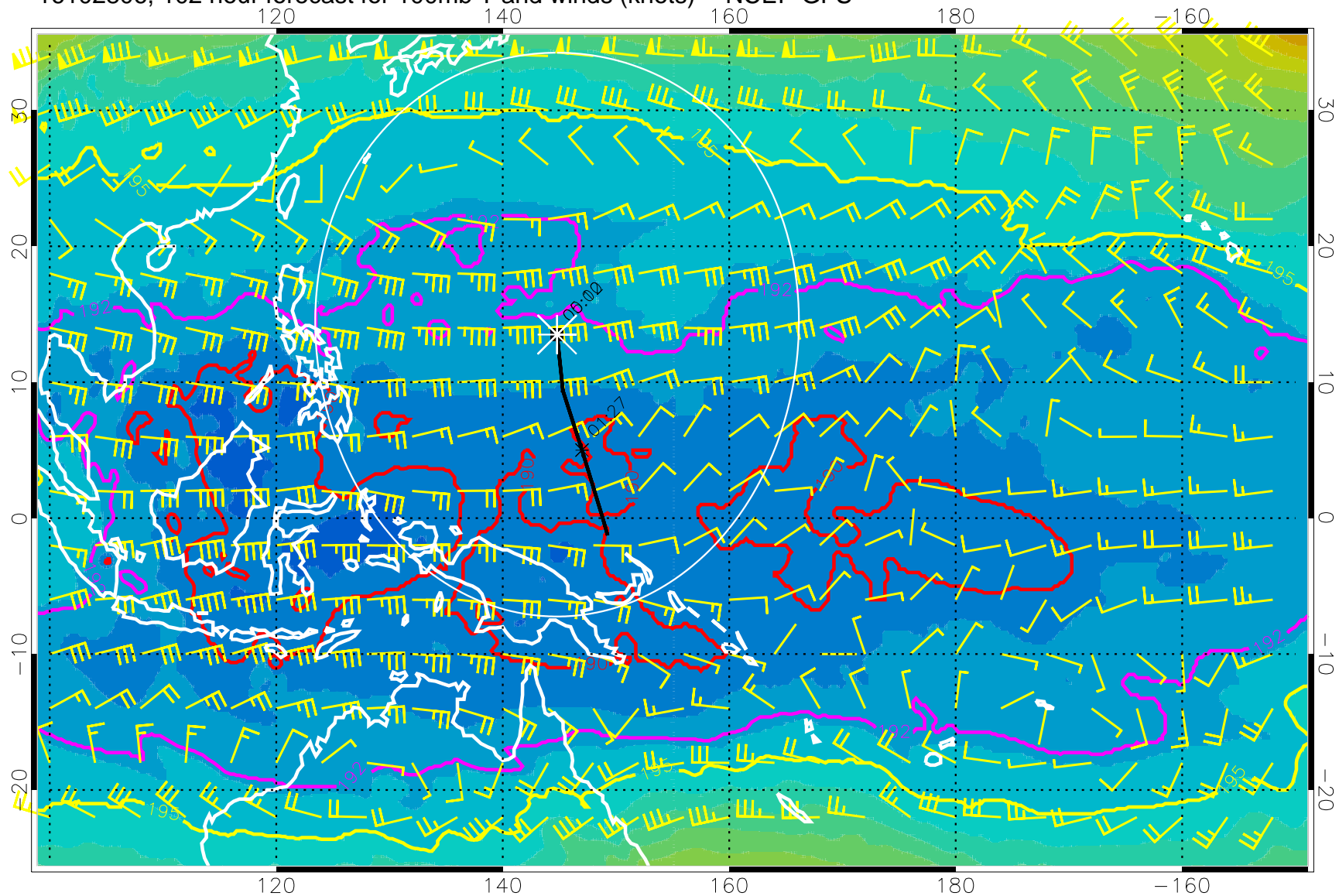
16102806, 102 hour forecast for 100mb T and winds (knots) -- NCEP GFS
