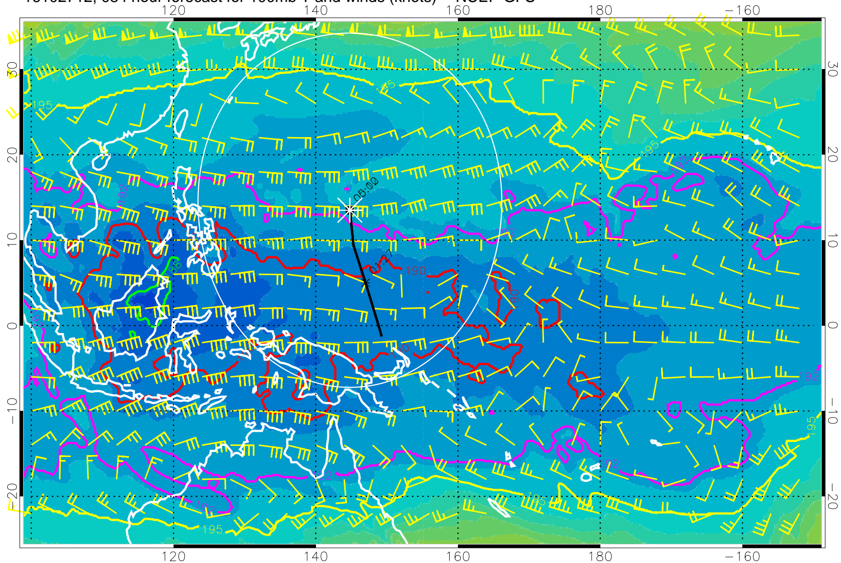
16102712, 084 hour forecast for 100mb T and winds (knots) -- NCEP GFS
