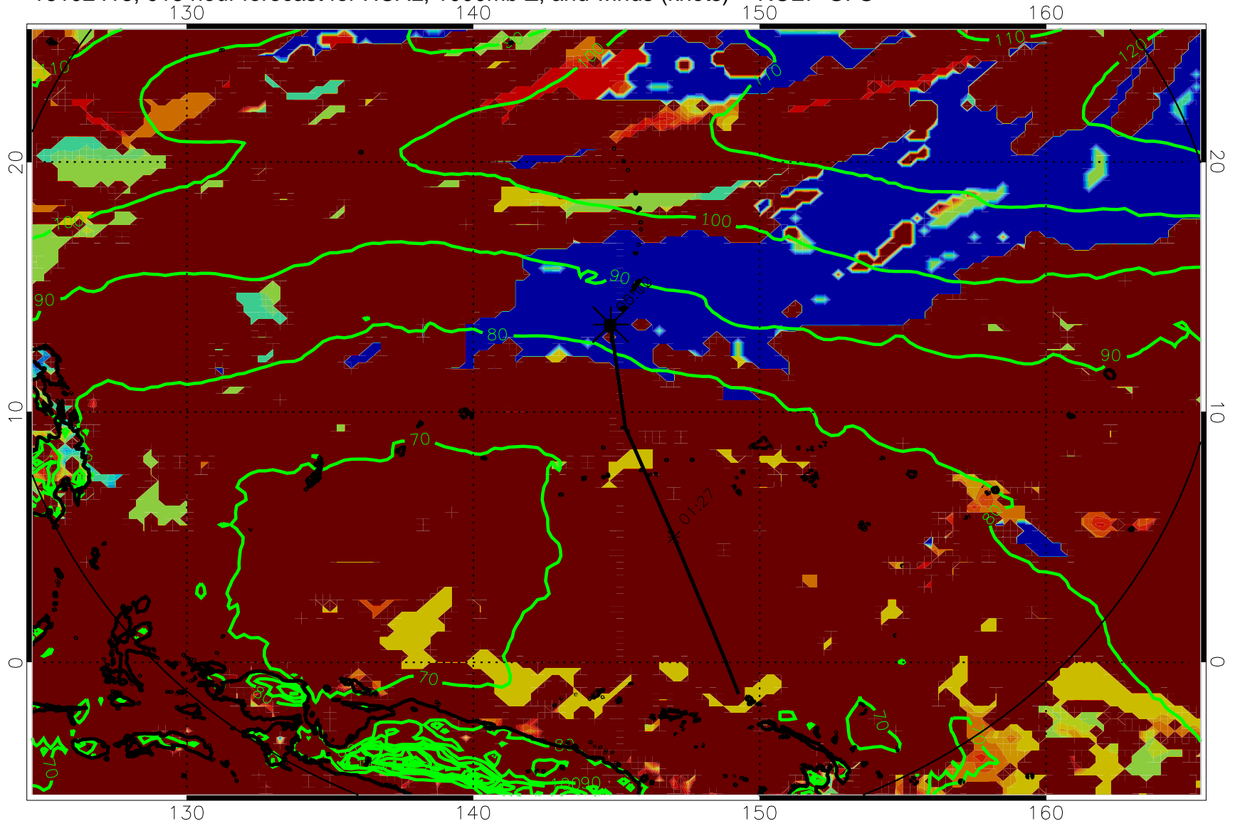
16102418, 018 hour forecast for HCAL, 1000mb Z, and winds (knots) -- NCEP GFS
