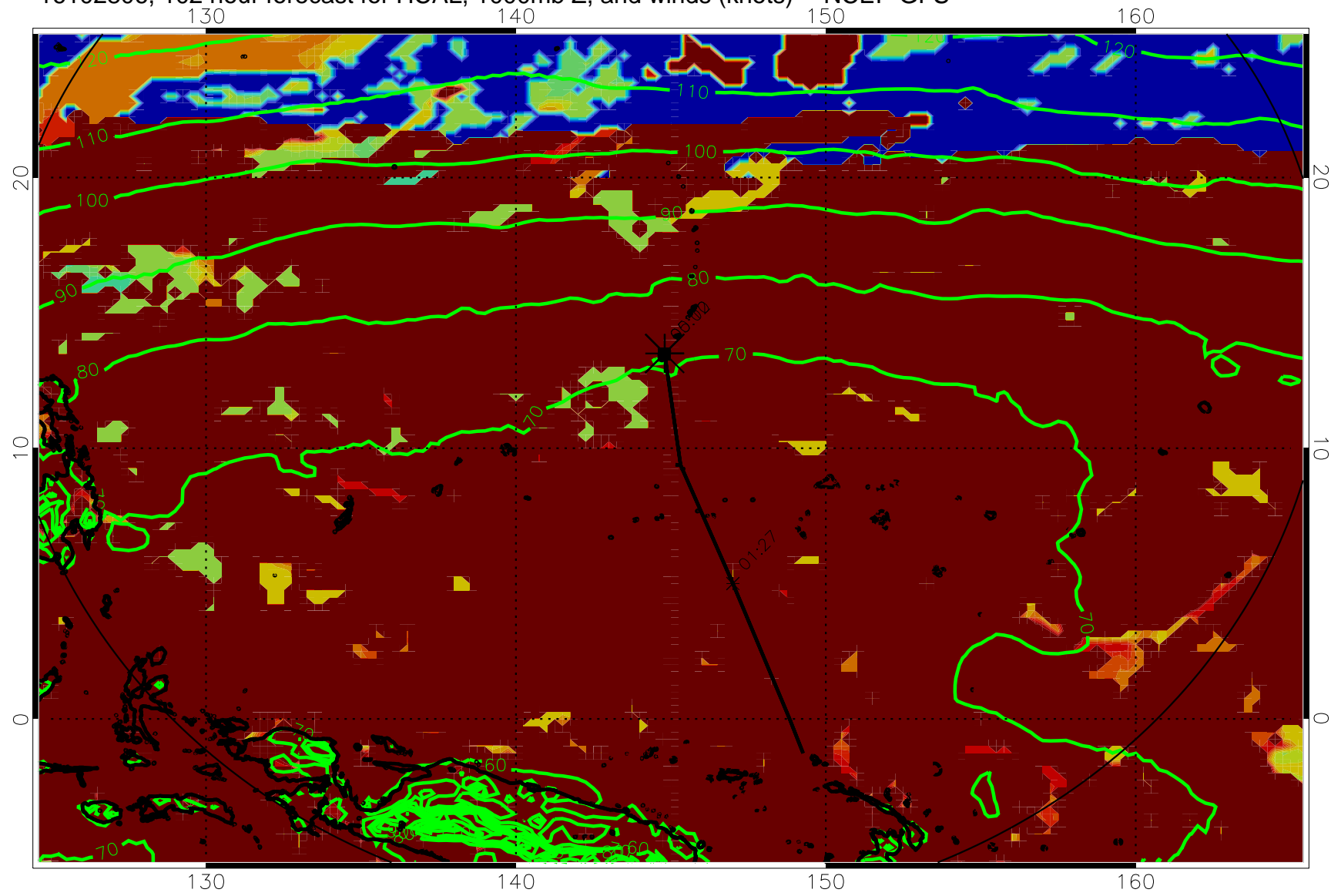
16102806, 102 hour forecast for HCAL, 1000mb Z, and winds (knots) -- NCEP GFS
