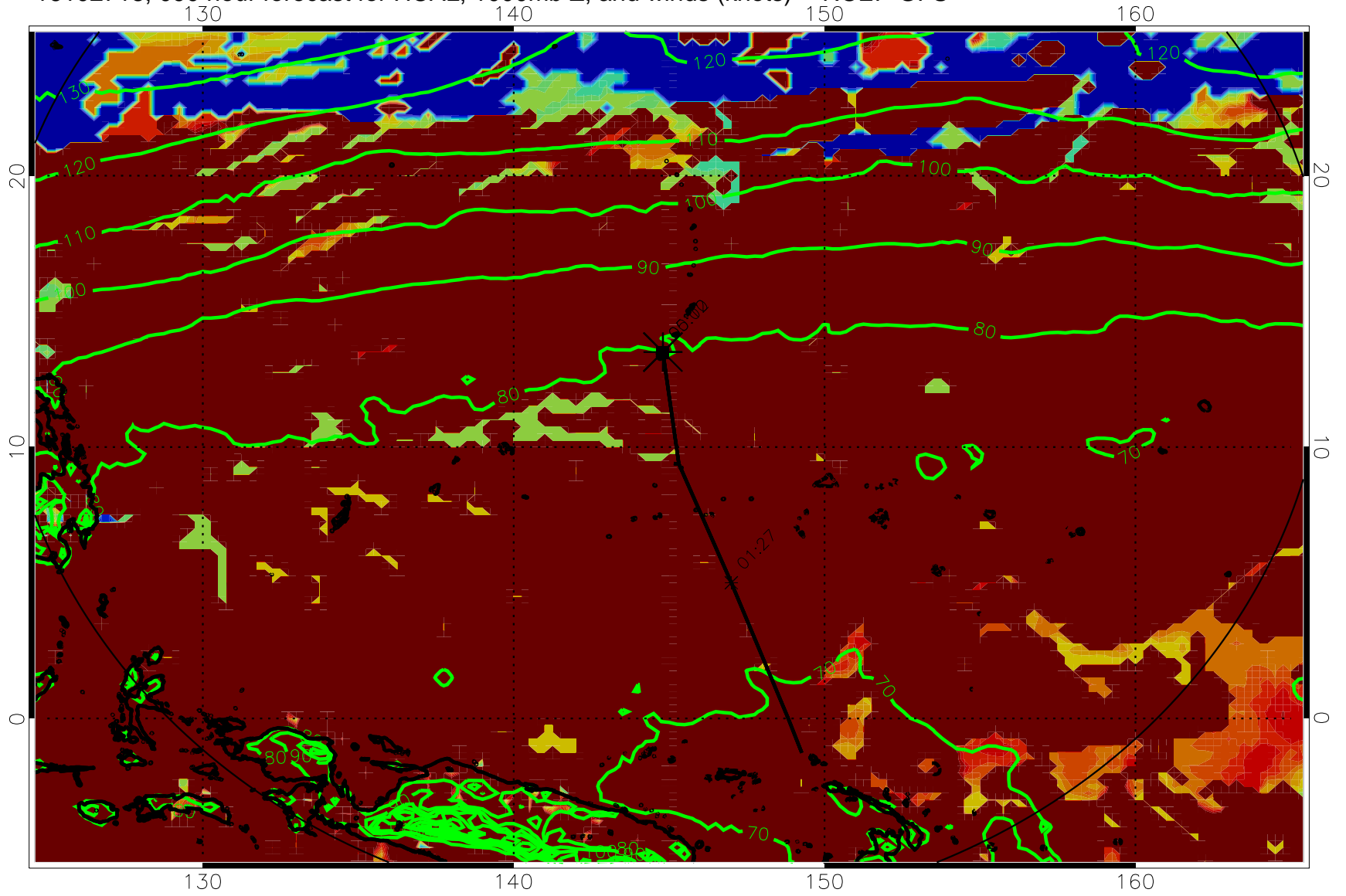
16102718, 090 hour forecast for HCAL, 1000mb Z, and winds (knots) -- NCEP GFS
