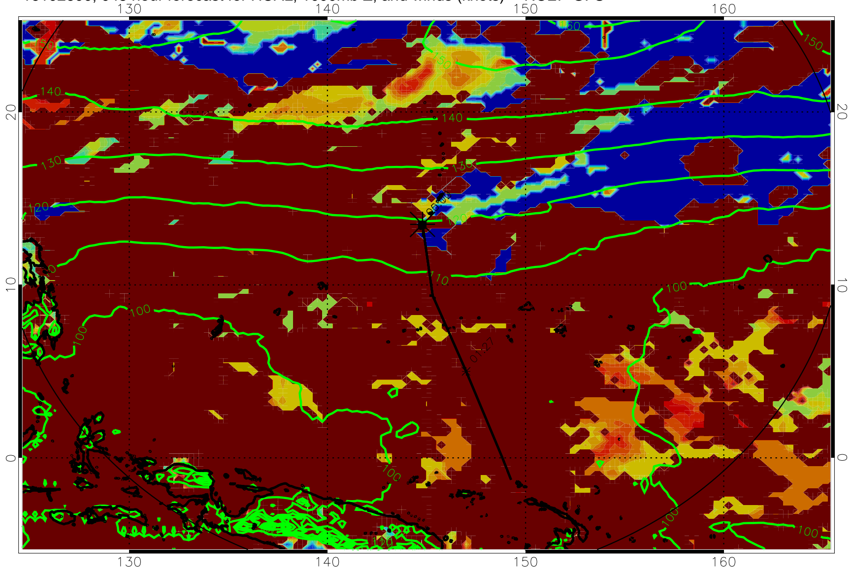
16102600, 048 hour forecast for HCAL, 1000mb Z, and winds (knots) -- NCEP GFS
