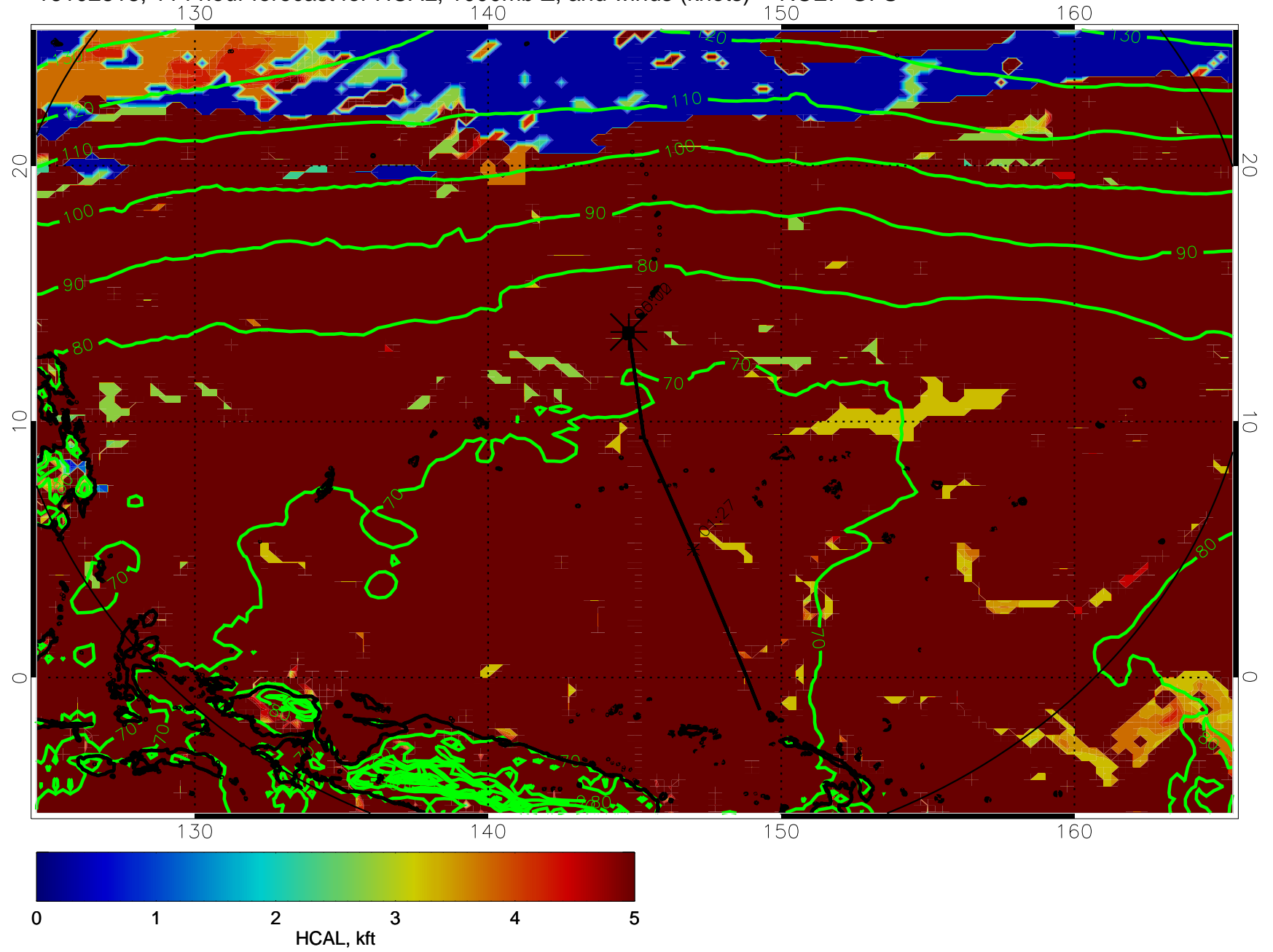
16102818, 114 hour forecast for HCAL, 1000mb Z, and winds (knots) -- NCEP GFS
