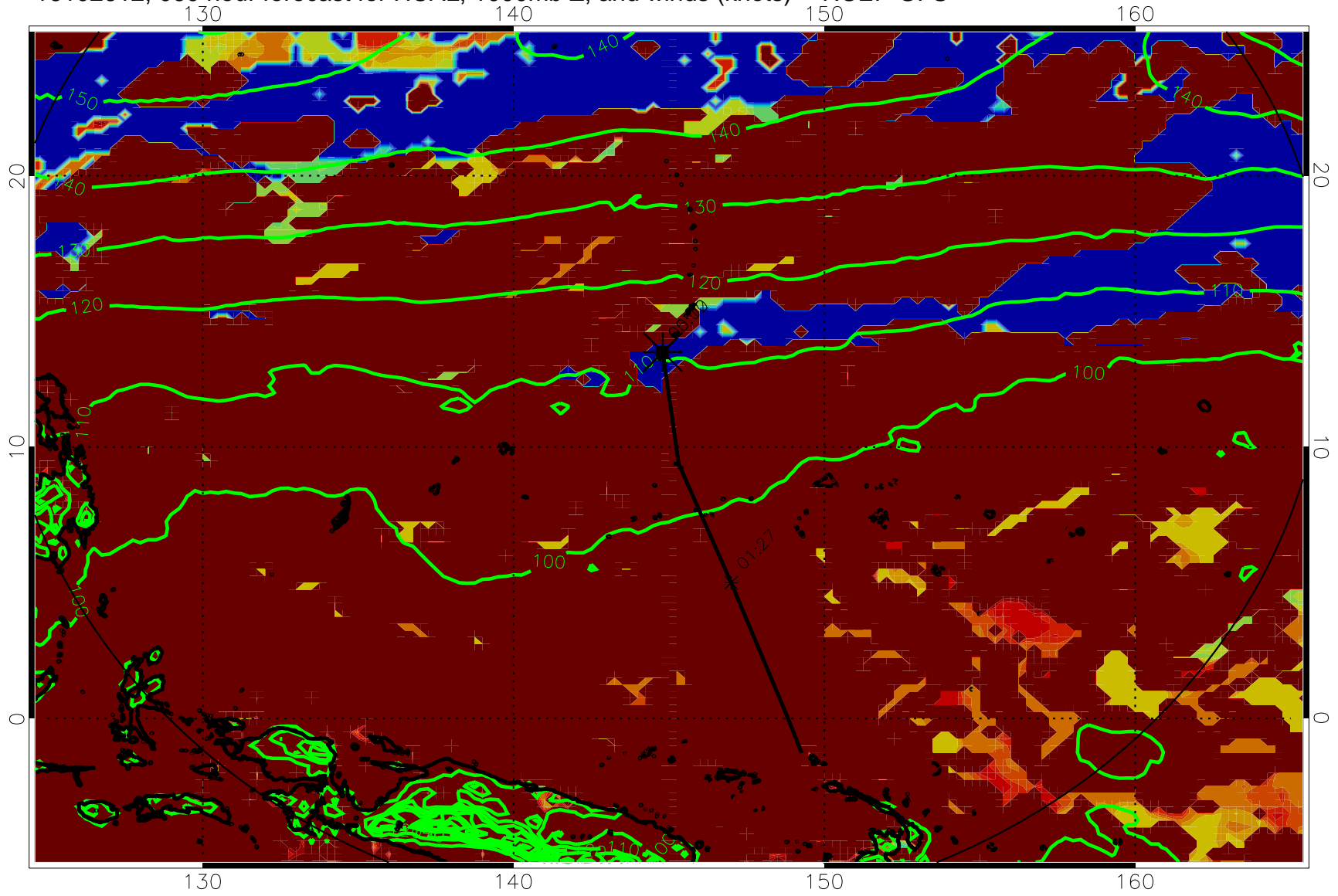
16102612, 060 hour forecast for HCAL, 1000mb Z, and winds (knots) -- NCEP GFS
