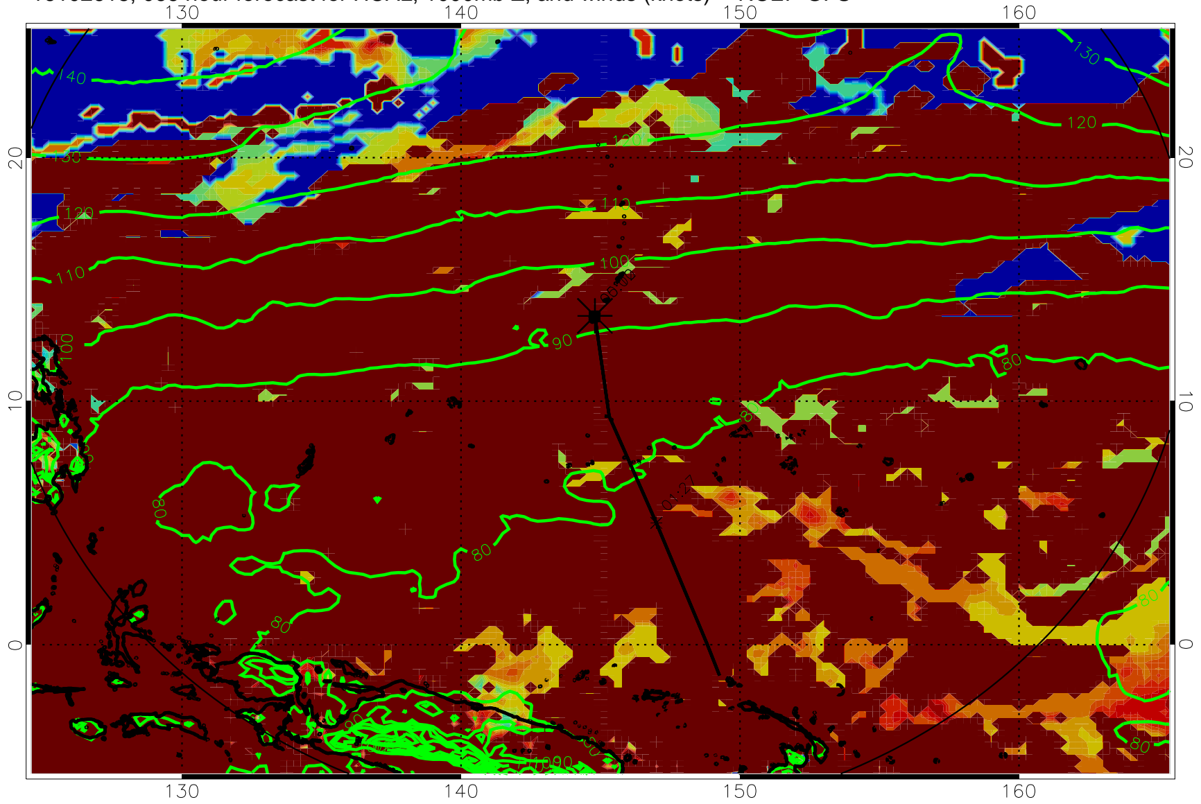
16102618, 066 hour forecast for HCAL, 1000mb Z, and winds (knots) -- NCEP GFS
