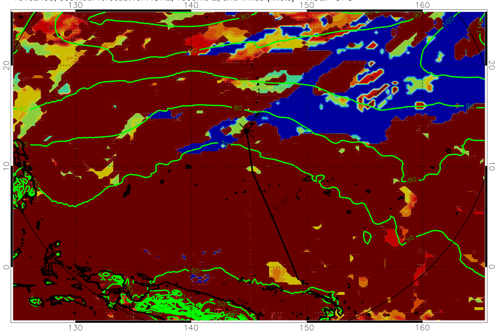
16102406, 006 hour forecast for HCAL, 1000mb Z, and winds (knots) -- NCEP GFS
