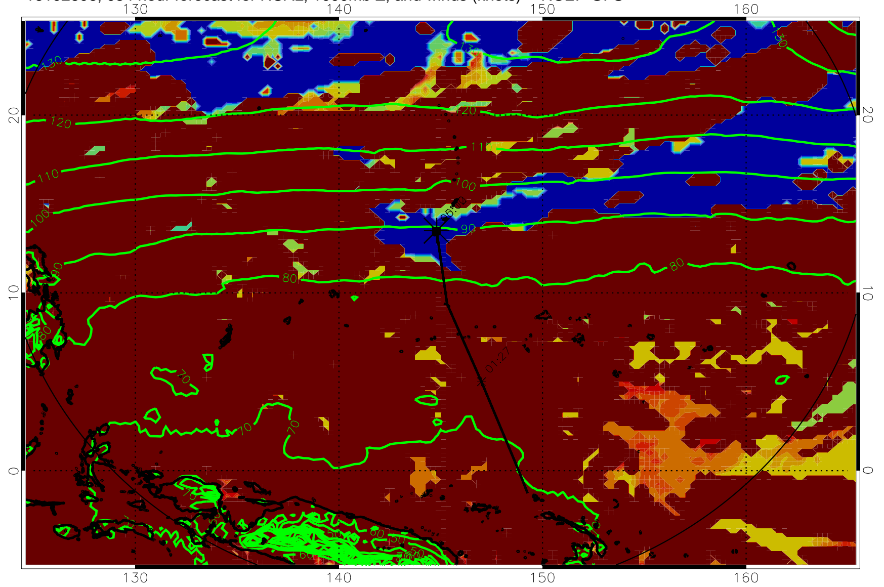
16102606, 054 hour forecast for HCAL, 1000mb Z, and winds (knots) -- NCEP GFS
