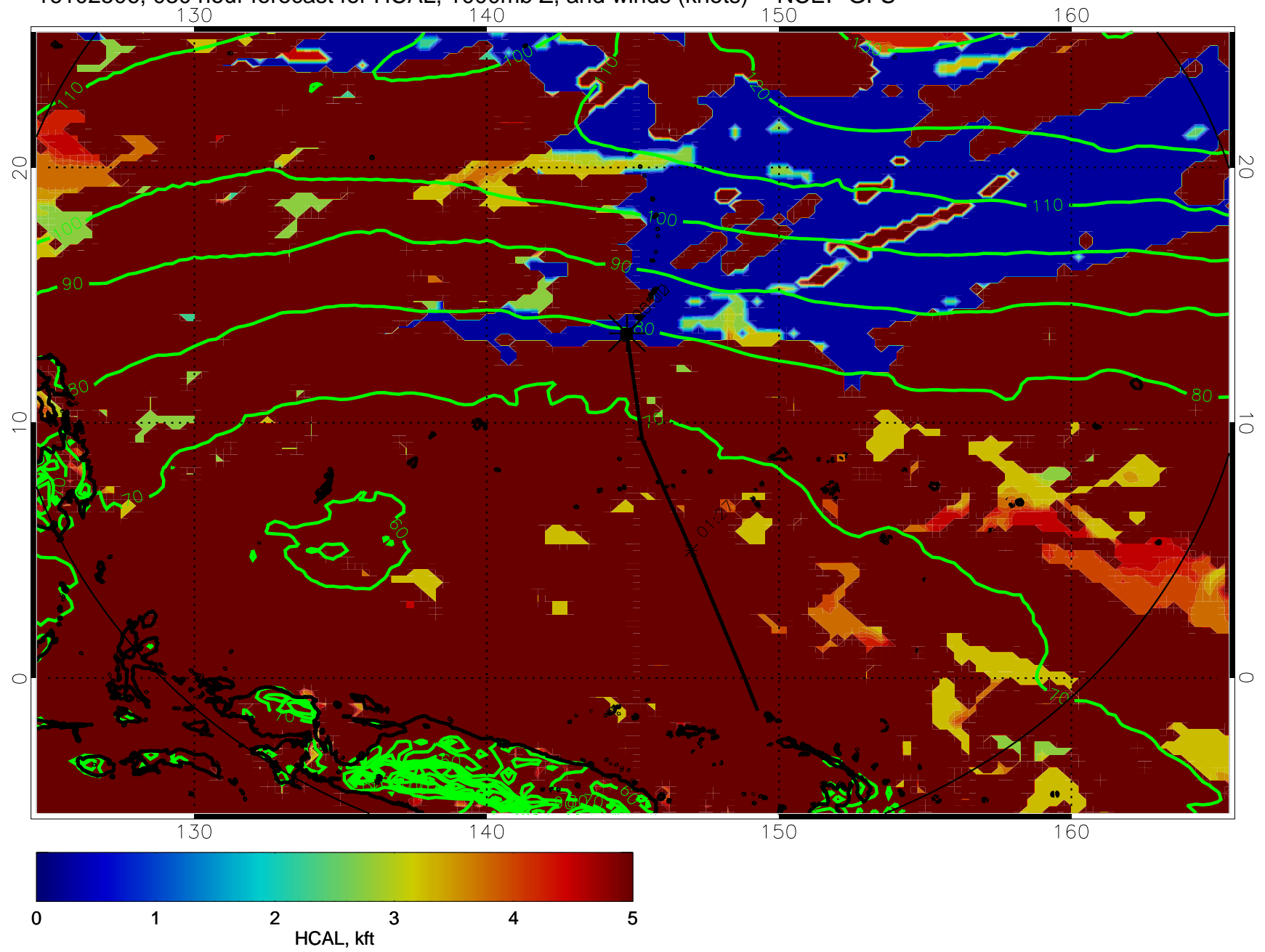
16102506, 030 hour forecast for HCAL, 1000mb Z, and winds (knots) -- NCEP GFS
