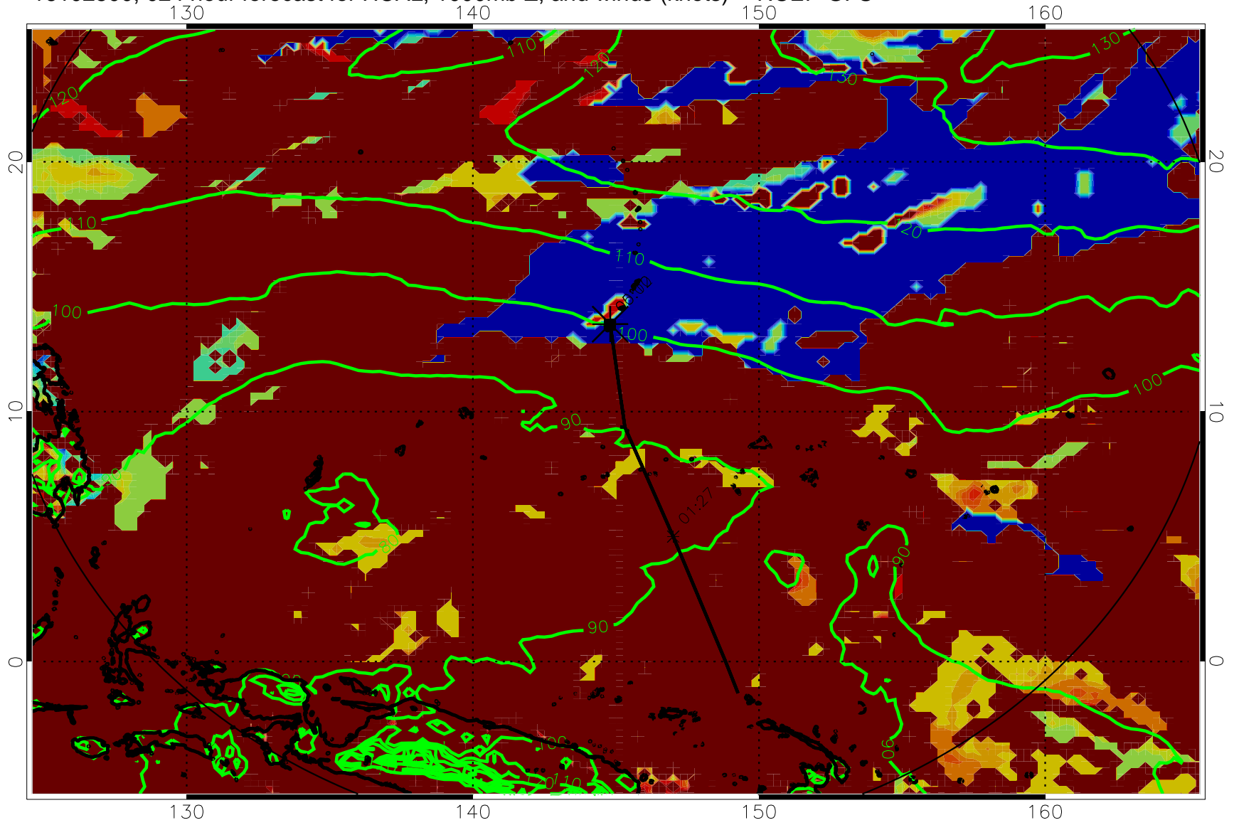
16102500, 024 hour forecast for HCAL, 1000mb Z, and winds (knots) -- NCEP GFS
