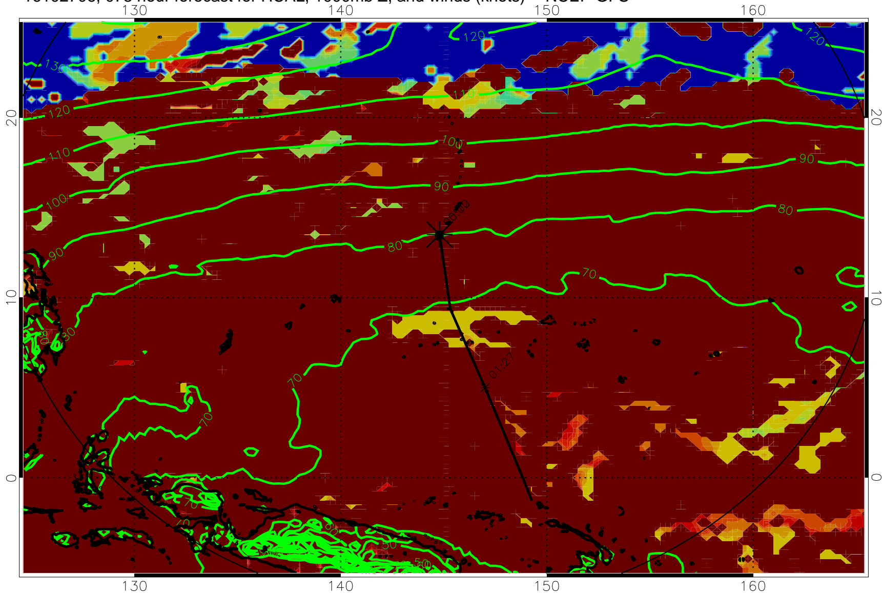
16102706, 078 hour forecast for HCAL, 1000mb Z, and winds (knots) -- NCEP GFS
