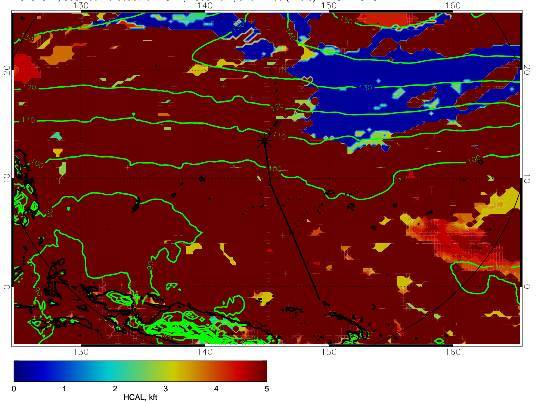
16102512, 036 hour forecast for HCAL, 1000mb Z, and winds (knots) -- NCEP GFS
