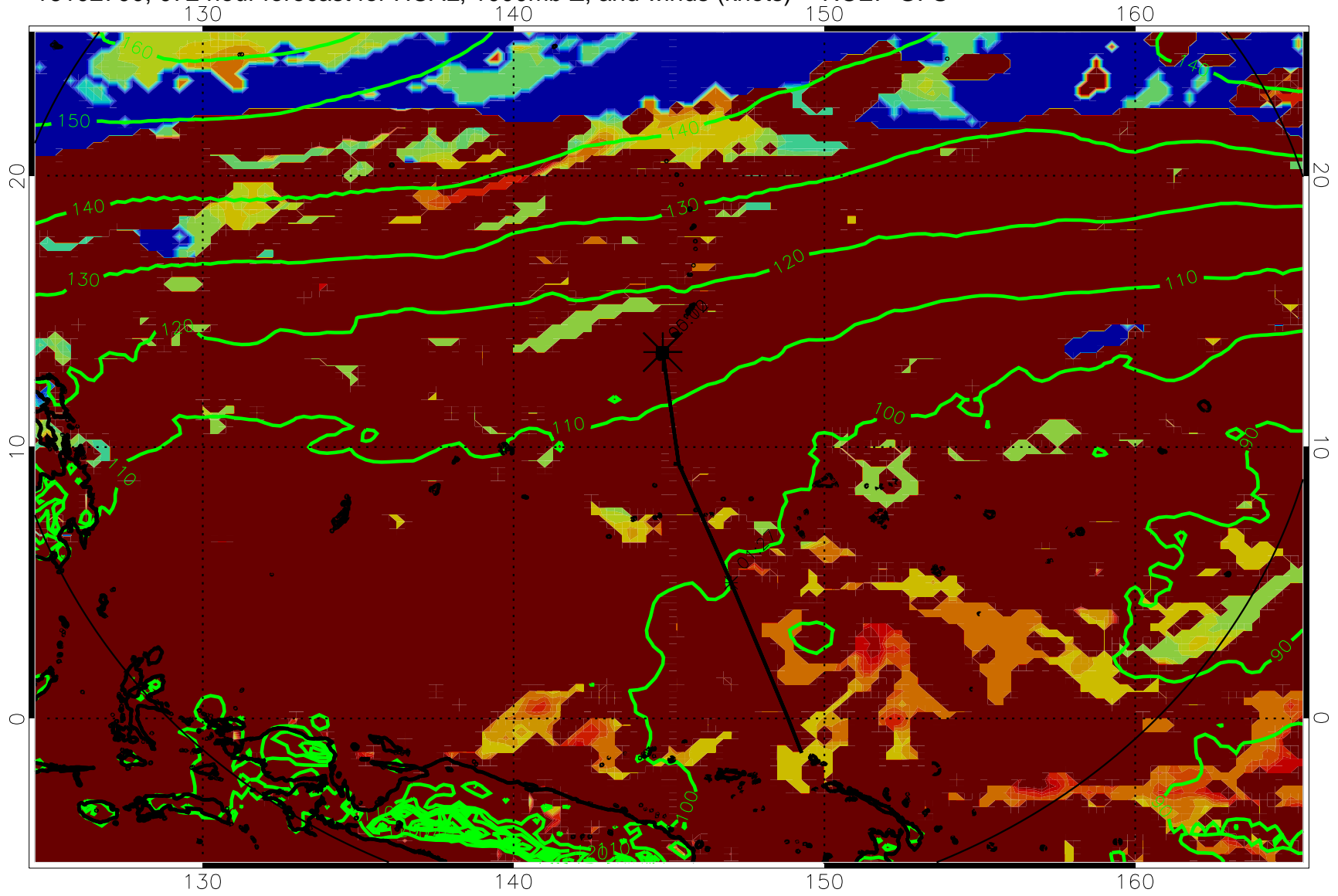
16102700, 072 hour forecast for HCAL, 1000mb Z, and winds (knots) -- NCEP GFS
