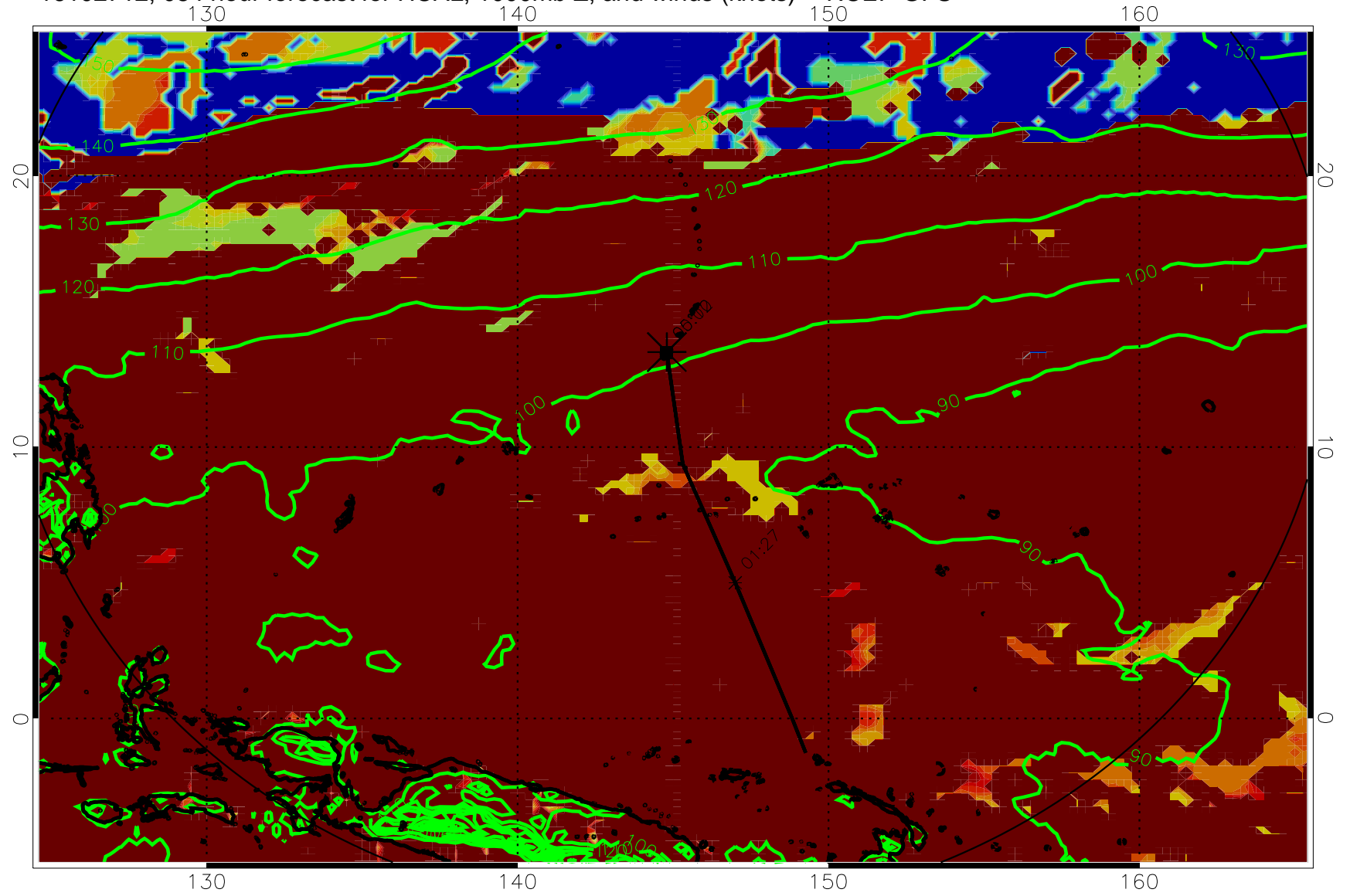
16102712, 084 hour forecast for HCAL, 1000mb Z, and winds (knots) -- NCEP GFS
