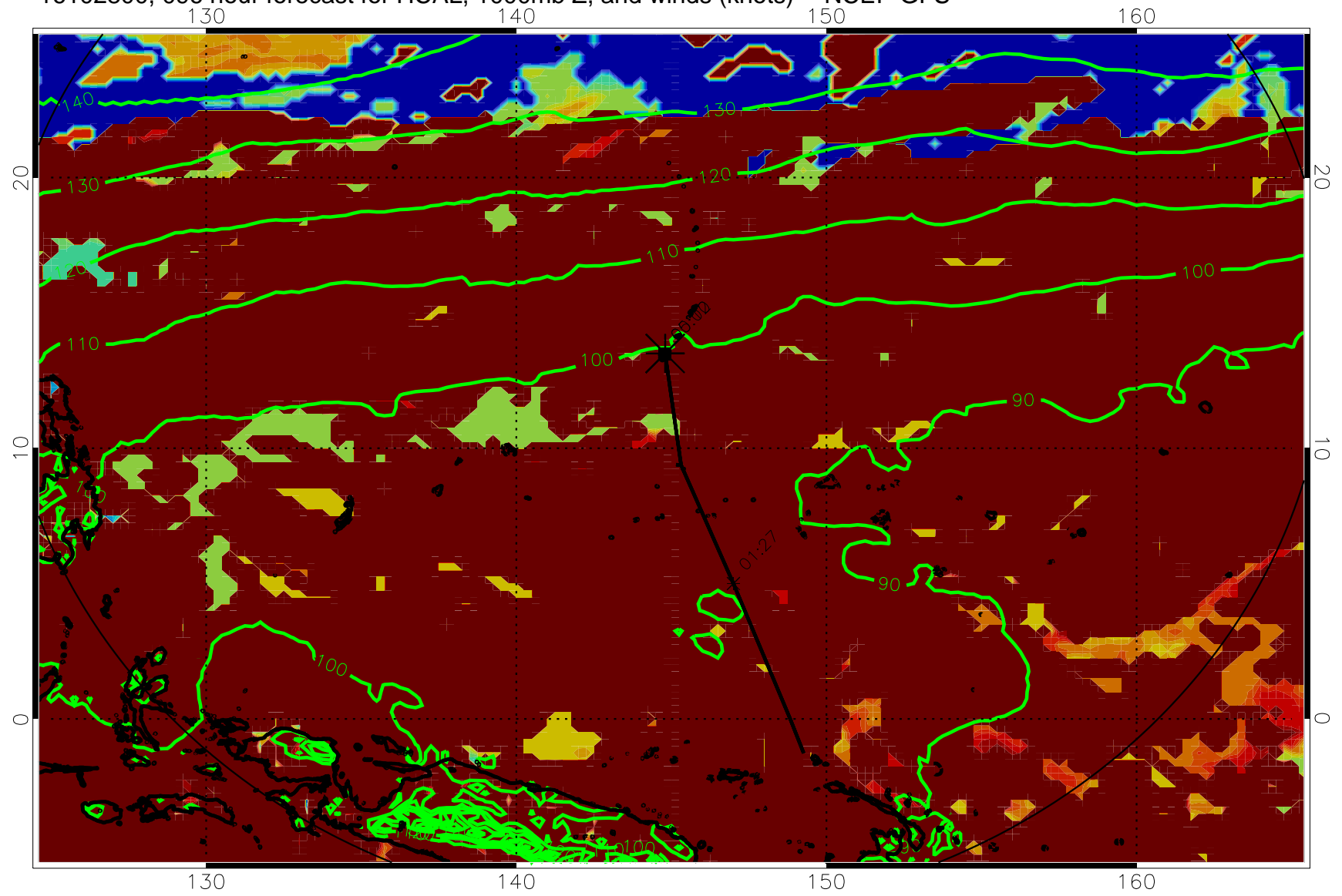
16102800, 096 hour forecast for HCAL, 1000mb Z, and winds (knots) -- NCEP GFS
