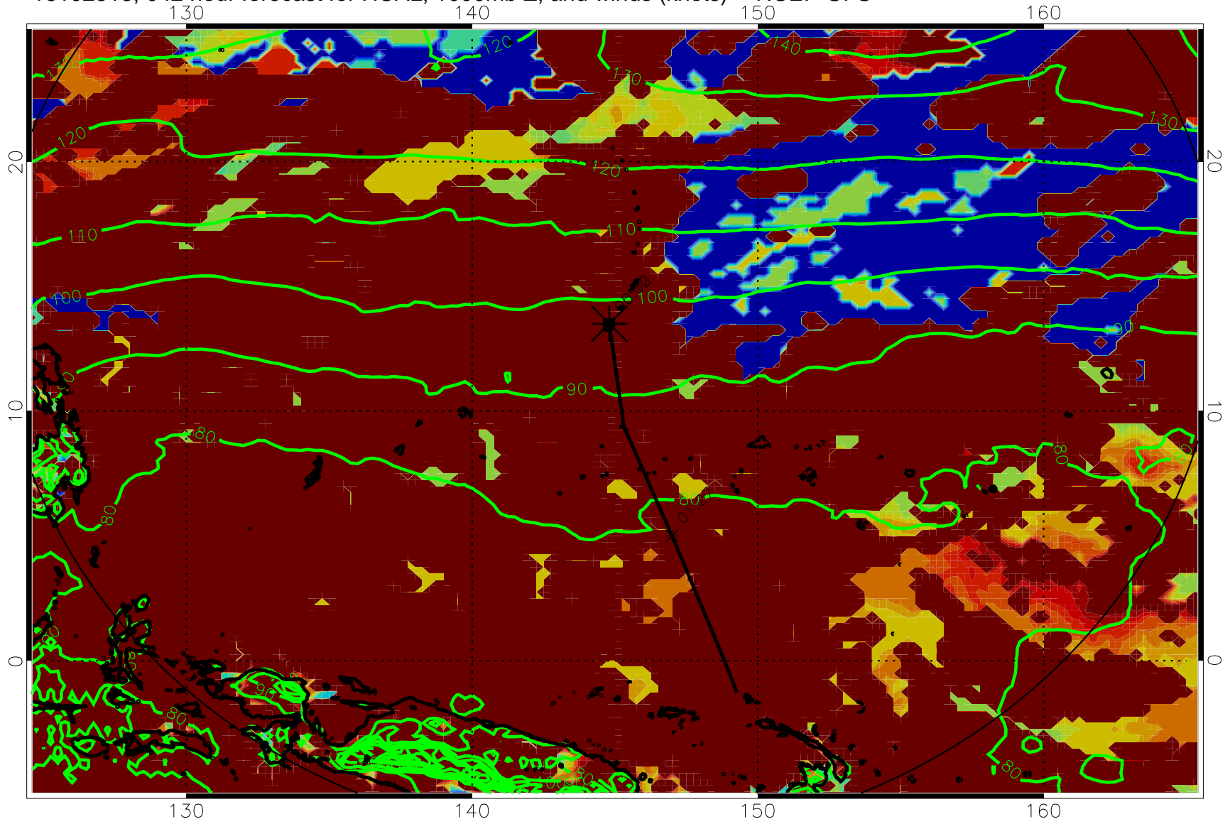
16102518, 042 hour forecast for HCAL, 1000mb Z, and winds (knots) -- NCEP GFS
