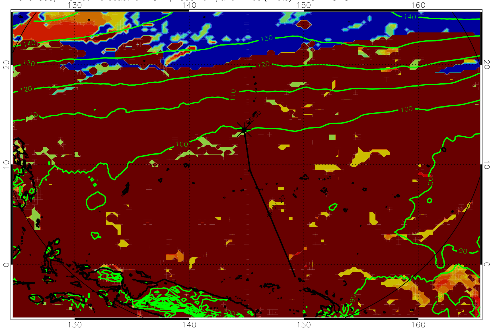
16102900, 120 hour forecast for HCAL, 1000mb Z, and winds (knots) -- NCEP GFS
