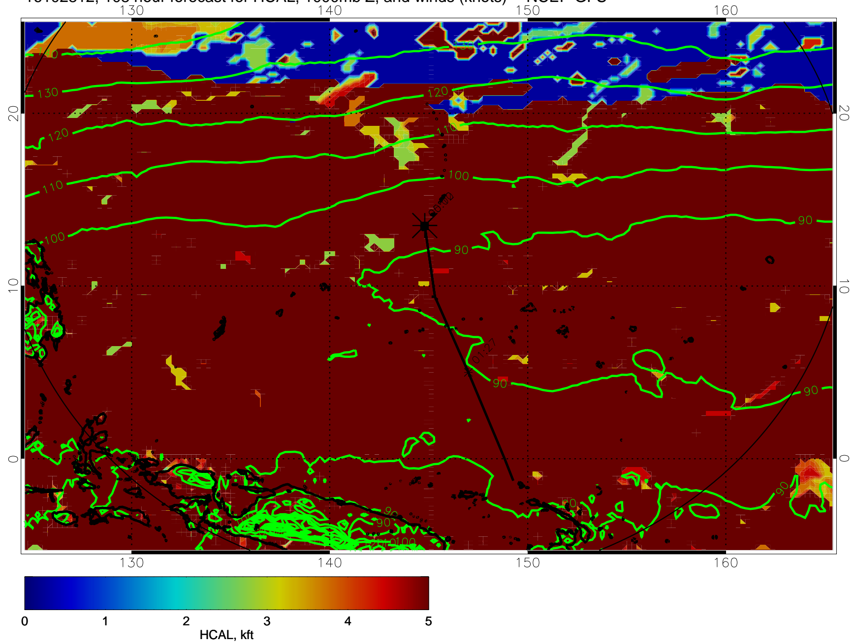
16102812, 108 hour forecast for HCAL, 1000mb Z, and winds (knots) -- NCEP GFS
