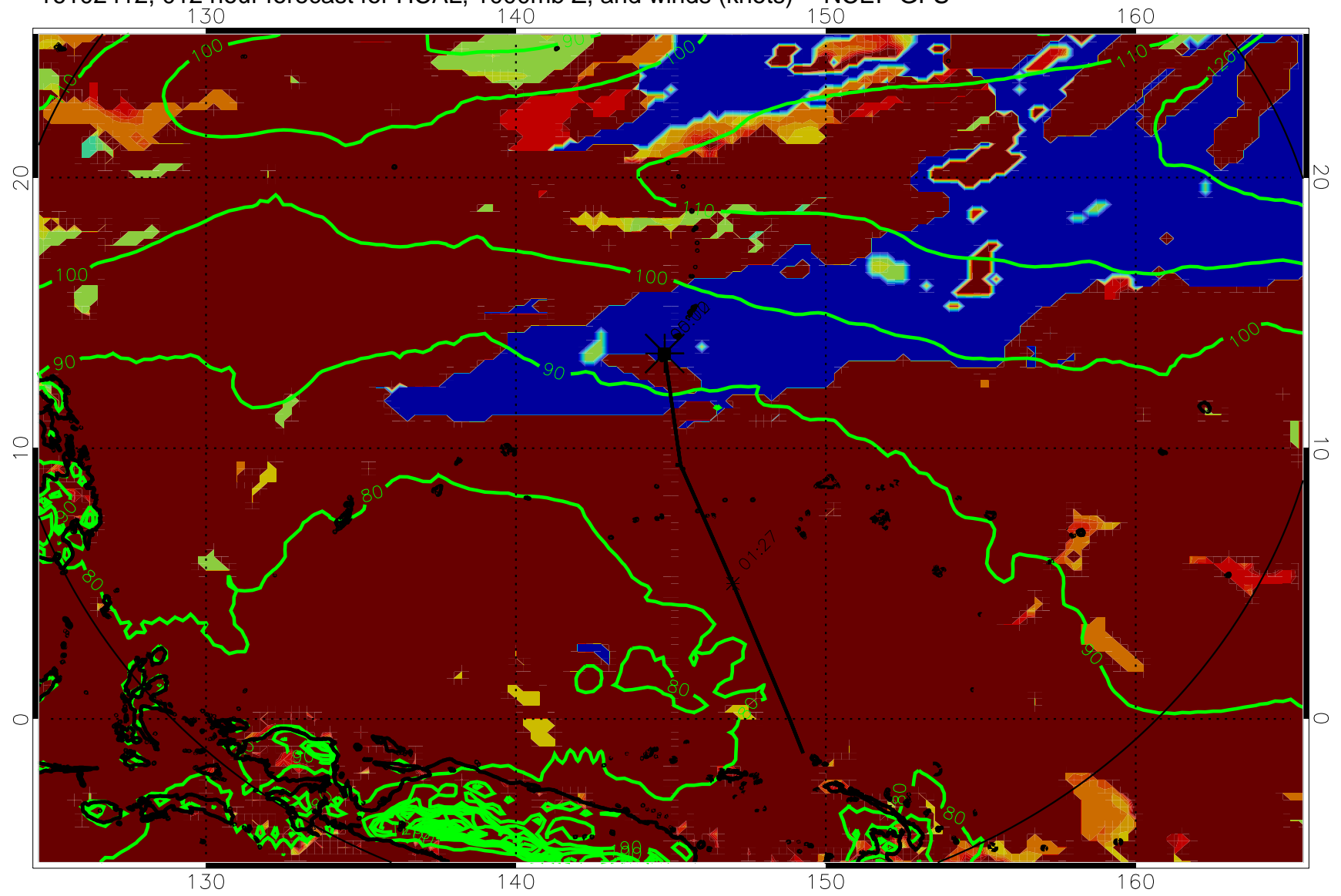
16102412, 012 hour forecast for HCAL, 1000mb Z, and winds (knots) -- NCEP GFS
