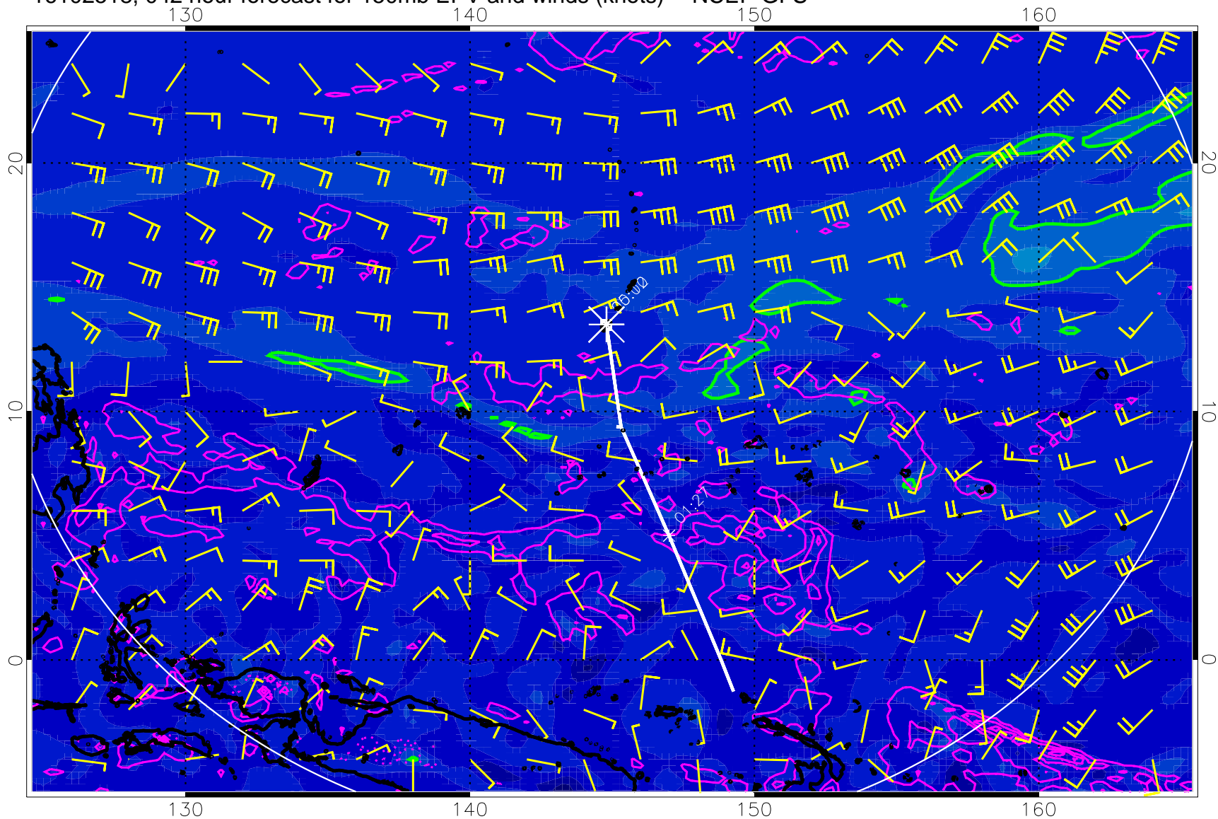
16102518, 042 hour forecast for 150mb EPV and winds (knots) -- NCEP GFS
